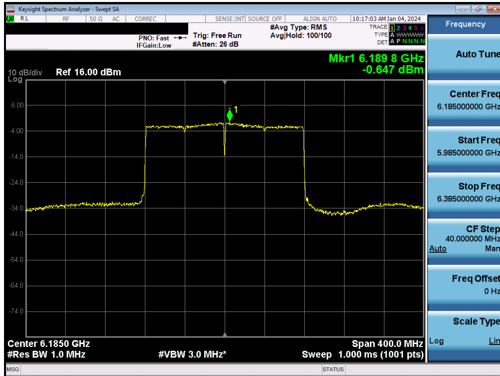
Plot 7-94. Power Spectral Density MIMO ANT2 (160MHz 802.11ax/be (UNII Band 5) – Ch. 47) - SP
