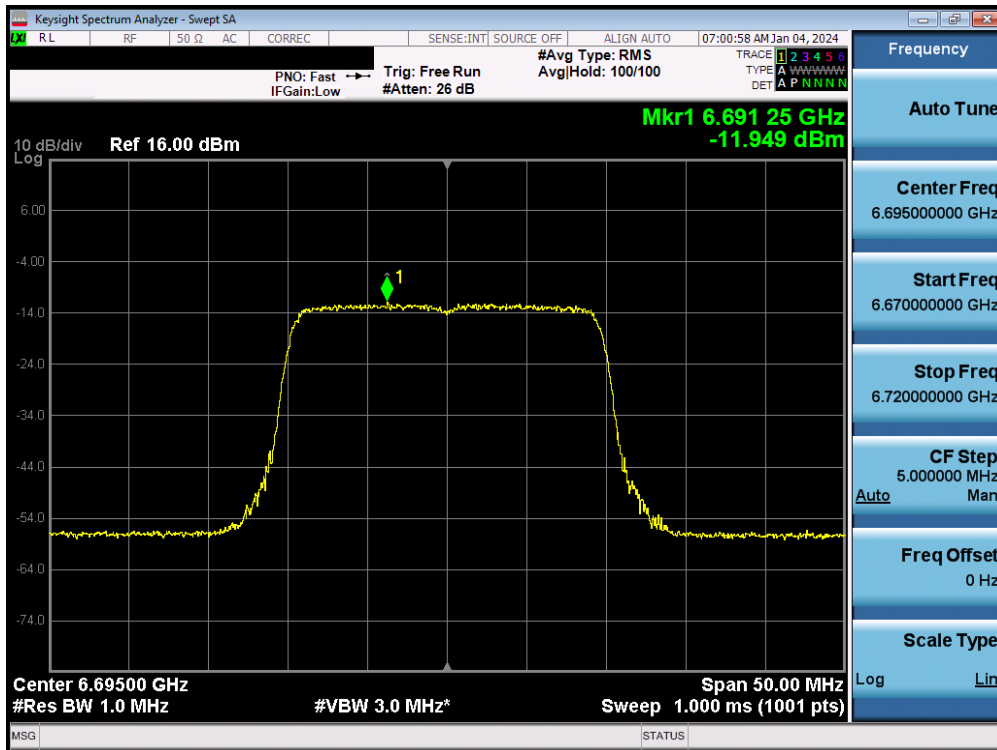
Plot 7-103. Power Spectral Density MIMO ANT2 (20MHz 802.11ax/be (UNII Band 7) – Ch. 149) - LPI
