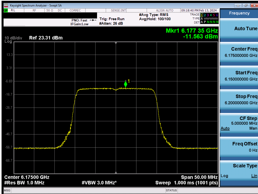
Plot 7-85. Power Spectral Density MIMO ANT2 (20MHz 802.11ax/be (UNII Band 5) – Ch. 45) - LPI
