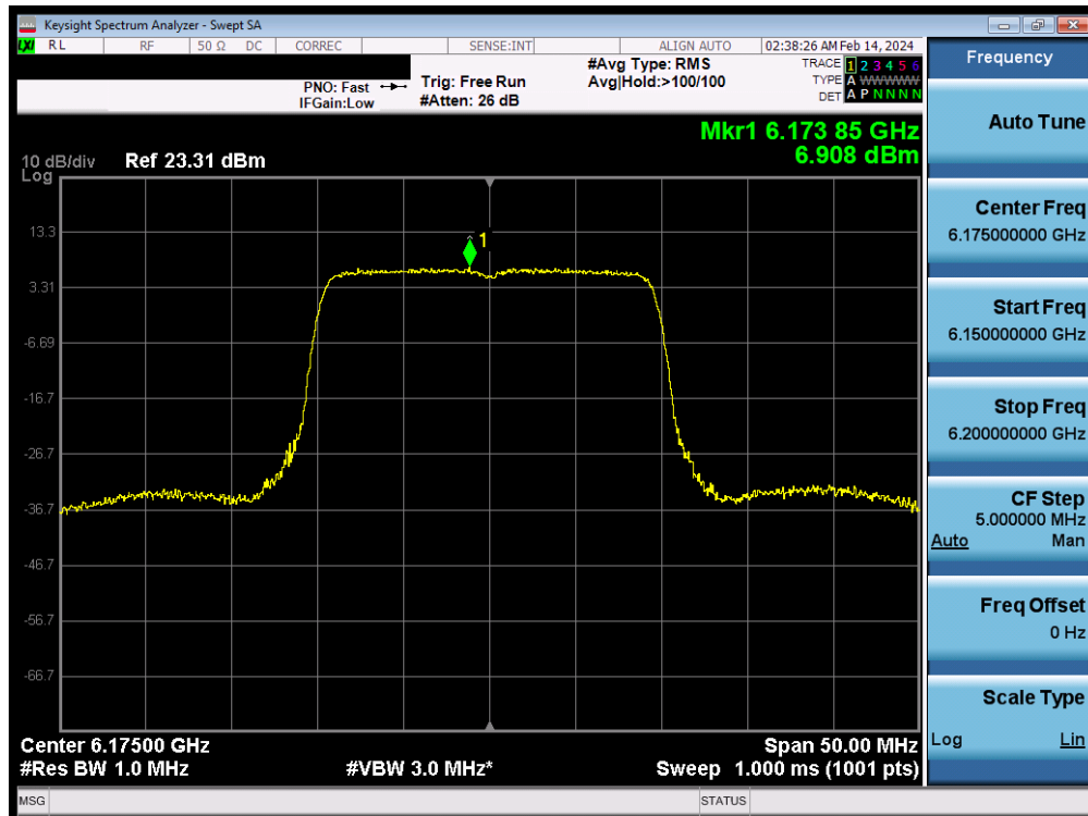
Plot 7-91. Power Spectral Density MIMO ANT2 (20MHz 802.11ax/be (UNII Band 5) – Ch. 45) – SP
