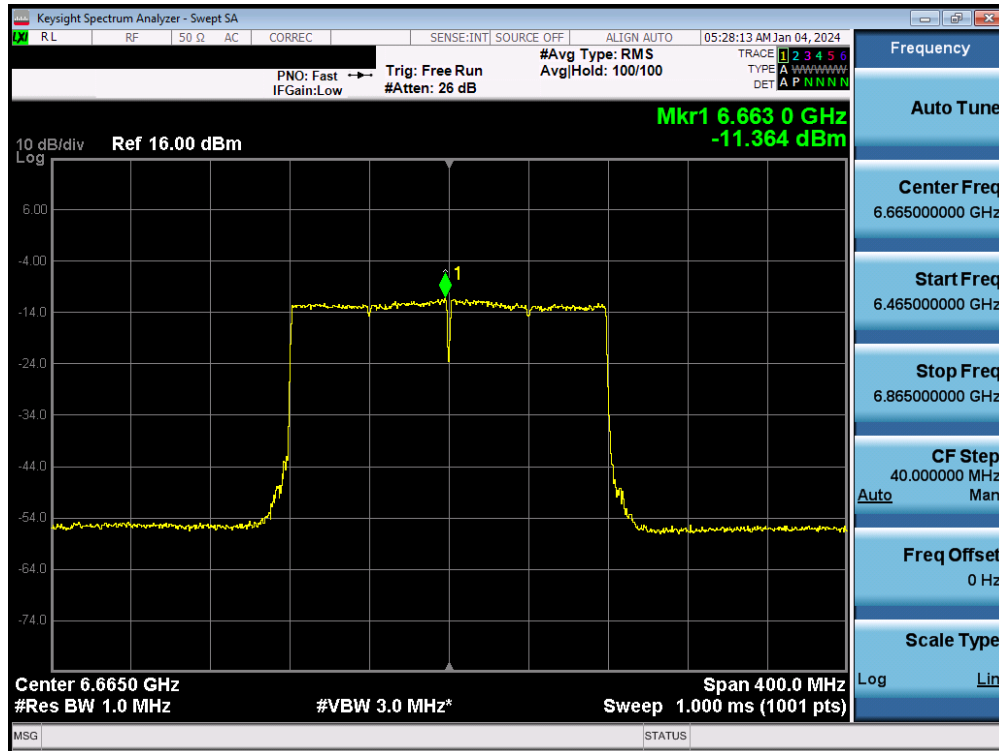
Plot 7-106. Power Spectral Density MIMO ANT2 (160MHz 802.11ax/be (UNII Band 7) – Ch. 143) - LPI
