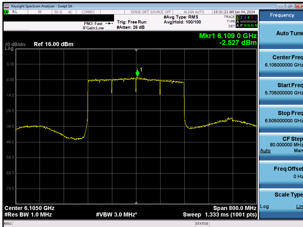
Plot 7-95. Power Spectral Density MIMO ANT2 (320MHz 802.11ax/be (UNII Band 5) – Ch.31) - SP
