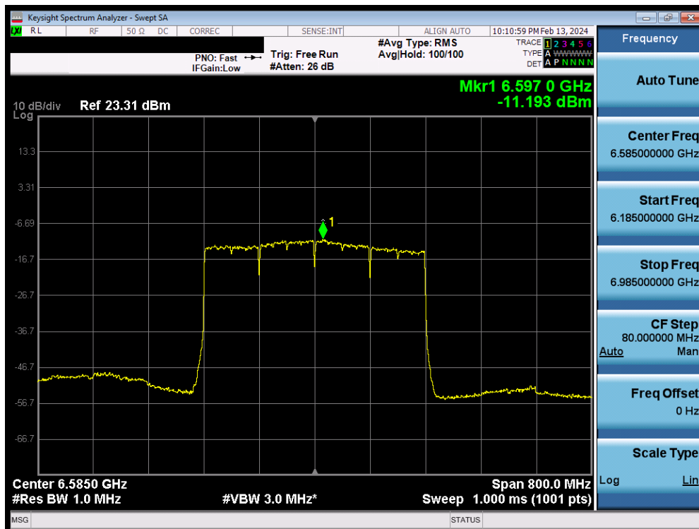
Plot 7-107. Power Spectral Density MIMO ANT2 (320MHz 802.11ax/be (UNII Band 6/7) – Ch. 127) - LPI
