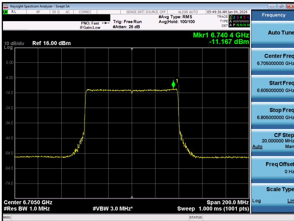
Plot 7-105. Power Spectral Density MIMO ANT2 (80MHz 802.11ax/be (UNII Band 7) – Ch. 151) - LPI
