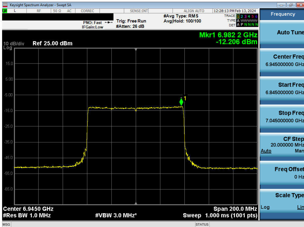
Plot 7-81. Power Spectral Density MIMO ANT1 (80MHz 802.11ax/be (UNII Band 8) – Ch. 199) - LPI
