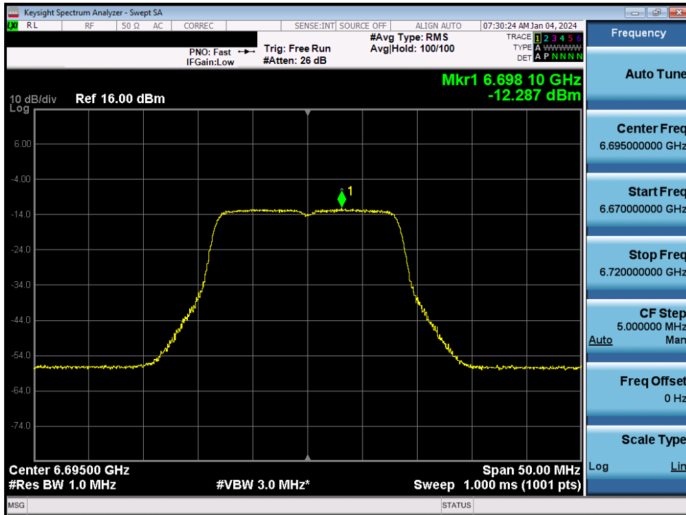
Plot 7-102. Power Spectral Density MIMO ANT2 (20MHz 802.11a (UNII Band 7) – Ch. 149) - LPI
