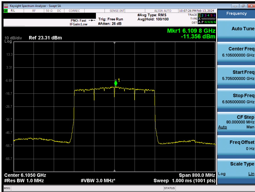
Plot 7-89. Power Spectral Density MIMO ANT2 (320MHz 802.11ax/be (UNII Band 5) – Ch.31) - LPI
