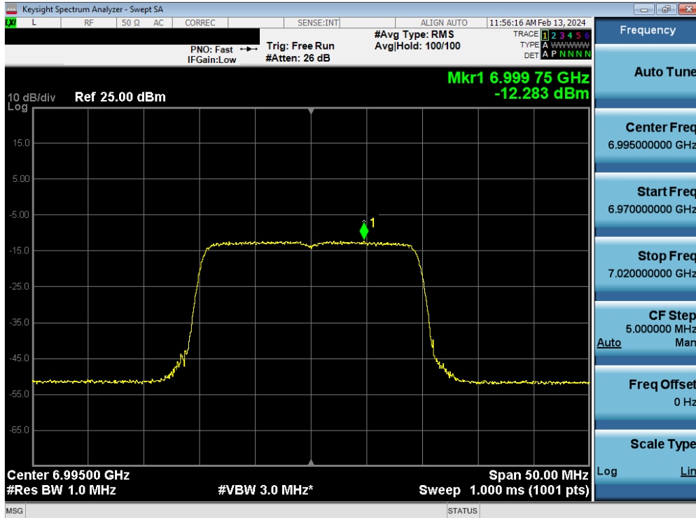
Plot 7-79. Power Spectral Density MIMO ANT1 (20MHz 802.11ax/be (UNII Band 8) – Ch. 209) - LPI
