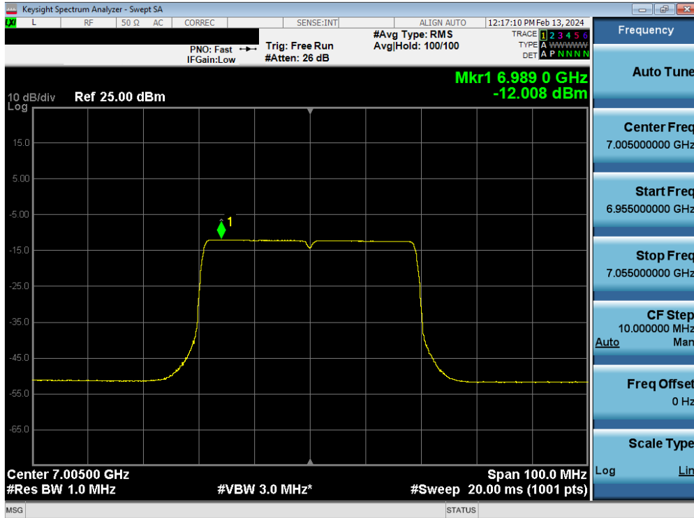
Plot 7-80. Power Spectral Density MIMO ANT1 (40MHz 802.11ax/be (UNII Band 8) – Ch. 211) - LPI
