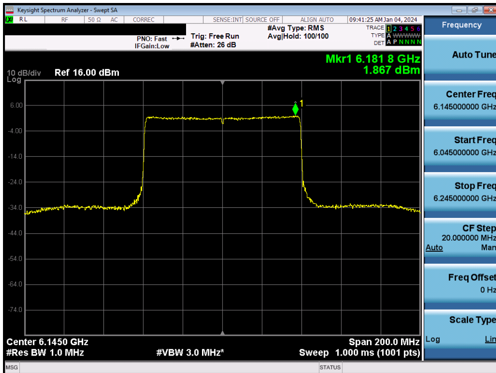
Plot 7-93. Power Spectral Density MIMO ANT2 (80MHz 802.11ax/be (UNII Band 5) – Ch. 39) - SP
