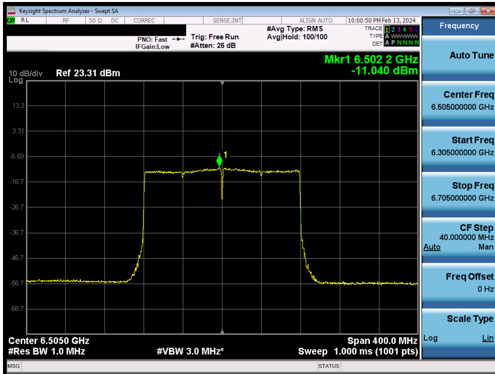
Plot 7-100. Power Spectral Density MIMO ANT2 (160MHz 802.11ax/be (UNII Band 6) – Ch. 111) - LPI
