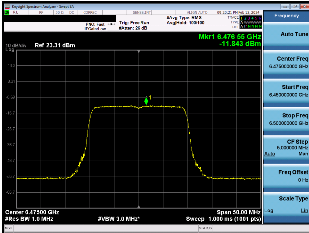
Plot 7-97. Power Spectral Density MIMO ANT2 (20MHz 802.11ax/be (UNII Band 6) – Ch. 105) - LPI
