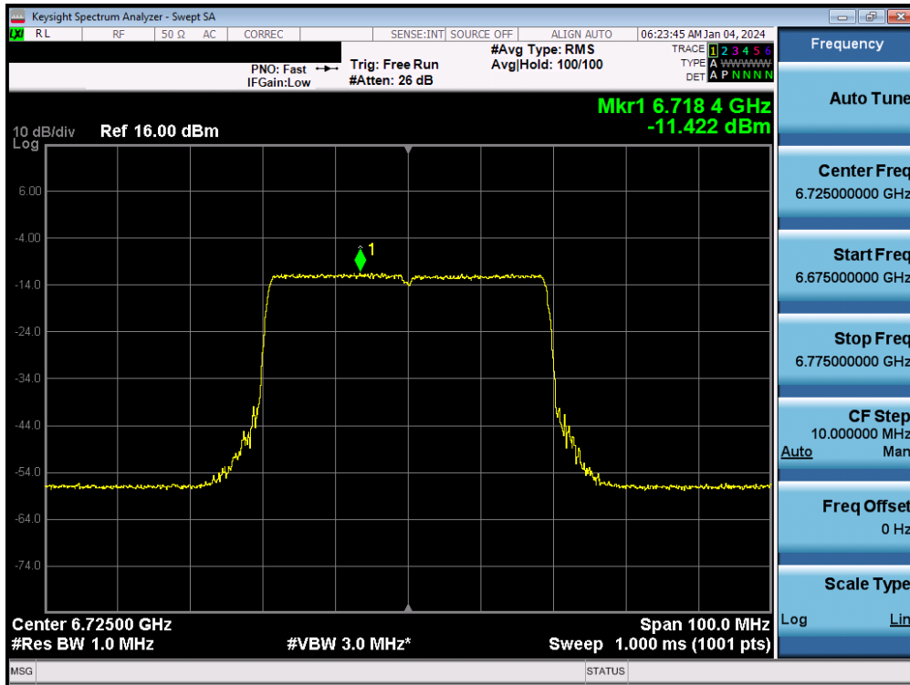
Plot 7-104. Power Spectral Density MIMO ANT2 (40MHz 802.11ax/be (UNII Band 7) – Ch. 155) - LPI
