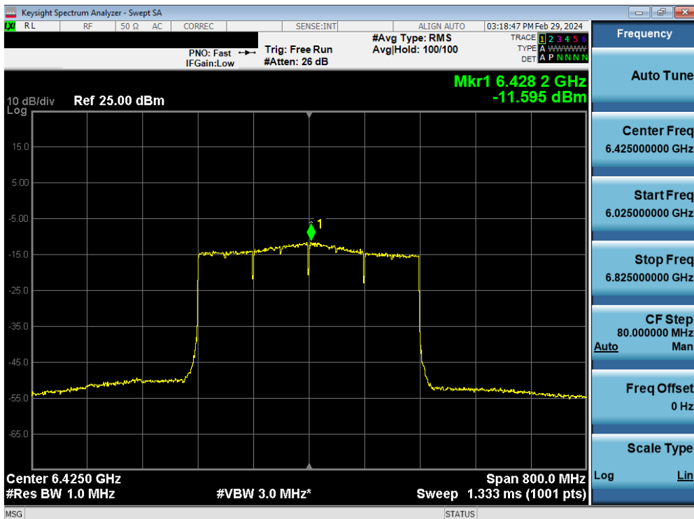
Plot 7-101. Power Spectral Density MIMO ANT2 (320MHz 802.11ax/be (UNII Band 5/6/7) – Ch. 95) - LPI
