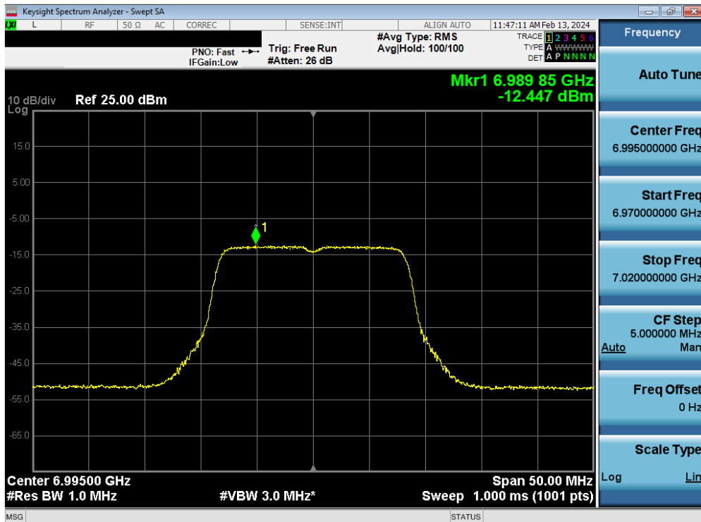
Plot 7-78. Power Spectral Density MIMO ANT1 (20MHz 802.11a (UNII Band 8) – Ch. 209) - LPI
