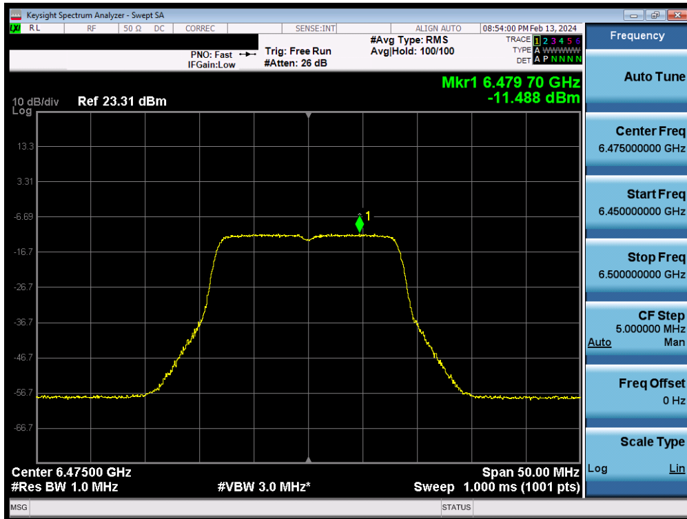
Plot 7-96. Power Spectral Density MIMO ANT2 (20MHz 802.11a (UNII Band 6) – Ch. 105) - LPI
