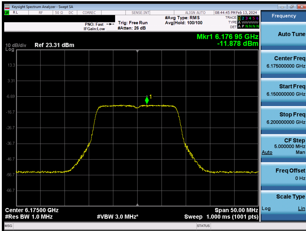
Plot 7-84. Power Spectral Density MIMO ANT2 (20MHz 802.11a (UNII Band 5) – Ch. 45) - LPI
