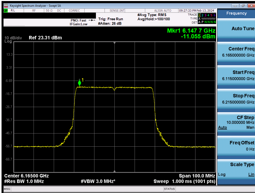
Plot 7-86. Power Spectral Density MIMO ANT2 (40MHz 802.11ax/be (UNII Band 5) – Ch. 43) - LPI
