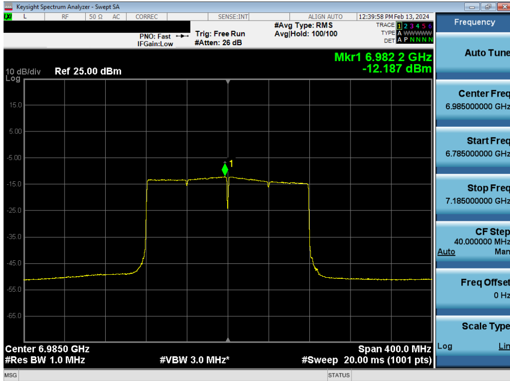
Plot 7-82. Power Spectral Density MIMO ANT1 (160MHz 802.11ax/be (UNII Band 8) – Ch. 207) - LPI
