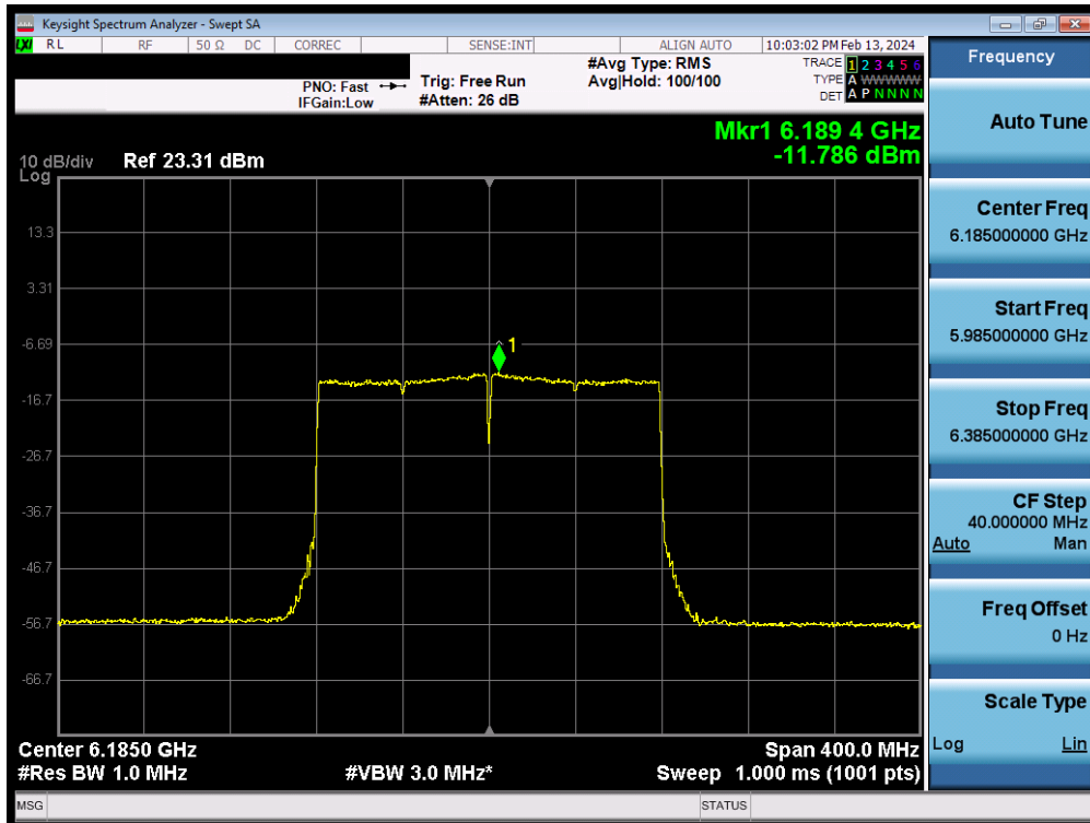
Plot 7-88. Power Spectral Density MIMO ANT2 (160MHz 802.11ax/be (UNII Band 5) – Ch. 47) - LPI
