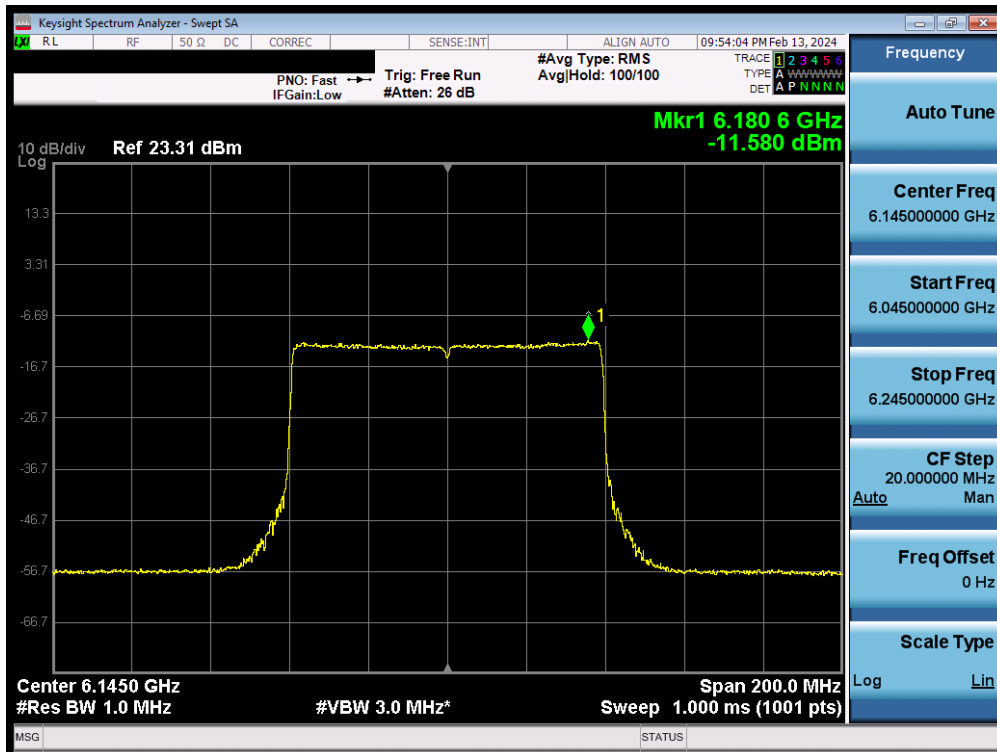
Plot 7-87. Power Spectral Density MIMO ANT2 (80MHz 802.11ax/be (UNII Band 5) – Ch. 39) - LPI
