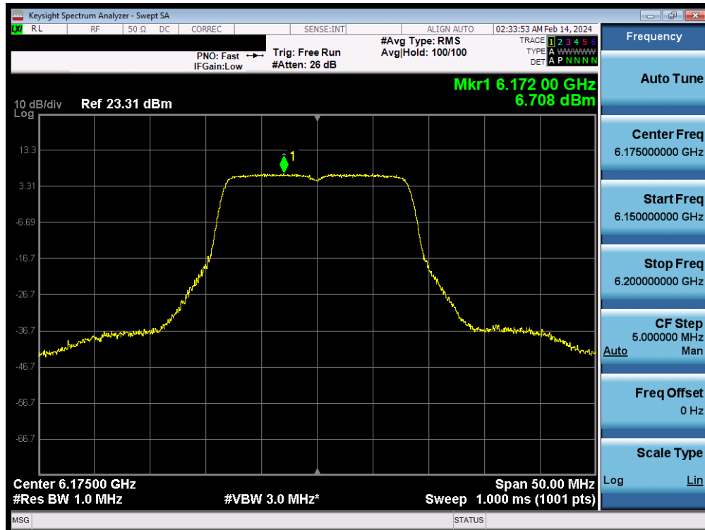
Plot 7-90. Power Spectral Density MIMO ANT2 (20MHz 802.11a (UNII Band 5) – Ch. 45) – SP
