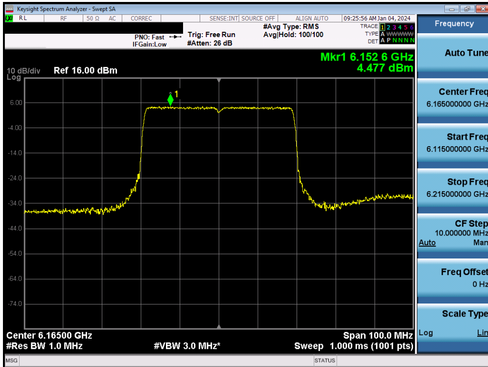
Plot 7-92. Power Spectral Density MIMO ANT2 (40MHz 802.11ax/be (UNII Band 5) – Ch. 43) - SP
