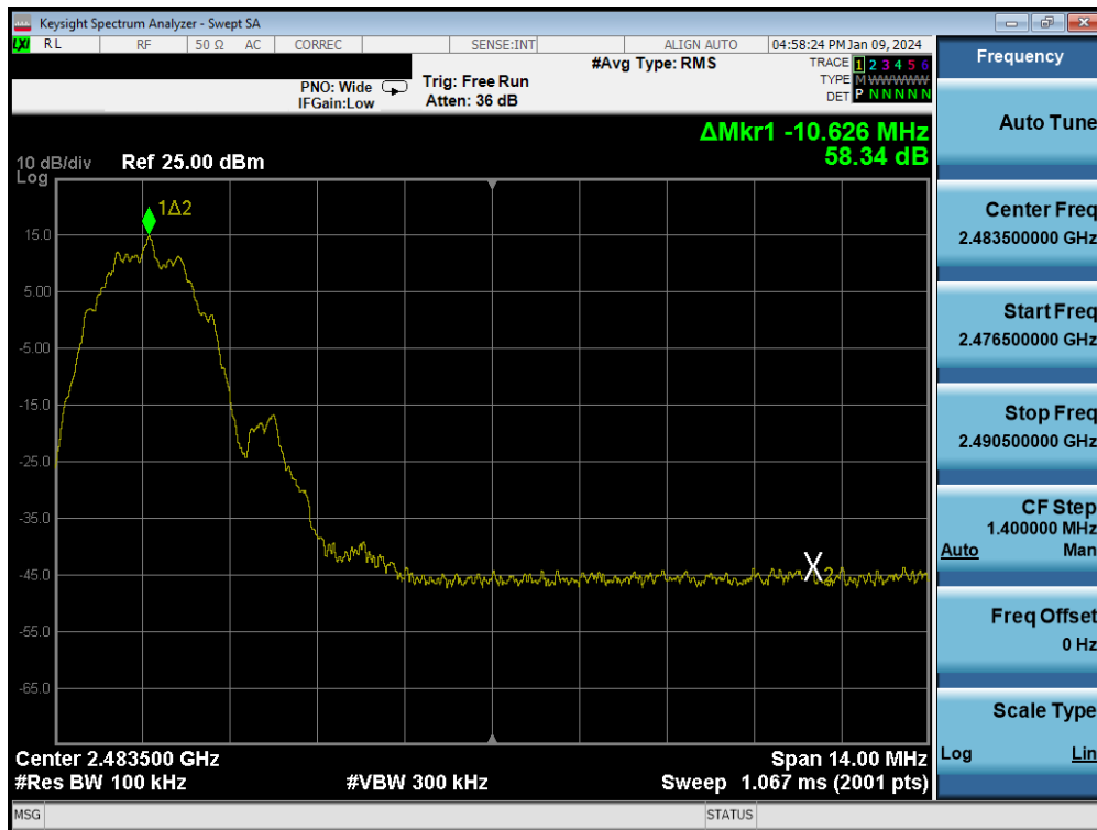
Plot 7-128. Band Edge Plot (Bluetooth (LE), 2Mbps – Ch. 36)
