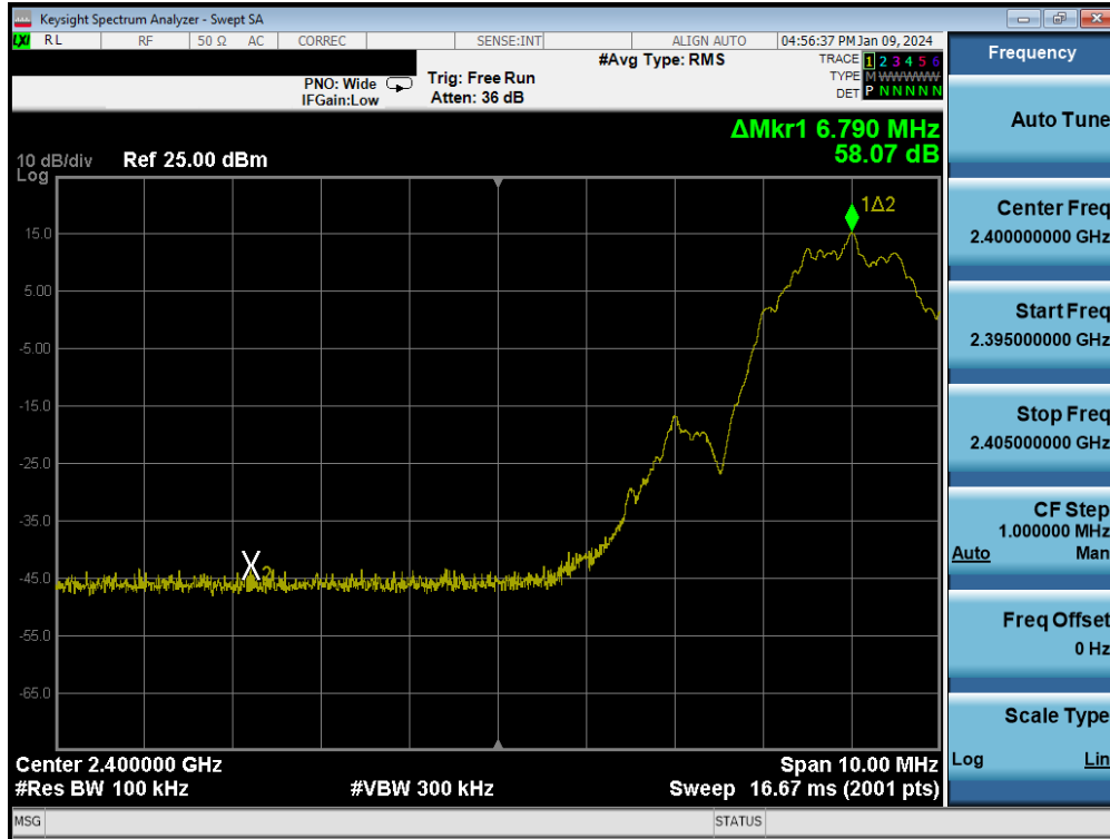
Plot 7-127. Band Edge Plot (Bluetooth (LE), 2Mbps – Ch. 0)
