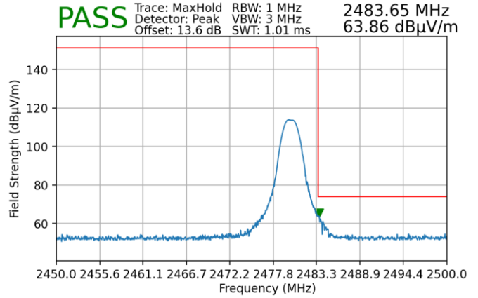
Plot 7-162. Radiated Restricted Upper Band Edge Measurement (Peak) – DUAL
