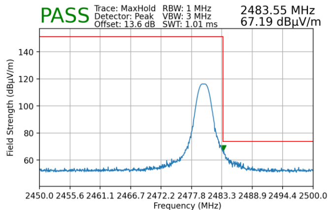
Plot 7-160. Radiated Restricted Upper Band Edge Measurement (Peak) – SISO ANT2
