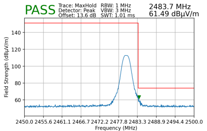
Plot 7-158. Radiated Restricted Upper Band Edge Measurement (Peak) – SISO ANT1
