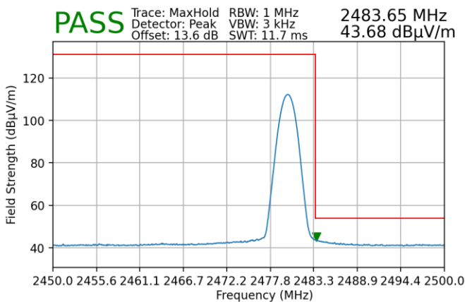
Plot 7-157. Radiated Restricted Upper Band Edge Measurement (Average) – SISO ANT1
