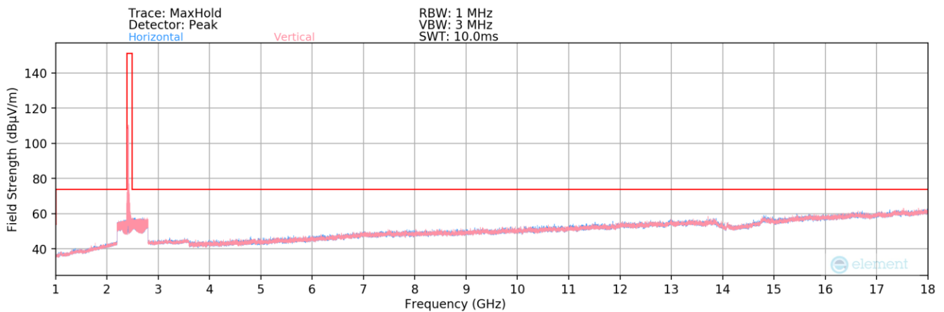
Plot 7-143. Radiated Spurious Plot above 1GHz MIMO (802.11be OFDMA – 242 Tones – Ch. 1)
