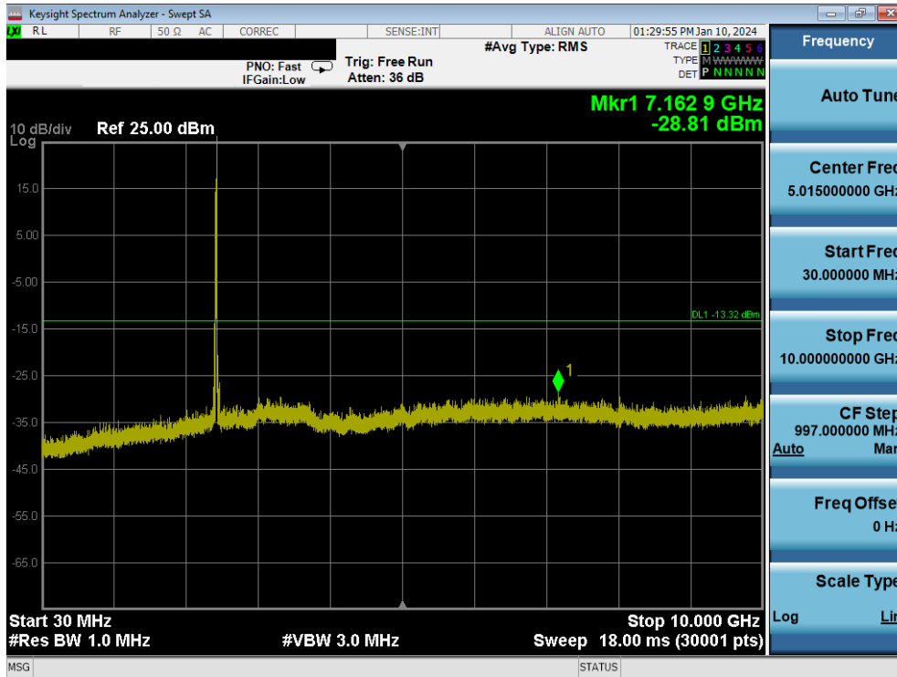
Plot 7-123. Conducted Spurious Plot MIMO ANT2 (802.11be OFDMA – 26 Tones – Ch. 6)
