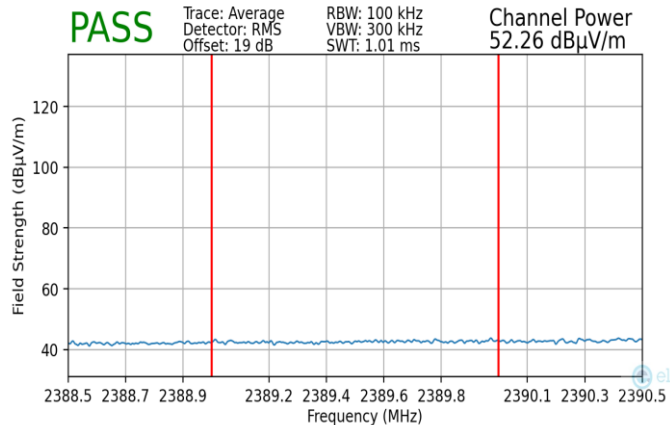
Plot 7-201. Radiated Restricted Lower Band Edge Measurement MIMO (Average – 242 Tones)
