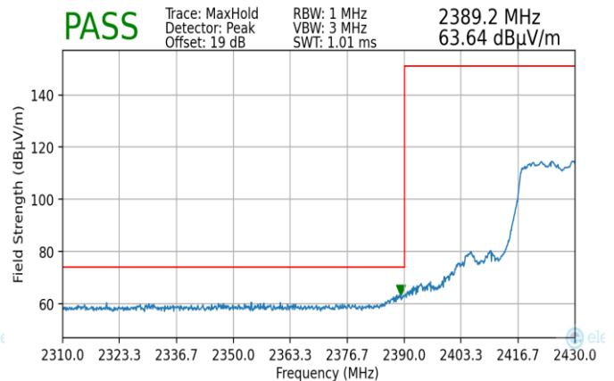
Plot 7-200. Radiated Restricted Lower Band Edge Measurement MIMO (Peak – 242 Tones)
