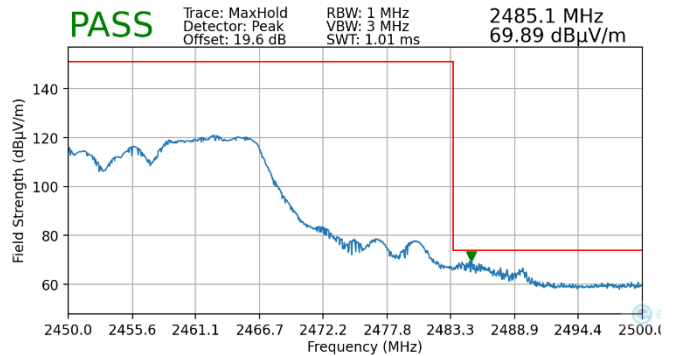
Plot 7-164. Radiated Restricted Upper Band Edge Measurement MIMO (Peak – 106 Tones)
