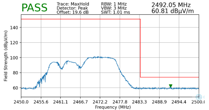
Plot 7-168. Radiated Restricted Upper Band Edge Measurement MIMO (Peak – 106 Tones)
