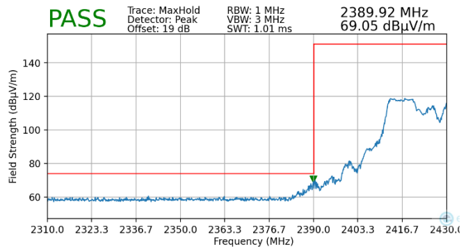
Plot 7-152. Radiated Restricted Lower Band Edge Measurement MIMO (Peak – 106 Tones)
