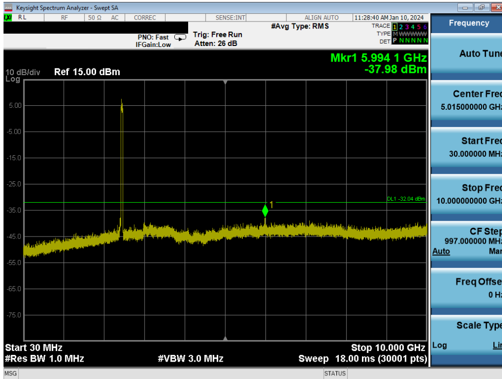
Plot 7-119. Conducted Spurious Plot MIMO ANT1 (802.11be OFDMA – 484 Tones – Ch. 11)
