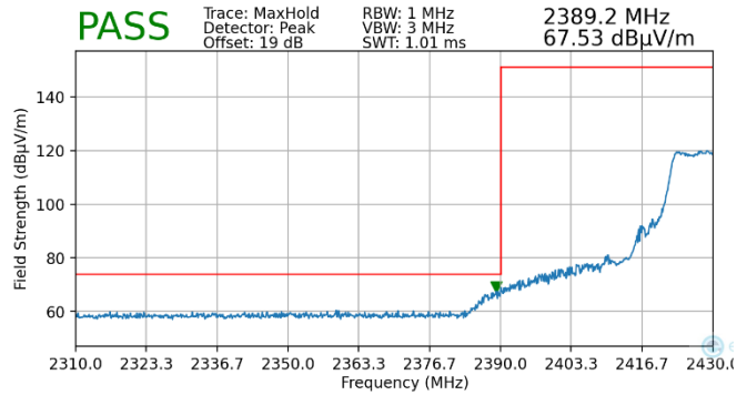
Plot 7-156. Radiated Restricted Lower Band Edge Measurement MIMO (Peak – 106 Tones)
