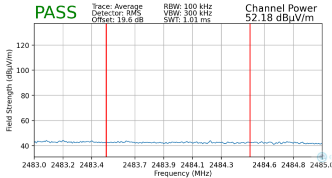
Plot 7-161. Radiated Restricted Upper Band Edge Measurement MIMO (Average – 106 Tones)
