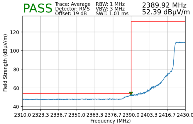
Plot 7-179. Radiated Restricted Lower Band Edge Measurement MIMO (Average – 106 + 26 Tones)
