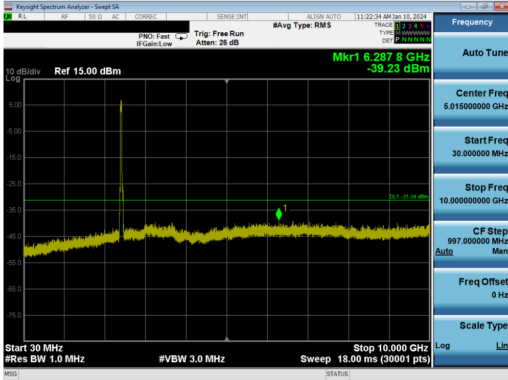
Plot 7-133. Conducted Spurious Plot MIMO ANT2 (802.11be OFDMA – 484 Tones – Ch. 3)
