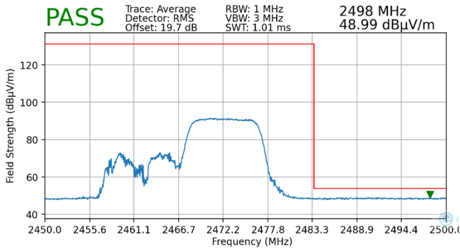
Plot 7-167. Radiated Restricted Upper Band Edge Measurement MIMO (Average – 106 Tones)
