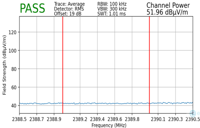
Plot 7-197. Radiated Restricted Lower Band Edge Measurement MIMO (Average – 242 Tones)
