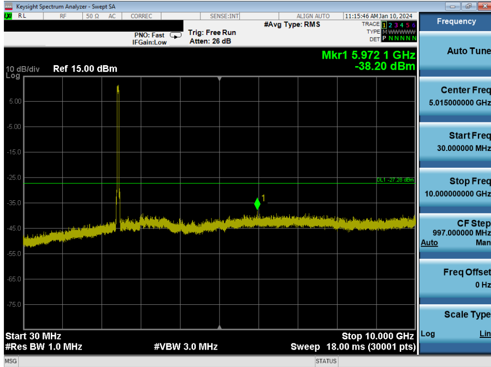
Plot 7-117. Conducted Spurious Plot MIMO ANT1 (802.11be OFDMA – 484 Tones – Ch. 6)
