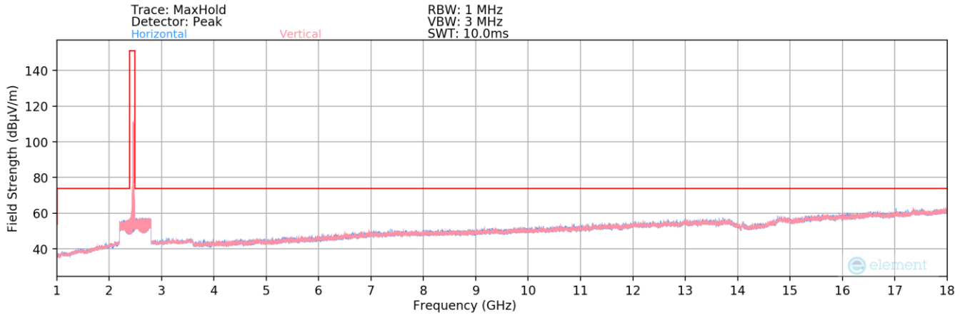
Plot 7-145. Radiated Spurious Plot above 1GHz MIMO (802.11be OFDMA – 242 Tones – Ch. 11)
