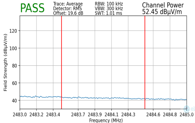
Plot 7-209. Radiated Restricted Upper Band Edge Measurement MIMO (Average – 242 Tones)
