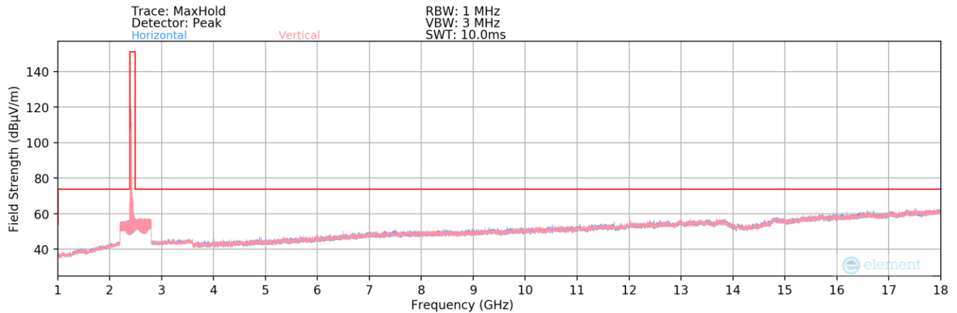
Plot 7-139. Radiated Spurious Plot above 1GHz MIMO (802.11be OFDMA – 26 Tones – Ch. 1)
