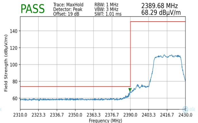
Plot 7-196. Radiated Restricted Lower Band Edge Measurement MIMO (Peak – 242 Tones)
