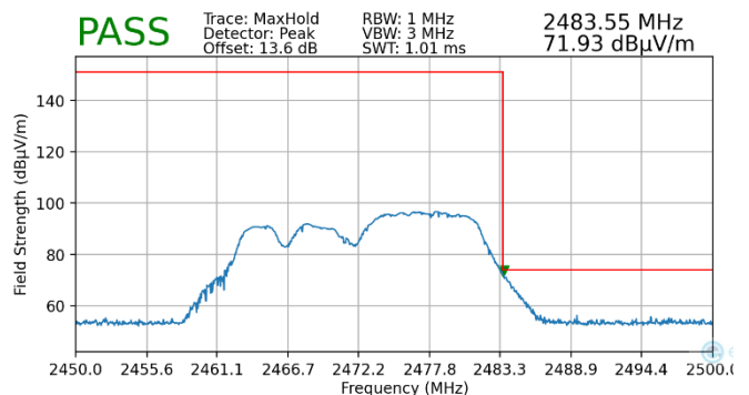
Plot 7-170. Radiated Restricted Upper Band Edge Measurement MIMO (Peak – 106 Tones)
