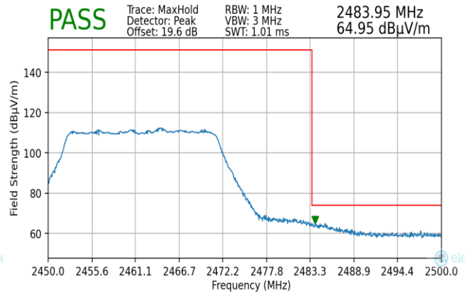
Plot 7-212. Radiated Restricted Upper Band Edge Measurement MIMO (Peak – 242 Tones)
