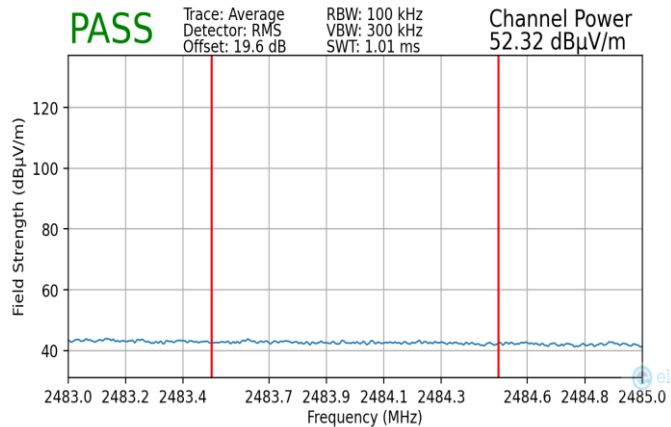
Plot 7-211. Radiated Restricted Upper Band Edge Measurement MIMO (Average – 242 Tones)
