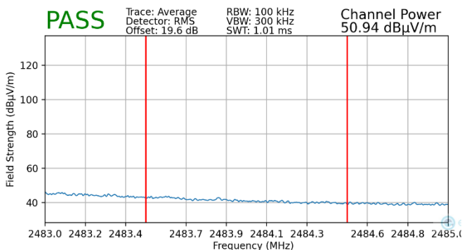
Plot 7-169. Radiated Restricted Upper Band Edge Measurement MIMO (Average – 106 Tones)
