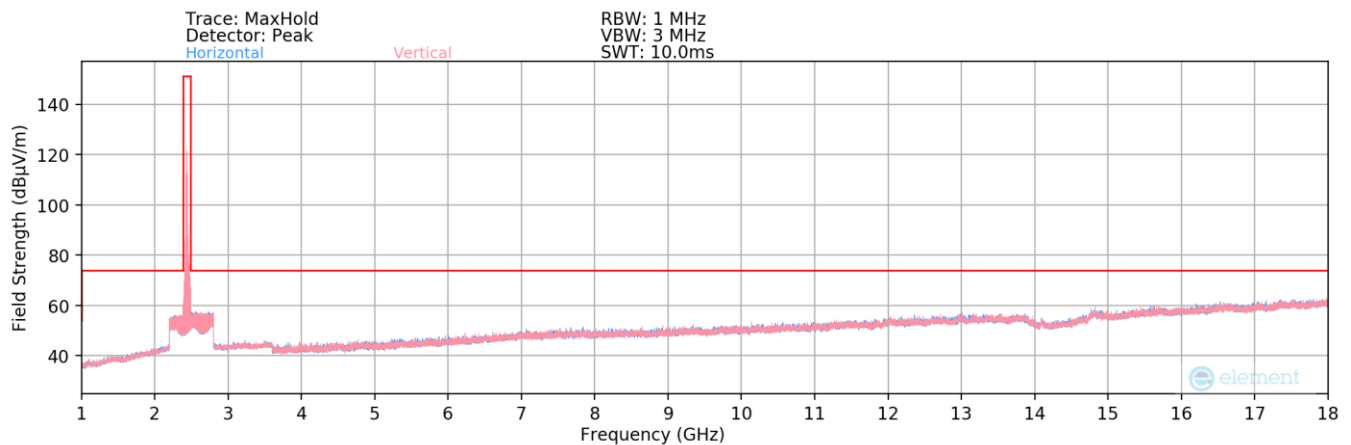
Plot 7-140. Radiated Spurious Plot above 1GHz MIMO (802.11be OFDMA – 26 Tones – Ch. 6)
