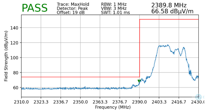
Plot 7-148. Radiated Restricted Lower Band Edge Measurement MIMO (Peak – 106 Tones)
