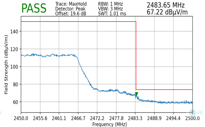
Plot 7-210. Radiated Restricted Upper Band Edge Measurement MIMO (Peak – 242 Tones)
