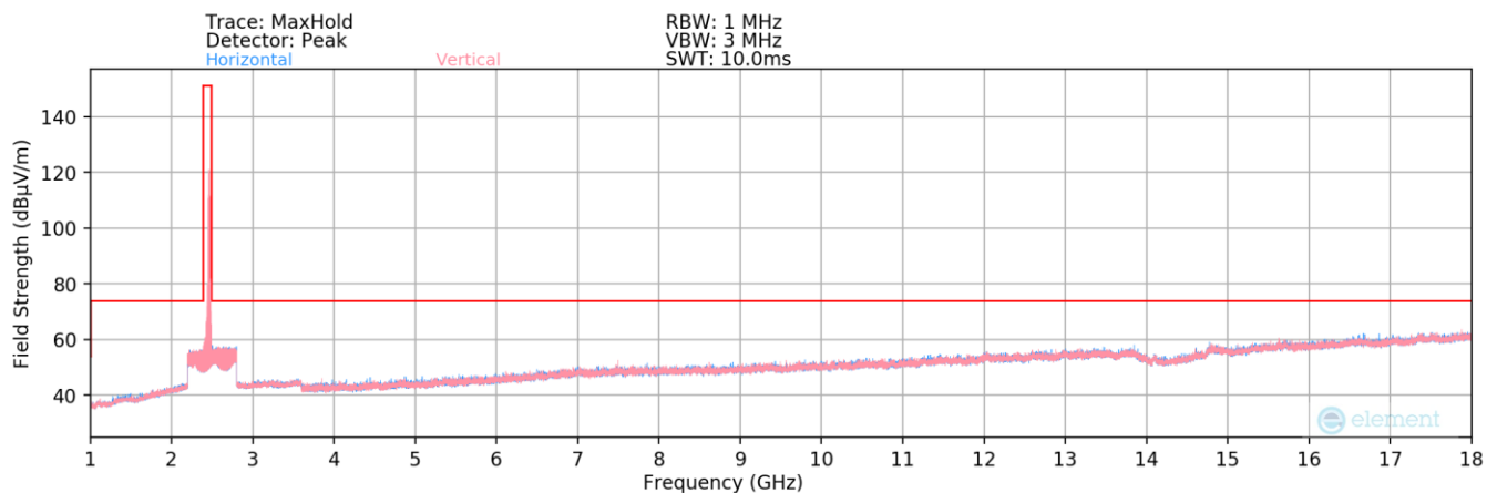
Plot 7-141. Radiated Spurious Plot above 1GHz MIMO (802.11be OFDMA – 26 Tones – Ch. 11)
