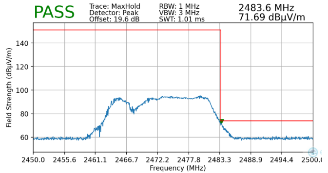
Plot 7-192. Radiated Restricted Upper Band Edge Measurement MIMO (Peak – 106 + 26 Tones)
