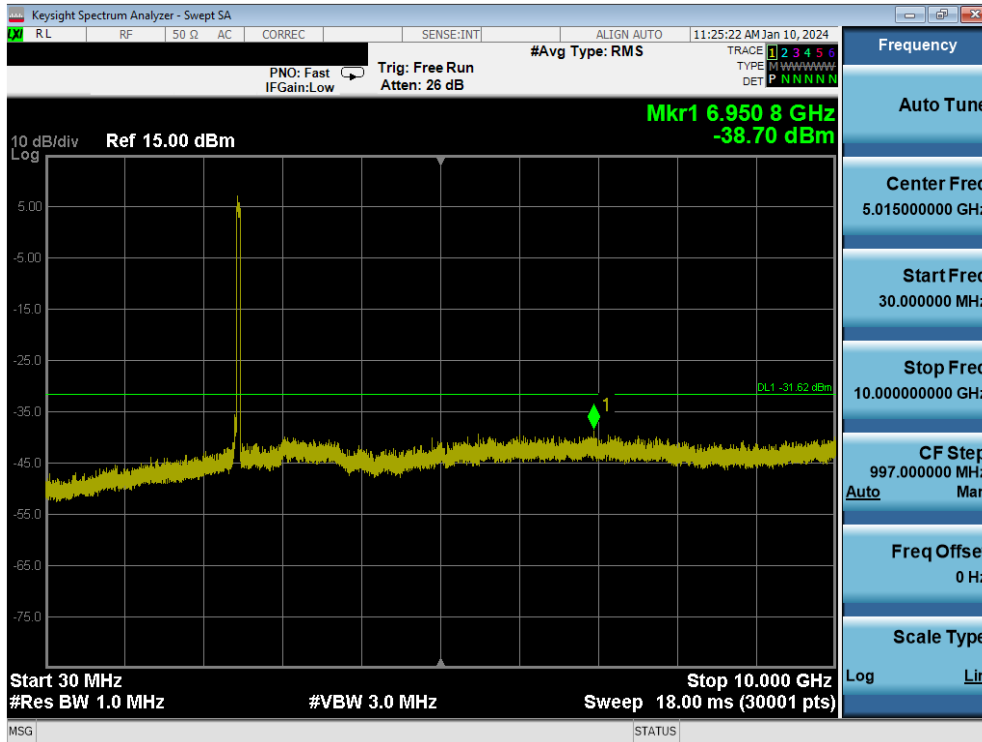
Plot 7-137. Conducted Spurious Plot MIMO ANT2 (802.11be OFDMA – 484 Tones – Ch. 11)
