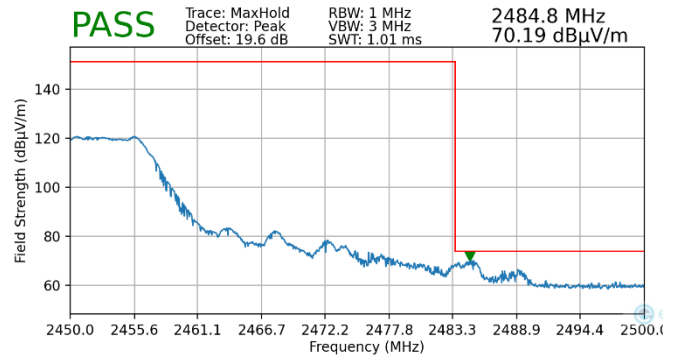
Plot 7-160. Radiated Restricted Upper Band Edge Measurement MIMO (Peak – 106 Tones)
