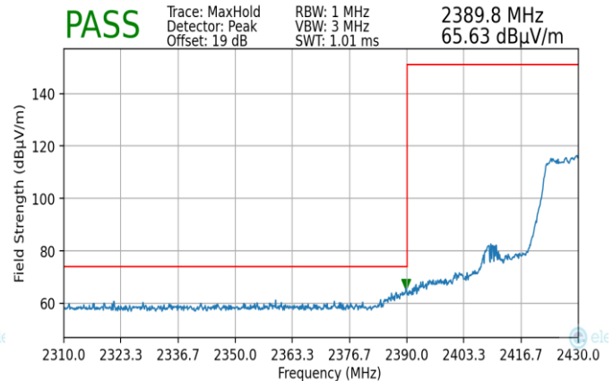
Plot 7-202. Radiated Restricted Lower Band Edge Measurement MIMO (Peak – 242 Tones)
