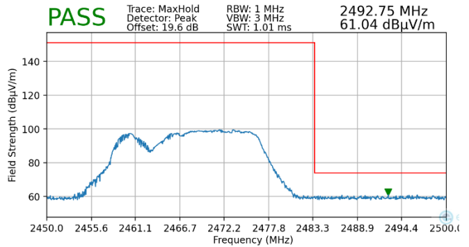
Plot 7-190. Radiated Restricted Upper Band Edge Measurement MIMO (Peak – 106 + 26 Tones)
