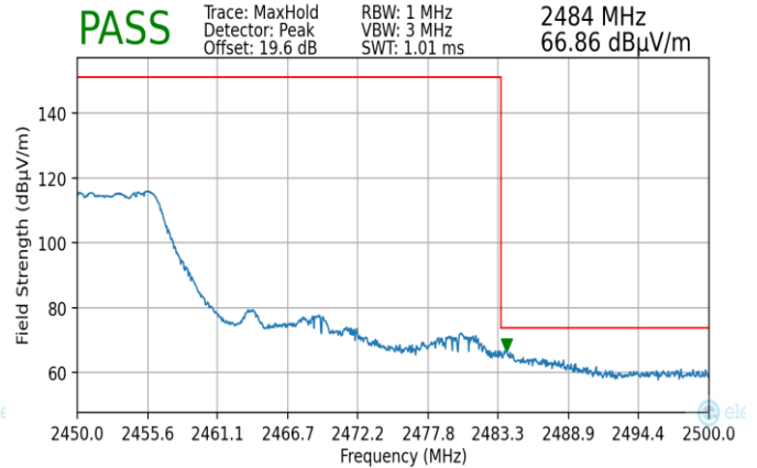
Plot 7-206. Radiated Restricted Upper Band Edge Measurement MIMO (Peak – 242 Tones)
