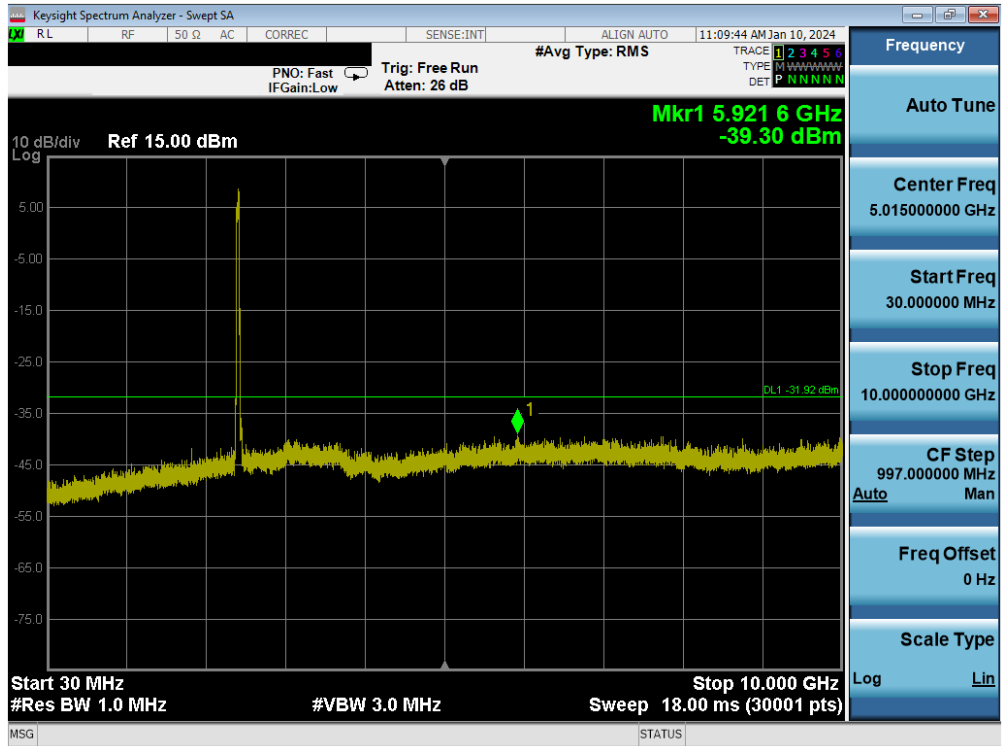
Plot 7-115. Conducted Spurious Plot MIMO ANT1 (802.11be OFDMA – 484 Tones – Ch. 3)
