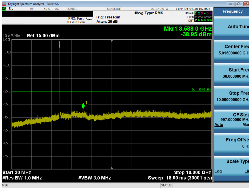
Plot 7-127. Conducted Spurious Plot MIMO ANT2 (802.11be OFDMA – 242 Tones – Ch. 1)
