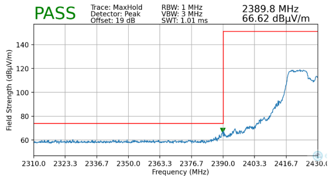
Plot 7-154. Radiated Restricted Lower Band Edge Measurement MIMO (Peak – 106 Tones)
