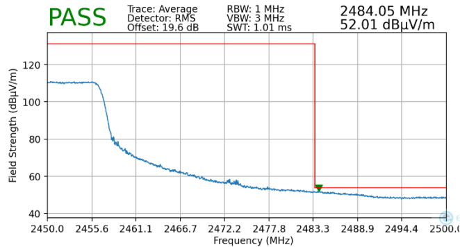
Plot 7-159. Radiated Restricted Upper Band Edge Measurement MIMO (Average – 106 Tones)
