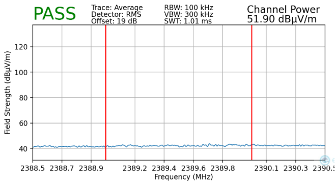
Plot 7-151. Radiated Restricted Lower Band Edge Measurement MIMO (Average – 106 Tones)
