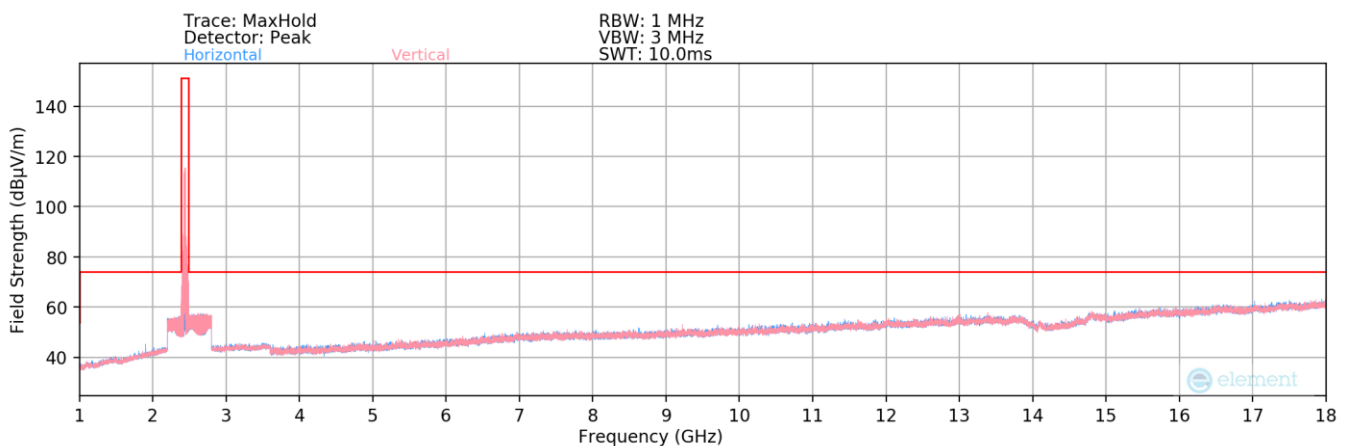
Plot 7-144. Radiated Spurious Plot above 1GHz MIMO (802.11be OFDMA – 242 Tones – Ch. 6)
