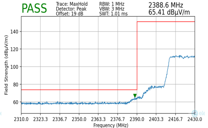
Plot 7-198. Radiated Restricted Lower Band Edge Measurement MIMO (Peak – 242 Tones)
