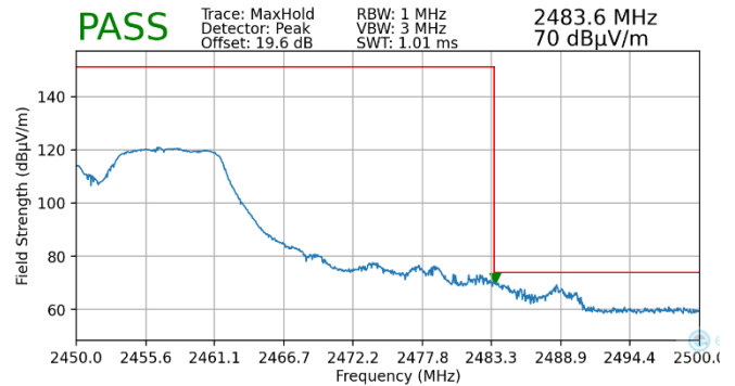
Plot 7-162. Radiated Restricted Upper Band Edge Measurement MIMO (Peak – 106 Tones)
