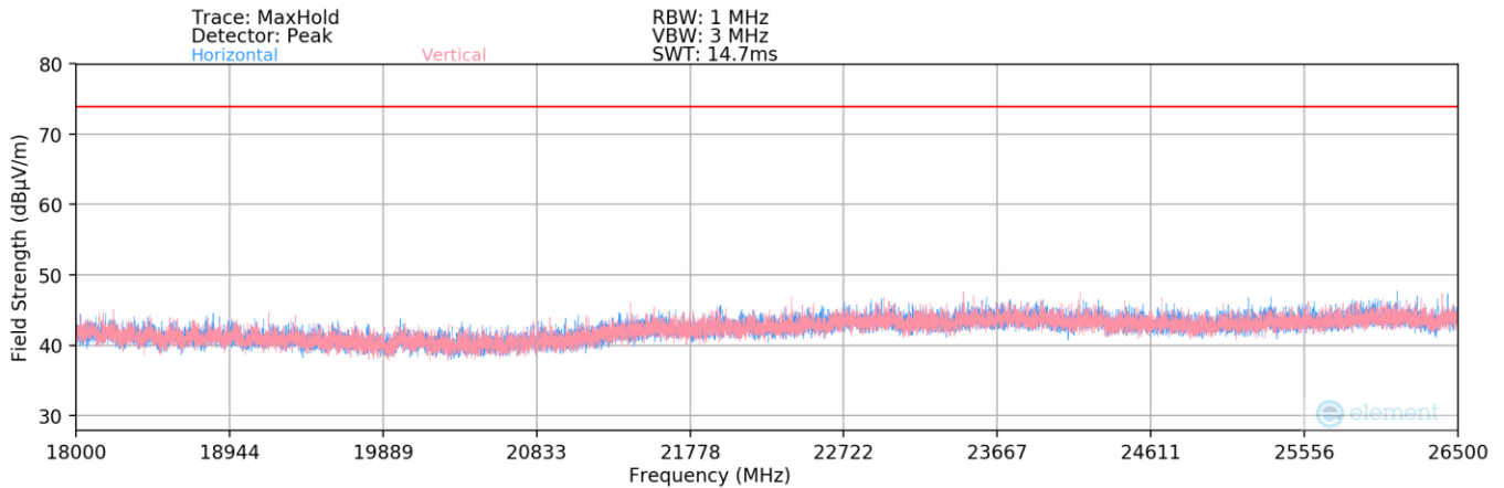
Plot 7-142. Radiated Spurious Plot above 18GHz MIMO (802.11be OFDMA – 26 Tones)
