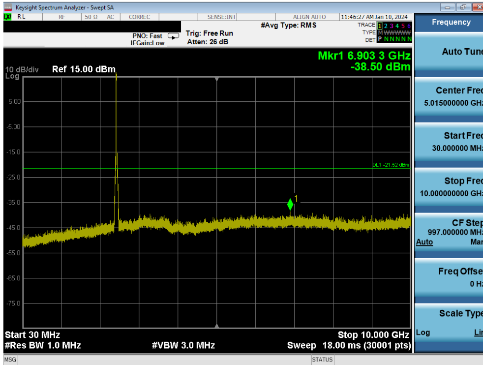
Plot 7-129. Conducted Spurious Plot MIMO ANT2 (802.11be OFDMA – 242 Tones – Ch. 6)
