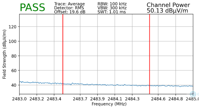
Plot 7-191. Radiated Restricted Upper Band Edge Measurement MIMO (Average – 106 + 26 Tones)
