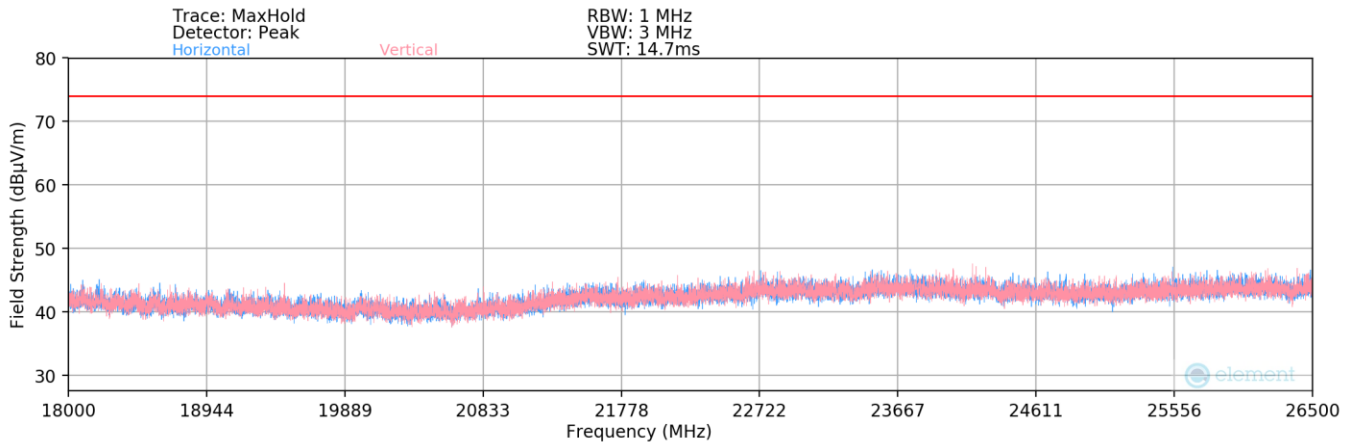
Plot 7-146. Radiated Spurious Plot above 18GHz MIMO (802.11be OFDMA – 242 Tones)
