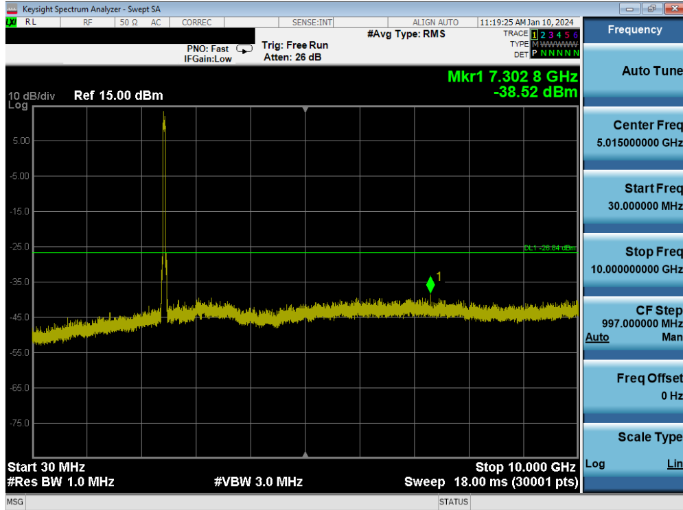
Plot 7-135. Conducted Spurious Plot MIMO ANT2 (802.11be OFDMA – 484 Tones – Ch. 6)
