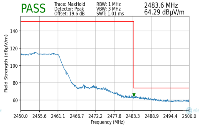
Plot 7-208. Radiated Restricted Upper Band Edge Measurement MIMO (Peak – 242 Tones)
