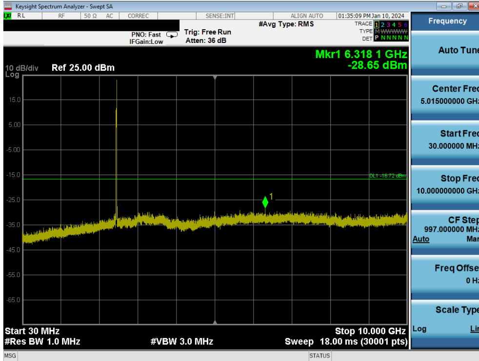
Plot 7-125. Conducted Spurious Plot MIMO ANT2 (802.11be OFDMA – 26 Tones – Ch. 11)
