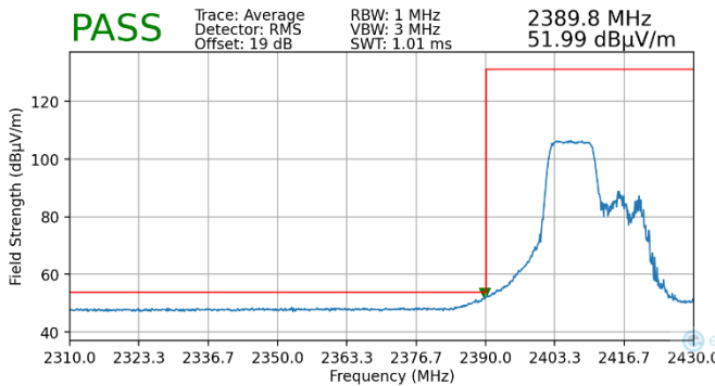
Plot 7-147. Radiated Restricted Lower Band Edge Measurement MIMO (Average – 106 Tones)
