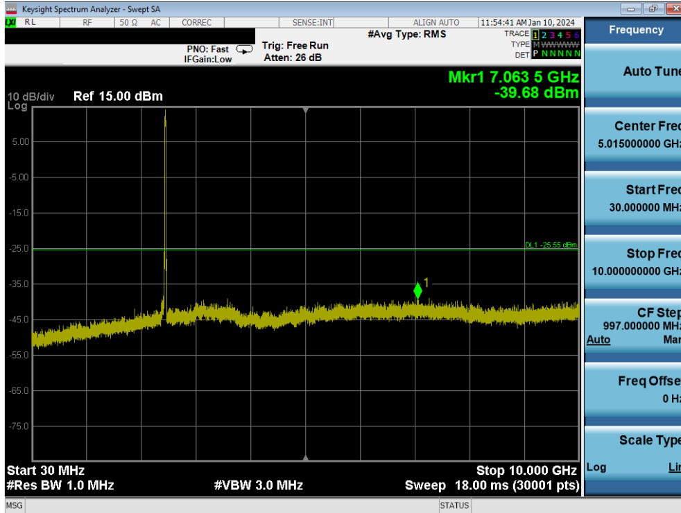
Plot 7-131. Conducted Spurious Plot MIMO ANT2 (802.11be OFDMA – 242 Tones – Ch. 11)
