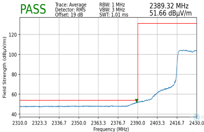
Plot 7-199. Radiated Restricted Lower Band Edge Measurement MIMO (Average – 242 Tones)
