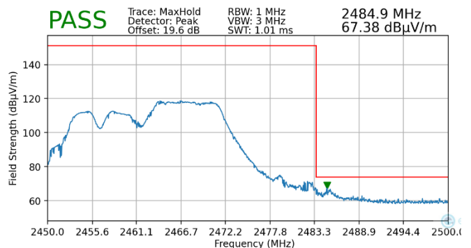
Plot 7-166. Radiated Restricted Upper Band Edge Measurement MIMO (Peak – 106 Tones)
