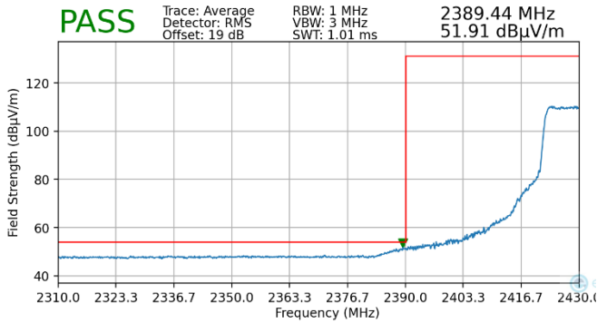
Plot 7-155. Radiated Restricted Lower Band Edge Measurement MIMO (Average – 106 Tones)
