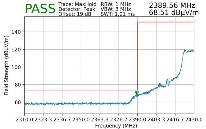
Plot 7-180. Radiated Restricted Lower Band Edge Measurement MIMO (Peak – 106 + 26 Tones)
