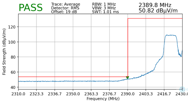
Plot 7-153. Radiated Restricted Lower Band Edge Measurement MIMO (Average – 106 Tones)
