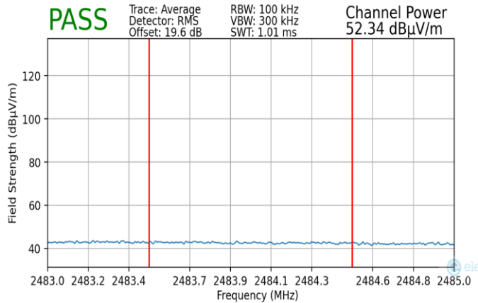
Plot 7-205. Radiated Restricted Upper Band Edge Measurement MIMO (Average)
