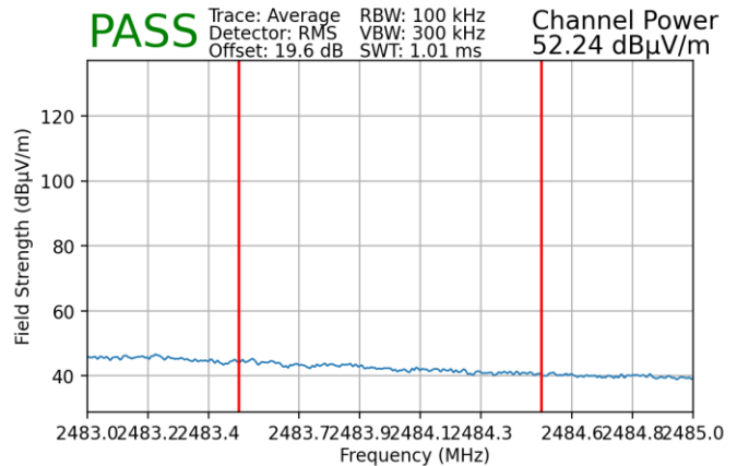
Plot 7-207. Radiated Restricted Upper Band Edge Measurement MIMO (Average)
