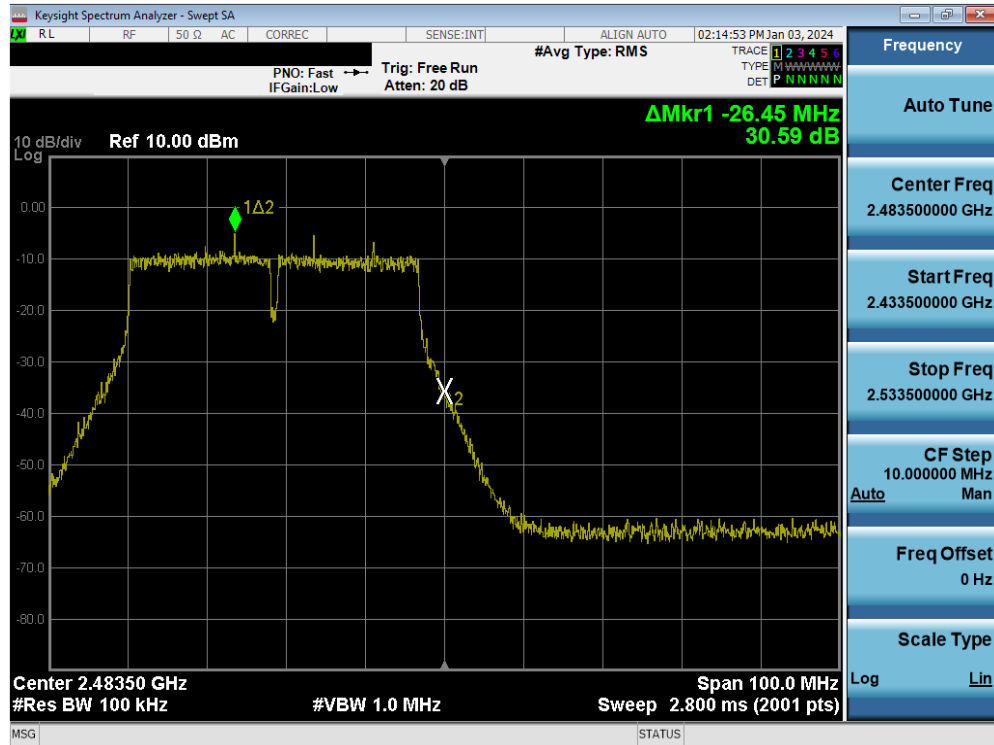
Plot 7-129. Band Edge Plot MIMO ANT1 (802.11n (2.4GHz) – Ch. 11)
