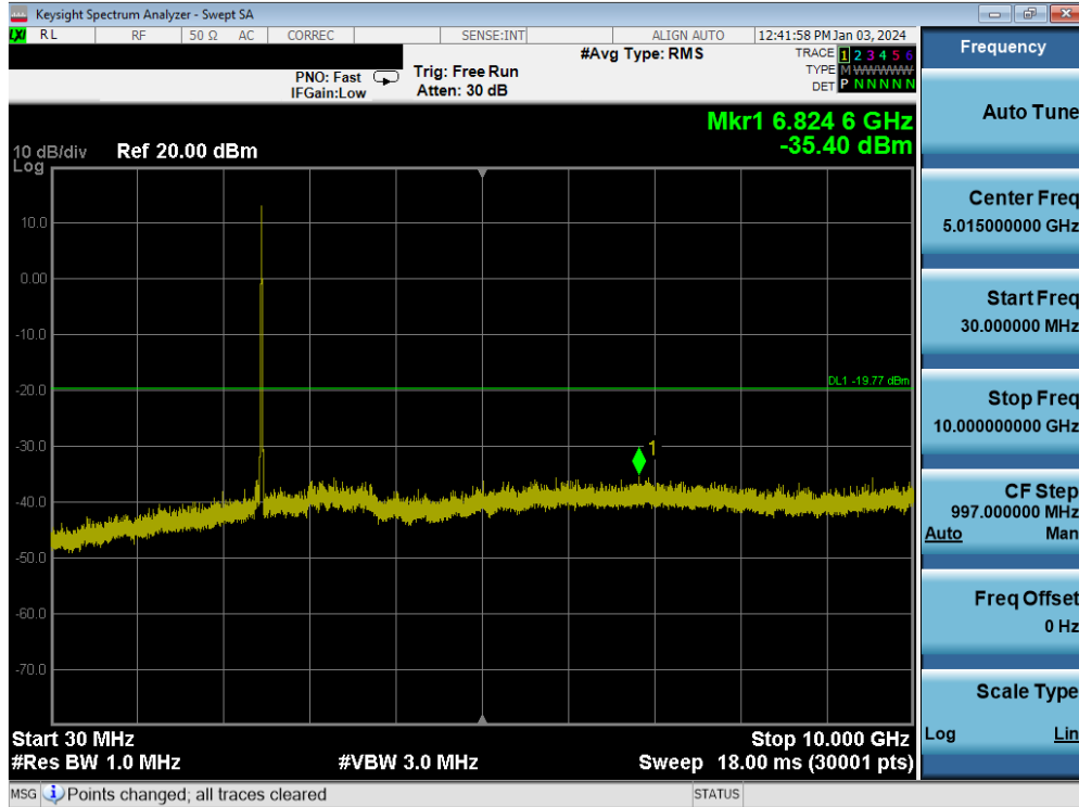
Plot 7-152. Conducted Spurious Plot MIMO ANT1 (802.11b – Ch. 11)
