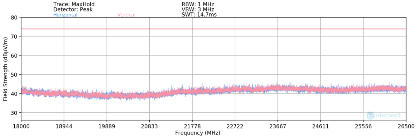
Plot 7-183. Radiated Spurious Plot 18GHz – 26.5GHz (2.4GHz – 6GHz)
