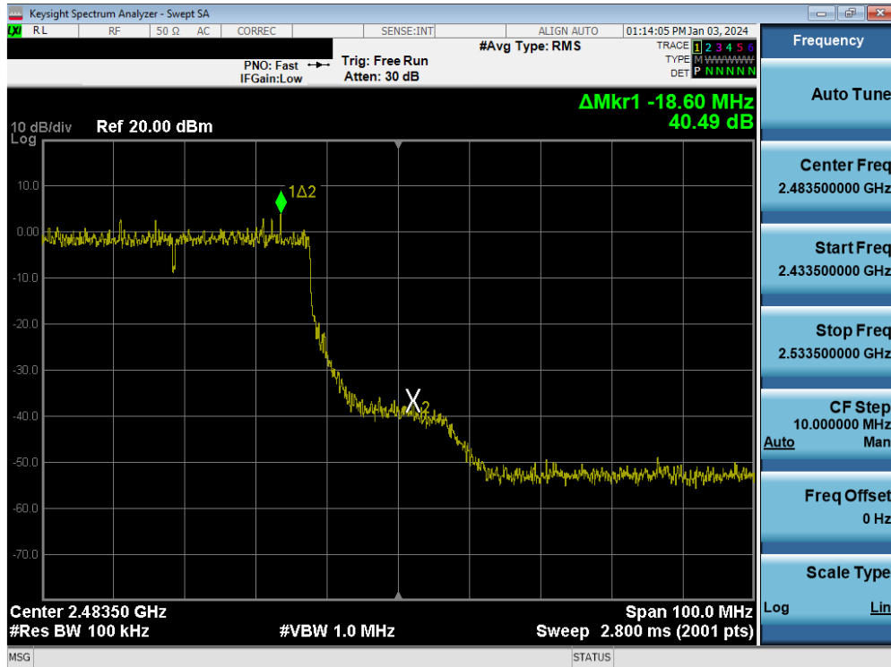
Plot 7-133. Band Edge Plot MIMO ANT1 (802.11be (2.4GHz) – Ch. 9)
