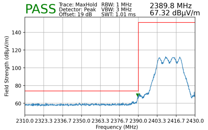
Plot 7-186. Radiated Restricted Lower Band Edge Measurement MIMO (Peak)
