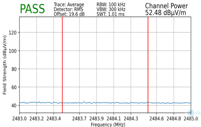
Plot 7-195. Radiated Restricted Upper Band Edge Measurement MIMO (Average)
