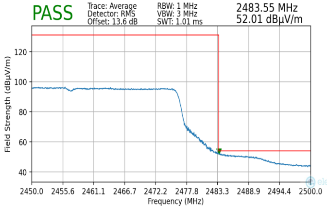
Plot 7-201. Radiated Restricted Upper Band Edge Measurement MIMO (Average)
