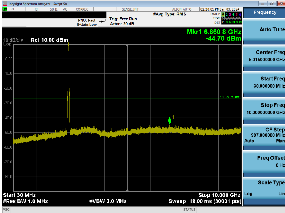
Plot 7-162. Conducted Spurious Plot MIMO ANT1 (802.11n – Ch. 6)
