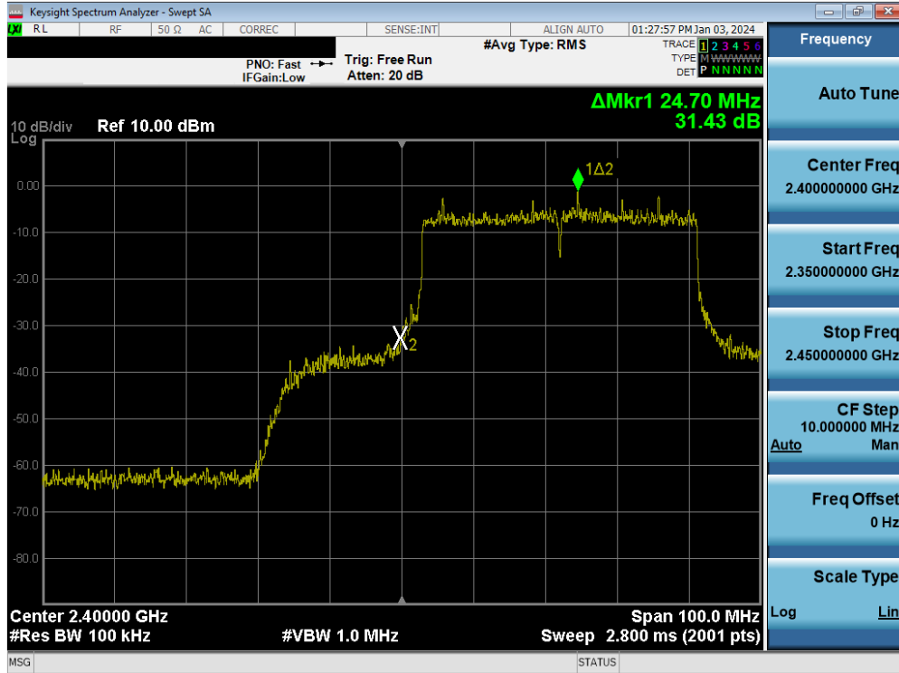
Plot 7-142. Band Edge Plot MIMO ANT2 (802.11be (2.4GHz) – Ch. 3)
