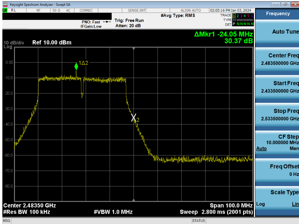
Plot 7-141. Band Edge Plot MIMO ANT2 (802.11n (2.4GHz) – Ch. 11)
