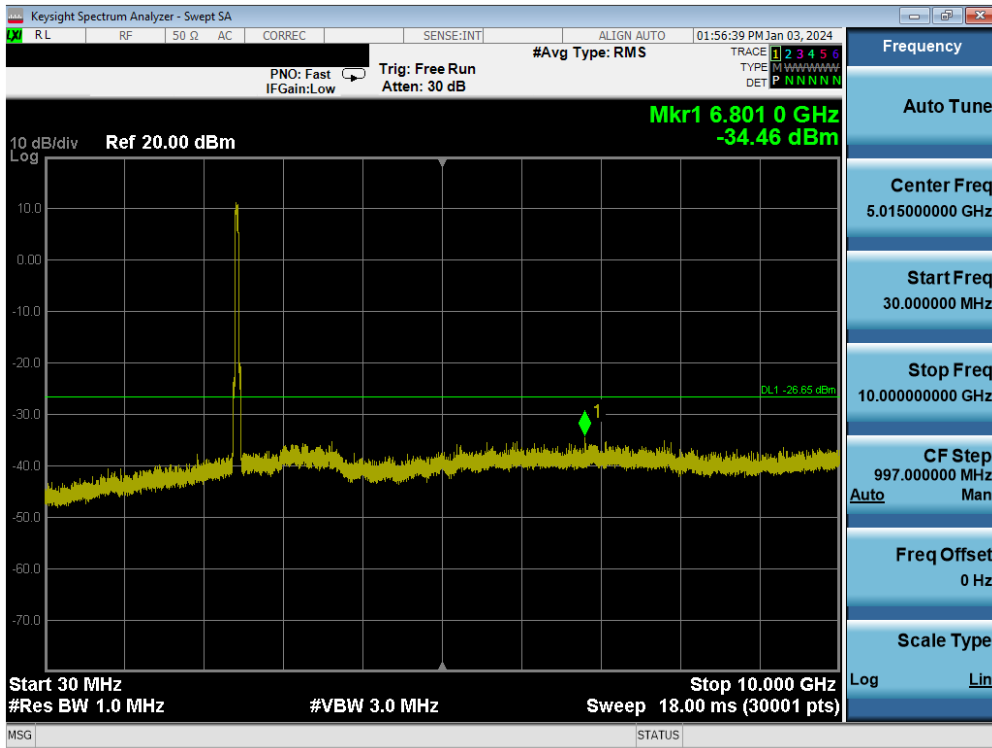
Plot 7-168. Conducted Spurious Plot MIMO ANT2 (802.11n – Ch. 6)
