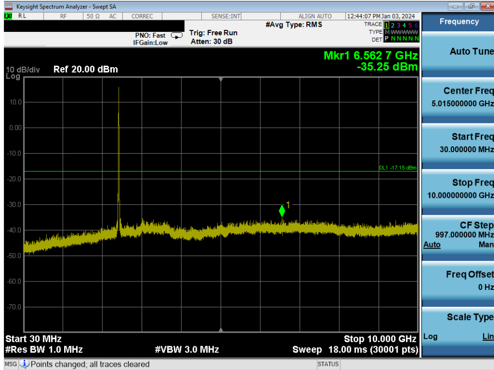
Plot 7-150. Conducted Spurious Plot MIMO ANT1 (802.11b – Ch. 6)
