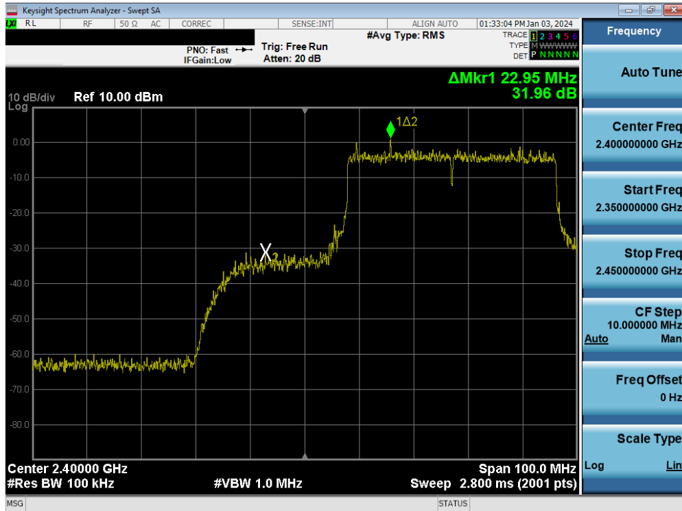
Plot 7-143. Band Edge Plot MIMO ANT2 (802.11be (2.4GHz) – Ch. 4)
