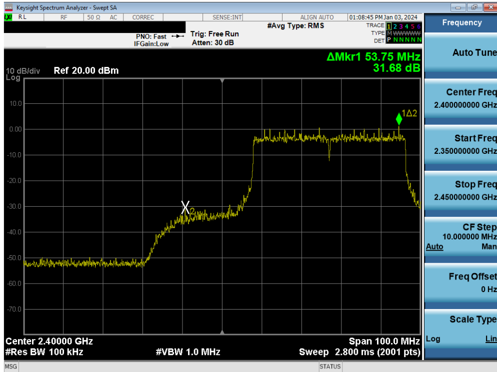
Plot 7-131. Band Edge Plot MIMO ANT1 (802.11be (2.4GHz) – Ch. 4)
