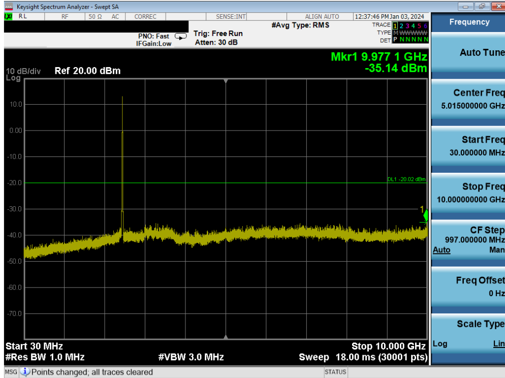
Plot 7-158. Conducted Spurious Plot MIMO ANT2 (802.11b – Ch. 11)
