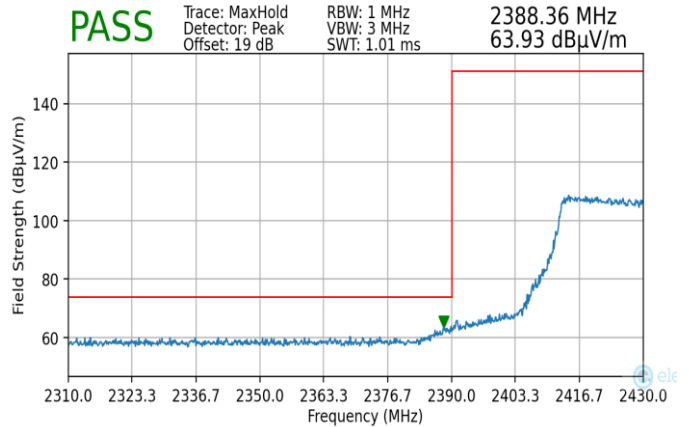
Plot 7-214. Radiated Restricted Lower Band Edge Measurement MIMO (Peak)
