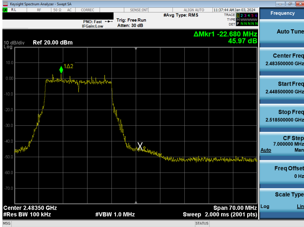
Plot 7-122. Band Edge Plot MIMO ANT2 (802.11be (2.4GHz) – Ch. 12)
