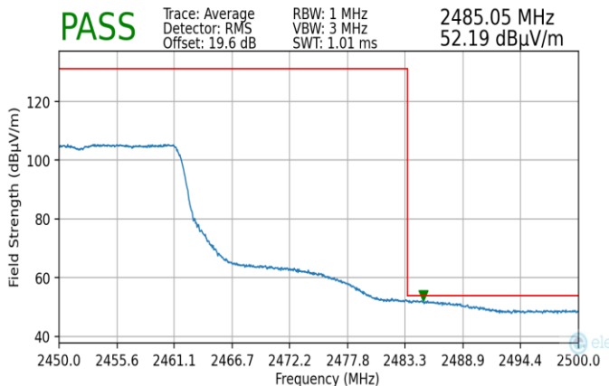
Plot 7-199. Radiated Restricted Upper Band Edge Measurement MIMO (Average)
