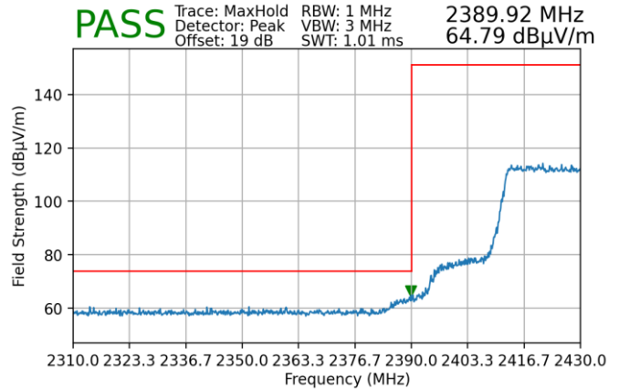
Plot 7-190. Radiated Restricted Lower Band Edge Measurement MIMO (Peak)
