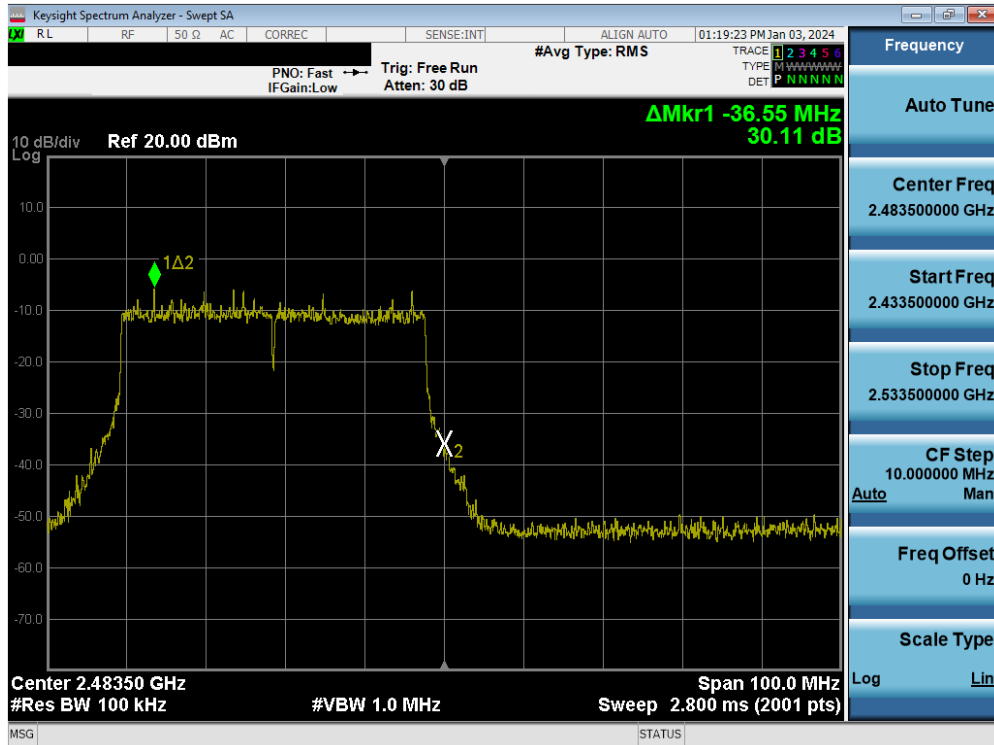
Plot 7-135. Band Edge Plot MIMO ANT1 (802.11be (2.4GHz) – Ch. 11)
