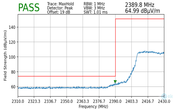
Plot 7-212. Radiated Restricted Lower Band Edge Measurement MIMO (Peak)
