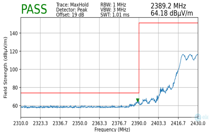
Plot 7-192. Radiated Restricted Lower Band Edge Measurement MIMO (Peak)
