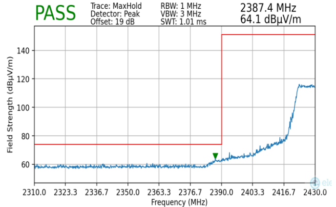
Plot 7-194. Radiated Restricted Lower Band Edge Measurement MIMO (Peak)
