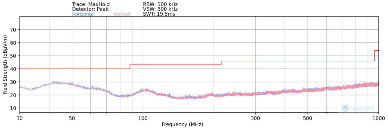
Plot 7-181. Radiated Spurious Plot below 1GHz (2.4GHz – 6GHz)
