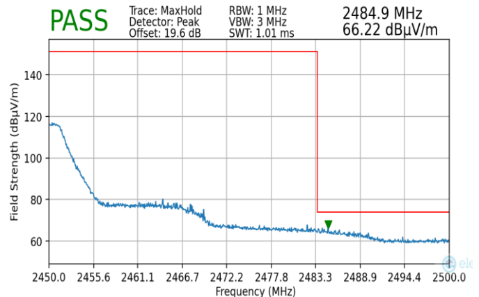
Plot 7-196. Radiated Restricted Upper Band Edge Measurement MIMO (Peak)
