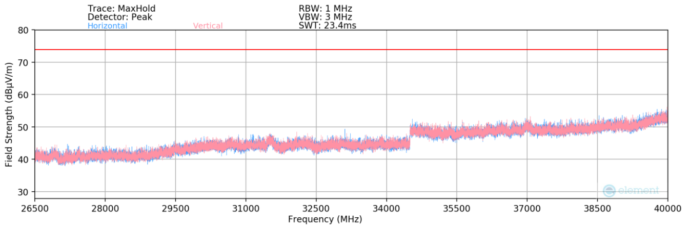
Plot 7-184. Radiated Spurious Plot above 26.5GHz (2.4GHz – 6GHz)
