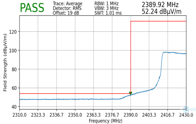
Plot 7-213. Radiated Restricted Lower Band Edge Measurement MIMO (Average)
