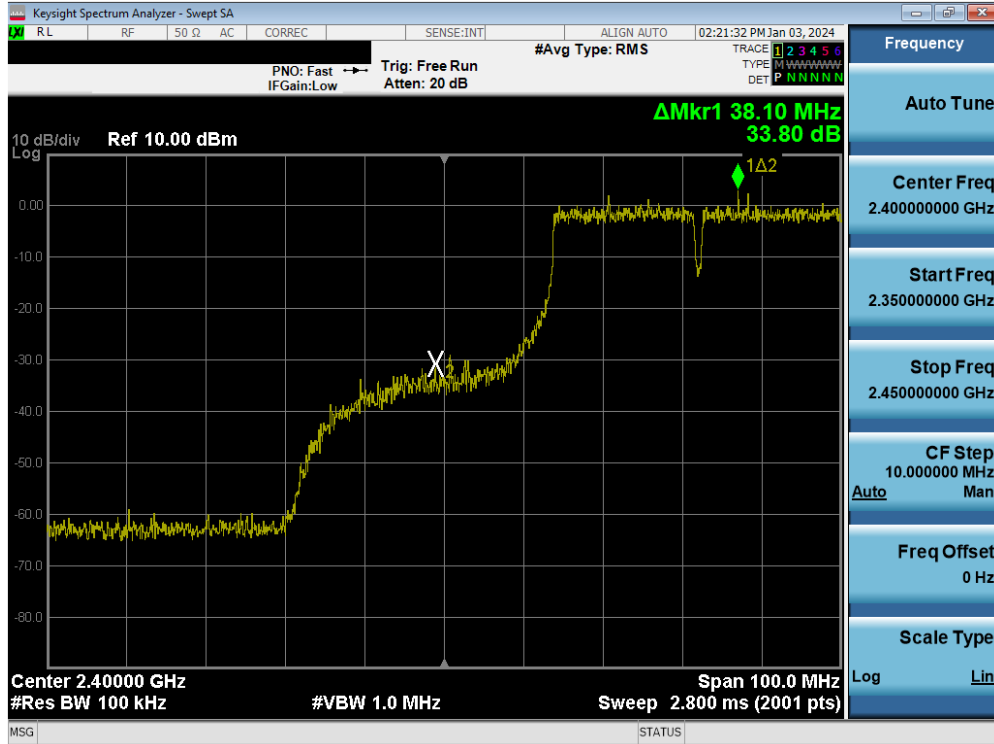
Plot 7-126. Band Edge Plot MIMO ANT1 (802.11n (2.4GHz) – Ch. 5)
