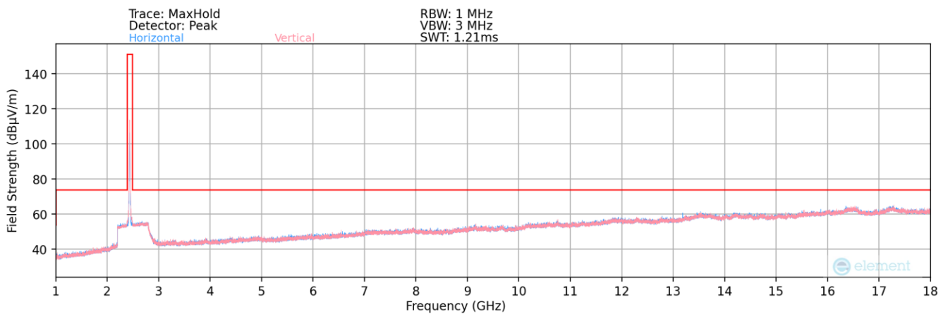
Plot 7-174. Radiated Spurious Plot above 1GHz MIMO (802.11b – Ch. 6)
