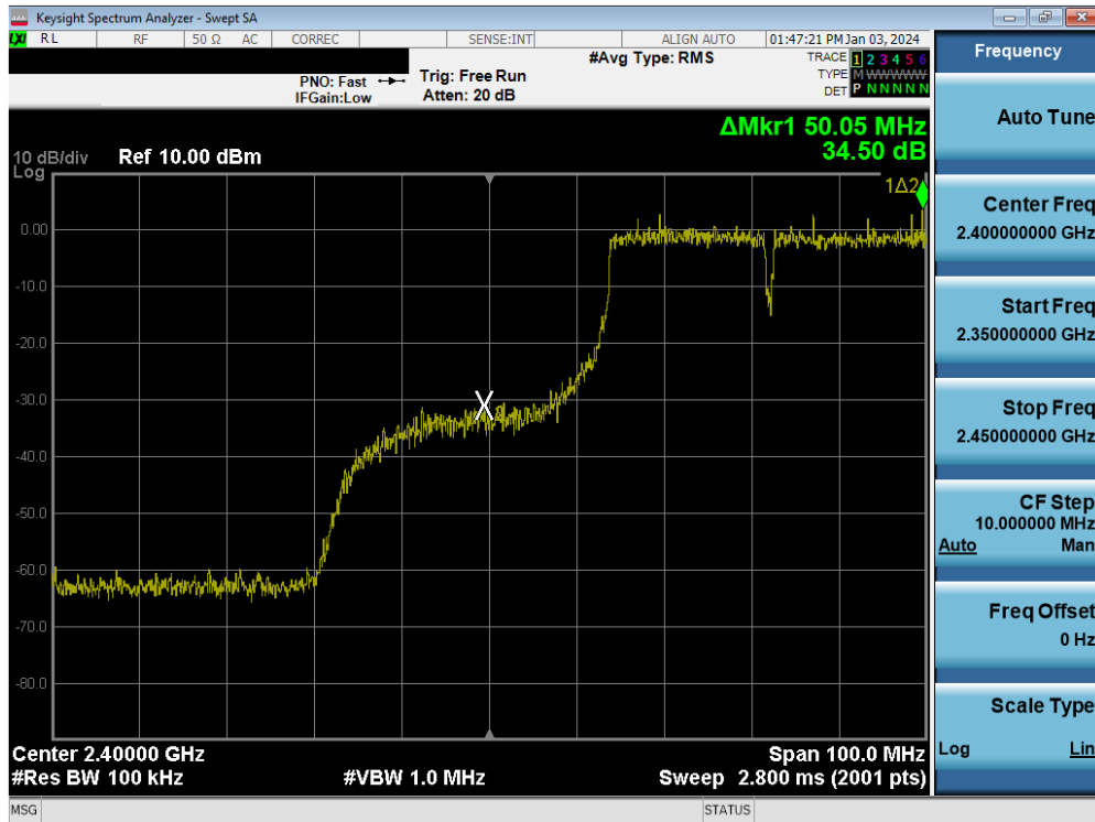
Plot 7-138. Band Edge Plot MIMO ANT2 (802.11n (2.4GHz) – Ch. 5)
