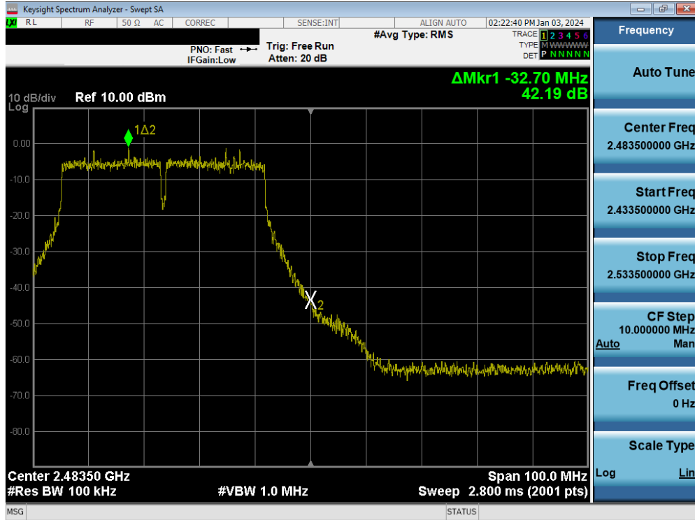
Plot 7-128. Band Edge Plot MIMO ANT1 (802.11n (2.4GHz) – Ch. 10)
