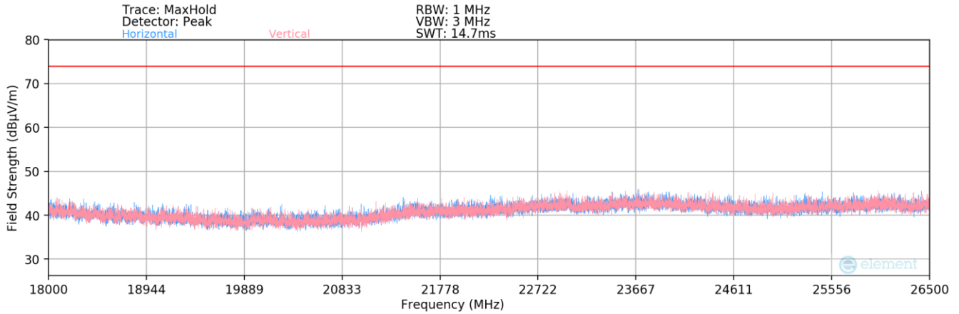
Plot 7-179. Radiated Spurious Plot 18GHz – 26.5GHz (2.4GHz – 5GHz)
