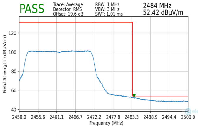
Plot 7-203. Radiated Restricted Upper Band Edge Measurement MIMO (Average)
