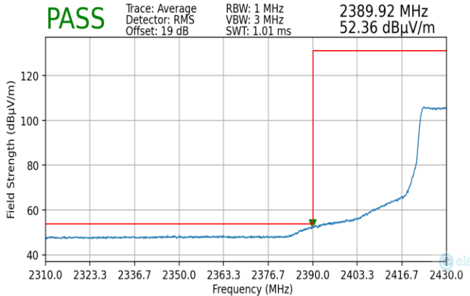
Plot 7-193. Radiated Restricted Lower Band Edge Measurement MIMO (Average)
