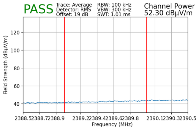
Plot 7-187. Radiated Restricted Lower Band Edge Measurement MIMO (Average)
