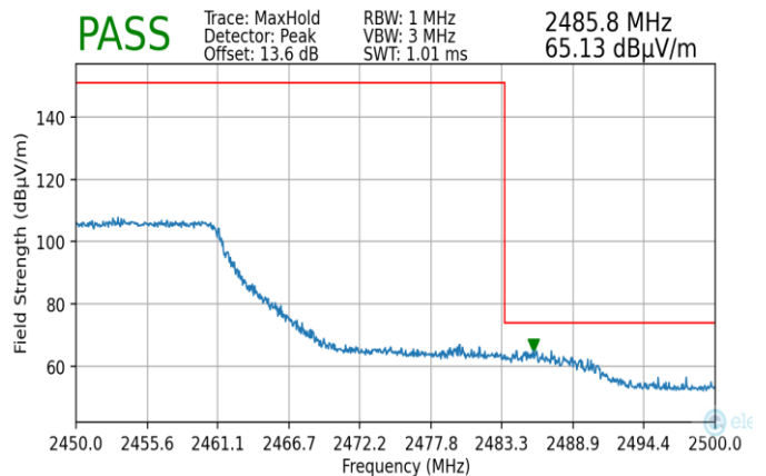
Plot 7-216. Radiated Restricted Upper Band Edge Measurement MIMO (Peak)
