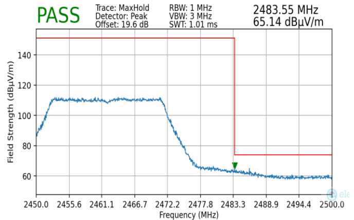
Plot 7-204. Radiated Restricted Upper Band Edge Measurement MIMO (Peak)
