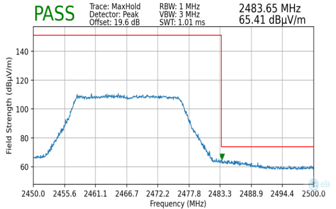
Plot 7-206. Radiated Restricted Upper Band Edge Measurement MIMO (Peak)
