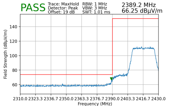
Plot 7-188. Radiated Restricted Lower Band Edge Measurement MIMO (Peak)
