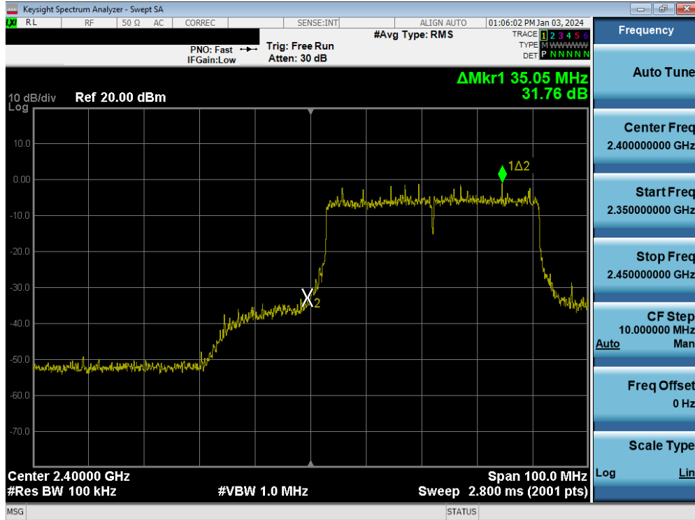
Plot 7-130. Band Edge Plot MIMO ANT1 (802.11be (2.4GHz) – Ch. 3)
