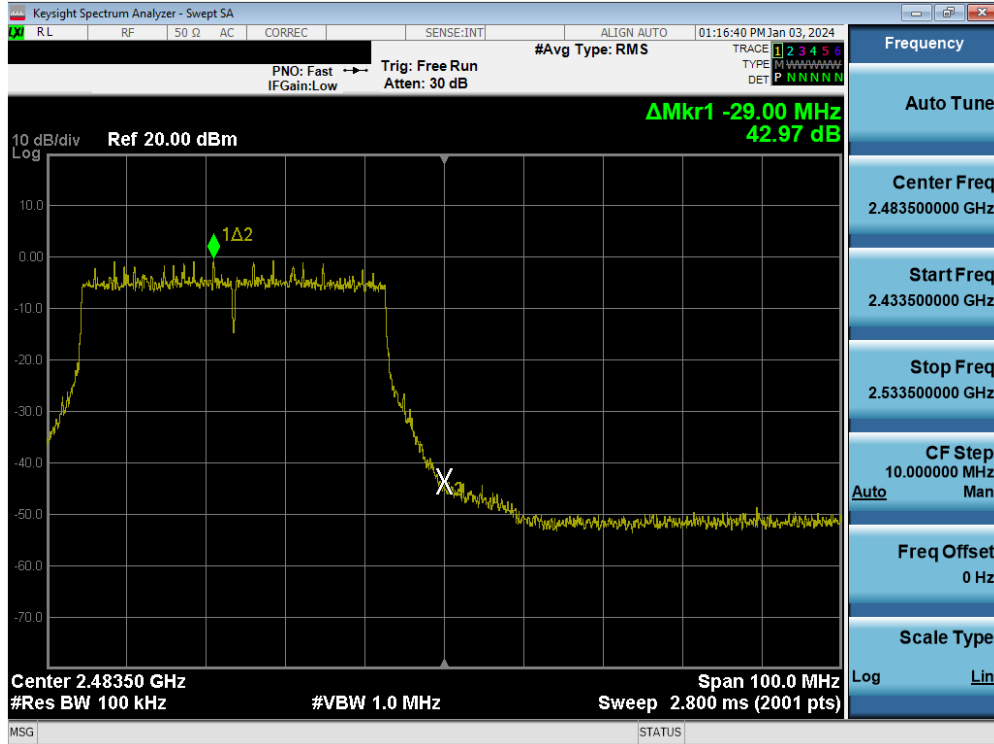
Plot 7-134. Band Edge Plot MIMO ANT1 (802.11be (2.4GHz) – Ch. 10)
