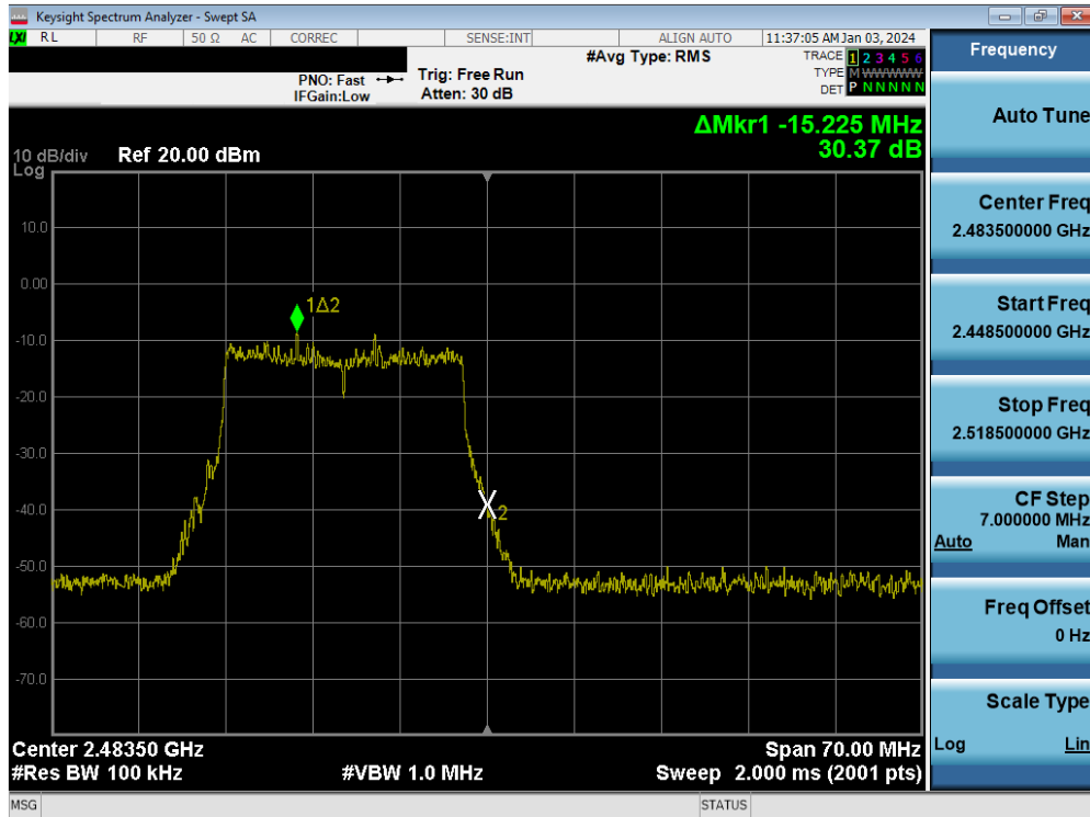
Plot 7-123. Band Edge Plot MIMO ANT2 (802.11be (2.4GHz) – Ch. 13)
