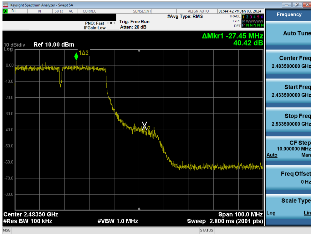
Plot 7-139. Band Edge Plot MIMO ANT2 (802.11n (2.4GHz) – Ch. 9)
