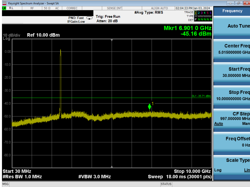
Plot 7-170. Conducted Spurious Plot MIMO ANT2 (802.11n – Ch. 11)
