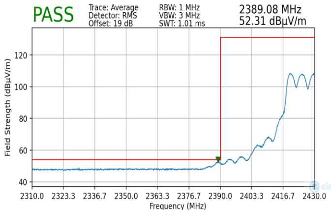
Plot 7-191. Radiated Restricted Lower Band Edge Measurement MIMO (Average)
