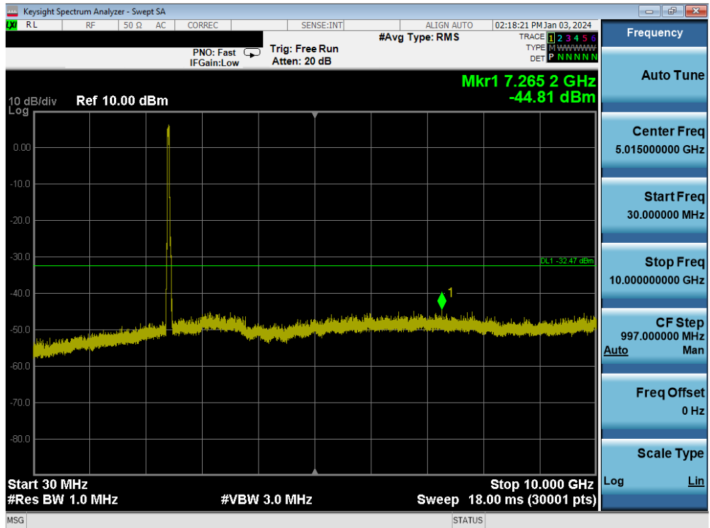
Plot 7-160. Conducted Spurious Plot MIMO ANT1 (802.11n – Ch. 3)
