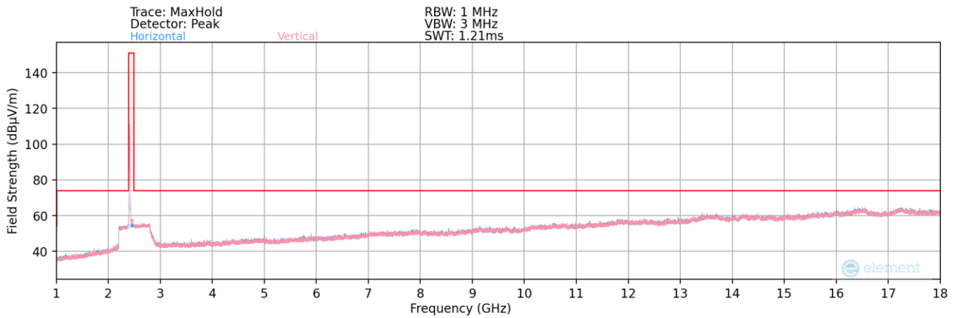
Plot 7-173. Radiated Spurious Plot above 1GHz MIMO (802.11b – Ch. 1)
