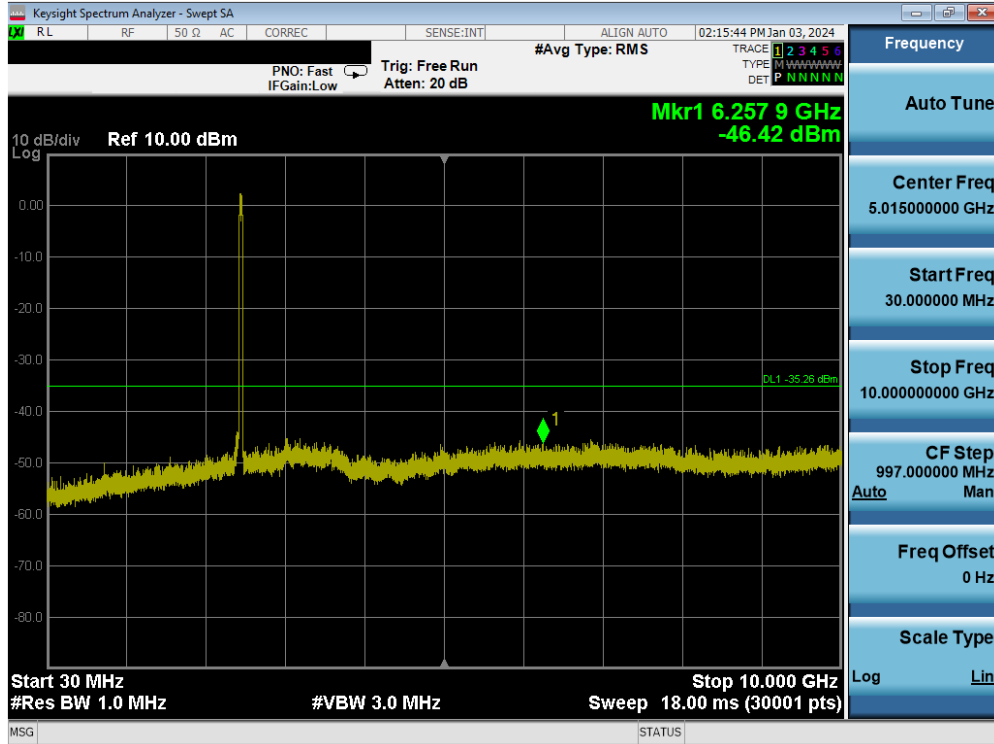
Plot 7-164. Conducted Spurious Plot MIMO ANT1 (802.11n – Ch. 11)
