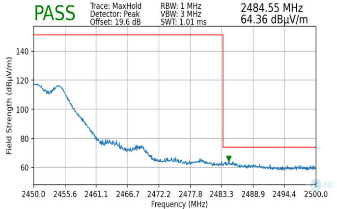
Plot 7-198. Radiated Restricted Upper Band Edge Measurement MIMO (Peak)
