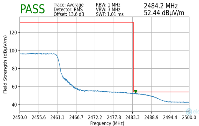
Plot 7-215. Radiated Restricted Upper Band Edge Measurement MIMO (Average)
