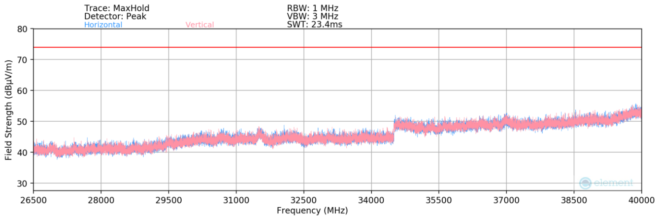
Plot 7-180. Radiated Spurious Plot above 26.5GHz (2.4GHz – 5GHz)
