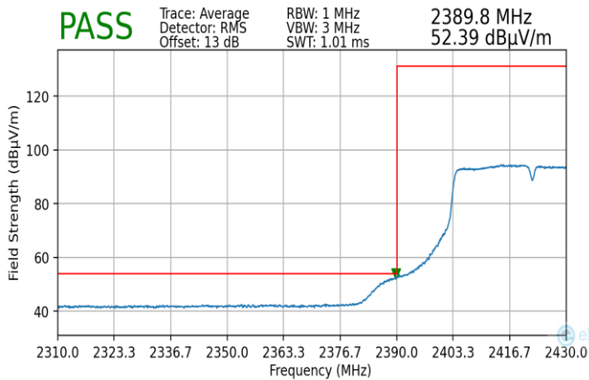
Plot 7-209. Radiated Restricted Lower Band Edge Measurement MIMO (Average)
