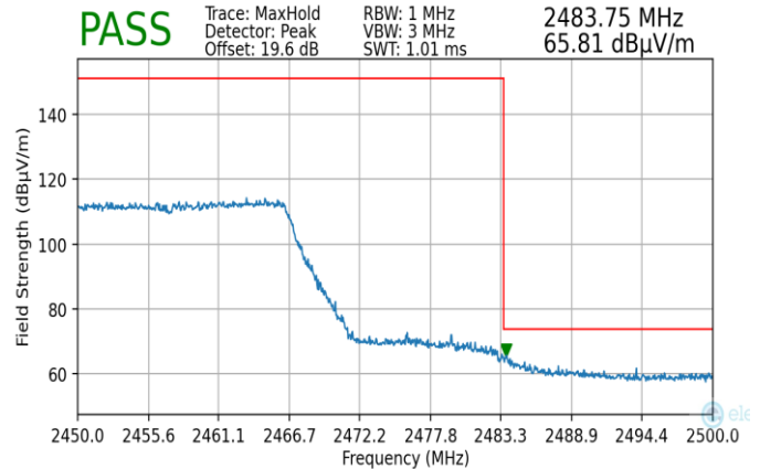
Plot 7-202. Radiated Restricted Upper Band Edge Measurement MIMO (Peak)
