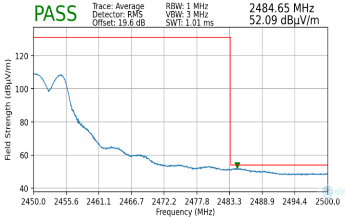
Plot 7-197. Radiated Restricted Upper Band Edge Measurement MIMO (Average)
