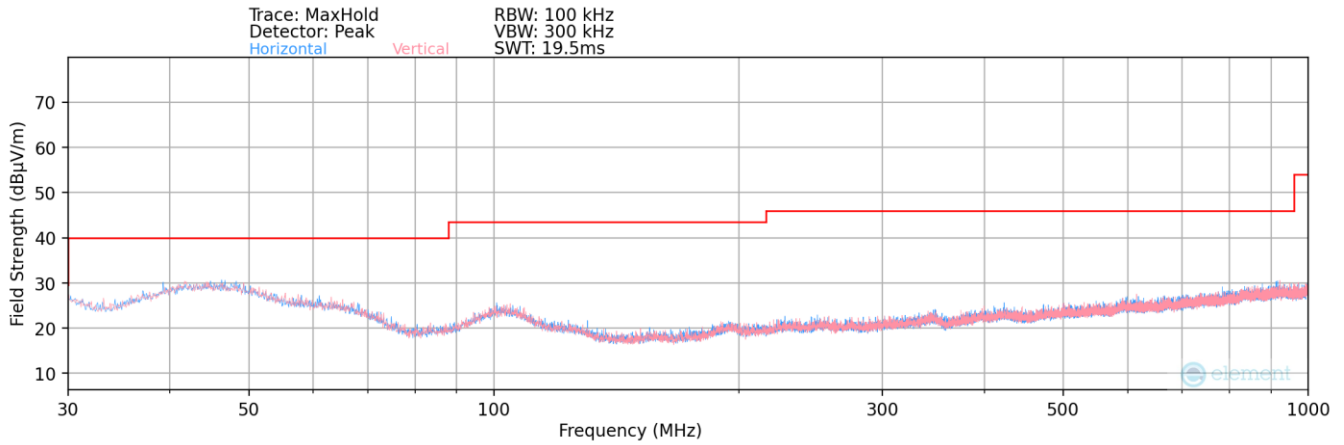
Plot 7-172. Radiated Spurious Plot below 1GHz MIMO
