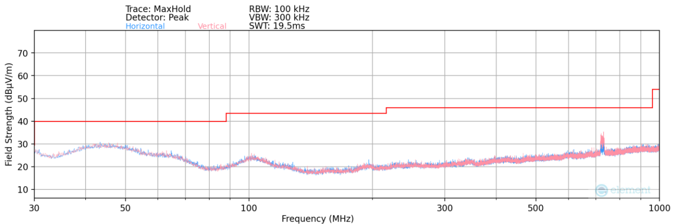
Plot 7-177. Radiated Spurious Plot below 1GHz (2.4GHz – 5GHz)
