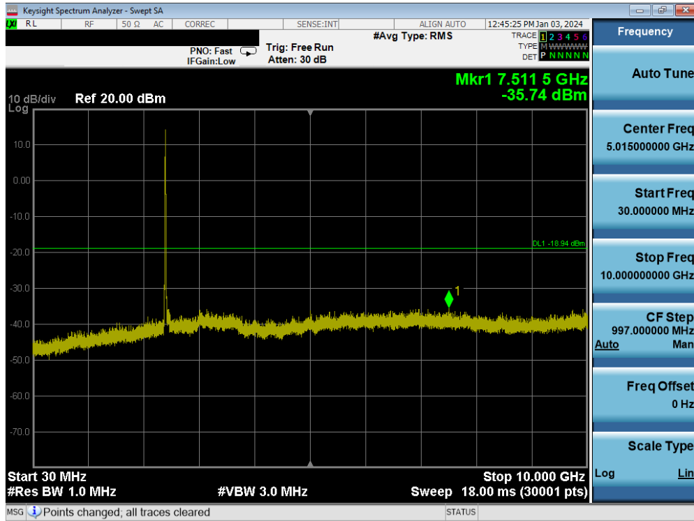
Plot 7-148. Conducted Spurious Plot MIMO ANT1 (802.11b – Ch. 1)
