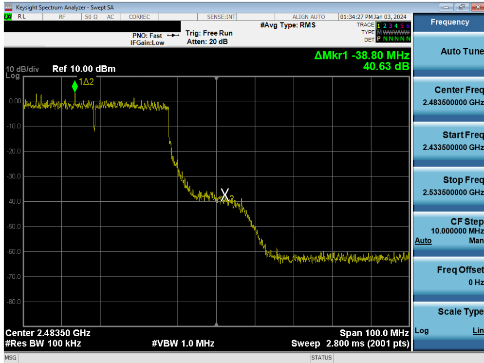
Plot 7-145. Band Edge Plot MIMO ANT2 (802.11be (2.4GHz) – Ch. 9)
