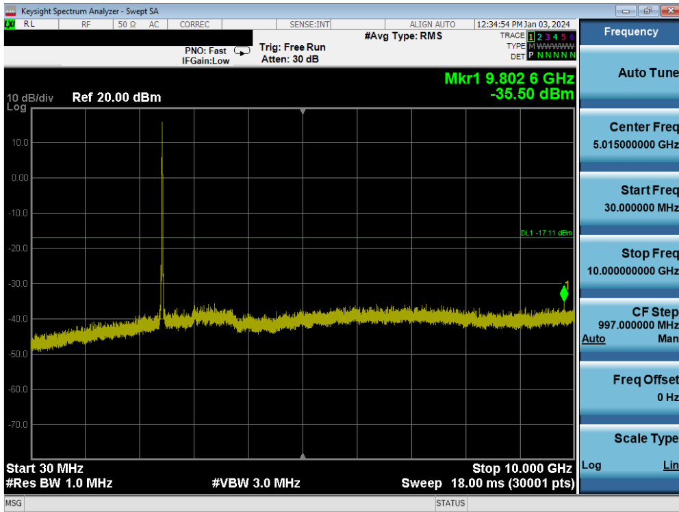
Plot 7-156. Conducted Spurious Plot MIMO ANT2 (802.11b – Ch. 6)
