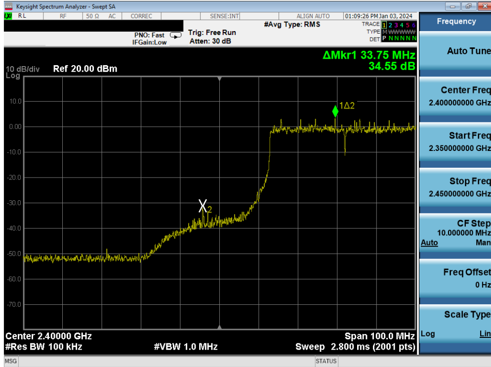
Plot 7-132. Band Edge Plot MIMO ANT1 (802.11be (2.4GHz) – Ch. 5)
