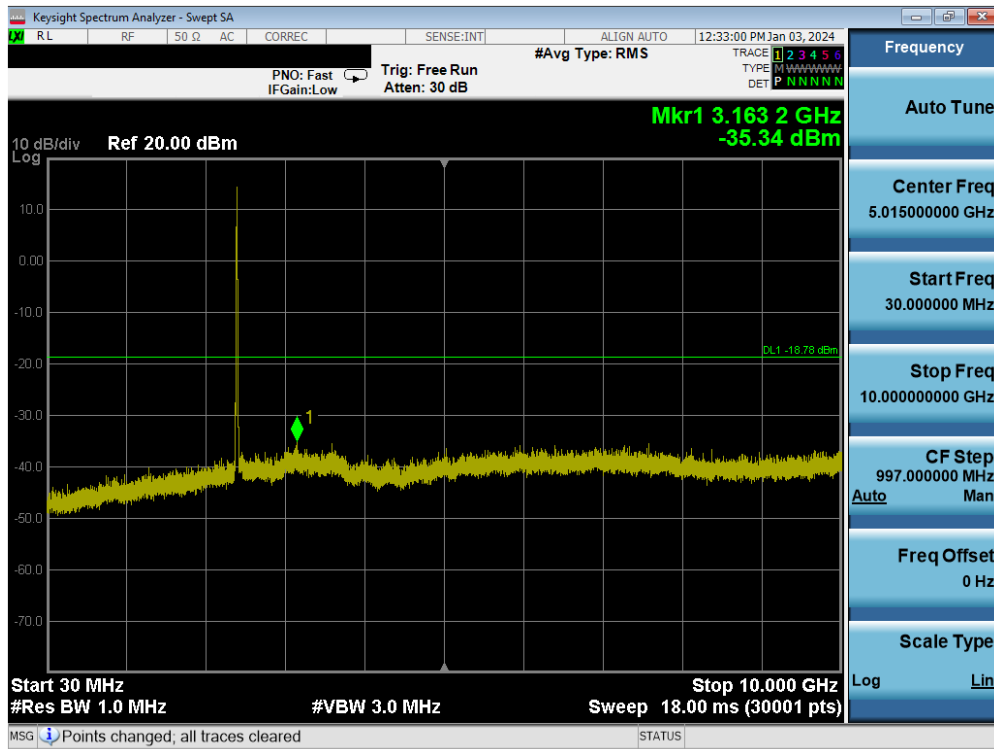
Plot 7-154. Conducted Spurious Plot MIMO ANT2 (802.11b – Ch. 1)
