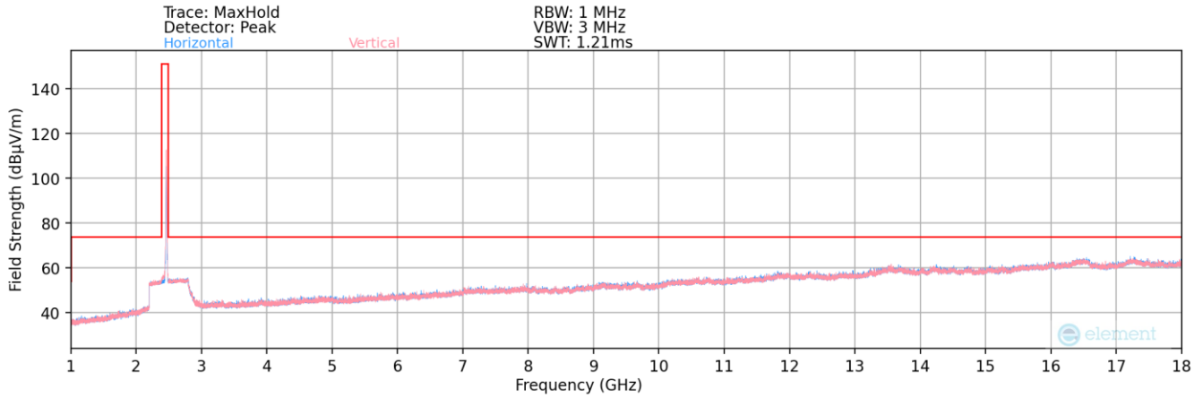
Plot 7-175. Radiated Spurious Plot above 1GHz MIMO (802.11b – Ch. 11)
