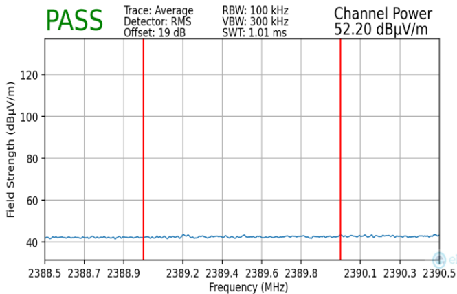
Plot 7-211. Radiated Restricted Lower Band Edge Measurement MIMO (Average)
