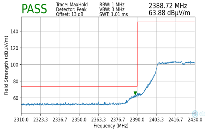
Plot 7-210. Radiated Restricted Lower Band Edge Measurement MIMO (Peak)
