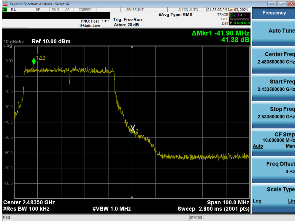
Plot 7-146. Band Edge Plot MIMO ANT2 (802.11be (2.4GHz) – Ch. 10)
