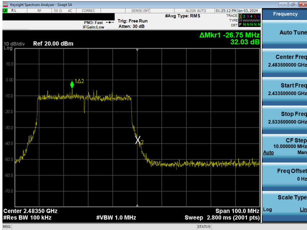
Plot 7-147. Band Edge Plot MIMO ANT2 (802.11be (2.4GHz) – Ch. 11)
