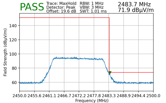
Plot 7-208. Radiated Restricted Upper Band Edge Measurement MIMO (Peak)
