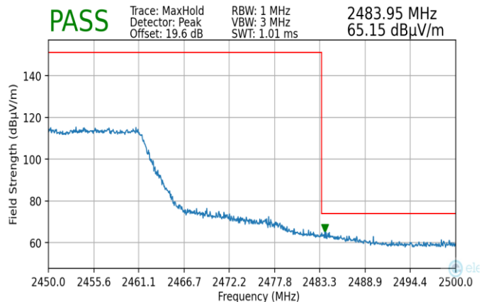
Plot 7-200. Radiated Restricted Upper Band Edge Measurement MIMO (Peak)
