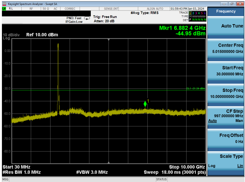
Plot 7-166. Conducted Spurious Plot MIMO ANT2 (802.11n – Ch. 3)
