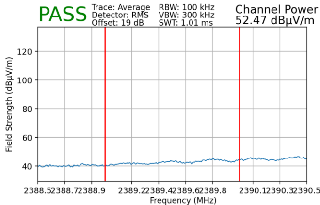
Plot 7-185. Radiated Restricted Lower Band Edge Measurement MIMO (Average)
