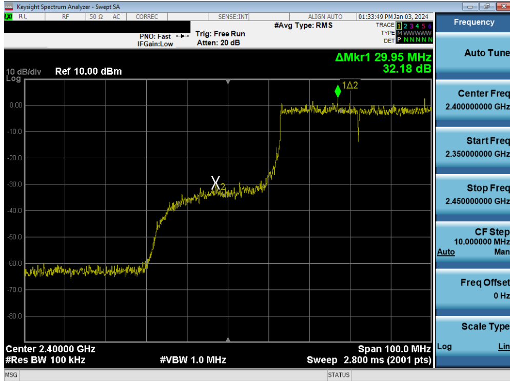
Plot 7-144. Band Edge Plot MIMO ANT2 (802.11be (2.4GHz) – Ch. 5)
