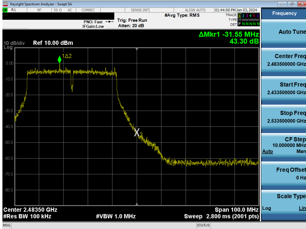
Plot 7-140. Band Edge Plot MIMO ANT2 (802.11n (2.4GHz) – Ch. 10)
