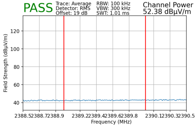
Plot 7-189. Radiated Restricted Lower Band Edge Measurement MIMO (Average)
