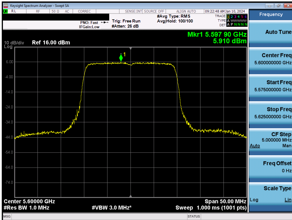
Plot 7-152. Power Spectral Density Plot MIMO ANT2 (20MHz BW 802.11be – 242 Tones (UNII Band 2C) – Ch. 120)
