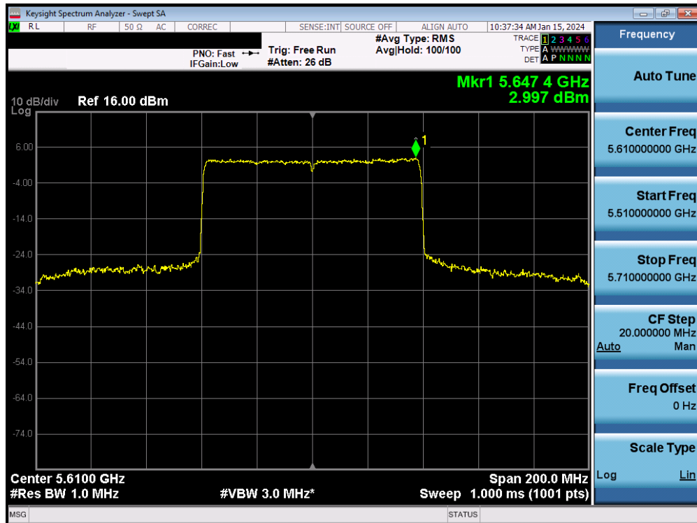
Plot 7-154. Power Spectral Density Plot MIMO ANT2 (80MHz BW 802.11be – 996 Tones (UNII Band 2C) – Ch. 122)
