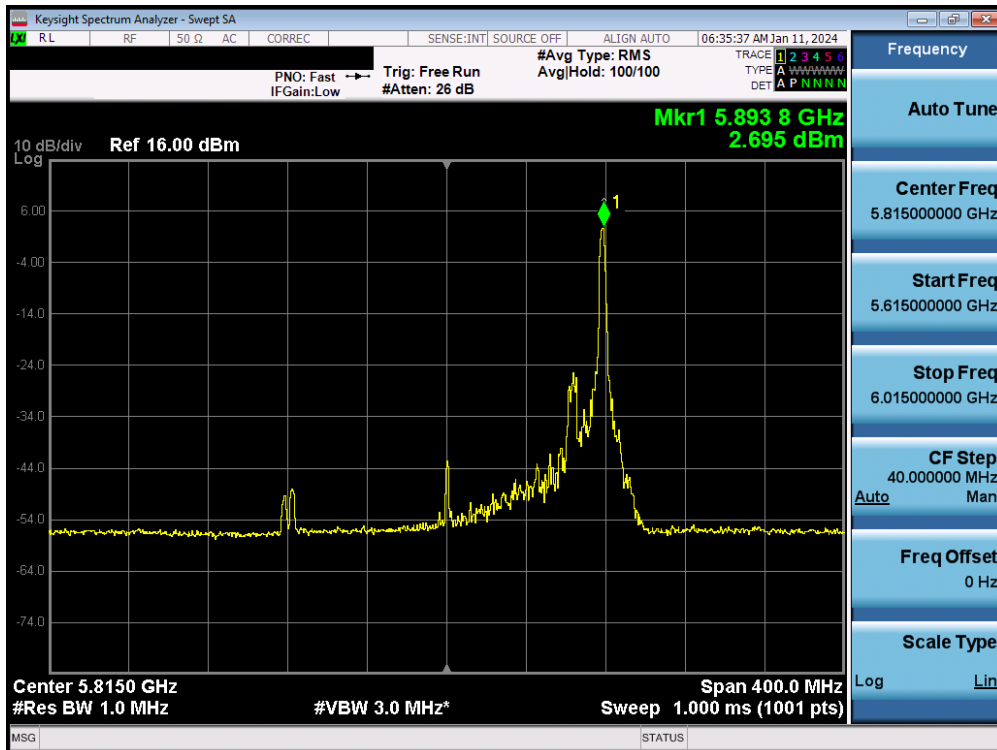
Plot 7-144. Power Spectral Density Plot MIMO ANT2 (160MHz(U) BW 802.11be – 26 Tones (UNII Band 3/4) – Ch. 163)
