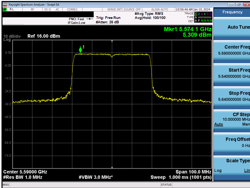
Plot 7-153. Power Spectral Density Plot MIMO ANT2 (40MHz BW 802.11be – 484 Tones (UNII Band 2C) – Ch. 118)
