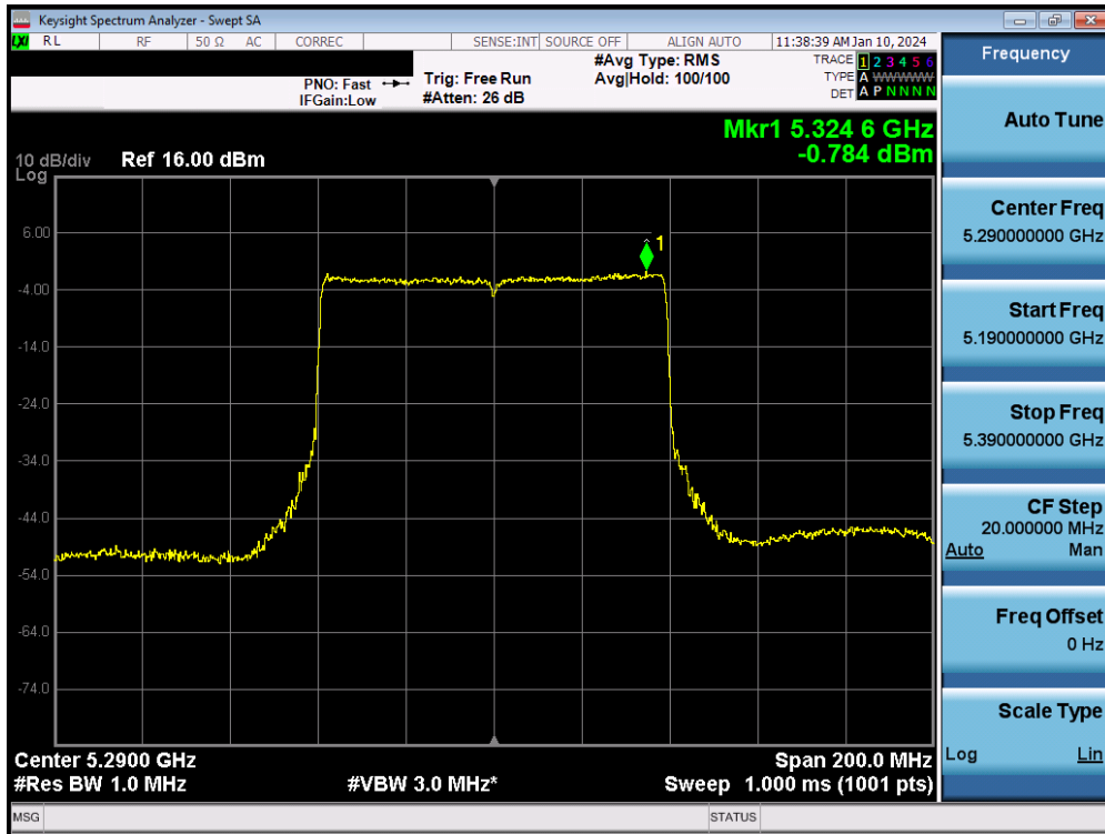
Plot 7-151. Power Spectral Density Plot MIMO ANT2 (80MHz BW 802.11be – 996 Tones (UNII Band 2A) – Ch. 58)
