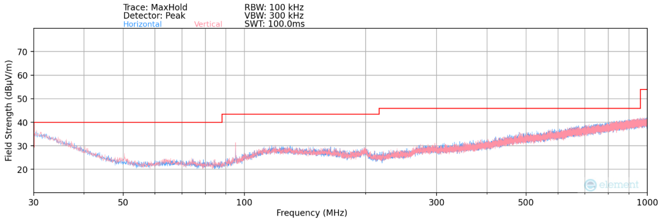
Plot 7-179. Radiated Spurious Plot below 1GHz MIMO (802.11a)
