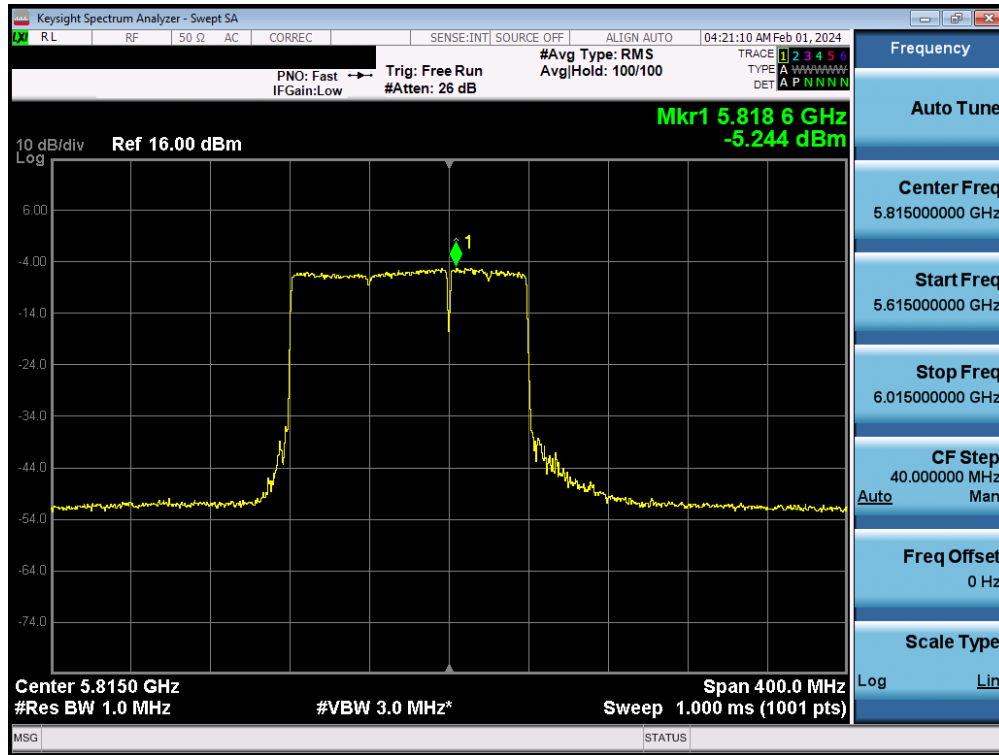
Plot 7-178. Power Spectral Density Plot MIMO ANT2 (160MHz BW 802.11be (UNII Band 3/4) – Ch. 163)
