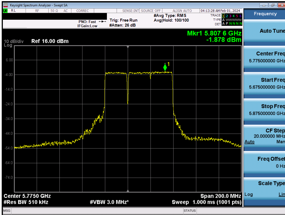
Plot 7-176. Power Spectral Density Plot MIMO ANT2 (80MHz BW 802.11be (UNII Band 3) – Ch. 155)
