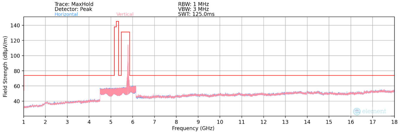
Plot 7-183. Radiated Spurious Plot above 1GHz MIMO (802.11a – UNII Band 3 Ch. 157)
