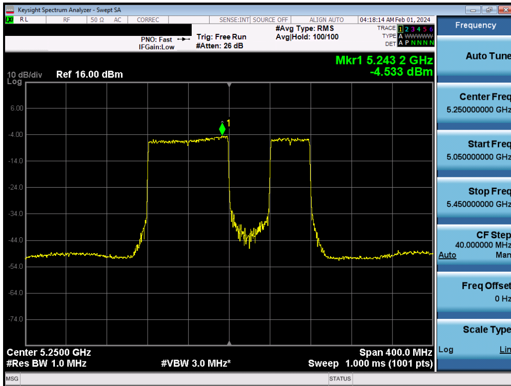
Plot 7-173. Power Spectral Density Plot MIMO ANT2 (160MHz BW 802.11be (UNII Band 1/2A) – Ch. 50)
