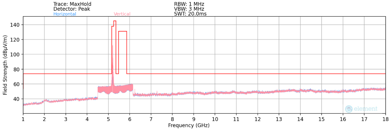
Plot 7-180. Radiated Spurious Plot above 1GHz MIMO (802.11a – UNII Band 1 Ch. 40)
