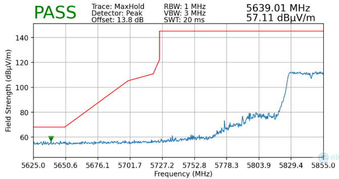
Plot 7-204. Radiated Lower Band Edge Plot MIMO (Peak – UNII Band 4)
