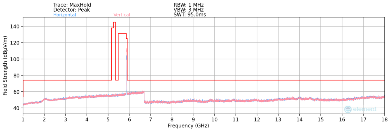
Plot 7-184. Radiated Spurious Plot above 1GHz MIMO (802.11a – UNII Band 4 Ch. 173)
