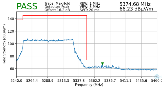
Plot 7-210. Radiated Upper Band Edge Plot MIMO (Peak – UNII Band 2A)
