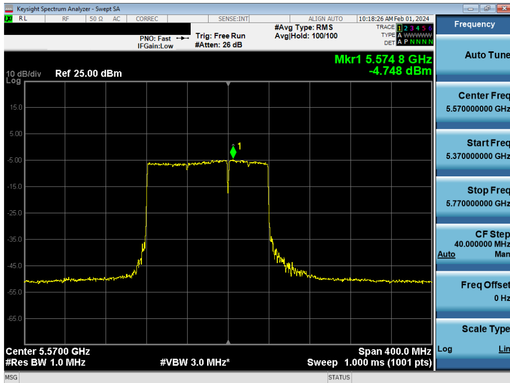
Plot 7-168. Power Spectral Density Plot MIMO ANT1 (160MHz BW 802.11be (UNII Band 2C) – Ch. 114)
