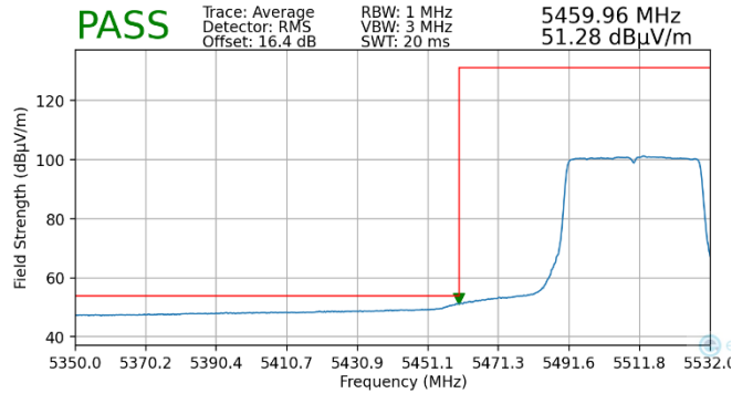
Plot 7-201. Radiated Lower Band Edge Plot MIMO (Average – UNII Band 2C)
