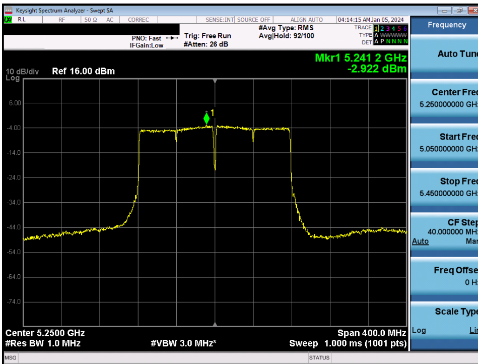
Plot 7-131. Power Spectral Density Plot MIMO ANT2 (160MHz BW 802.11ac (UNII Band 1/2A) – Ch. 50)
