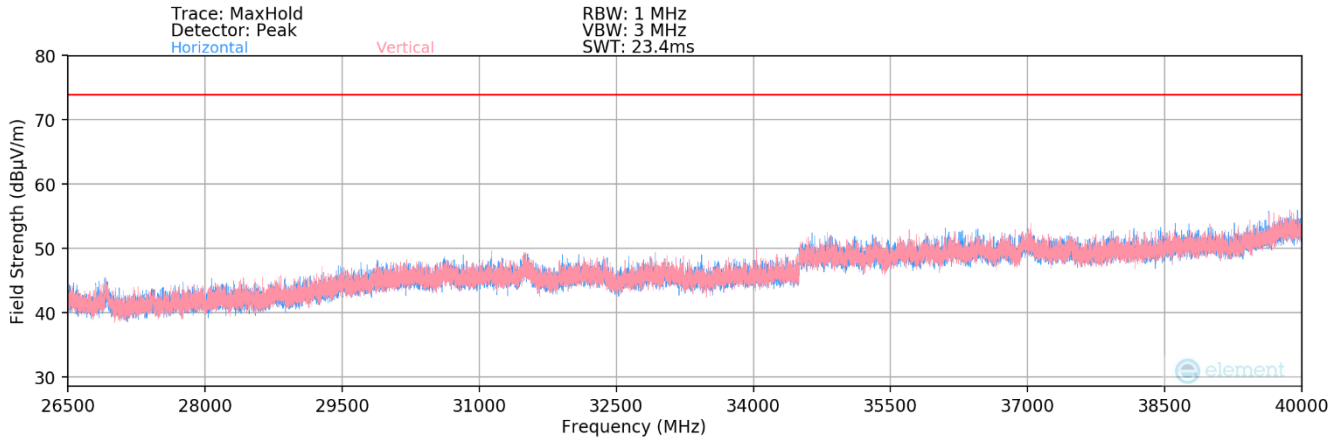
Plot 7-186. Radiated Spurious Plot 26.5GHz – 40GHz MIMO (802.11a)
