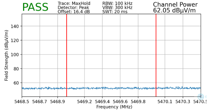
Plot 7-202. Radiated Lower Band Edge Plot MIMO (Peak – UNII Band 2C)
