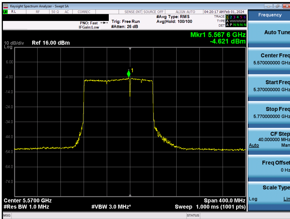
Plot 7-175. Power Spectral Density Plot MIMO ANT2 (160MHz BW 802.11be (UNII Band 2C) – Ch. 114)
