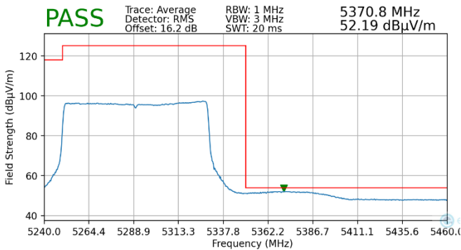
Plot 7-209. Radiated Upper Band Edge Plot MIMO (Average – UNII Band 2A)
