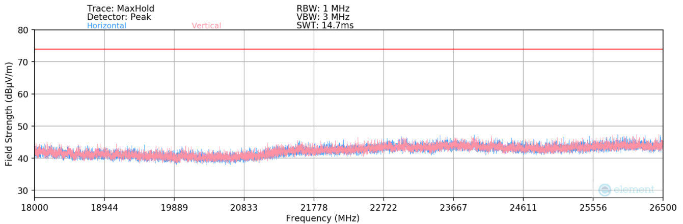
Plot 7-185. Radiated Spurious Plot 18GHz – 26.5GHz MIMO (802.11a)
