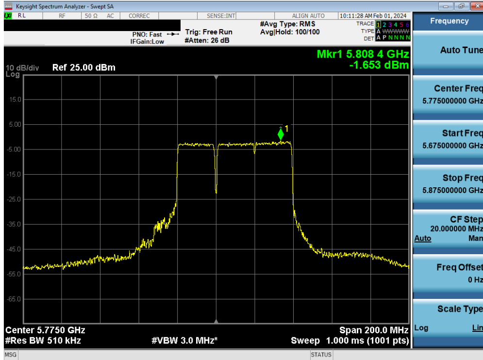
Plot 7-169. Power Spectral Density Plot MIMO ANT1 (80MHz BW 802.11be (UNII Band 3) – Ch. 155)
