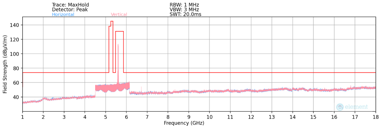
Plot 7-182. Radiated Spurious Plot above 1GHz MIMO (802.11a – UNII Band 2C Ch. 120)
