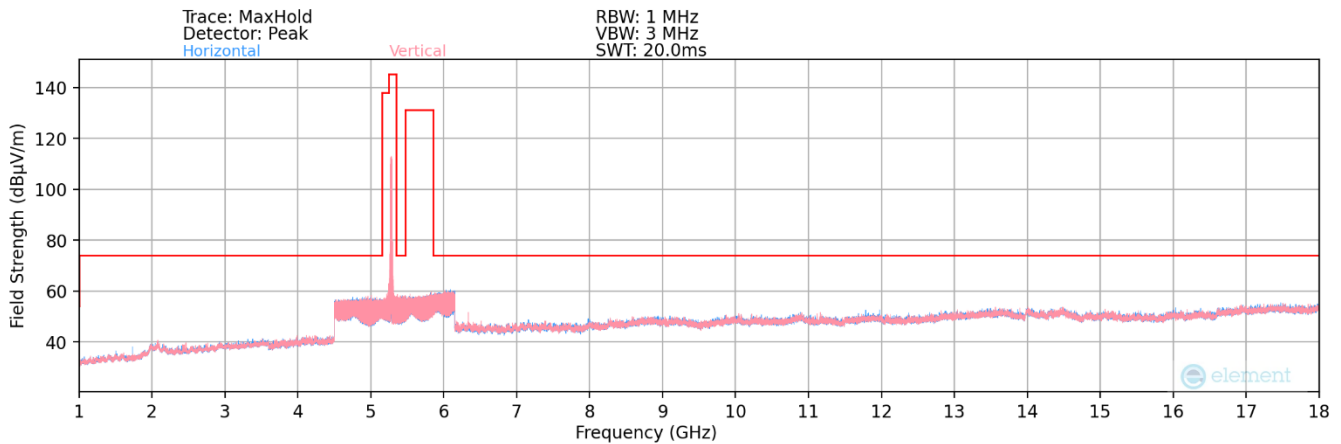
Plot 7-181. Radiated Spurious Plot above 1GHz MIMO (802.11a – UNII Band 2A Ch. 56)
