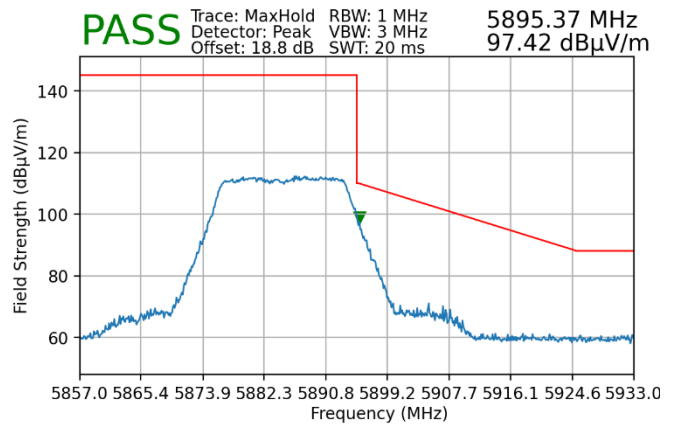
Plot 7-196. Radiated Upper Band Edge Plot MIMO (Peak – UNII Band 4)
