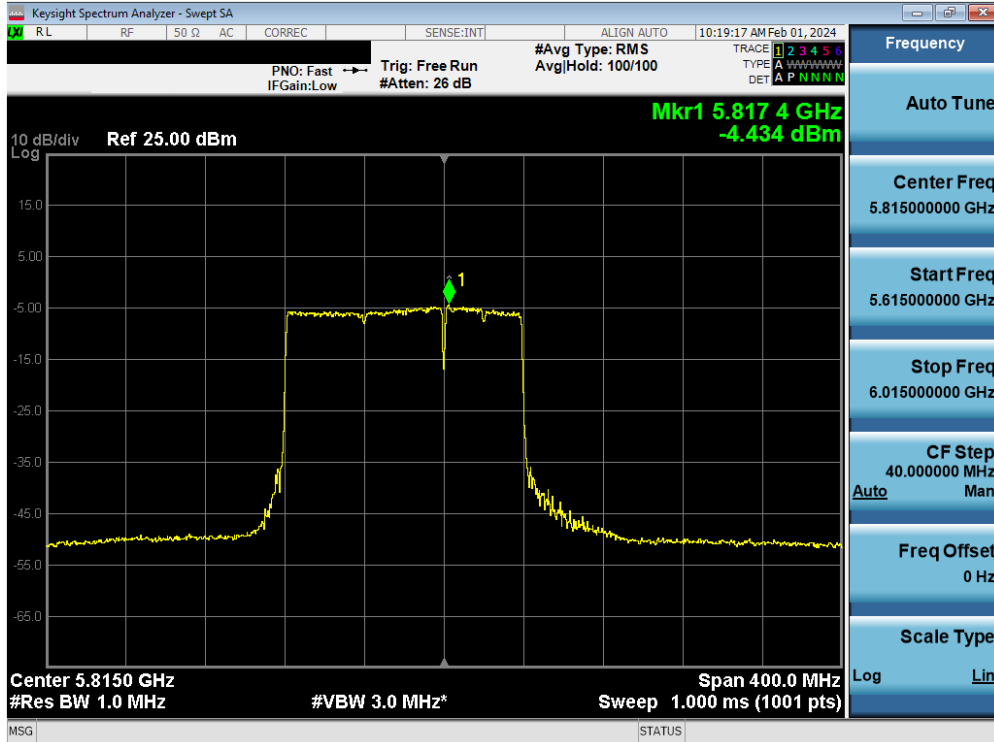
Plot 7-171. Power Spectral Density Plot MIMO ANT1 (160MHz BW 802.11be (UNII Band 3/4) – Ch. 163)
