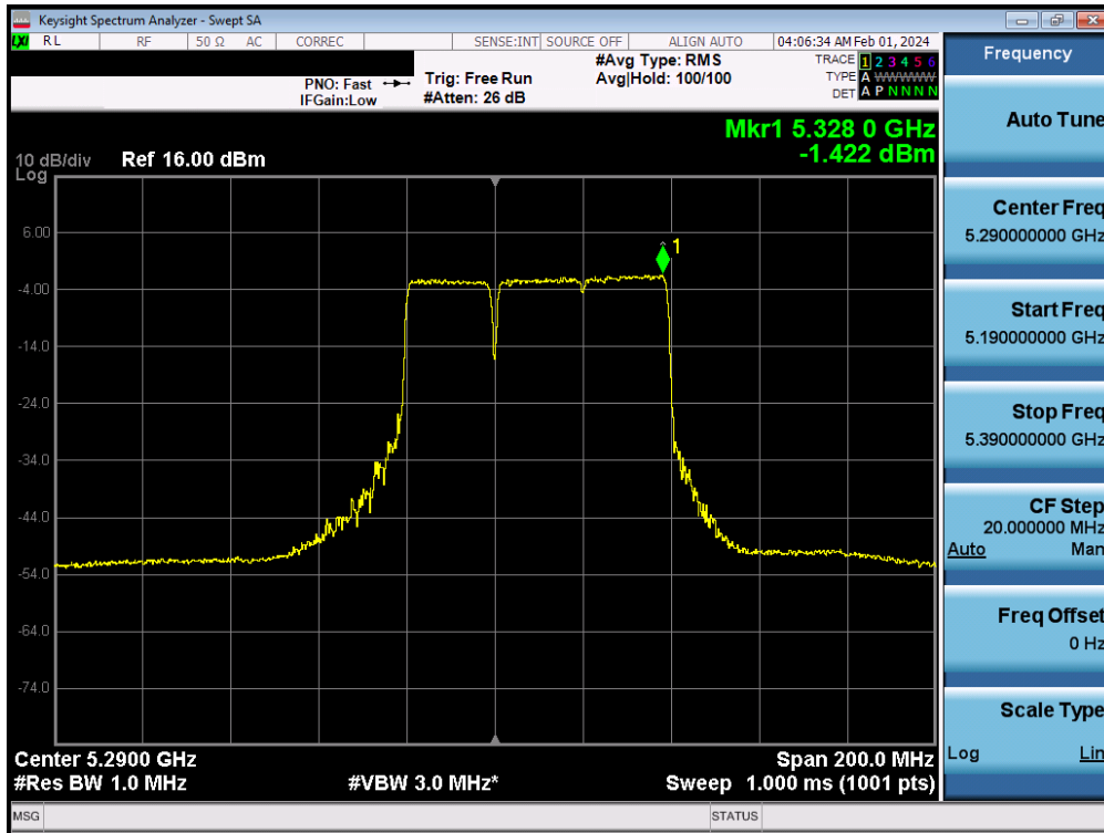
Plot 7-174. Power Spectral Density Plot MIMO ANT2 (80MHz BW 802.11be (UNII Band 2A) – Ch. 58)
