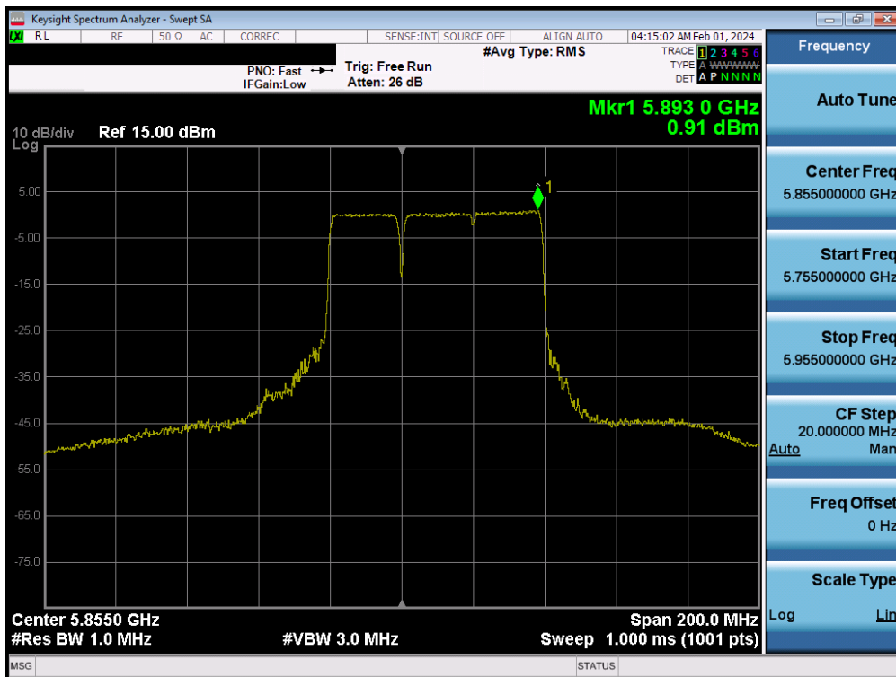
Plot 7-177. Power Spectral Density Plot MIMO ANT2 (80MHz BW 802.11be (UNII Band 3/4) – Ch. 171)
