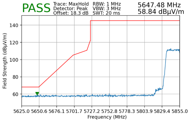
Plot 7-194. Radiated Lower Band Edge Plot MIMO (Peak – UNII Band 4)
