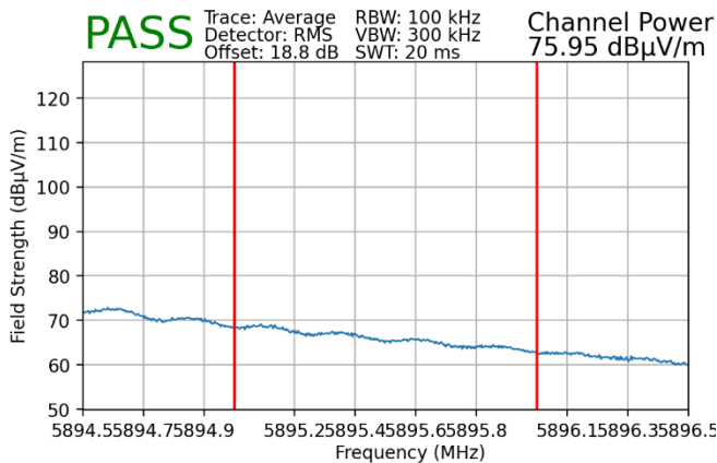
Plot 7-195. Radiated Upper Band Edge Plot MIMO (Average – UNII Band 4)
