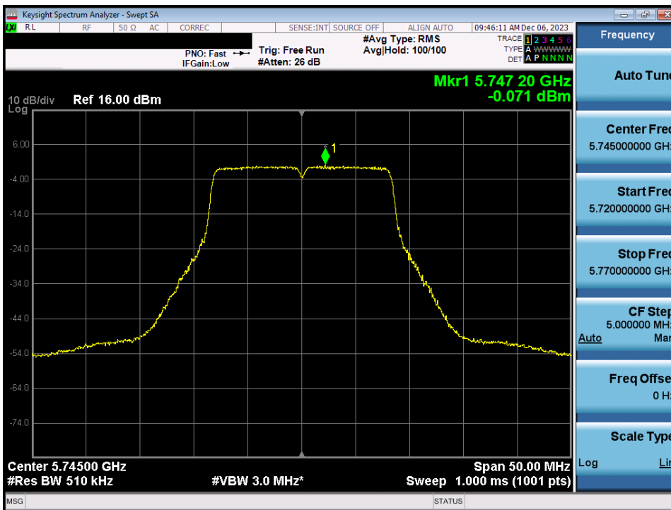
Plot 7-108. Power Spectral Density Plot MIMO ANT1 (802.11a (UNII Band 3) – Ch. 149)
