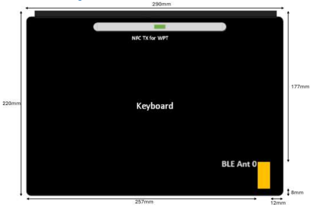
Fig. 1 – Antenna Position Diagram
