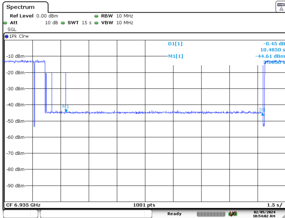
Plot 7-395. Contention Based Protocol Timing Plot (20MHz (UNII Band 8) – Ch. 197)
