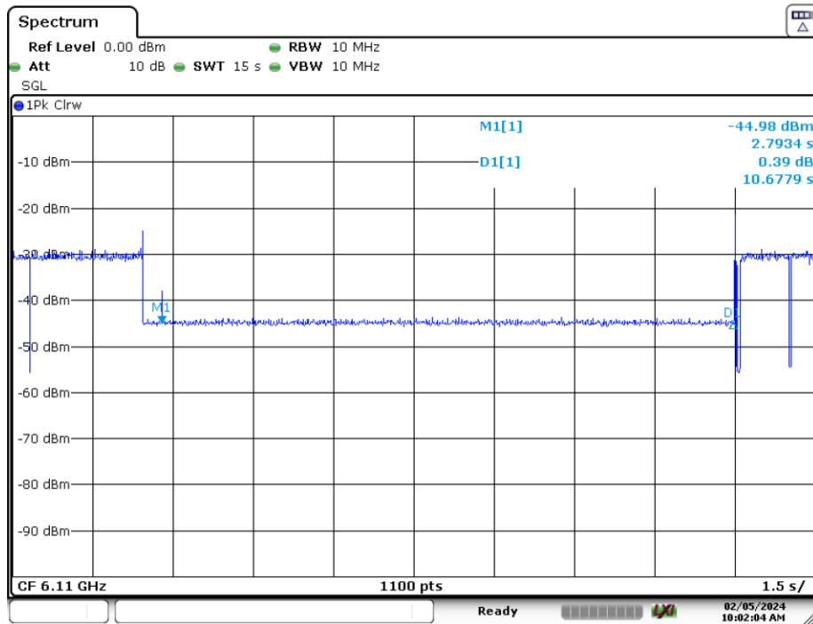
Plot 7-384. Contention Based Protocol Timing Plot (320MHz (UNII Band 5) – Ch. 31 Low)
