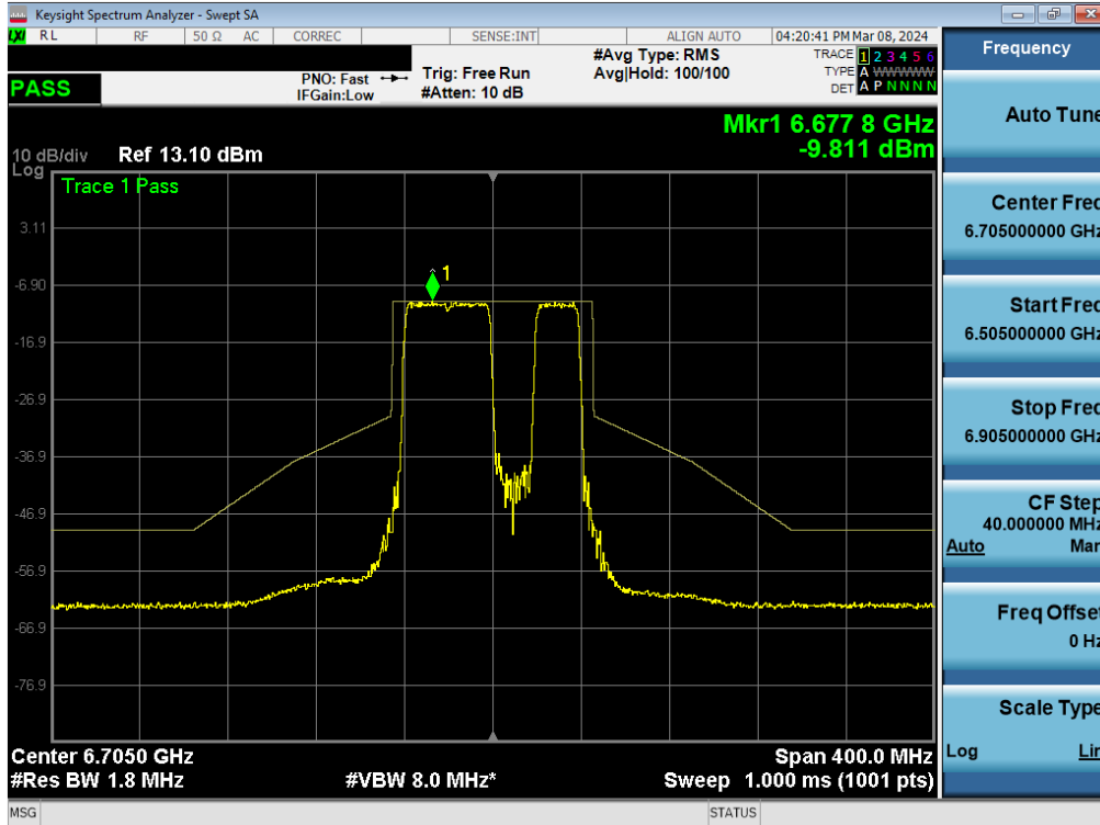
Plot 7-352. In-Band Emission Plot MIMO ANT2 (80MHz BW 802.11be (484+242 Tone) (UNII Band 7) – Ch. 151)
