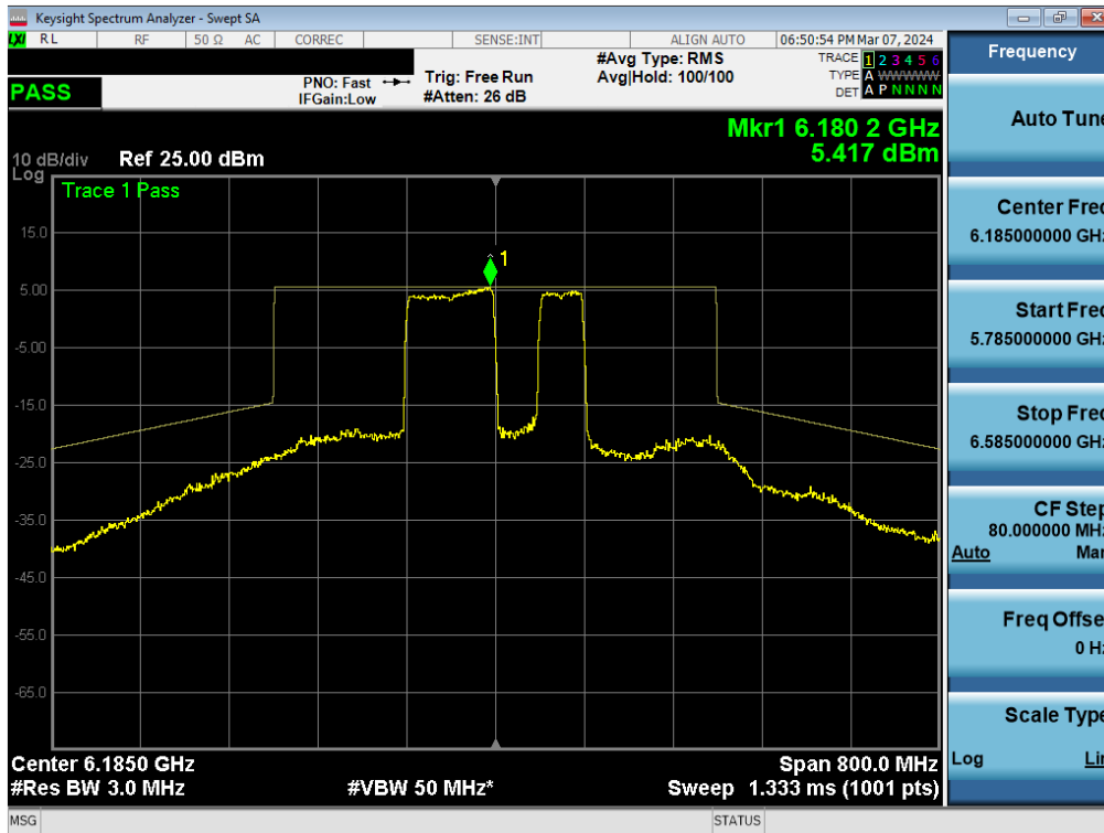
Plot 7-378. In-Band Emission Plot MIMO ANT2 (160MHz BW 802.11be (996+484 Tone) (UNII Band 5) – Ch. 47) - SP
