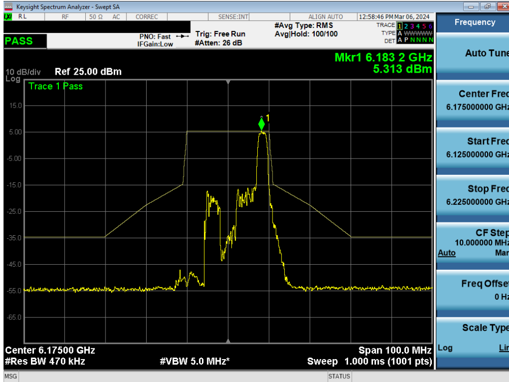
Plot 7-358. In-Band Emission Plot MIMO ANT1 (20MHz BW 802.11be (26 Tones) (UNII Band 5) – Ch. 45) - SP
