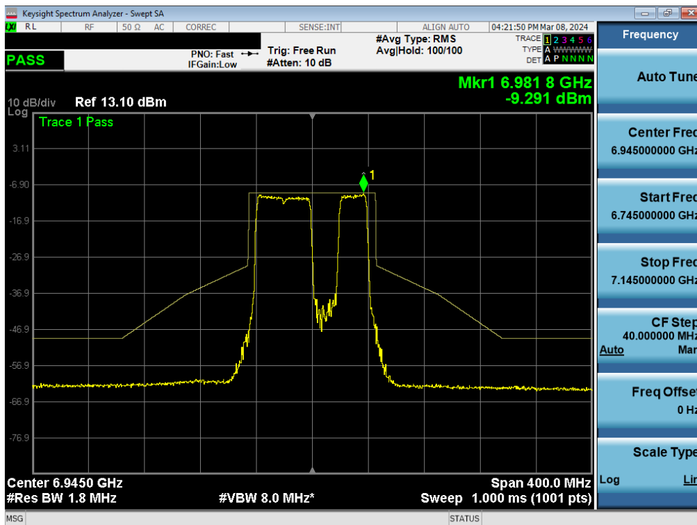
Plot 7-355. In-Band Emission Plot MIMO ANT2 (80MHz BW 802.11be (484+242 Tone) (UNII Band 8) – Ch. 199)
