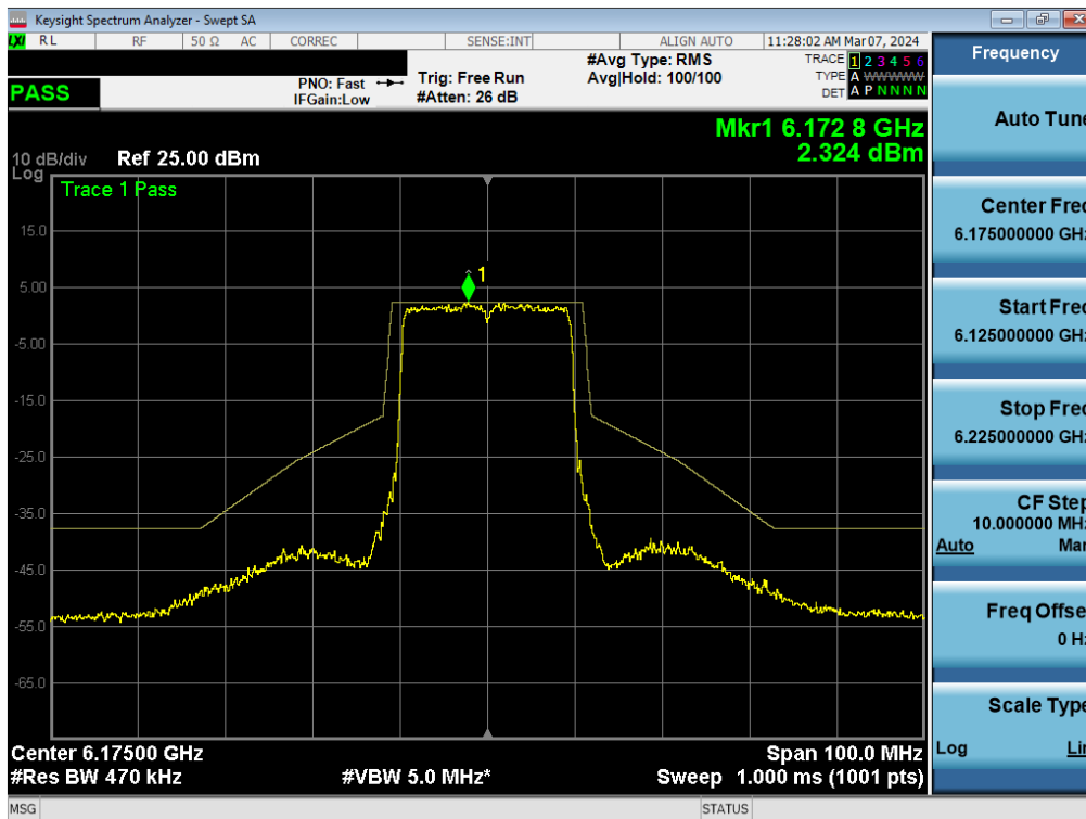
Plot 7-367. In-Band Emission Plot MIMO ANT1 (20MHz BW 802.11be (Full Tones) (UNII Band 5) – Ch. 45) - SP
