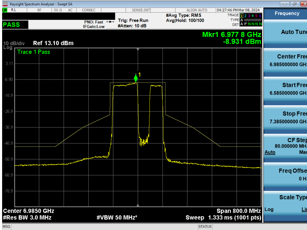
Plot 7-356. In-Band Emission Plot MIMO ANT2 (160MHz BW 802.11be (996+484 Tone) (UNII Band 8) – Ch. 207)
