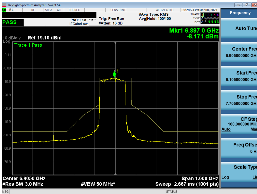
Plot 7-357. In-Band Emission Plot MIMO ANT2 (320MHz BW 802.11be (2*996+484 Tone) (UNII Band 8) – Ch. 191)
