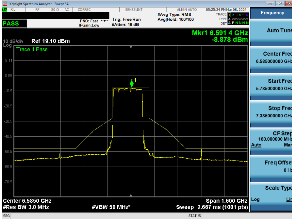
Plot 7-354. In-Band Emission Plot MIMO ANT2 (320MHz BW 802.11be (2*996+484 Tone) (UNII Band 7) – Ch. 127)
