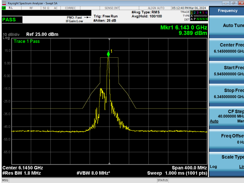
Plot 7-360. In-Band Emission Plot MIMO ANT1 (80MHz BW 802.11be (26 Tones) (UNII Band 5) – Ch. 39) - SP
