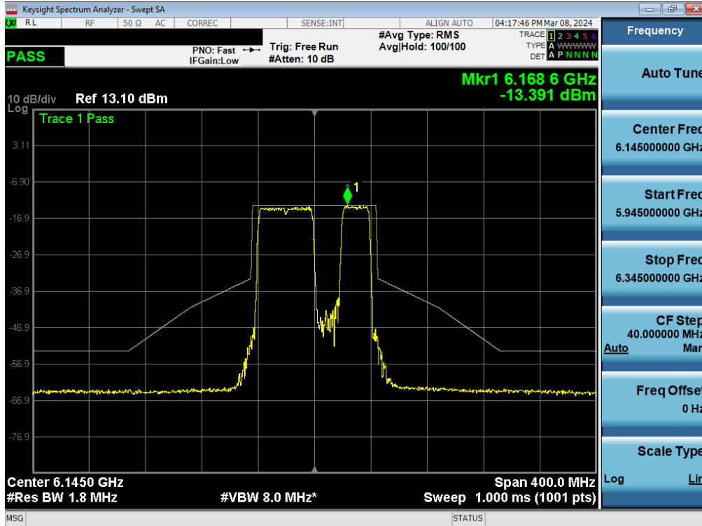
Plot 7-346. In-Band Emission Plot MIMO ANT2 (80MHz BW 802.11be (484+242 Tone) (UNII Band 5) – Ch. 39)
