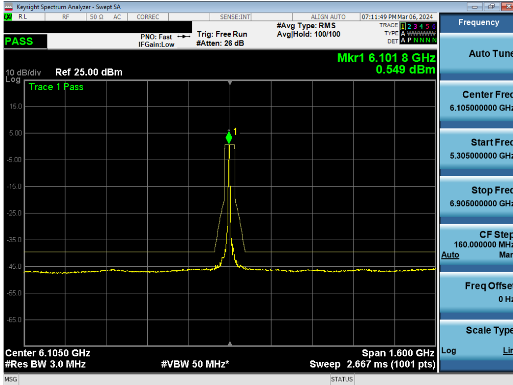
Plot 7-362. In-Band Emission Plot MIMO ANT1 (320MHz BW 802.11be (26 Tones) (UNII Band 5) – Ch. 31) – SP
