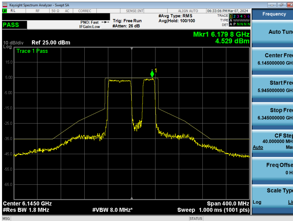
Plot 7-377. In-Band Emission Plot MIMO ANT2 (80MHz BW 802.11be (484+242 Tone) (UNII Band 5) – Ch. 39) - SP
