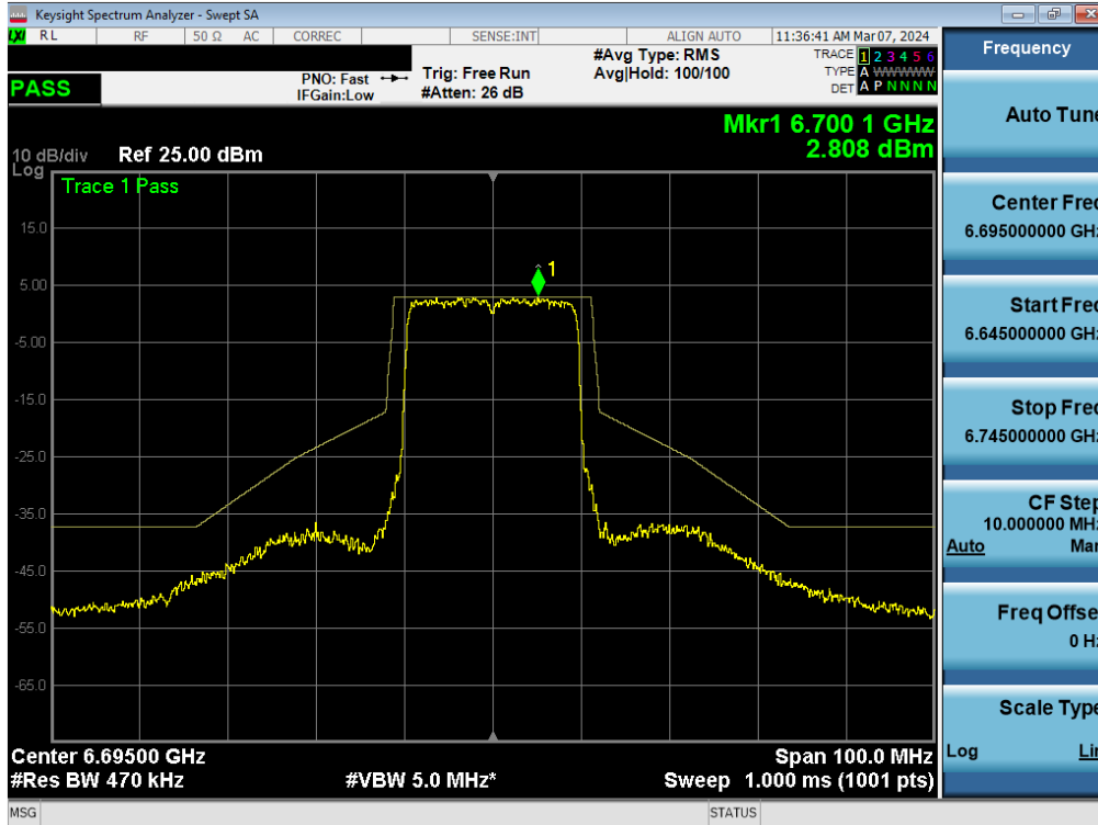
Plot 7-372. In-Band Emission Plot MIMO ANT1 (20MHz BW 802.11be (Full Tone) (UNII Band 7) – Ch. 149) – SP
