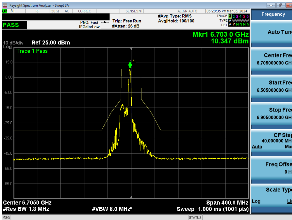
Plot 7-365. In-Band Emission Plot MIMO ANT1 (80MHz BW 802.11be (26 Tone) (UNII Band 7) – Ch. 151) – SP
