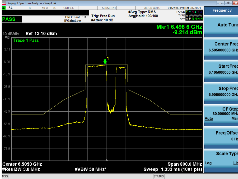
Plot 7-350. In-Band Emission Plot MIMO ANT2 (160MHz BW 802.11be (996+484 Tone) (UNII Band 6) – Ch. 111)
