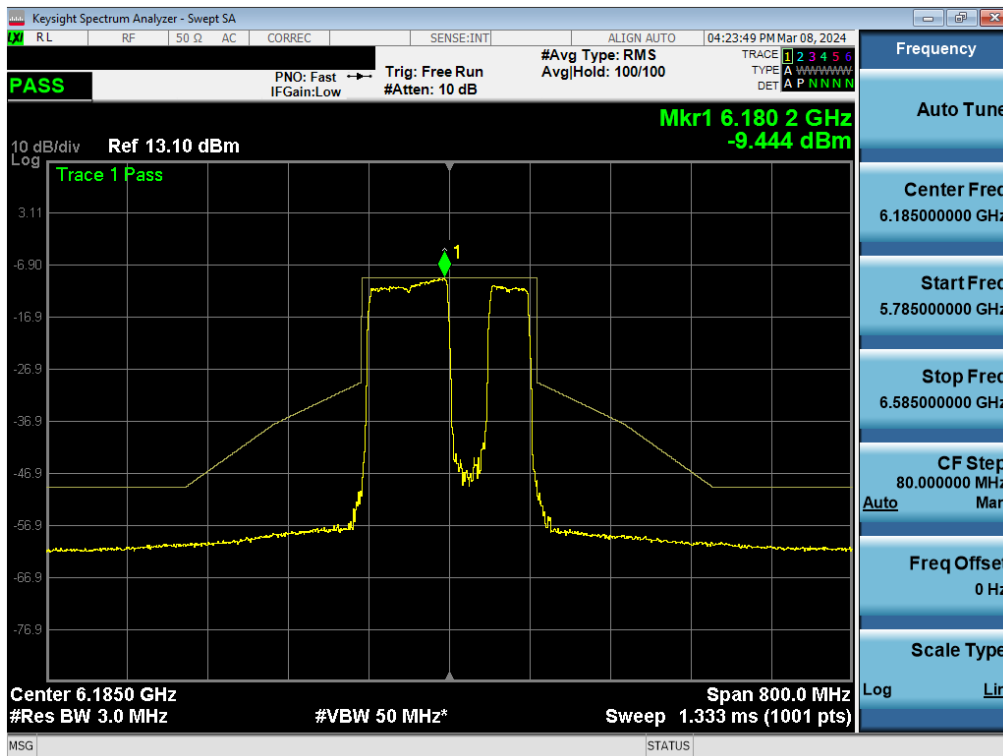
Plot 7-347. In-Band Emission Plot MIMO ANT2 (160MHz BW 802.11be (996+484 Tone) (UNII Band 5) – Ch. 47)
