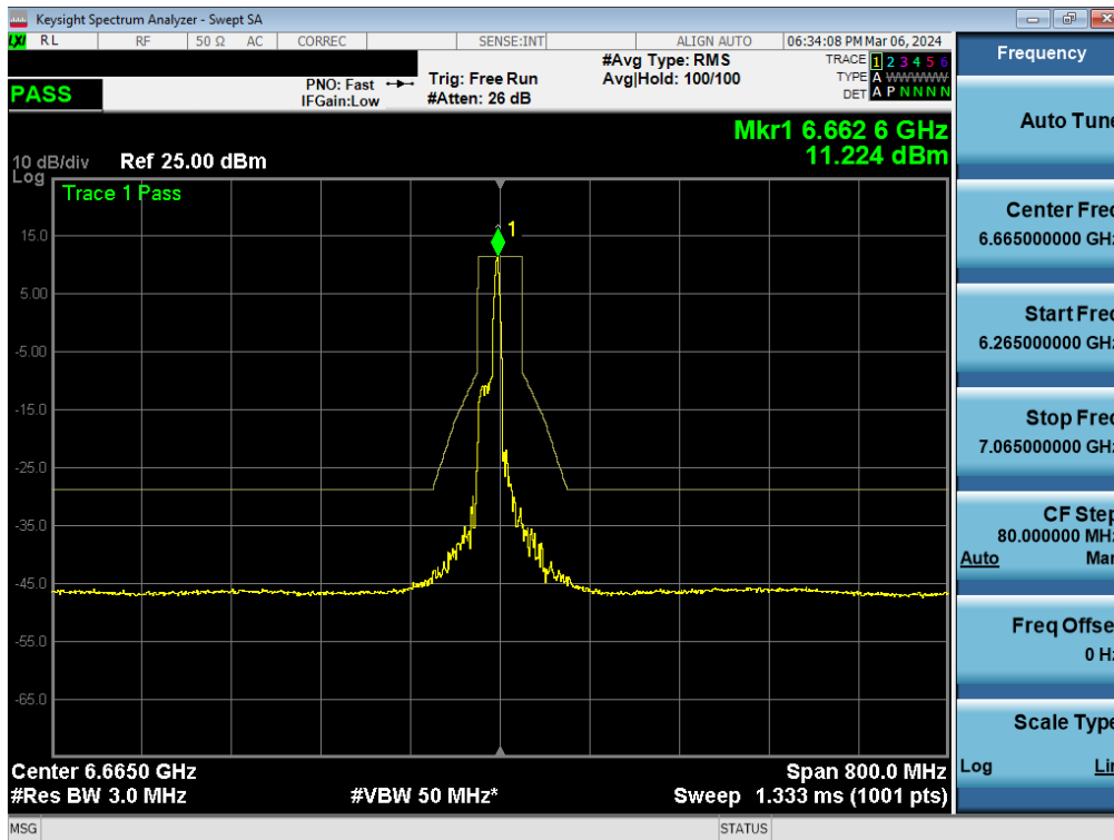
Plot 7-366. In-Band Emission Plot MIMO ANT1 (160MHz BW 802.11be (26 Tone) (UNII Band 7) – Ch. 143) – SP
