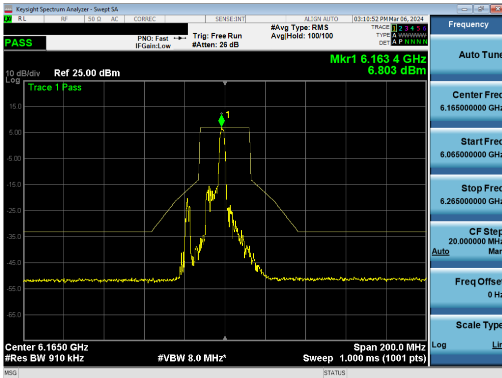
Plot 7-359. In-Band Emission Plot MIMO ANT1 (40MHz BW 802.11be (26 Tones) (UNII Band 5) – Ch. 43) - SP
