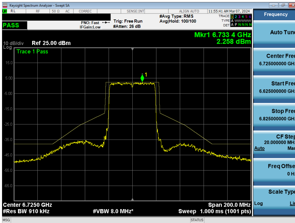
Plot 7-373. In-Band Emission Plot MIMO ANT1 (40MHz BW 802.11be (Full Tone) (UNII Band 7) – Ch. 155) – SP
