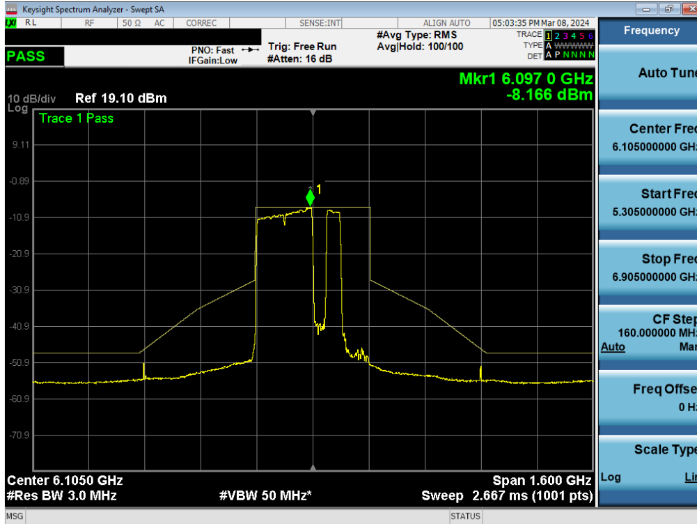
Plot 7-348. In-Band Emission Plot MIMO ANT2 (320MHz BW 802.11be (2*996+484 Tone) (UNII Band 5) – Ch. 31)
