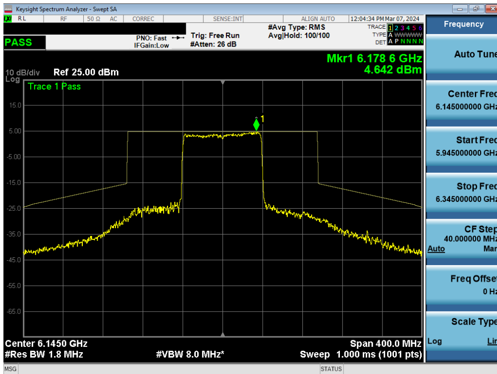
Plot 7-369. In-Band Emission Plot MIMO ANT1 (80MHz BW 802.11be (Full Tones) (UNII Band 5) – Ch. 39) - SP
