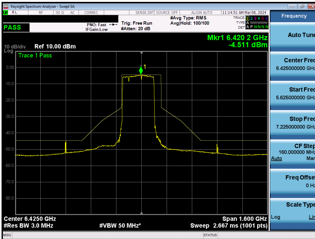
Plot 7-351. In-Band Emission Plot MIMO ANT2 (320MHz BW 802.11be (2*996+484 Tone) (UNII Band 6) – Ch. 95)
