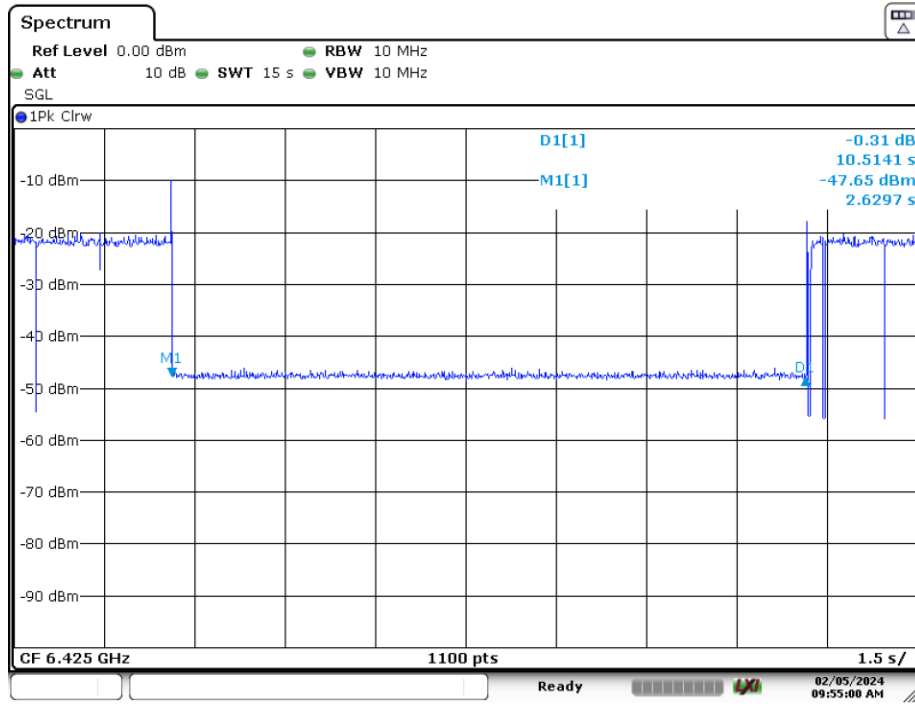
Plot 7-389. Contention Based Protocol Timing Plot (320MHz (UNII Band 6) – Ch. 95 Mid)
