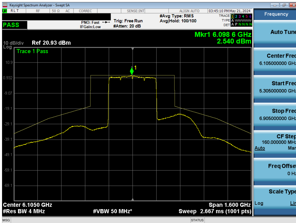
Plot 7-371. In-Band Emission Plot MIMO ANT1 (320MHz BW 802.11be (Full Tones) (UNII Band 5) – Ch. 31) – SP
