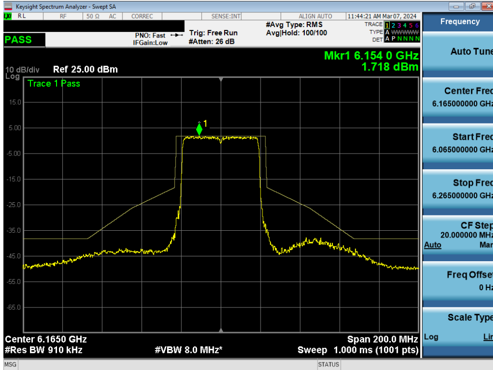
Plot 7-368. In-Band Emission Plot MIMO ANT1 (40MHz BW 802.11be (Full Tones) (UNII Band 5) – Ch. 43) - SP
