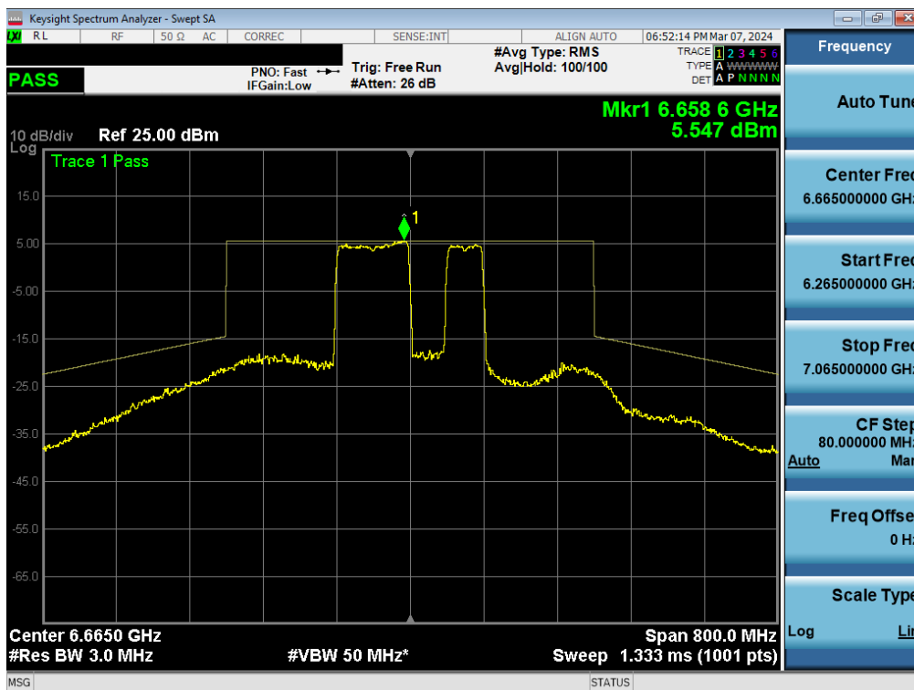
Plot 7-381. In-Band Emission Plot MIMO ANT2 (160MHz BW 802.11be (996+484 Tone) (UNII Band 7) – Ch. 143) - SP
