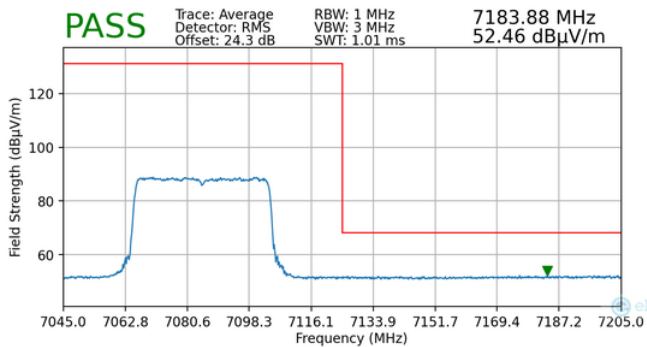
Plot 7-424. Radiated Upper Band Edge Plot MIMO (Average – UNII Band 8 – 484T)
