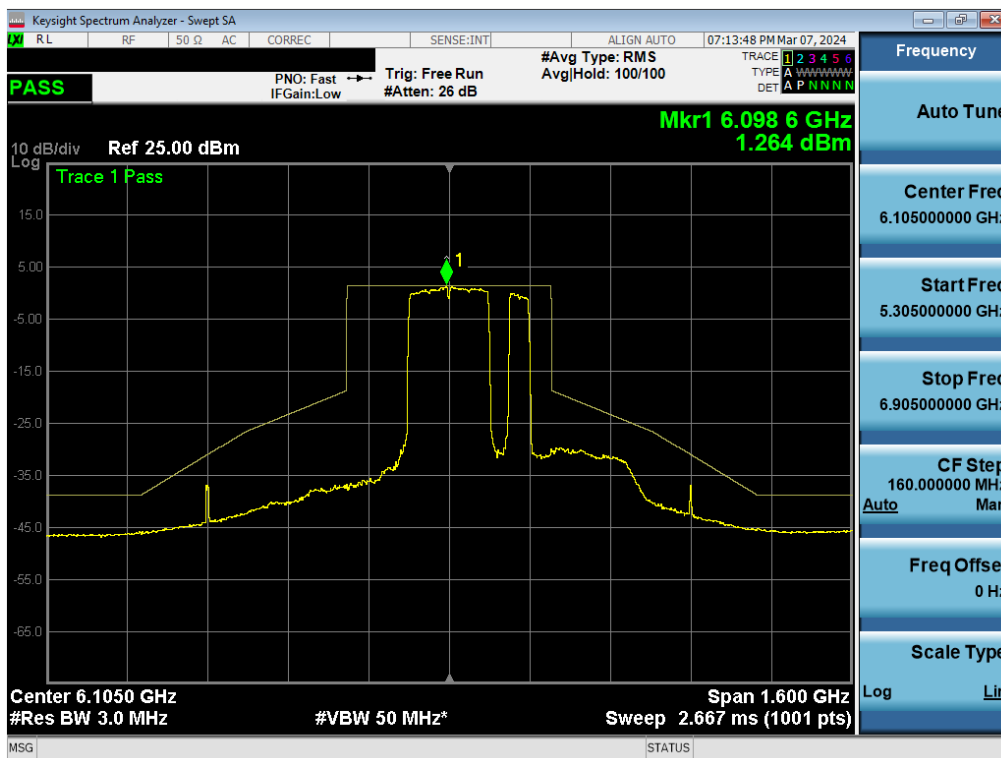
Plot 7-379. In-Band Emission Plot MIMO ANT2 (320MHz BW 802.11be (2*996+484 Tone) (UNII Band 5) – Ch. 31) – SP
