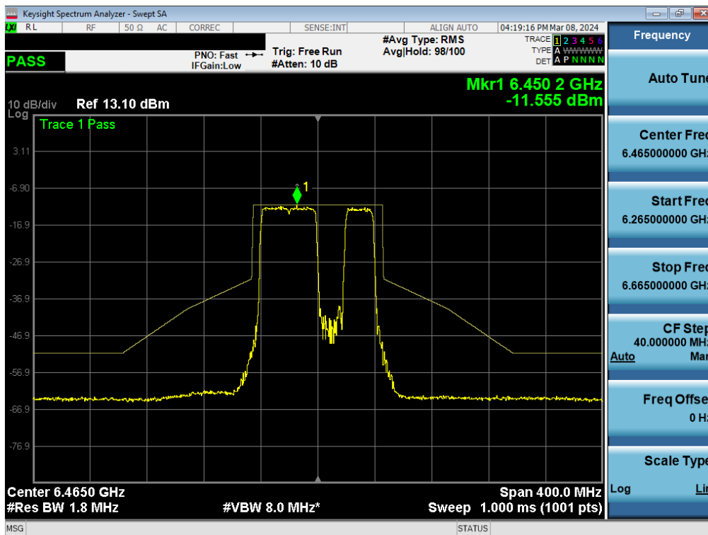
Plot 7-349. In-Band Emission Plot MIMO ANT2 (80MHz BW 802.11be (484+242 Tone) (UNII Band 6) – Ch. 103)
