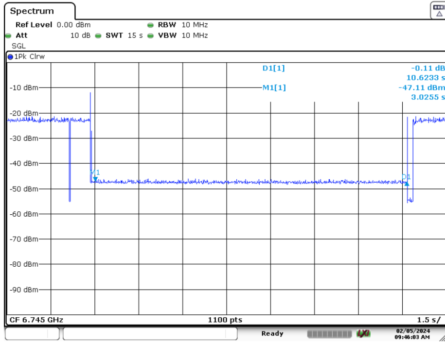
Plot 7-393. Contention Based Protocol Timing Plot (320MHz (UNII Band 7) – Ch. 159 Mid)
