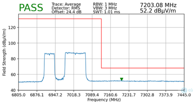
Plot 7-436. Radiated Upper Band Edge Plot MIMO (Average – UNII Band 8 – 996T+484T)
