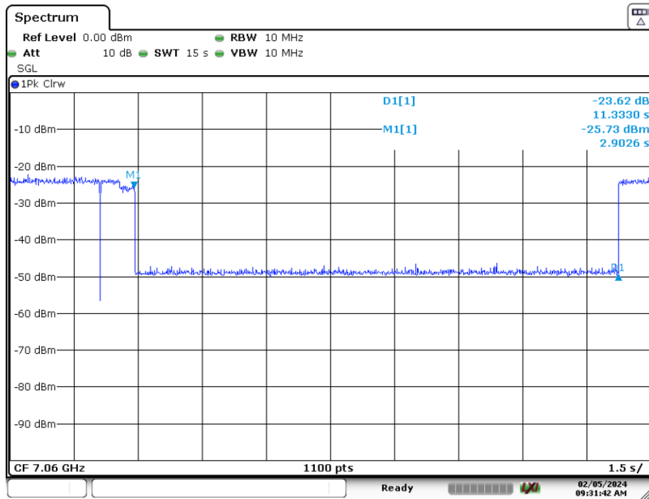
Plot 7-398. Contention Based Protocol Timing Plot (320MHz (UNII Band 8) – Ch. 191 High)
