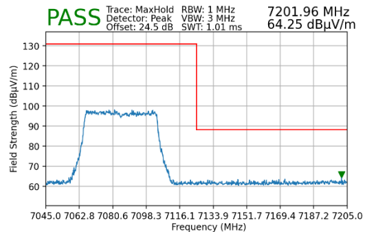
Plot 7-425. Radiated Upper Band Edge Plot MIMO (Peak – UNII Band 8 – 484T)
