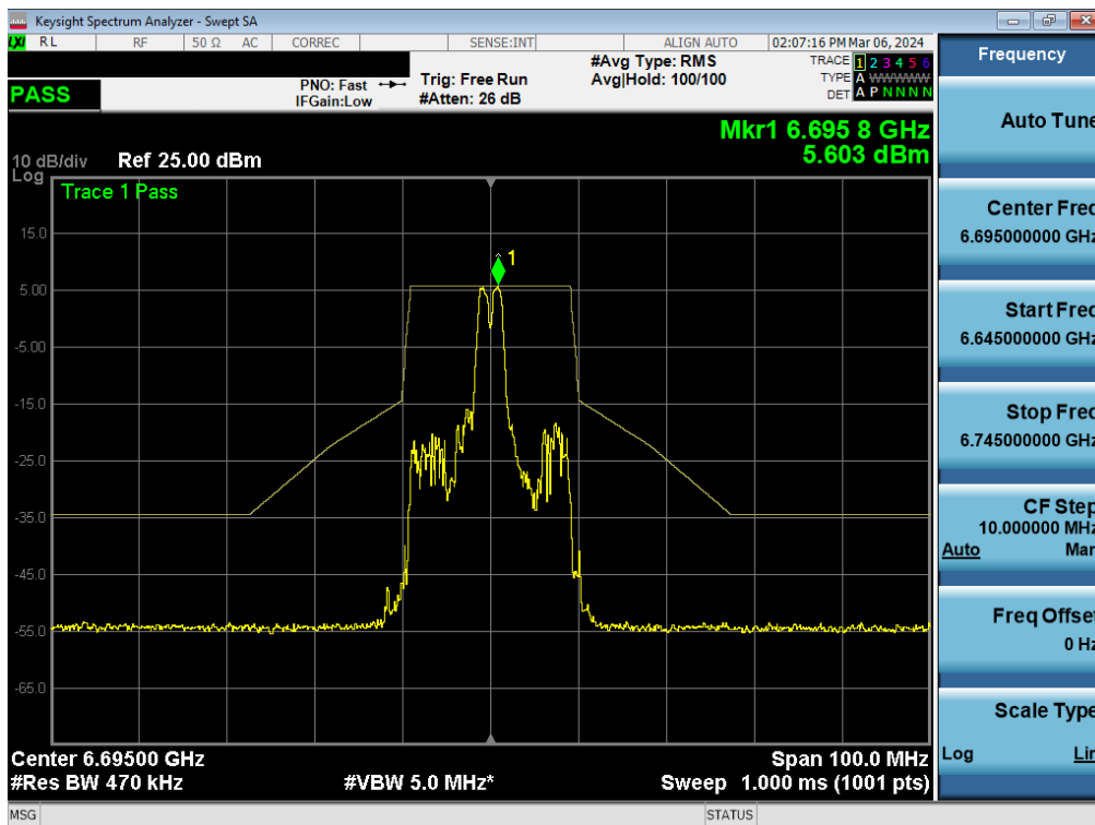
Plot 7-363. In-Band Emission Plot MIMO ANT1 (20MHz BW 802.11be (26 Tone) (UNII Band 7) – Ch. 149) – SP
