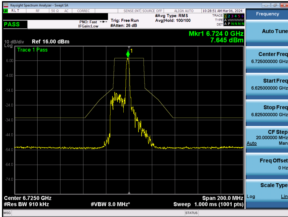
Plot 7-364. In-Band Emission Plot MIMO ANT1 (40MHz BW 802.11be (26 Tone) (UNII Band 7) – Ch. 155) – SP
