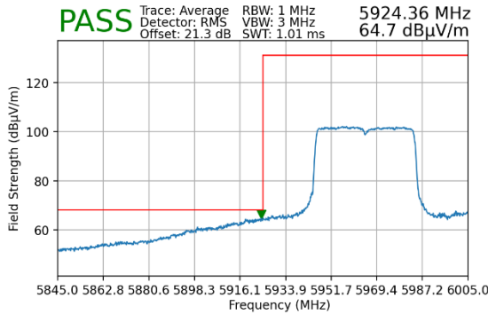
Plot 7-422. Radiated Lower Band Edge Plot MIMO (Average – UNII Band 5 – 484T)
