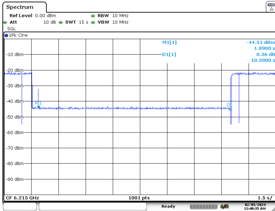
Plot 7-383. Contention Based Protocol Timing Plot (20MHz (UNII Band 5) – Ch. 53)
