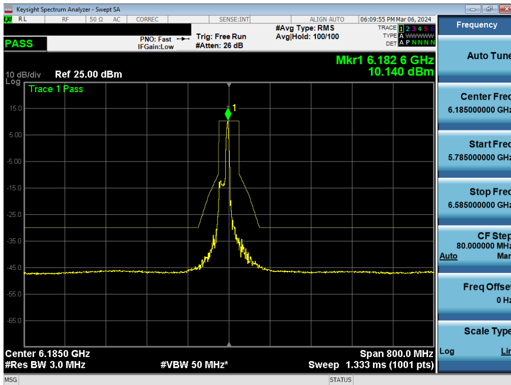
Plot 7-361. In-Band Emission Plot MIMO ANT1 (160MHz BW 802.11be (26 Tones) (UNII Band 5) – Ch. 47) - SP
