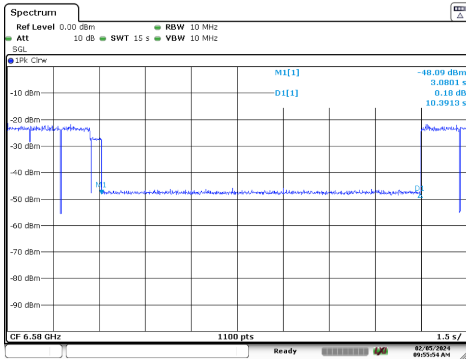
Plot 7-390. Contention Based Protocol Timing Plot (320MHz (UNII Band 6) – Ch. 95 High)
