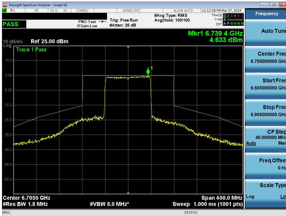
Plot 7-374. In-Band Emission Plot MIMO ANT1 (80MHz BW 802.11be (Full Tone) (UNII Band 7) – Ch. 151) – SP
