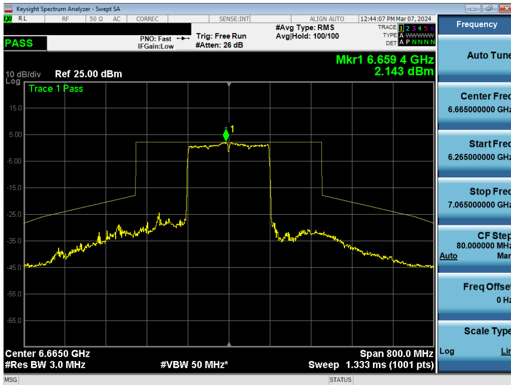
Plot 7-375. In-Band Emission Plot MIMO ANT1 (160MHz BW 802.11be (Full Tone) (UNII Band 7) – Ch. 143) – SP
