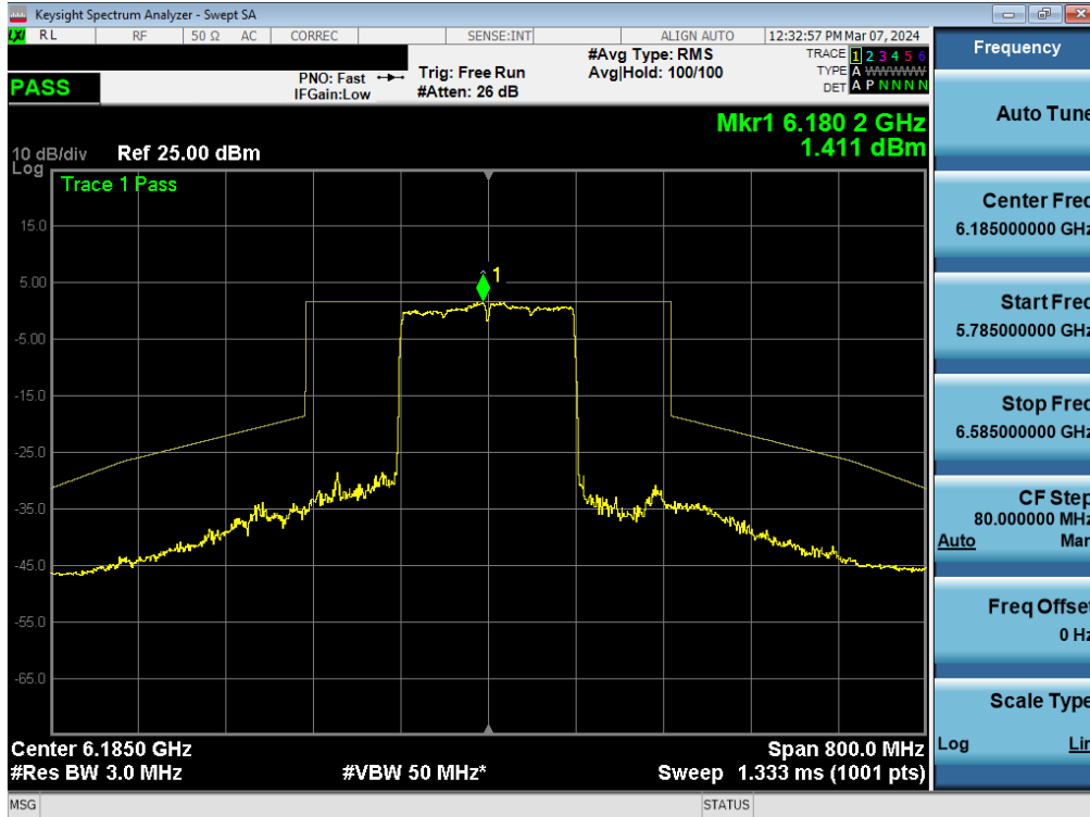
Plot 7-370. In-Band Emission Plot MIMO ANT1 (160MHz BW 802.11be (Full Tones) (UNII Band 5) – Ch. 47) - SP
