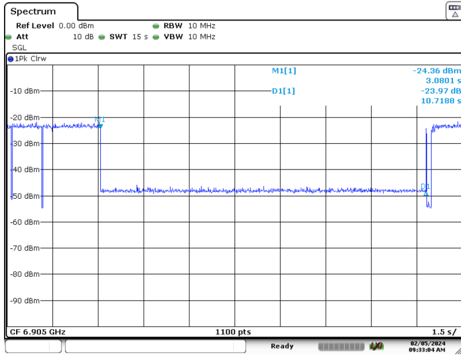
Plot 7-397. Contention Based Protocol Timing Plot (320MHz (UNII Band 8) – Ch. 191 Mid)
