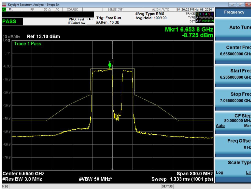
Plot 7-353. In-Band Emission Plot MIMO ANT2 (160MHz BW 802.11be (996+484 Tone) (UNII Band 7) – Ch. 143)
