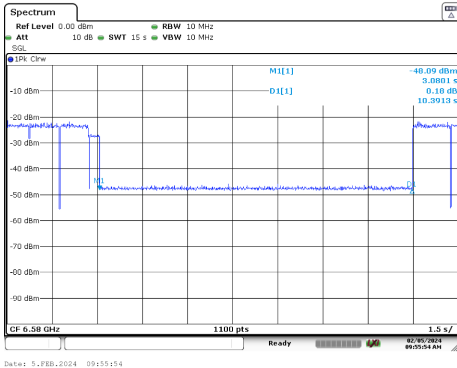
Plot 7-200. Contention Based Protocol Timing Plot (320MHz (UNII Band 6) – Ch. 95 High)
