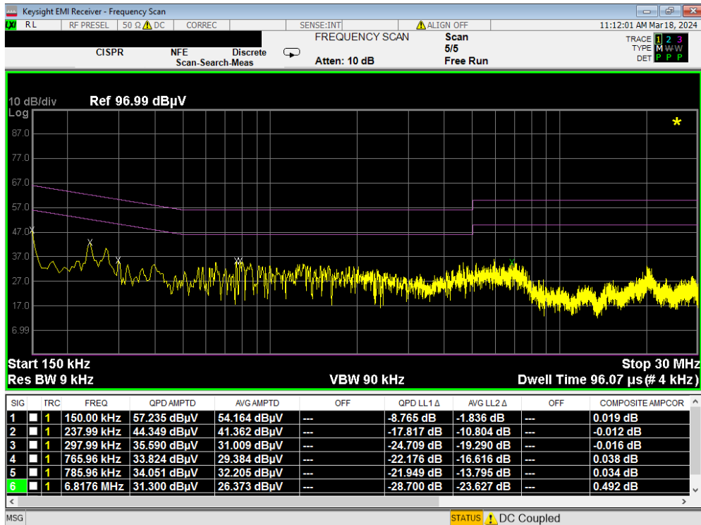
Plot 7-248. Line Conducted Plot with 802.11a UNII Band 8 (N)
