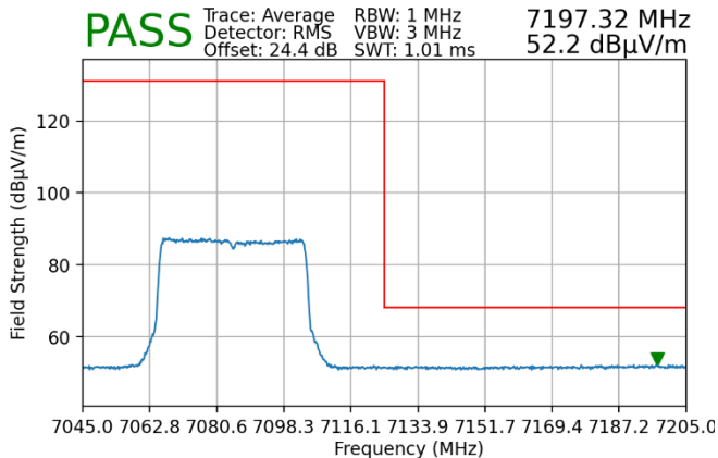
Plot 7-227. Radiated Upper Band Edge Plot MIMO (Average – UNII Band 8)
