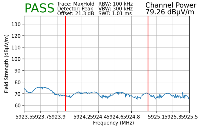
Plot 7-234. Radiated Lower Band Edge Plot MIMO (Peak – UNII Band 5)
