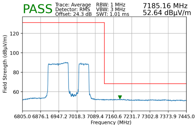
Plot 7-235. Radiated Upper Band Edge Plot MIMO (Average – UNII Band 8)
