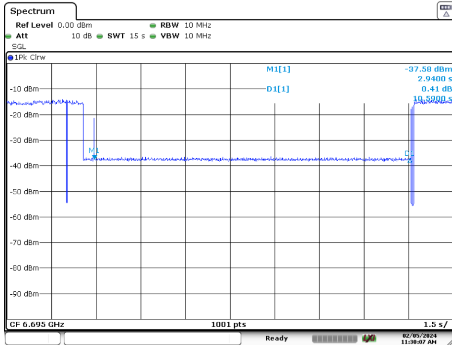
Plot 7-201. Contention Based Protocol Timing Plot (20MHz (UNII Band 7) – Ch. 149)
