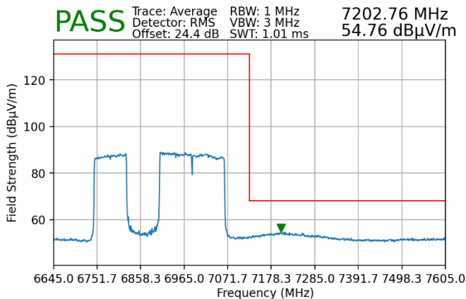
Plot 7-239. Radiated Upper Band Edge Plot MIMO (Average – UNII Band 8)
