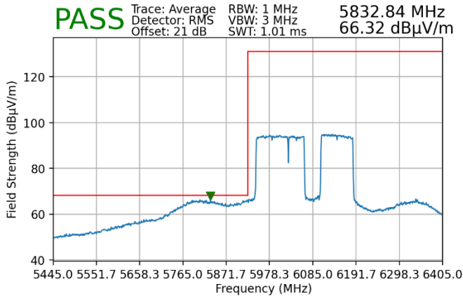
Plot 7-237. Radiated Lower Band Edge Plot MIMO (Average – UNII Band 5)
