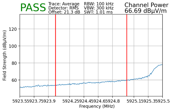
Plot 7-221. Radiated Lower Band Edge Plot MIMO (Average – UNII Band 5)
