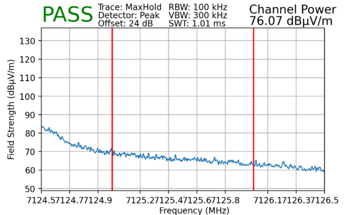
Plot 7-224. Radiated Upper Band Edge Plot MIMO (Peak – UNII Band 8)
