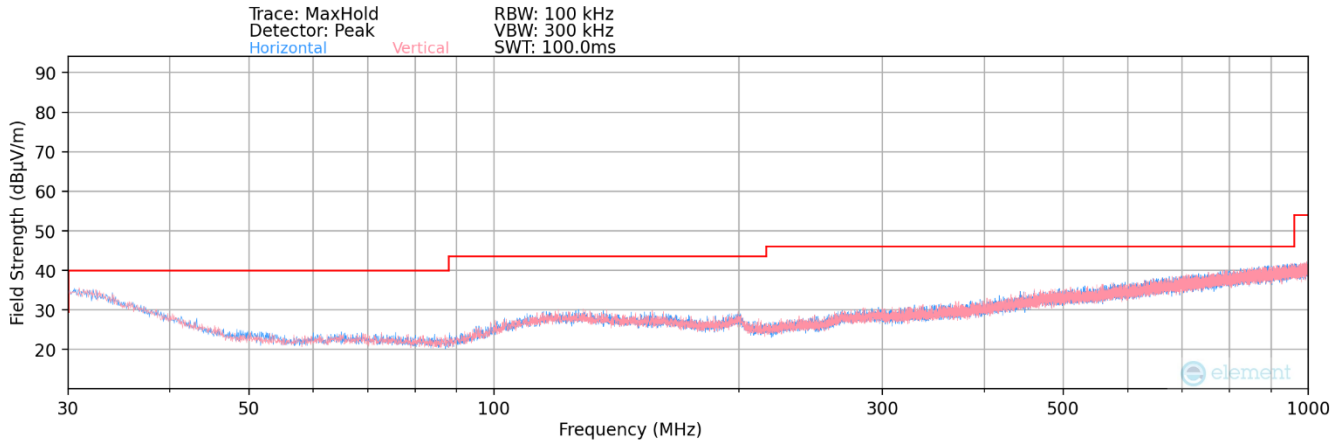
Plot 7-212. Radiated Spurious Plot below 1GHz MIMO (802.11a)
