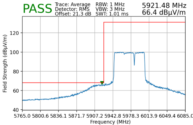
Plot 7-229. Radiated Lower Band Edge Plot MIMO (Average – UNII Band 5)
