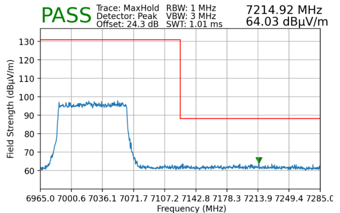
Plot 7-232. Radiated Upper Band Edge Plot MIMO (Peak – UNII Band 8)
