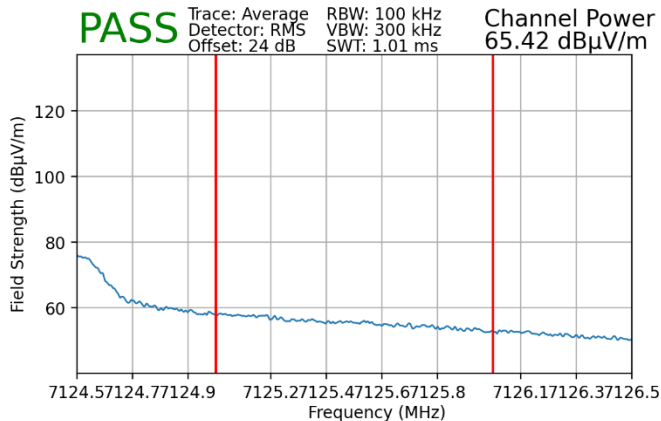
Plot 7-223. Radiated Upper Band Edge Plot MIMO (Average – UNII Band 8)
