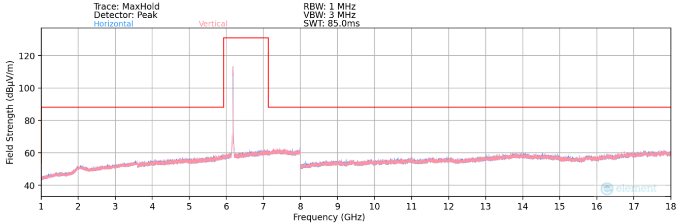
Plot 7-214. Radiated Spurious Plot 1GHz – 18GHz MIMO (802.11a – UNII Band 5 Ch. 45 – SP)
