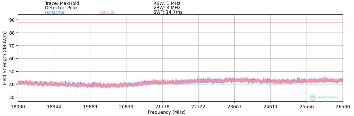
Plot 7-219. Radiated Spurious Plot 18GHz - 26.5GHz (802.11a)
