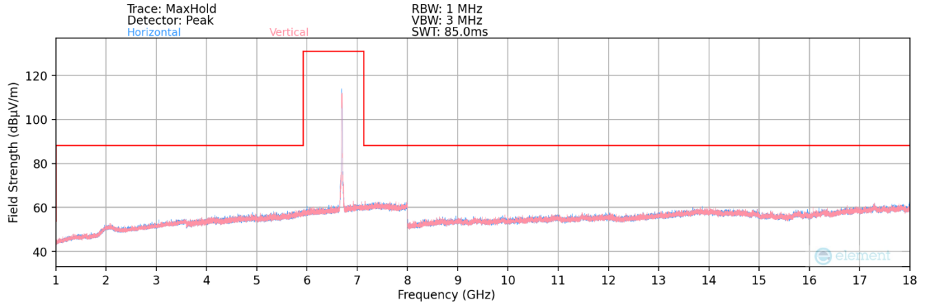
Plot 7-217. Radiated Spurious Plot 1GHz – 18GHz MIMO (802.11a – UNII Band 7 Ch. 149 – SP)
