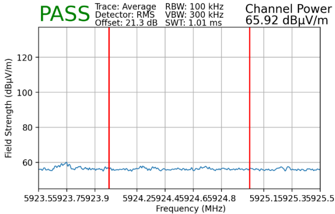
Plot 7-233. Radiated Lower Band Edge Plot MIMO (Average – UNII Band 5)
