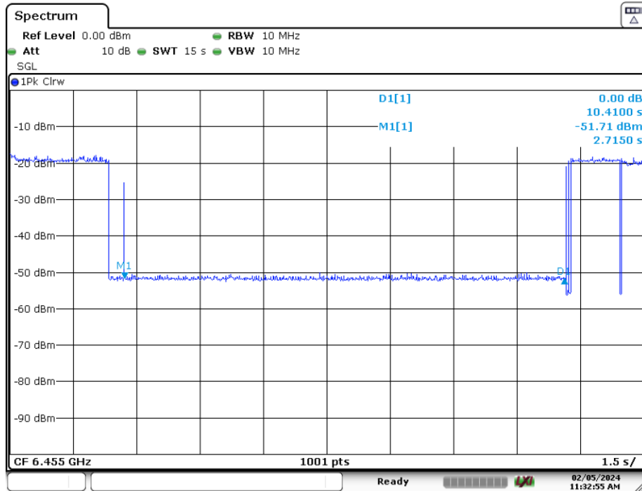
Plot 7-197. Contention Based Protocol Timing Plot (20MHz (UNII Band 6) – Ch. 101)
