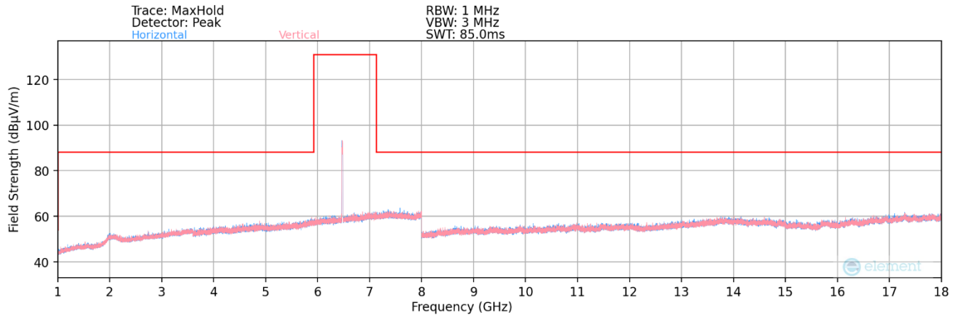
Plot 7-215. Radiated Spurious Plot 1GHz – 18GHz MIMO (802.11a – UNII Band 6 Ch. 105 – LPI)
