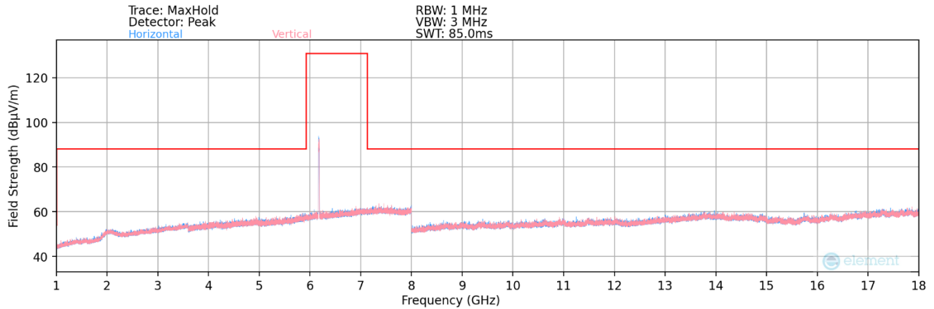
Plot 7-213. Radiated Spurious Plot 1GHz – 18GHz MIMO (802.11a – UNII Band 5 Ch. 45 – LPI)
