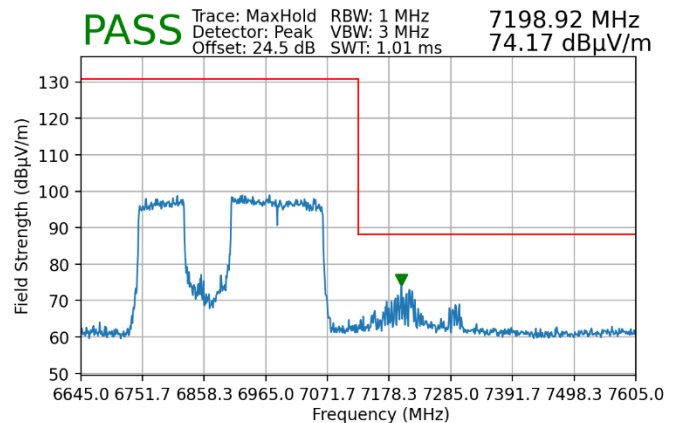
Plot 7-240. Radiated Upper Band Edge Plot MIMO (Peak – UNII Band 8)
