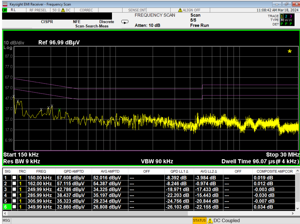
Plot 7-245. Line Conducted Plot with 802.11a UNII Band 7 (L1)
