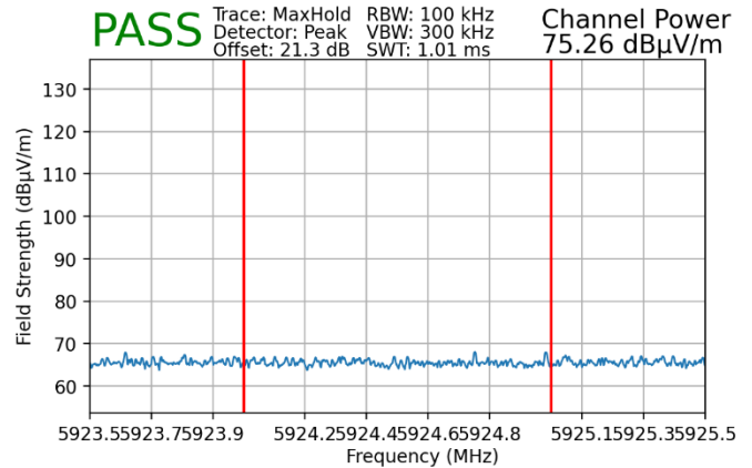
Plot 7-238. Radiated Lower Band Edge Plot MIMO (Peak – UNII Band 5)
