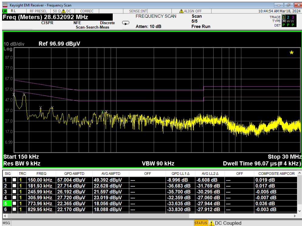
Plot 7-242. Line Conducted Plot with 802.11a UNII Band 5 (N)
