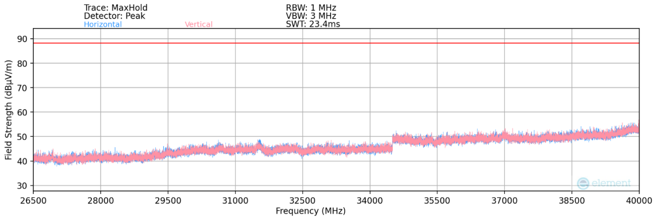
Plot 7-220. Radiated Spurious Plot 26.5GHz - 40GHz (802.11a)
