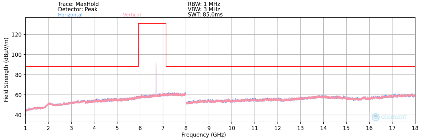
Plot 7-216. Radiated Spurious Plot 1GHz – 18GHz MIMO (802.11a – UNII Band 7 Ch. 149 – LPI)
