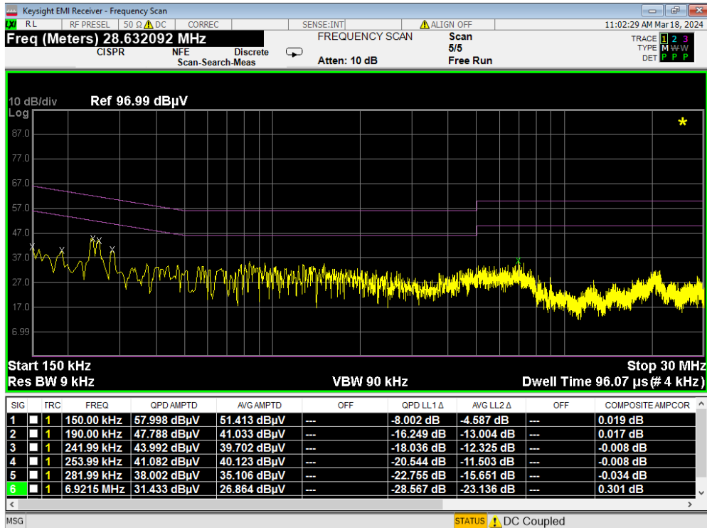
Plot 7-244. Line Conducted Plot with 802.11a UNII Band 6 (N)
