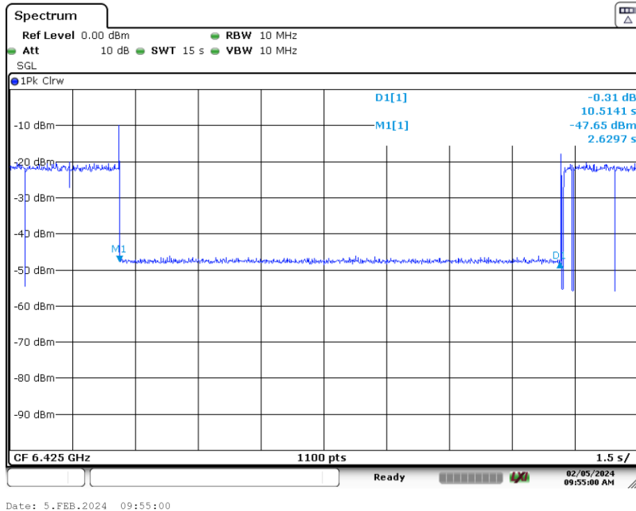
Plot 7-199. Contention Based Protocol Timing Plot (320MHz (UNII Band 6) – Ch. 95 Mid)
