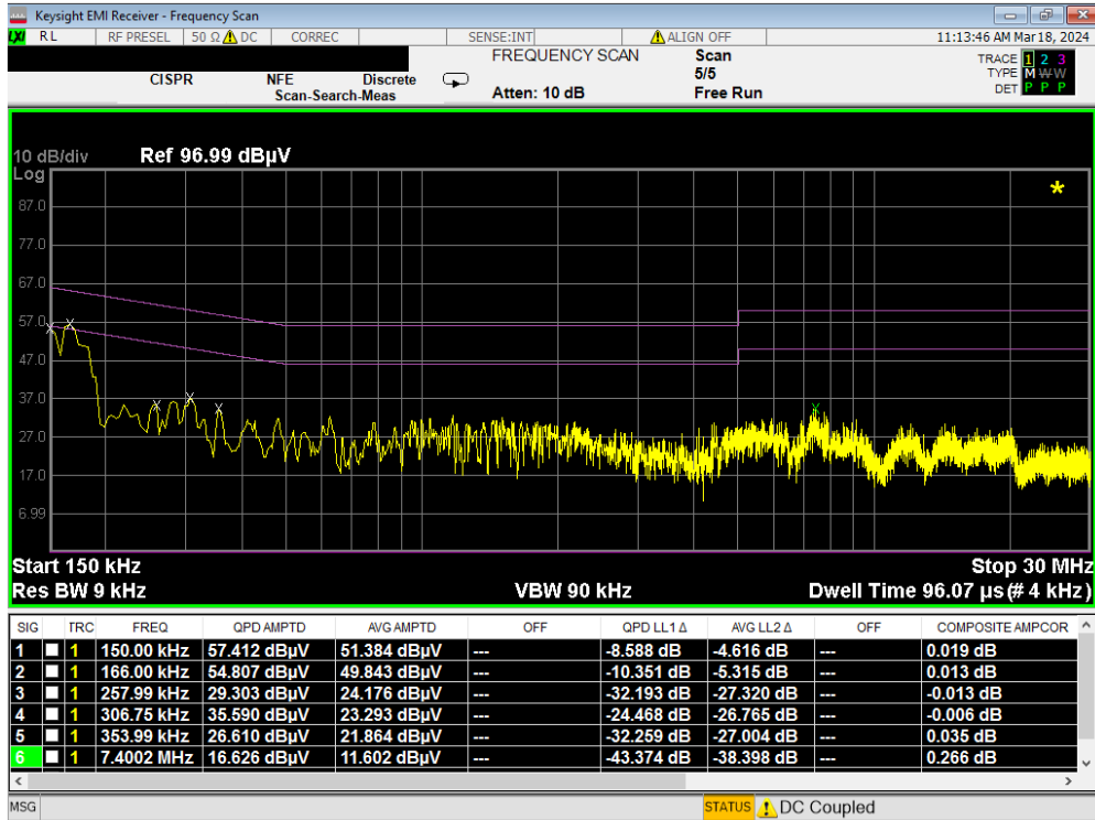
Plot 7-247. Line Conducted Plot with 802.11a UNII Band 8 (L1)
