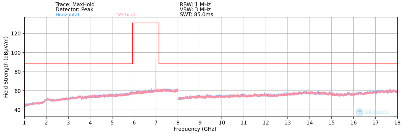
Plot 7-218. Radiated Spurious Plot 1GHz – 18GHz MIMO (802.11a – U Band 8 Ch. 209 – LPI)
