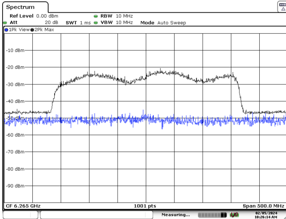
Plot 7-210. CBP 320MHz Channel - Injection Center – [6265 MHz]
