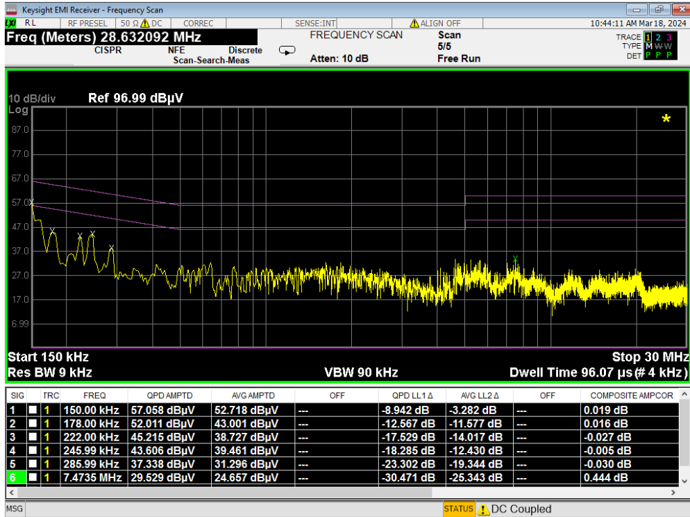
Plot 7-241. Line Conducted Plot with 802.11a UNII Band 5 (L1)
