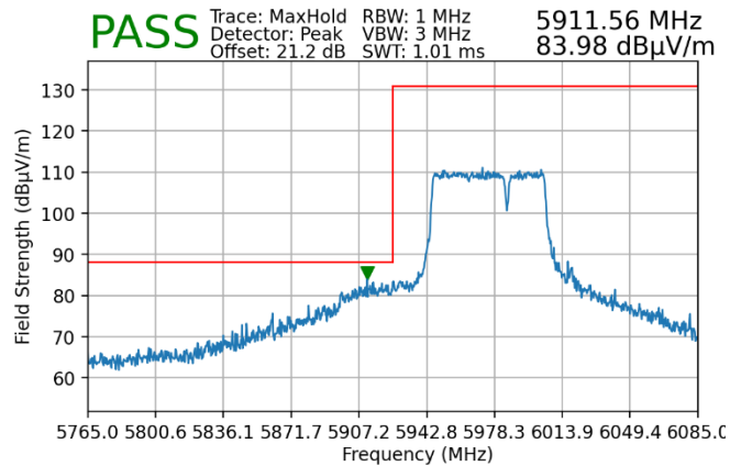
Plot 7-230. Radiated Lower Band Edge Plot MIMO (Peak – UNII Band 5)
