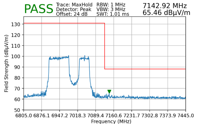
Plot 7-236. Radiated Upper Band Edge Plot MIMO (Peak – UNII Band 8)
