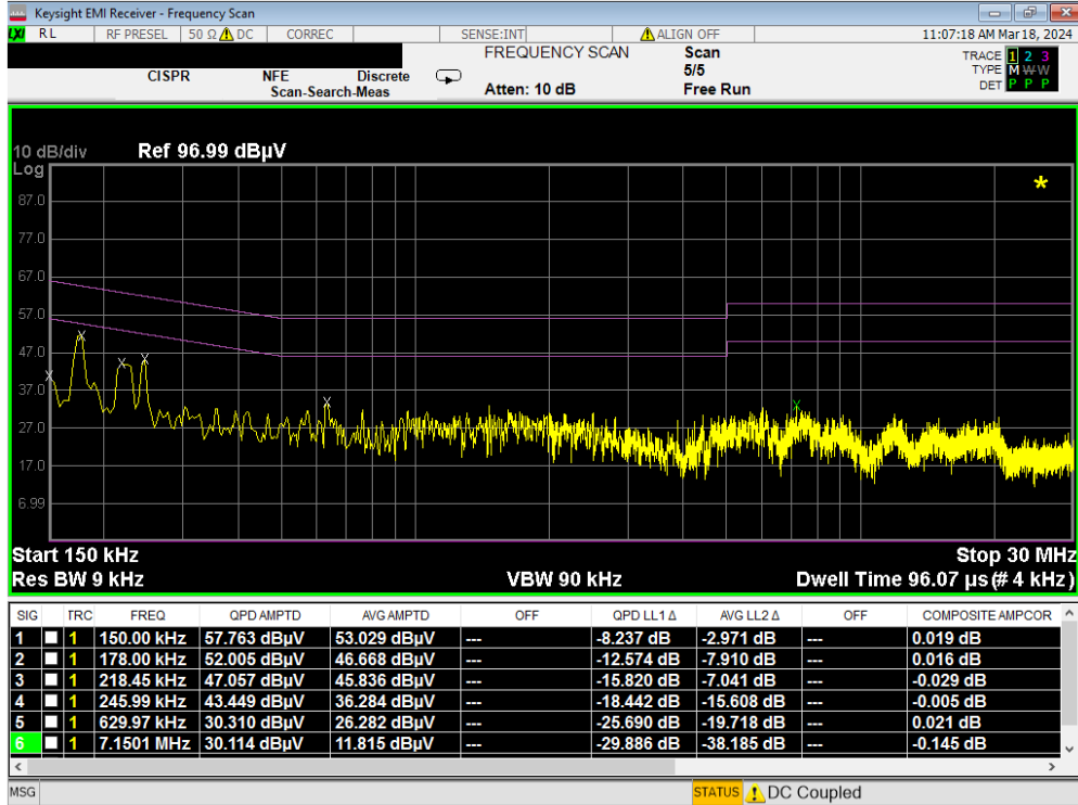
Plot 7-243. Line Conducted Plot with 802.11a UNII Band 6 (L1)
