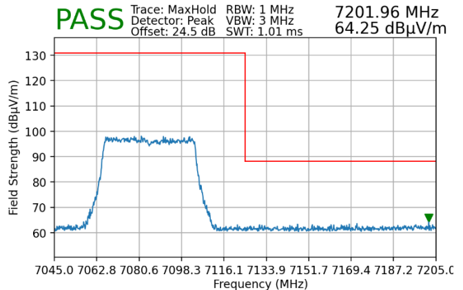
Plot 7-228. Radiated Upper Band Edge Plot MIMO (Peak – UNII Band 8)
