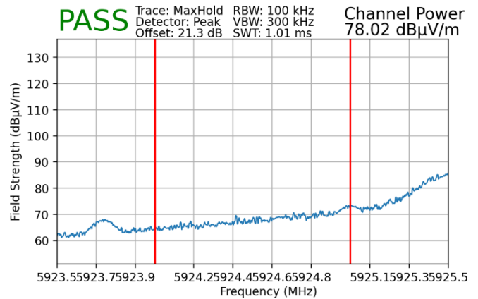
Plot 7-222. Radiated Lower Band Edge Plot MIMO (Peak – UNII Band 5)
