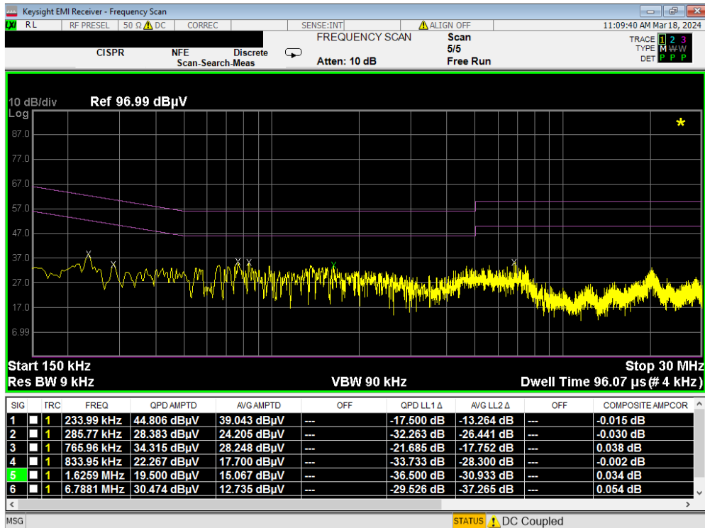
Plot 7-246. Line Conducted Plot with 802.11a UNII Band 7 (N)
