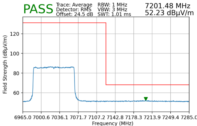
Plot 7-231. Radiated Upper Band Edge Plot MIMO (Average – UNII Band 8)
