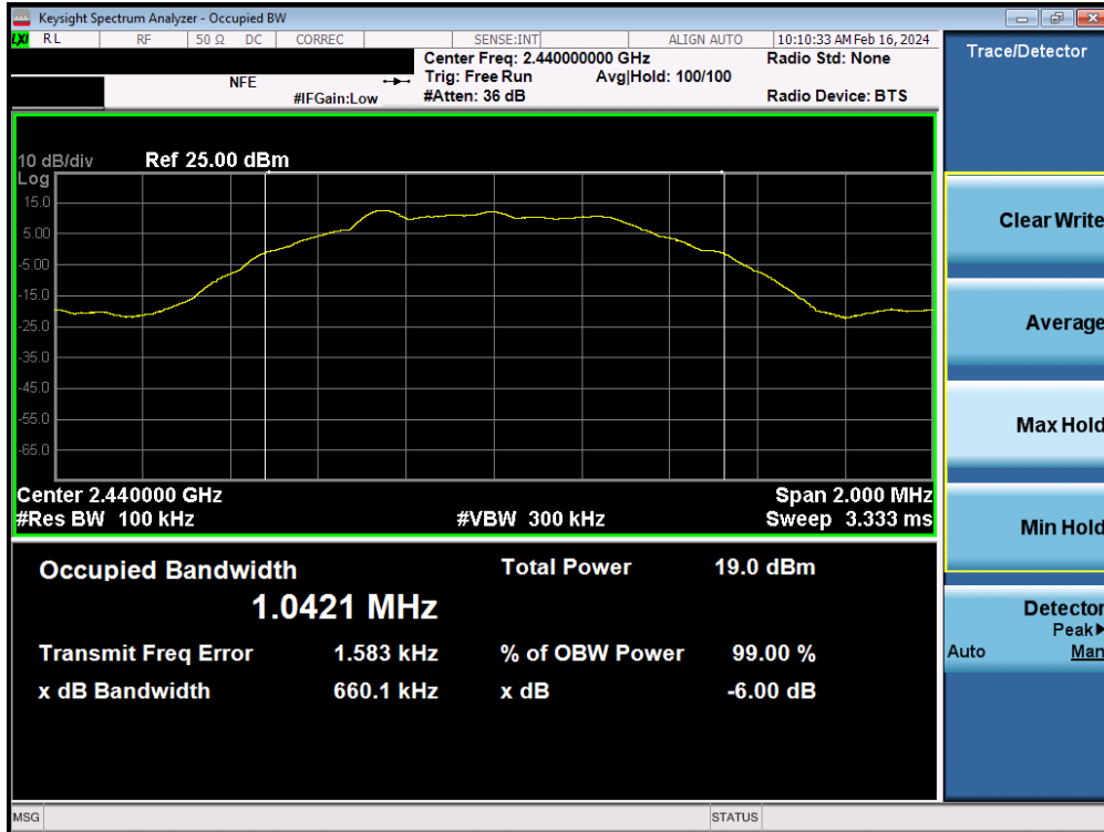
Plot 7-17. 6dB Bandwidth Plot (Bluetooth (LE), 500kbps – Ch. 17)
