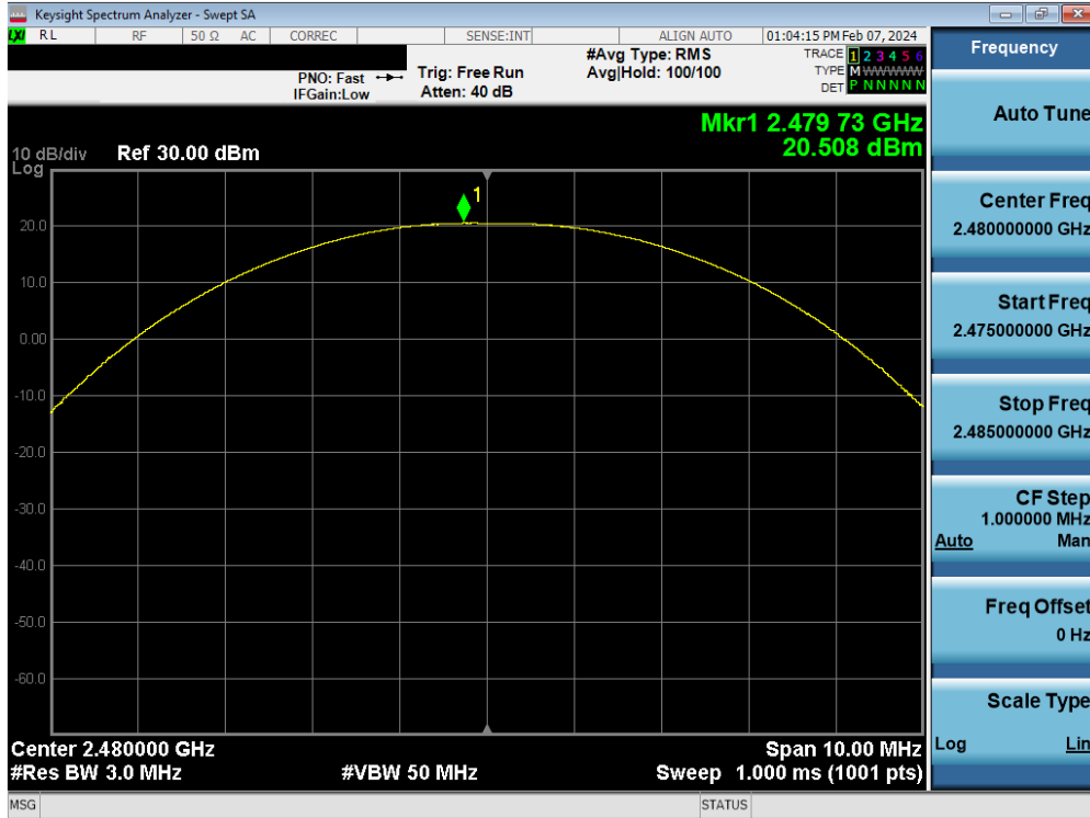
Plot 7-45. Peak Power Plot (Bluetooth (LE), 1Mbps – Ch. 39)
