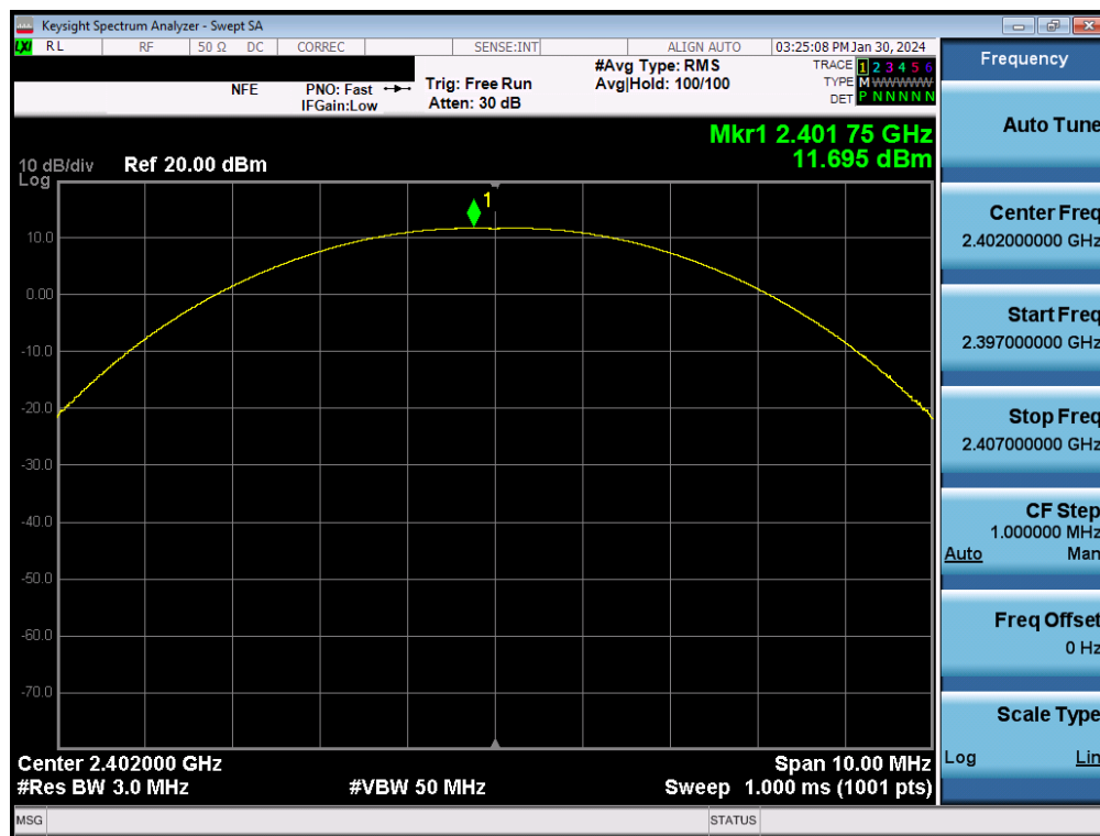
Plot 7-49. Peak Power Plot (Bluetooth (LE), 125kbps – Ch. 37)
