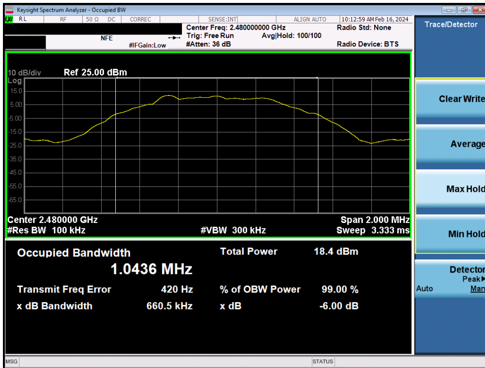
Plot 7-18. 6dB Bandwidth Plot (Bluetooth (LE), 500kbps – Ch. 39)
