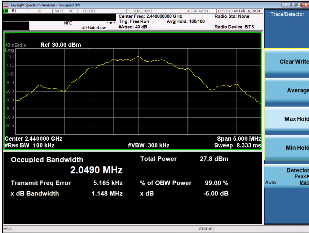
Plot 7-23. 6dB Bandwidth Plot (Bluetooth (LE), 2Mbps – Ch. 17)
