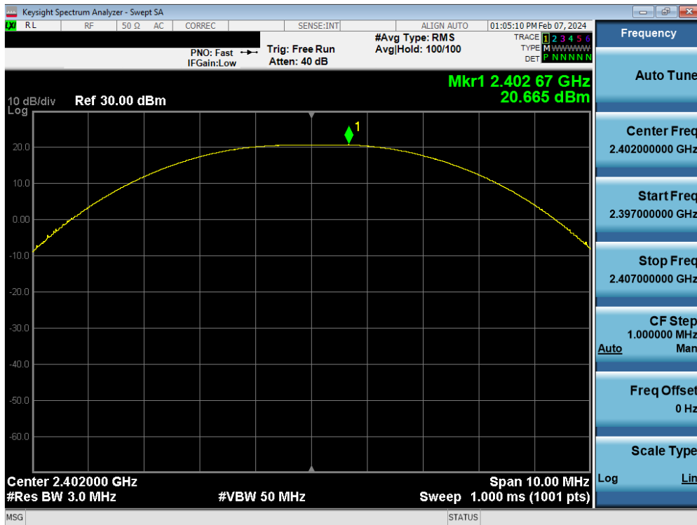
Plot 7-46. Peak Power Plot (Bluetooth (LE), 2Mbps – Ch. 0)
