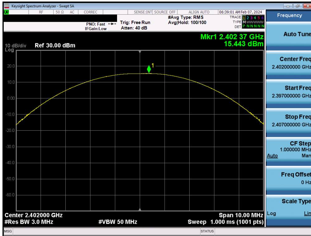
Plot 7-61. Peak Power Plot (Bluetooth (LE), 1Mbps – Ch. 37)
