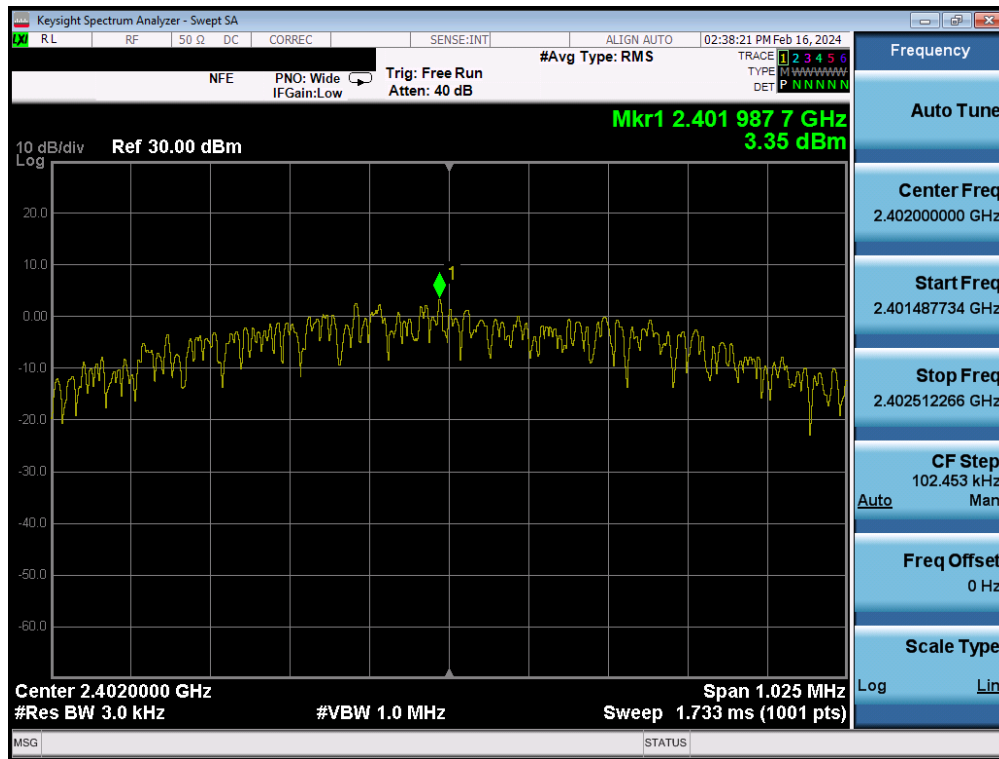
Plot 7-97. Power Spectral Density Plot (Bluetooth (LE), 1Mbps – Ch. 37)
