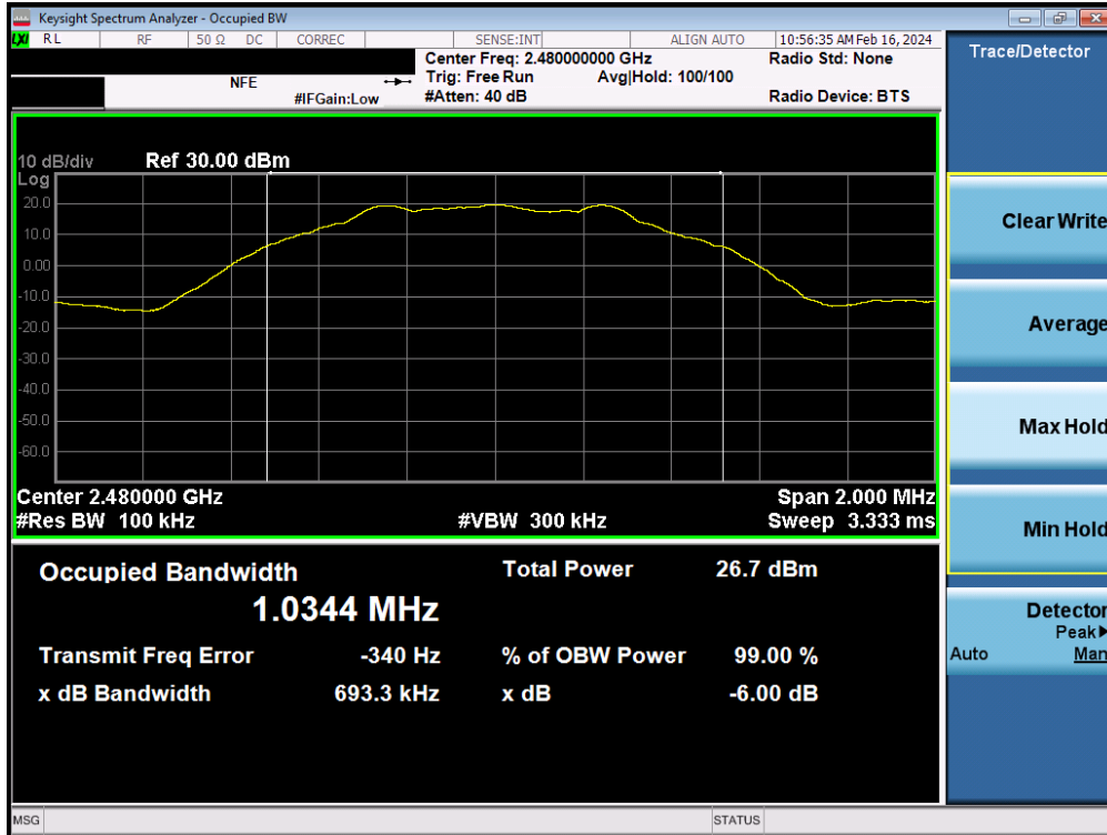
Plot 7-21. 6dB Bandwidth Plot (Bluetooth (LE), 1Mbps – Ch. 39)
