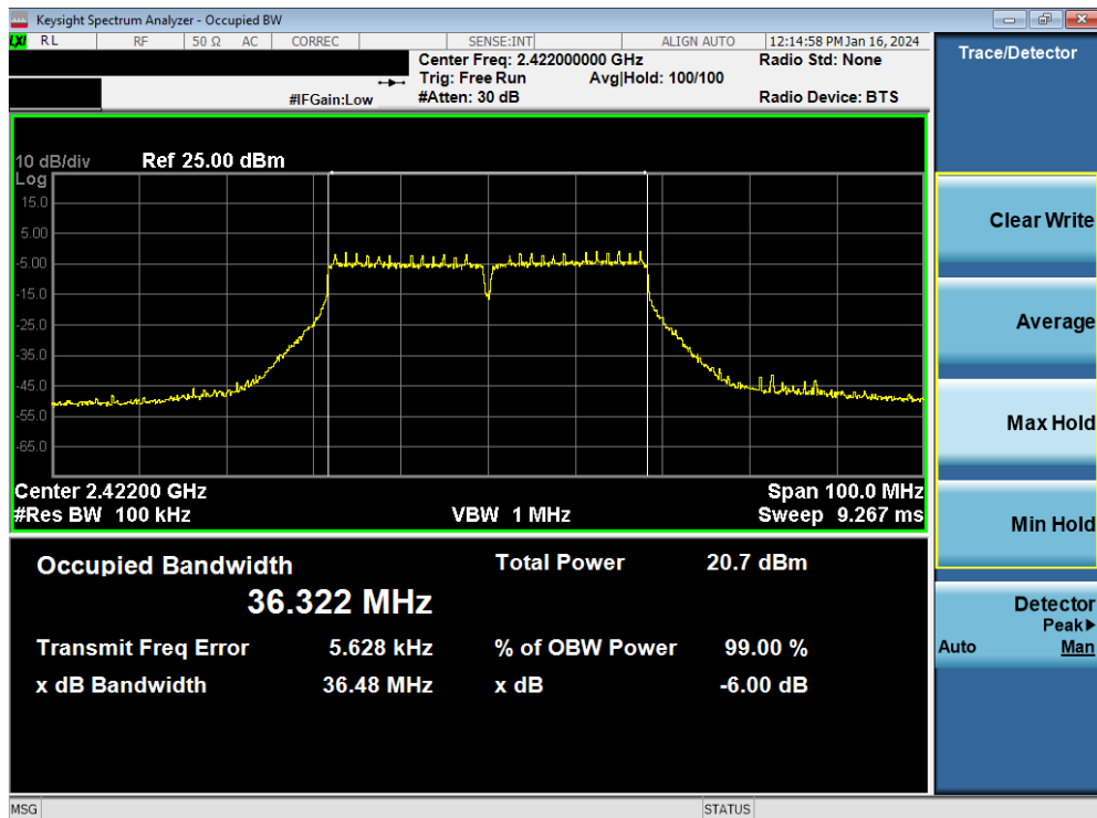
Plot 7-28. 6dB Bandwidth Plot MIMO ANT1 (802.11ac (2.4GHz - 40MHz) – Ch. 3)
