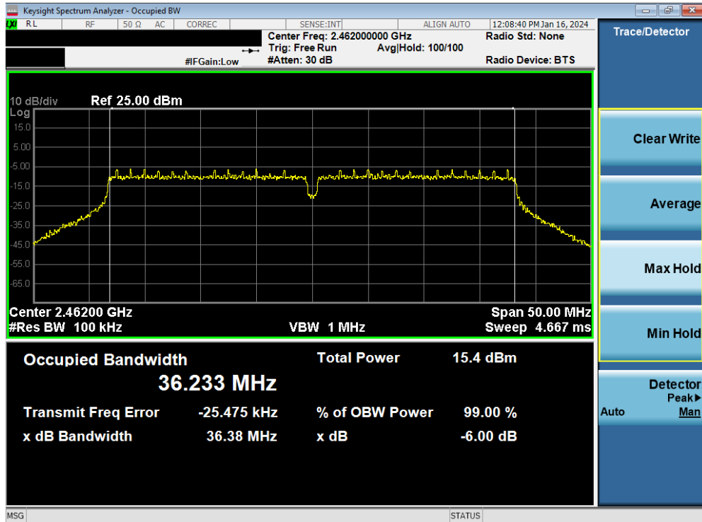
Plot 7-27. 6dB Bandwidth Plot MIMO ANT1 (802.11n (2.4GHz - 40MHz) – Ch. 11)
