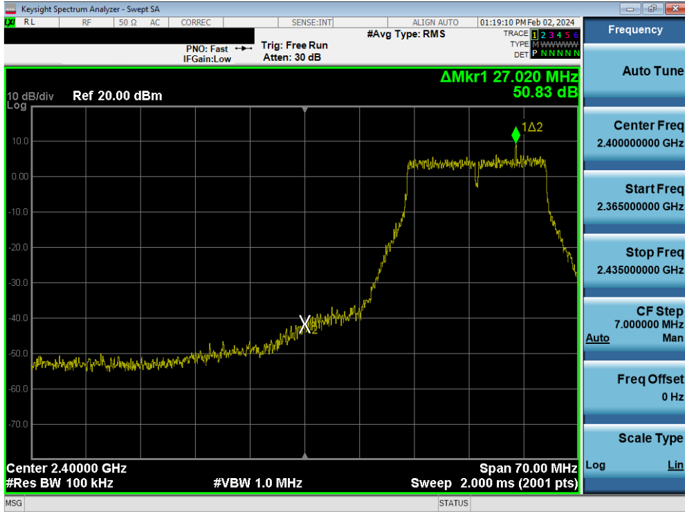
Plot 7-105. Band Edge Plot MIMO ANT1 (802.11n – Ch. 3)
