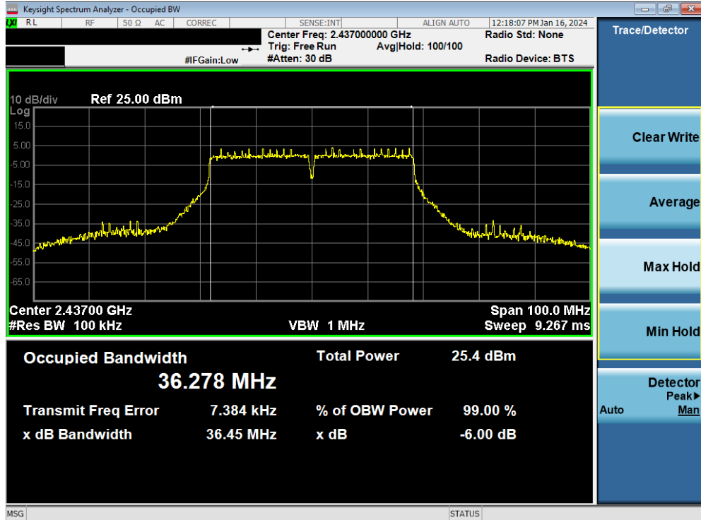
Plot 7-38. 6dB Bandwidth Plot MIMO ANT1 (802.11ac (2.4GHz - 40MHz) – Ch. 6)
