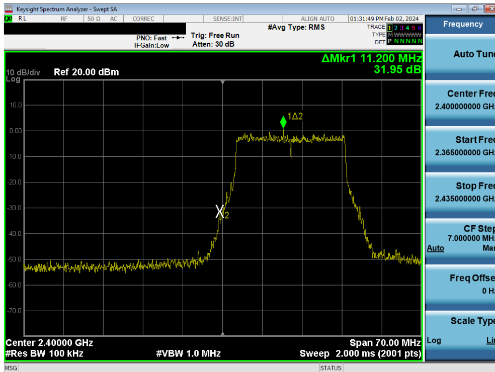
Plot 7-112. Band Edge Plot MIMO ANT1 (802.11be – Ch. 1)
