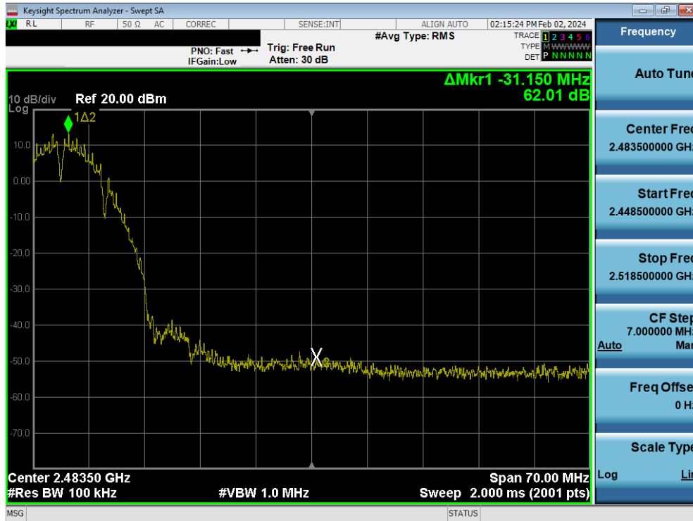
Plot 7-89. Band Edge Plot MIMO ANT1 (802.11b – Ch. 9)
