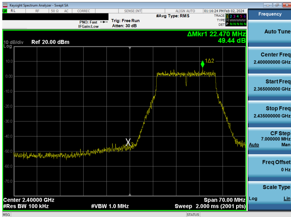
Plot 7-104. Band Edge Plot MIMO ANT1 (802.11n – Ch. 2)
