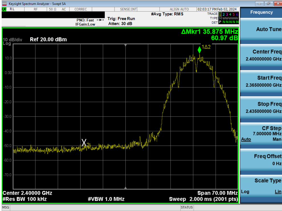
Plot 7-123. Band Edge Plot MIMO ANT2 (802.11b – Ch. 3)
