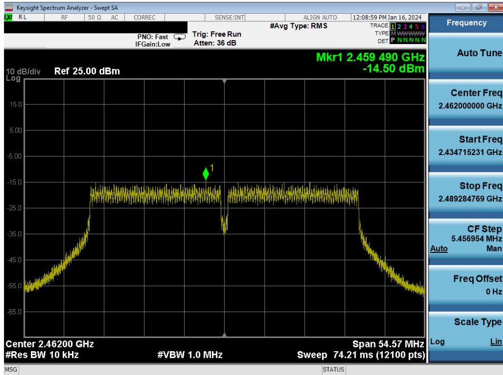
Plot 7-69. Power Spectral Density Plot MIMO ANT1 (802.11n (2.4GHz - 40MHz) – Ch. 11)
