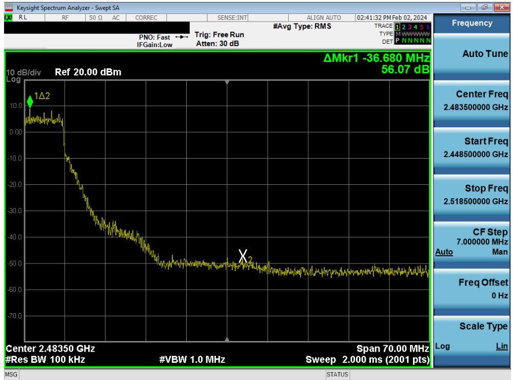
Plot 7-97. Band Edge Plot MIMO ANT1 (802.11g – Ch. 8)
