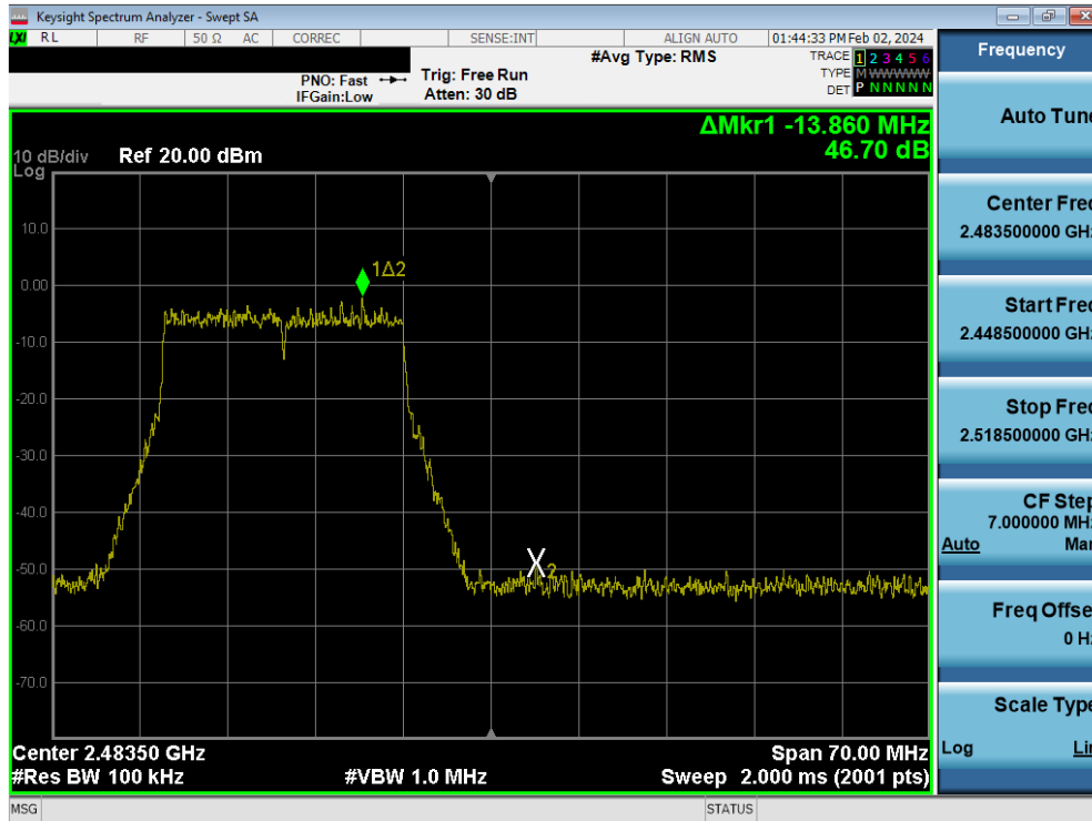
Plot 7-119. Band Edge Plot MIMO ANT1 (802.11be – Ch. 12)
