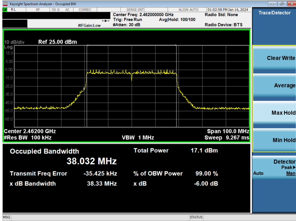
Plot 7-42. 6dB Bandwidth Plot MIMO ANT2 (802.11be (2.4GHz - 40MHz) – Ch. 11)
