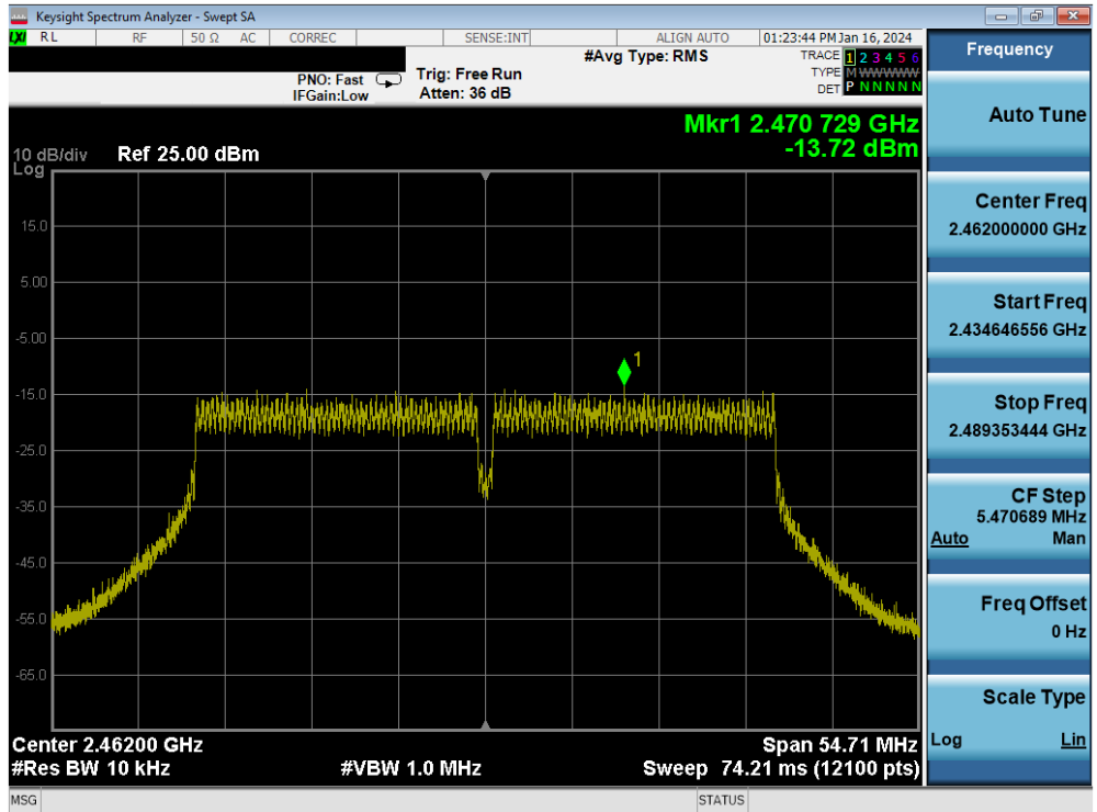
Plot 7-78. Power Spectral Density Plot MIMO ANT2 (802.11n (2.4GHz - 40MHz) – Ch. 11)
