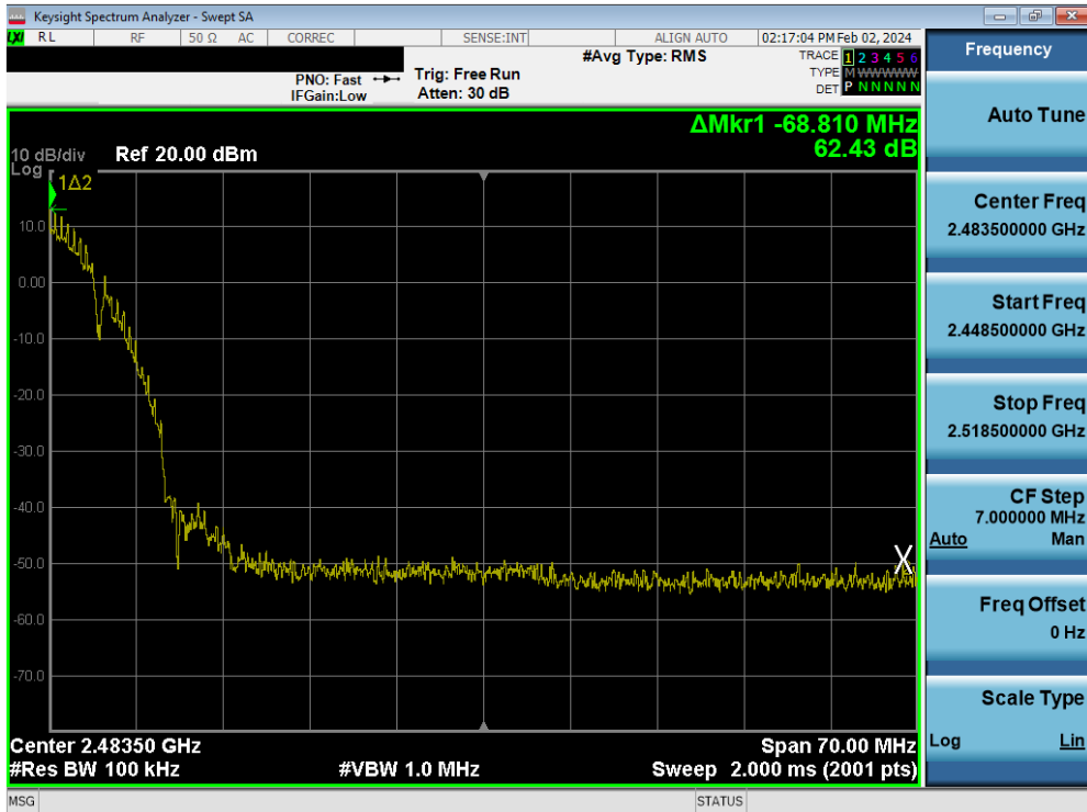
Plot 7-124. Band Edge Plot MIMO ANT2 (802.11b – Ch. 8)
