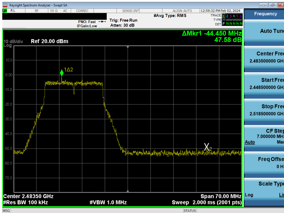
Plot 7-110. Band Edge Plot MIMO ANT1 (802.11n – Ch. 12)
