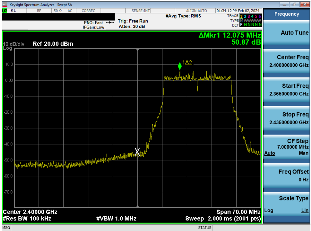
Plot 7-113. Band Edge Plot MIMO ANT1 (802.11be – Ch. 2)
