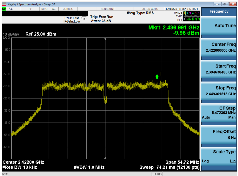
Plot 7-79. Power Spectral Density Plot MIMO ANT1 (802.11ac (2.4GHz - 40MHz) – Ch. 3)
