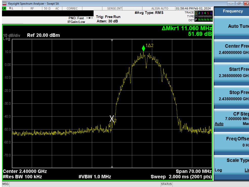
Plot 7-121. Band Edge Plot MIMO ANT2 (802.11b – Ch. 1)
