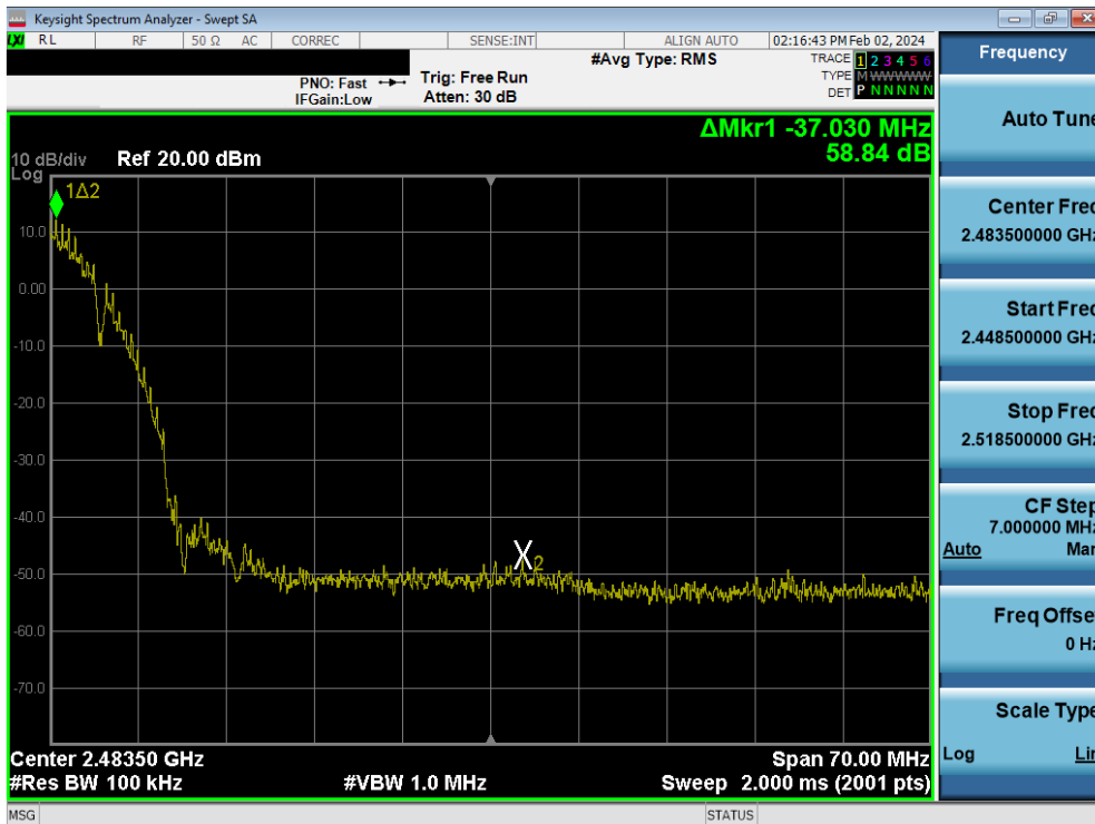
Plot 7-88. Band Edge Plot MIMO ANT1 (802.11b – Ch. 8)
