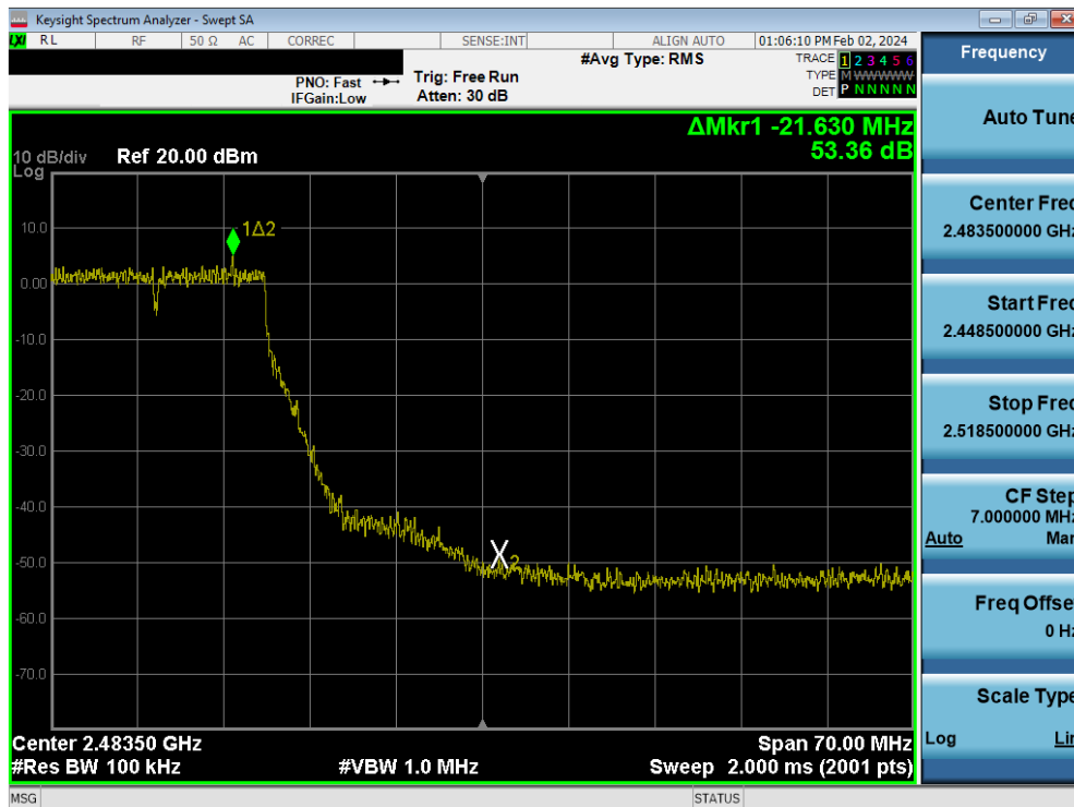
Plot 7-108. Band Edge Plot MIMO ANT1 (802.11n – Ch. 10)
