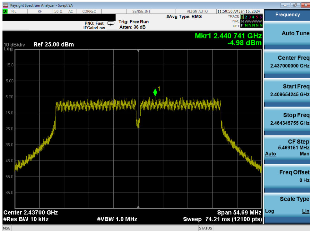
Plot 7-68. Power Spectral Density Plot MIMO ANT1 (802.11n (2.4GHz - 40MHz) – Ch. 6)
