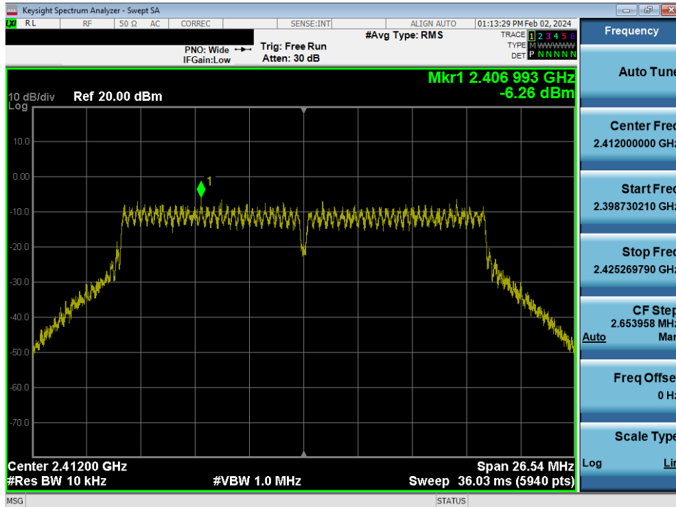
Plot 7-61. Power Spectral Density Plot MIMO ANT2 (802.11n (2.4GHz) – Ch. 1)
