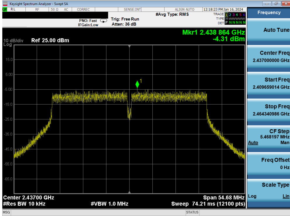
Plot 7-80. Power Spectral Density Plot MIMO ANT1 (802.11ac (2.4GHz - 40MHz) – Ch. 6)
