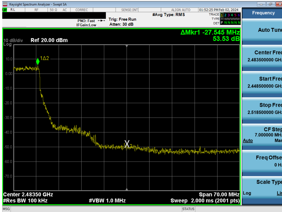
Plot 7-115. Band Edge Plot MIMO ANT1 (802.11be – Ch. 8)
