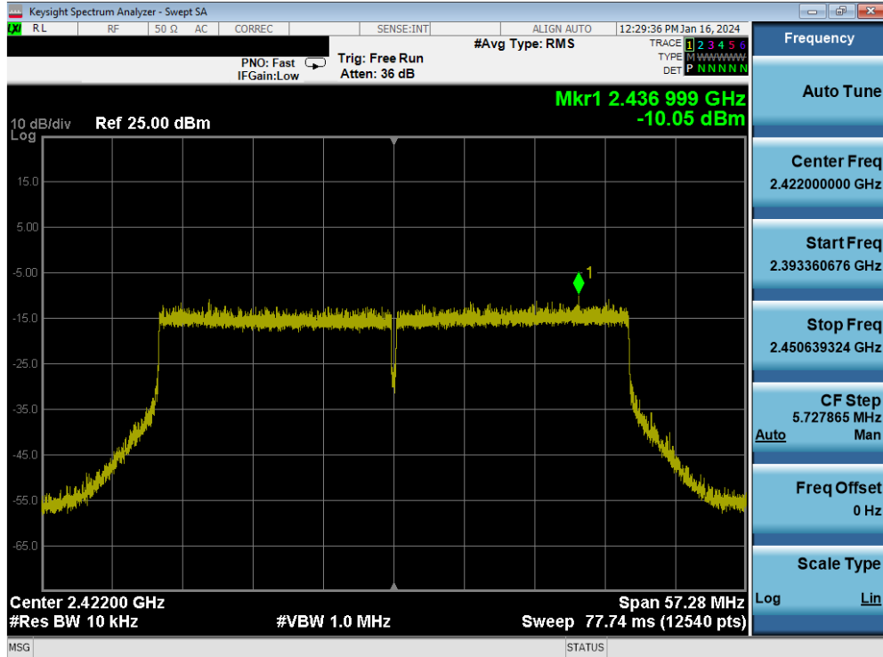
Plot 7-73. Power Spectral Density Plot MIMO ANT1 (802.11be (2.4GHz - 40MHz) – Ch. 3)
