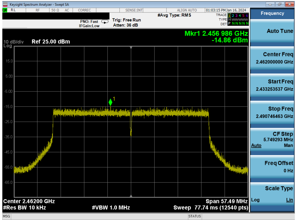
Plot 7-84. Power Spectral Density Plot MIMO ANT2 (802.11be (2.4GHz - 40MHz) – Ch. 11)
