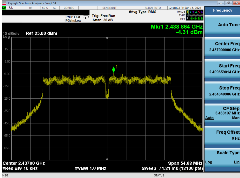
Plot 7-71. Power Spectral Density Plot MIMO ANT1 (802.11ac (2.4GHz - 40MHz) – Ch. 6)
