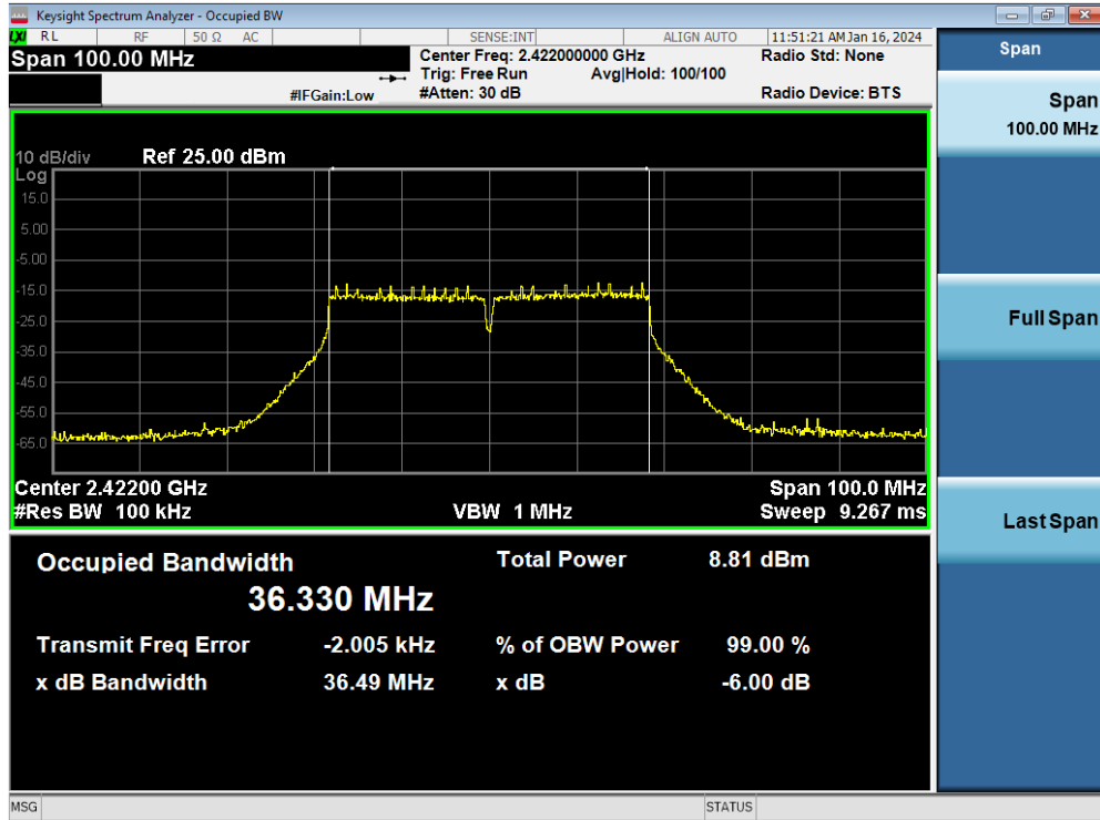
Plot 7-25. 6dB Bandwidth Plot MIMO ANT1 (802.11n (2.4GHz - 40MHz) – Ch. 3)
