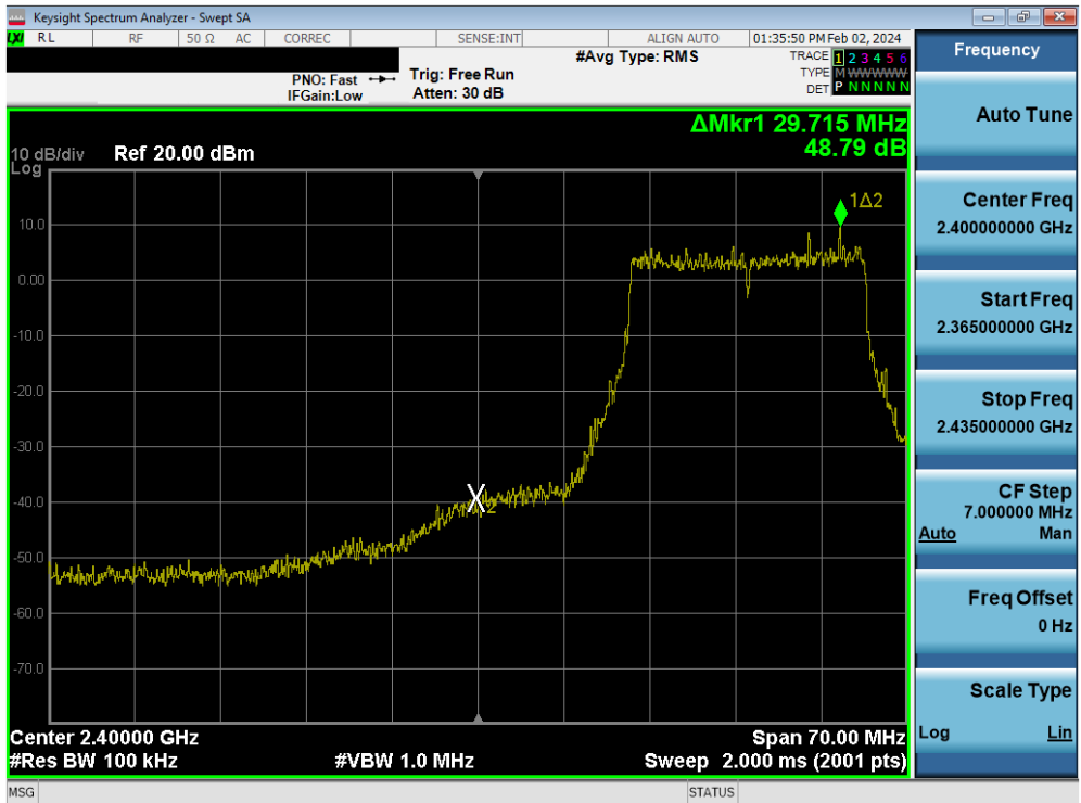
Plot 7-114. Band Edge Plot MIMO ANT1 (802.11be – Ch. 3)
