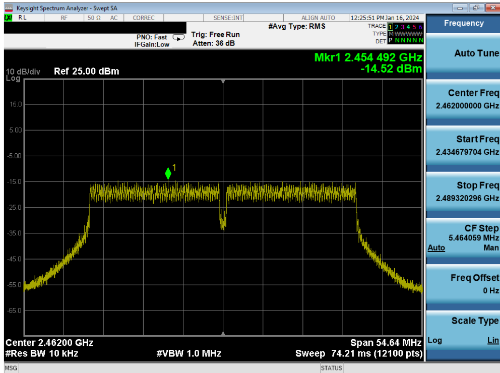
Plot 7-81. Power Spectral Density Plot MIMO ANT1 (802.11ac (2.4GHz - 40MHz) – Ch. 11)
