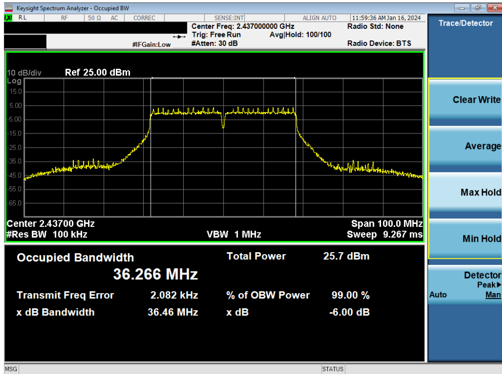
Plot 7-26. 6dB Bandwidth Plot MIMO ANT1 (802.11n (2.4GHz - 40MHz) – Ch. 6)
