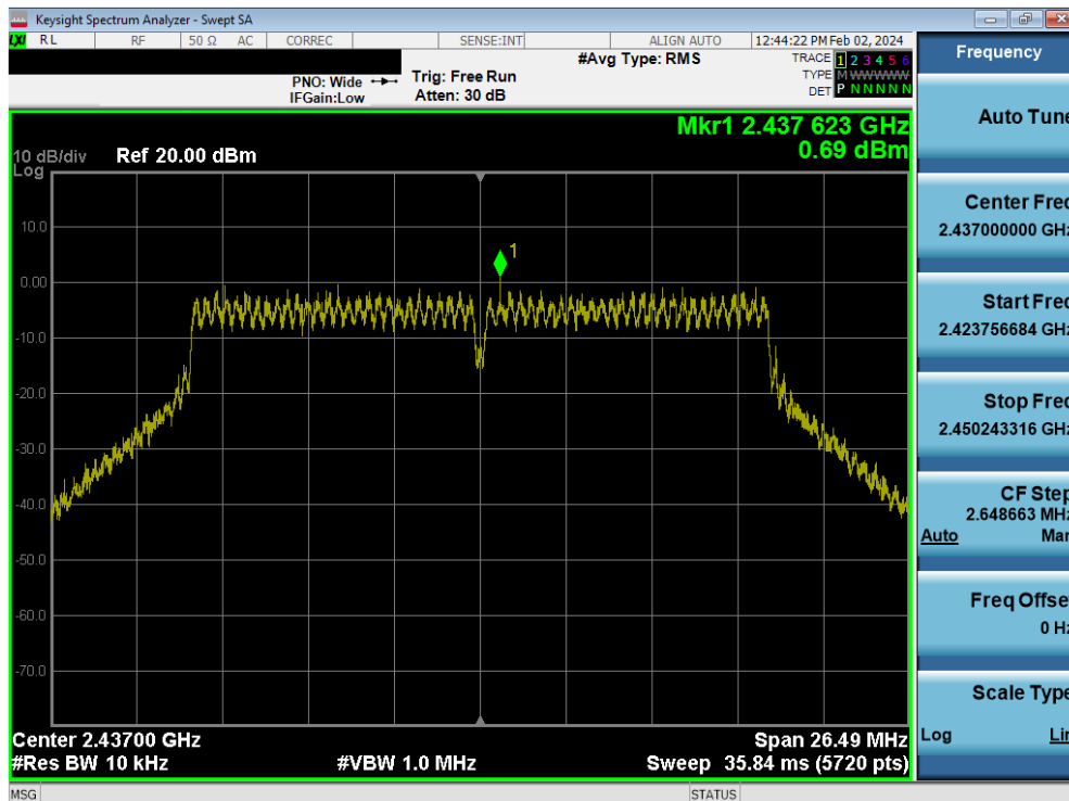
Plot 7-50. Power Spectral Density Plot MIMO ANT1 (802.11n (2.4GHz) – Ch. 6)
