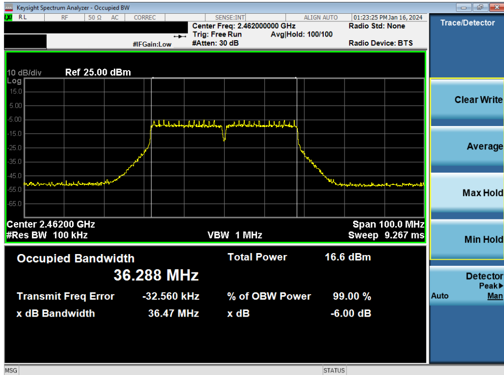
Plot 7-36. 6dB Bandwidth Plot MIMO ANT2 (802.11n (2.4GHz - 40MHz) – Ch. 11)
