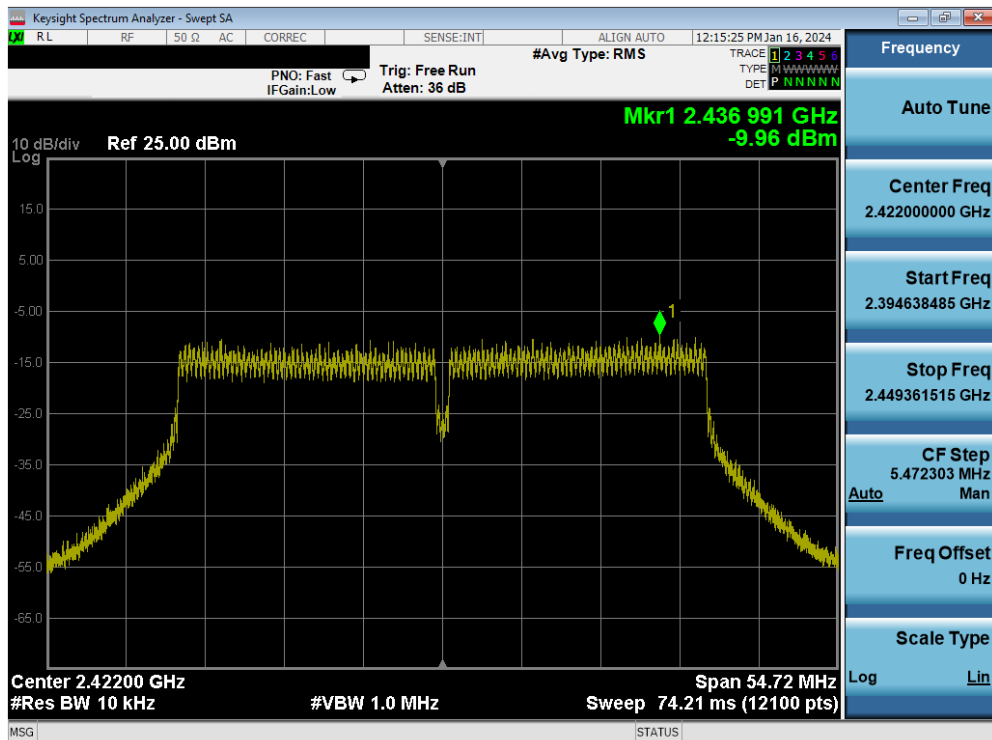
Plot 7-70. Power Spectral Density Plot MIMO ANT1 (802.11ac (2.4GHz - 40MHz) – Ch. 3)
