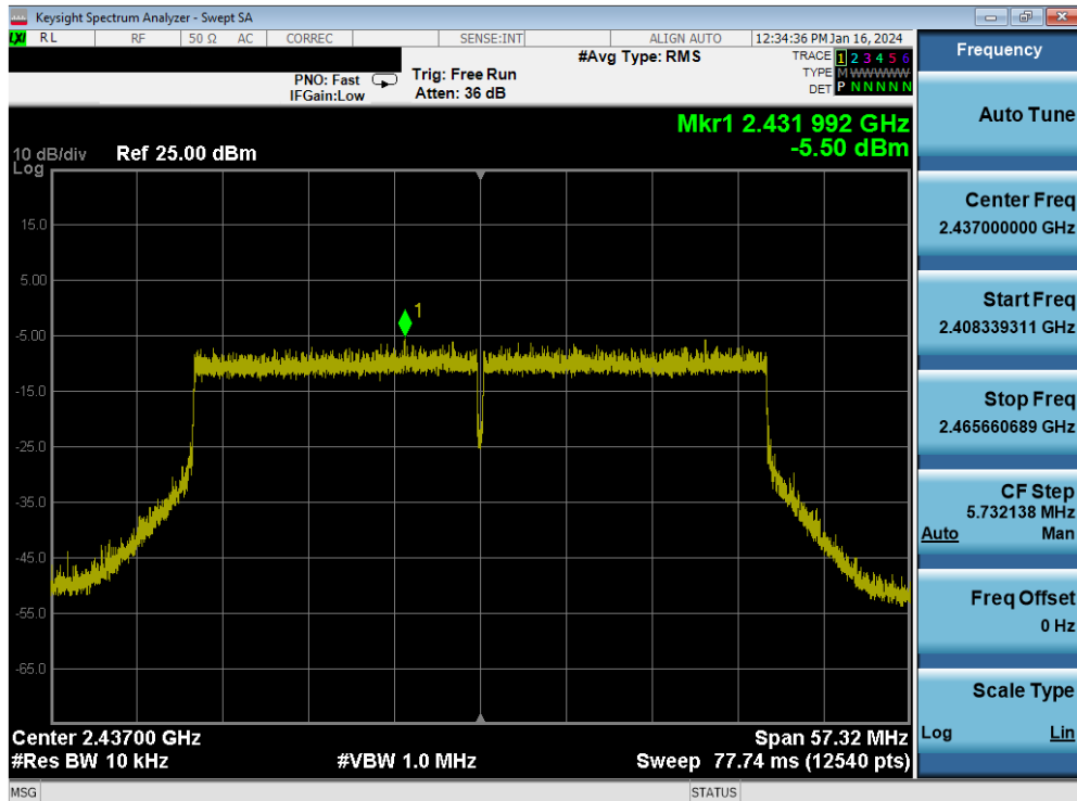
Plot 7-74. Power Spectral Density Plot MIMO ANT1 (802.11be (2.4GHz - 40MHz) – Ch. 6)
