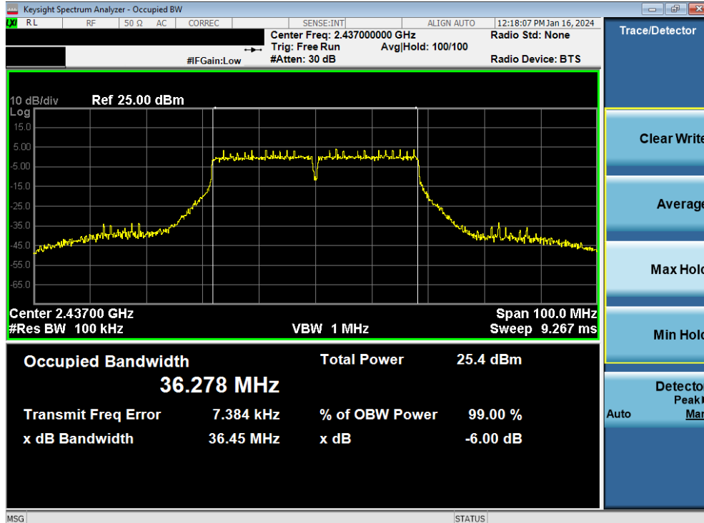
Plot 7-29. 6dB Bandwidth Plot MIMO ANT1 (802.11ac (2.4GHz - 40MHz) – Ch. 6)
