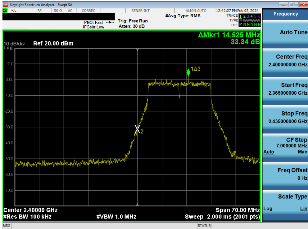
Plot 7-103. Band Edge Plot MIMO ANT1 (802.11n – Ch. 1)
