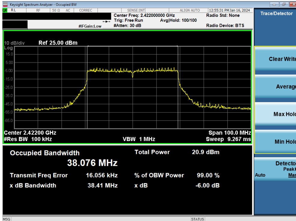
Plot 7-40. 6dB Bandwidth Plot MIMO ANT2 (802.11be (2.4GHz - 40MHz) – Ch. 3)
