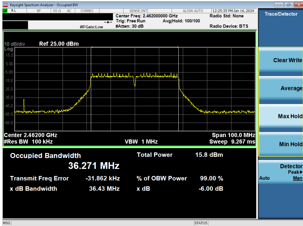
Plot 7-39. 6dB Bandwidth Plot MIMO ANT1 (802.11ac (2.4GHz - 40MHz) – Ch. 11)
