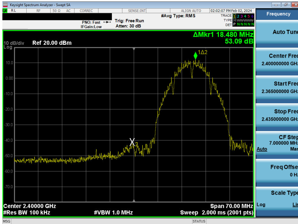
Plot 7-86. Band Edge Plot MIMO ANT1 (802.11b – Ch. 2)
