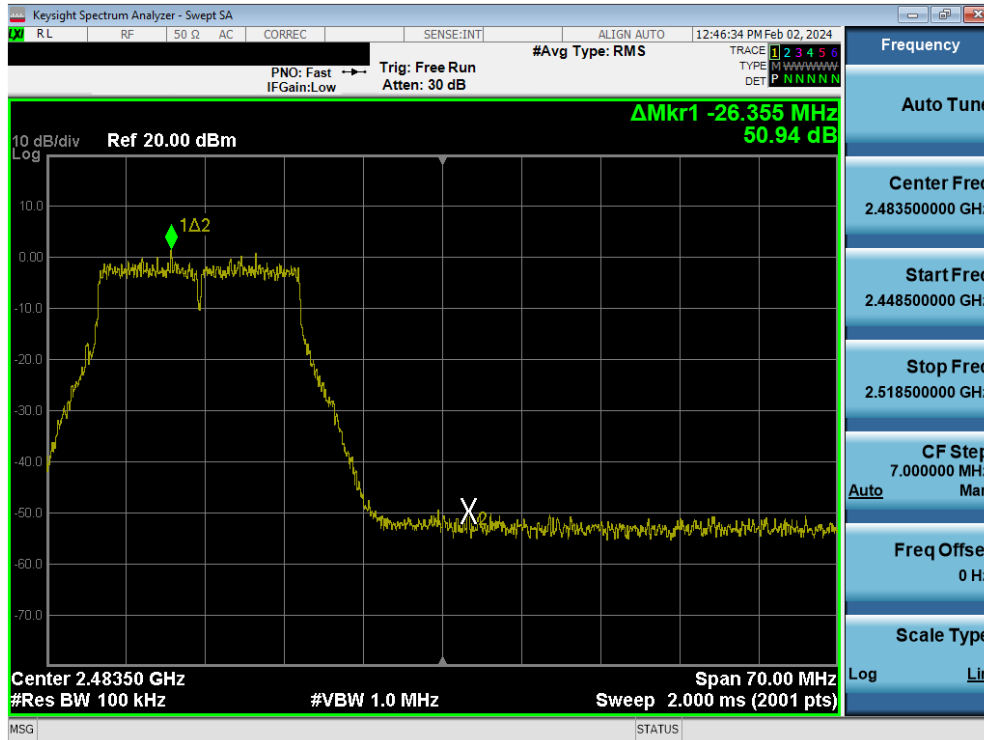
Plot 7-109. Band Edge Plot MIMO ANT1 (802.11n – Ch. 11)
