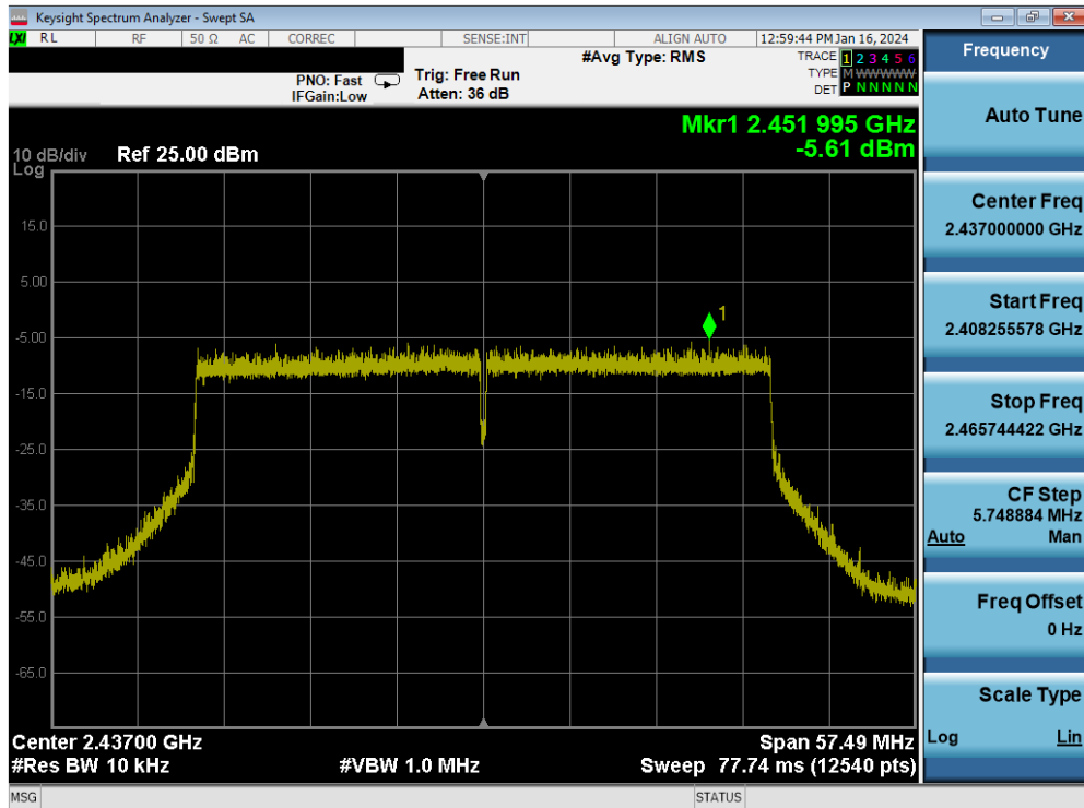
Plot 7-83. Power Spectral Density Plot MIMO ANT2 (802.11be (2.4GHz - 40MHz) – Ch. 6)
