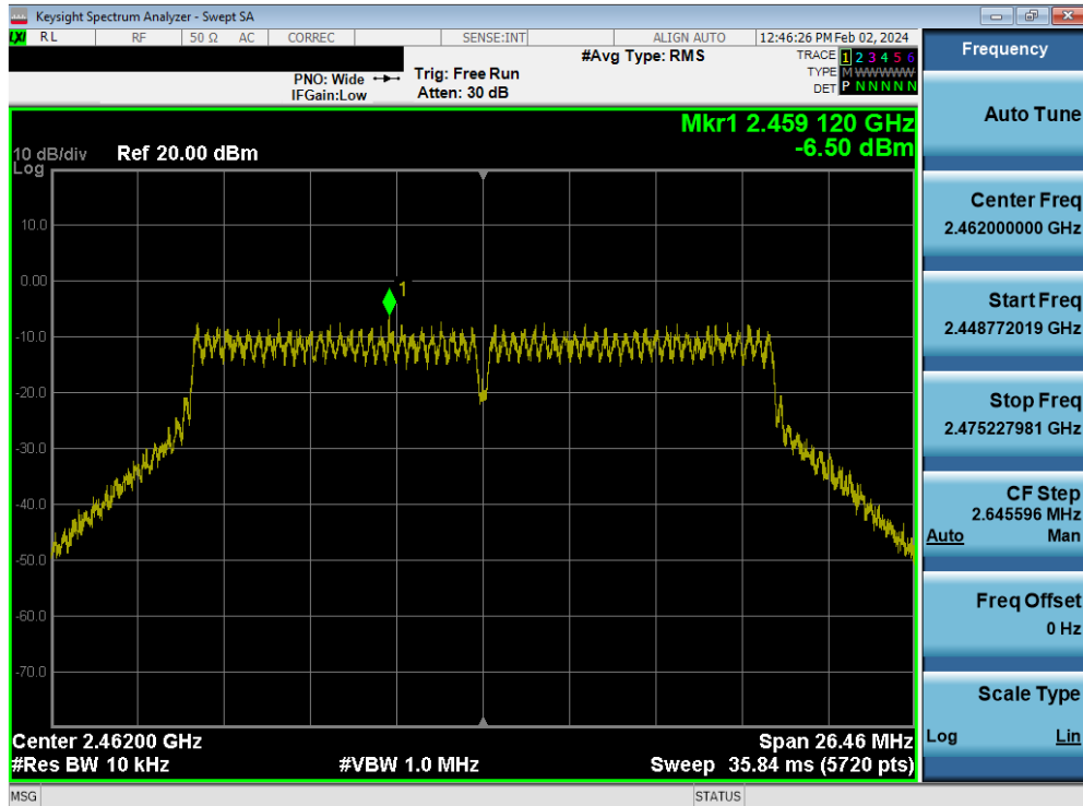
Plot 7-51. Power Spectral Density Plot MIMO ANT1 (802.11n (2.4GHz) – Ch. 11)
