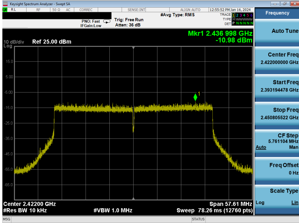
Plot 7-82. Power Spectral Density Plot MIMO ANT2 (802.11be (2.4GHz - 40MHz) – Ch. 3)
