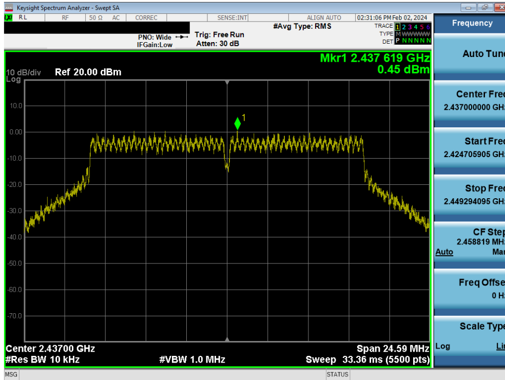
Plot 7-47. Power Spectral Density Plot MIMO ANT1 (802.11g – Ch. 6)
