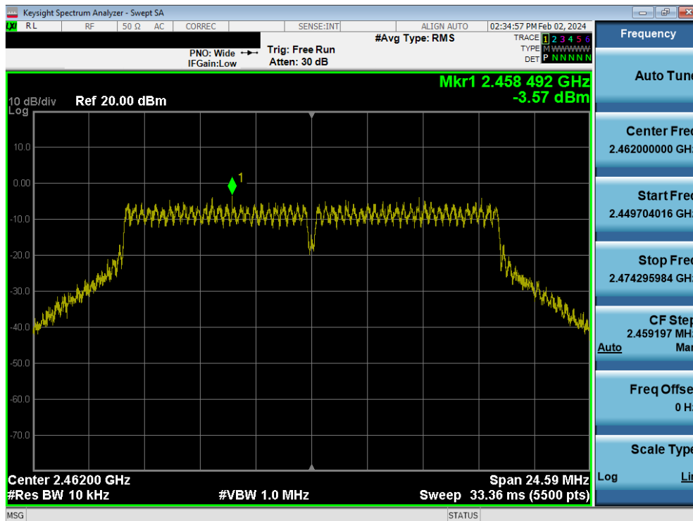
Plot 7-48. Power Spectral Density Plot MIMO ANT1 (802.11g – Ch. 11)
