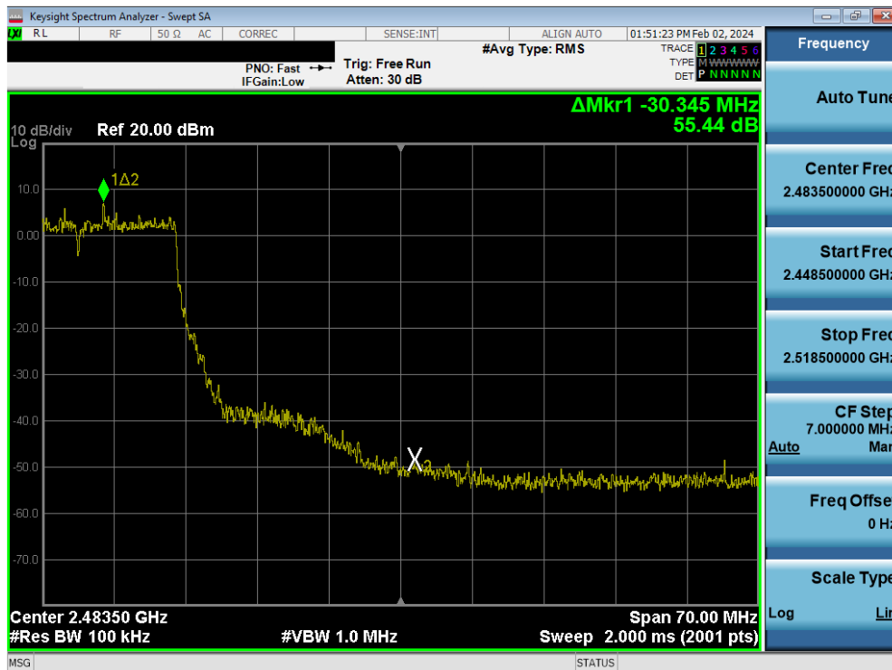
Plot 7-116. Band Edge Plot MIMO ANT1 (802.11be – Ch. 9)
