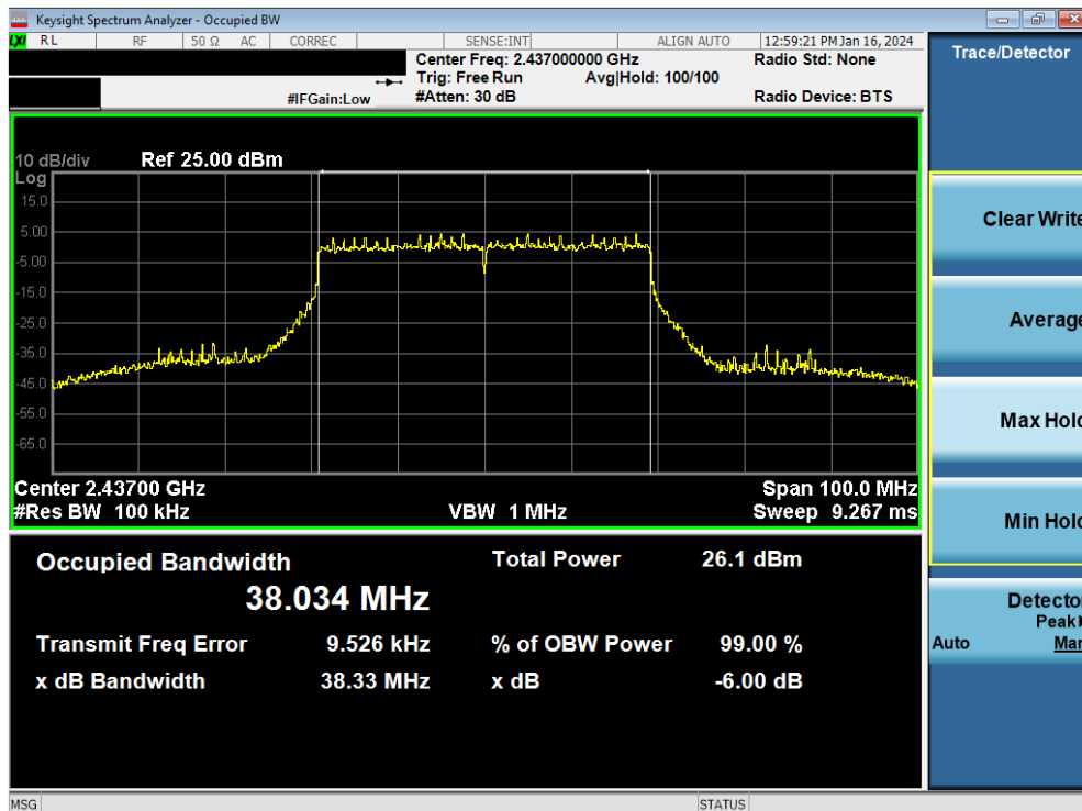
Plot 7-41. 6dB Bandwidth Plot MIMO ANT2 (802.11be (2.4GHz - 40MHz) – Ch. 6)
