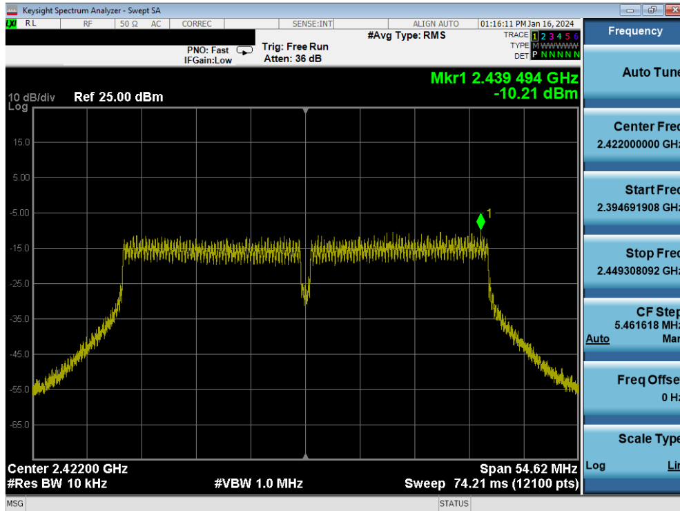
Plot 7-76. Power Spectral Density Plot MIMO ANT2 (802.11n (2.4GHz - 40MHz) – Ch. 3)
