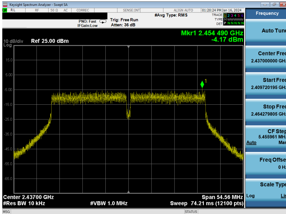
Plot 7-77. Power Spectral Density Plot MIMO ANT2 (802.11n (2.4GHz - 40MHz) – Ch. 6)
