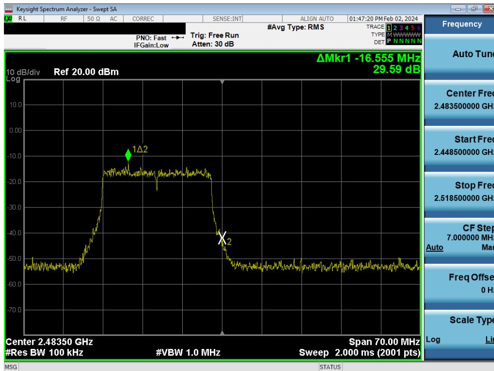
Plot 7-120. Band Edge Plot MIMO ANT1 (802.11be – Ch. 13)
