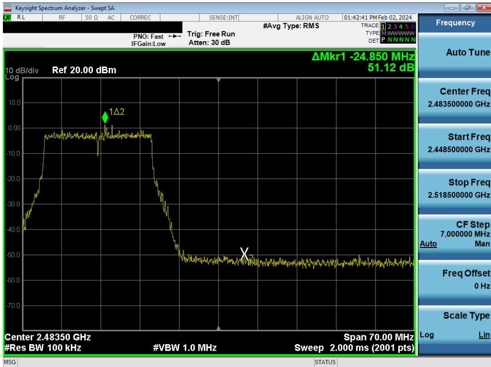
Plot 7-118. Band Edge Plot MIMO ANT1 (802.11be – Ch. 11)
