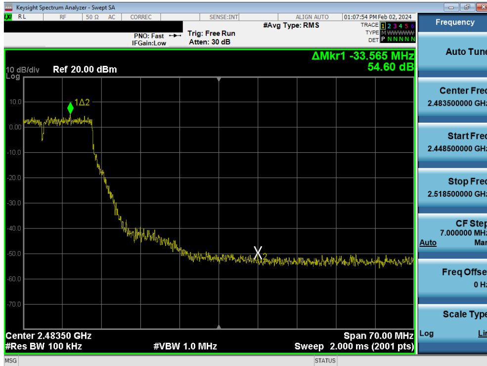
Plot 7-107. Band Edge Plot MIMO ANT1 (802.11n – Ch. 9)
