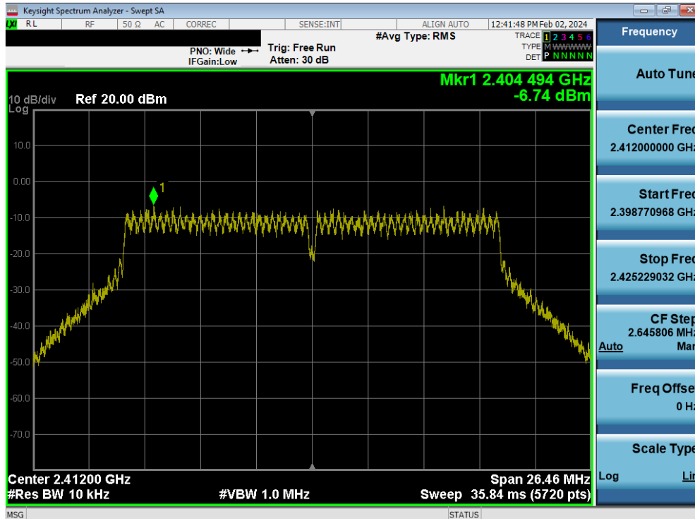
Plot 7-49. Power Spectral Density Plot MIMO ANT1 (802.11n (2.4GHz) – Ch. 1)
