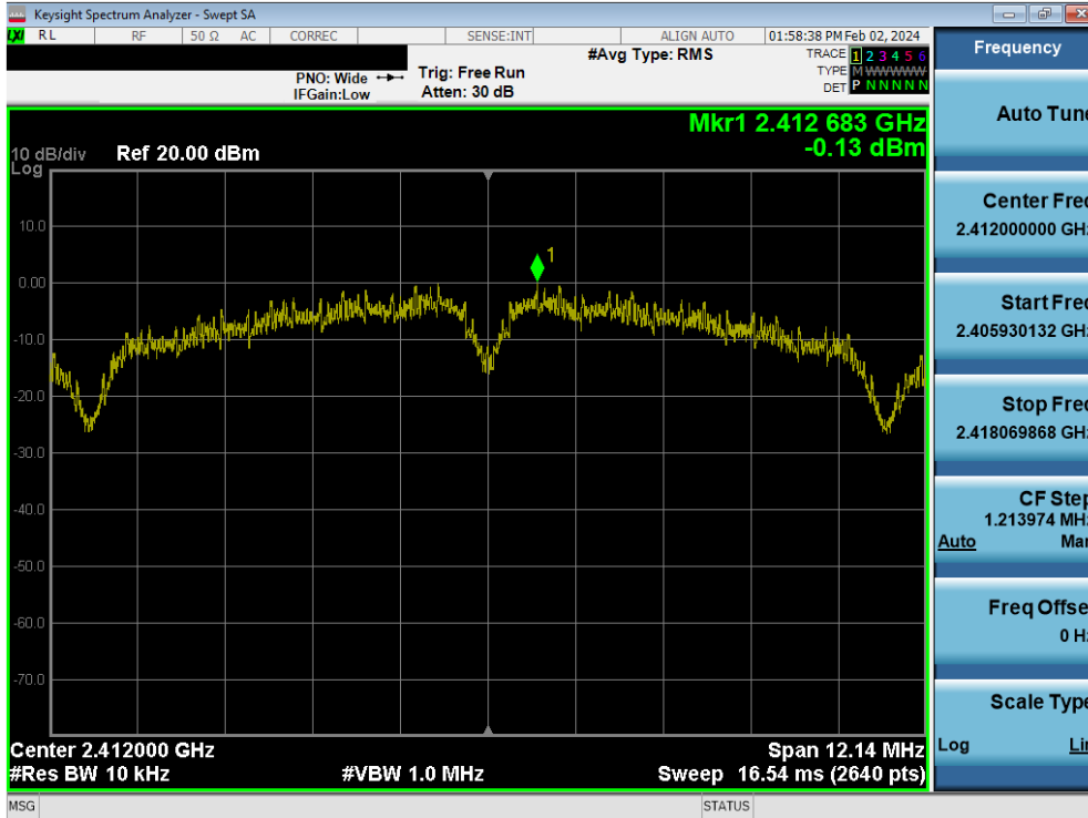
Plot 7-55. Power Spectral Density Plot MIMO ANT2 (802.11b – Ch. 1)
