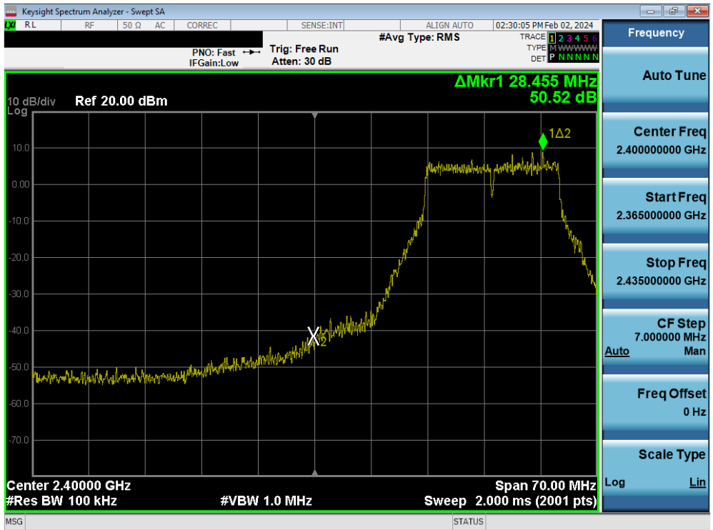
Plot 7-96. Band Edge Plot MIMO ANT1 (802.11g – Ch. 3)
