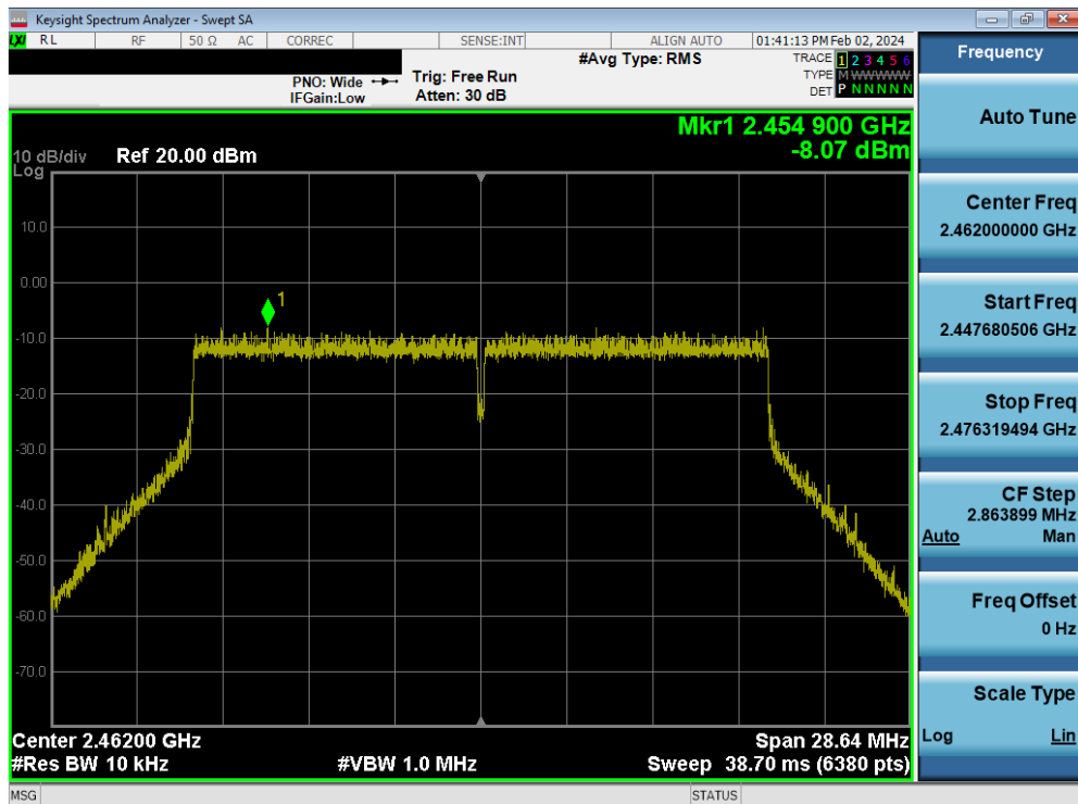
Plot 7-66. Power Spectral Density Plot MIMO ANT2 (802.11be (2.4GHz) – Ch. 11)
