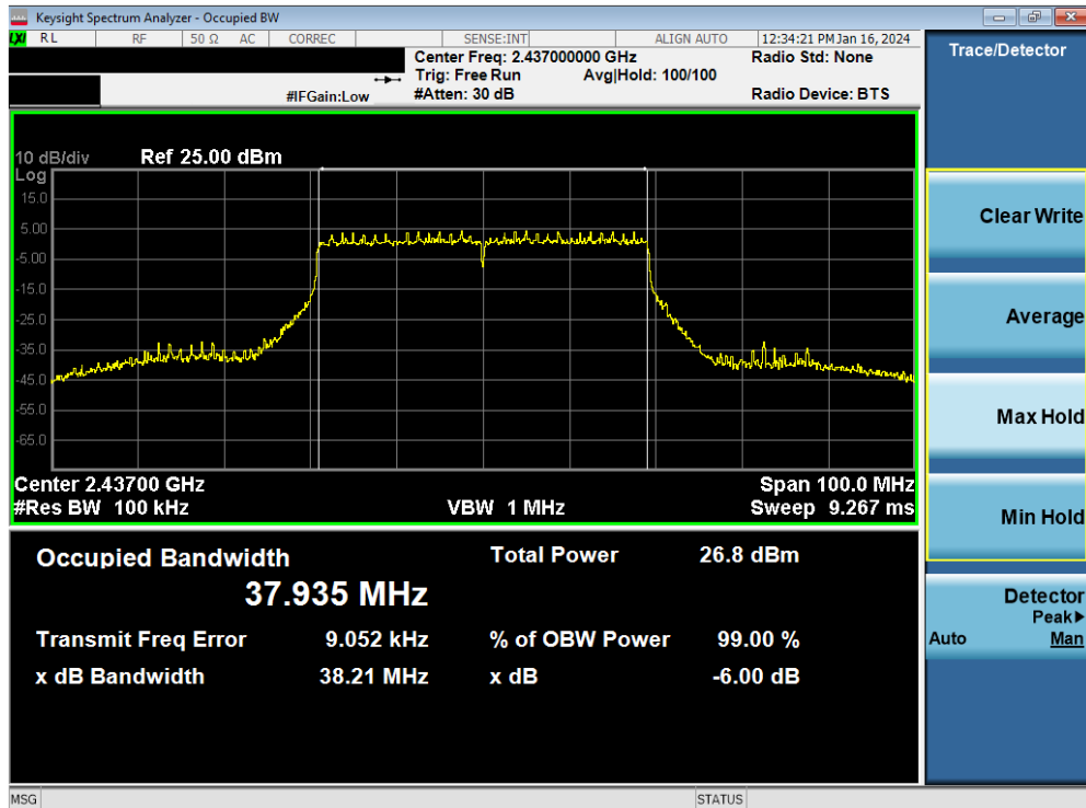
Plot 7-32. 6dB Bandwidth Plot MIMO ANT1 (802.11be (2.4GHz - 40MHz) – Ch. 6)
