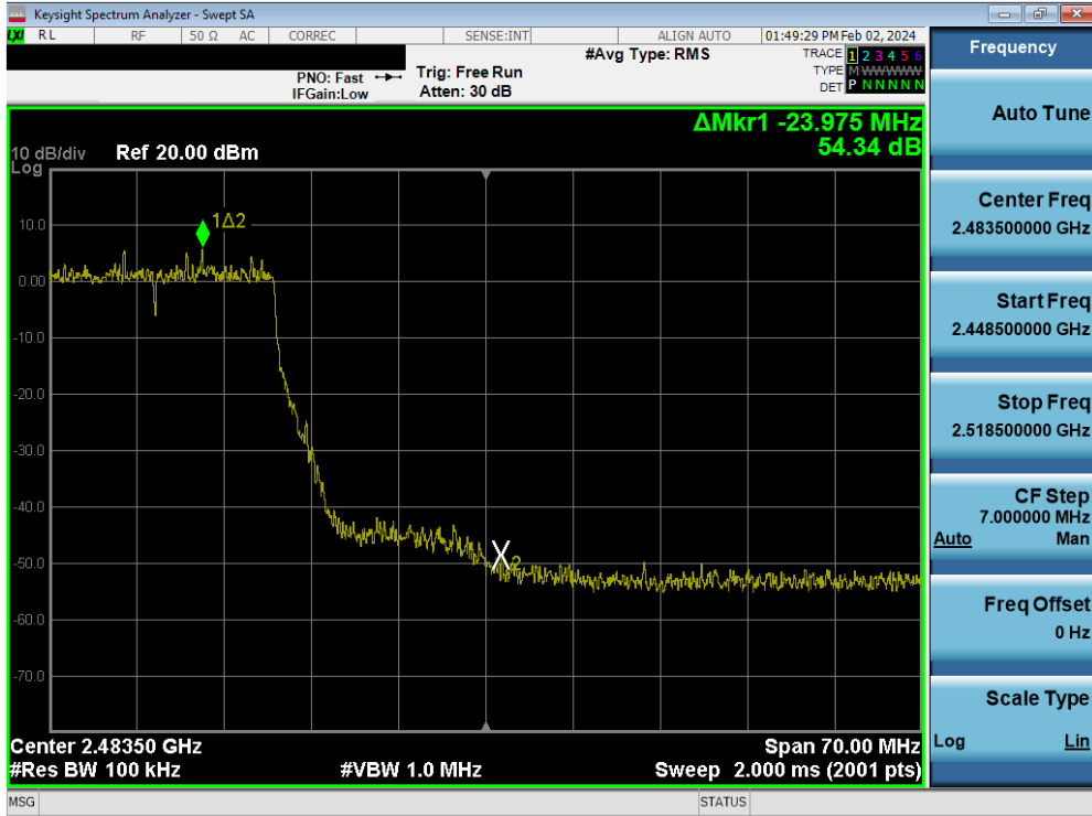
Plot 7-117. Band Edge Plot MIMO ANT1 (802.11be – Ch. 10)
