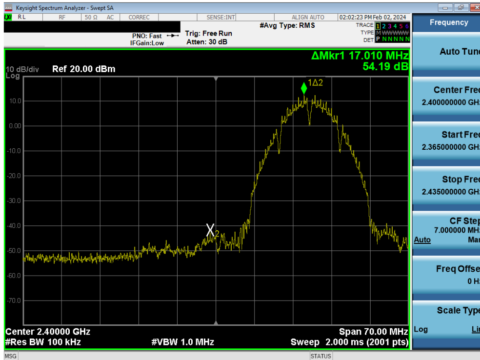
Plot 7-122. Band Edge Plot MIMO ANT2 (802.11b – Ch. 2)
