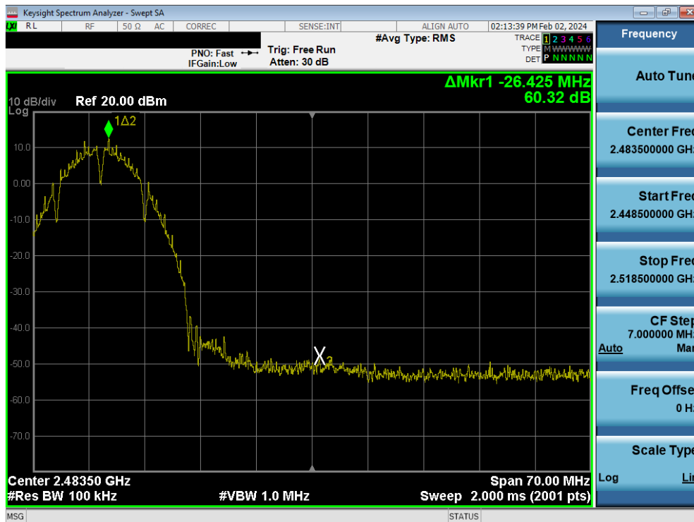
Plot 7-90. Band Edge Plot MIMO ANT1 (802.11b – Ch. 10)
