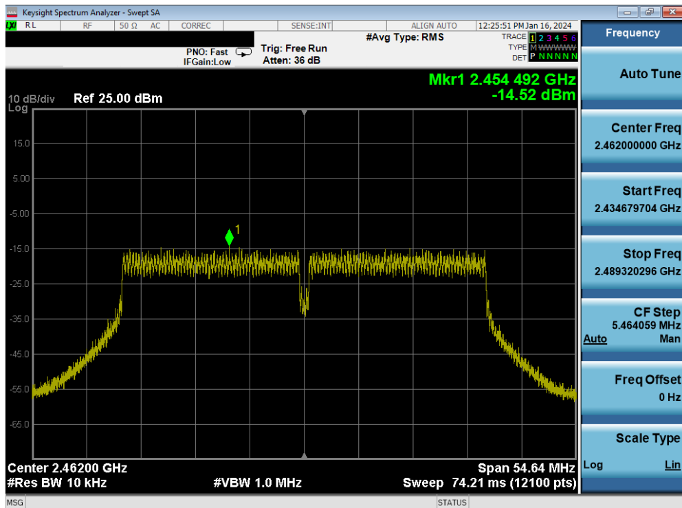
Plot 7-72. Power Spectral Density Plot MIMO ANT1 (802.11ac (2.4GHz - 40MHz) – Ch. 11)
