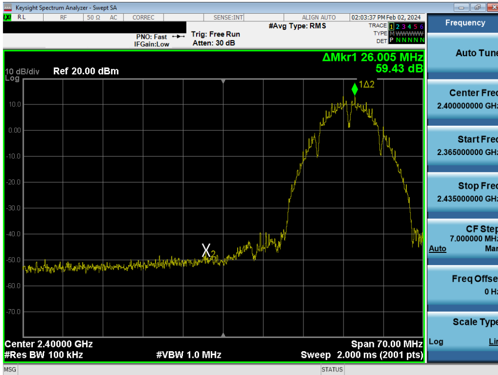
Plot 7-87. Band Edge Plot MIMO ANT1 (802.11b – Ch. 3)
