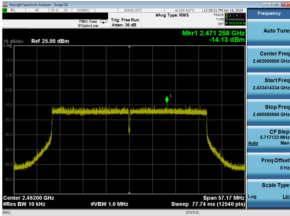
Plot 7-75. Power Spectral Density Plot MIMO ANT1 (802.11be (2.4GHz - 40MHz) – Ch. 11)
