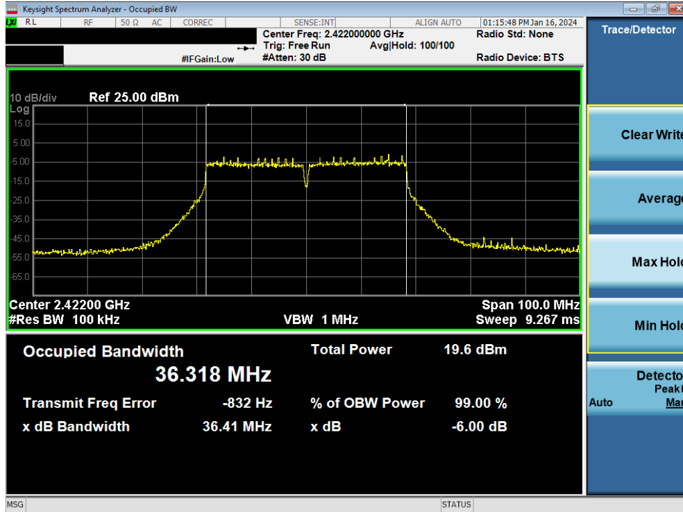
Plot 7-34. 6dB Bandwidth Plot MIMO ANT2 (802.11n (2.4GHz - 40MHz) – Ch. 3)
