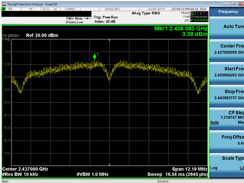
Plot 7-56. Power Spectral Density Plot MIMO ANT2 (802.11b – Ch. 6)
