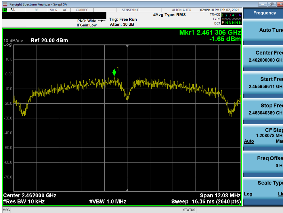
Plot 7-45. Power Spectral Density Plot MIMO ANT1 (802.11b – Ch. 11)
