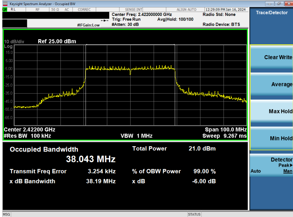
Plot 7-31. 6dB Bandwidth Plot MIMO ANT1 (802.11be (2.4GHz - 40MHz) – Ch. 3)
