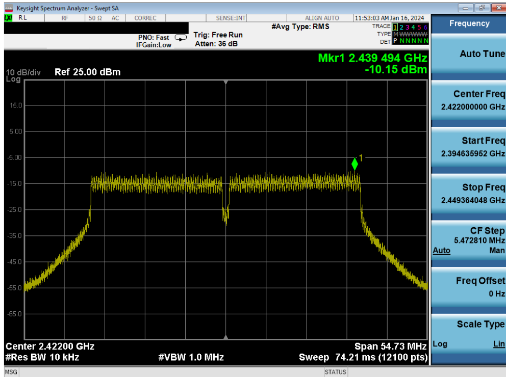
Plot 7-67. Power Spectral Density Plot MIMO ANT1 (802.11n (2.4GHz - 40MHz) – Ch. 3)
