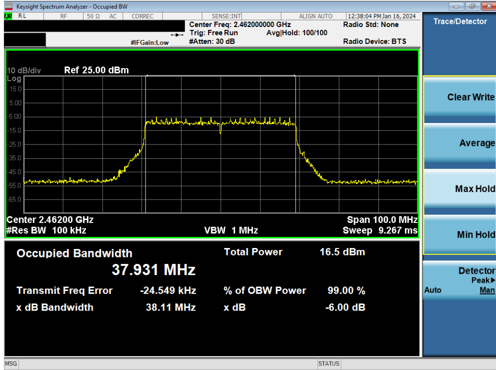
Plot 7-33. 6dB Bandwidth Plot MIMO ANT1 (802.11be (2.4GHz - 40MHz) – Ch. 11)
