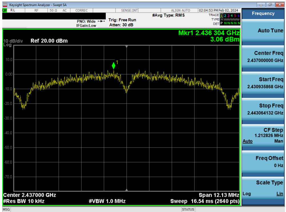
Plot 7-44. Power Spectral Density Plot MIMO ANT1 (802.11b – Ch. 6)
