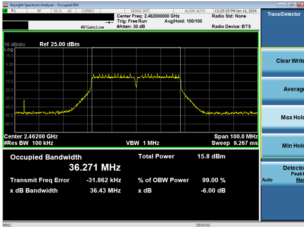
Plot 7-30. 6dB Bandwidth Plot MIMO ANT1 (802.11ac (2.4GHz - 40MHz) – Ch. 11)
