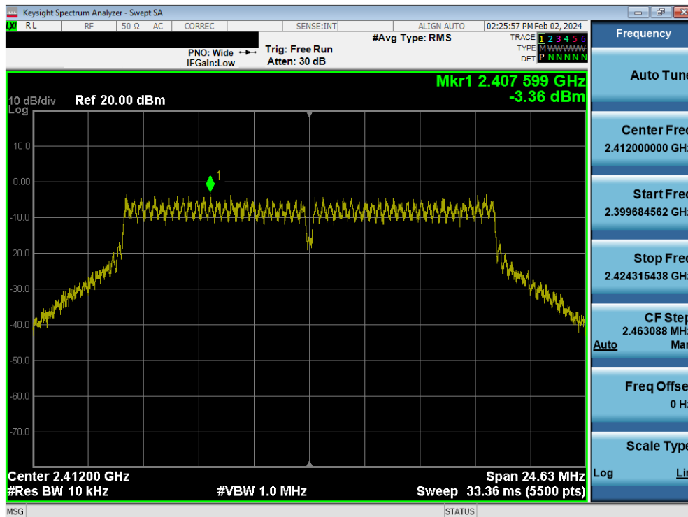
Plot 7-46. Power Spectral Density Plot MIMO ANT1 (802.11g – Ch. 1)
