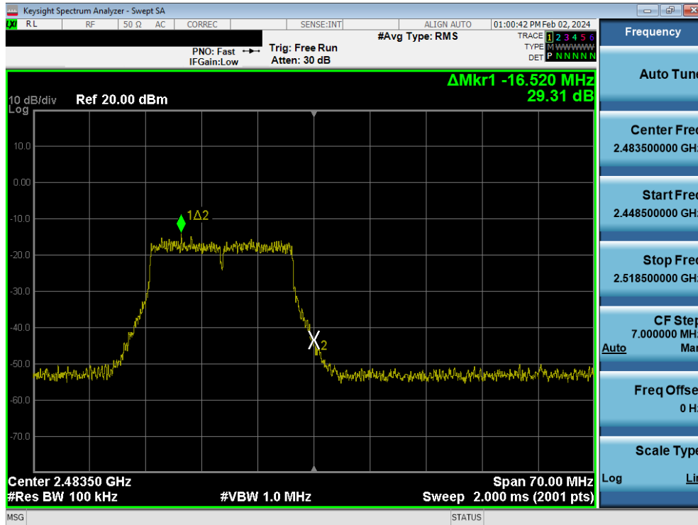
Plot 7-111. Band Edge Plot MIMO ANT1 (802.11n – Ch. 13)
