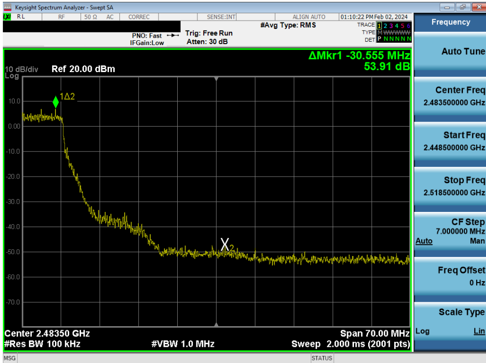
Plot 7-106. Band Edge Plot MIMO ANT1 (802.11n – Ch. 8)
