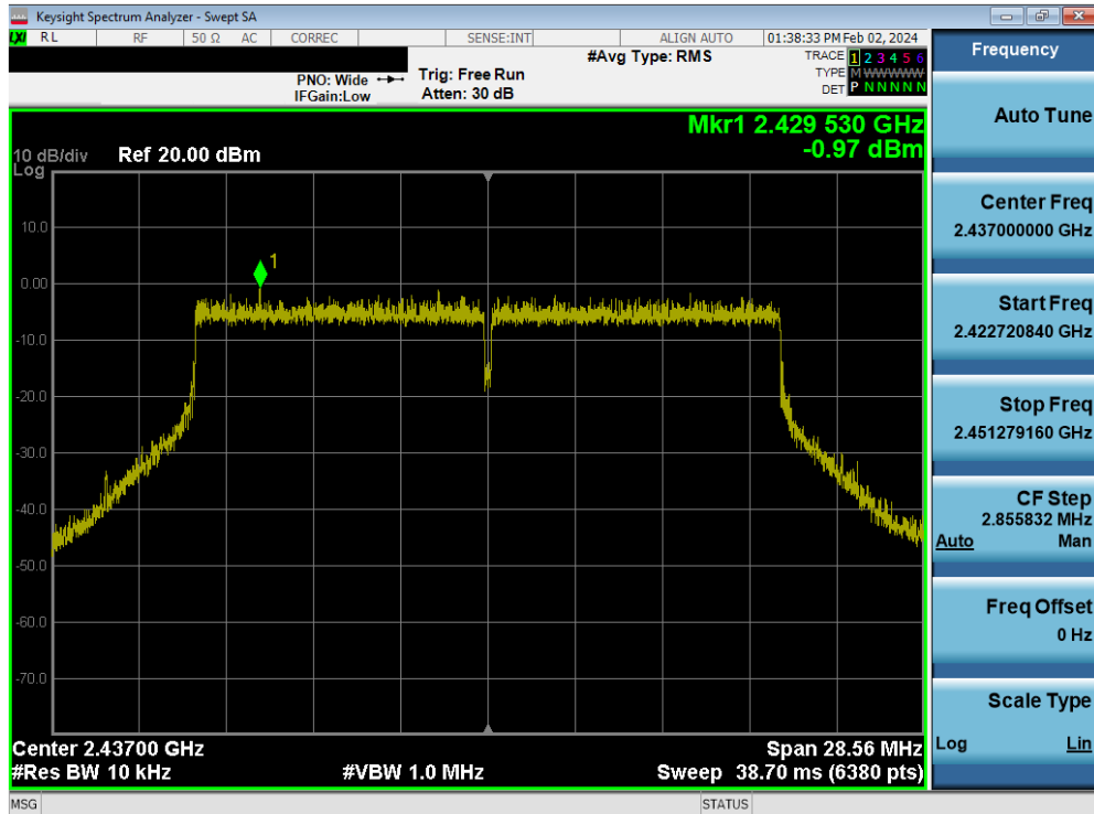
Plot 7-65. Power Spectral Density Plot MIMO ANT2 (802.11be (2.4GHz) – Ch. 6)
