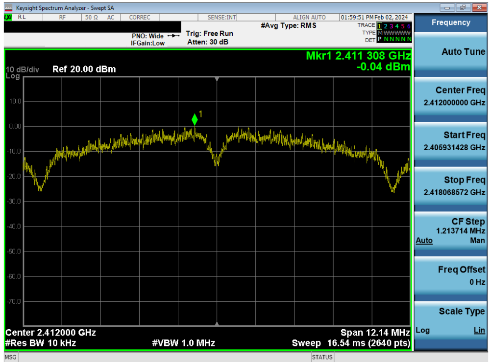
Plot 7-43. Power Spectral Density Plot MIMO ANT1 (802.11b – Ch. 1)
