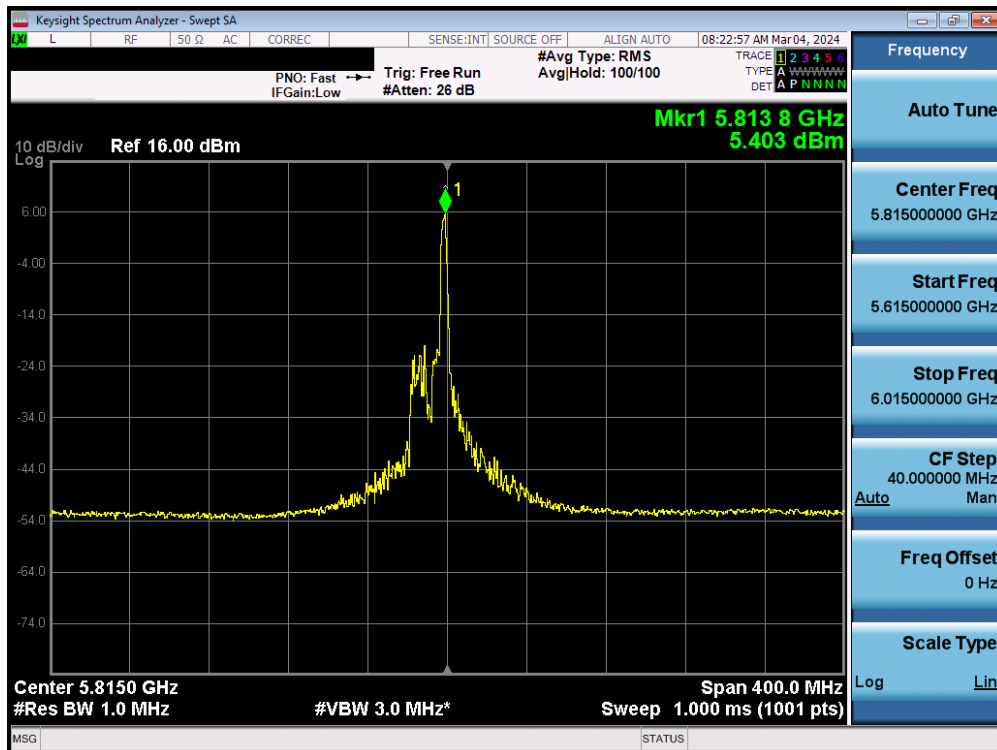
Plot 7-90. Power Spectral Density Plot MIMO ANT1 (160MHz BW 802.11be – 26 Tones (UNII Band 3/4) – Ch. 163)
