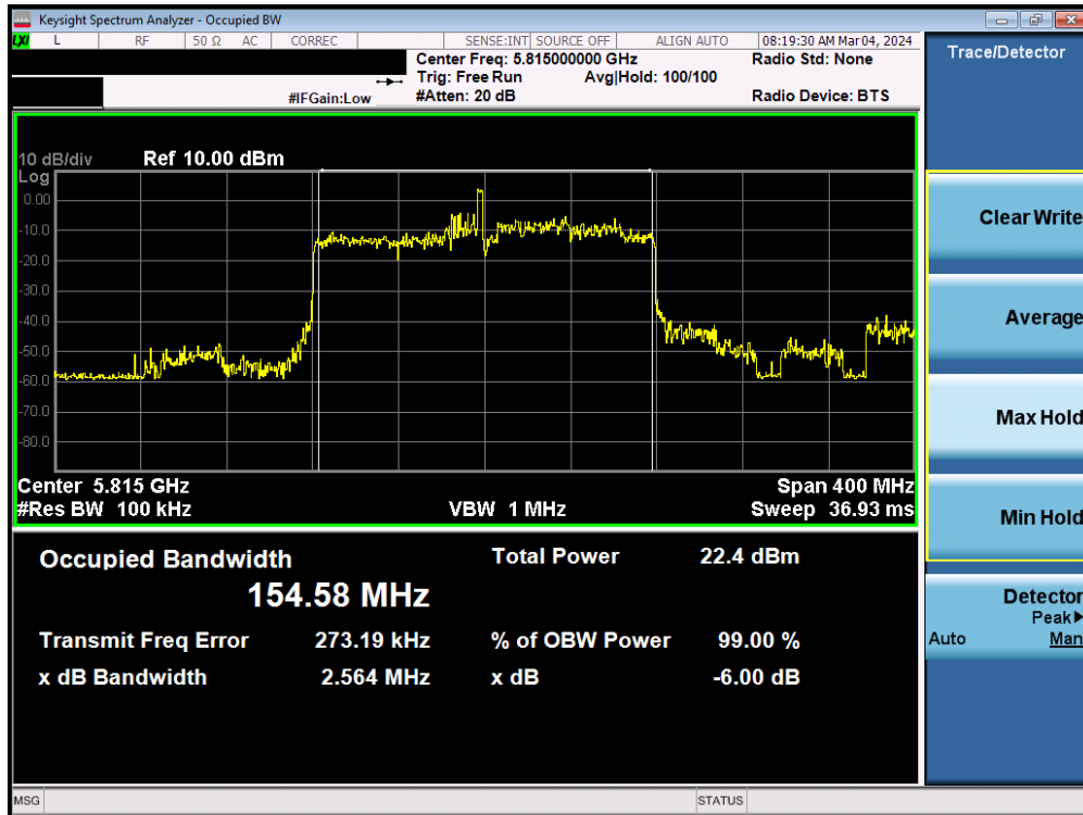
Plot 7-51. 6dB Bandwidth Plot MIMO ANT1 (160MHz BW 802.11be – 26 Tones (UNII Band 3/4) – Ch. 163)
