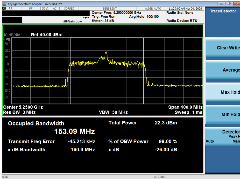
Plot 7-26. 26dB Bandwidth Plot MIMO ANT2 (160MHz BW 802.11be – 26 Tones (UNII Band 1/2A) – Ch. 50)
