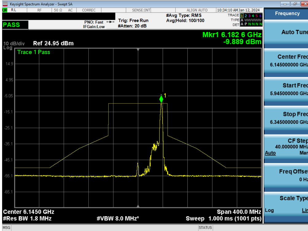
Plot 7-235. In-Band Emission Plot MIMO ANT1 (80MHz BW 802.11be (26 Tones) (UNII Band 5) – Ch. 39) - LPI
