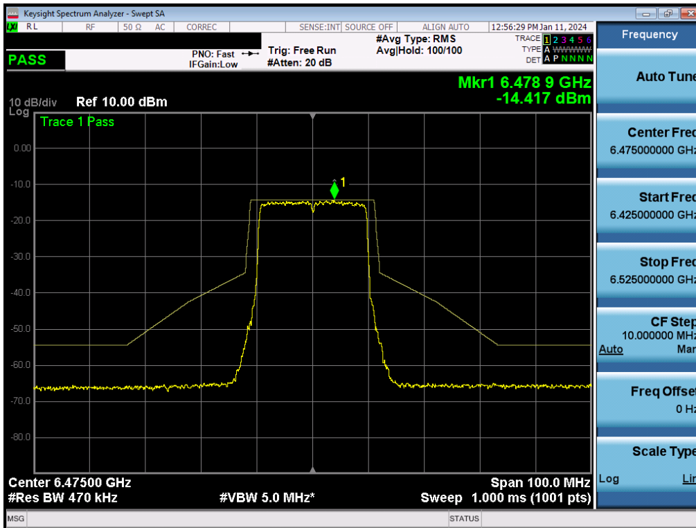
Plot 7-333. In-Band Emission Plot MIMO ANT2 (20MHz BW 802.11be (Full Tone) (UNII Band 6) – Ch. 105) - LPI
