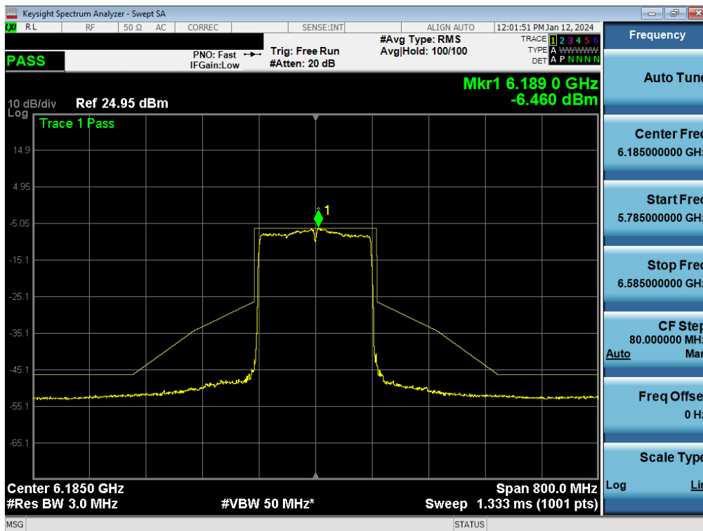
Plot 7-256. In-Band Emission Plot MIMO ANT1 (160MHz BW 802.11be (Full Tone) (UNII Band 5) – Ch. 47) - LPI
