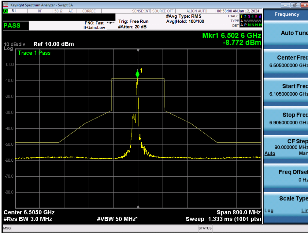
Plot 7-316. In-Band Emission Plot MIMO ANT2 (160MHz BW 802.11be (26 Tones) (UNII Band 6) – Ch. 111) - LPI
