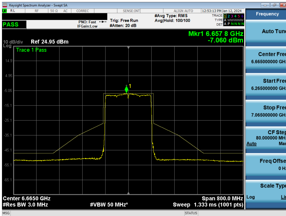
Plot 7-266. In-Band Emission Plot MIMO ANT1 (160MHz BW 802.11be (Full Tone) (UNII Band 7) – Ch. 143) - LPI
