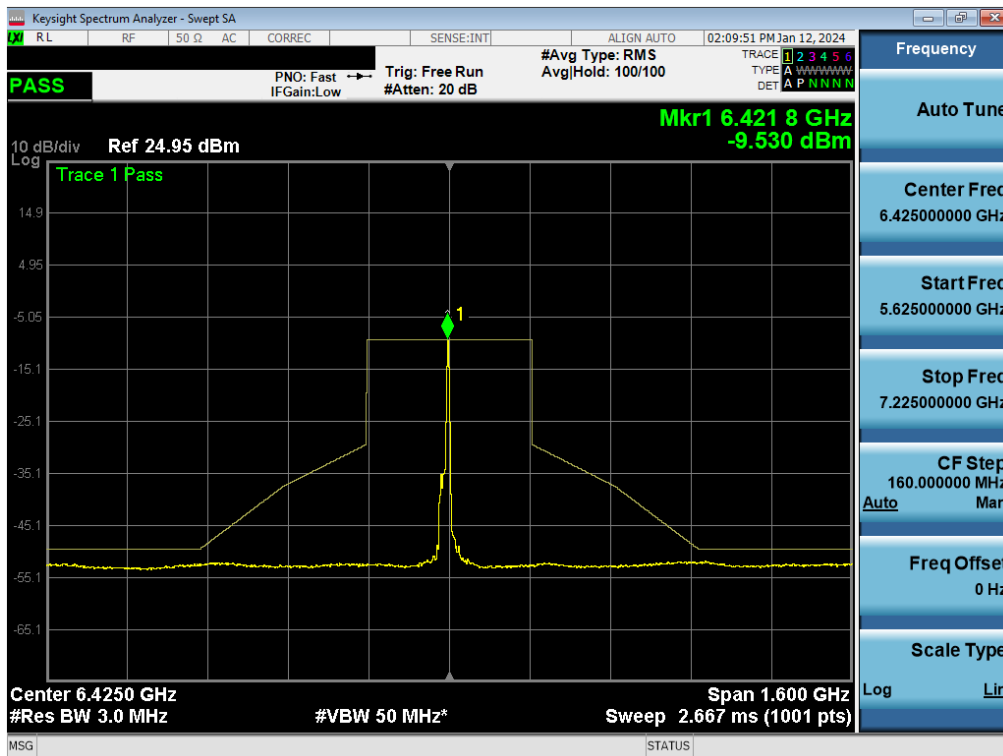
Plot 7-242. In-Band Emission Plot MIMO ANT1 (320MHz BW 802.11be (26 Tones) (UNII Band 6) – Ch. 95) - LPI
