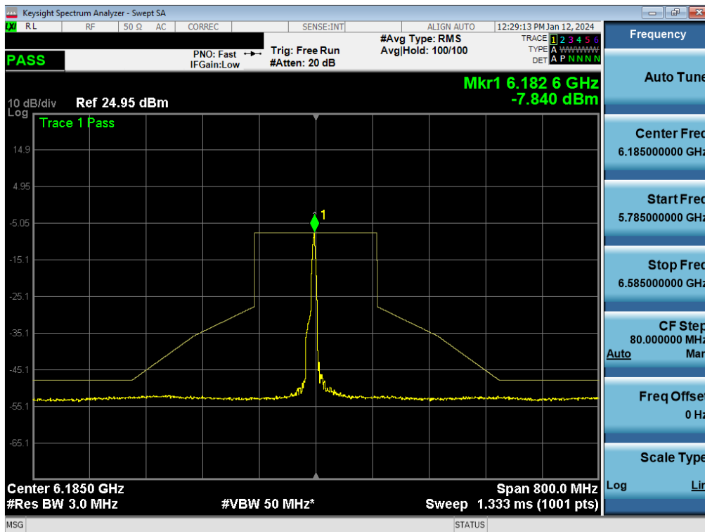
Plot 7-236. In-Band Emission Plot MIMO ANT1 (160MHz BW 802.11be (26 Tones) (UNII Band 5) – Ch. 47) - LPI
