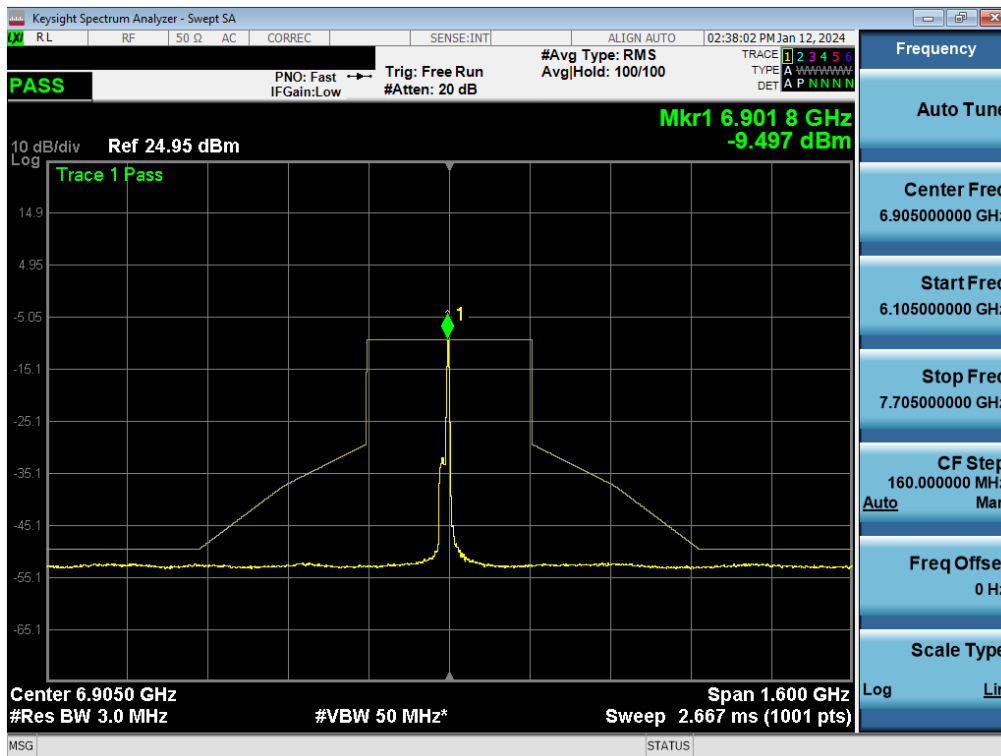
Plot 7-252. In-Band Emission Plot MIMO ANT1 (320MHz BW 802.11be (26 Tones) (UNII Band 8) – Ch. 191) - LPI
