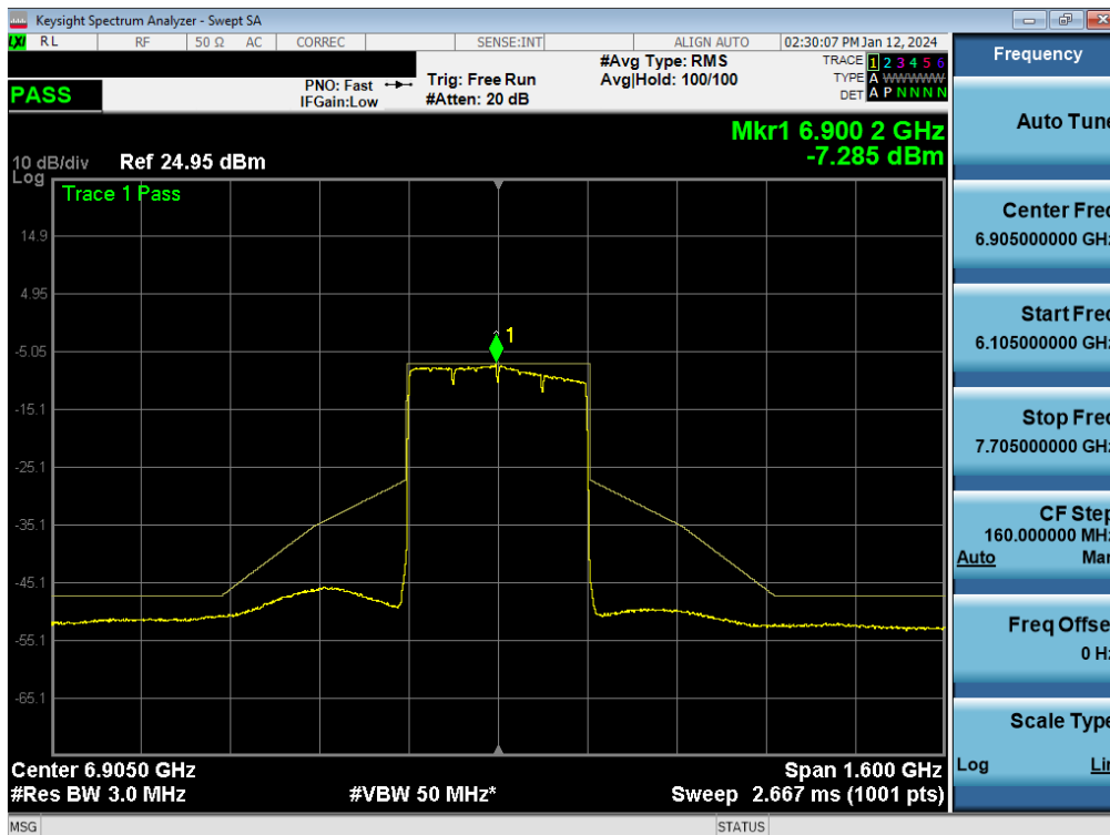
Plot 7-272. In-Band Emission Plot MIMO ANT1 (320MHz BW 802.11be (Full Tone) (UNII Band 8) – Ch. 191) - LPI
