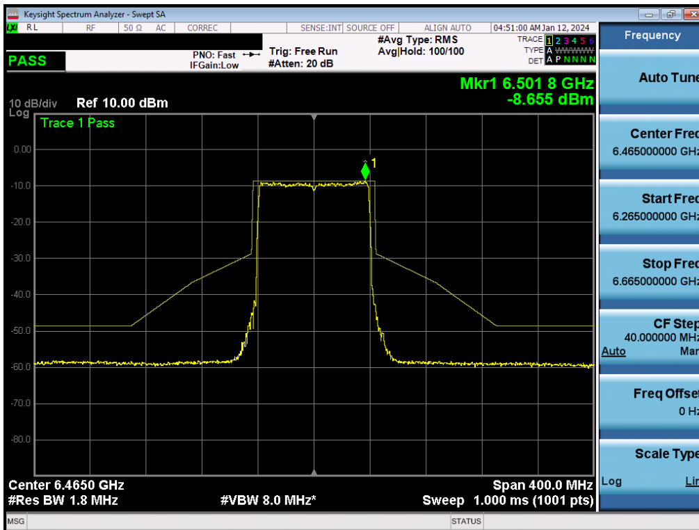
Plot 7-335. In-Band Emission Plot MIMO ANT2 (80MHz BW 802.11be (Full Tone) (UNII Band 6) – Ch. 103) - LPI
