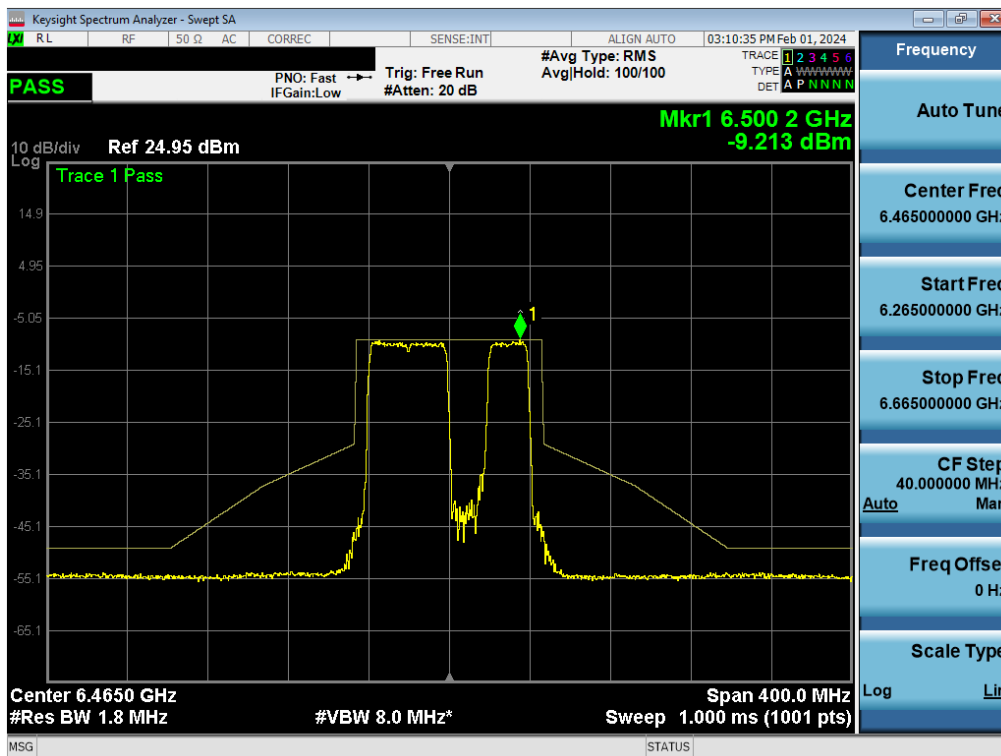
Plot 7-276. In-Band Emission Plot MIMO ANT1 (80MHz BW 802.11be (484+242 Tone) (UNII Band 6) – Ch. 103) - LPI
