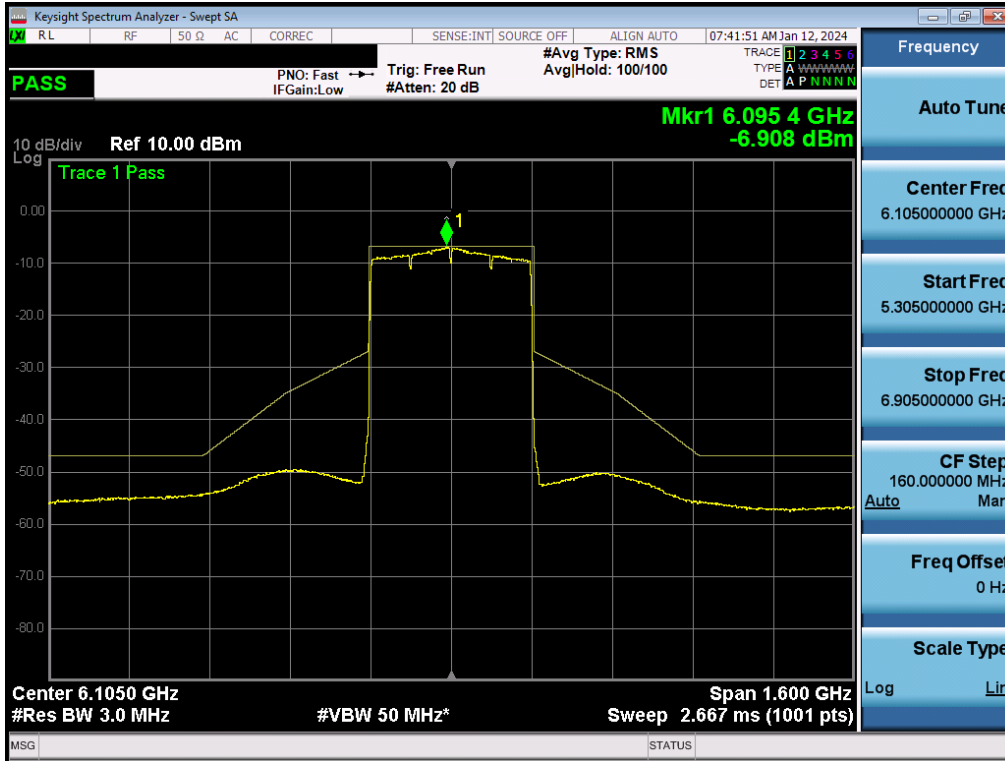
Plot 7-332. In-Band Emission Plot MIMO ANT2 (320MHz BW 802.11be (Full Tone) (UNII Band 5) – Ch. 31) - LPI
