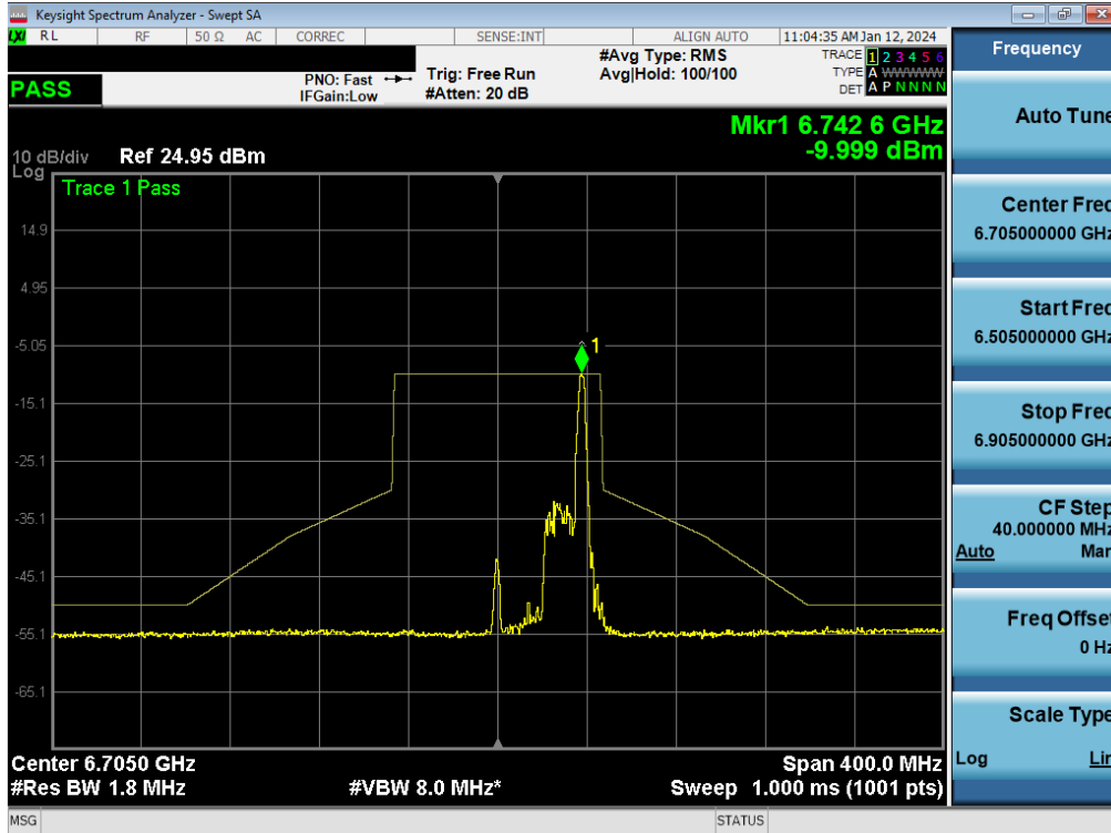
Plot 7-245. In-Band Emission Plot MIMO ANT1 (80MHz BW 802.11be (26 Tones) (UNII Band 7) – Ch. 151) - LPI
