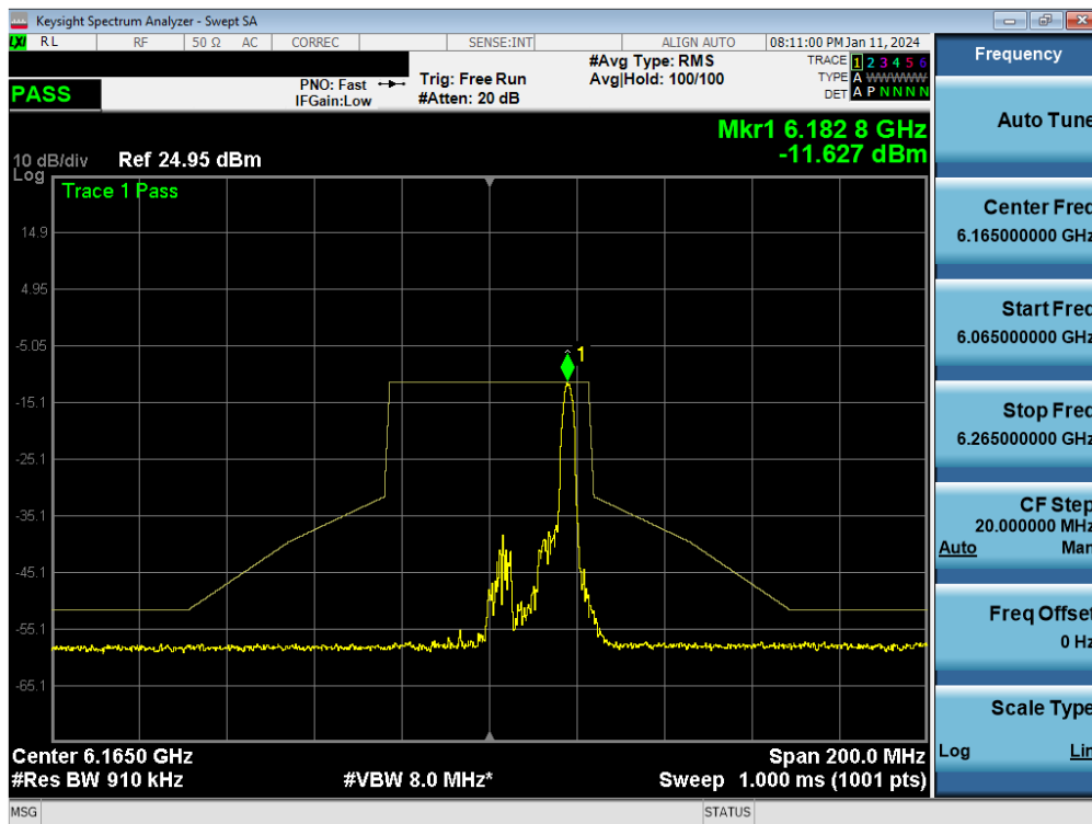
Plot 7-234. In-Band Emission Plot MIMO ANT1 (40MHz BW 802.11be (26 Tones) (UNII Band 5) – Ch. 43) - LPI
