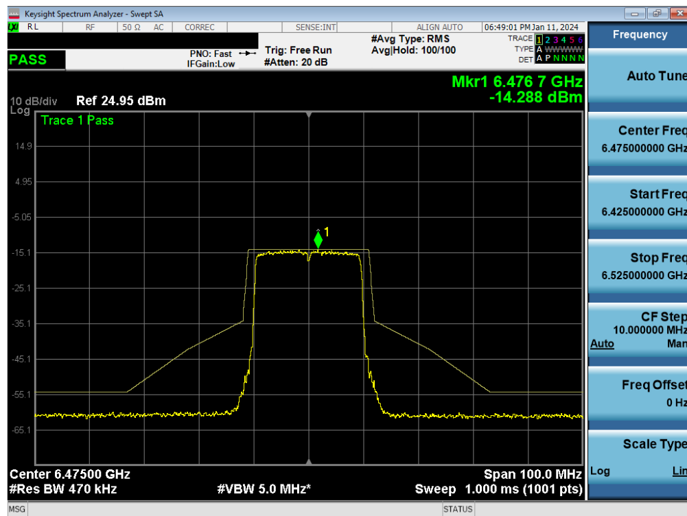
Plot 7-258. In-Band Emission Plot MIMO ANT1 (20MHz BW 802.11be (Full Tone) (UNII Band 6) – Ch. 105) - LPI
