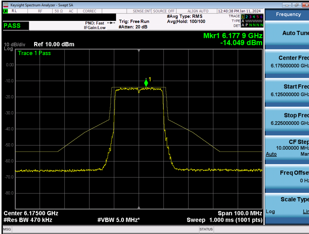
Plot 7-328. In-Band Emission Plot MIMO ANT2 (20MHz BW 802.11be (Full Tone) (UNII Band 5) – Ch. 45) - LPI
