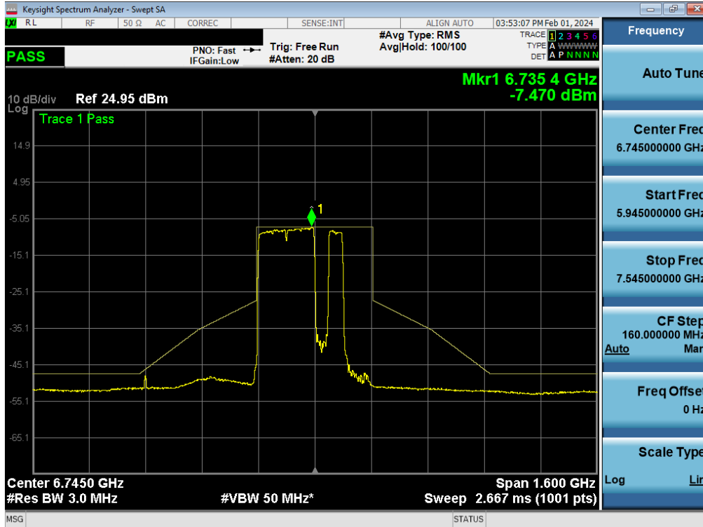
Plot 7-281. In-Band Emission Plot MIMO ANT1 (320MHz BW 802.11be (2*996+484 Tone) (UNII Band 7) – Ch. 159) - LPI
