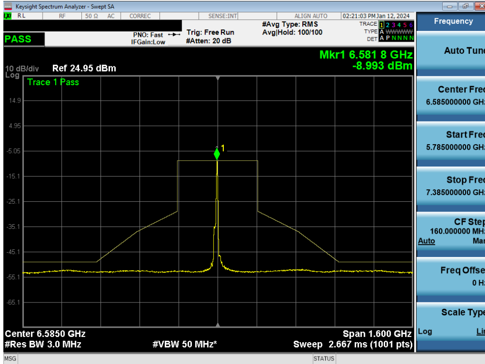
Plot 7-247. In-Band Emission Plot MIMO ANT1 (320MHz BW 802.11be (26 Tones) (UNII Band 7) – Ch. 127) - LPI
