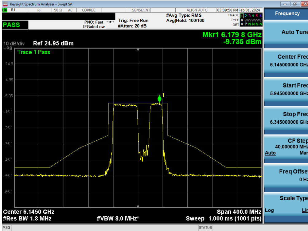
Plot 7-273. In-Band Emission Plot MIMO ANT1 (80MHz BW 802.11be (484+242 Tone) (UNII Band 5) – Ch. 39) - LPI
