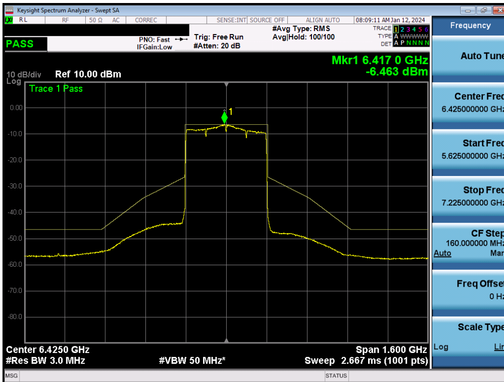
Plot 7-337. In-Band Emission Plot MIMO ANT2 (320MHz BW 802.11be (Full Tone) (UNII Band 6) – Ch. 95) - LPI
