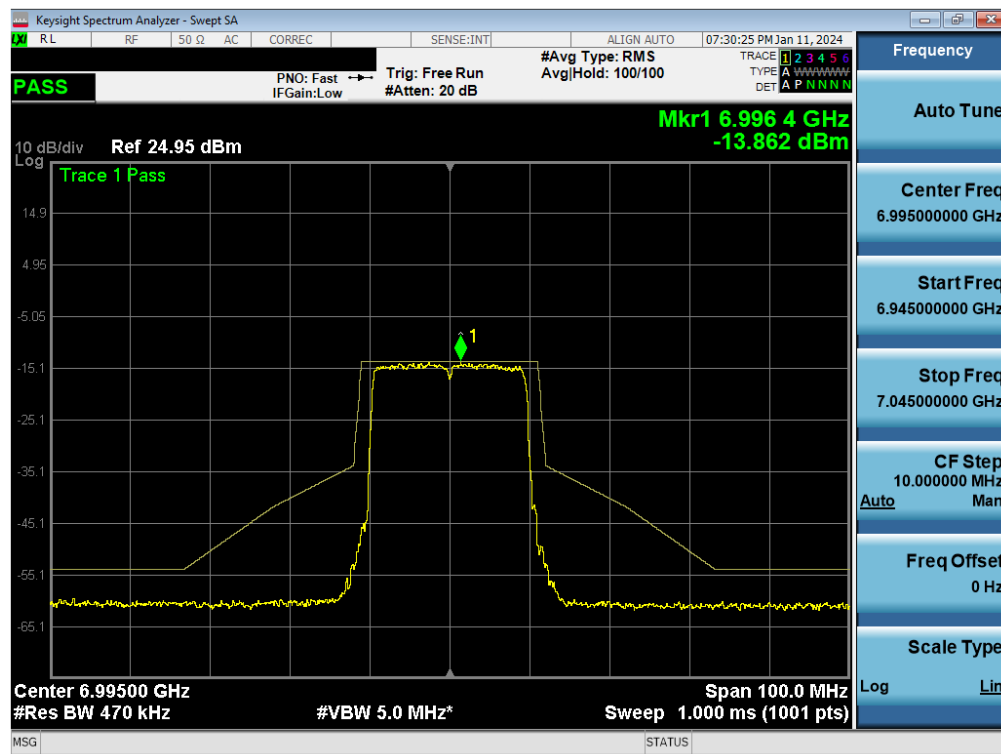
Plot 7-268. In-Band Emission Plot MIMO ANT1 (20MHz BW 802.11be (Full Tone) (UNII Band 8) – Ch. 209) - LPI
