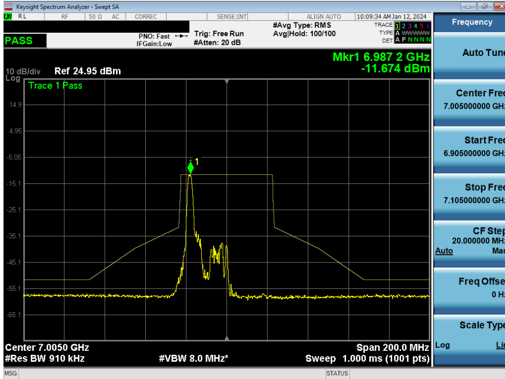
Plot 7-249. In-Band Emission Plot MIMO ANT1 (40MHz BW 802.11be (26 Tones) (UNII Band 8) – Ch. 211) - LPI
