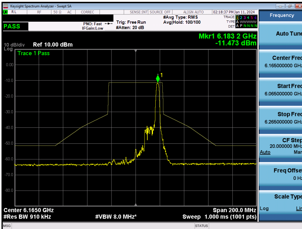
Plot 7-309. In-Band Emission Plot MIMO ANT2 (40MHz BW 802.11be (26 Tones) (UNII Band 5) – Ch. 43) - LPI
