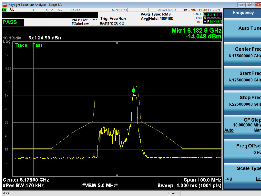
Plot 7-233. In-Band Emission Plot MIMO ANT1 (20MHz BW 802.11be (26 Tones) (UNII Band 5) – Ch. 45) - LPI
