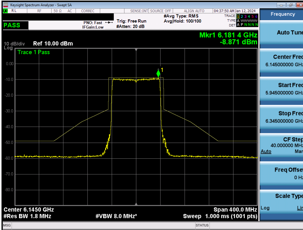
Plot 7-330. In-Band Emission Plot MIMO ANT2 (80MHz BW 802.11be (Full Tone) (UNII Band 5) – Ch. 39) - LPI
