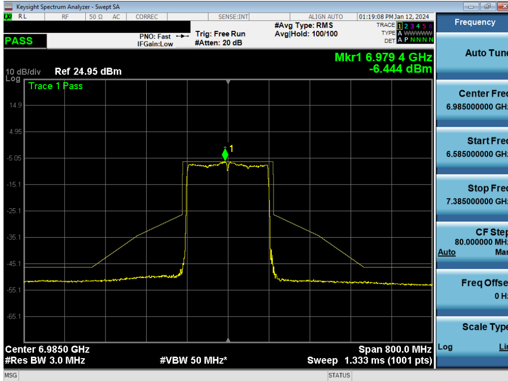
Plot 7-271. In-Band Emission Plot MIMO ANT1 (160MHz BW 802.11be (Full Tone) (UNII Band 8) – Ch. 207) - LPI
