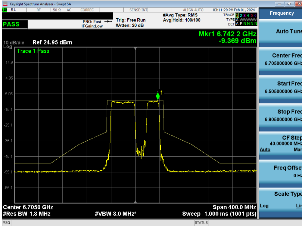
Plot 7-279. In-Band Emission Plot MIMO ANT1 (80MHz BW 802.11be (484+242 Tone) (UNII Band 7) – Ch. 151) - LPI
