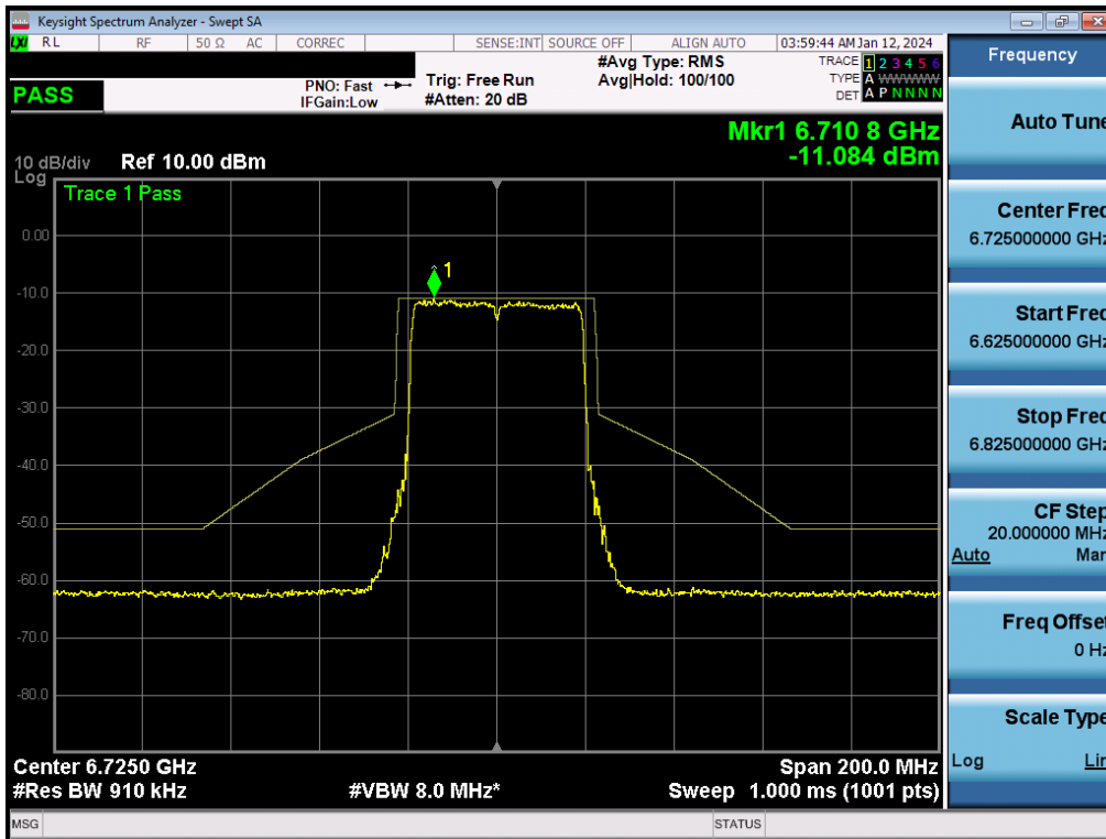
Plot 7-339. In-Band Emission Plot MIMO ANT2 (40MHz BW 802.11be (Full Tone) (UNII Band 7) – Ch. 155) - LPI
