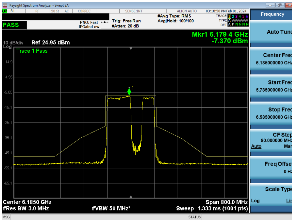
Plot 7-274. In-Band Emission Plot MIMO ANT1 (160MHz BW 802.11be (996+484 Tone) (UNII Band 5) – Ch. 47) - LPI
