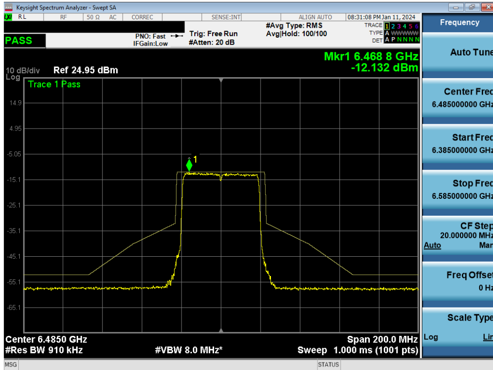
Plot 7-259. In-Band Emission Plot MIMO ANT1 (40MHz BW 802.11be (Full Tone) (UNII Band 6) – Ch. 107) - LPI
