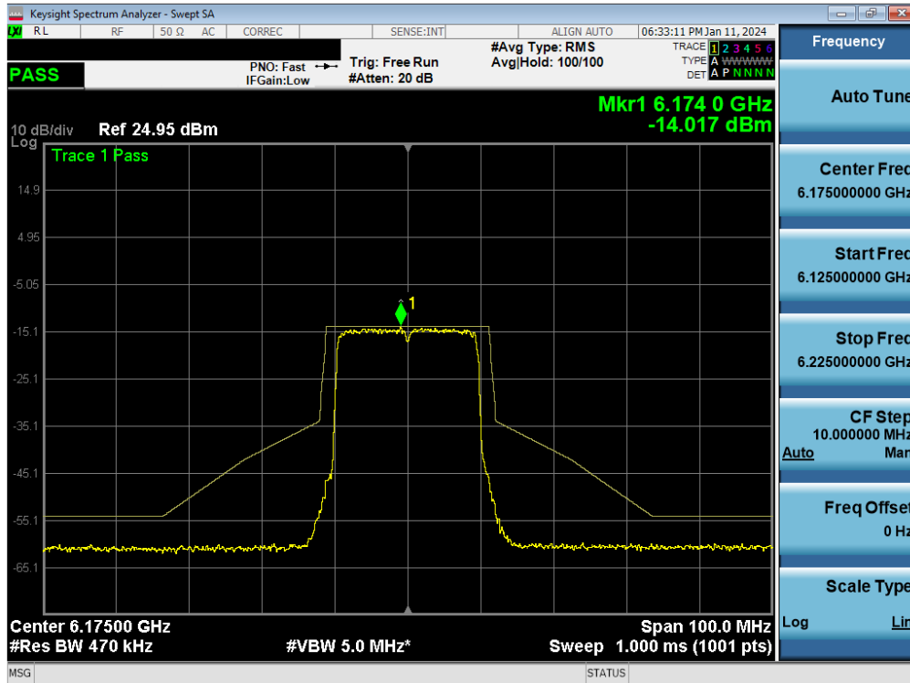
Plot 7-253. In-Band Emission Plot MIMO ANT1 (20MHz BW 802.11be (Full Tone) (UNII Band 5) – Ch. 45) - LPI
