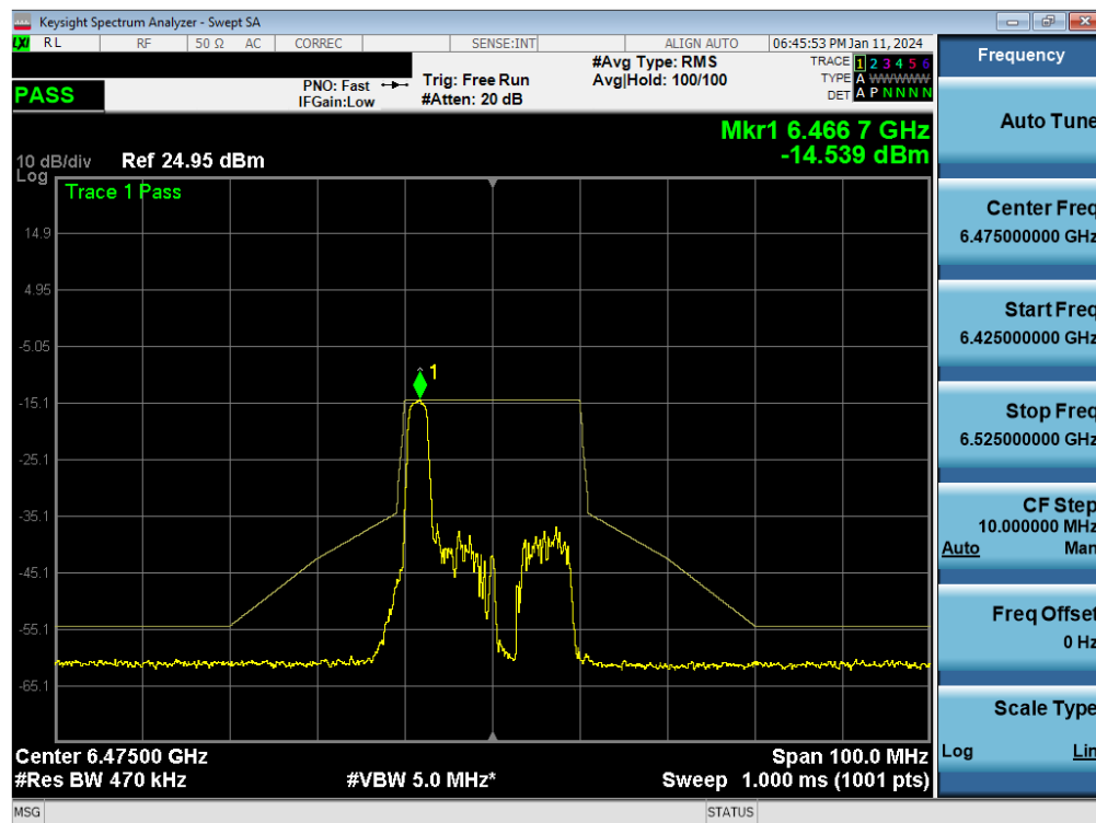
Plot 7-238. In-Band Emission Plot MIMO ANT1 (20MHz BW 802.11be (26 Tones) (UNII Band 6) – Ch. 105) - LPI
