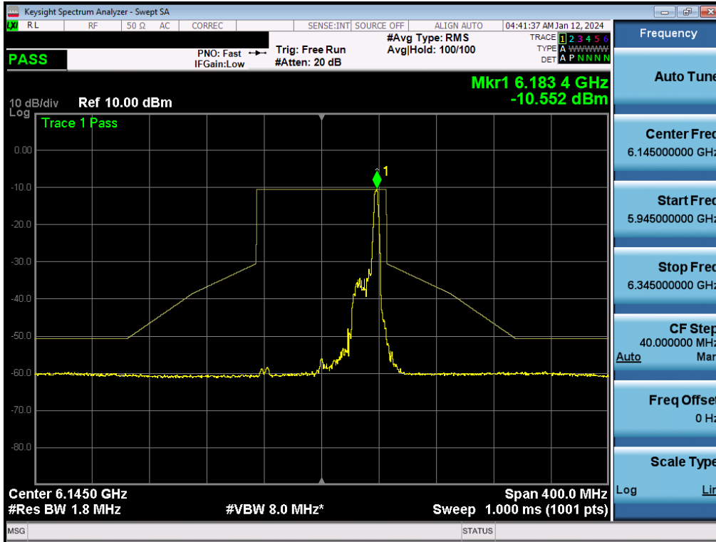
Plot 7-310. In-Band Emission Plot MIMO ANT2 (80MHz BW 802.11be (26 Tones) (UNII Band 5) – Ch. 39) - LPI
