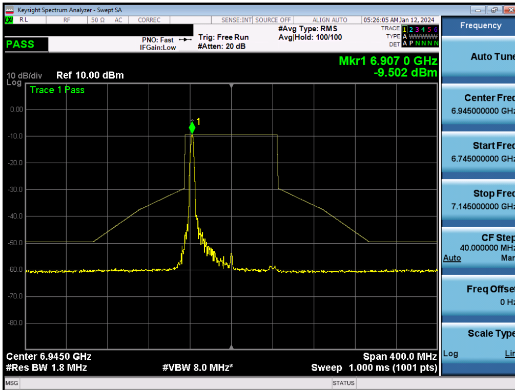
Plot 7-325. In-Band Emission Plot MIMO ANT2 (80MHz BW 802.11be (26 Tones) (UNII Band 8) – Ch. 199) - LPI
