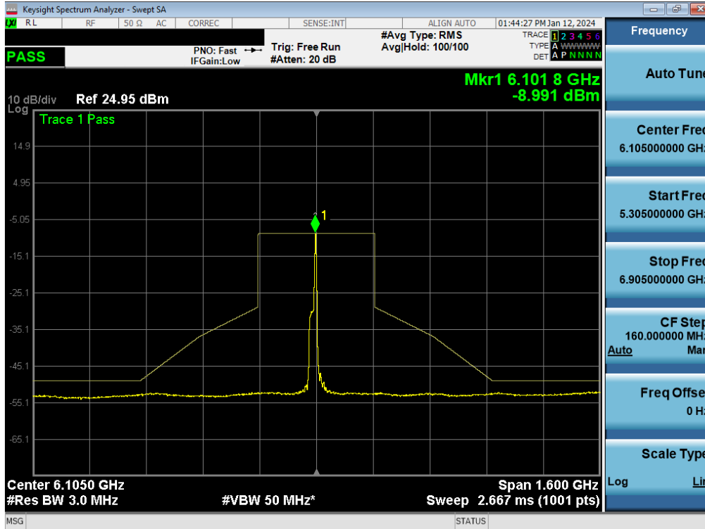
Plot 7-237. In-Band Emission Plot MIMO ANT1 (320MHz BW 802.11be (26 Tones) (UNII Band 5) – Ch. 31) - LPI
