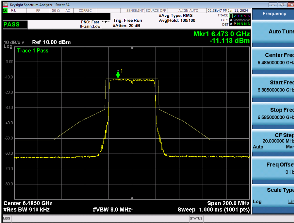
Plot 7-334. In-Band Emission Plot MIMO ANT2 (40MHz BW 802.11be (Full Tone) (UNII Band 6) – Ch. 107) - LPI
