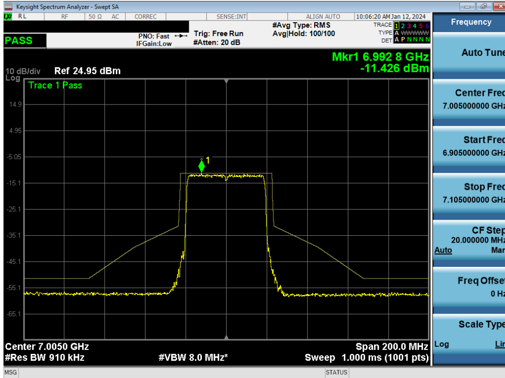
Plot 7-269. In-Band Emission Plot MIMO ANT1 (40MHz BW 802.11be (Full Tone) (UNII Band 8) – Ch. 211) - LPI
