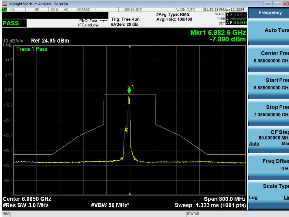
Plot 7-251. In-Band Emission Plot MIMO ANT1 (160MHz BW 802.11be (26 Tones) (UNII Band 8) – Ch. 207) - LPI
