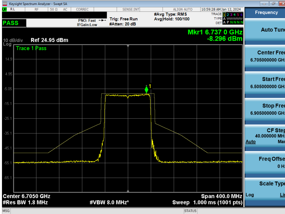
Plot 7-265. In-Band Emission Plot MIMO ANT1 (80MHz BW 802.11be (Full Tone) (UNII Band 7) – Ch. 151) - LPI
