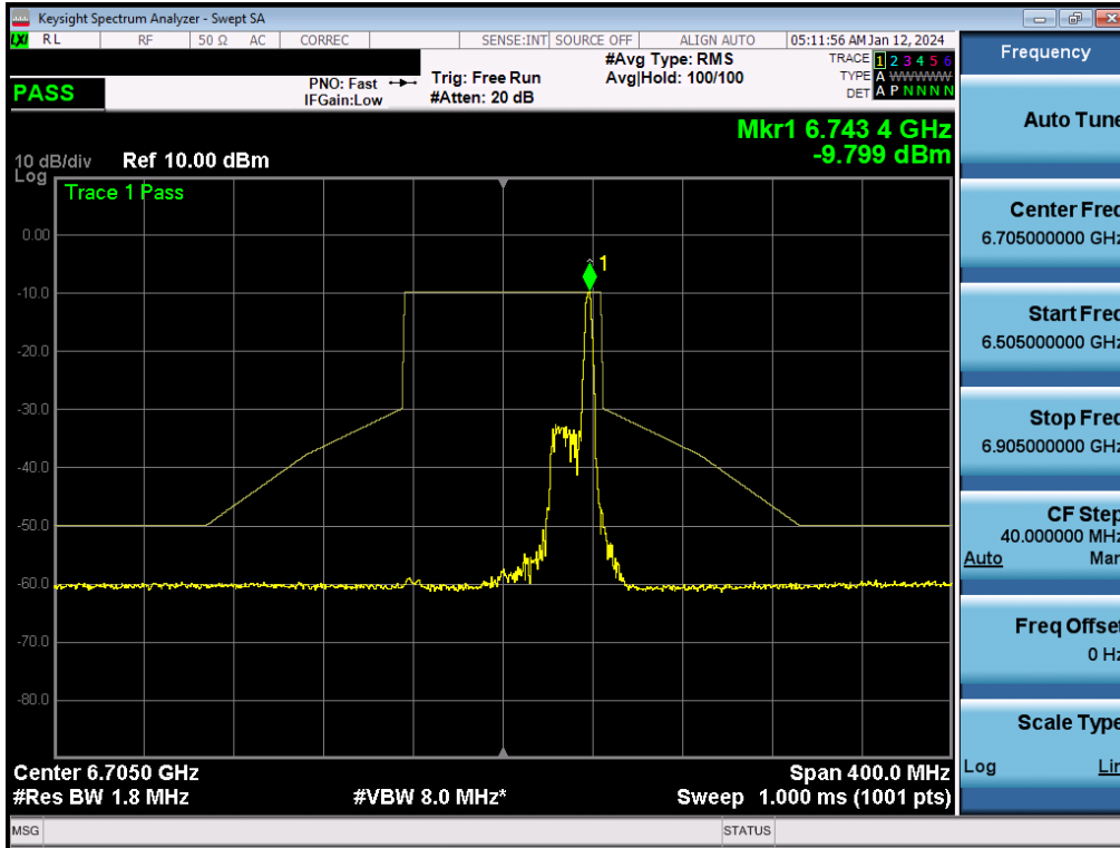
Plot 7-320. In-Band Emission Plot MIMO ANT2 (80MHz BW 802.11be (26 Tones) (UNII Band 7) – Ch. 151) - LPI
