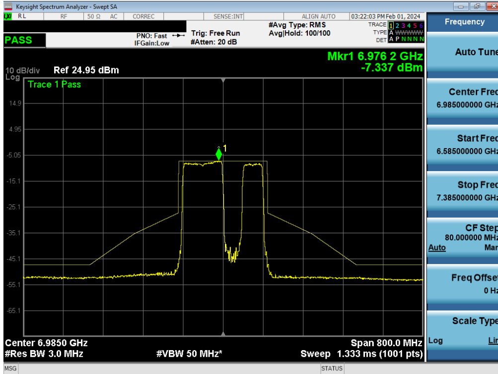
Plot 7-283. In-Band Emission Plot MIMO ANT1 (160MHz BW 802.11be (996+484 Tone) (UNII Band 8) – Ch. 207) - LPI
