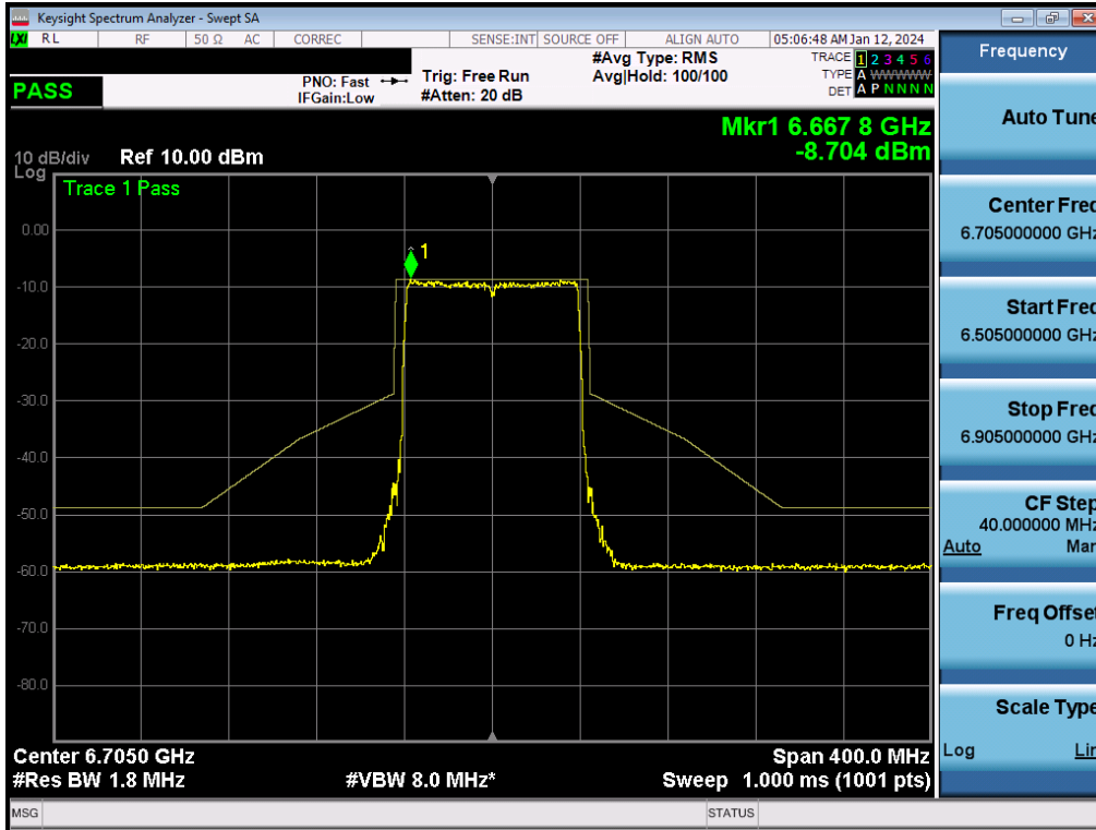
Plot 7-340. In-Band Emission Plot MIMO ANT2 (80MHz BW 802.11be (Full Tone) (UNII Band 7) – Ch. 151) - LPI
