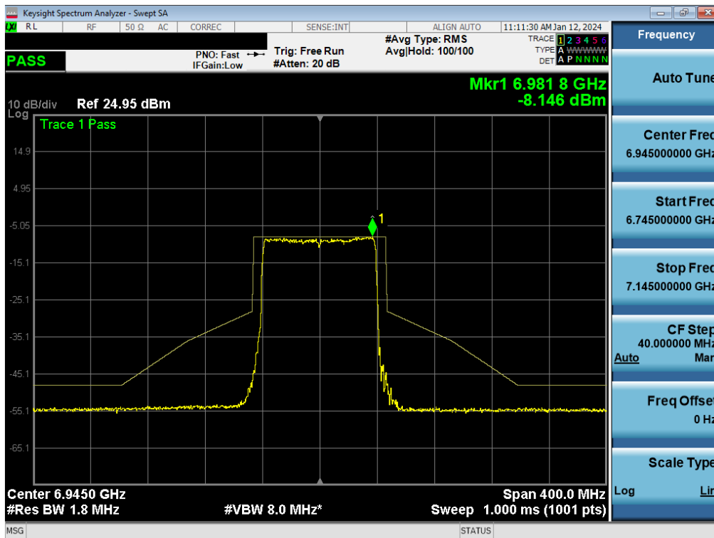
Plot 7-270. In-Band Emission Plot MIMO ANT1 (80MHz BW 802.11be (Full Tone) (UNII Band 8) – Ch. 199) - LPI
