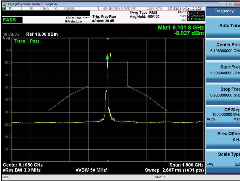
Plot 7-312. In-Band Emission Plot MIMO ANT2 (320MHz BW 802.11be (26 Tones) (UNII Band 5) – Ch. 31) - LPI
