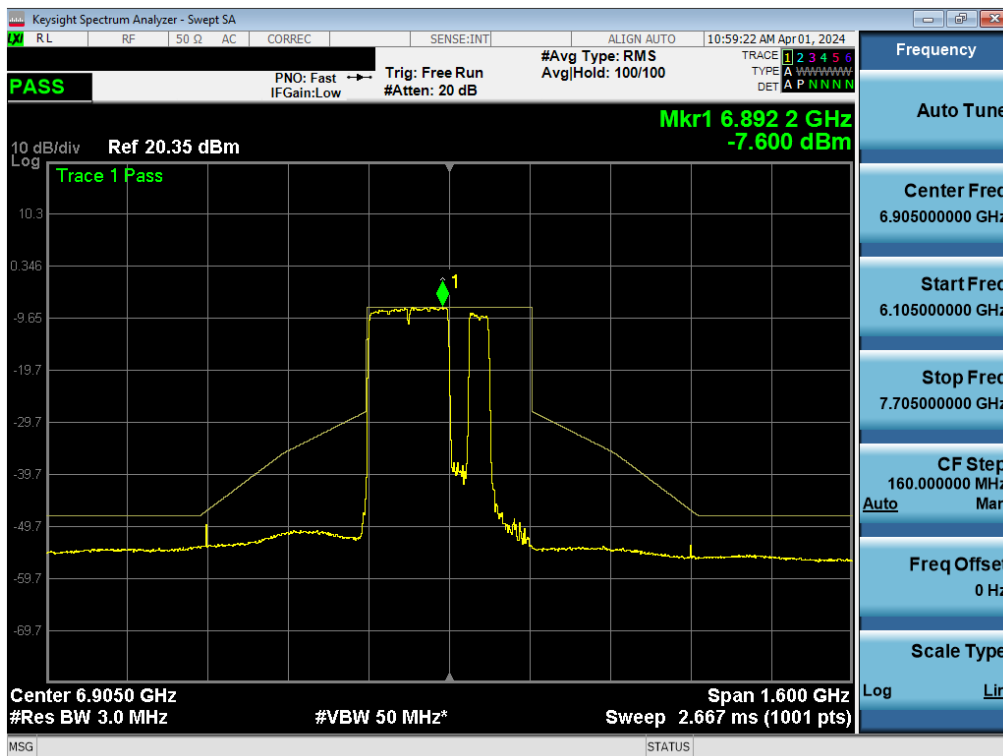
Plot 7-284. In-Band Emission Plot MIMO ANT1 (320MHz BW 802.11be (2*996+484 Tone) (UNII Band 8) – Ch. 191) - LPI
