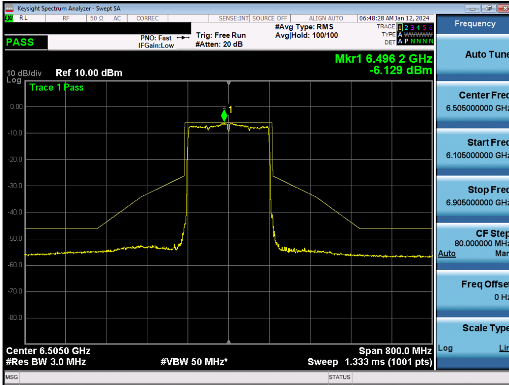
Plot 7-336. In-Band Emission Plot MIMO ANT2 (160MHz BW 802.11be (Full Tone) (UNII Band 6) – Ch. 111) - LPI
