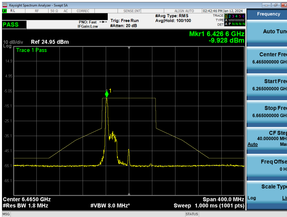
Plot 7-240. In-Band Emission Plot MIMO ANT1 (80MHz BW 802.11be (26 Tones) (UNII Band 6) – Ch. 103) - LPI
