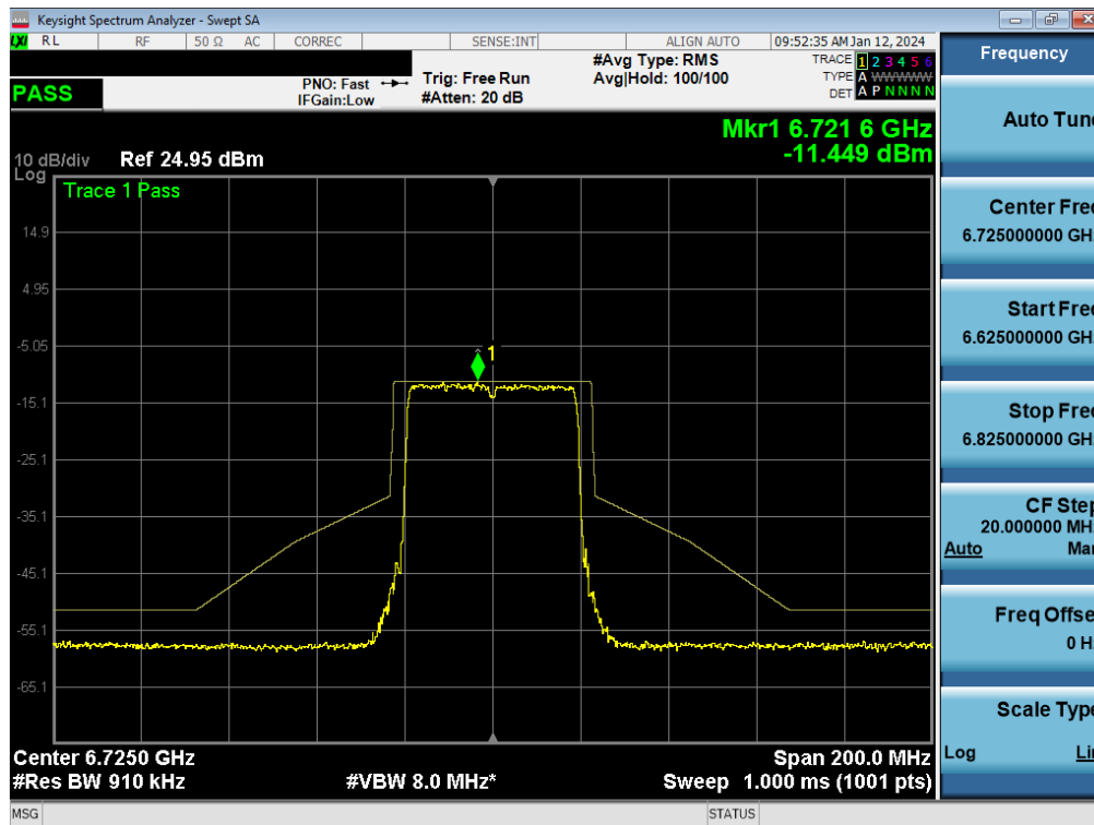
Plot 7-264. In-Band Emission Plot MIMO ANT1 (40MHz BW 802.11be (Full Tone) (UNII Band 7) – Ch. 155) - LPI
