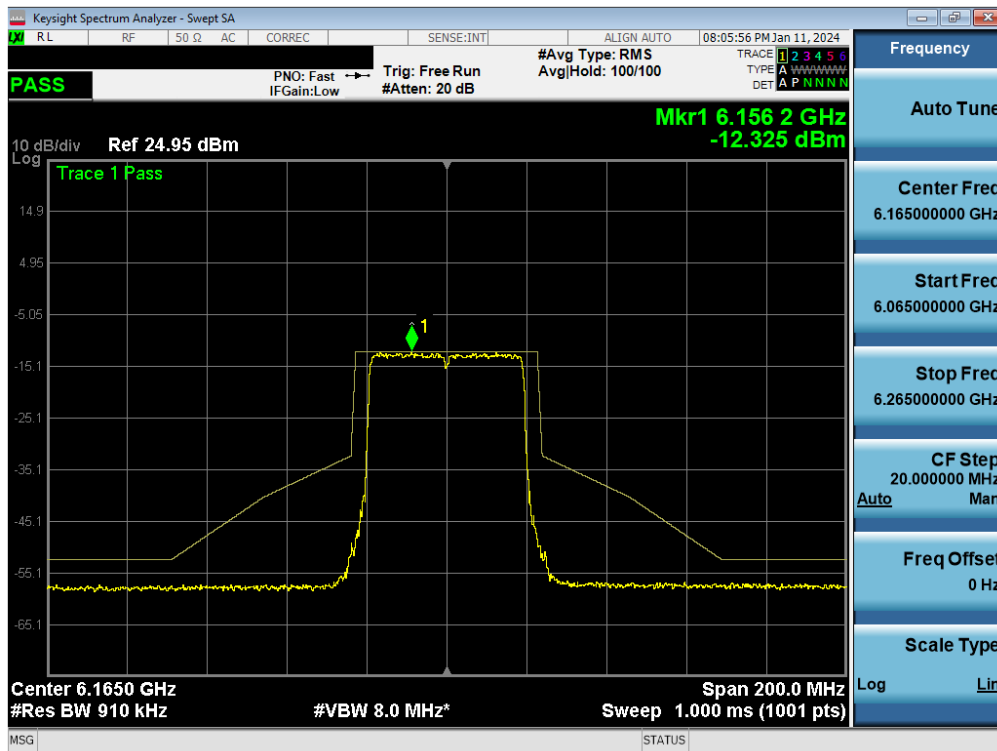
Plot 7-254. In-Band Emission Plot MIMO ANT1 (40MHz BW 802.11be (Full Tone) (UNII Band 5) – Ch. 43) - LPI
