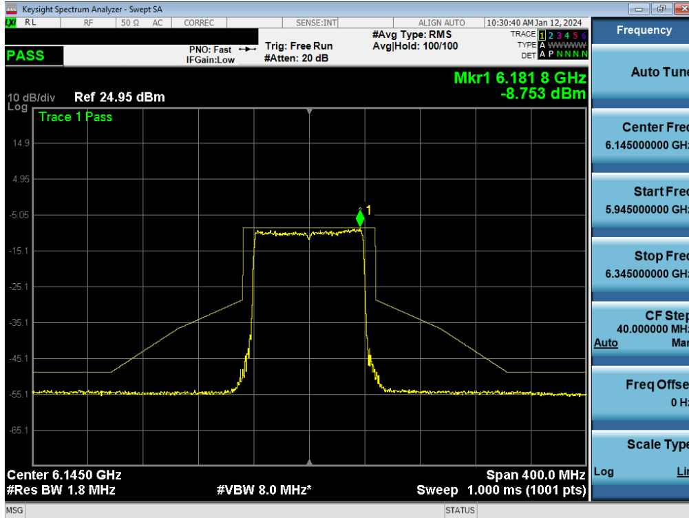
Plot 7-255. In-Band Emission Plot MIMO ANT1 (80MHz BW 802.11be (Full Tone) (UNII Band 5) – Ch. 39) - LPI
