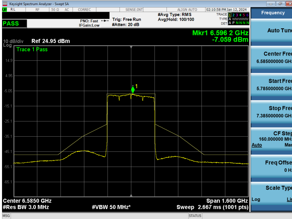
Plot 7-267. In-Band Emission Plot MIMO ANT1 (320MHz BW 802.11be (Full Tone) (UNII Band 7) – Ch. 127) - LPI
