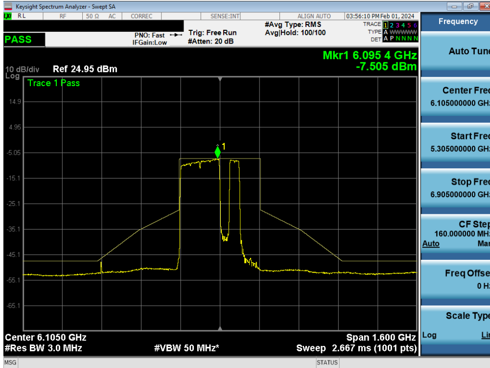
Plot 7-275. In-Band Emission Plot MIMO ANT1 (320MHz BW 802.11be (3*996 Tone) (UNII Band 5) – Ch. 31) - LPI
