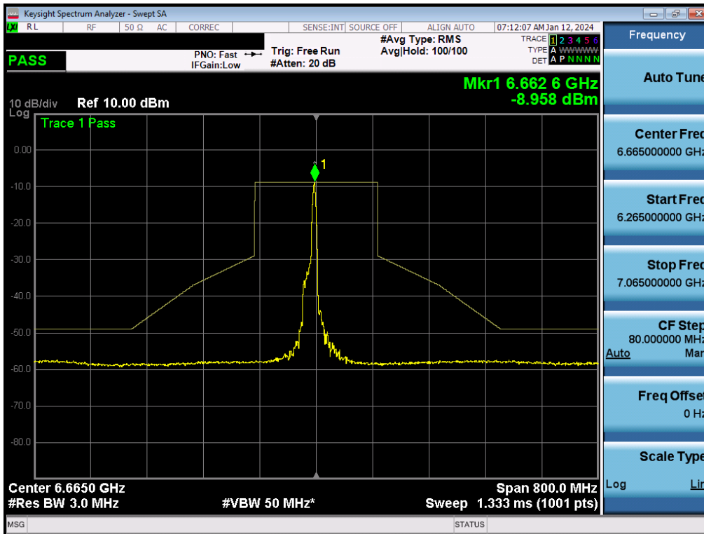
Plot 7-321. In-Band Emission Plot MIMO ANT2 (160MHz BW 802.11be (26 Tones) (UNII Band 7) – Ch. 143) - LPI
