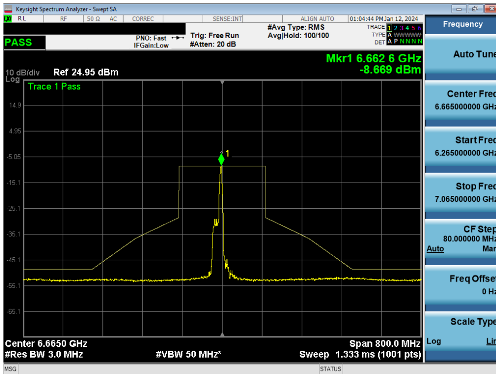
Plot 7-246. In-Band Emission Plot MIMO ANT1 (160MHz BW 802.11be (26 Tones) (UNII Band 7) – Ch. 143) - LPI
