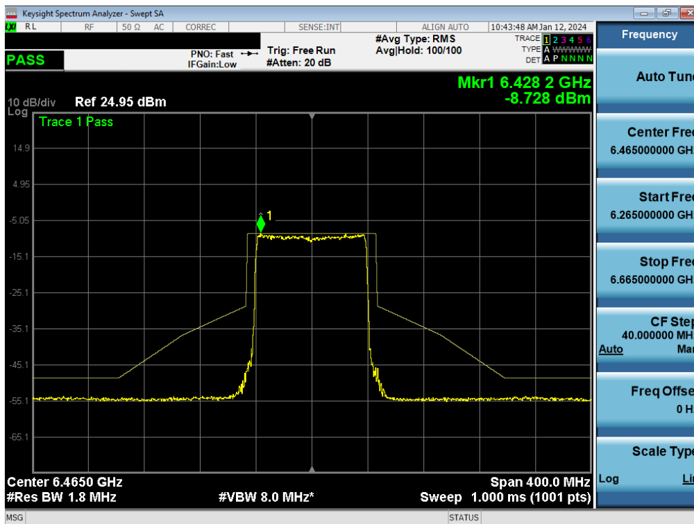
Plot 7-260. In-Band Emission Plot MIMO ANT1 (80MHz BW 802.11be (Full Tone) (UNII Band 6) – Ch. 103) - LPI
