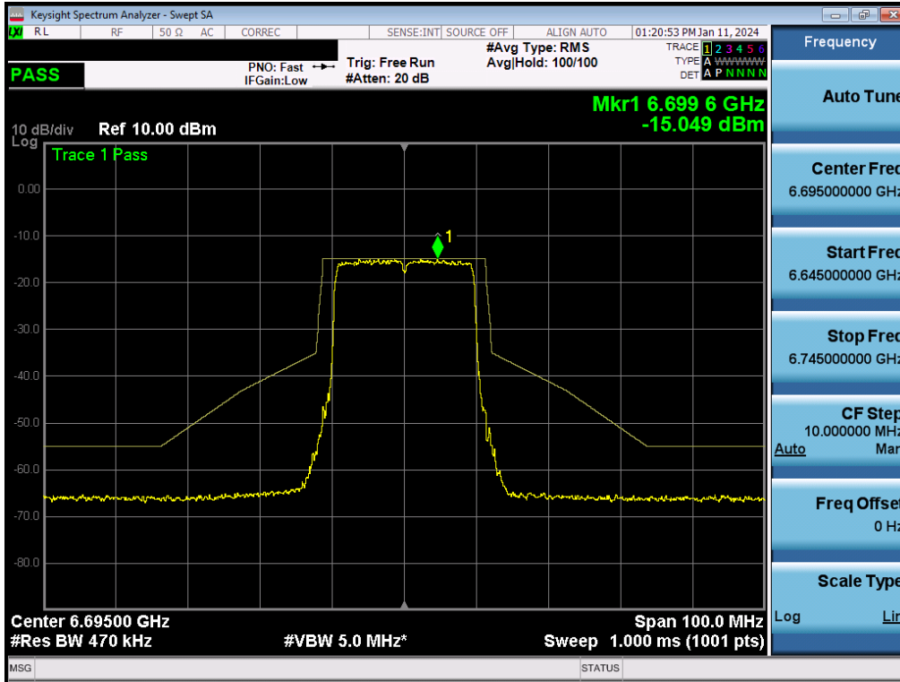
Plot 7-338. In-Band Emission Plot MIMO ANT2 (20MHz BW 802.11be (Full Tone) (UNII Band 7) – Ch. 149) - LPI
