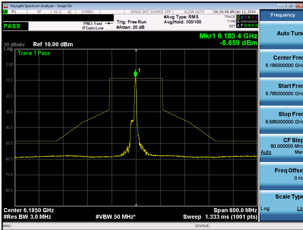
Plot 7-311. In-Band Emission Plot MIMO ANT2 (160MHz BW 802.11be (26 Tones) (UNII Band 5) – Ch. 47) - LPI
