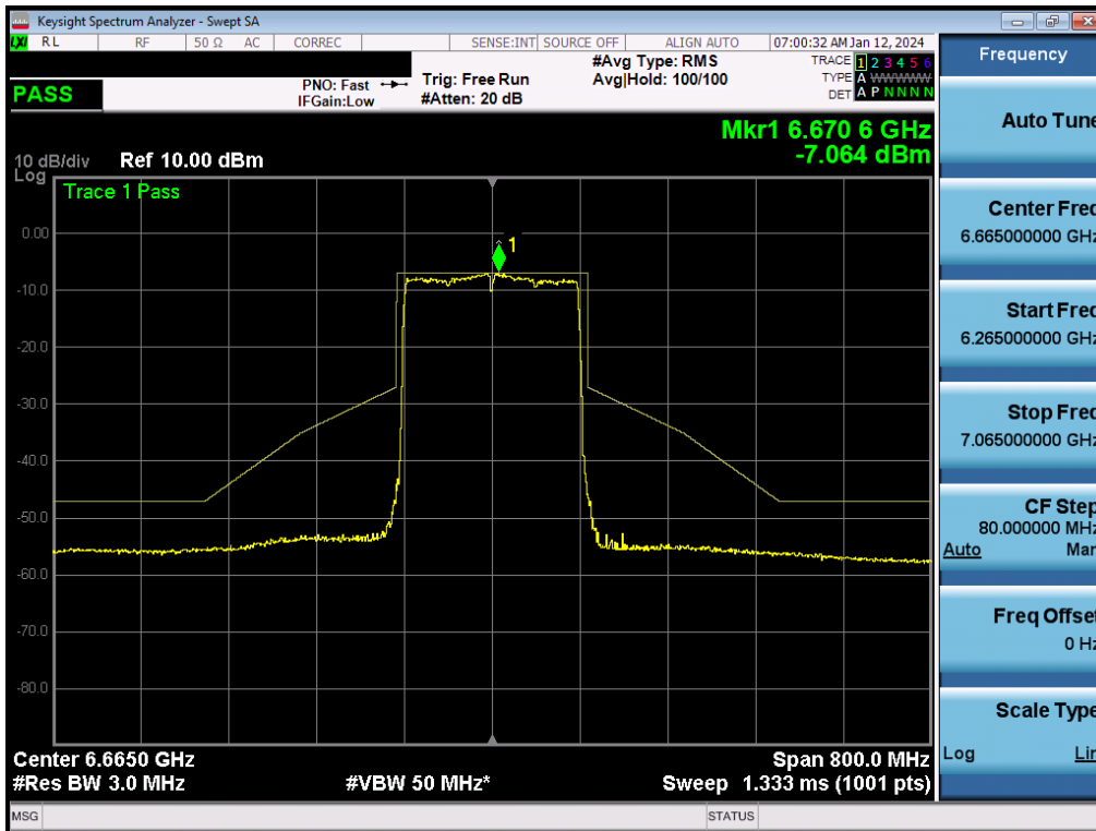
Plot 7-341. In-Band Emission Plot MIMO ANT2 (160MHz BW 802.11be (Full Tone) (UNII Band 7) – Ch. 143) - LPI
