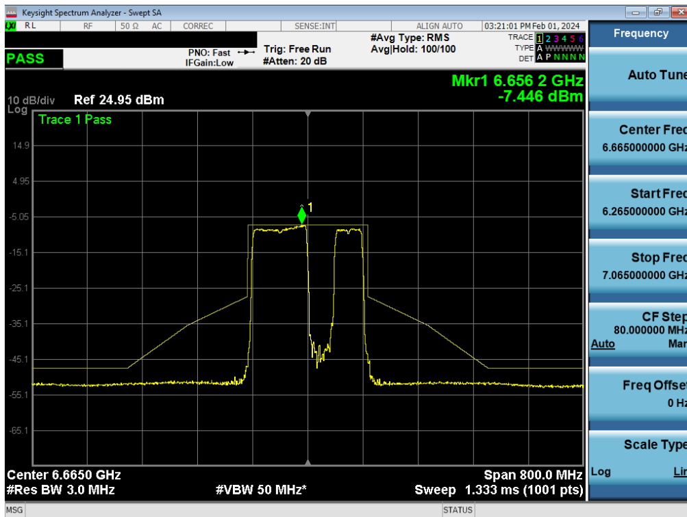
Plot 7-280. In-Band Emission Plot MIMO ANT1 (160MHz BW 802.11be (996+484 Tone) (UNII Band 7) – Ch. 143) - LPI
