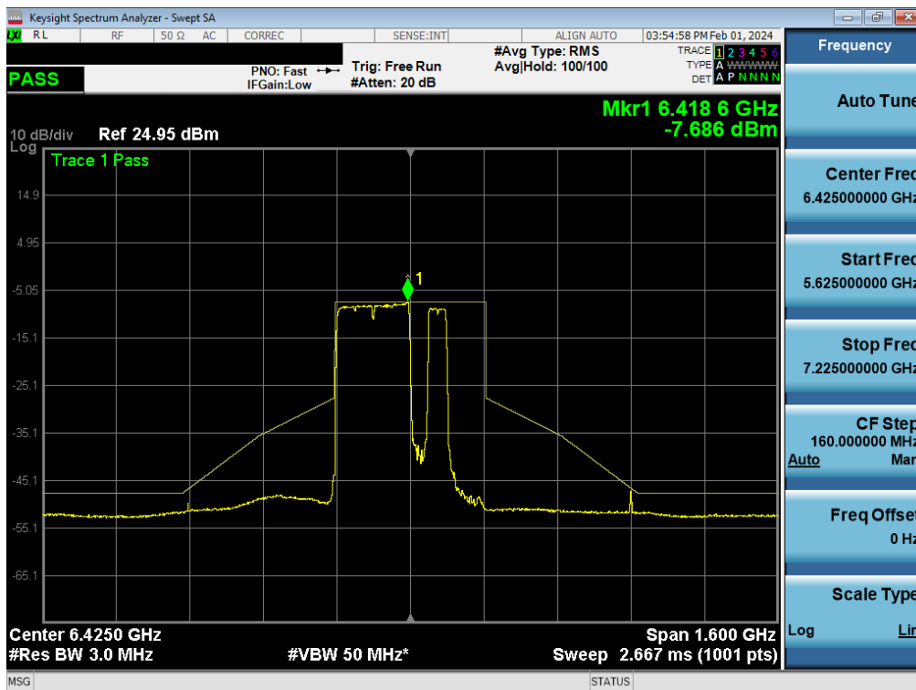
Plot 7-278. In-Band Emission Plot MIMO ANT1 (320MHz BW 802.11be (2*996+484 Tone) (UNII Band 6) – Ch. 95) - LPI
