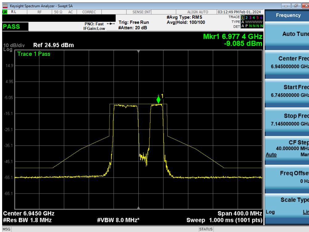
Plot 7-282. In-Band Emission Plot MIMO ANT1 (80MHz BW 802.11be (484+242 Tone) (UNII Band 8) – Ch. 199) - LPI
