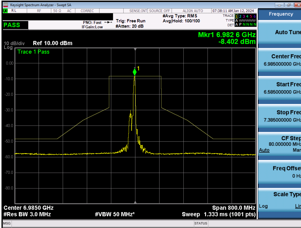
Plot 7-326. In-Band Emission Plot MIMO ANT2 (160MHz BW 802.11be (26 Tones) (UNII Band 8) – Ch. 207) - LPI
