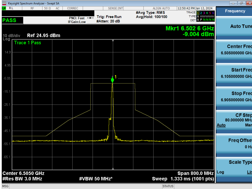
Plot 7-241. In-Band Emission Plot MIMO ANT1 (160MHz BW 802.11be (26 Tones) (UNII Band 6) – Ch. 111) - LPI
