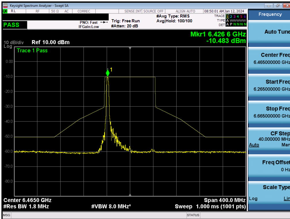
Plot 7-315. In-Band Emission Plot MIMO ANT2 (80MHz BW 802.11be (26 Tones) (UNII Band 6) – Ch. 103) - LPI
