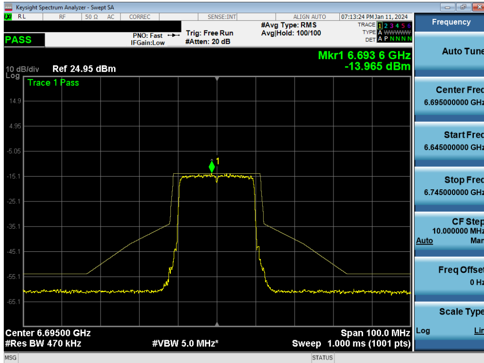
Plot 7-263. In-Band Emission Plot MIMO ANT1 (20MHz BW 802.11be (Full Tone) (UNII Band 7) – Ch. 149) - LPI
