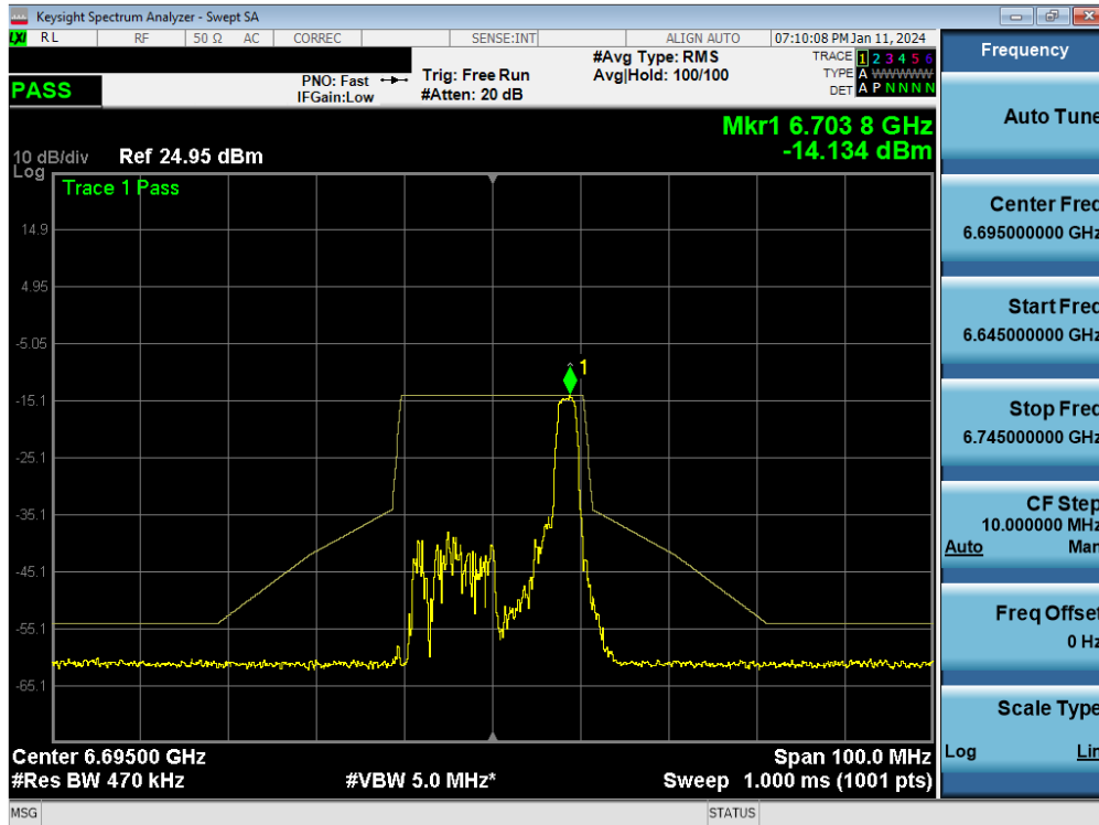
Plot 7-243. In-Band Emission Plot MIMO ANT1 (20MHz BW 802.11be (26 Tones) (UNII Band 7) – Ch. 149) - LPI
