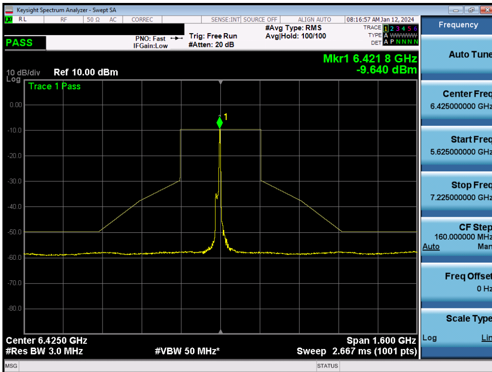
Plot 7-317. In-Band Emission Plot MIMO ANT2 (320MHz BW 802.11be (26 Tones) (UNII Band 6) – Ch. 95) - LPI
