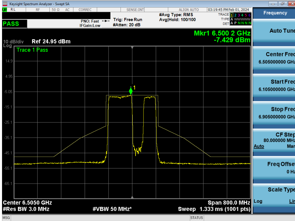
Plot 7-277. In-Band Emission Plot MIMO ANT1 (160MHz BW 802.11be (996+484 Tone) (UNII Band 6) – Ch. 111) - LPI
