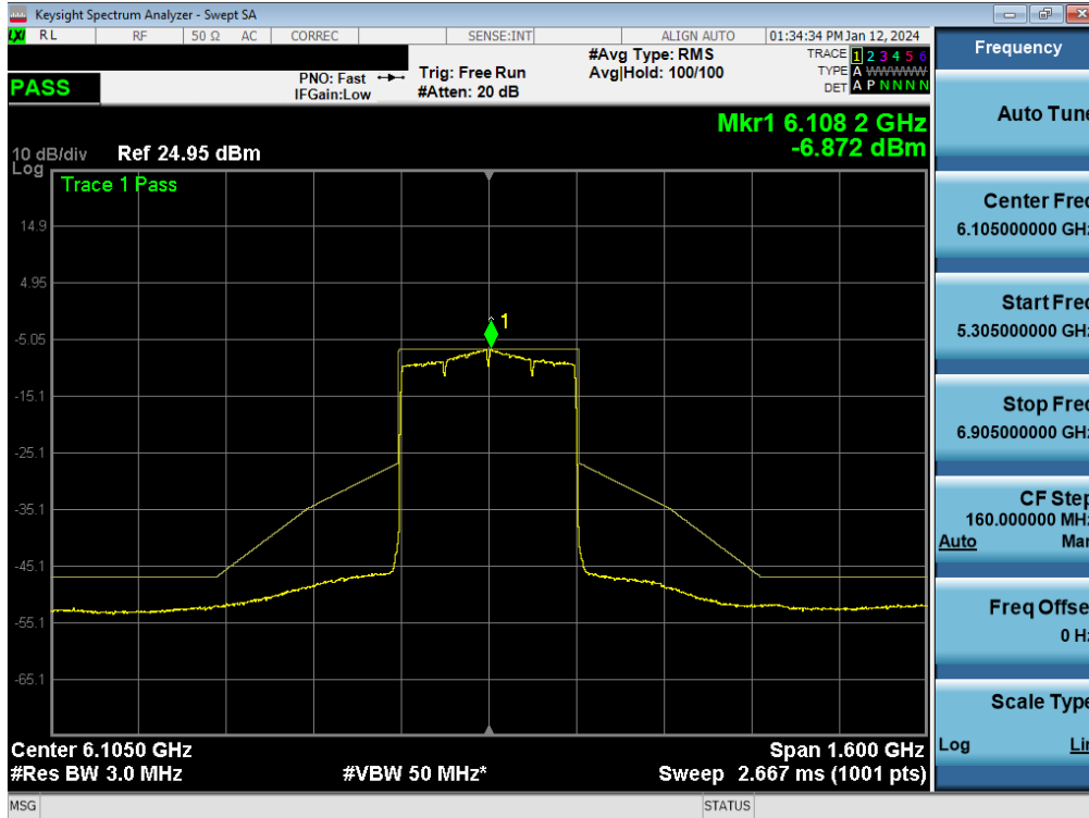
Plot 7-257. In-Band Emission Plot MIMO ANT1 (320MHz BW 802.11be (Full Tone) (UNII Band 5) – Ch. 31) - LPI
