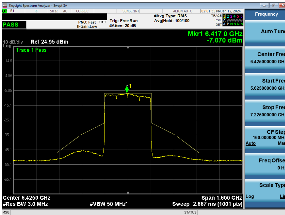
Plot 7-262. In-Band Emission Plot MIMO ANT1 (320MHz BW 802.11be (Full Tone) (UNII Band 6) – Ch. 95) - LPI
