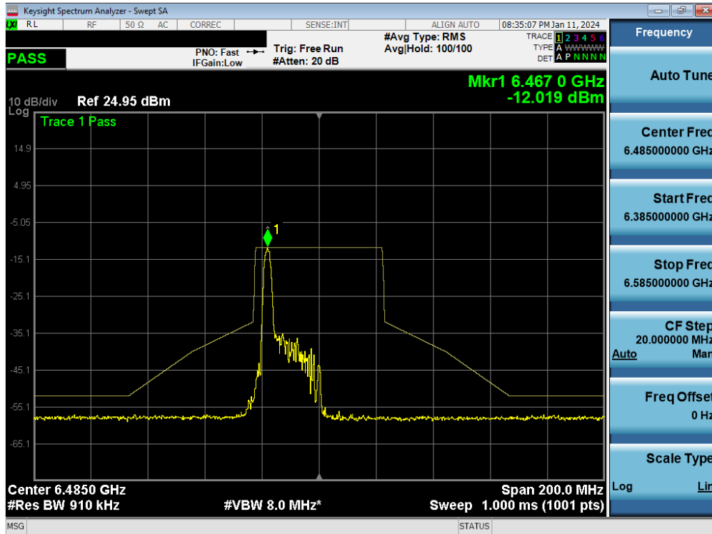
Plot 7-239. In-Band Emission Plot MIMO ANT1 (40MHz BW 802.11be (26 Tones) (UNII Band 6) – Ch. 107) - LPI
