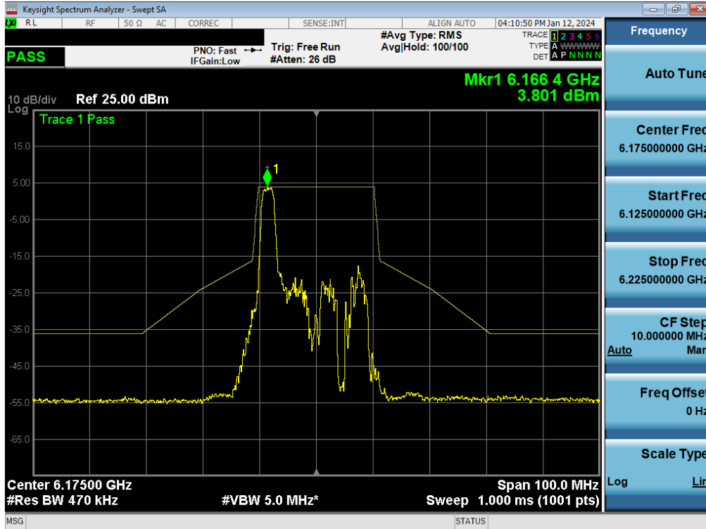
Plot 7-285. In-Band Emission Plot MIMO ANT1 (20MHz BW 802.11be (26 Tones) (UNII Band 5) – Ch. 45) - SP
