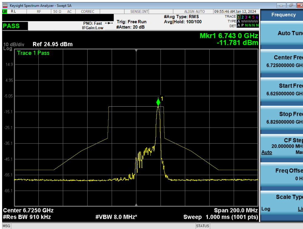
Plot 7-244. In-Band Emission Plot MIMO ANT1 (40MHz BW 802.11be (26 Tones) (UNII Band 7) – Ch. 155) - LPI
