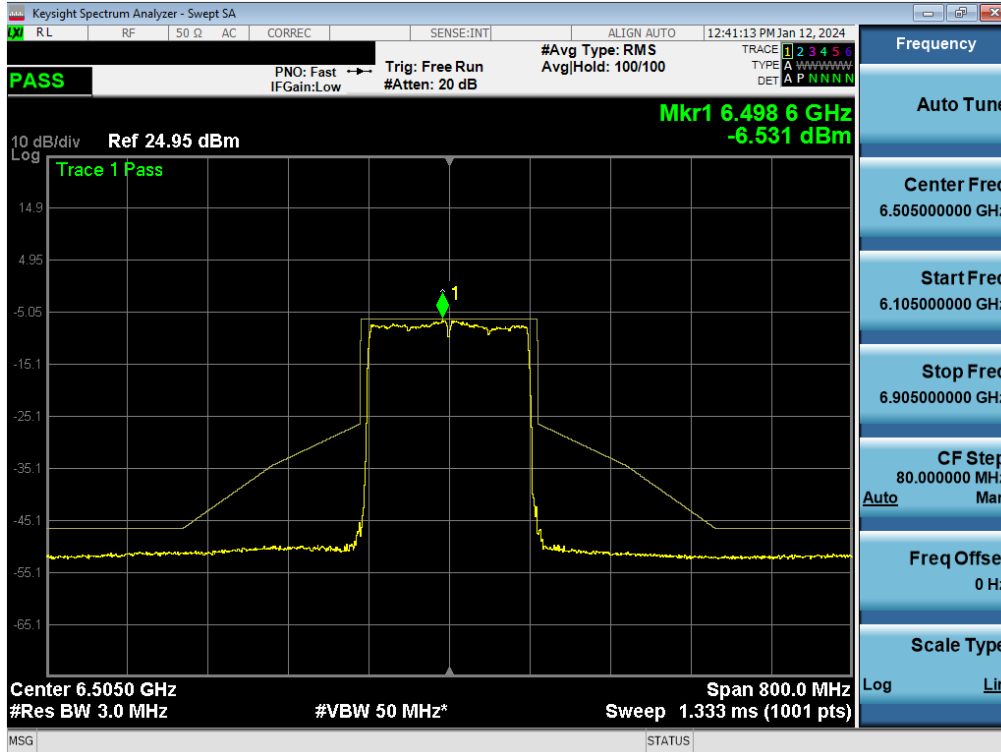
Plot 7-261. In-Band Emission Plot MIMO ANT1 (160MHz BW 802.11be (Full Tone) (UNII Band 6) – Ch. 111) - LPI
