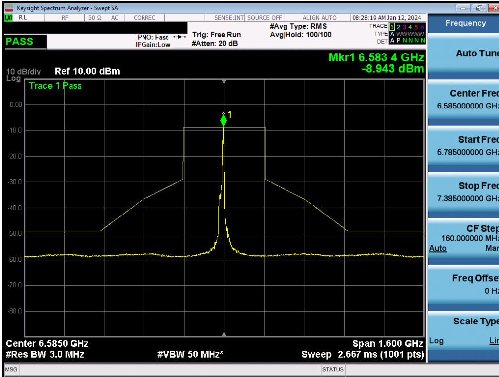
Plot 7-322. In-Band Emission Plot MIMO ANT2 (320MHz BW 802.11be (26 Tones) (UNII Band 7) – Ch. 127) - LPI
