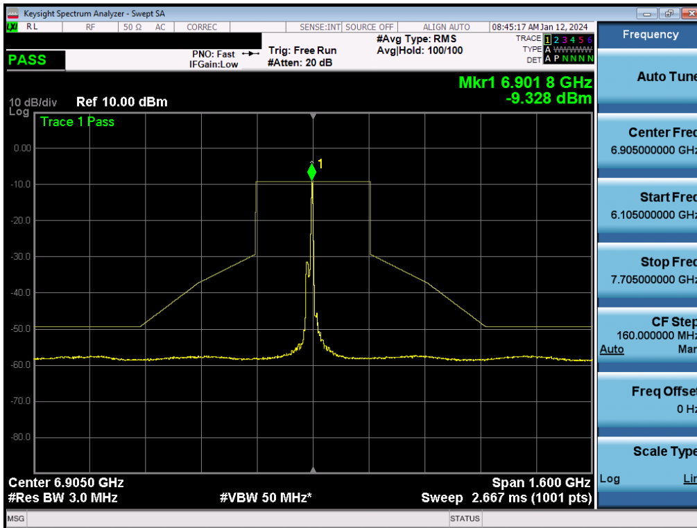
Plot 7-327. In-Band Emission Plot MIMO ANT2 (320MHz BW 802.11be (26 Tones) (UNII Band 8) – Ch. 191) - LPI
