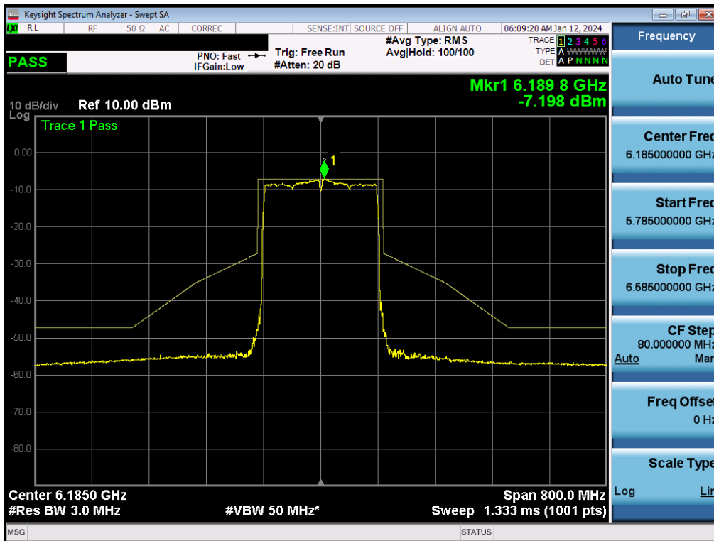
Plot 7-331. In-Band Emission Plot MIMO ANT2 (160MHz BW 802.11be (Full Tone) (UNII Band 5) – Ch. 47) - LPI
