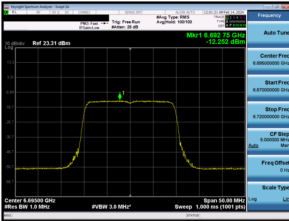
Plot 7-188. Power Spectral Density Plot MIMO ANT2 (20MHz BW 802.11be (Full Tone) (UNII Band 7) – Ch. 149) – LPI
