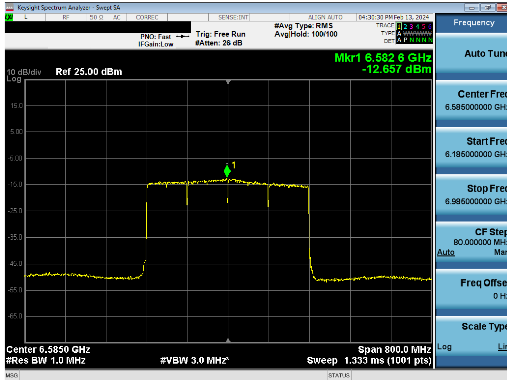
Plot 7-117. Power Spectral Density Plot MIMO ANT1 (320MHz BW 802.11be (Full Tone) (UNII Band 7) – Ch. 127) - LPI
