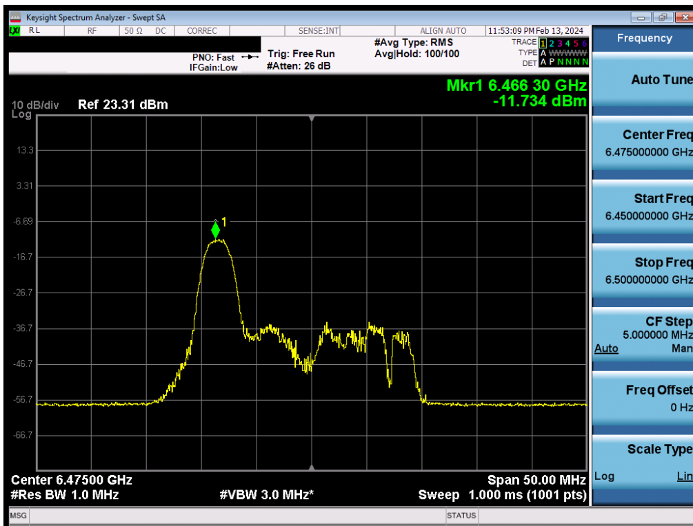
Plot 7-163. Power Spectral Density Plot MIMO ANT2 (20MHz BW 802.11be (26 Tones) (UNII Band 6) – Ch. 105) – LPI
