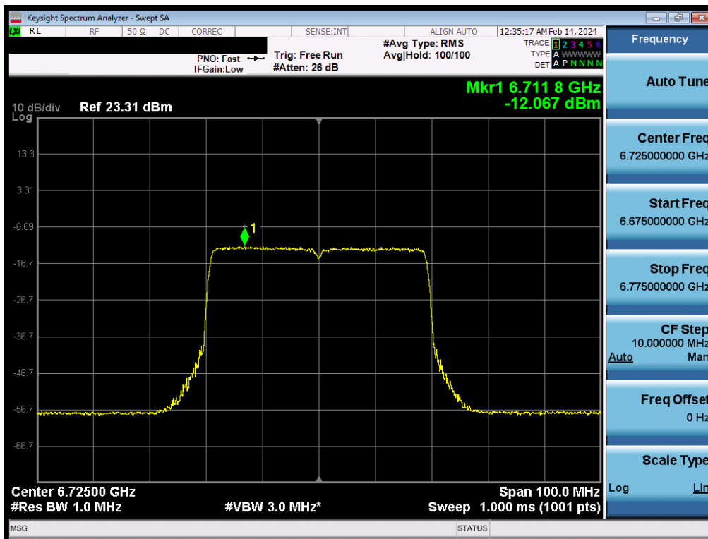
Plot 7-189. Power Spectral Density Plot MIMO ANT2 (40MHz BW 802.11be (Full Tone) (UNII Band 7) – Ch. 155) – LPI
