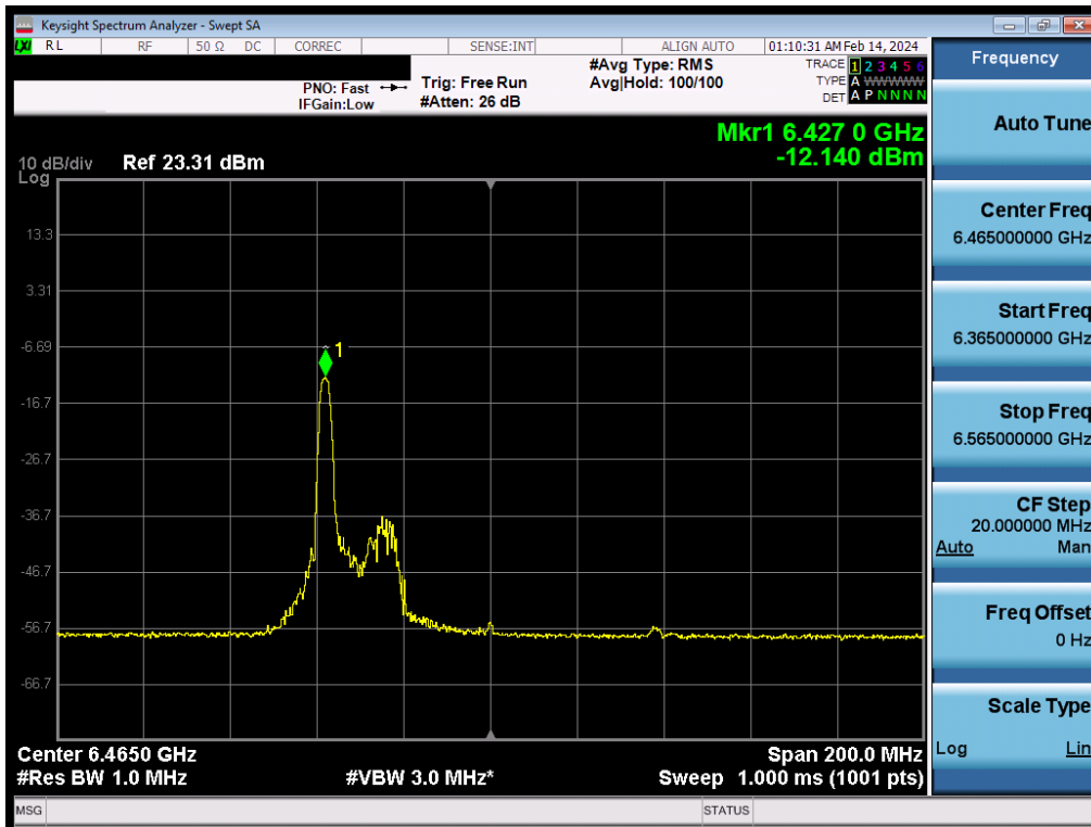
Plot 7-165. Power Spectral Density Plot MIMO ANT2 (80MHz BW 802.11be (26 Tones) (UNII Band 6) – Ch. 103) – LPI
