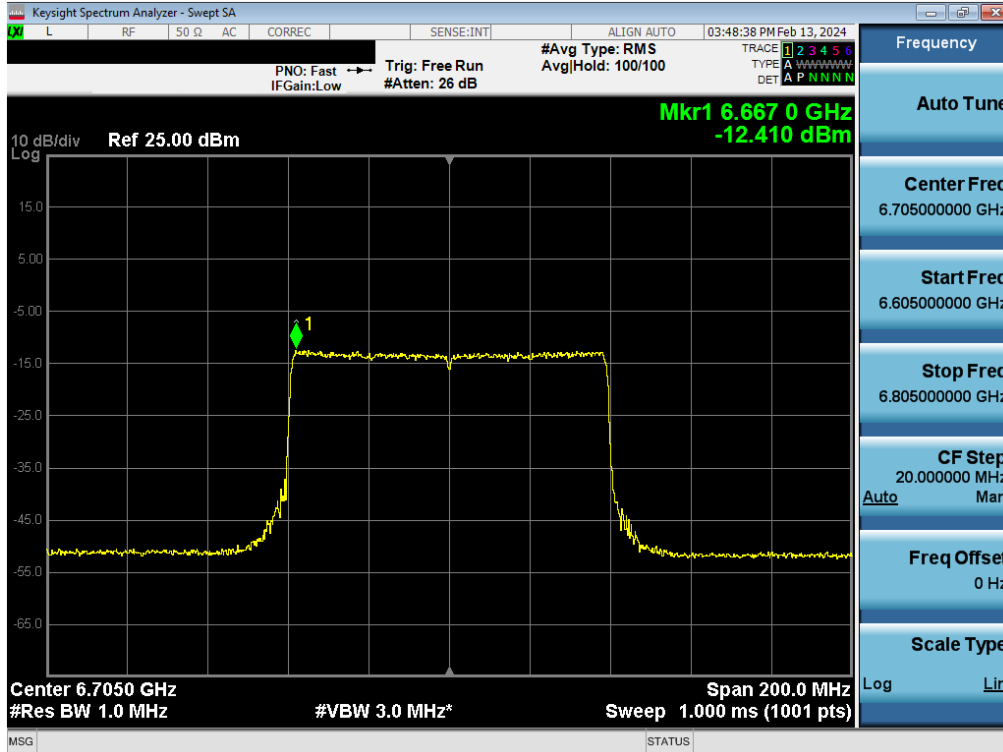
Plot 7-115. Power Spectral Density Plot MIMO ANT1 (80MHz BW 802.11be (Full Tone) (UNII Band 7) – Ch. 151) - LPI
