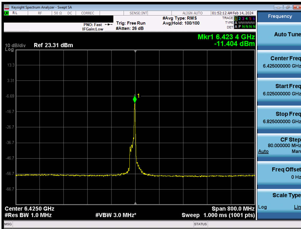
Plot 7-167. Power Spectral Density Plot MIMO ANT2 (320MHz BW 802.11be (26 Tones) (UNII Band 6) – Ch. 95) – LPI
