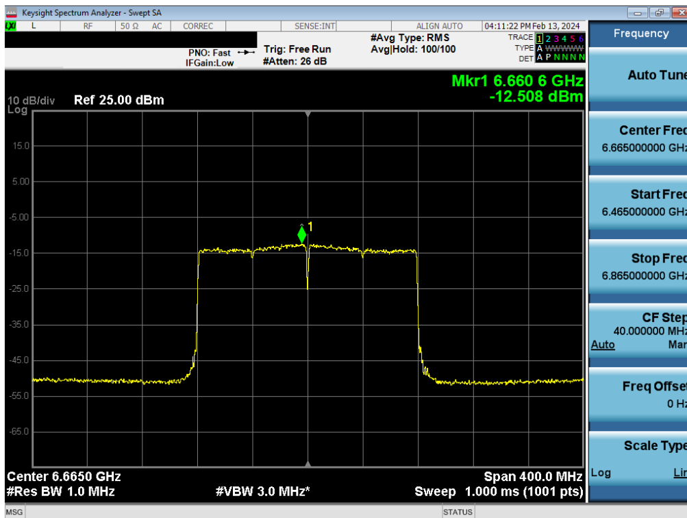
Plot 7-116. Power Spectral Density Plot MIMO ANT1 (160MHz BW 802.11be (Full Tone) (UNII Band 7) – Ch. 143) - LPI
