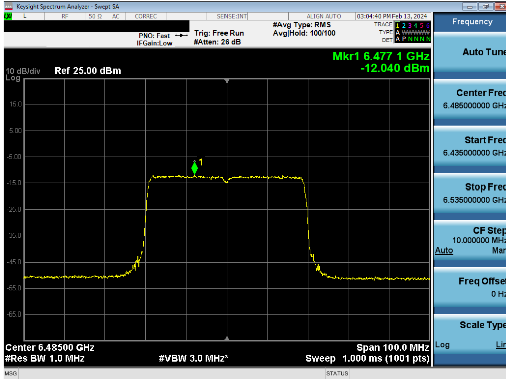
Plot 7-109. Power Spectral Density Plot MIMO ANT1 (40MHz BW 802.11be (Full Tone) (UNII Band 6) – Ch. 107) - LPI
