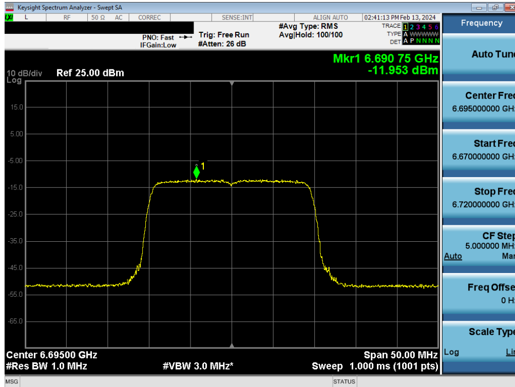
Plot 7-113. Power Spectral Density Plot MIMO ANT1 (20MHz BW 802.11be (Full Tone) (UNII Band 7) – Ch. 149) - LPI
