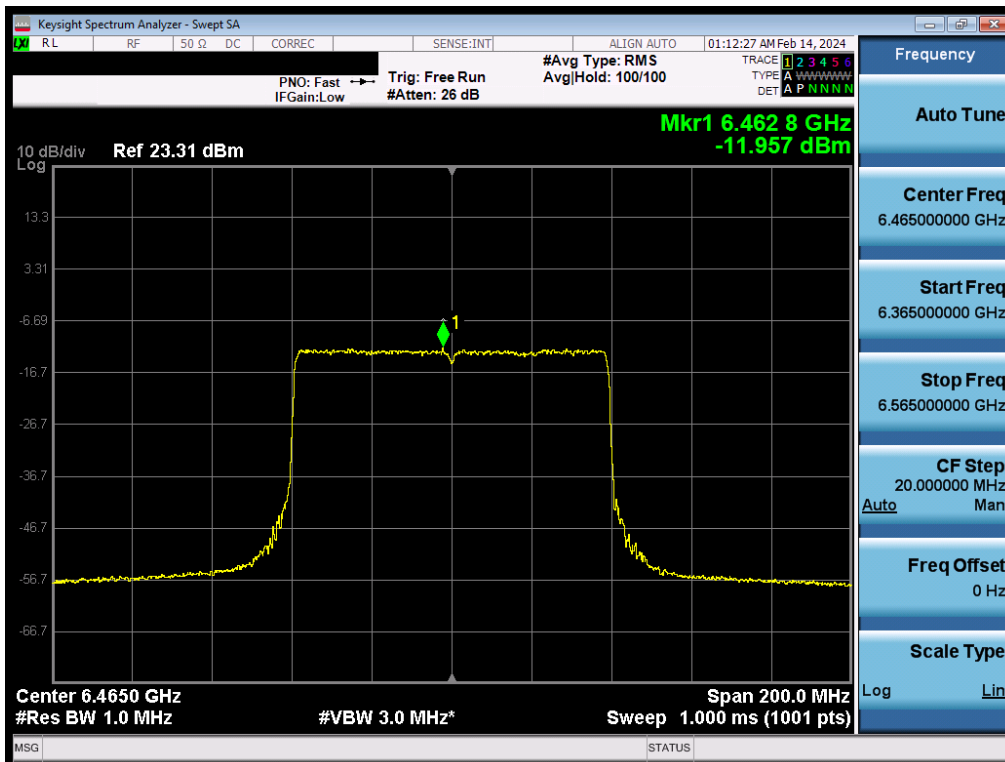
Plot 7-185. Power Spectral Density Plot MIMO ANT2 (80MHz BW 802.11be (Full Tone) (UNII Band 6) – Ch. 103) – LPI
