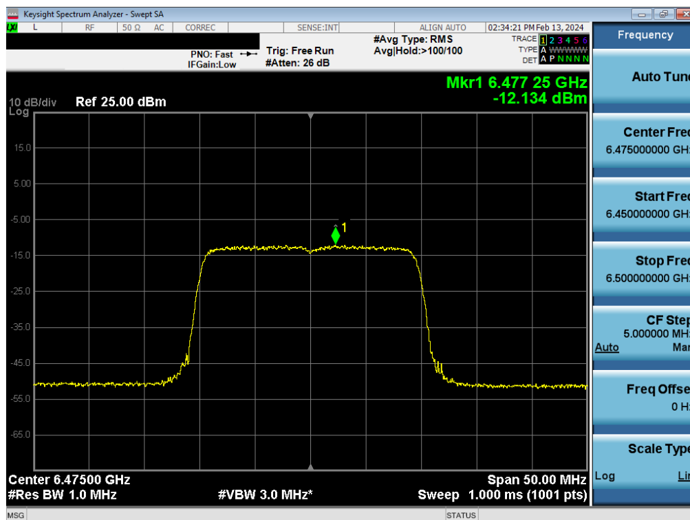
Plot 7-108. Power Spectral Density Plot MIMO ANT1 (20MHz BW 802.11be (Full Tone) (UNII Band 6) – Ch. 105) - LPI
