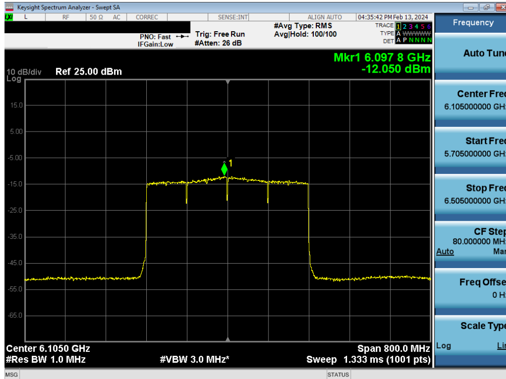
Plot 7-107. Power Spectral Density Plot MIMO ANT1 (320MHz BW 802.11be (Full Tone) (UNII Band 5) – Ch. 31) - LPI
