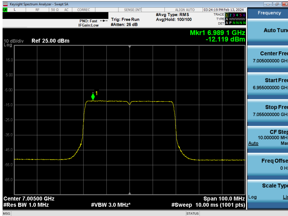
Plot 7-119. Power Spectral Density Plot MIMO ANT1 (40MHz BW 802.11be (Full Tone) (UNII Band 8) – Ch. 211) - LPI
