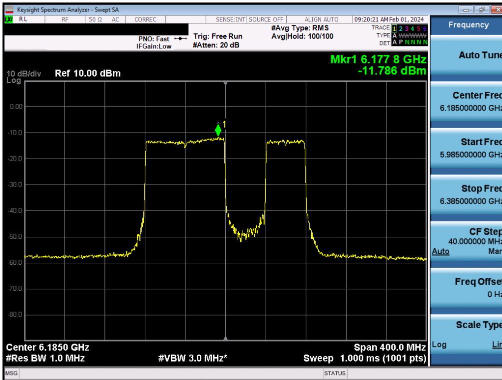
Plot 7-199. Power Spectral Density Plot MIMO ANT2 (160MHz BW 802.11be (996+484 Tone) (UNII Band 5) – Ch. 47) – LPI
