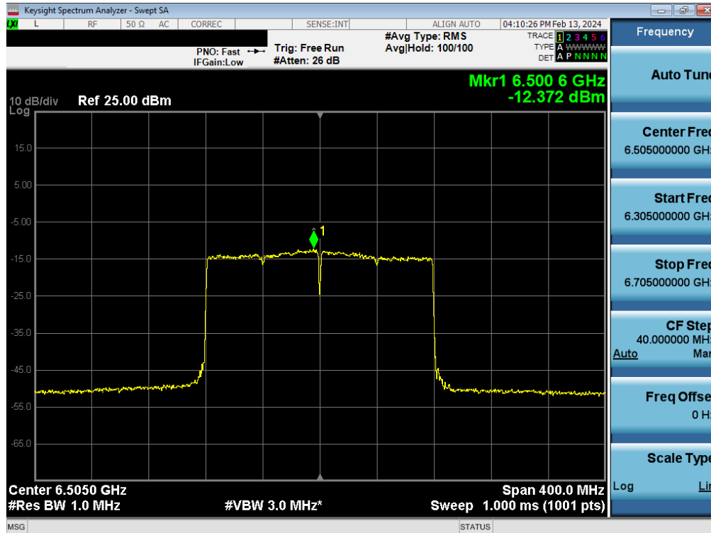
Plot 7-111. Power Spectral Density Plot MIMO ANT1 (160MHz BW 802.11be (Full Tone) (UNII Band 6) – Ch. 111) - LPI
