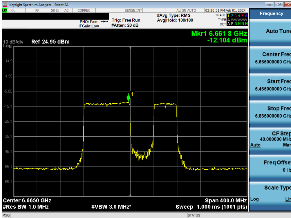
Plot 7-130. Power Spectral Density Plot MIMO ANT1 (160MHz BW 802.11be (996+484 Tone) (UNII Band 7) – Ch. 143) - LPI
