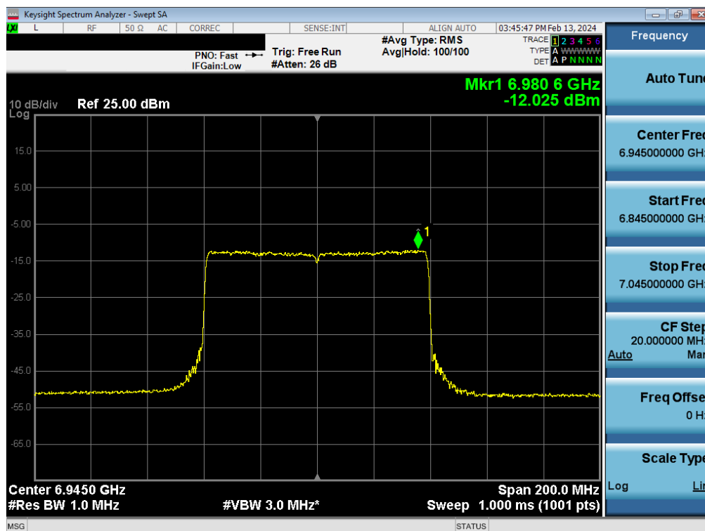
Plot 7-120. Power Spectral Density Plot MIMO ANT1 (80MHz BW 802.11be (Full Tone) (UNII Band 8) – Ch. 199) - LPI
