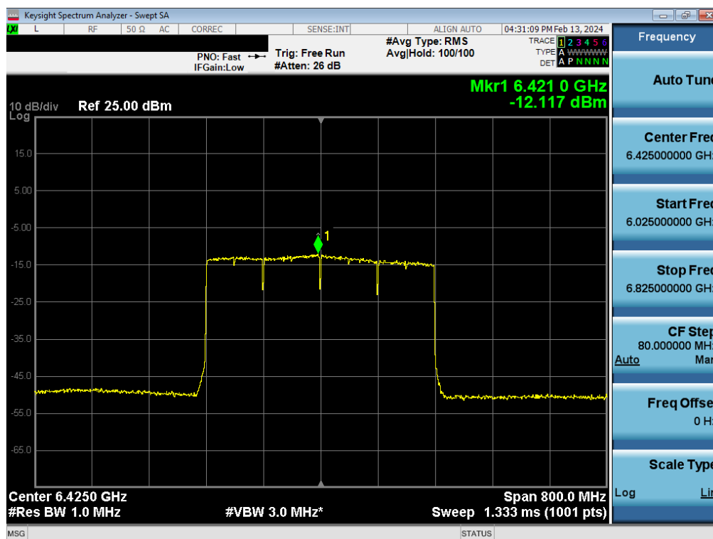
Plot 7-112. Power Spectral Density Plot MIMO ANT1 (320MHz BW 802.11be (Full Tone) (UNII Band 6) – Ch. 95) - LPI
