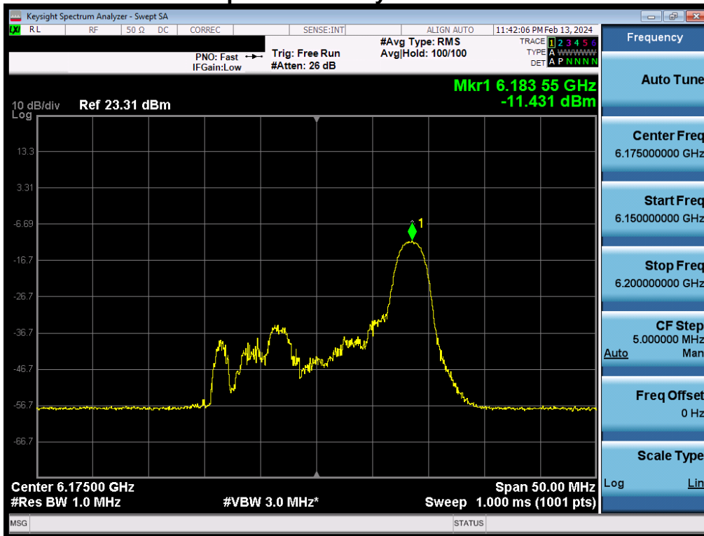
Plot 7-158. Power Spectral Density Plot MIMO ANT2 (20MHz BW 802.11be (26 Tones) (UNII Band 5) – Ch. 45) – LPI
