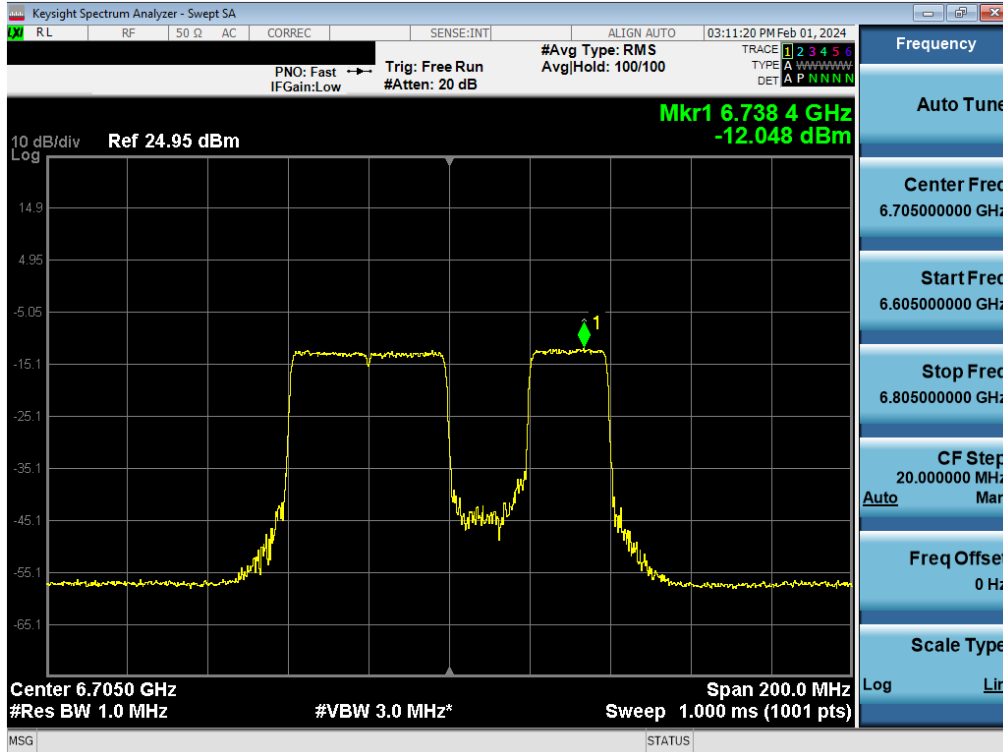
Plot 7-129. Power Spectral Density Plot MIMO ANT1 (80MHz BW 802.11be (484+242 Tone) (UNII Band 7) – Ch. 151) - LPI
