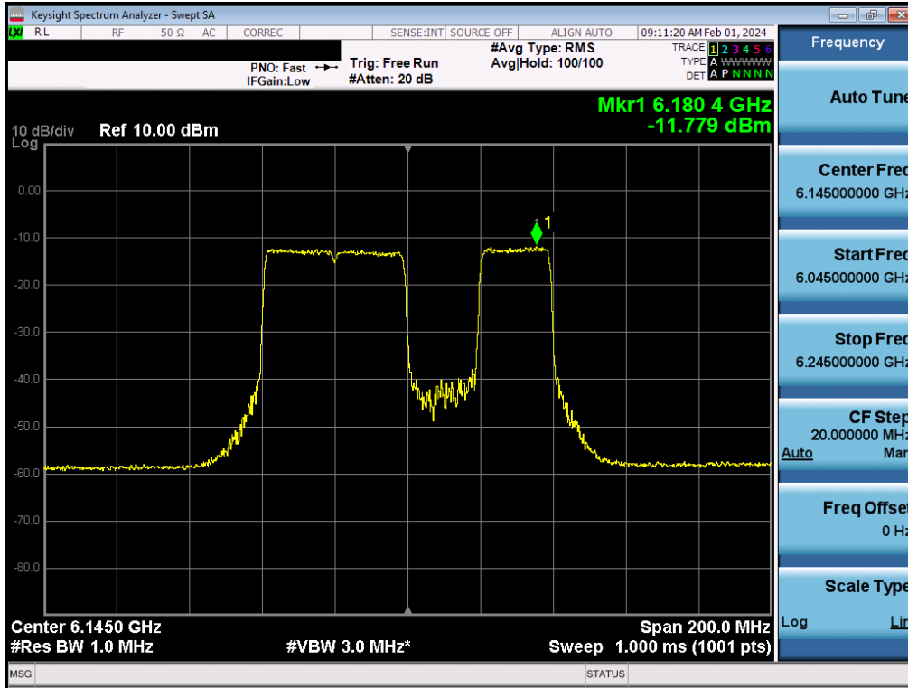
Plot 7-198. Power Spectral Density Plot MIMO ANT2 (80MHz BW 802.11be (484+242 Tone) (UNII Band 5) – Ch. 39) – LPI
