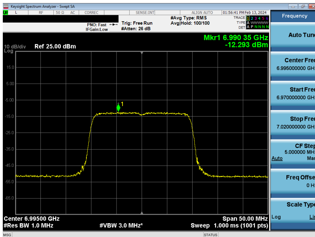
Plot 7-118. Power Spectral Density Plot MIMO ANT1 (20MHz BW 802.11be (Full Tone) (UNII Band 8) – Ch. 209) - LPI
