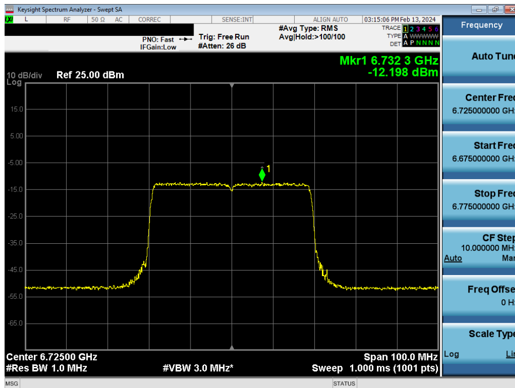
Plot 7-114. Power Spectral Density Plot MIMO ANT1 (40MHz BW 802.11be (Full Tone) (UNII Band 7) – Ch. 155) - LPI
