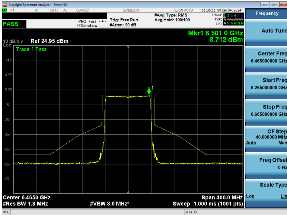
Plot 7-136. In-Band Emission MIMO ANT1 (80MHz 802.11ax/be (UNII Band 6) – Ch. 103)
