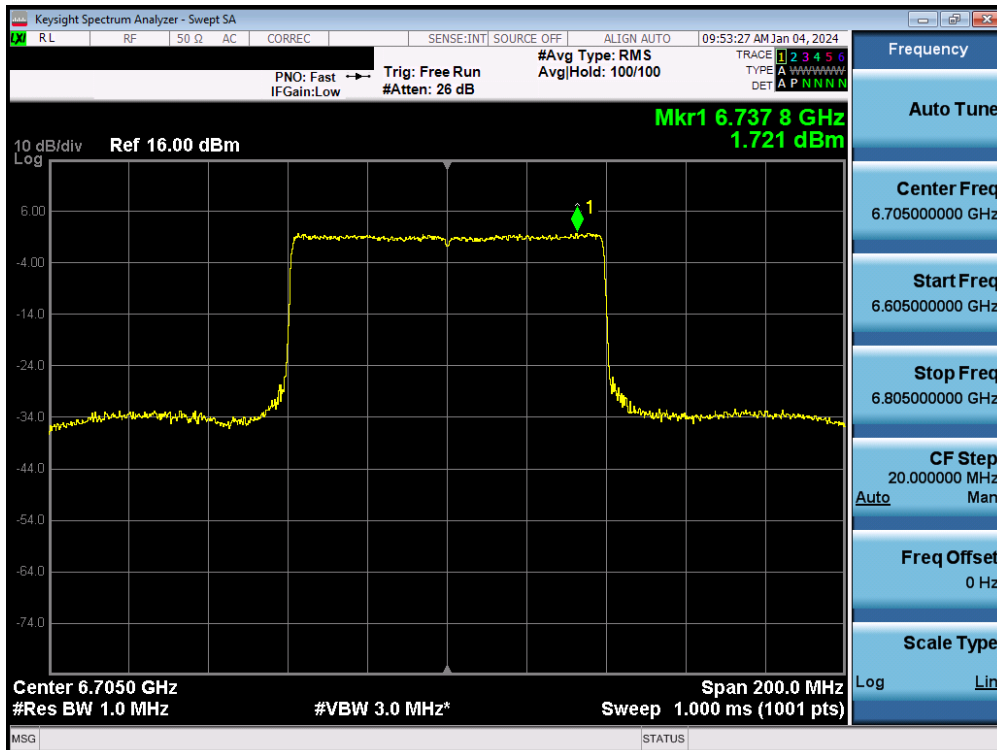
Plot 7-113. Power Spectral Density MIMO ANT2 (80MHz 802.11ax/be (UNII Band 7) – Ch. 151) - SP
