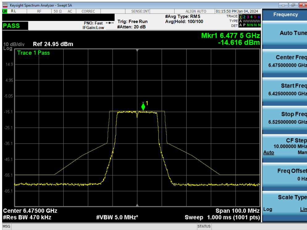
Plot 7-133. In-Band Emission MIMO ANT1 (20MHz 802.11a (UNII Band 6) – Ch. 105)
