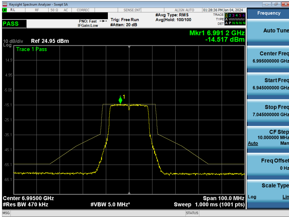
Plot 7-145. In-Band Emission MIMO ANT1 (20MHz 802.11a (UNII Band 8) – Ch. 209)
