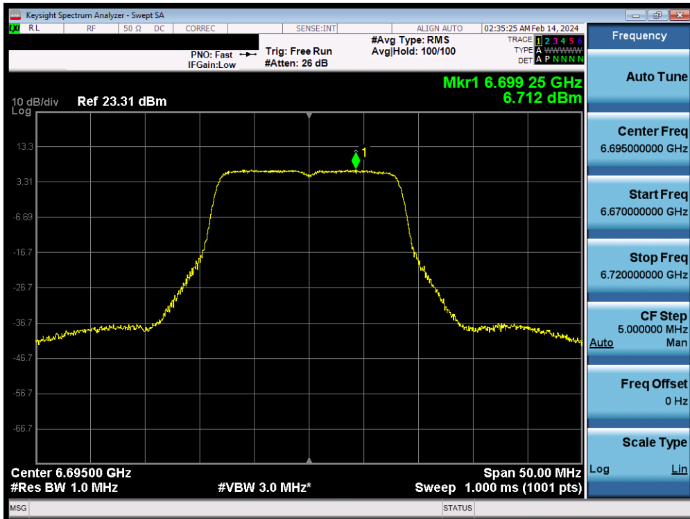
Plot 7-110. Power Spectral Density MIMO ANT2 (20MHz 802.11a (UNII Band 7) – Ch. 149) - SP
