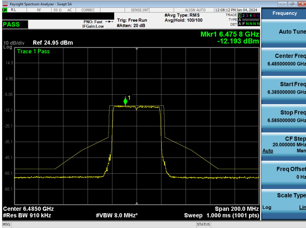
Plot 7-135. In-Band Emission MIMO ANT1 (40MHz 802.11ax/be (UNII Band 6) – Ch. 107)
