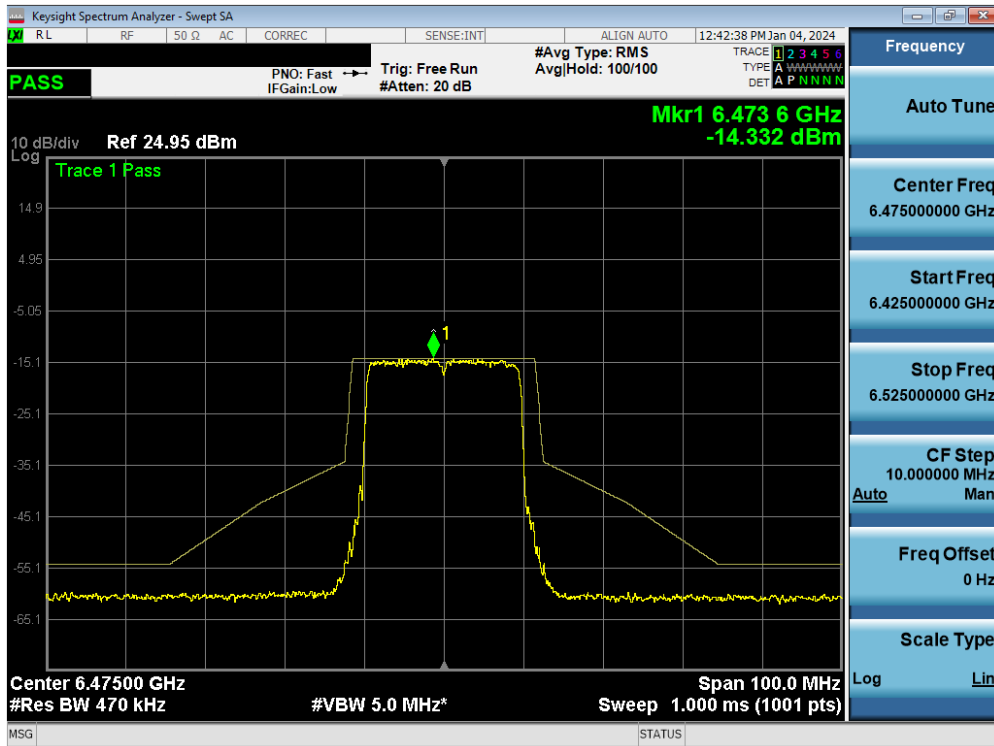
Plot 7-134. In-Band Emission MIMO ANT1 (20MHz 802.11ax/be (UNII Band 6) – Ch. 105)
