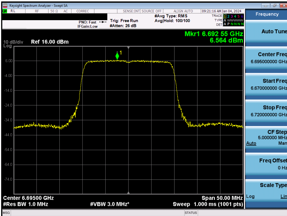
Plot 7-111. Power Spectral Density MIMO ANT2 (20MHz 802.11ax/be (UNII Band 7) – Ch. 149) - SP
