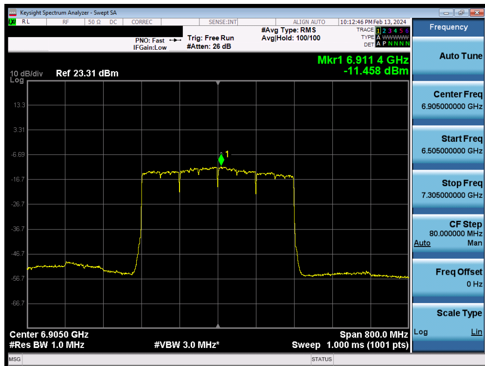
Plot 7-120. Power Spectral Density MIMO ANT2 (320MHz 802.11ax/be (UNII Band 7/8) – Ch. 191) - LPI
