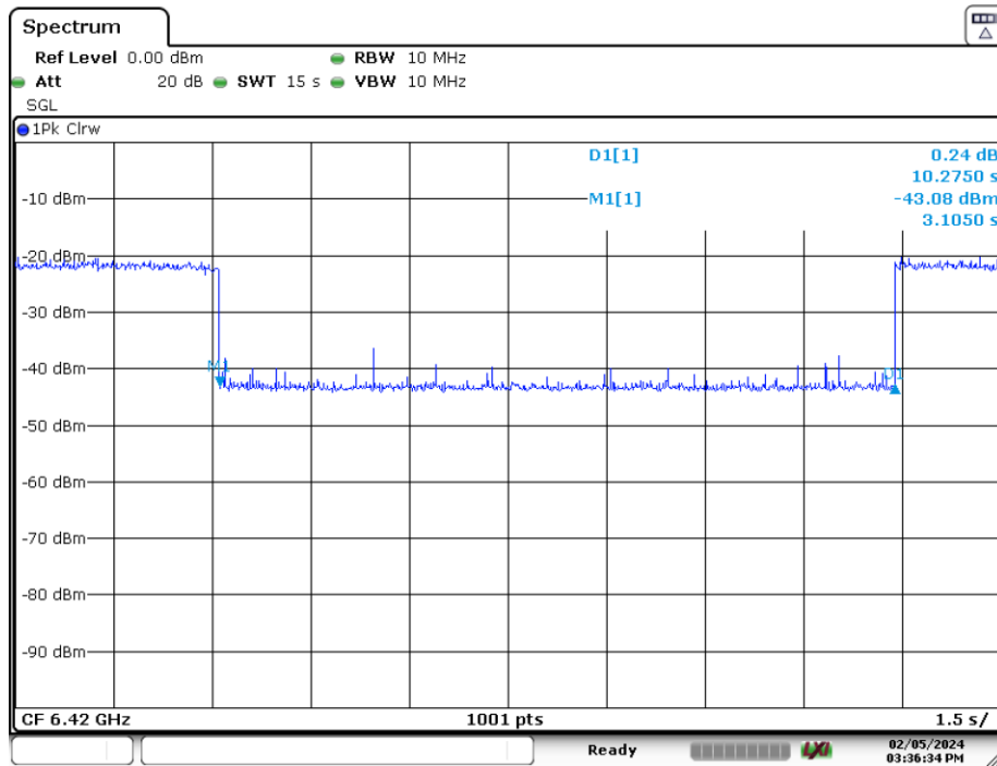
Plot 7-196. Contention Based Protocol Timing Plot (320MHz (UNII Band 5) – Ch. 31 High)
