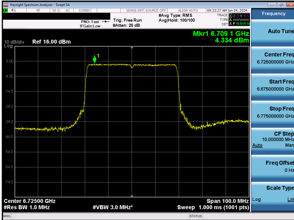
Plot 7-112. Power Spectral Density MIMO ANT2 (40MHz 802.11ax/be (UNII Band 7) – Ch. 155) - SP
