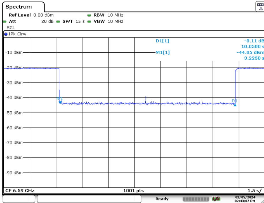
Plot 7-202. Contention Based Protocol Timing Plot (320MHz (UNII Band 7) – Ch. 159 Low)
