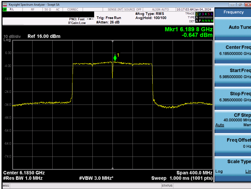
Plot 7-96. Power Spectral Density MIMO ANT2 (160MHz 802.11ax/be (UNII Band 5) – Ch. 47) - SP
