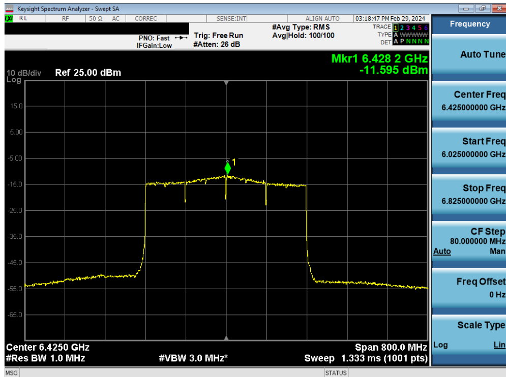
Plot 7-103. Power Spectral Density MIMO ANT2 (320MHz 802.11ax/be (UNII Band 5/6/7) – Ch. 95) - LPI
