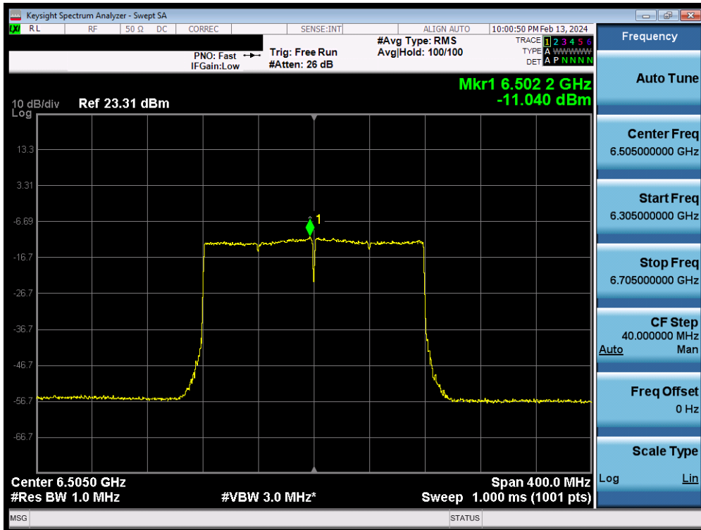
Plot 7-102. Power Spectral Density MIMO ANT2 (160MHz 802.11ax/be (UNII Band 6) – Ch. 111) - LPI
