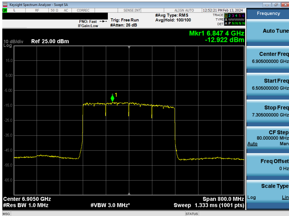
Plot 7-85. Power Spectral Density MIMO ANT1 (320MHz 802.11ax/be (UNII Band 7/8) – Ch. 191) - LPI
