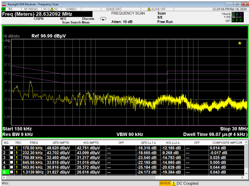
Plot 7-199. Line-Conducted Test Plot (N)
