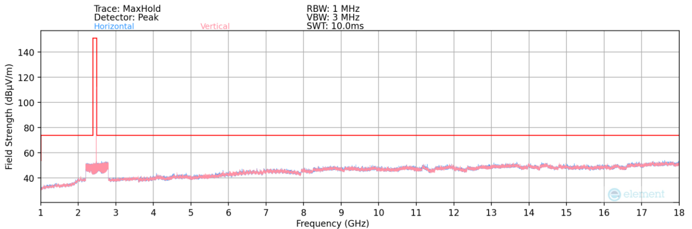
Plot 7-175. Radiated Spurious Plot above 1GHz (BT – Ch. 78)
