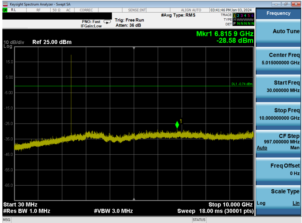
Plot 7-143. Conducted Spurious Plot (Bluetooth, 1Mbps – Ch. 0)
