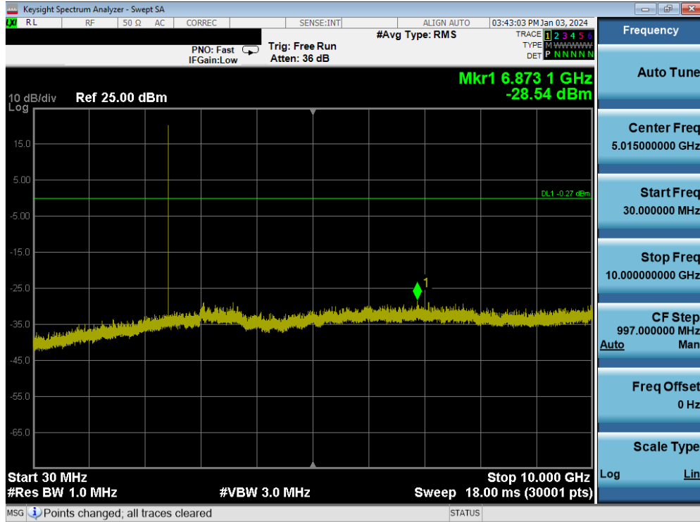
Plot 7-145. Conducted Spurious Plot (Bluetooth, 1Mbps – Ch. 39)
