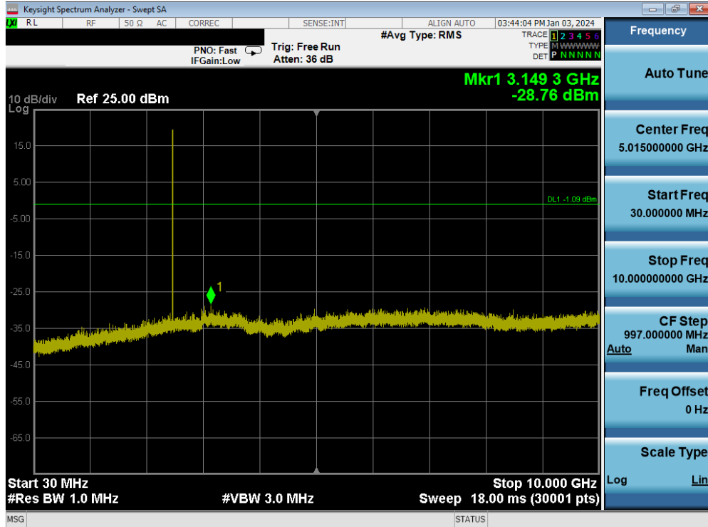
Plot 7-147. Conducted Spurious Plot (Bluetooth, 1Mbps – Ch. 78)
