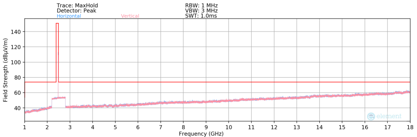
Plot 7-172. Radiated Spurious Plot above 1GHz (BT – Ch. 78)
