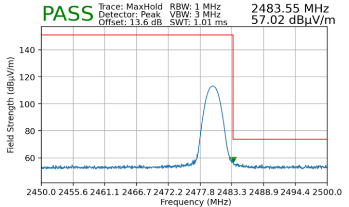
Plot 7-180. Radiated Restricted Upper Band Edge Measurement (Peak) – SISO ANT1
