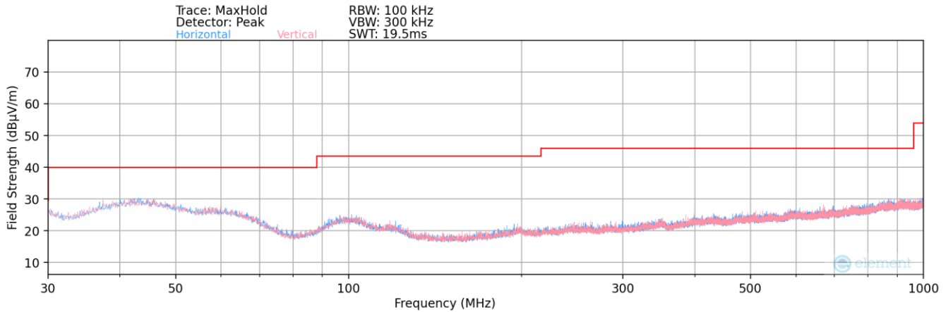
Plot 7-195. Radiated Spurious Plot below 1GHz – SISO ANT1
