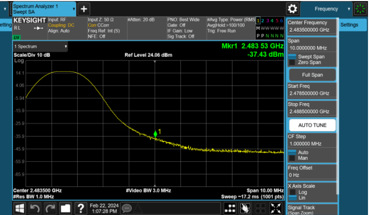
Plot 7-184. Radiated Restricted Upper Band Edge Measurement (Peak) – DUAL ANT1
