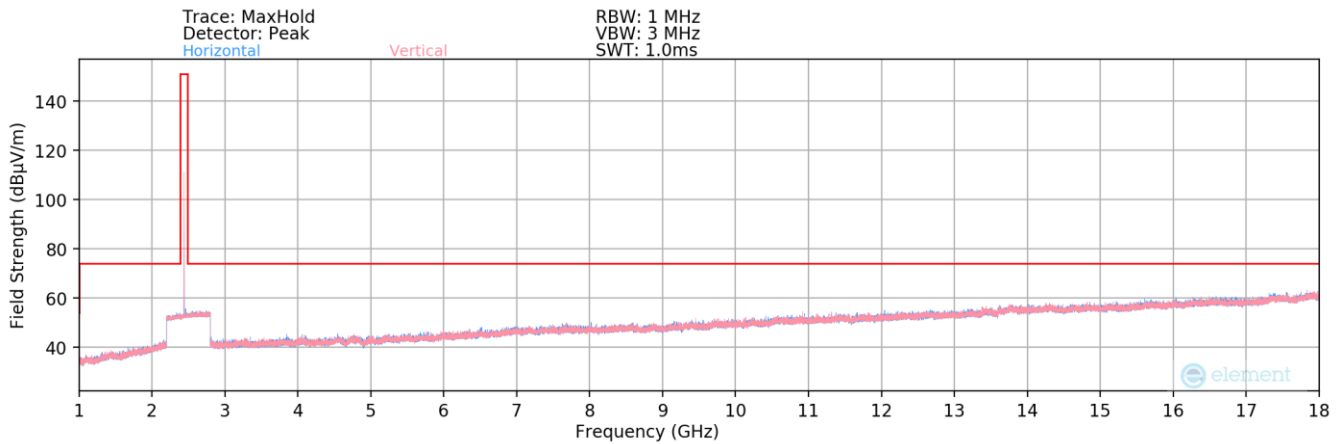
Plot 7-168. Radiated Spurious Plot above 1GHz (BT – Ch. 39)
