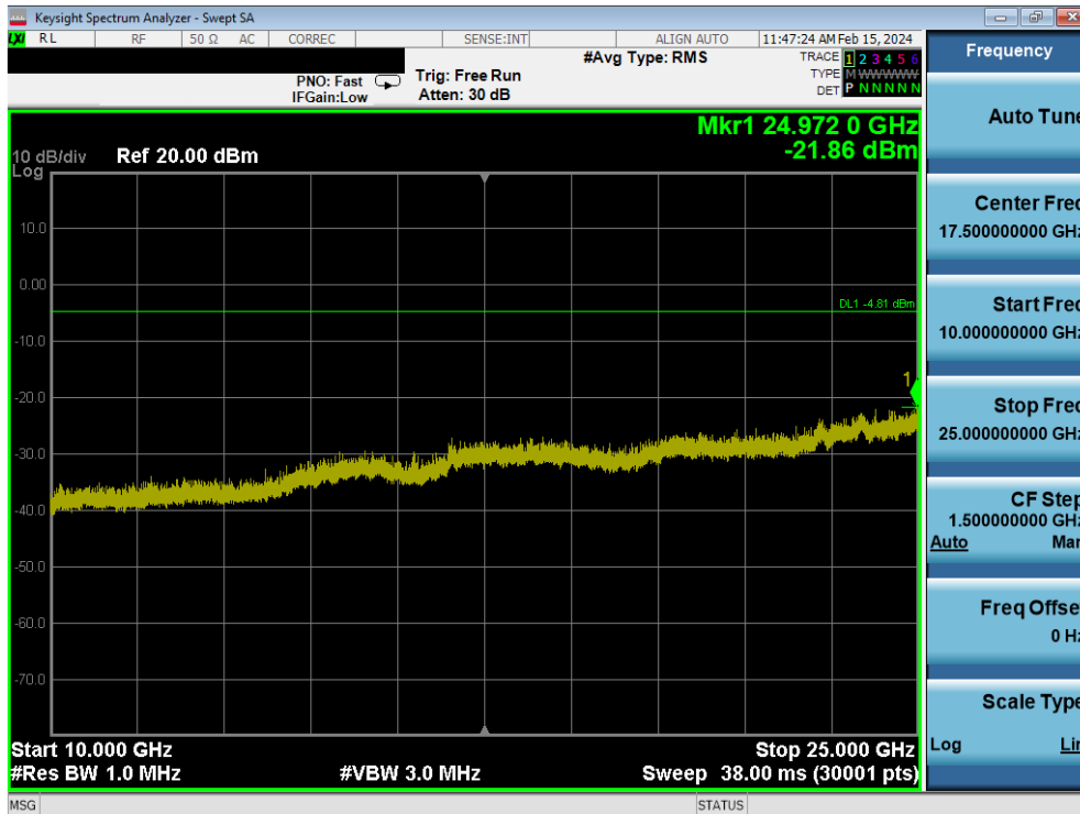
Plot 7-164. Conducted Spurious Plot (Bluetooth, 1Mbps – Ch. 39)
