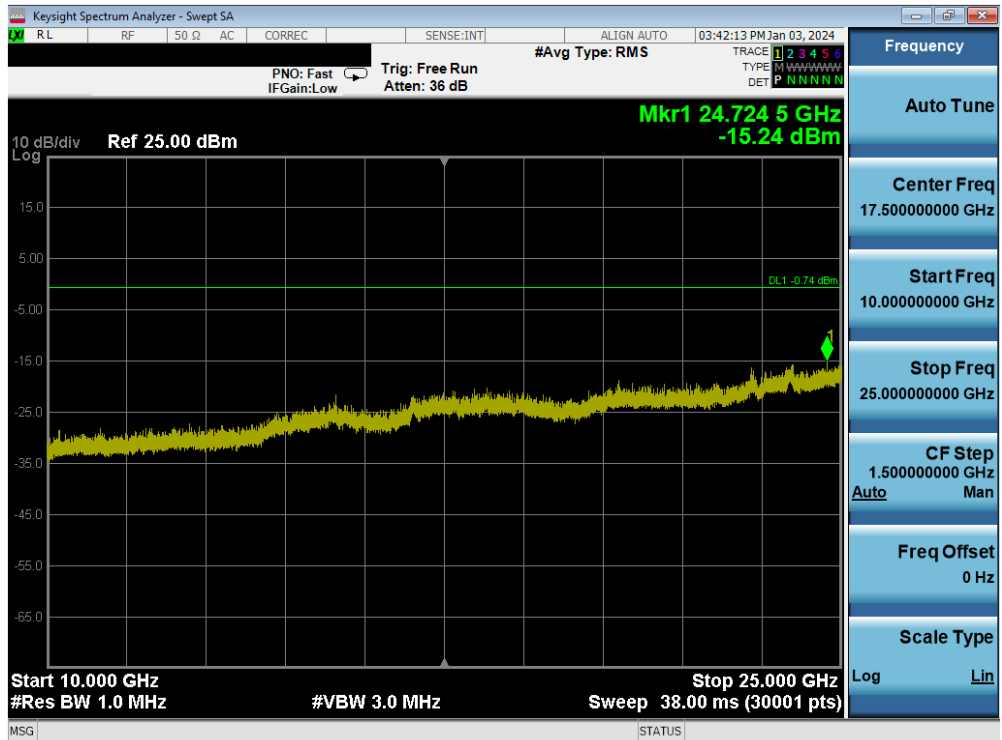
Plot 7-144. Conducted Spurious Plot (Bluetooth, 1Mbps – Ch. 0)
