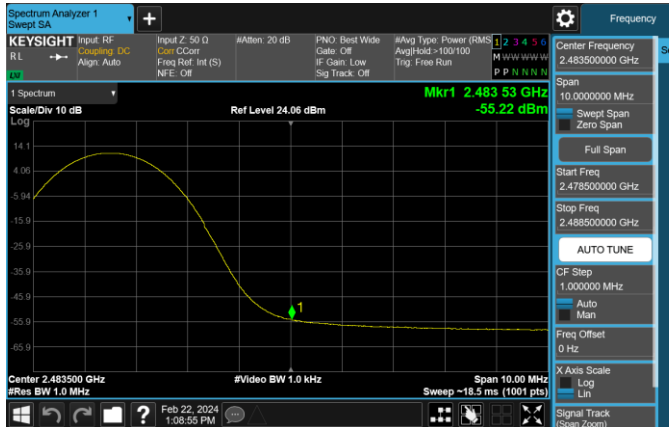
Plot 7-187. Radiated Restricted Upper Band Edge Measurement (Average) – DUAL ANT1
