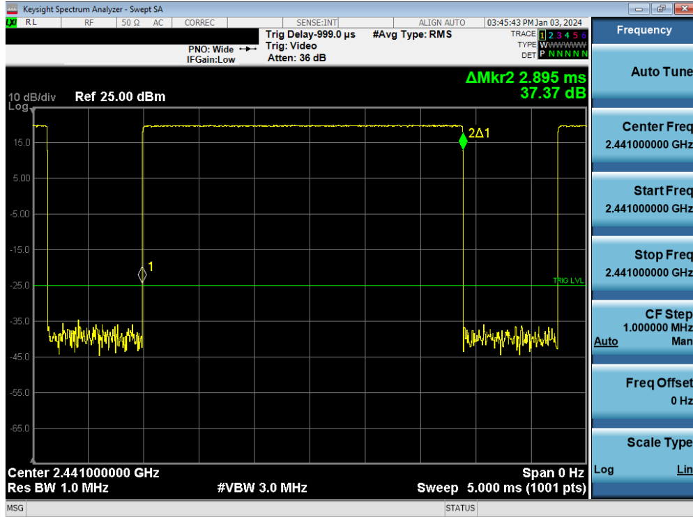
Plot 7-131. Time of Occupancy Plot (Bluetooth) – SISO ANT1
