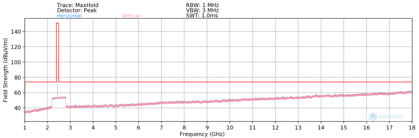
Plot 7-171. Radiated Spurious Plot above 1GHz (BT – Ch. 39)
