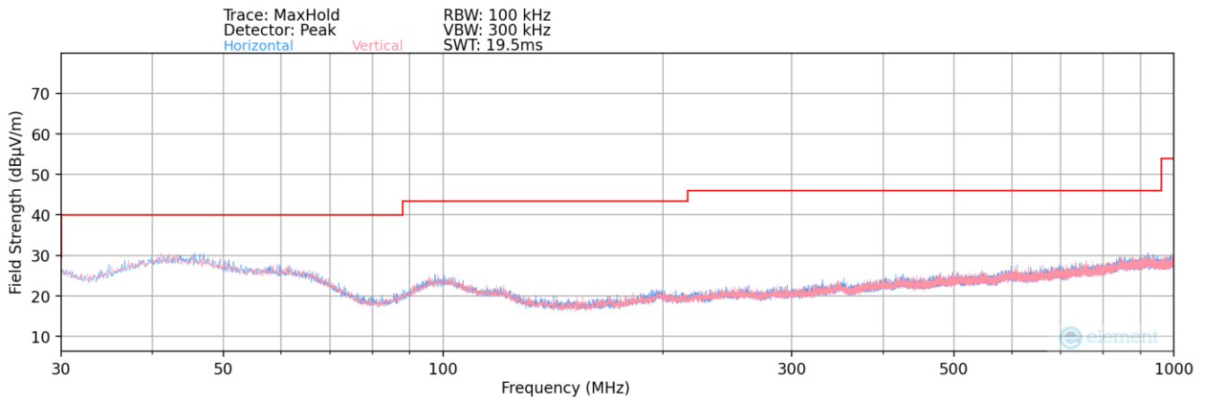
Plot 7-196. Radiated Spurious Plot below 1GHz – SISO ANT2
