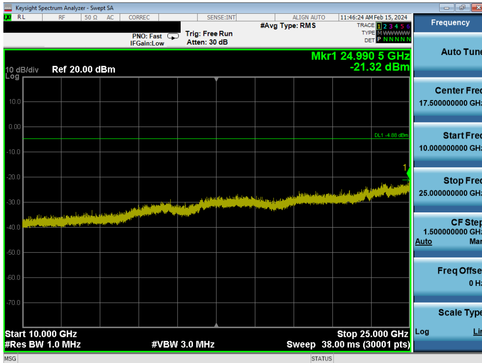
Plot 7-162. Conducted Spurious Plot (Bluetooth, 1Mbps – Ch. 0)
