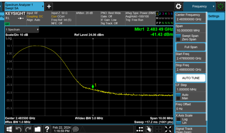
Plot 7-190. Radiated Restricted Upper Band Edge Measurement (Peak) – DUAL ANT2
