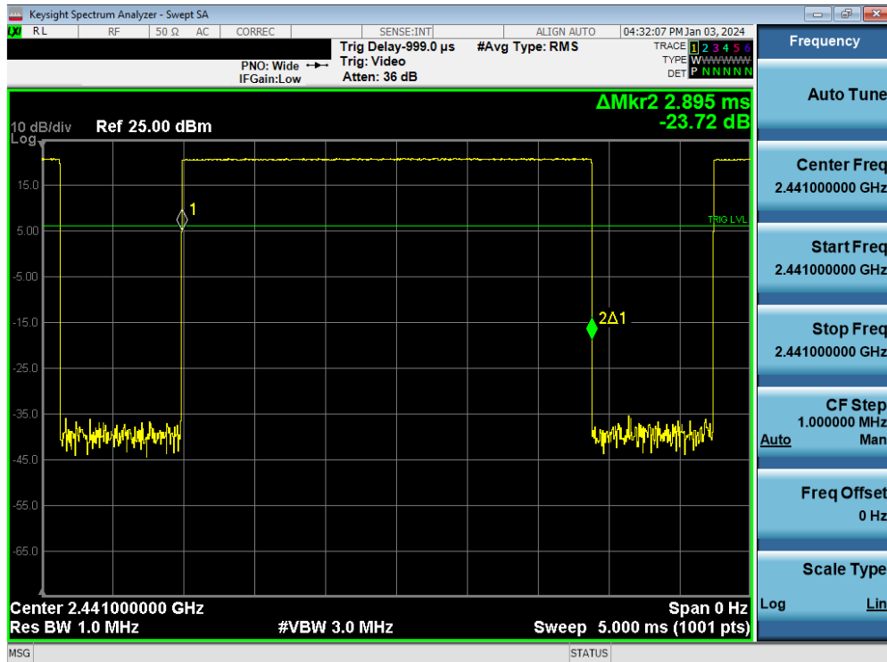
Plot 7-132. Time of Occupancy Plot (Bluetooth) – SISO ANT2
