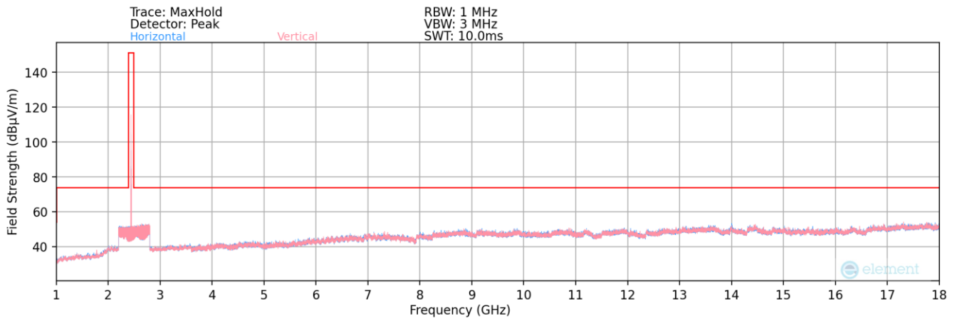
Plot 7-174. Radiated Spurious Plot above 1GHz (BT – Ch. 39)
