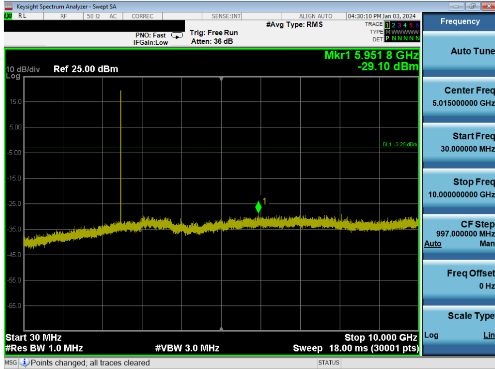
Plot 7-153. Conducted Spurious Plot (Bluetooth, 1Mbps – Ch. 78)
