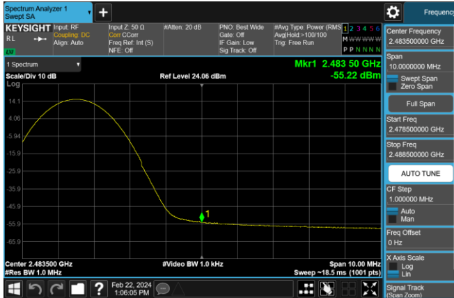
Plot 7-183. Radiated Restricted Upper Band Edge Measurement (Average) – DUAL ANT1
