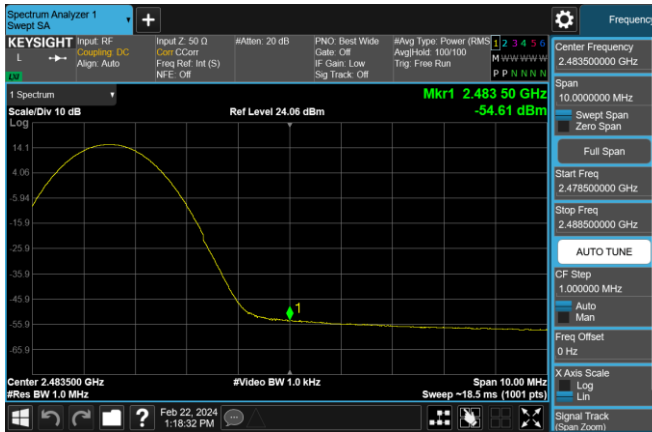
Plot 7-185. Radiated Restricted Upper Band Edge Measurement (Average) – DUAL ANT2
