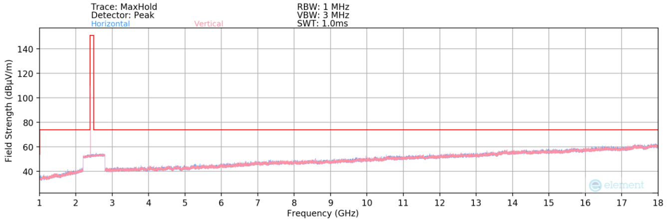
Plot 7-170. Radiated Spurious Plot above 1GHz (BT – Ch. 0)
