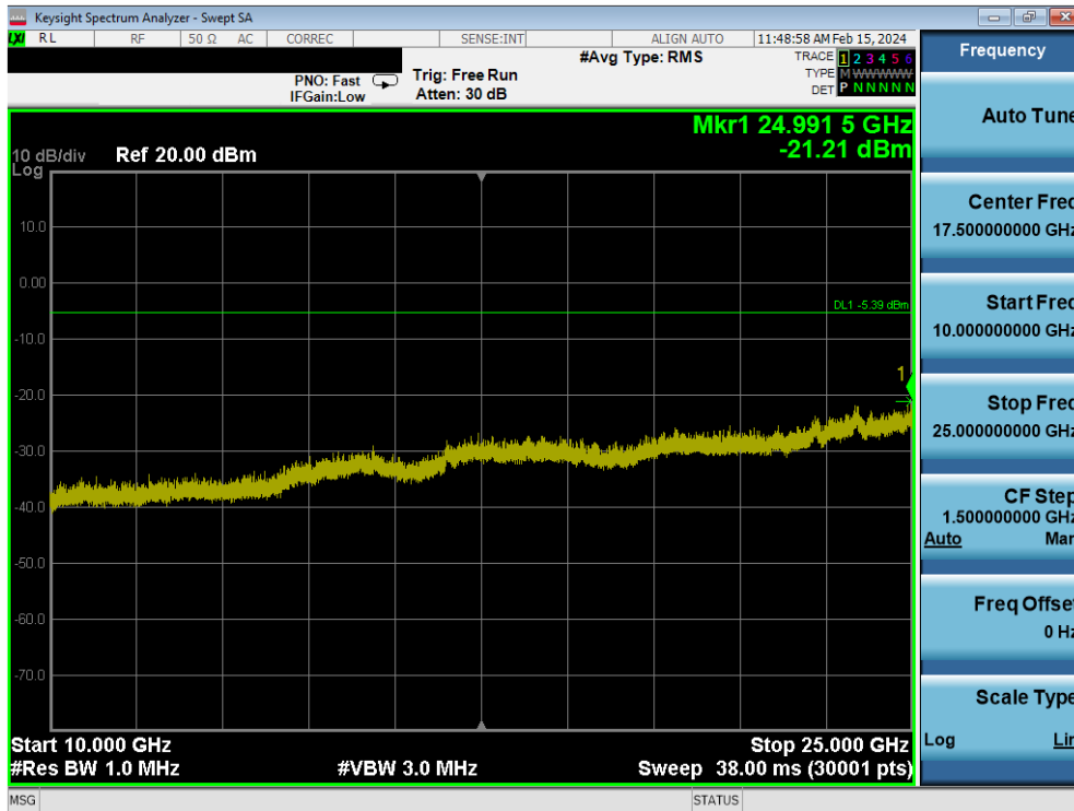
Plot 7-166. Conducted Spurious Plot (Bluetooth, 1Mbps – Ch. 78)
