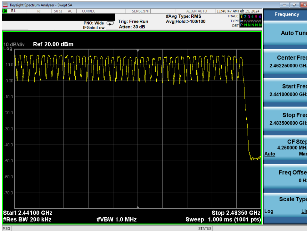
Plot 7-142. High End Spectrum Channel Hopping Plot (Bluetooth)
