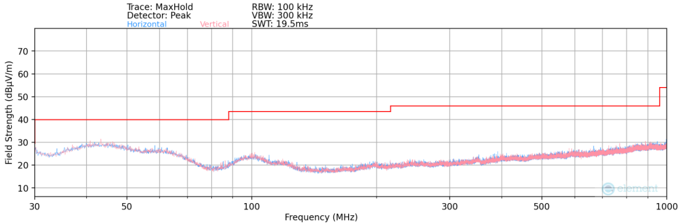
Plot 7-197. Radiated Spurious Plot below 1GHz – DUAL
