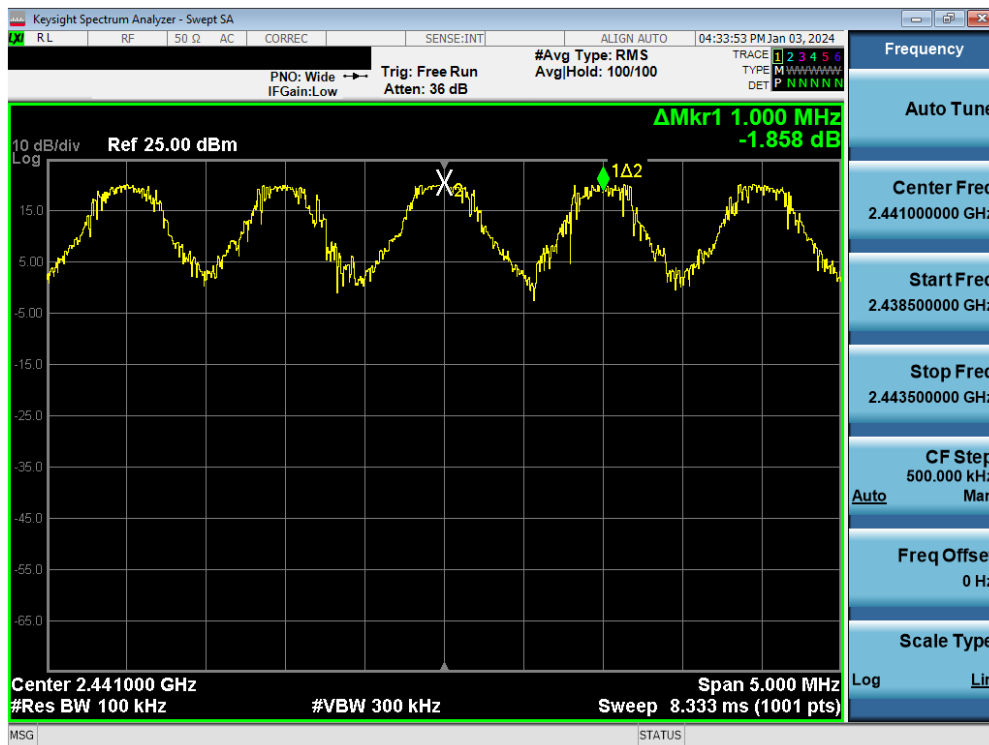
Plot 7-128. Channel Spacing Plot (Bluetooth) – SISO ANT2
