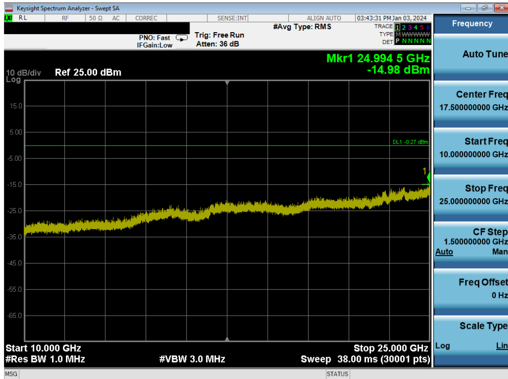
Plot 7-146. Conducted Spurious Plot (Bluetooth, 1Mbps – Ch. 39)
