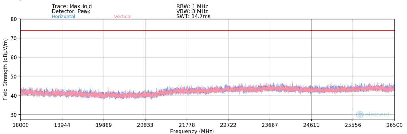
Plot 7-178. Radiated Spurious Plot above 18GHz
