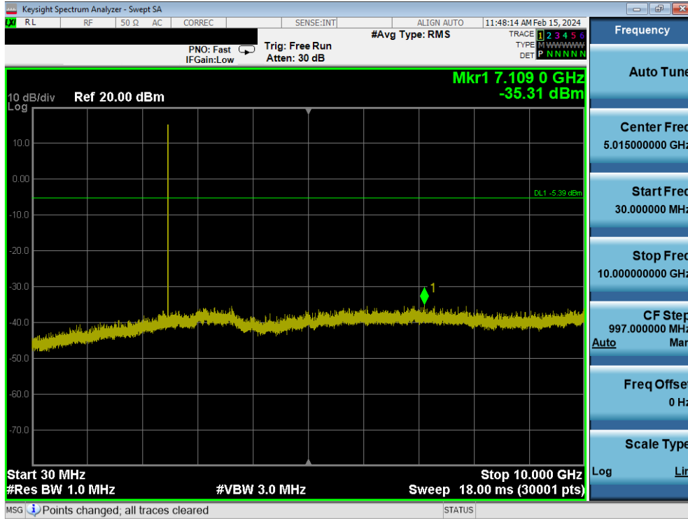
Plot 7-165. Conducted Spurious Plot (Bluetooth, 1Mbps – Ch. 78)
