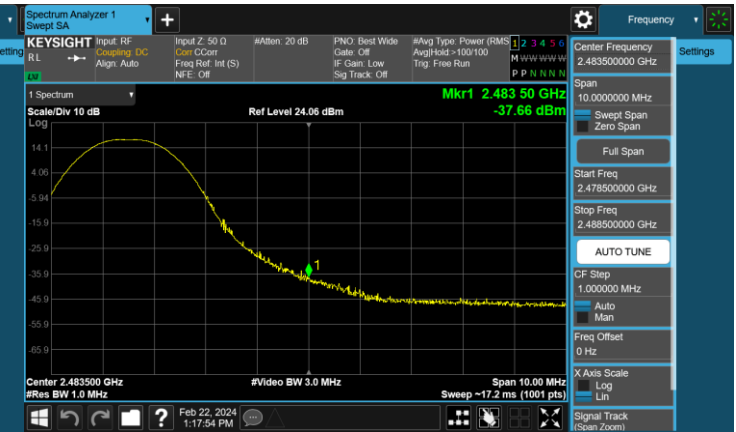
Plot 7-186. Radiated Restricted Upper Band Edge Measurement (Peak) – DUAL ANT2
