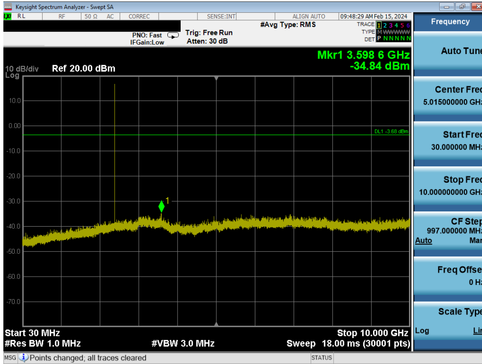
Plot 7-155. Conducted Spurious Plot (Bluetooth, 1Mbps – Ch. 0)
