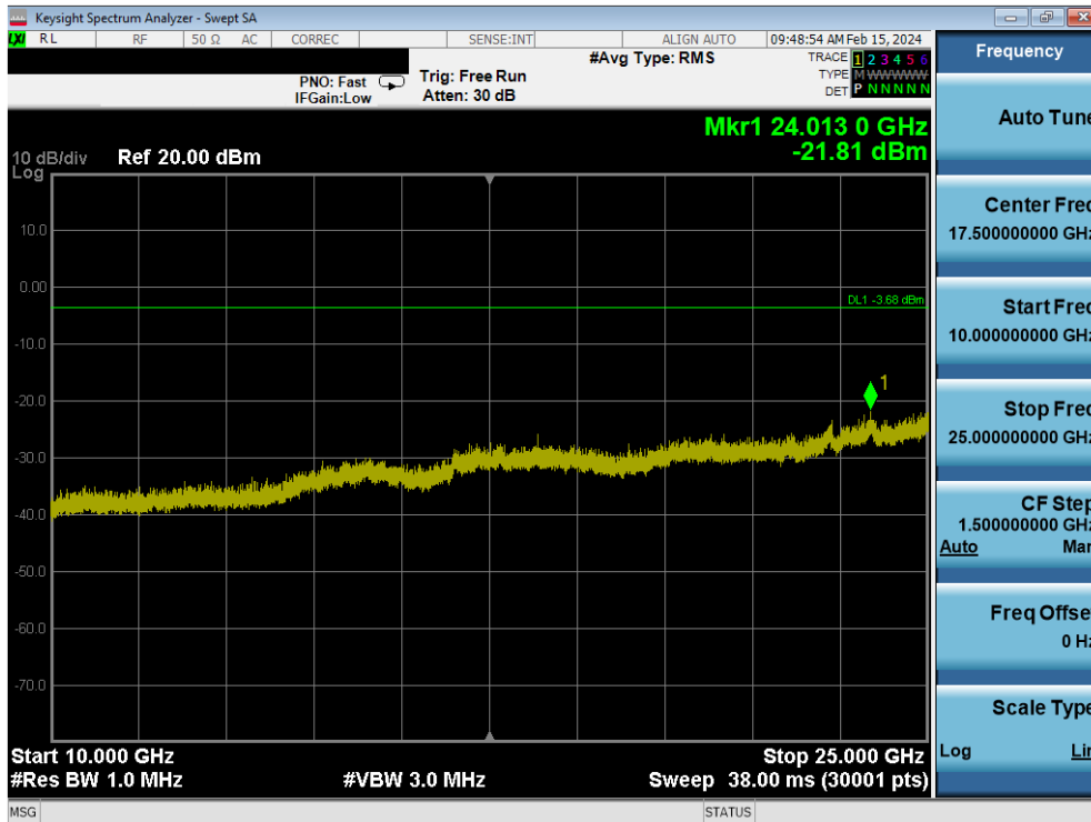
Plot 7-156. Conducted Spurious Plot (Bluetooth, 1Mbps – Ch. 0)
