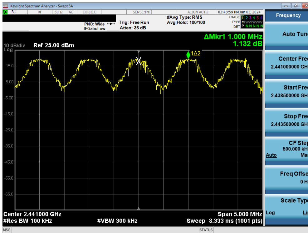
Plot 7-127. Channel Spacing Plot (Bluetooth) – SISO ANT1
