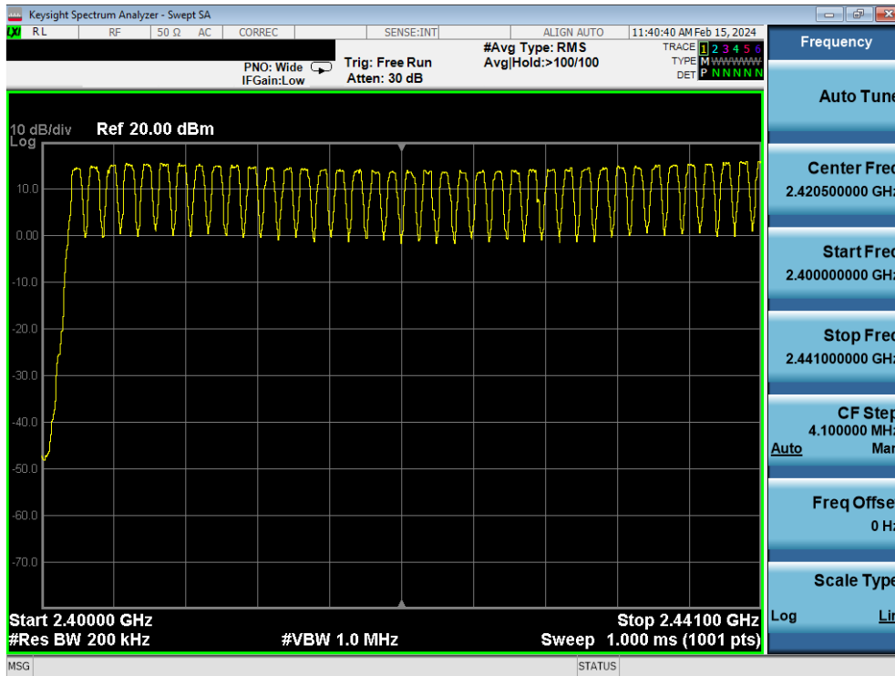
Plot 7-141. Low End Spectrum Channel Hopping Plot (Bluetooth)
