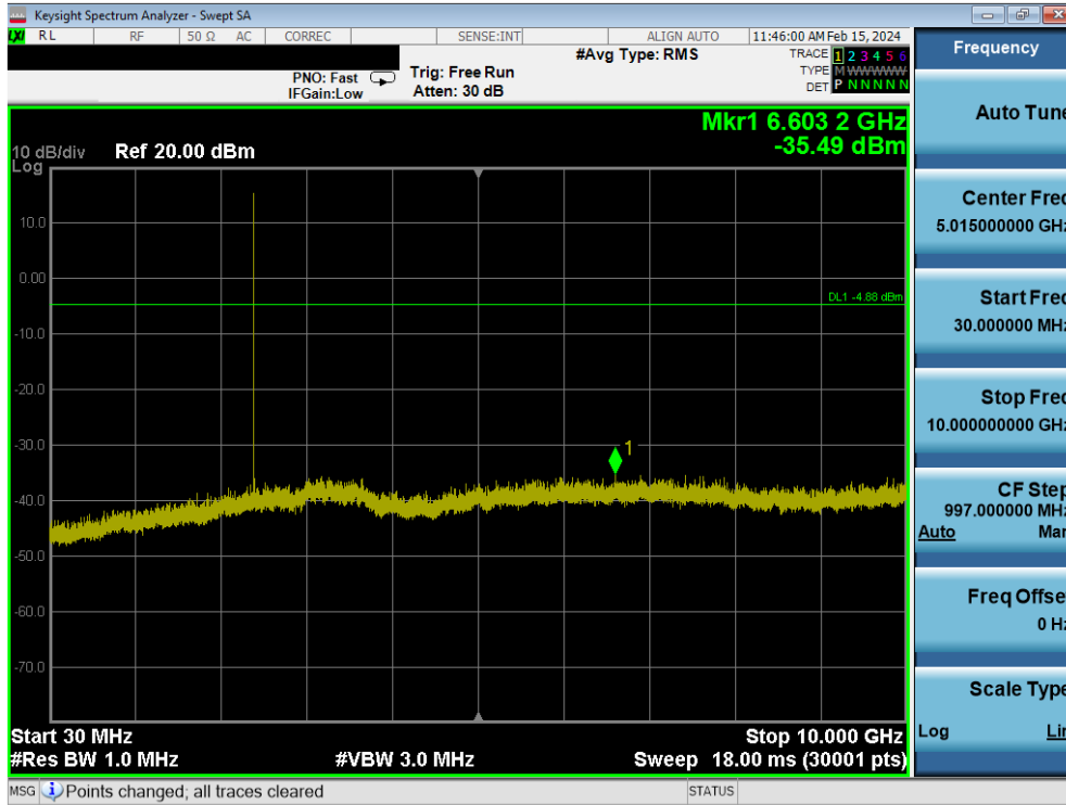
Plot 7-161. Conducted Spurious Plot (Bluetooth, 1Mbps – Ch. 0)
