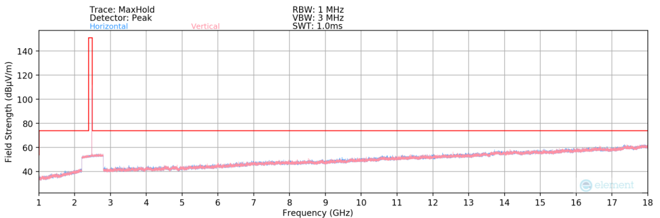
Plot 7-169. Radiated Spurious Plot above 1GHz (BT – Ch. 78)
