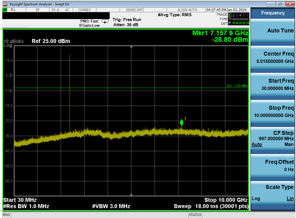
Plot 7-149. Conducted Spurious Plot (Bluetooth, 1Mbps – Ch. 0)
