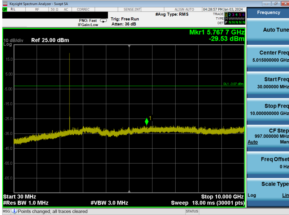
Plot 7-151. Conducted Spurious Plot (Bluetooth, 1Mbps - Ch. 39)
