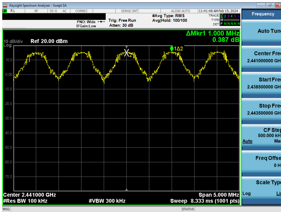
Plot 7-130. Channel Spacing Plot (Bluetooth) – DUAL ANT2
