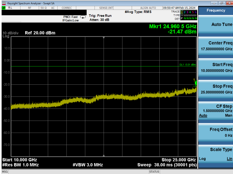
Plot 7-160. Conducted Spurious Plot (Bluetooth, 1Mbps – Ch. 78)
