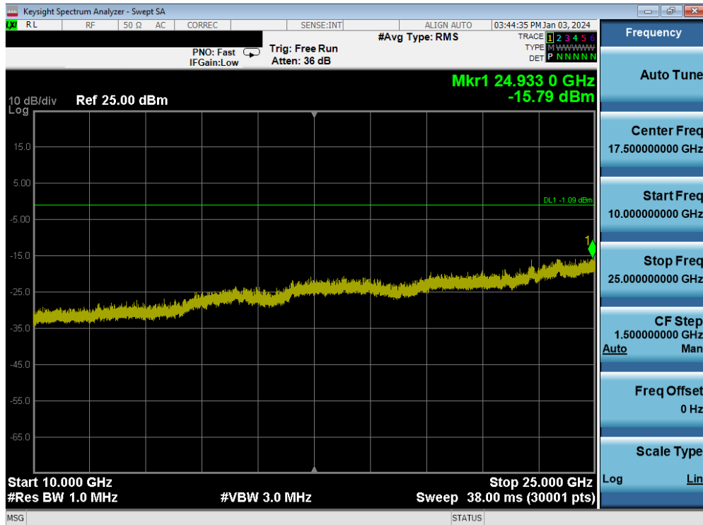
Plot 7-148. Conducted Spurious Plot (Bluetooth, 1Mbps – Ch. 78)
