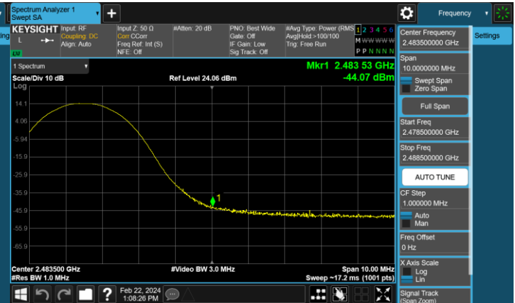
Plot 7-188. Radiated Restricted Upper Band Edge Measurement (Peak) – DUAL ANT1
