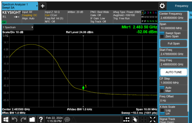
Plot 7-193. Radiated Restricted Upper Band Edge Measurement (Average) – DUAL ANT2
