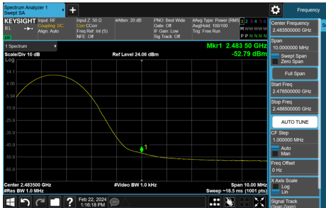
Plot 7-189. Radiated Restricted Upper Band Edge Measurement (Average) – DUAL ANT2
