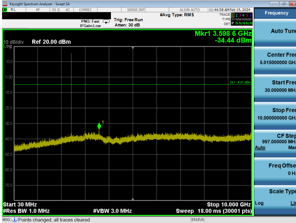
Plot 7-163. Conducted Spurious Plot (Bluetooth, 1Mbps – Ch. 39)
