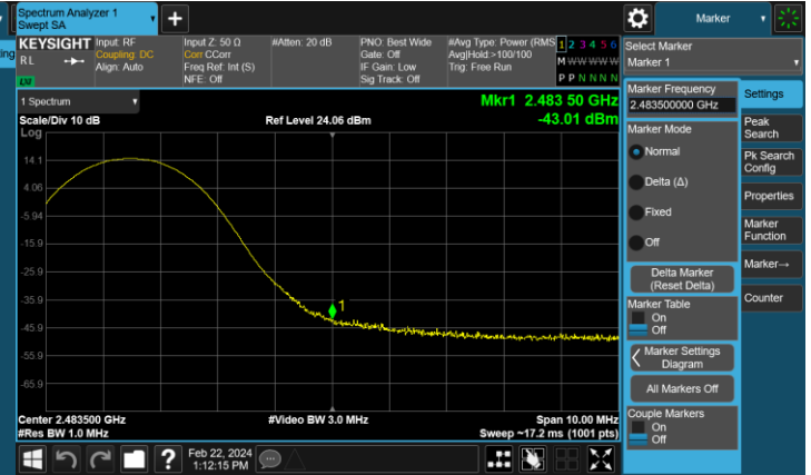
Plot 7-192. Radiated Restricted Upper Band Edge Measurement (Peak) – DUAL ANT1
