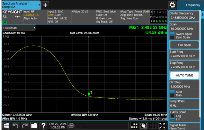
Plot 7-191. Radiated Restricted Upper Band Edge Measurement (Average) – DUAL ANT1
