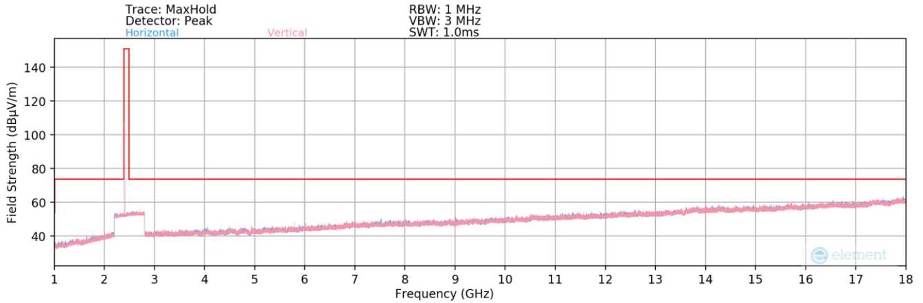
Plot 7-167. Radiated Spurious Plot above 1GHz (BT – Ch. 0)
