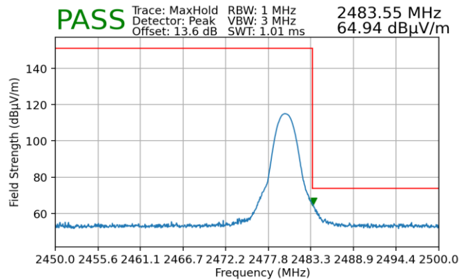
Plot 7-182. Radiated Restricted Upper Band Edge Measurement (Peak) – SISO ANT2
