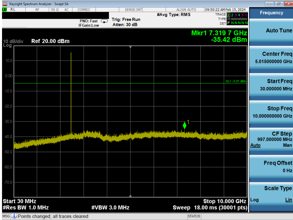
Plot 7-159. Conducted Spurious Plot (Bluetooth, 1Mbps – Ch. 78)
