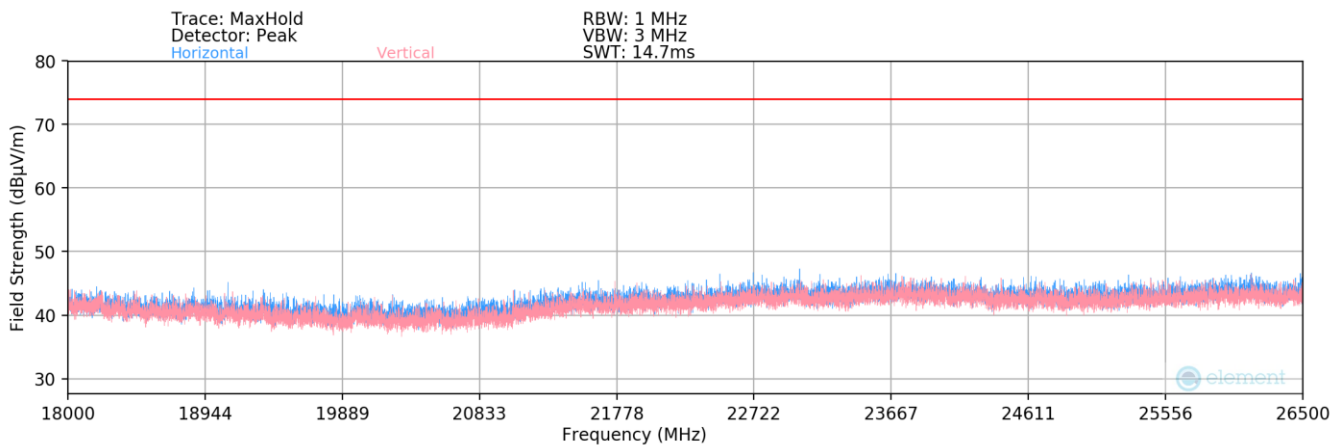
Plot 7-177. Radiated Spurious Plot above 18GHz
