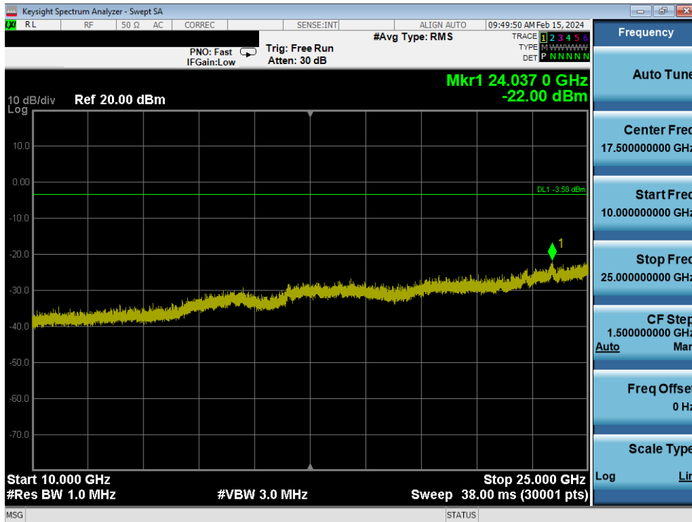
Plot 7-158. Conducted Spurious Plot (Bluetooth, 1Mbps – Ch. 39)
