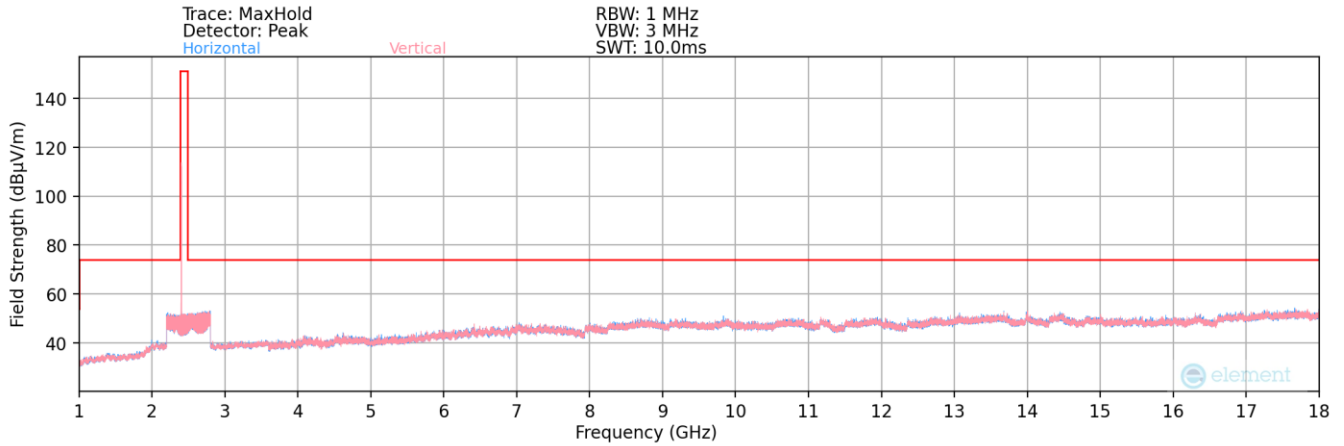
Plot 7-173. Radiated Spurious Plot above 1GHz (BT – Ch. 0)
