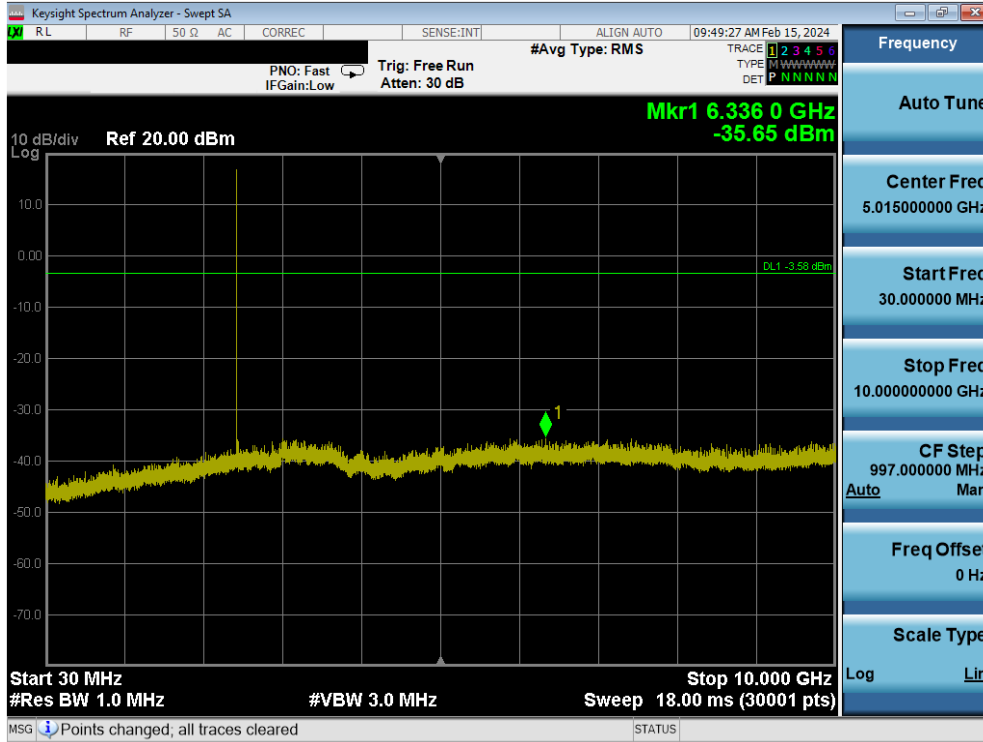
Plot 7-157. Conducted Spurious Plot (Bluetooth, 1Mbps – Ch. 39)
