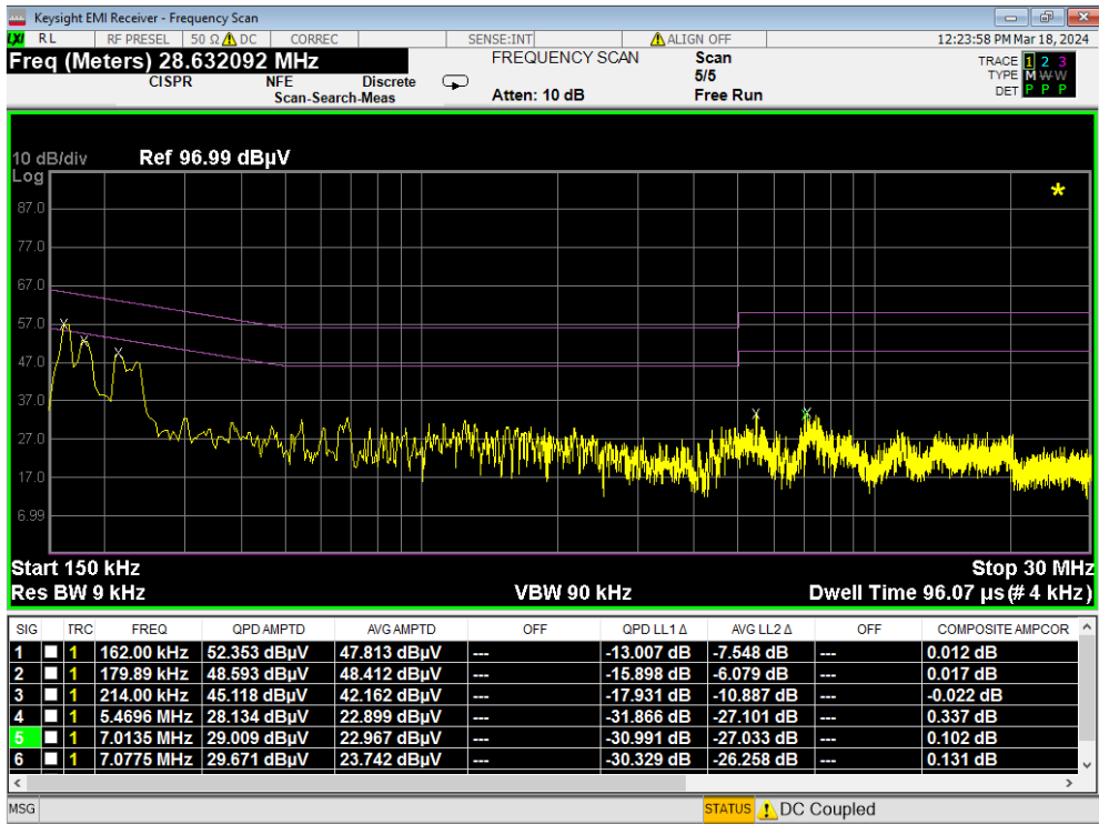
Plot 7-198. Line-Conducted Test Plot (L1)
