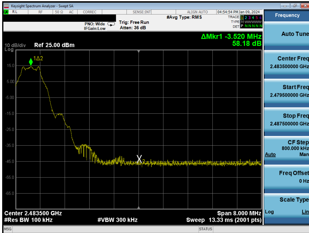
Plot 7-128. Band Edge Plot (Bluetooth (LE), 1Mbps – Ch. 39)
