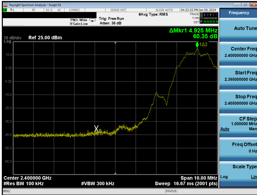
Plot 7-125. Band Edge Plot (Bluetooth (LE), 2Mbps – Ch. 0)
