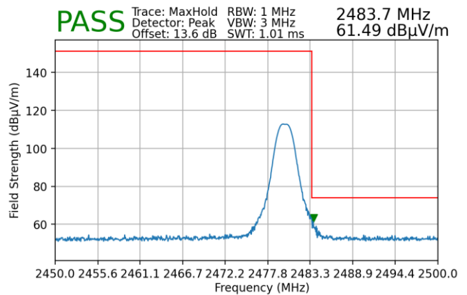
Plot 7-160. Radiated Restricted Upper Band Edge Measurement (Peak) – SISO ANT1
