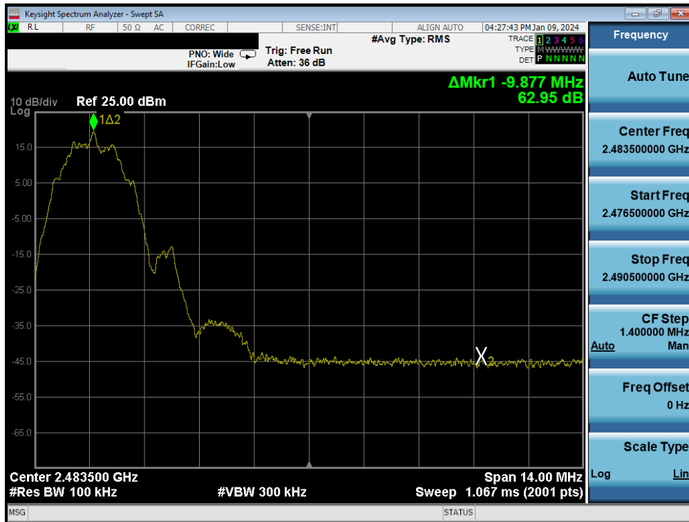
Plot 7-126. Band Edge Plot (Bluetooth (LE), 2Mbps – Ch. 36)
