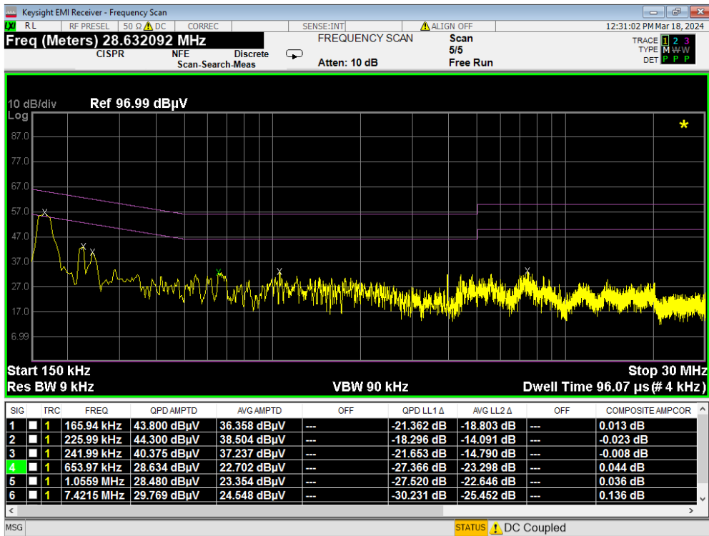
Plot 7-165. Line Conducted Plot with Bluetooth LE (L1)
