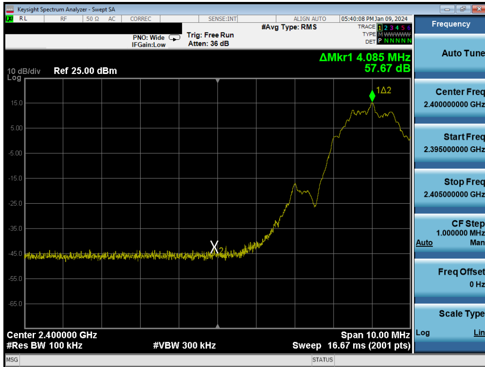
Plot 7-133. Band Edge Plot (Bluetooth (LE), 2Mbps – Ch. 0)
