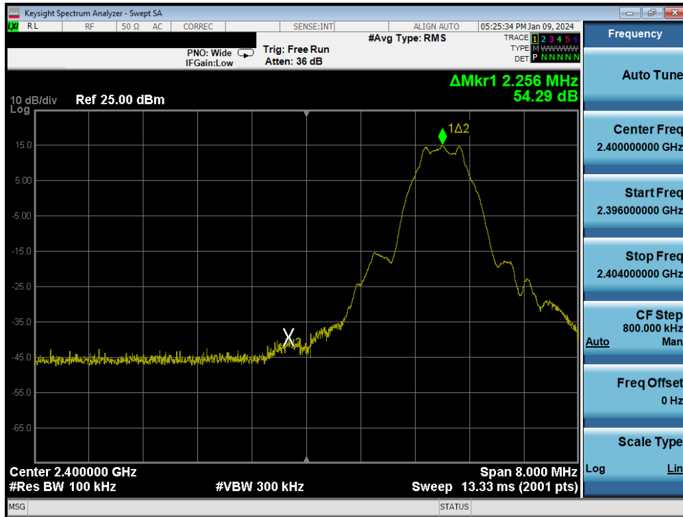
Plot 7-131. Band Edge Plot (Bluetooth (LE), 1Mbps – Ch. 37)
