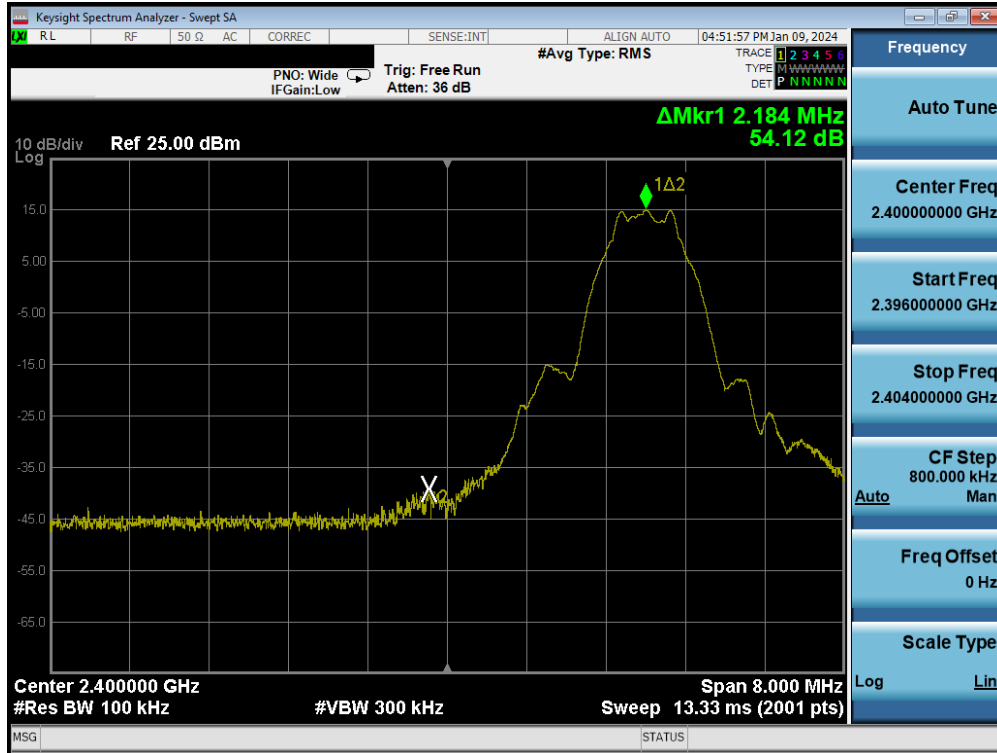
Plot 7-127. Band Edge Plot (Bluetooth (LE), 1Mbps – Ch. 37)
