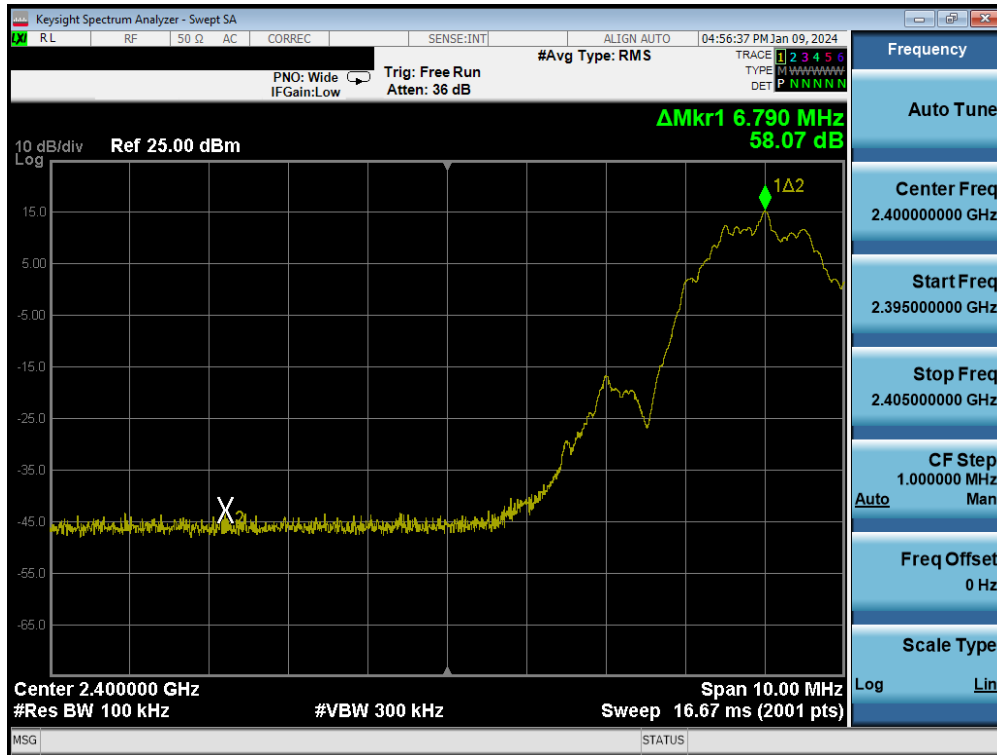
Plot 7-129. Band Edge Plot (Bluetooth (LE), 2Mbps – Ch. 0)
