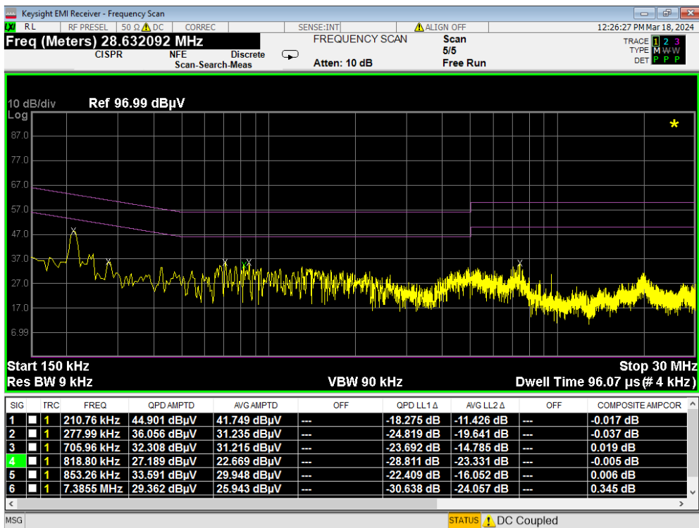
Plot 7-166. Line Conducted Plot with Bluetooth LE (N)
