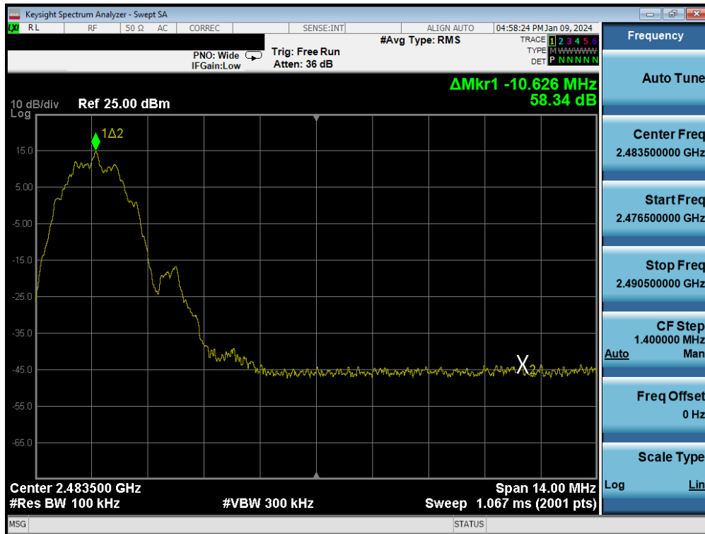
Plot 7-130. Band Edge Plot (Bluetooth (LE), 2Mbps – Ch. 36)
