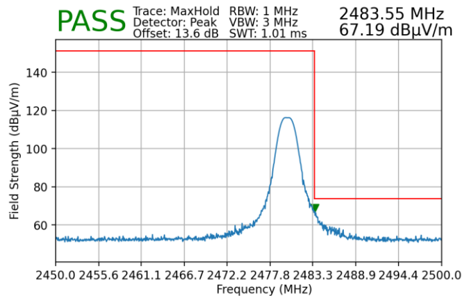
Plot 7-162. Radiated Restricted Upper Band Edge Measurement (Peak) – SISO ANT2
