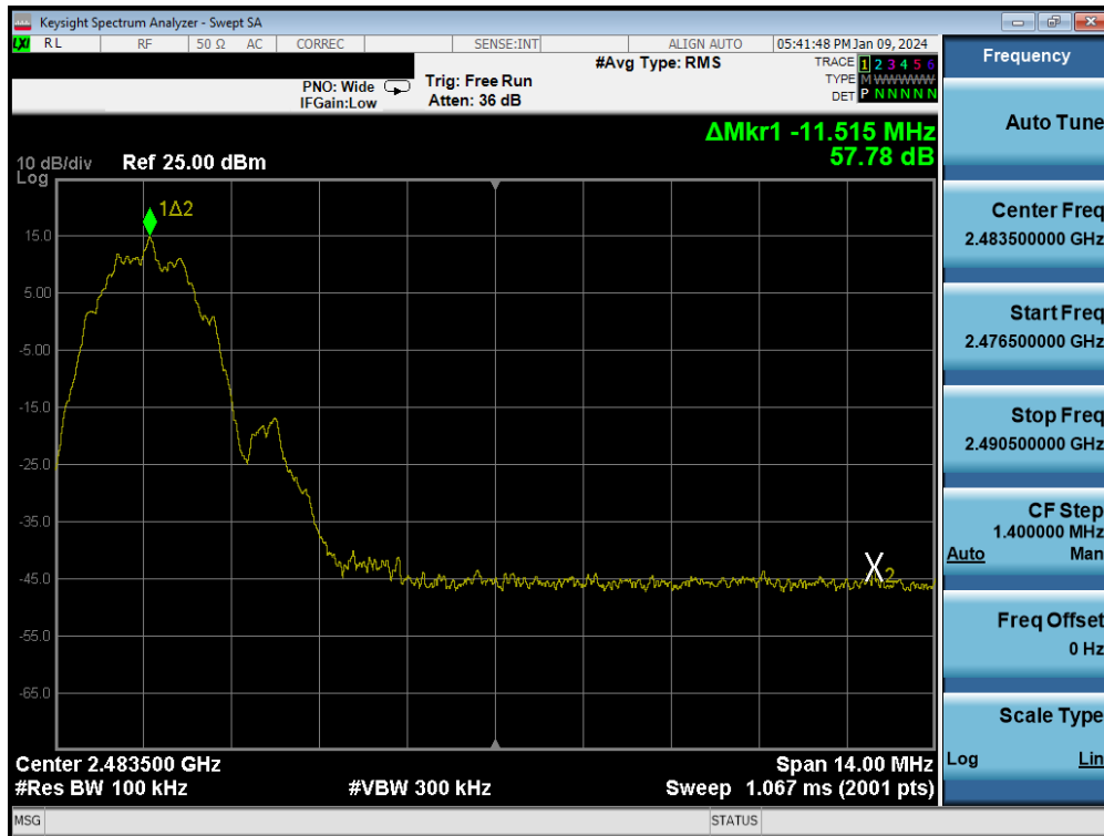
Plot 7-134. Band Edge Plot (Bluetooth (LE), 2Mbps – Ch. 36)
