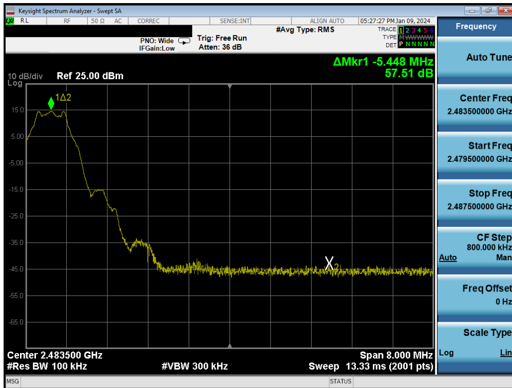
Plot 7-132. Band Edge Plot (Bluetooth (LE), 1Mbps – Ch. 39)
