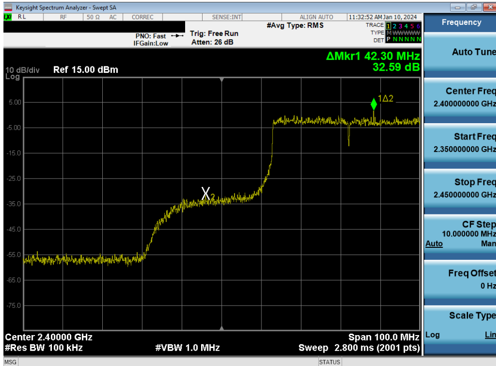
Plot 7-100. Band Edge Plot MIMO ANT2 (802.11be OFDMA – 484 Tones – Ch. 5)
