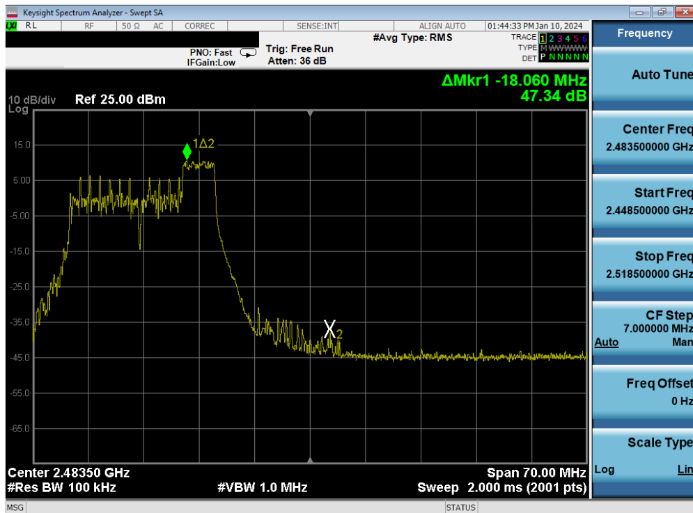
Plot 7-57. Band Edge Plot MIMO ANT1 (802.11be OFDMA – 52 Tones – Ch. 11)
