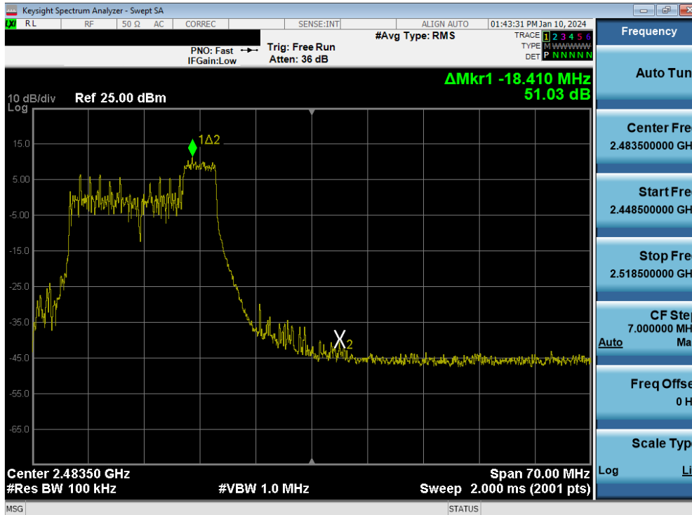
Plot 7-84. Band Edge Plot MIMO ANT2 (802.11be OFDMA – 52 Tones – Ch. 11)
