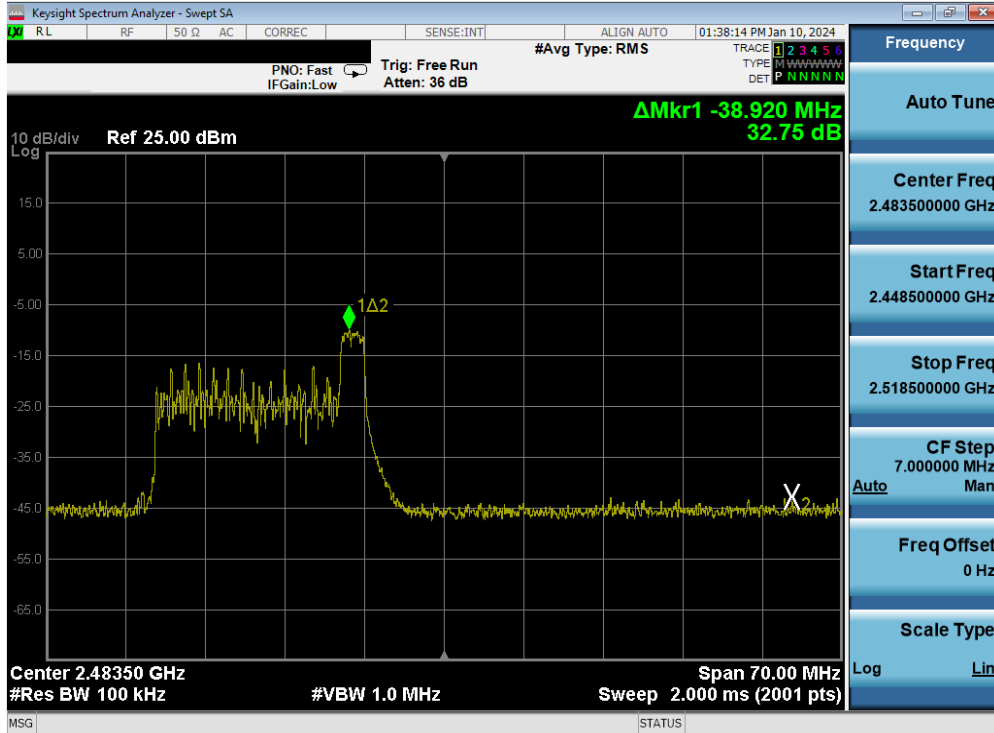
Plot 7-81. Band Edge Plot MIMO ANT2 (802.11be OFDMA – 26 Tones – Ch. 12)
