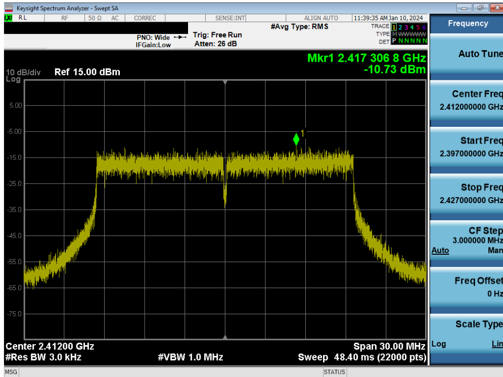
Plot 7-29. Power Spectral Density Plot MIMO ANT1 (802.11be OFDMA – 242 Tones – Ch. 1)
