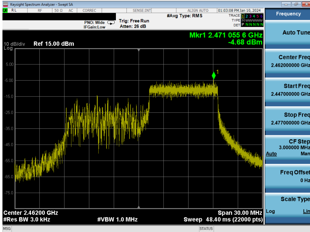
Plot 7-43. Power Spectral Density Plot MIMO ANT2 (802.11be OFDMA – 106 Tones – Ch. 11)
