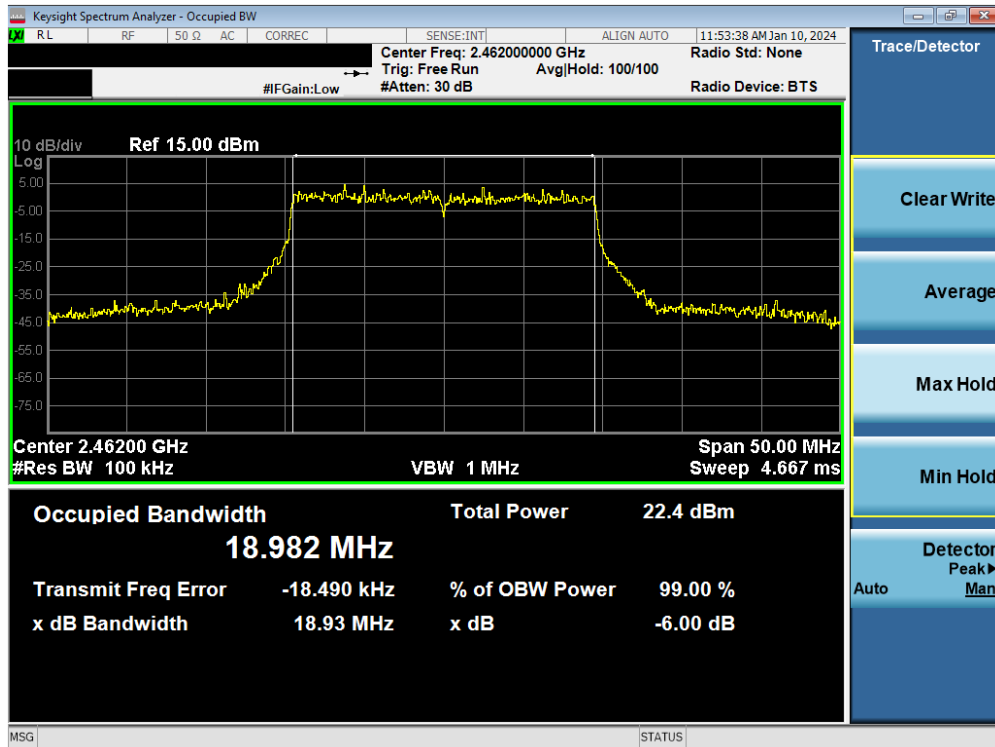
Plot 7-16. 6dB Bandwidth Plot MIMO ANT2 (802.11be OFDMA – 242 Tones – Ch. 11)
