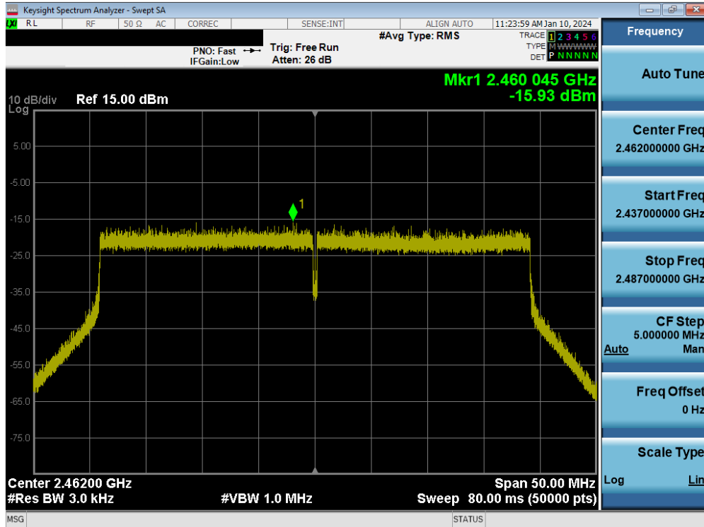
Plot 7-49. Power Spectral Density Plot MIMO ANT2 (802.11be OFDMA – 484 Tones – Ch. 11)
