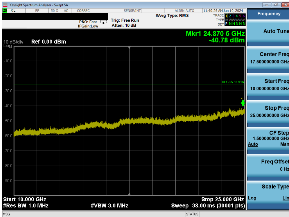
Plot 7-111. Conducted Spurious Plot MIMO ANT1 (802.11be OFDMA – 242 Tones – Ch. 1)
