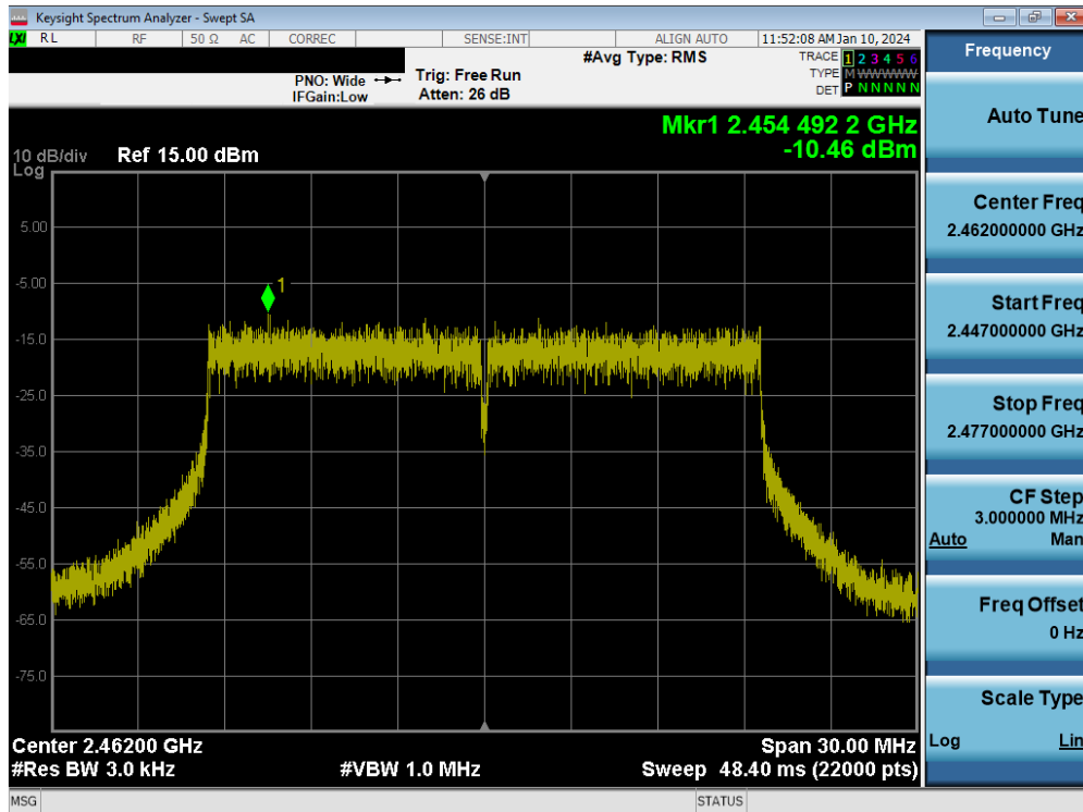
Plot 7-31. Power Spectral Density Plot MIMO ANT1 (802.11be OFDMA – 242 Tones – Ch. 11)
