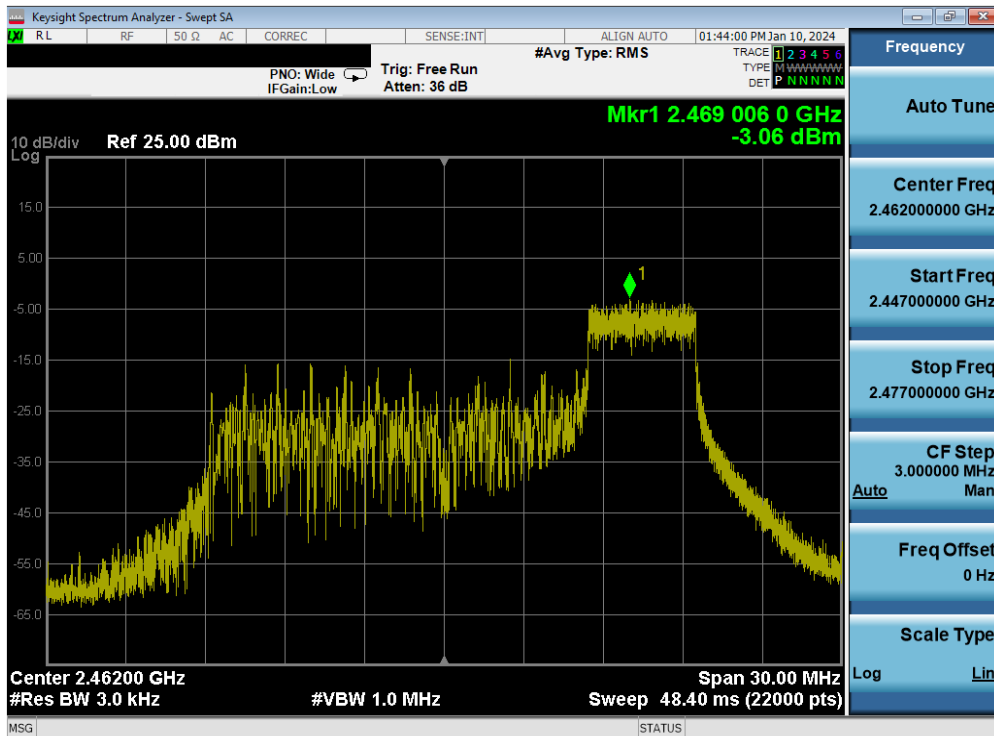
Plot 7-25. Power Spectral Density Plot MIMO ANT1 (802.11be OFDMA – 52 Tones – Ch. 11)
