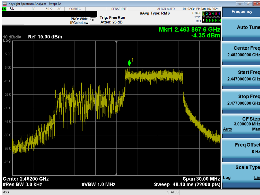
Plot 7-28. Power Spectral Density Plot MIMO ANT1 (802.11be OFDMA – 106 Tones – Ch. 11)
