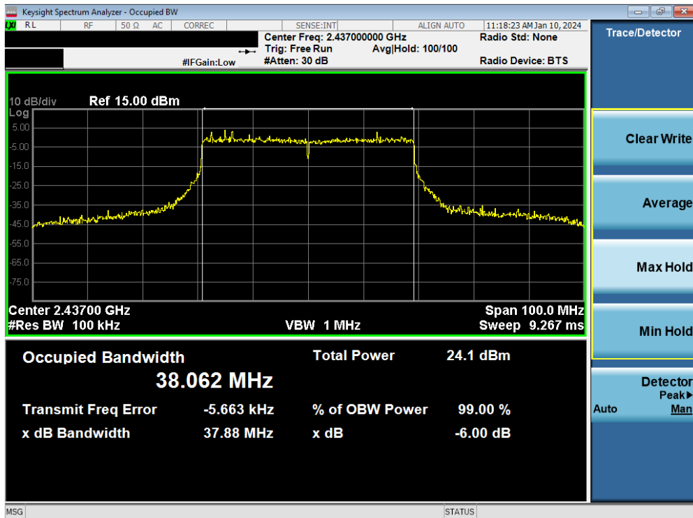
Plot 7-18. 6dB Bandwidth Plot MIMO ANT2 (802.11be OFDMA – 484 Tones – Ch. 6)
