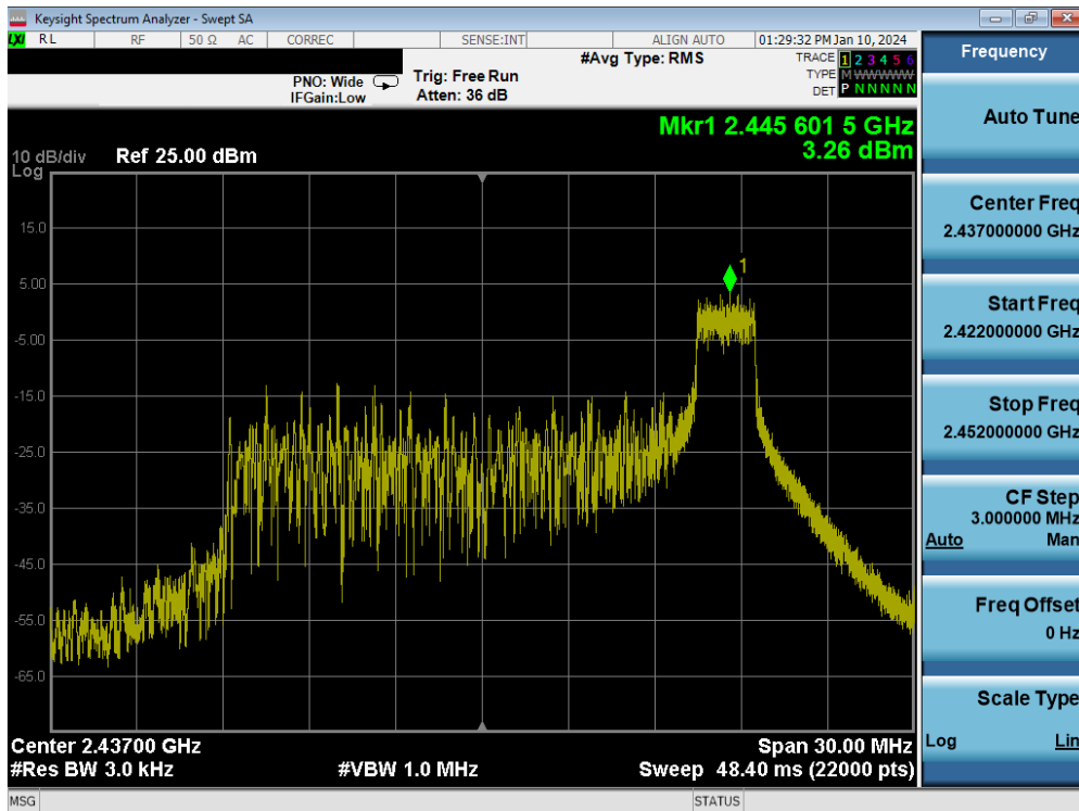
Plot 7-36. Power Spectral Density Plot MIMO ANT2 (802.11be OFDMA – 26 Tones – Ch. 6)
