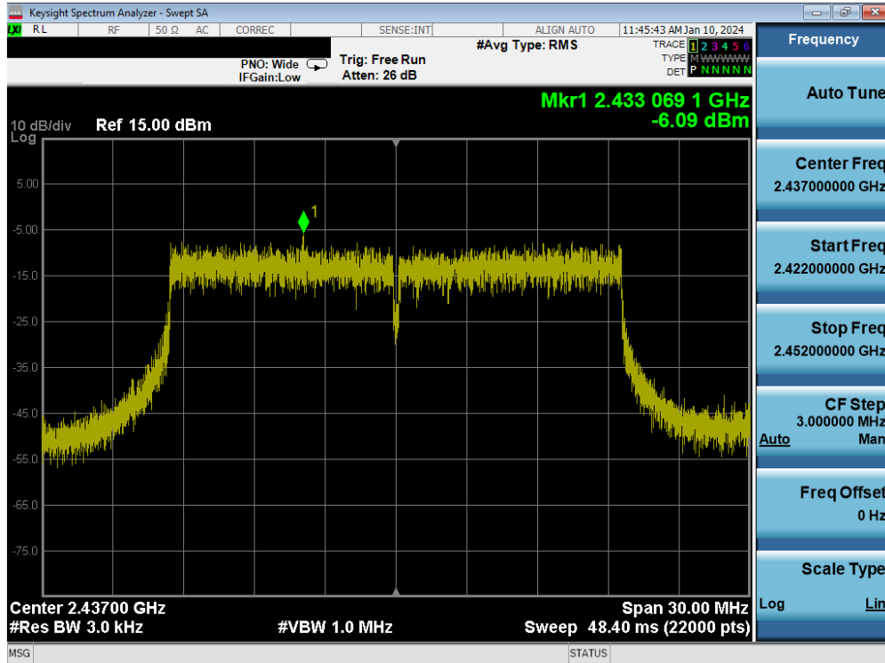
Plot 7-45. Power Spectral Density Plot MIMO ANT2 (802.11be OFDMA – 242 Tones – Ch. 6)
