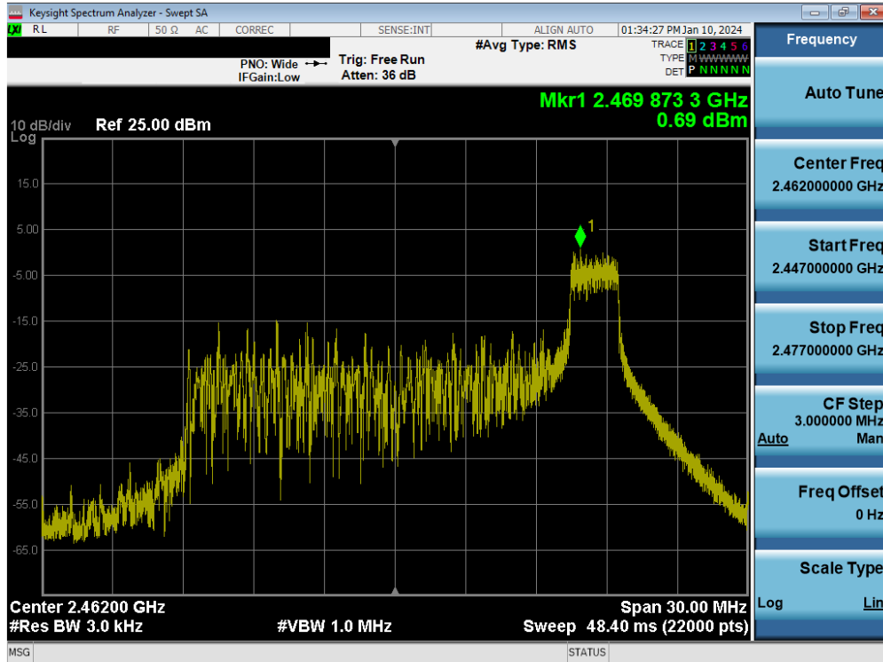
Plot 7-37. Power Spectral Density Plot MIMO ANT2 (802.11be OFDMA – 26 Tones – Ch. 11)
