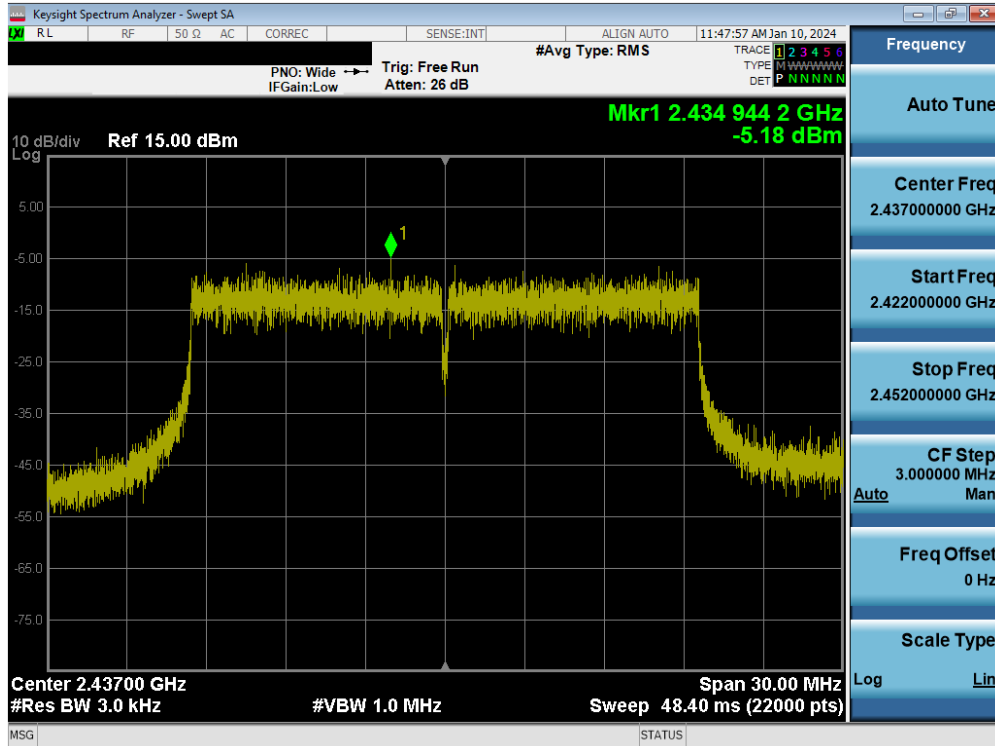
Plot 7-30. Power Spectral Density Plot MIMO ANT1 (802.11be OFDMA – 242 Tones – Ch. 6)
