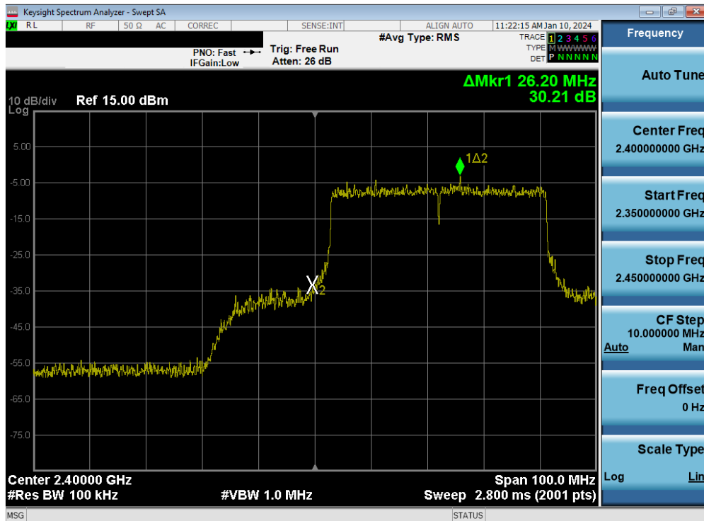
Plot 7-98. Band Edge Plot MIMO ANT2 (802.11be OFDMA – 484 Tones – Ch. 3)
