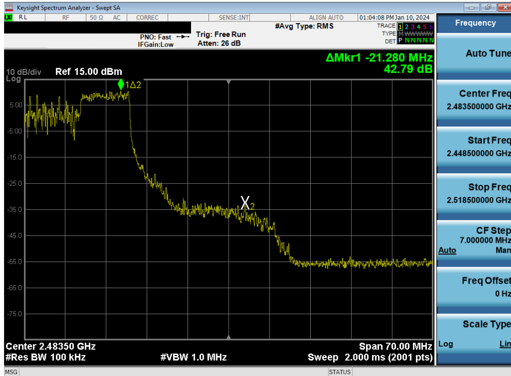
Plot 7-87. Band Edge Plot MIMO ANT2 (802.11be OFDMA – 106 Tones – Ch. 10)
