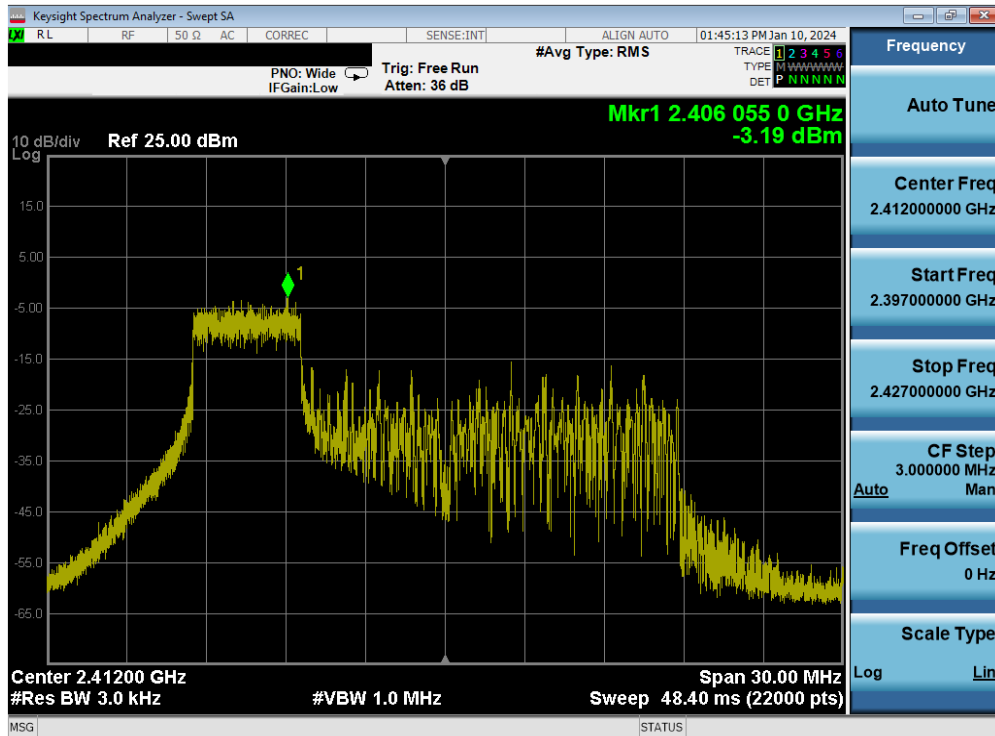
Plot 7-23. Power Spectral Density Plot MIMO ANT1 (802.11be OFDMA – 52 Tones – Ch. 1)
