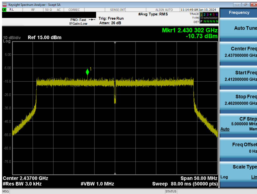
Plot 7-33. Power Spectral Density Plot MIMO ANT1 (802.11be OFDMA – 484 Tones – Ch. 6)
