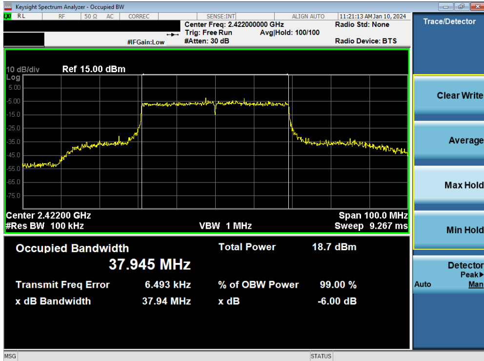
Plot 7-17. 6dB Bandwidth Plot MIMO ANT2 (802.11be OFDMA – 484 Tones – Ch. 3)
