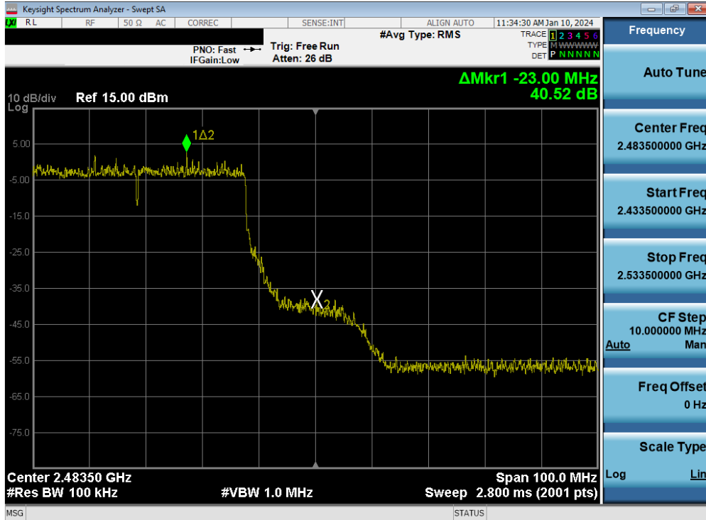
Plot 7-74. Band Edge Plot MIMO ANT1 (802.11be OFDMA – 484 Tones – Ch. 9)
