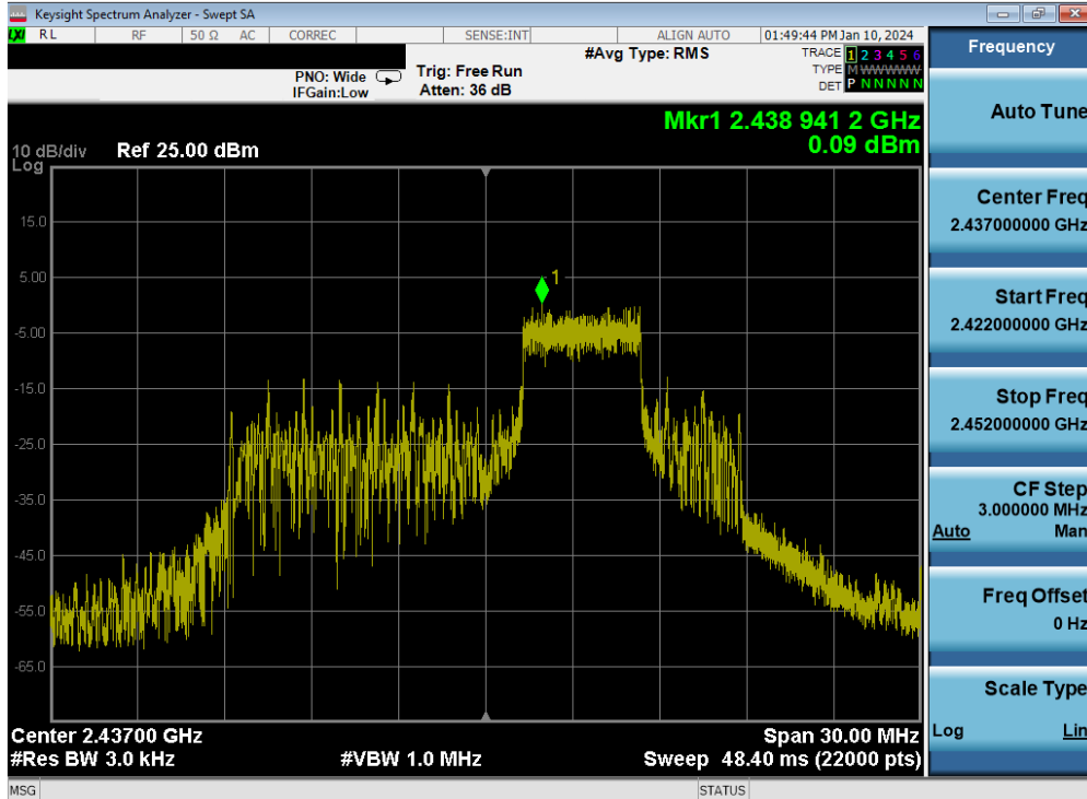
Plot 7-24. Power Spectral Density Plot MIMO ANT1 (802.11be OFDMA – 52 Tones – Ch. 6)
