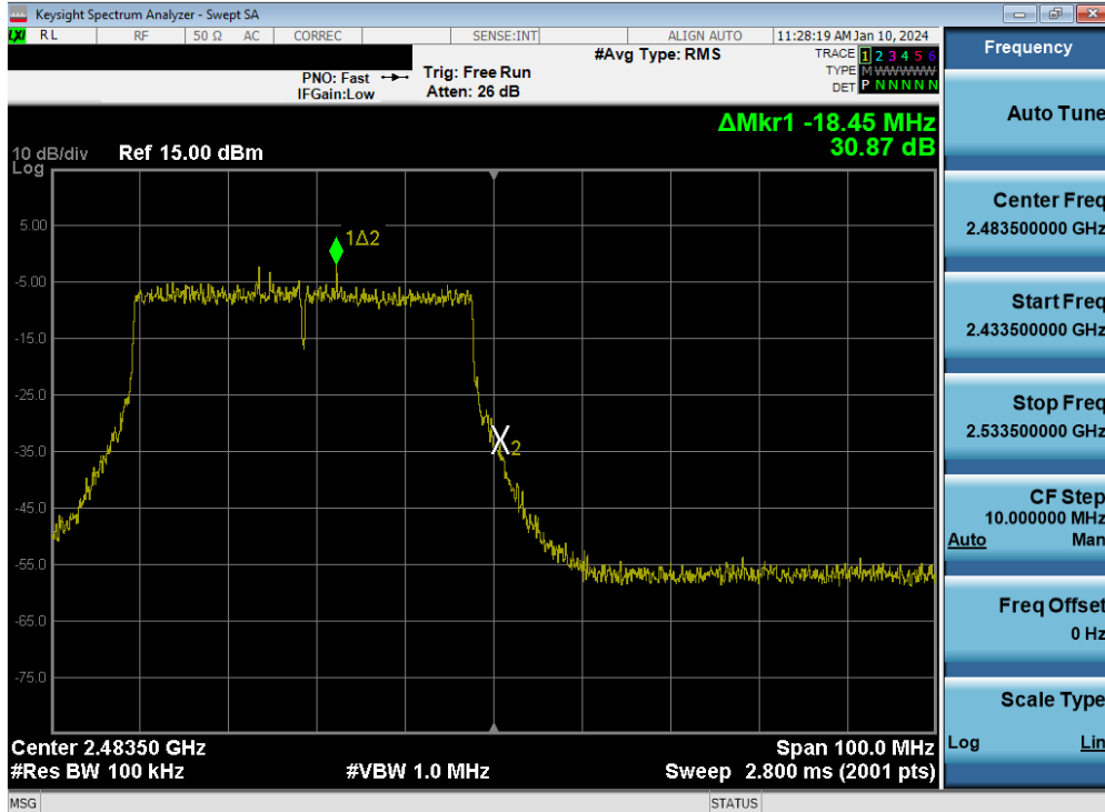
Plot 7-76. Band Edge Plot MIMO ANT1 (802.11be OFDMA – 484 Tones – Ch. 11)
