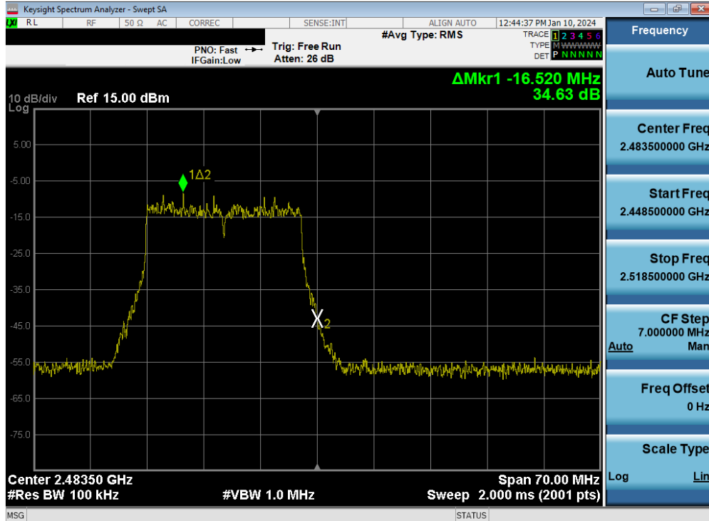
Plot 7-70. Band Edge Plot MIMO ANT1 (802.11be OFDMA – 242 Tones – Ch. 13)
