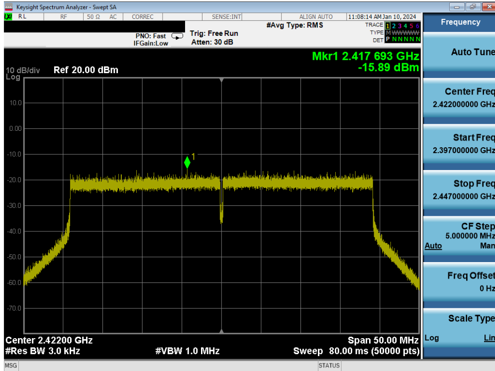
Plot 7-32. Power Spectral Density Plot MIMO ANT1 (802.11be OFDMA – 484 Tones – Ch. 3)
