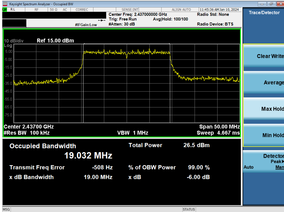
Plot 7-15. 6dB Bandwidth Plot MIMO ANT2 (802.11be OFDMA – 242 Tones – Ch. 6)
