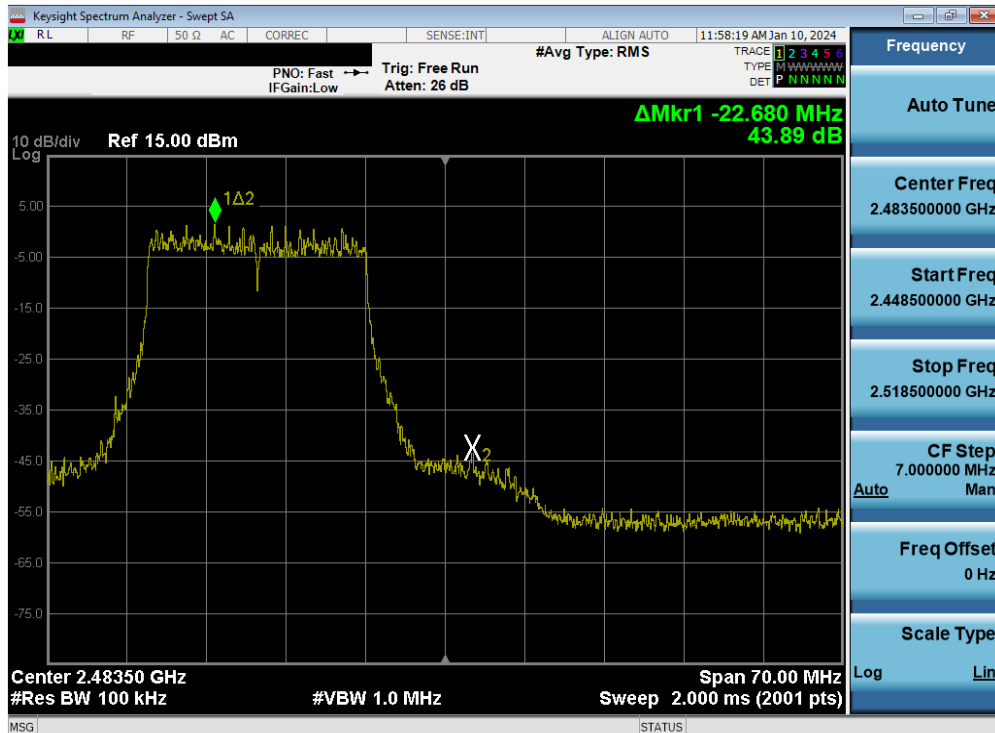
Plot 7-96. Band Edge Plot MIMO ANT2 (802.11be OFDMA – 242 Tones – Ch. 12)
