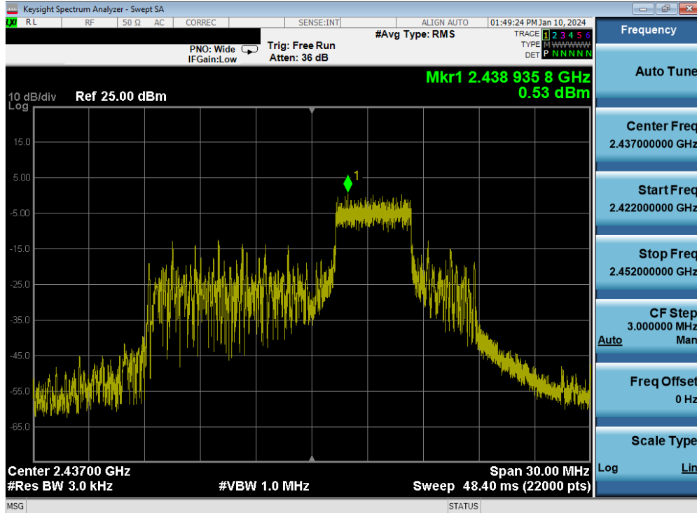
Plot 7-39. Power Spectral Density Plot MIMO ANT2 (802.11be OFDMA – 52 Tones – Ch. 6)
