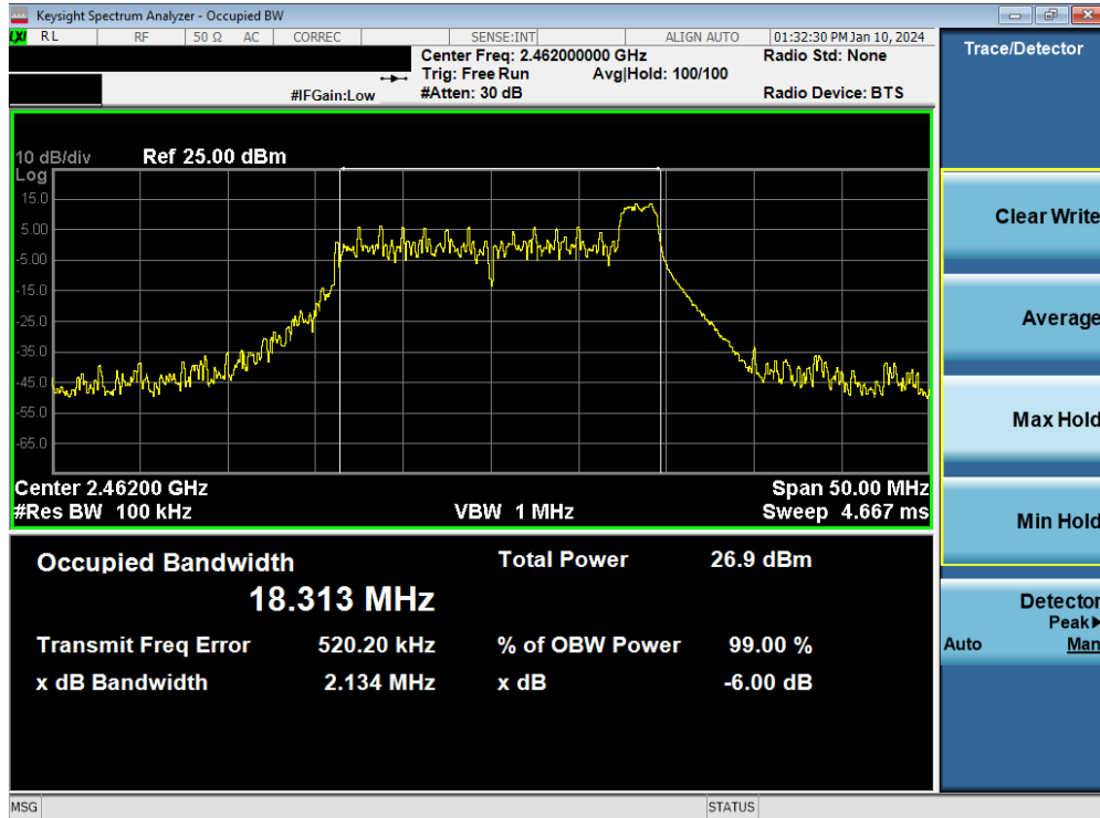
Plot 7-4. 6dB Bandwidth Plot MIMO ANT1 (802.11be OFDMA – 26 Tones – Ch. 11)
