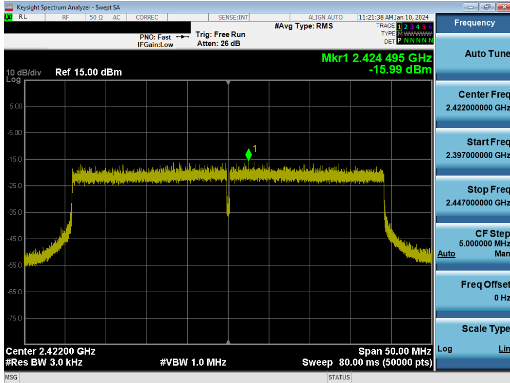
Plot 7-47. Power Spectral Density Plot MIMO ANT2 (802.11be OFDMA – 484 Tones – Ch. 3)
