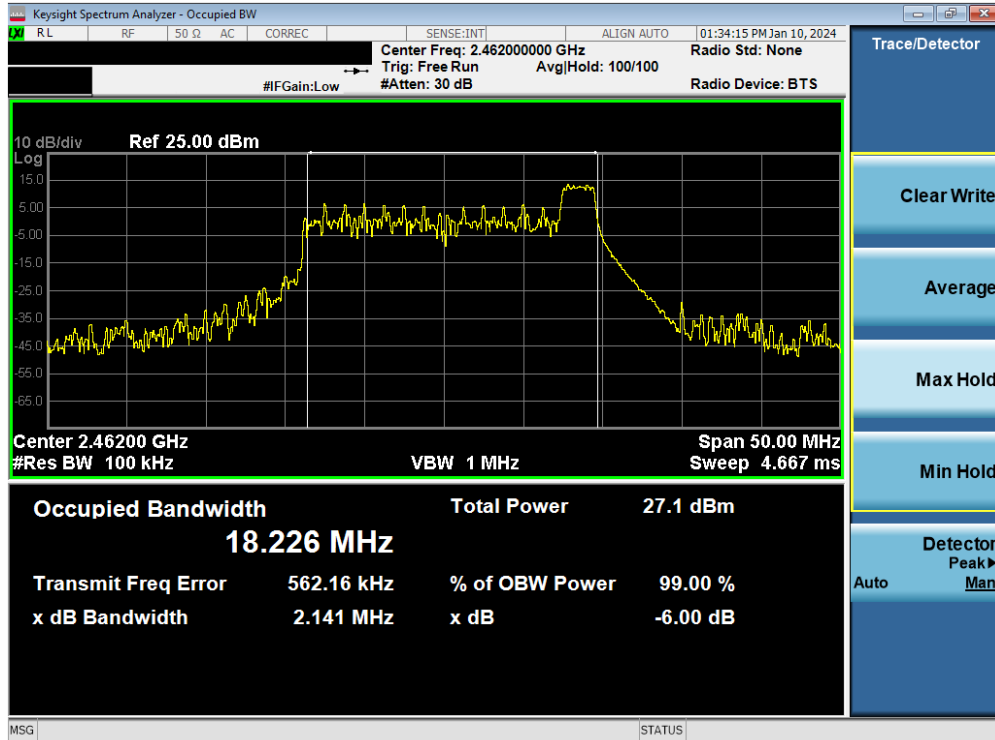
Plot 7-13. 6dB Bandwidth Plot MIMO ANT2 (802.11be OFDMA – 26 Tones – Ch. 11)
