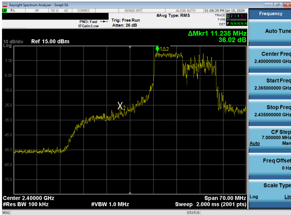
Plot 7-86. Band Edge Plot MIMO ANT2 (802.11be OFDMA – 106 Tones – Ch. 2)
