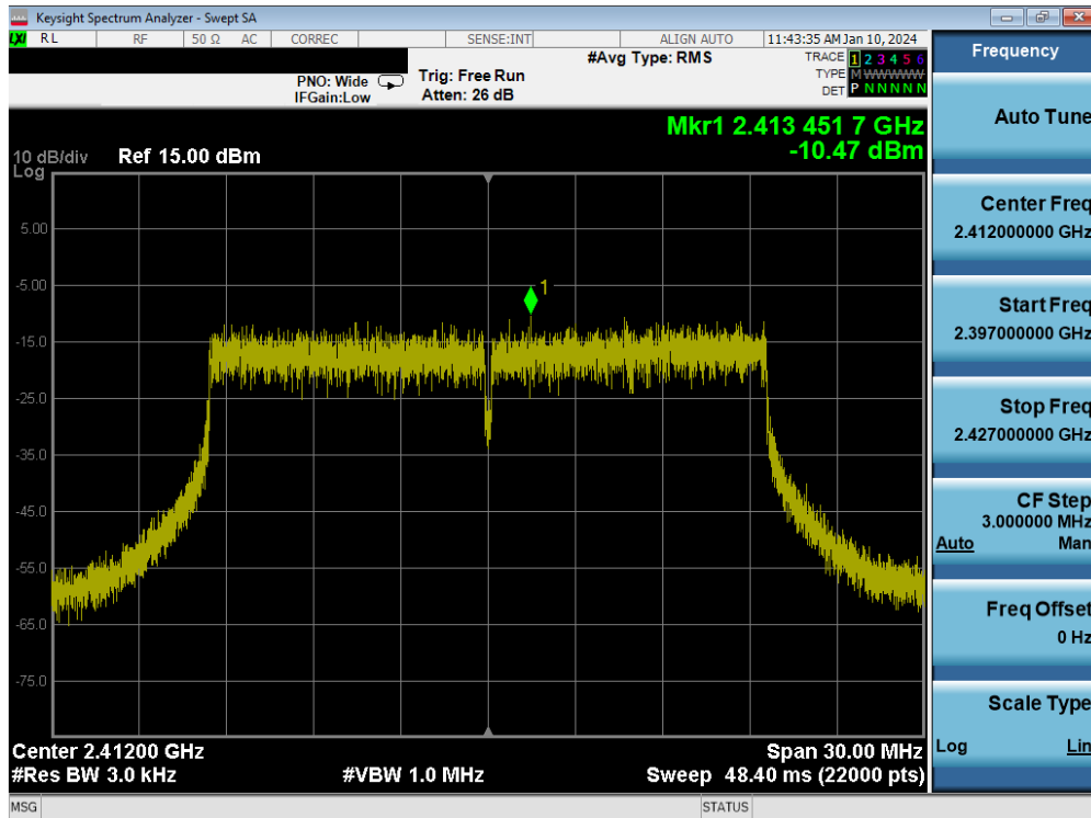
Plot 7-44. Power Spectral Density Plot MIMO ANT2 (802.11be OFDMA – 242 Tones – Ch. 1)
