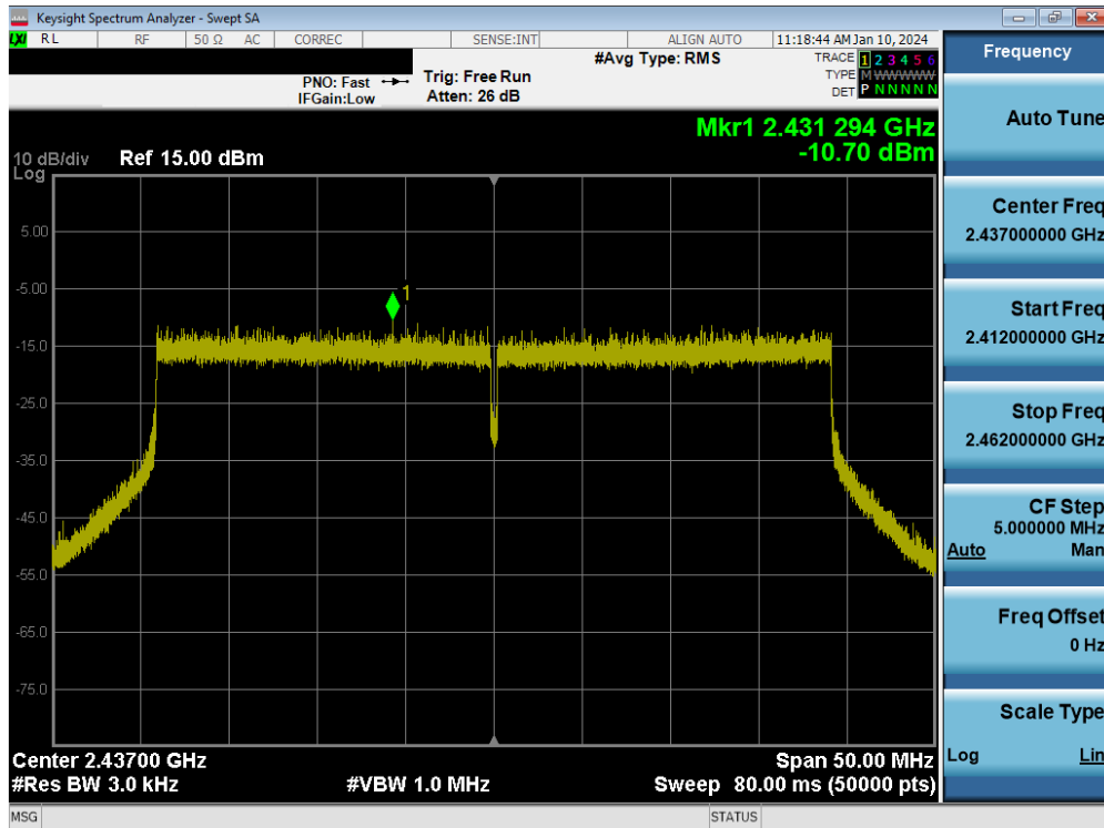
Plot 7-48. Power Spectral Density Plot MIMO ANT2 (802.11be OFDMA – 484 Tones – Ch. 6)
