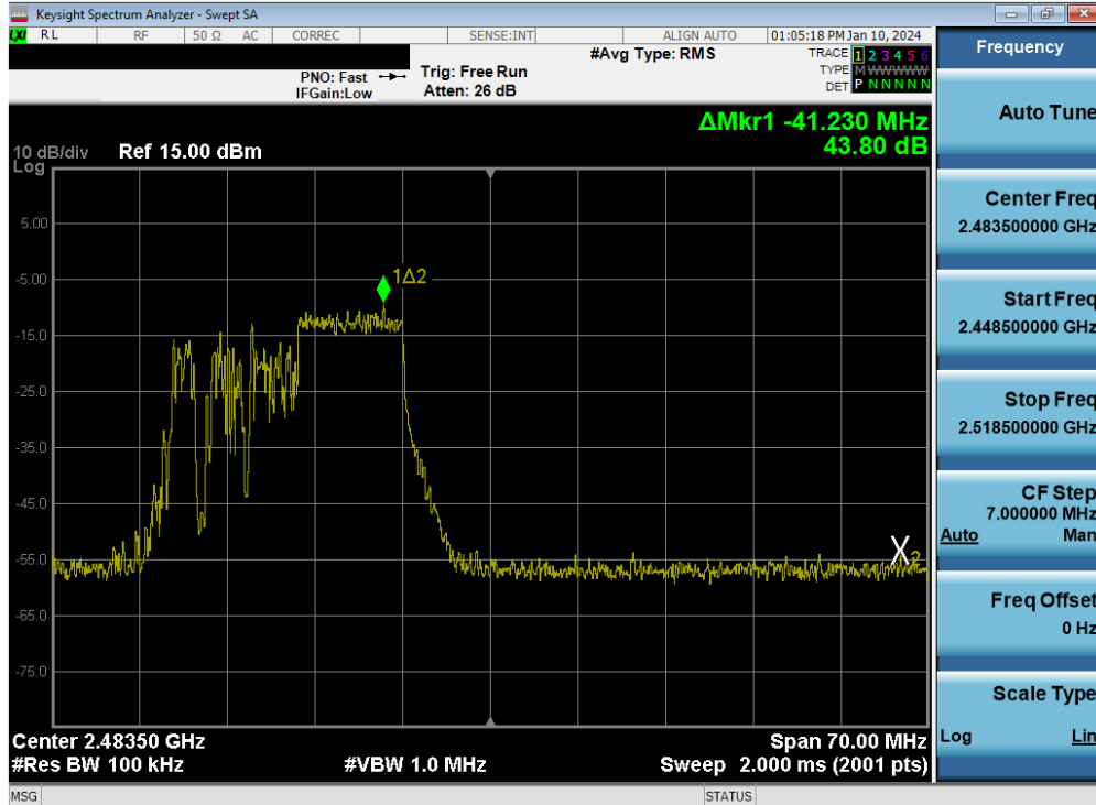
Plot 7-62. Band Edge Plot MIMO ANT1 (802.11be OFDMA – 106 Tones – Ch. 12)
