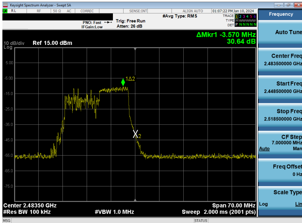
Plot 7-63. Band Edge Plot MIMO ANT1 (802.11be OFDMA – 106 Tones – Ch. 13)
