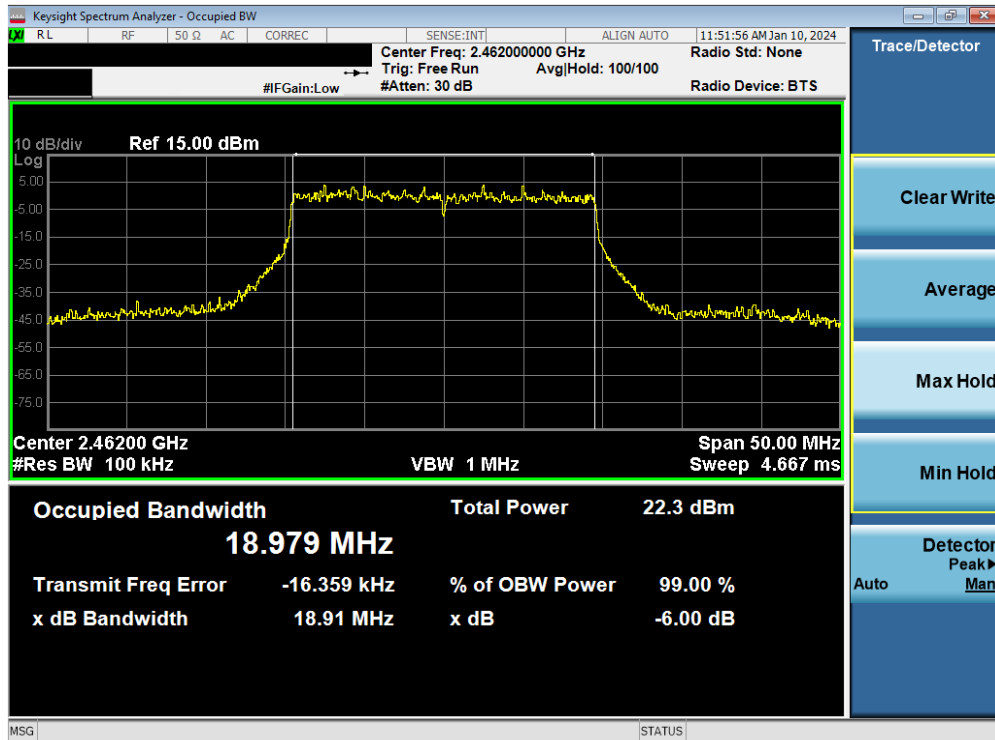
Plot 7-7. 6dB Bandwidth Plot MIMO ANT1 (802.11be OFDMA – 242 Tones – Ch. 11)
