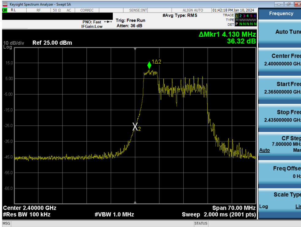
Plot 7-83. Band Edge Plot MIMO ANT2 (802.11be OFDMA – 52 Tones – Ch. 1)
