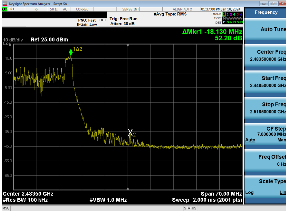
Plot 7-52. Band Edge Plot MIMO ANT1 (802.11be OFDMA – 26 Tones – Ch. 10)
