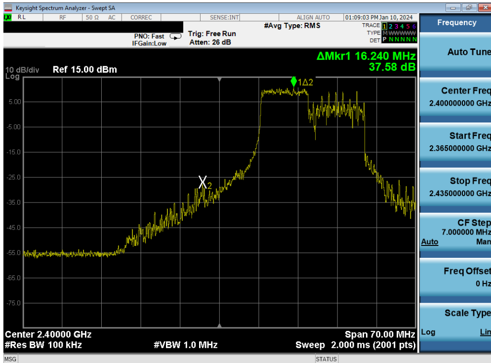
Plot 7-59. Band Edge Plot MIMO ANT1 (802.11be OFDMA – 106 Tones – Ch. 2)
