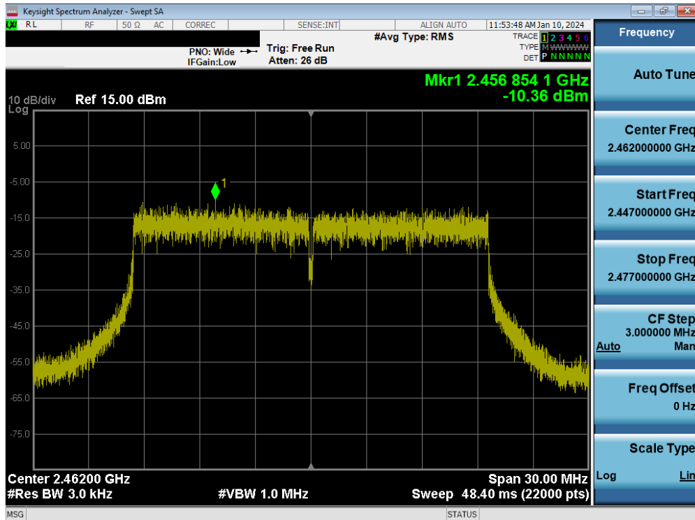
Plot 7-46. Power Spectral Density Plot MIMO ANT2 (802.11be OFDMA – 242 Tones – Ch. 11)
