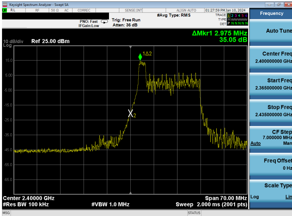
Plot 7-77. Band Edge Plot MIMO ANT2 (802.11be OFDMA – 26 Tones – Ch. 1)
