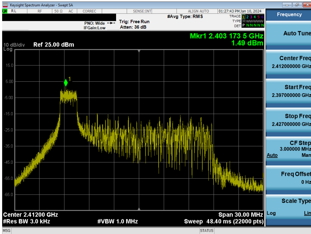
Plot 7-35. Power Spectral Density Plot MIMO ANT2 (802.11be OFDMA – 26 Tones – Ch. 1)
