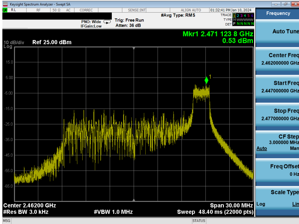
Plot 7-22. Power Spectral Density Plot MIMO ANT1 (802.11be OFDMA – 26 Tones – Ch. 11)
