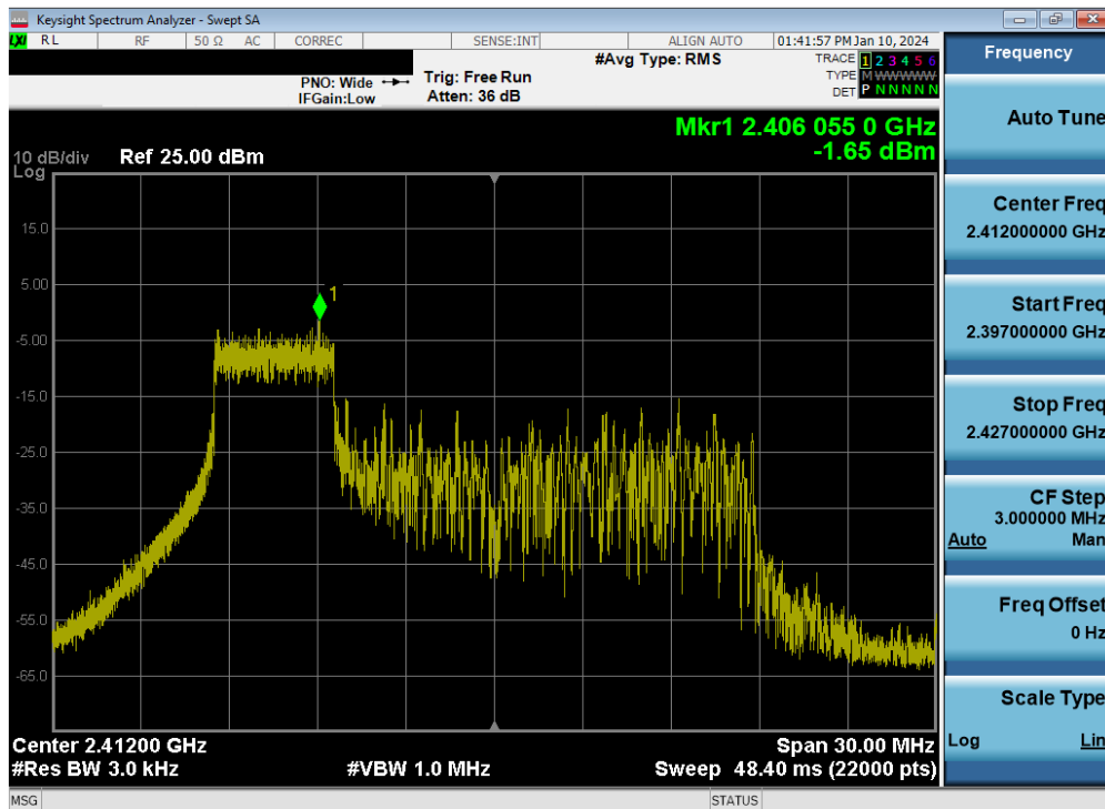
Plot 7-38. Power Spectral Density Plot MIMO ANT2 (802.11be OFDMA – 52 Tones – Ch. 1)
