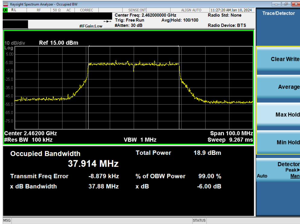
Plot 7-10. 6dB Bandwidth Plot MIMO ANT1 (802.11be OFDMA – 484 Tones – Ch. 11)
