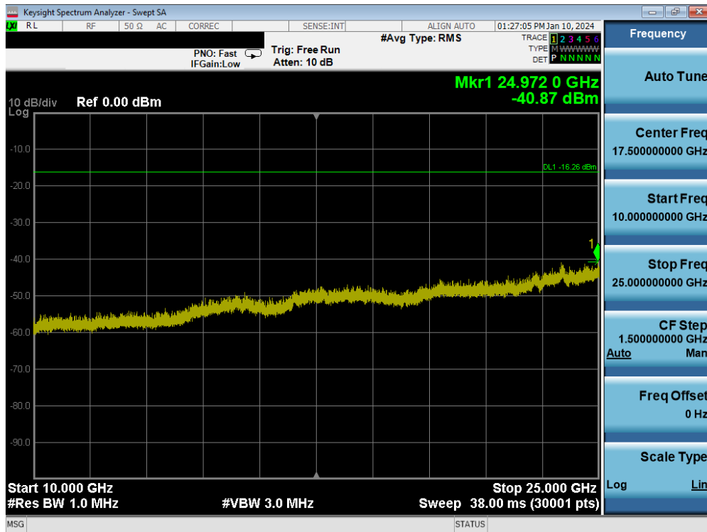
Plot 7-105. Conducted Spurious Plot MIMO ANT1 (802.11be OFDMA – 26 Tones – Ch. 1)
