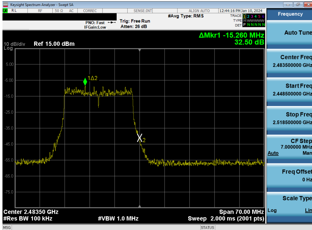
Plot 7-97. Band Edge Plot MIMO ANT2 (802.11be OFDMA – 242 Tones – Ch. 13)
