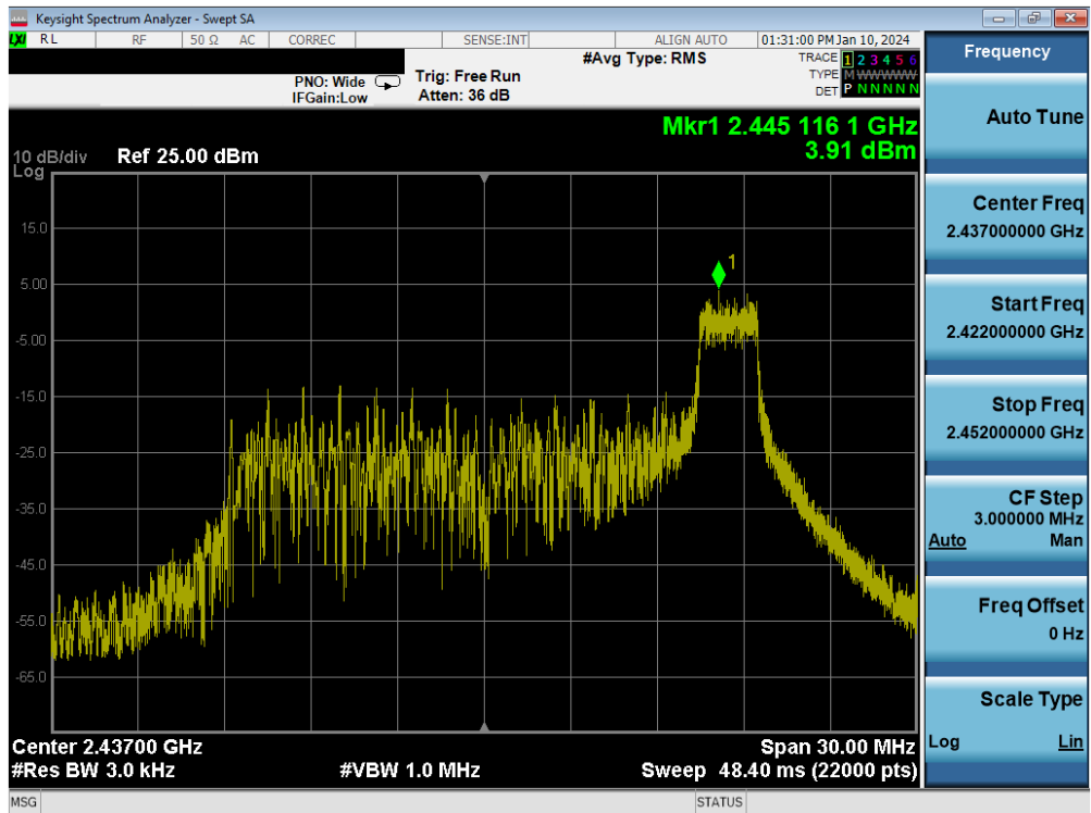
Plot 7-21. Power Spectral Density Plot MIMO ANT1 (802.11be OFDMA – 26 Tones – Ch. 6)
