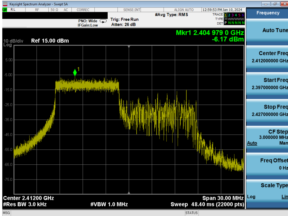
Plot 7-41. Power Spectral Density Plot MIMO ANT2 (802.11be OFDMA – 106 Tones – Ch. 1)
