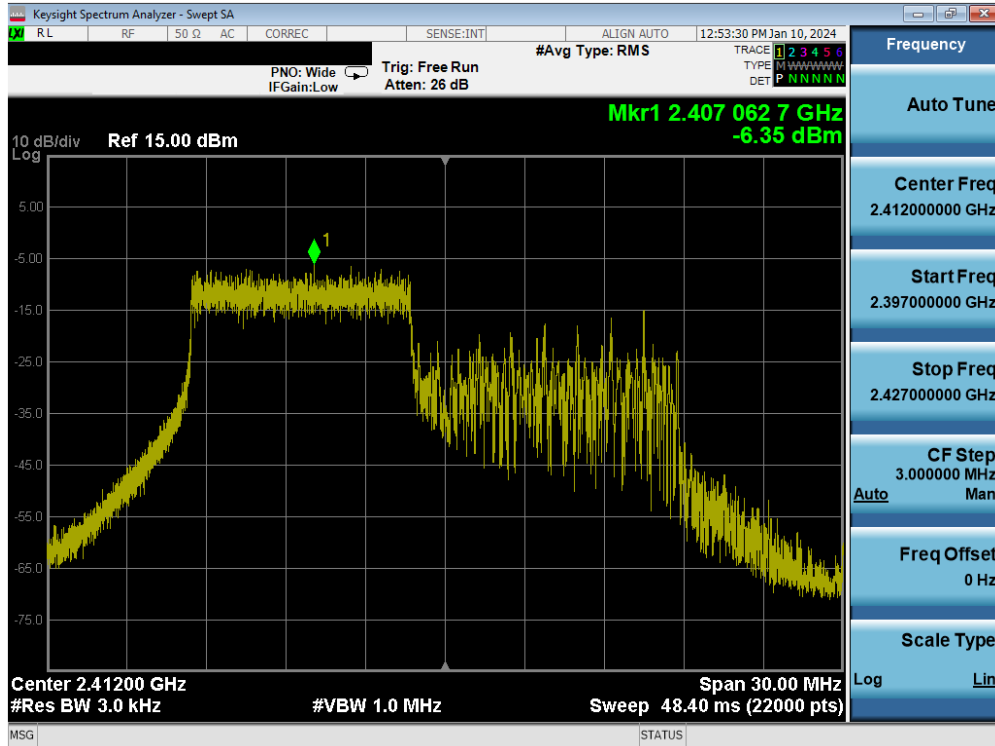
Plot 7-26. Power Spectral Density Plot MIMO ANT1 (802.11be OFDMA – 106 Tones – Ch. 1)
