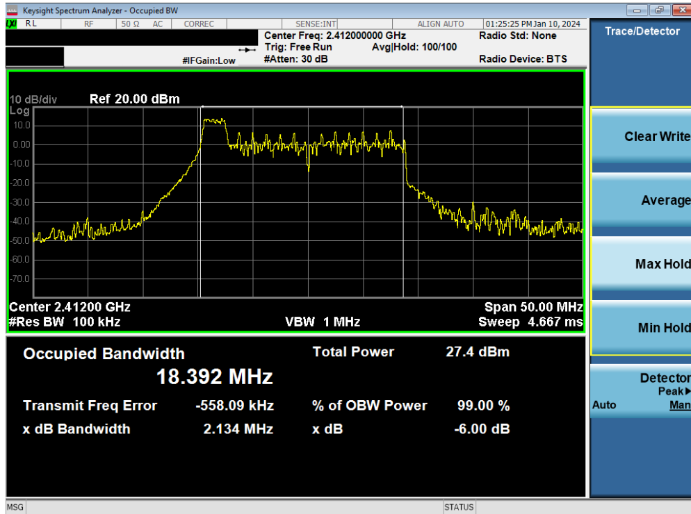
Plot 7-2. 6dB Bandwidth Plot MIMO ANT1 (802.11be OFDMA – 26 Tones – Ch. 1)
