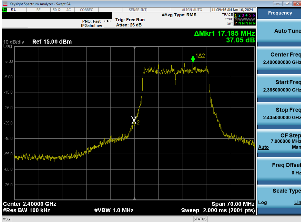
Plot 7-64. Band Edge Plot MIMO ANT1 (802.11be OFDMA – 242 Tones – Ch. 1)
