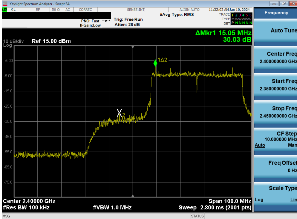
Plot 7-99. Band Edge Plot MIMO ANT2 (802.11be OFDMA – 484 Tones – Ch. 4)
