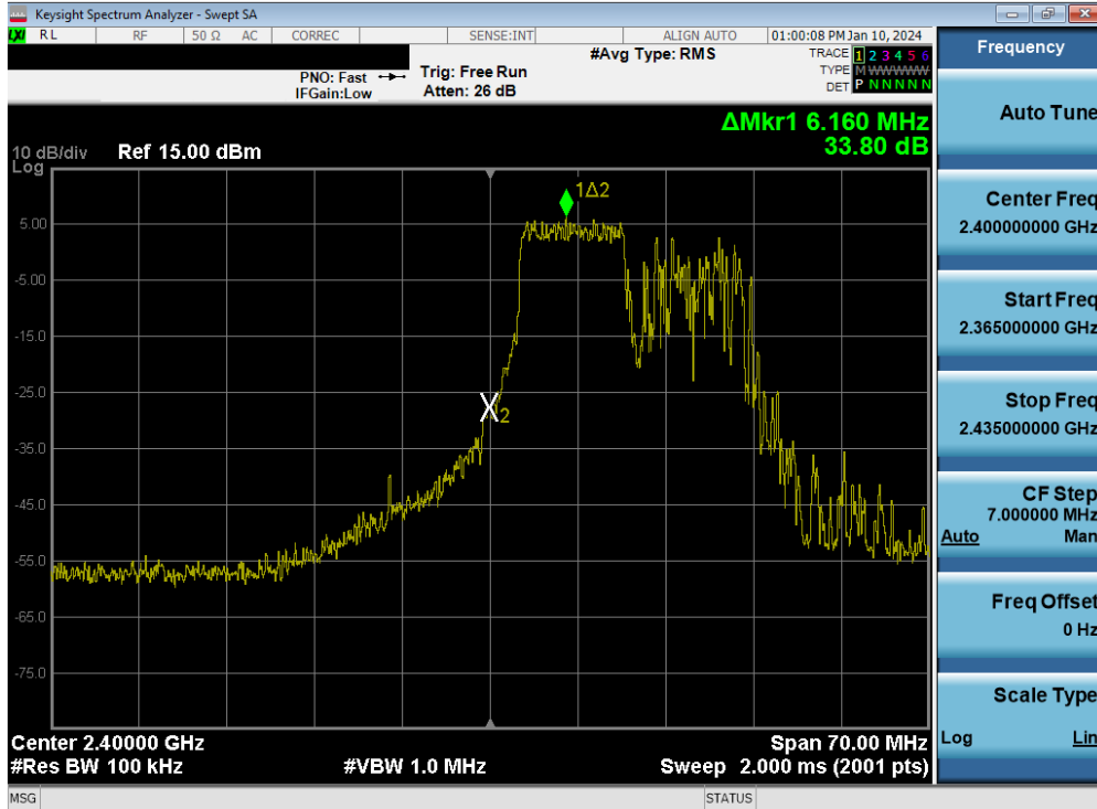
Plot 7-85. Band Edge Plot MIMO ANT2 (802.11be OFDMA – 106 Tones – Ch. 1)
