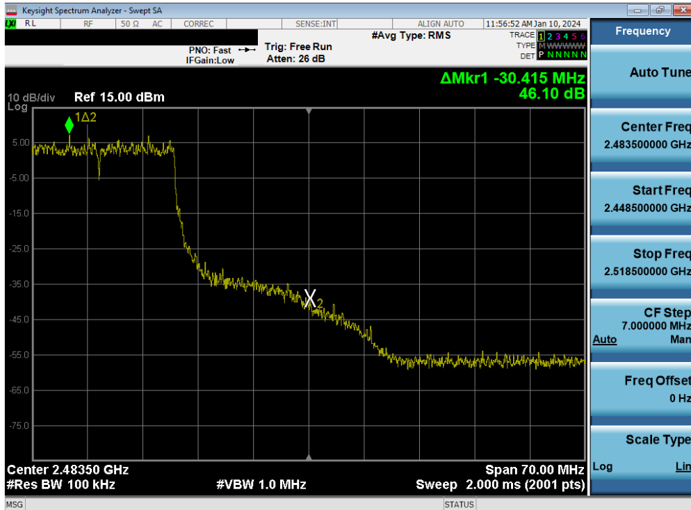
Plot 7-67. Band Edge Plot MIMO ANT1 (802.11be OFDMA – 242 Tones – Ch. 10)
