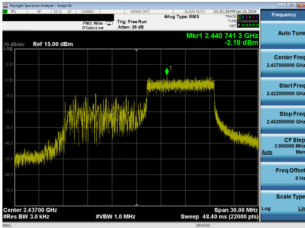
Plot 7-27. Power Spectral Density Plot MIMO ANT1 (802.11be OFDMA – 106 Tones – Ch. 6)
