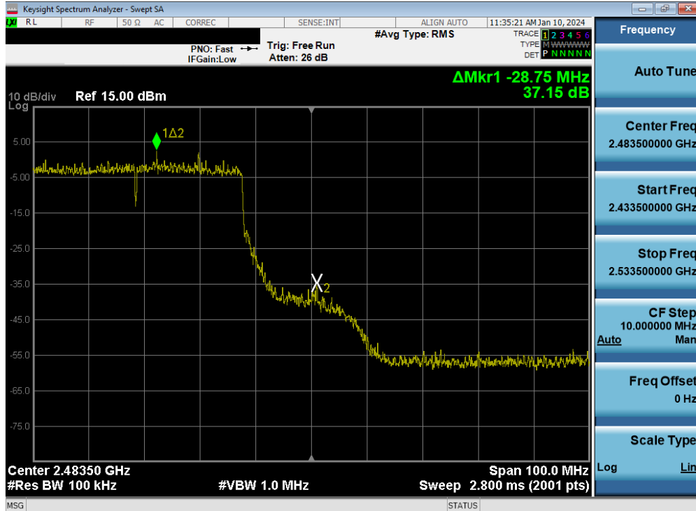
Plot 7-101. Band Edge Plot MIMO ANT2 (802.11be OFDMA – 484 Tones – Ch. 9)
