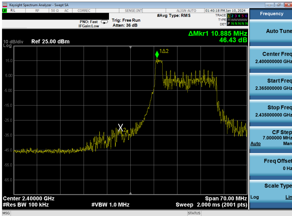
Plot 7-78. Band Edge Plot MIMO ANT2 (802.11be OFDMA – 26 Tones – Ch. 2)
