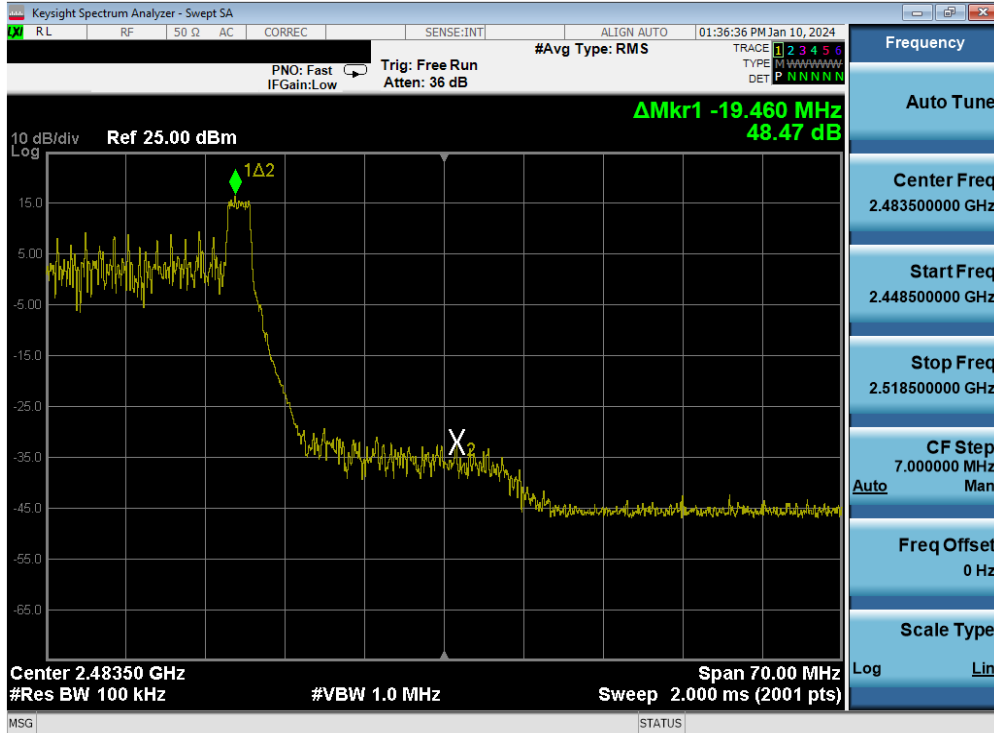
Plot 7-79. Band Edge Plot MIMO ANT2 (802.11be OFDMA – 26 Tones – Ch. 10)
