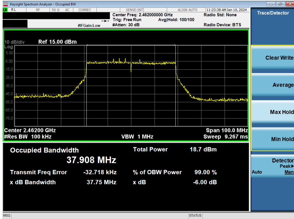
Plot 7-19. 6dB Bandwidth Plot MIMO ANT2 (802.11be OFDMA – 484 Tones – Ch. 11)
