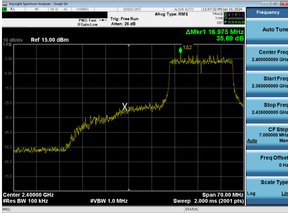
Plot 7-93. Band Edge Plot MIMO ANT2 (802.11be OFDMA – 242 Tones – Ch. 3)
