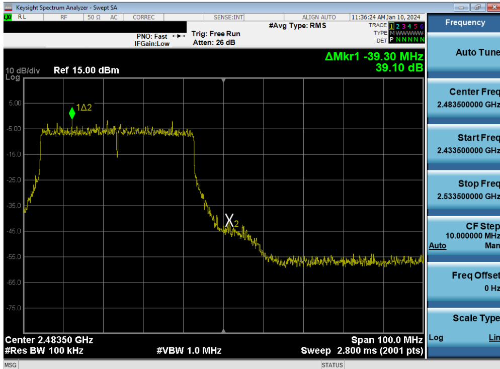
Plot 7-75. Band Edge Plot MIMO ANT1 (802.11be OFDMA – 484 Tones – Ch. 10)
