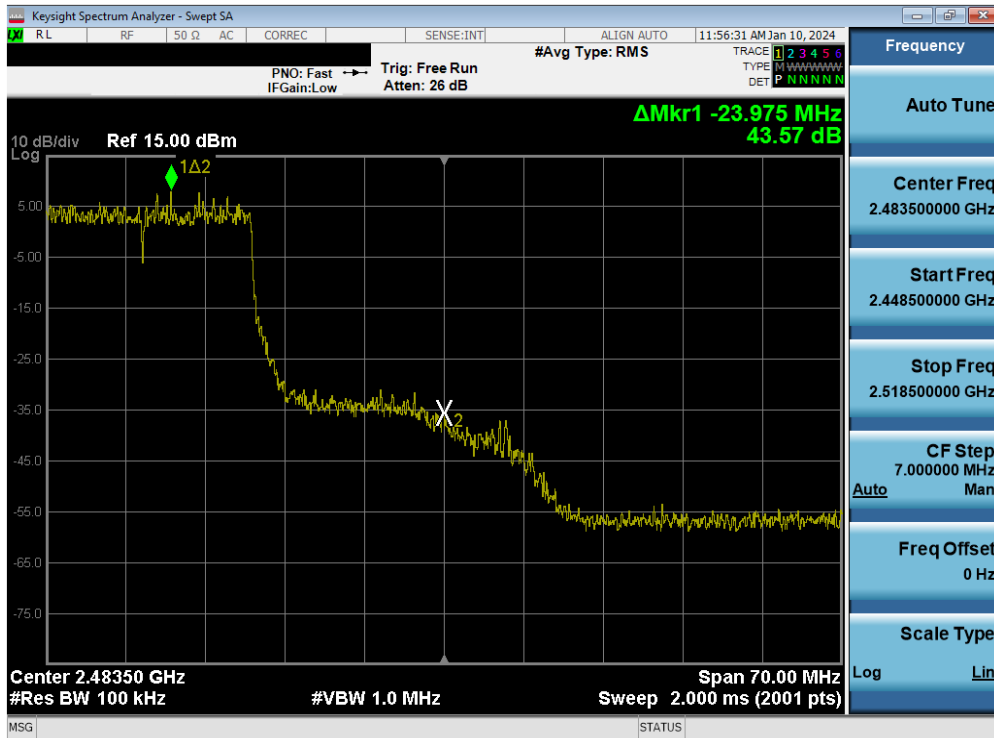
Plot 7-94. Band Edge Plot MIMO ANT2 (802.11be OFDMA – 242 Tones – Ch. 10)
