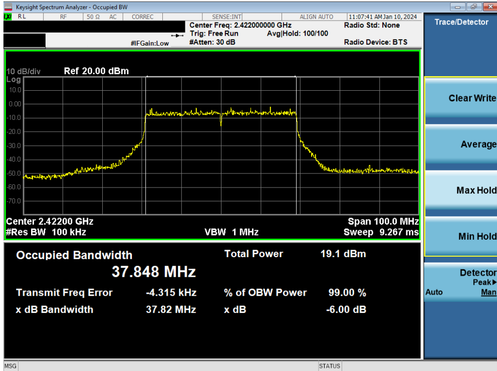
Plot 7-8. 6dB Bandwidth Plot MIMO ANT1 (802.11be OFDMA – 484 Tones – Ch. 3)
