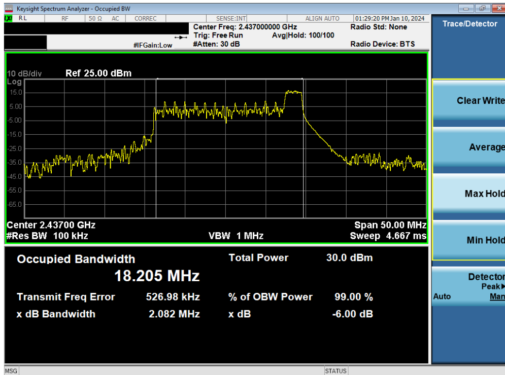
Plot 7-12. 6dB Bandwidth Plot MIMO ANT2 (802.11be OFDMA – 26 Tones – Ch. 6)
