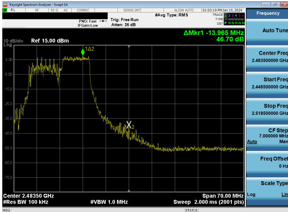
Plot 7-88. Band Edge Plot MIMO ANT2 (802.11be OFDMA – 106 Tones – Ch. 11)
