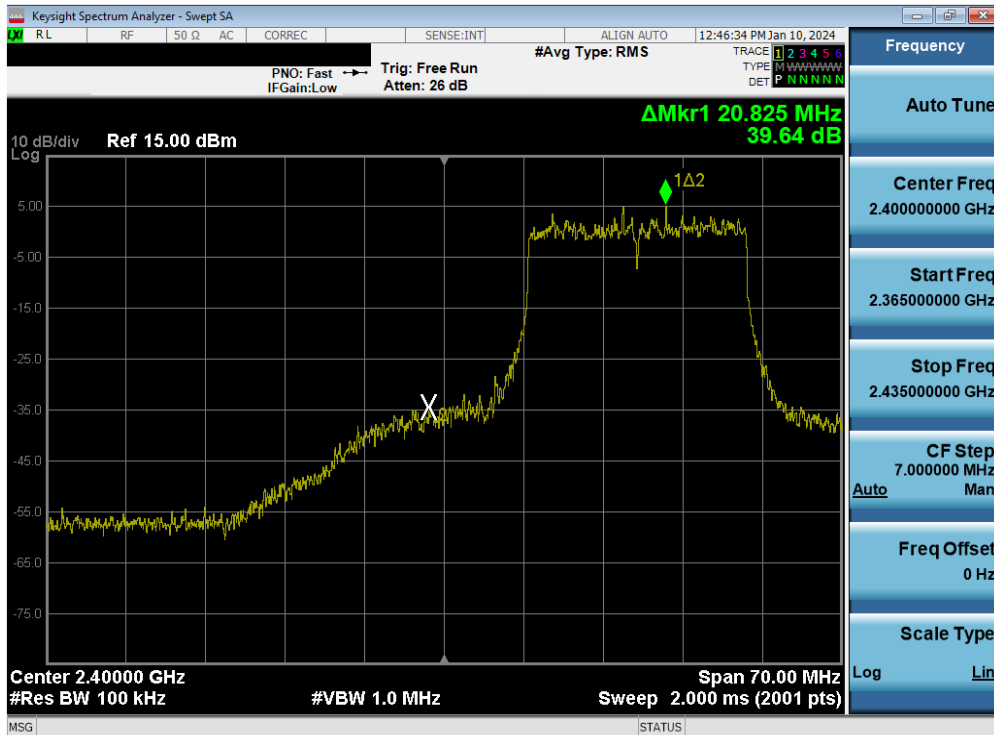
Plot 7-65. Band Edge Plot MIMO ANT1 (802.11be OFDMA – 242 Tones – Ch. 2)
