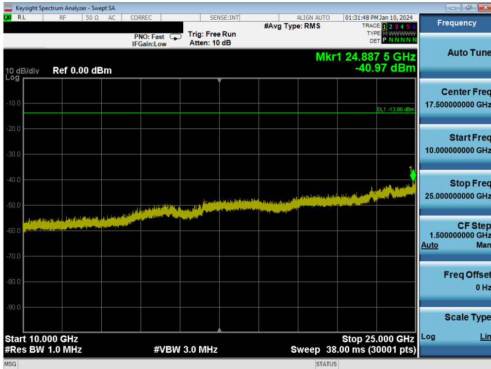
Plot 7-107. Conducted Spurious Plot MIMO ANT1 (802.11be OFDMA – 26 Tones – Ch. 6)
