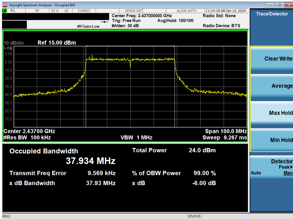
Plot 7-9. 6dB Bandwidth Plot MIMO ANT1 (802.11be OFDMA – 484 Tones – Ch. 6)
