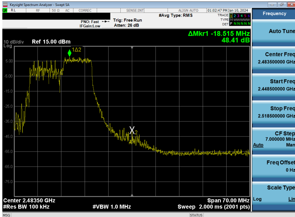
Plot 7-61. Band Edge Plot MIMO ANT1 (802.11be OFDMA – 106 Tones – Ch. 11)
