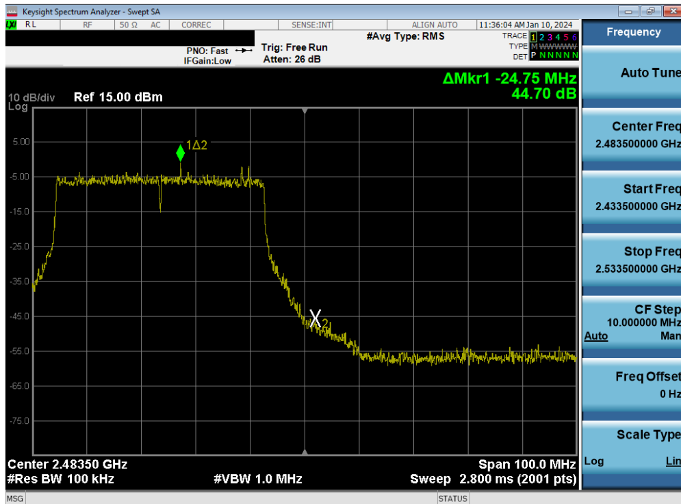
Plot 7-102. Band Edge Plot MIMO ANT2 (802.11be OFDMA – 484 Tones – Ch. 10)
