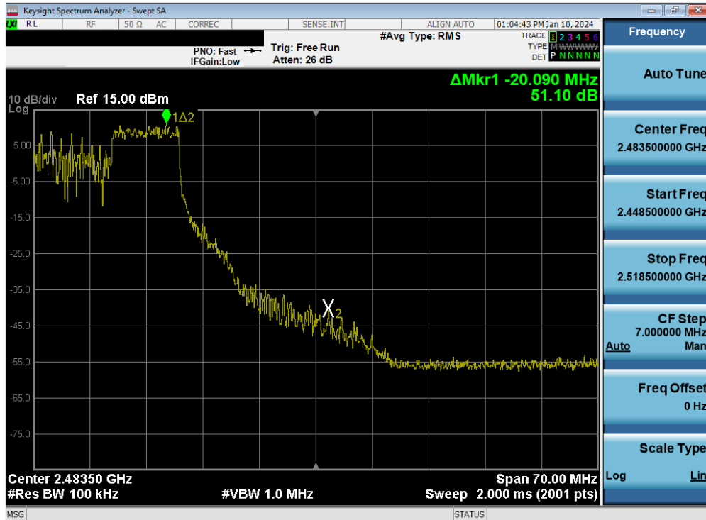
Plot 7-60. Band Edge Plot MIMO ANT1 (802.11be OFDMA – 106 Tones – Ch. 10)
