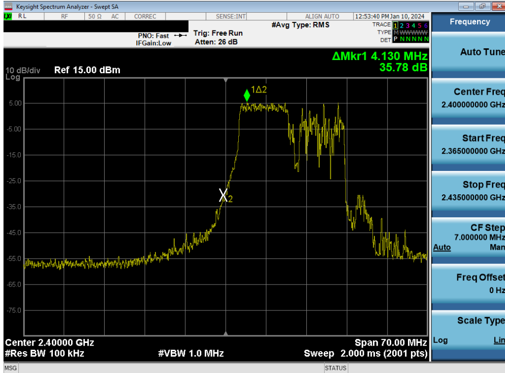
Plot 7-58. Band Edge Plot MIMO ANT1 (802.11be OFDMA – 106 Tones – Ch. 1)
