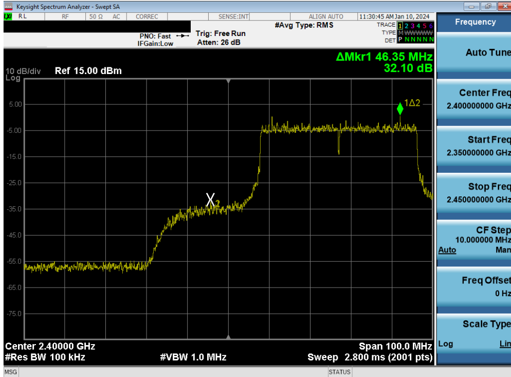
Plot 7-72. Band Edge Plot MIMO ANT1 (802.11be OFDMA – 484 Tones – Ch. 4)
