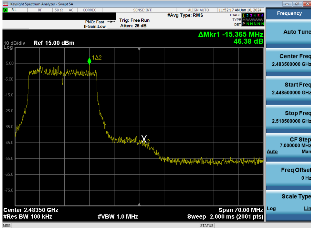
Plot 7-68. Band Edge Plot MIMO ANT1 (802.11be OFDMA – 242 Tones – Ch. 11)
