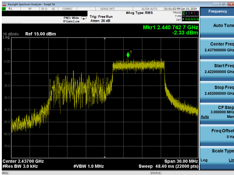
Plot 7-42. Power Spectral Density Plot MIMO ANT2 (802.11be OFDMA – 106 Tones – Ch. 6)
