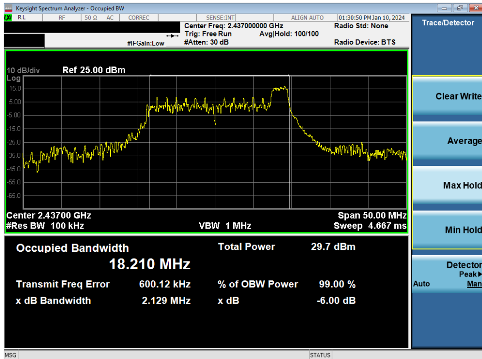
Plot 7-3. 6dB Bandwidth Plot MIMO ANT1 (802.11be OFDMA – 26 Tones – Ch. 6)
