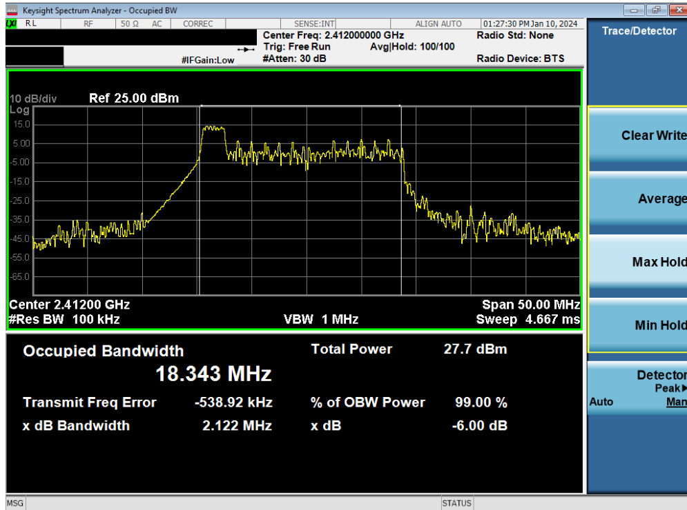
Plot 7-11. 6dB Bandwidth Plot MIMO ANT2 (802.11be OFDMA – 26 Tones – Ch. 1)
