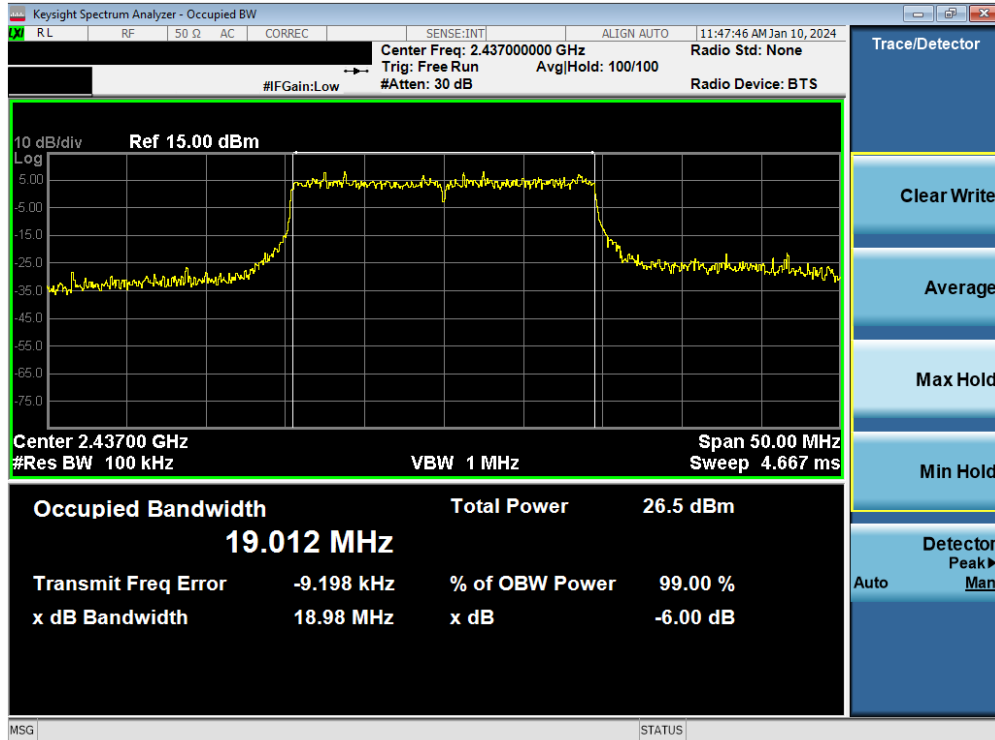
Plot 7-6. 6dB Bandwidth Plot MIMO ANT1 (802.11be OFDMA – 242 Tones – Ch. 6)
