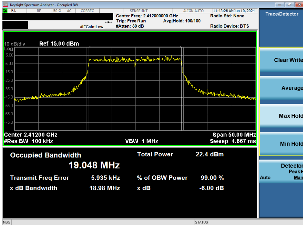
Plot 7-14. 6dB Bandwidth Plot MIMO ANT2 (802.11be OFDMA – 242 Tones – Ch. 1)
