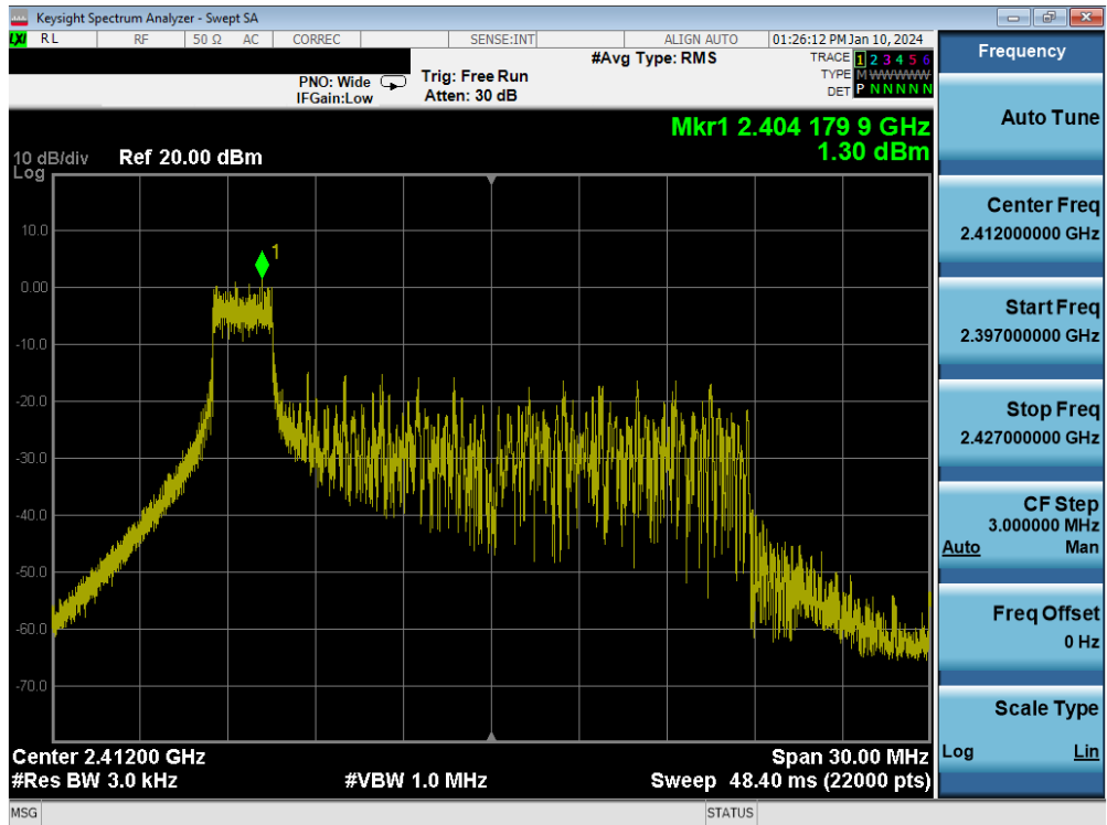
Plot 7-20. Power Spectral Density Plot MIMO ANT1 (802.11be OFDMA – 26 Tones – Ch. 1)
