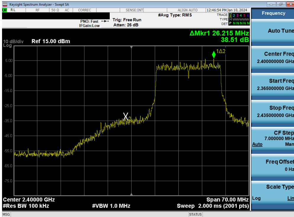
Plot 7-92. Band Edge Plot MIMO ANT2 (802.11be OFDMA – 242 Tones – Ch. 2)
