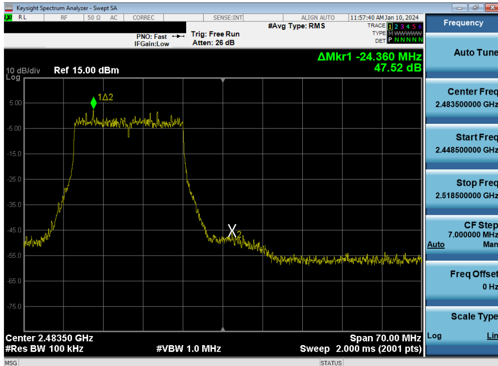
Plot 7-69. Band Edge Plot MIMO ANT1 (802.11be OFDMA – 242 Tones – Ch. 12)
