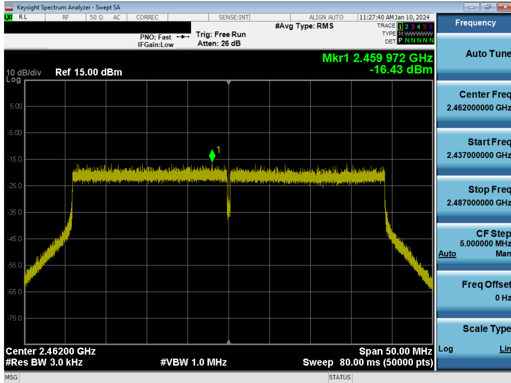
Plot 7-34. Power Spectral Density Plot MIMO ANT1 (802.11be OFDMA – 484 Tones – Ch. 11)
