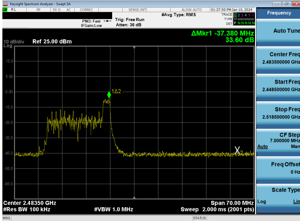
Plot 7-54. Band Edge Plot MIMO ANT1 (802.11be OFDMA – 26 Tones – Ch. 12)
