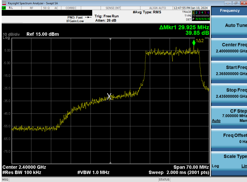
Plot 7-66. Band Edge Plot MIMO ANT1 (802.11be OFDMA – 242 Tones – Ch. 3)
