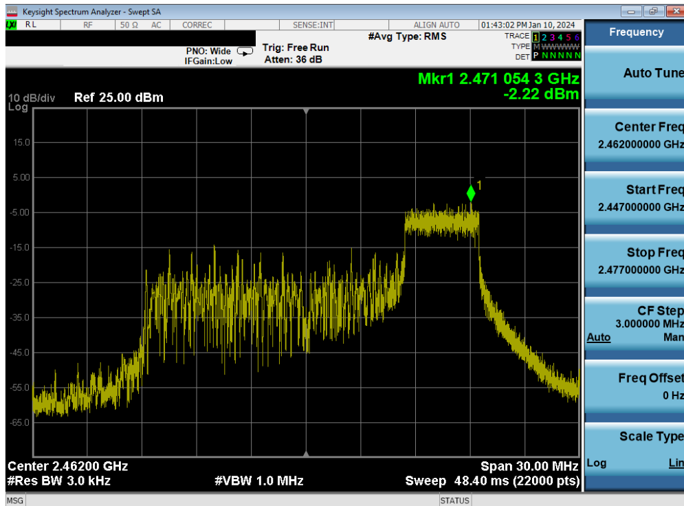
Plot 7-40. Power Spectral Density Plot MIMO ANT2 (802.11be OFDMA – 52 Tones – Ch. 11)
