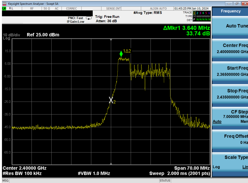
Plot 7-56. Band Edge Plot MIMO ANT1 (802.11be OFDMA – 52 Tones – Ch. 1)
