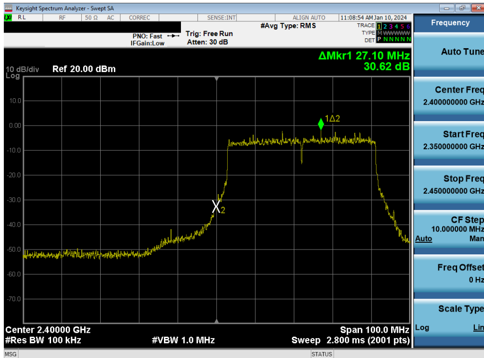
Plot 7-71. Band Edge Plot MIMO ANT1 (802.11be OFDMA – 484 Tones – Ch. 3)
