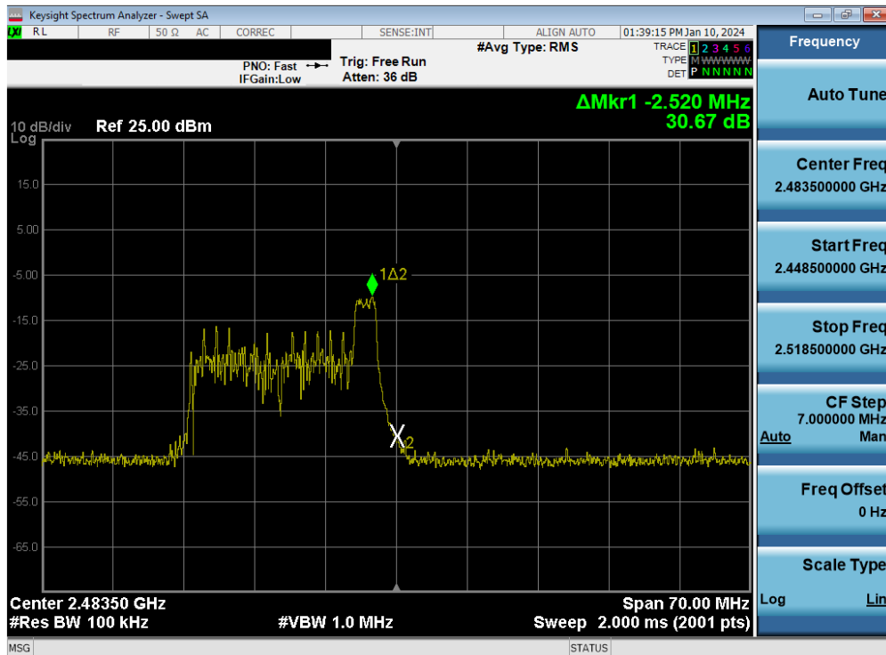
Plot 7-55. Band Edge Plot MIMO ANT1 (802.11be OFDMA – 26 Tones – Ch. 13)
