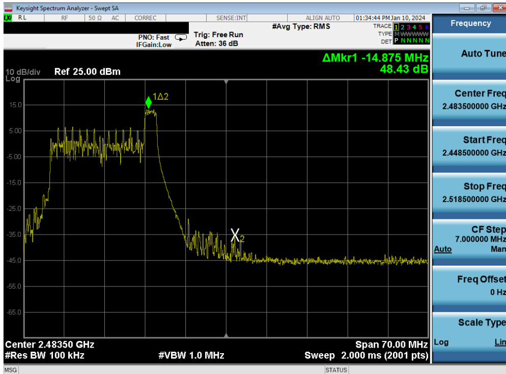
Plot 7-80. Band Edge Plot MIMO ANT2 (802.11be OFDMA – 26 Tones – Ch. 11)
