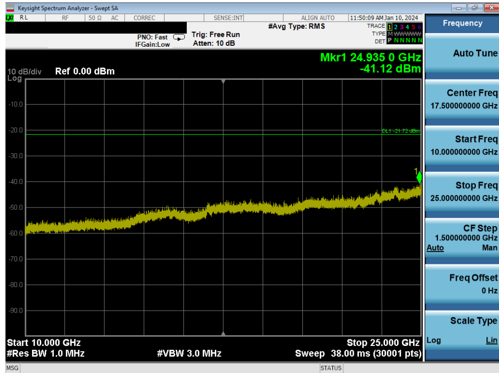
Plot 7-113. Conducted Spurious Plot MIMO ANT1 (802.11be OFDMA – 242 Tones – Ch. 6)
