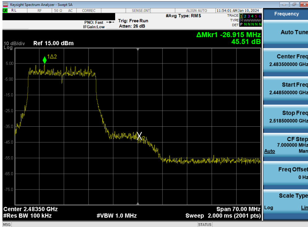
Plot 7-95. Band Edge Plot MIMO ANT2 (802.11be OFDMA – 242 Tones – Ch. 11)
