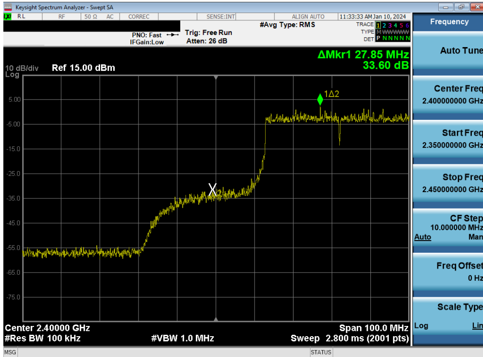
Plot 7-73. Band Edge Plot MIMO ANT1 (802.11be OFDMA – 484 Tones – Ch. 5)
