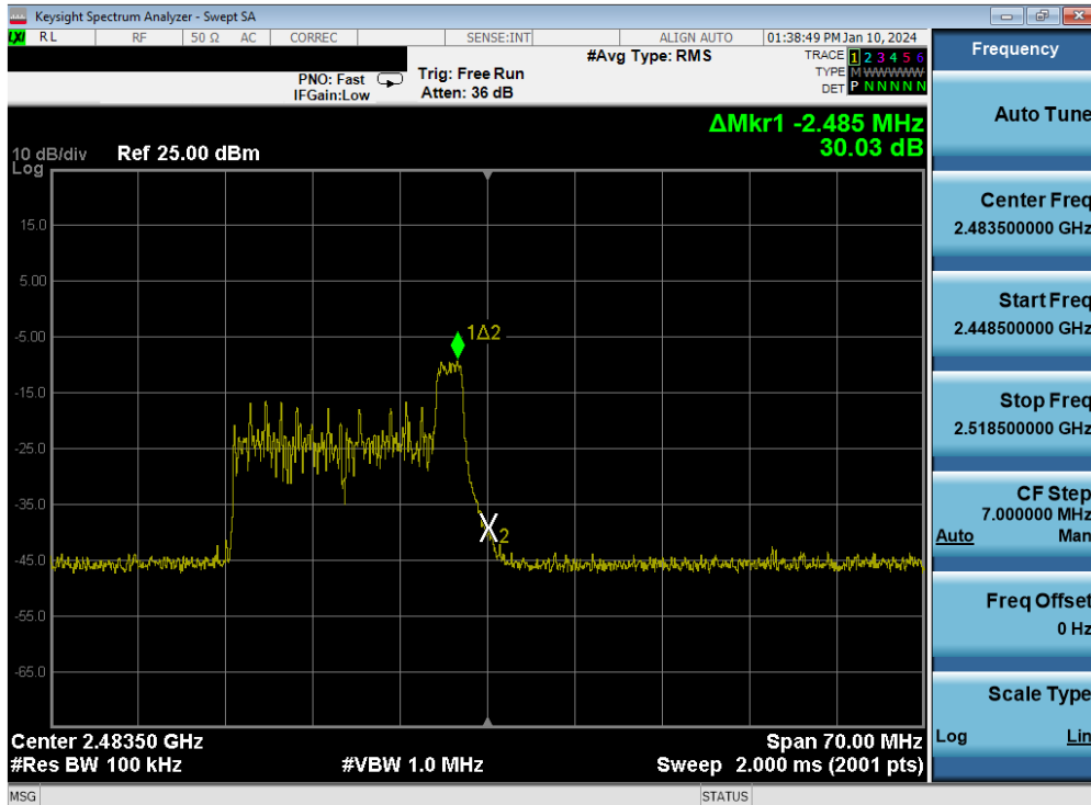
Plot 7-82. Band Edge Plot MIMO ANT2 (802.11be OFDMA – 26 Tones – Ch. 13)
