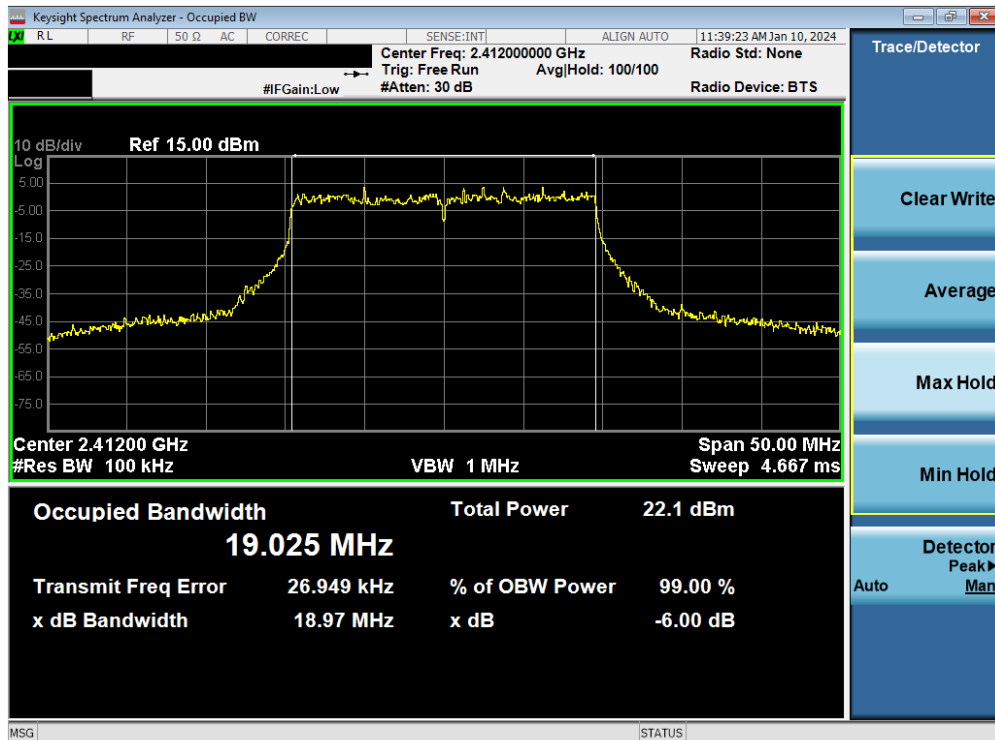
Plot 7-5. 6dB Bandwidth Plot MIMO ANT1 (802.11be OFDMA – 242 Tones – Ch. 1)
