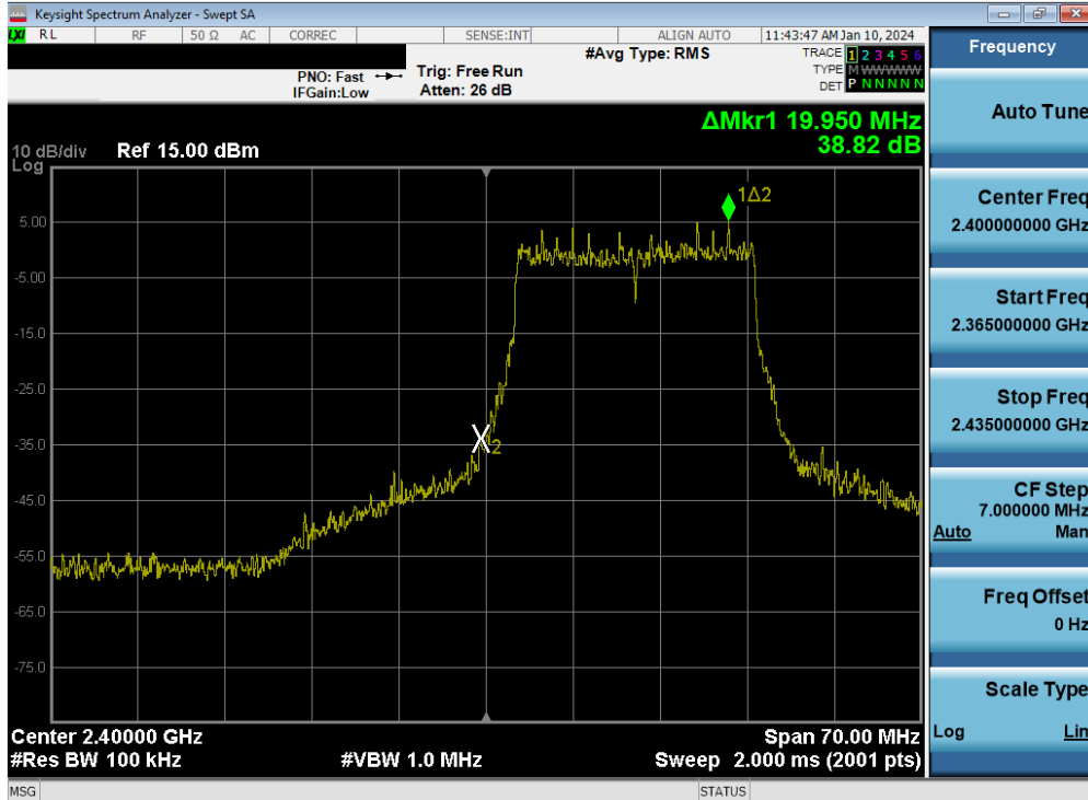
Plot 7-91. Band Edge Plot MIMO ANT2 (802.11be OFDMA – 242 Tones – Ch. 1)
