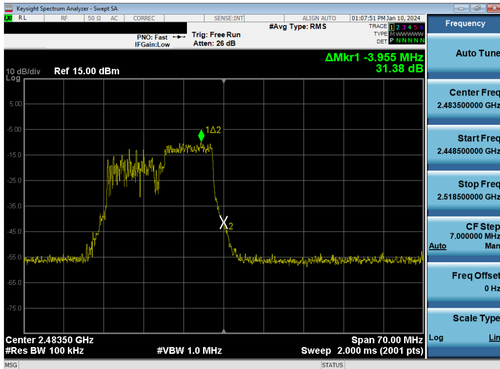
Plot 7-90. Band Edge Plot MIMO ANT2 (802.11be OFDMA – 106 Tones – Ch. 13)
