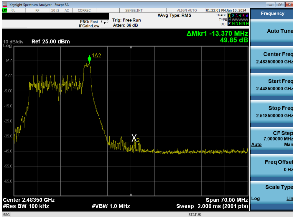
Plot 7-53. Band Edge Plot MIMO ANT1 (802.11be OFDMA – 26 Tones – Ch. 11)
