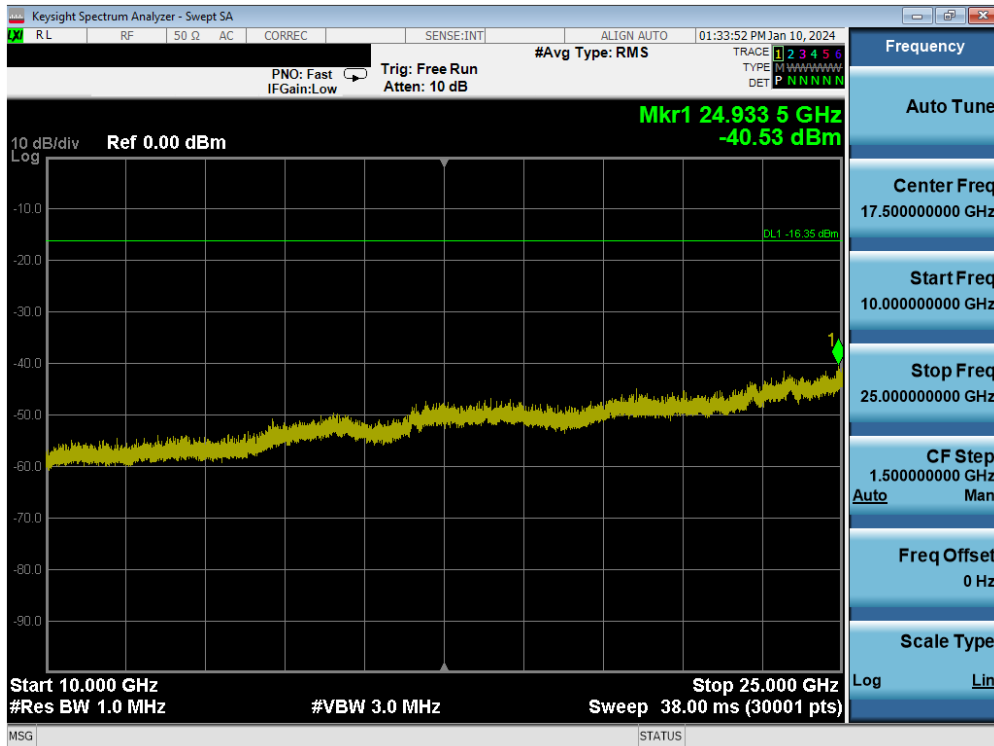
Plot 7-109. Conducted Spurious Plot MIMO ANT1 (802.11be OFDMA – 26 Tones – Ch. 11)
