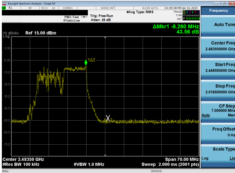
Plot 7-89. Band Edge Plot MIMO ANT2 (802.11be OFDMA – 106 Tones – Ch. 12)
