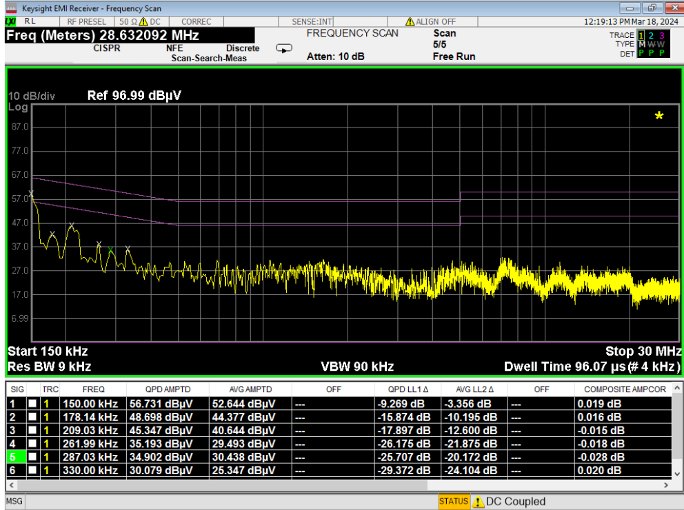
Plot 7-226. Line Conducted Plot with 802.11b (L1)
