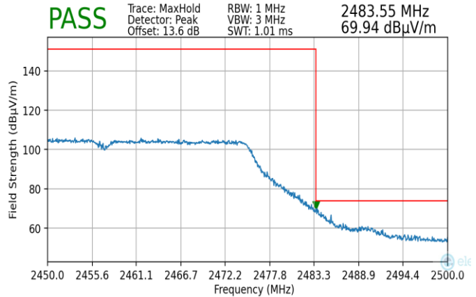
Plot 7-223. Radiated Restricted Upper Band Edge Measurement MIMO (Peak)
