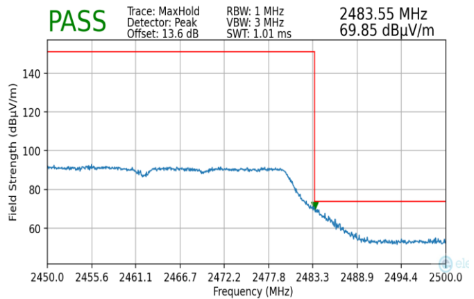
Plot 7-225. Radiated Restricted Upper Band Edge Measurement MIMO (Peak)
