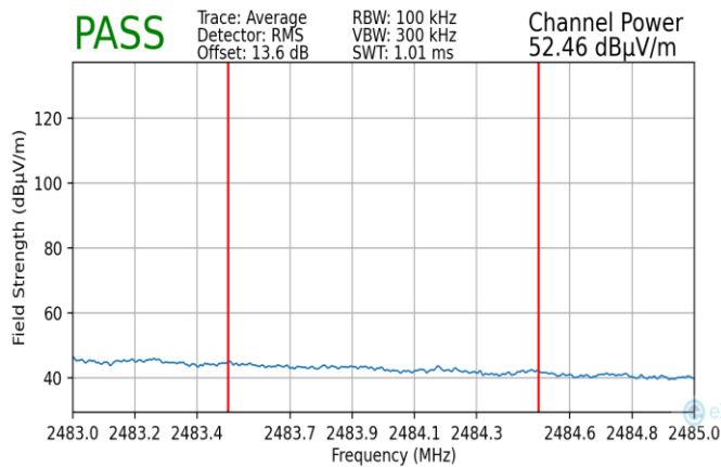
Plot 7-224. Radiated Restricted Upper Band Edge Measurement MIMO (Average)
