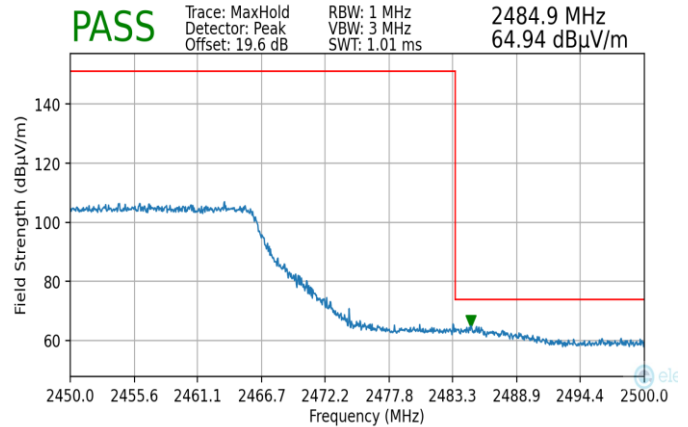
Plot 7-219. Radiated Restricted Upper Band Edge Measurement MIMO (Peak)
