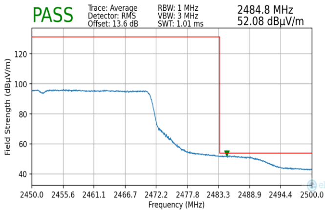
Plot 7-220. Radiated Restricted Upper Band Edge Measurement MIMO (Average)
