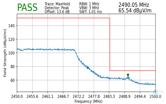
Plot 7-221. Radiated Restricted Upper Band Edge Measurement MIMO (Peak)
