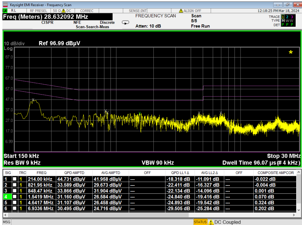
Plot 7-227. Line Conducted Plot with 802.11b (N)
