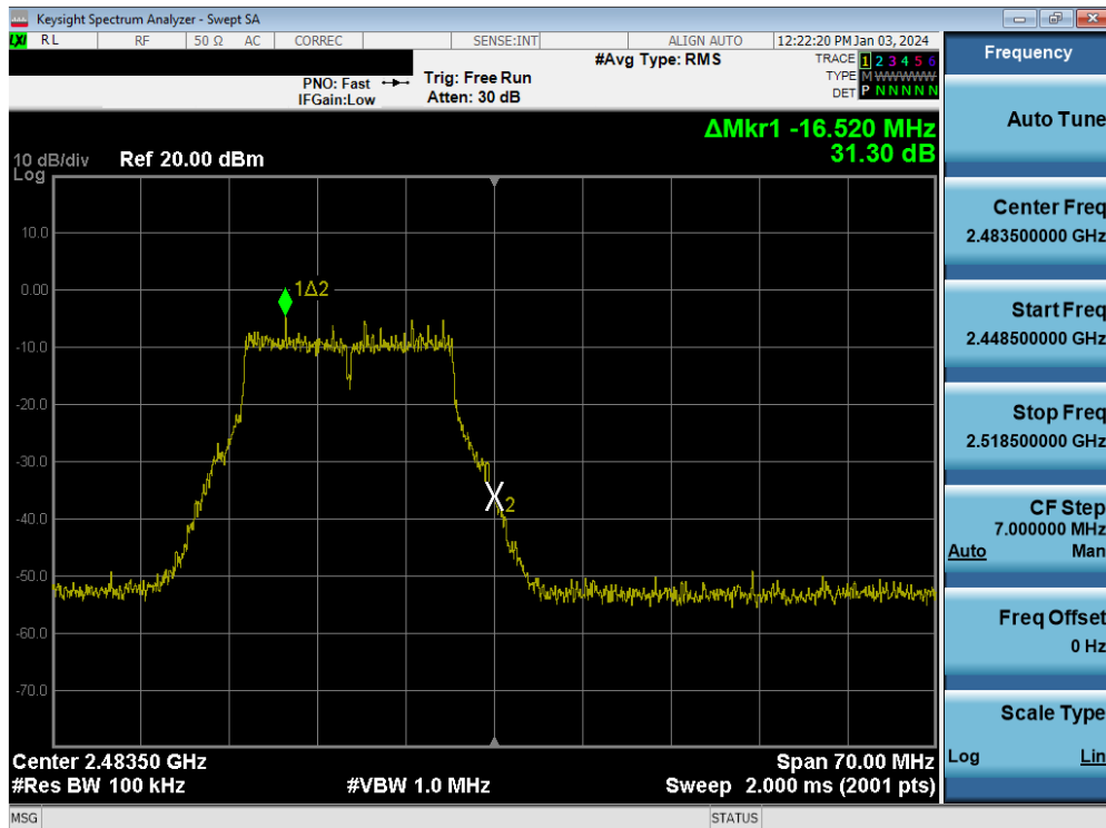
Plot 7-85. Band Edge Plot MIMO ANT1 (802.11g – Ch. 13)
