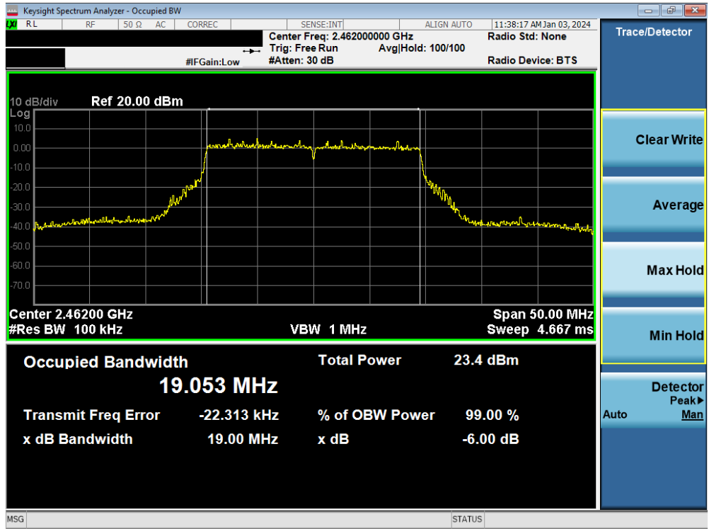
Plot 7-25. 6dB Bandwidth Plot MIMO ANT2 (802.11be (2.4GHz) – Ch. 11)
