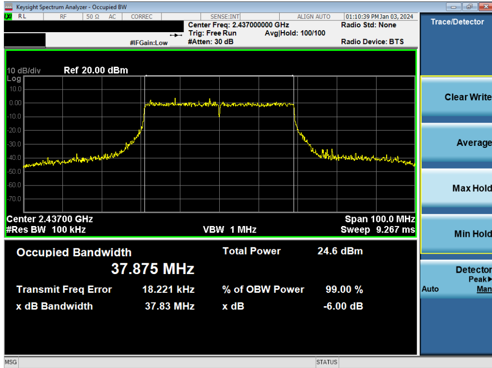
Plot 7-30. 6dB Bandwidth Plot MIMO ANT1 (802.11be (2.4GHz) – Ch. 6)
