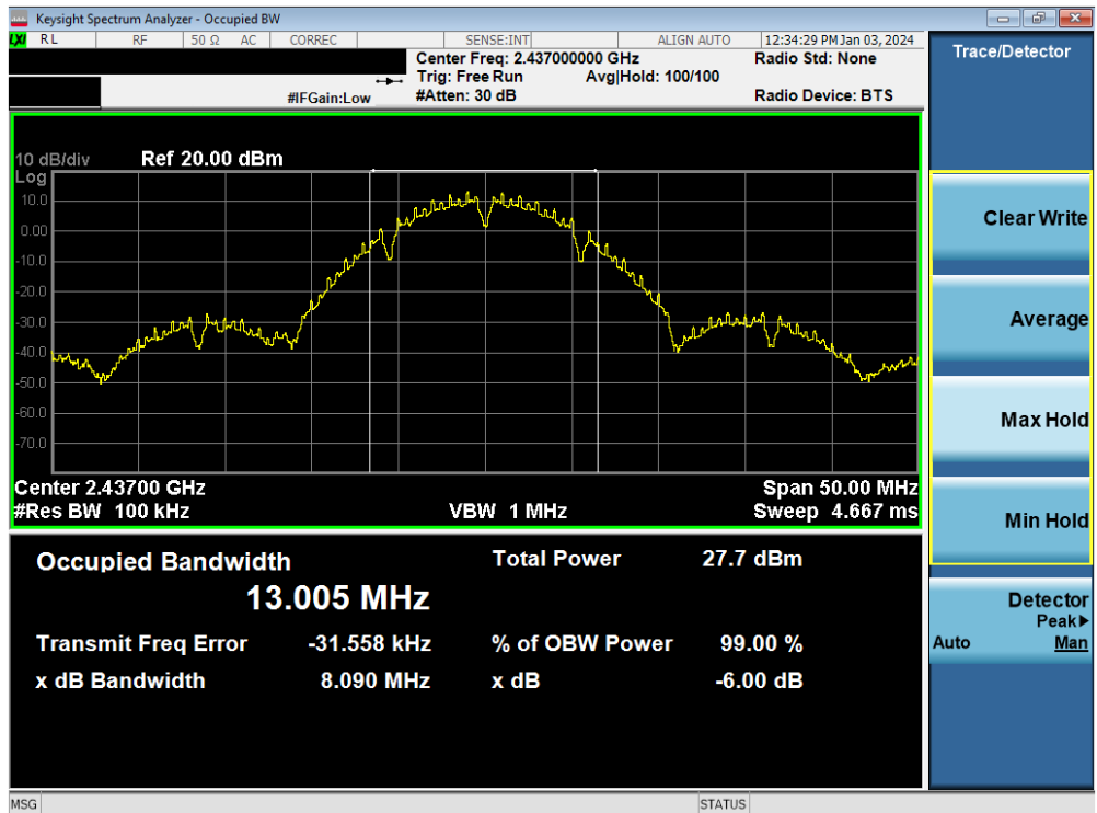
Plot 7-15. 6dB Bandwidth Plot MIMO ANT2 (802.11b – Ch. 6)
