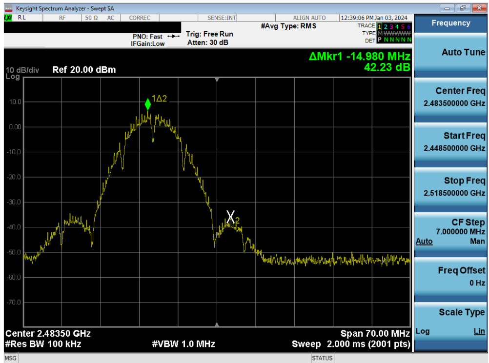
Plot 7-104. Band Edge Plot MIMO ANT2 (802.11b – Ch. 13)
