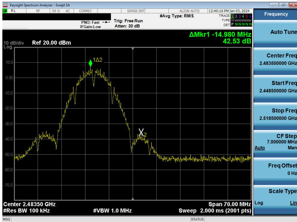
Plot 7-79. Band Edge Plot MIMO ANT1 (802.11b – Ch. 13)
