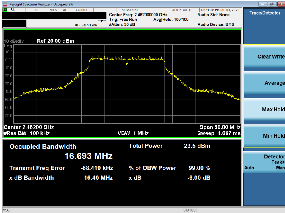
Plot 7-19. 6dB Bandwidth Plot MIMO ANT2 (802.11g – Ch. 11)
