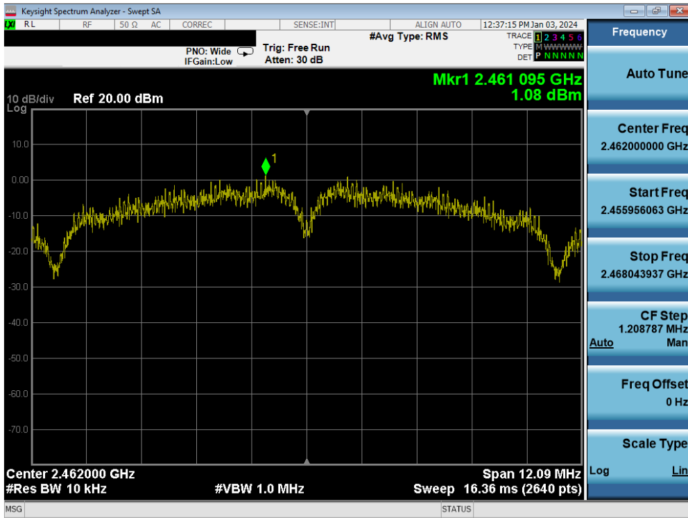
Plot 7-52. Power Spectral Density Plot MIMO ANT2 (802.11g – Ch. 11)
