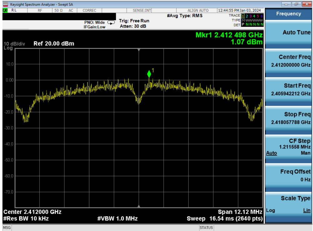
Plot 7-38. Power Spectral Density Plot MIMO ANT1 (802.11b – Ch. 1)
