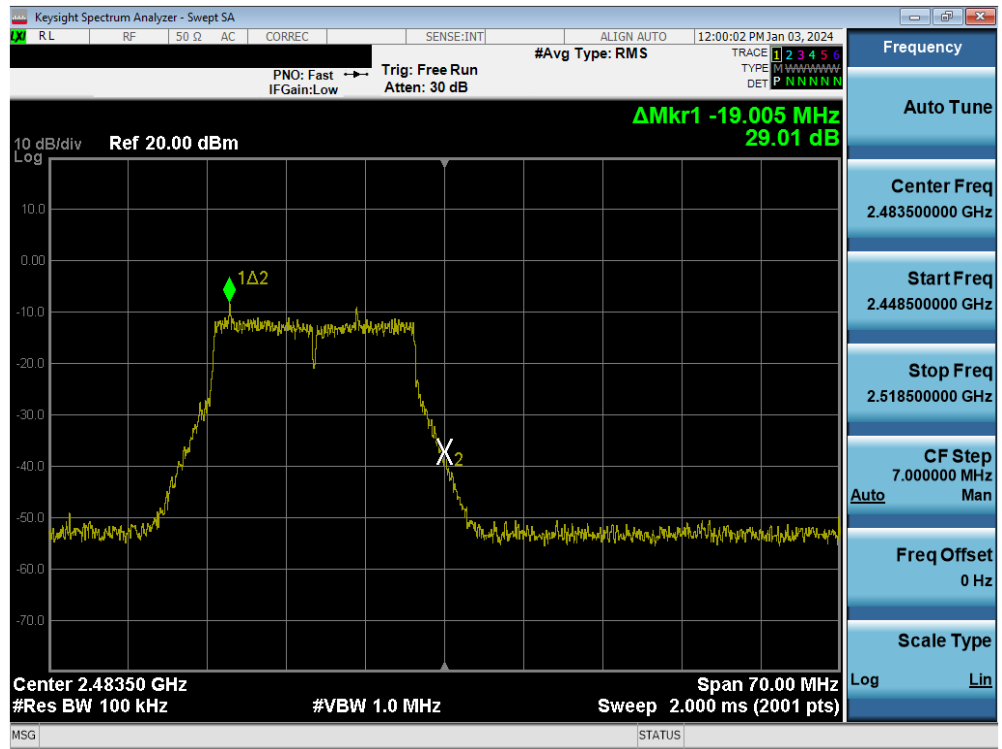
Plot 7-91. Band Edge Plot MIMO ANT1 (802.11n (2.4GHz) – Ch. 13)
