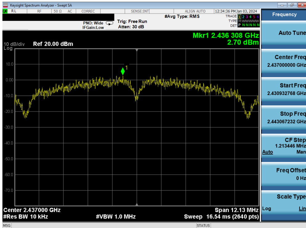
Plot 7-51. Power Spectral Density Plot MIMO ANT2 (802.11g – Ch. 6)
