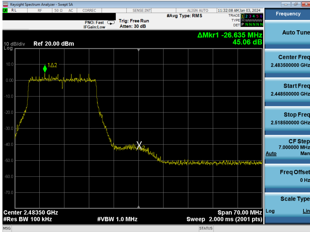
Plot 7-96. Band Edge Plot MIMO ANT1 (802.11be (2.4GHz) – Ch. 11)
