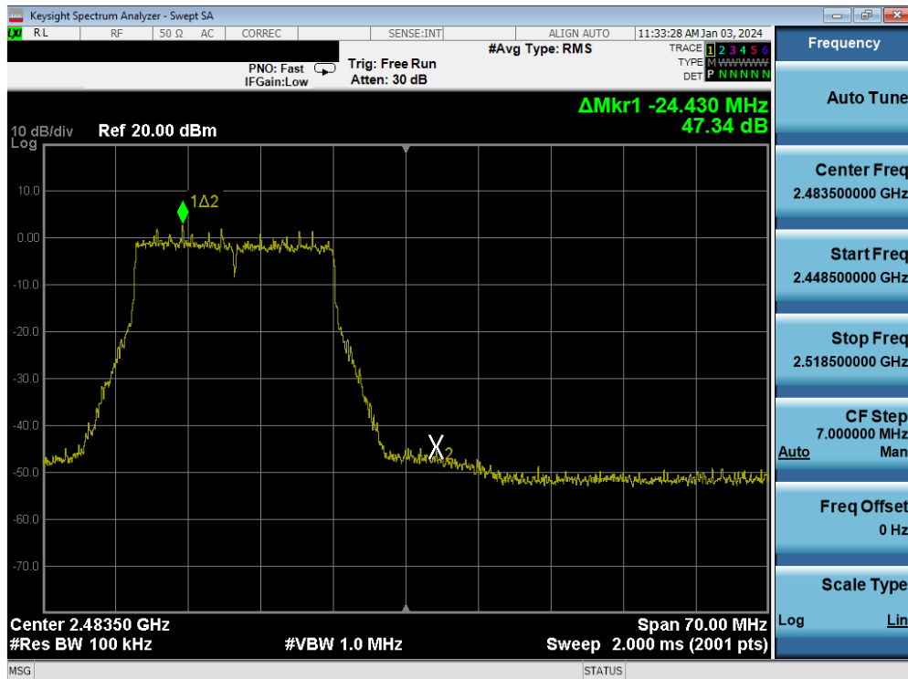
Plot 7-97. Band Edge Plot MIMO ANT1 (802.11be (2.4GHz) – Ch. 12)
