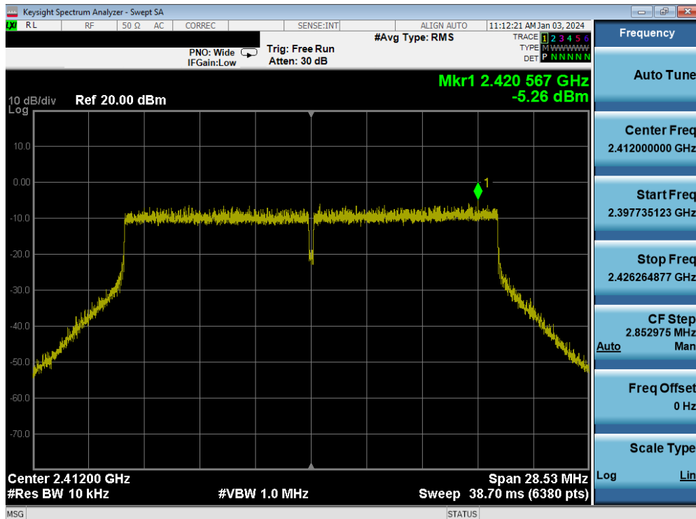
Plot 7-47. Power Spectral Density Plot MIMO ANT1 (802.11be (2.4GHz) – Ch. 1)
