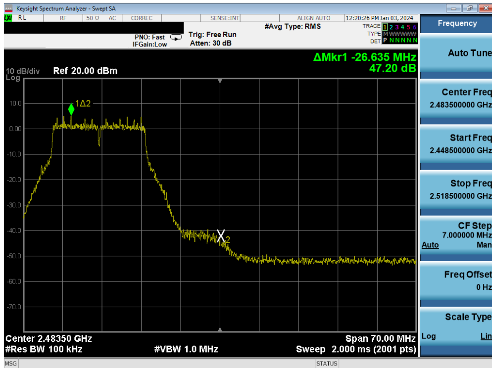
Plot 7-83. Band Edge Plot MIMO ANT1 (802.11g – Ch. 11)
