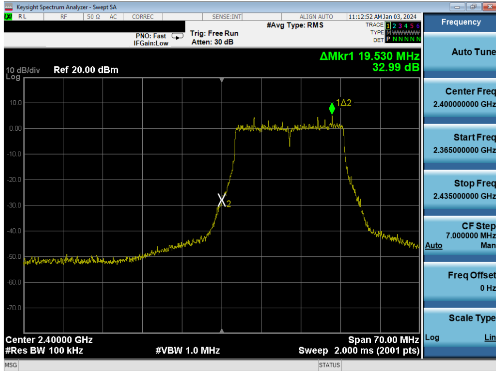
Plot 7-92. Band Edge Plot MIMO ANT1 (802.11be (2.4GHz) – Ch. 1)
