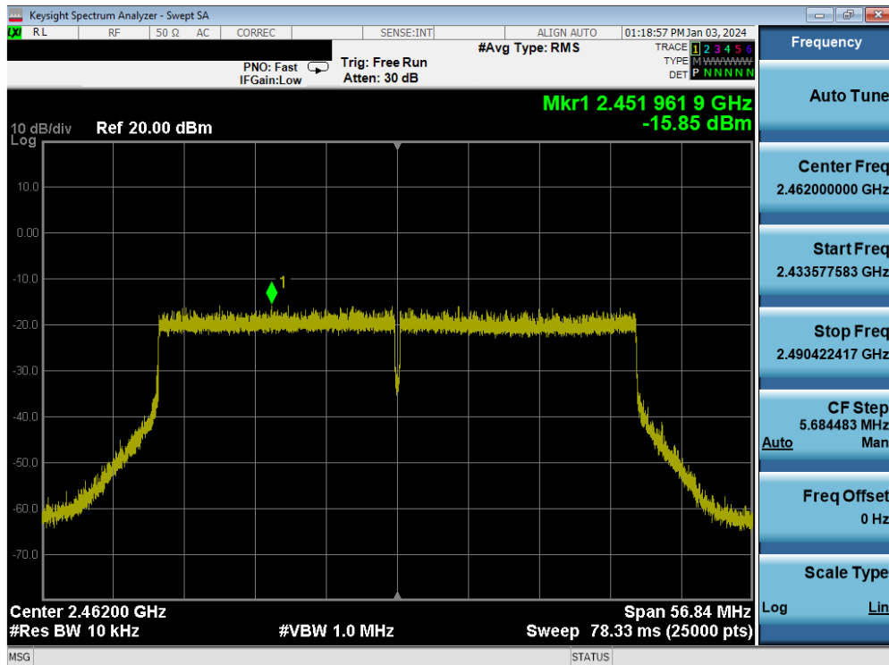
Plot 7-67. Power Spectral Density Plot MIMO ANT1 (802.11be (2.4GHz) – Ch. 11)
