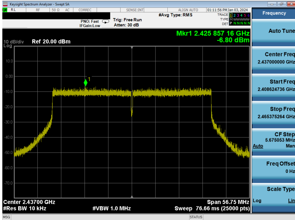
Plot 7-66. Power Spectral Density Plot MIMO ANT1 (802.11be (2.4GHz) – Ch. 6)
