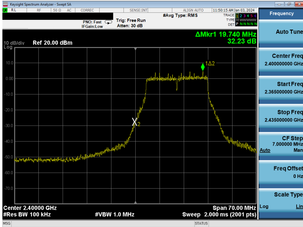
Plot 7-111. Band Edge Plot MIMO ANT2 (802.11n (2.4GHz) – Ch. 1)
