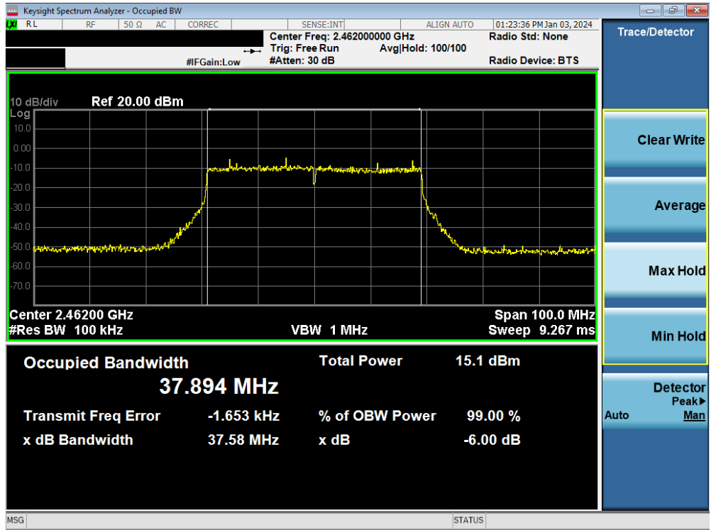
Plot 7-37. 6dB Bandwidth Plot MIMO ANT2 (802.11be (2.4GHz) – Ch. 11)
