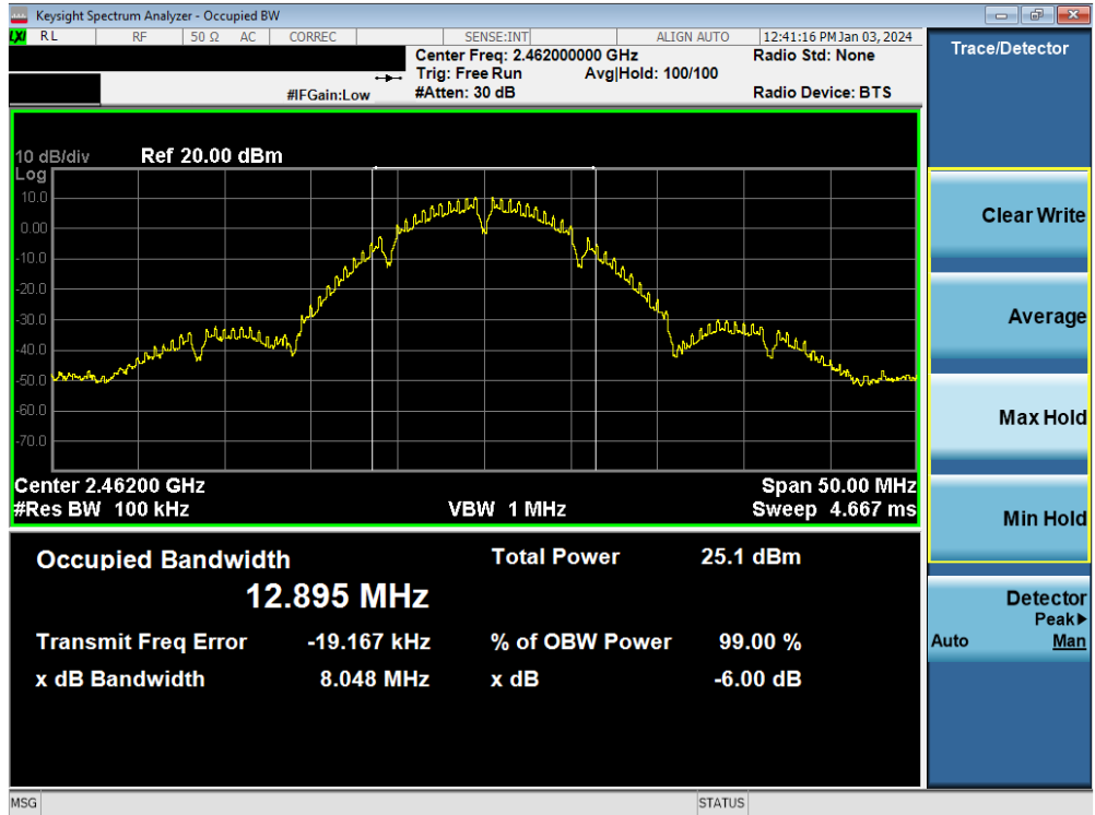
Plot 7-4. 6dB Bandwidth Plot MIMO ANT1 (802.11b – Ch. 11)
