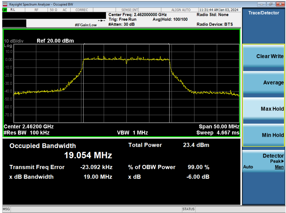
Plot 7-13. 6dB Bandwidth Plot MIMO ANT1 (802.11be (2.4GHz) – Ch. 11)
