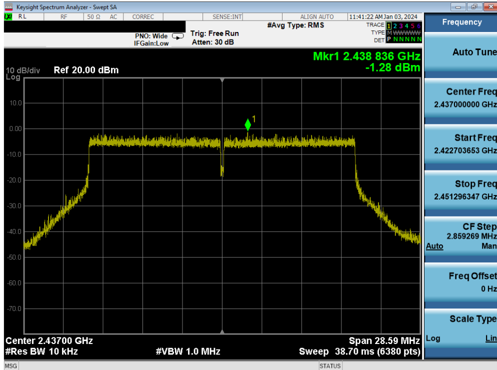
Plot 7-60. Power Spectral Density Plot MIMO ANT2 (802.11be (2.4GHz) – Ch. 6)
