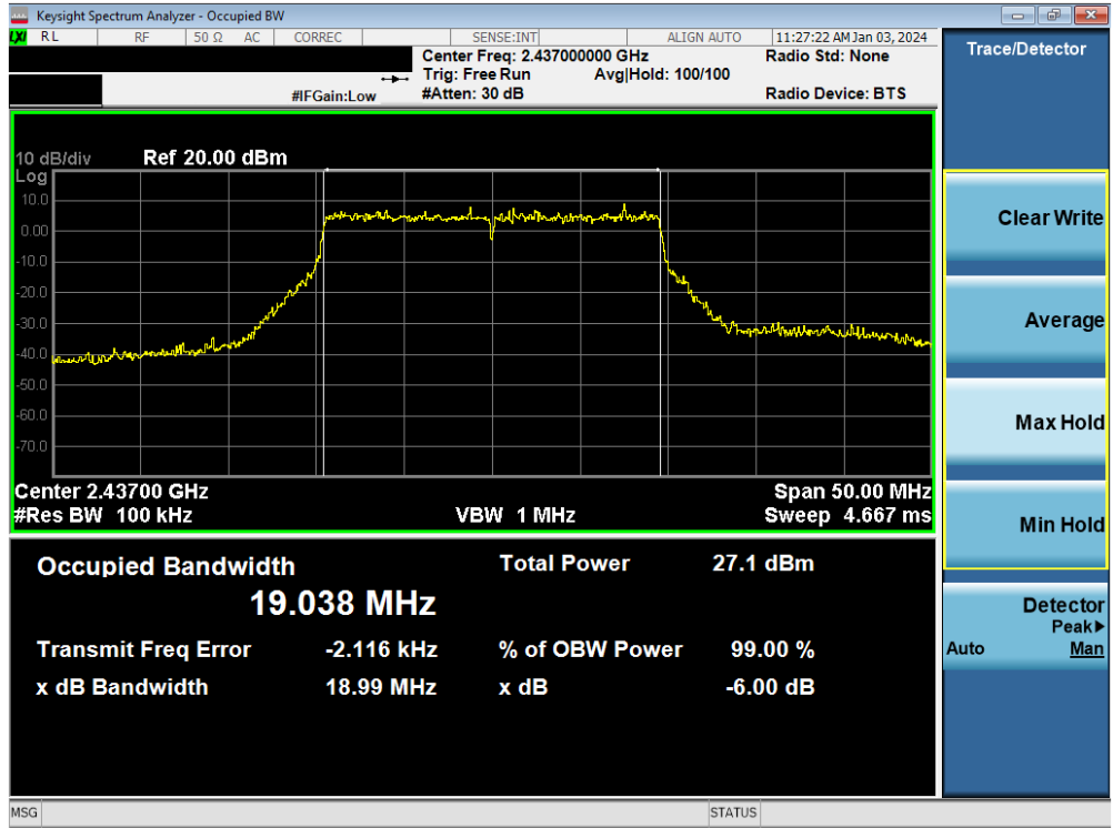
Plot 7-12. 6dB Bandwidth Plot MIMO ANT1 (802.11be (2.4GHz) – Ch. 6)
