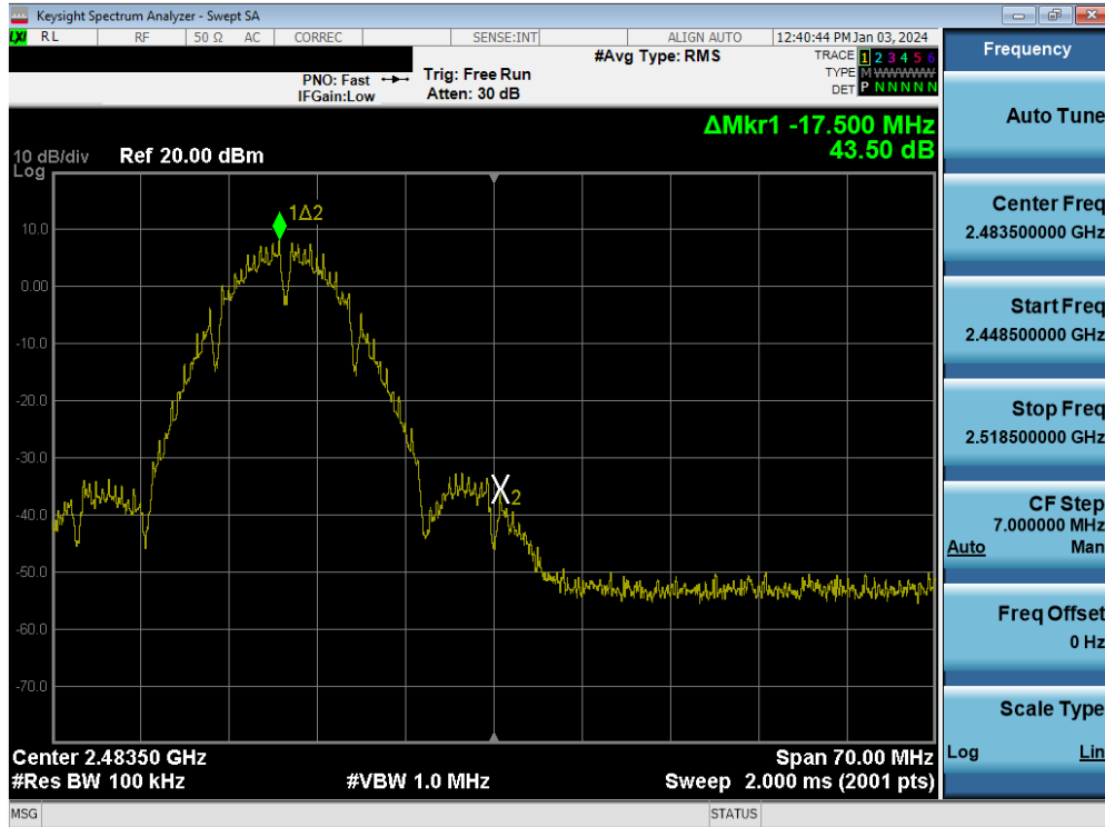
Plot 7-78. Band Edge Plot MIMO ANT1 (802.11b – Ch. 12)
