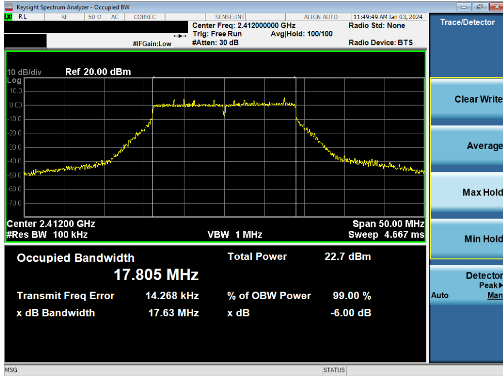
Plot 7-20. 6dB Bandwidth Plot MIMO ANT2 (802.11n (2.4GHz) – Ch. 1)
