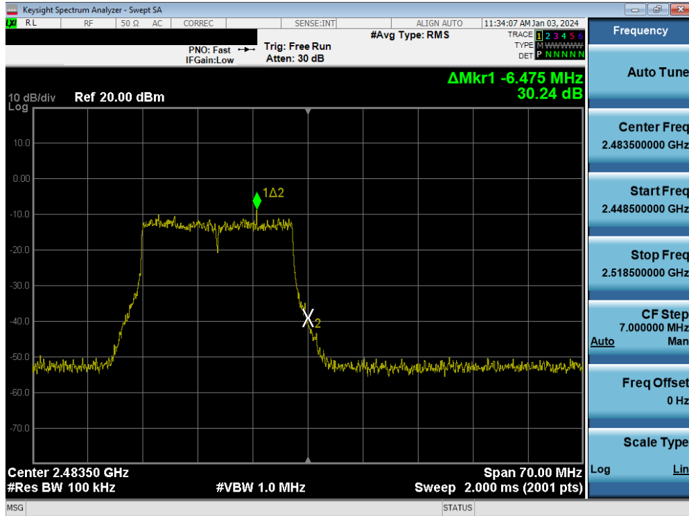
Plot 7-98. Band Edge Plot MIMO ANT1 (802.11be (2.4GHz) – Ch. 13)
