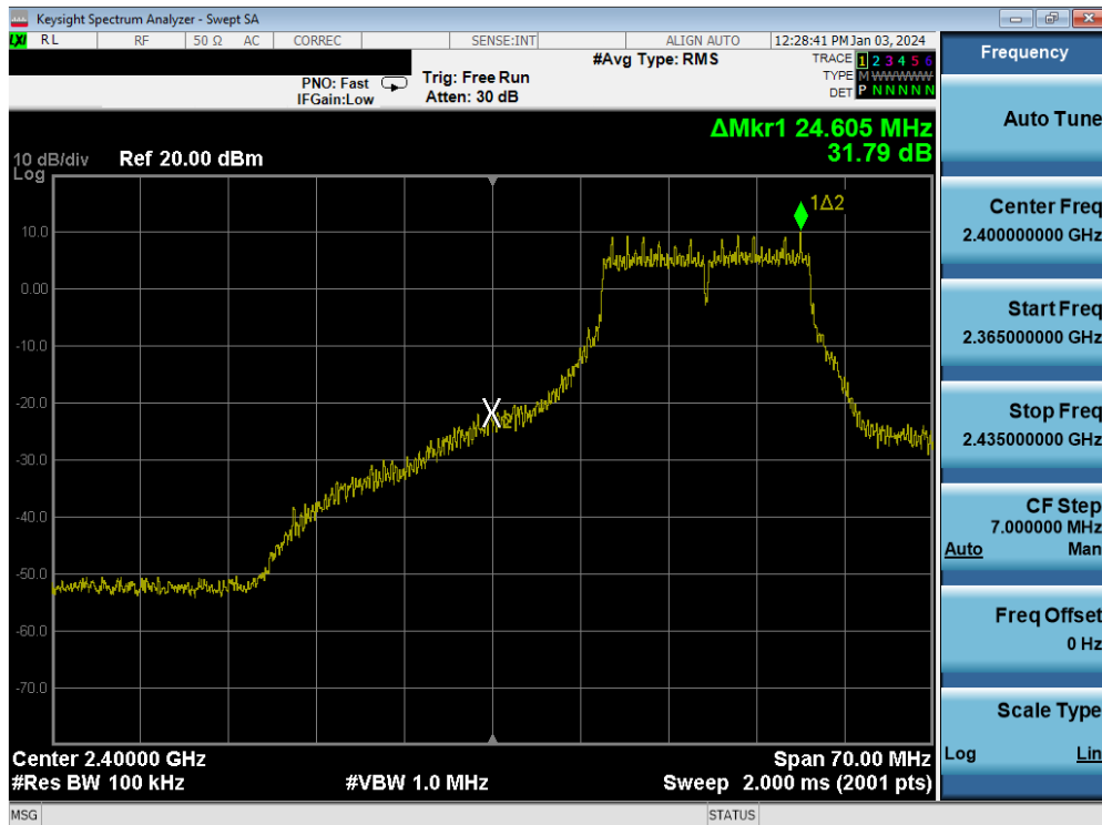
Plot 7-106. Band Edge Plot MIMO ANT2 (802.11g- Ch. 2)
