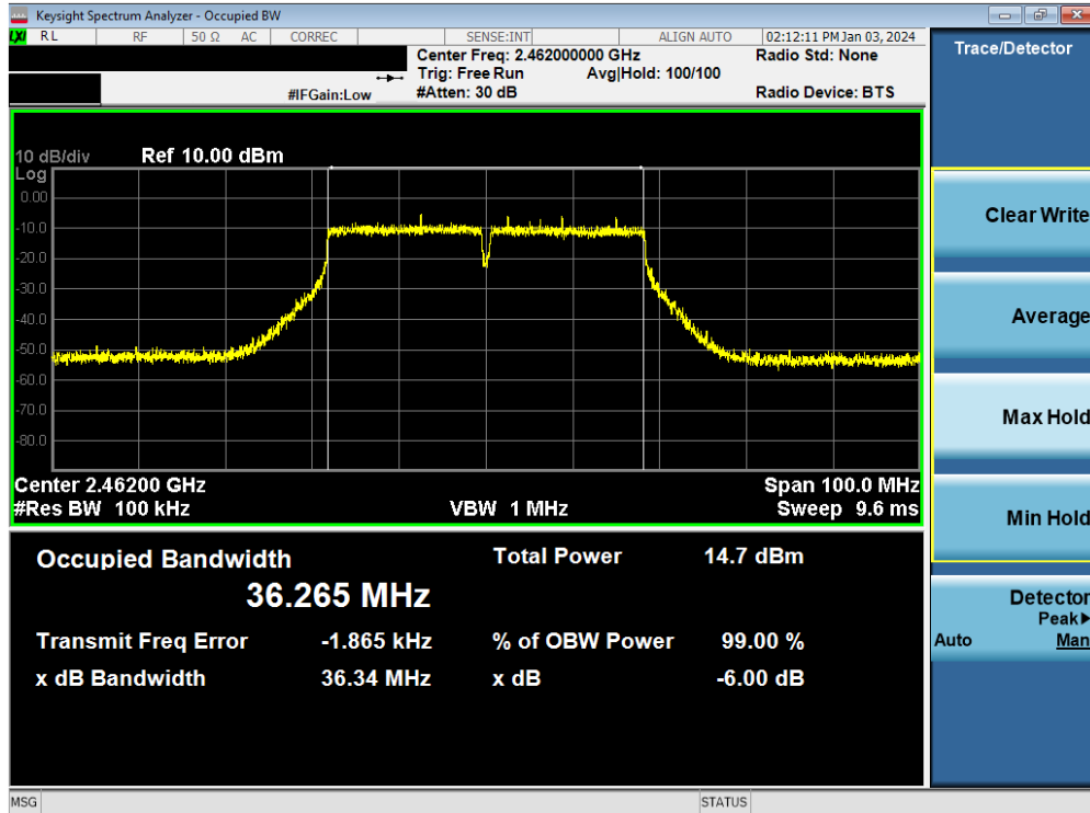
Plot 7-28. 6dB Bandwidth Plot MIMO ANT1 (802.11n (2.4GHz) – Ch. 11)
