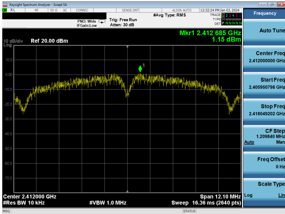
Plot 7-50. Power Spectral Density Plot MIMO ANT2 (802.11g – Ch. 1)
