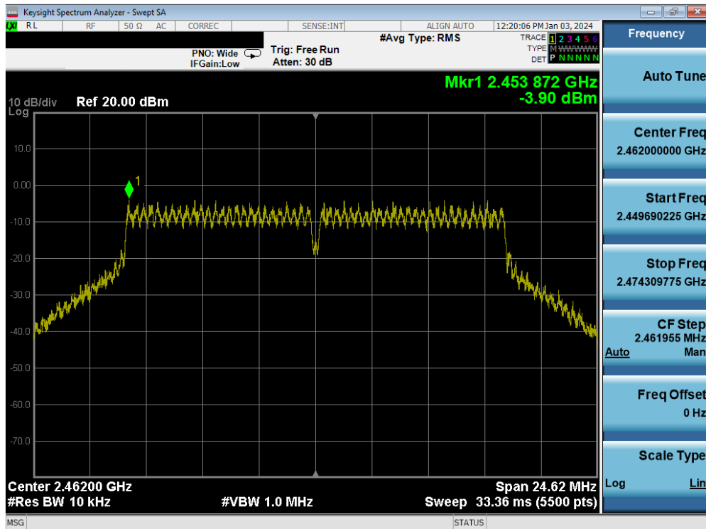
Plot 7-43. Power Spectral Density Plot MIMO ANT1 (802.11g – Ch. 11)
