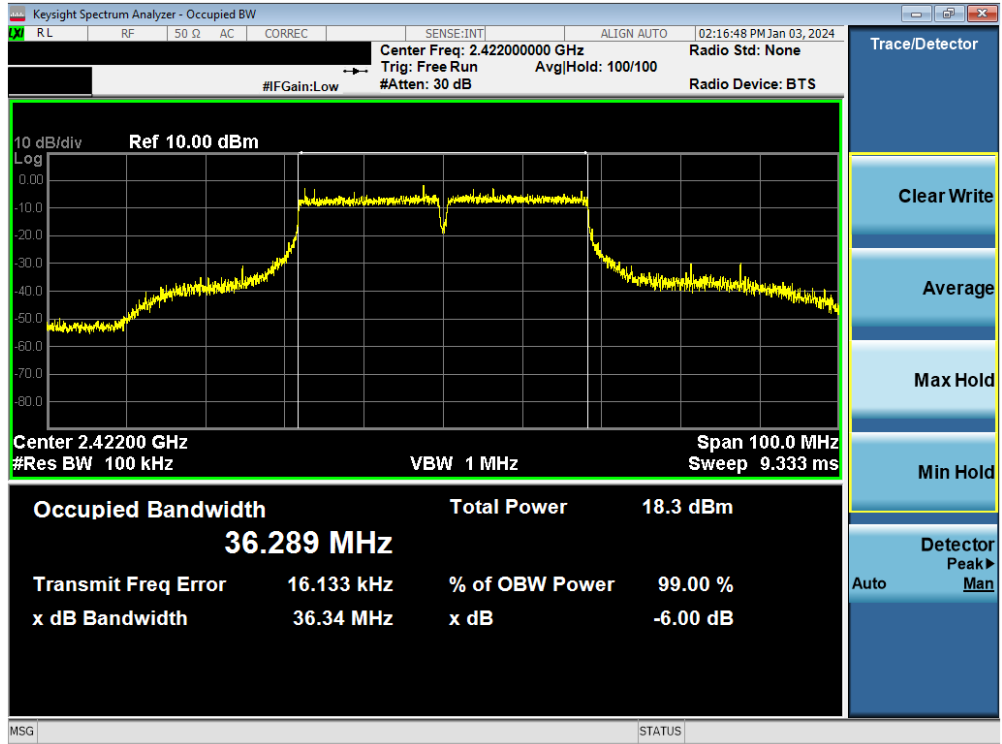
Plot 7-26. 6dB Bandwidth Plot MIMO ANT1 (802.11n (2.4GHz) – Ch. 3)
