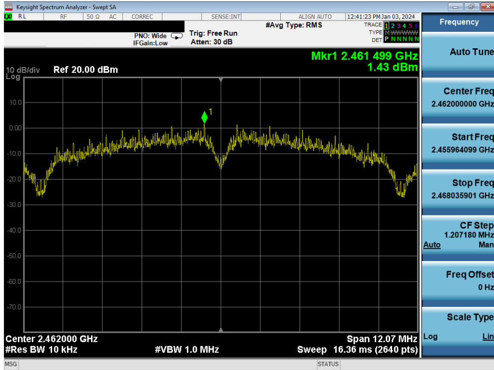
Plot 7-40. Power Spectral Density Plot MIMO ANT1 (802.11b – Ch. 11)
