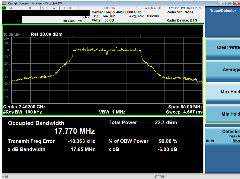
Plot 7-10. 6dB Bandwidth Plot MIMO ANT1 (802.11n (2.4GHz) – Ch. 11)
