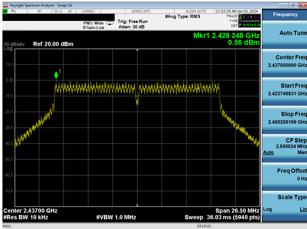
Plot 7-57. Power Spectral Density Plot MIMO ANT2 (802.11n (2.4GHz) – Ch. 6)
