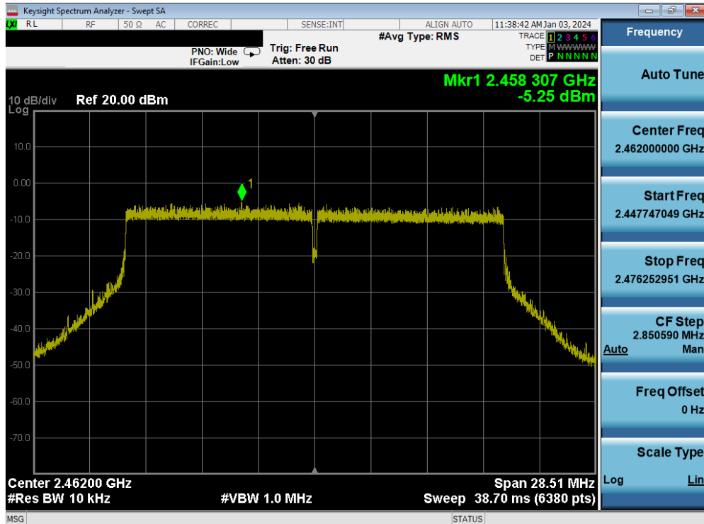
Plot 7-61. Power Spectral Density Plot MIMO ANT2 (802.11be (2.4GHz) – Ch. 11)
