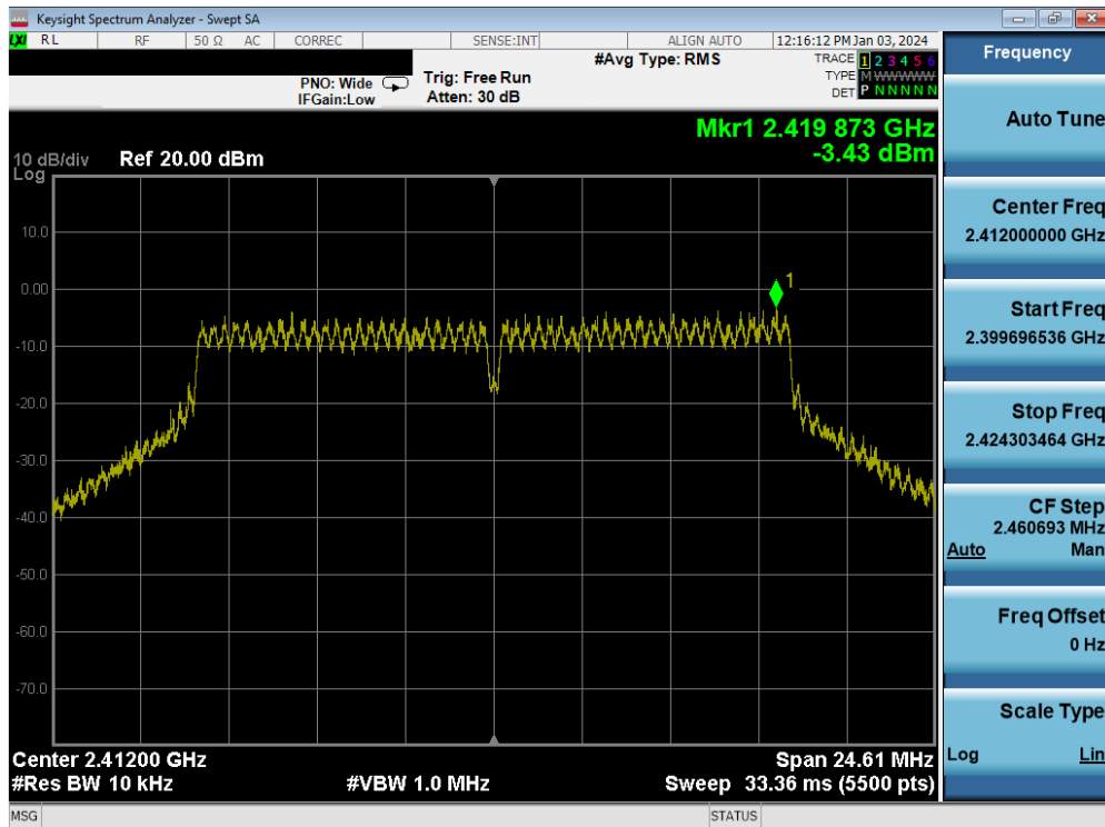
Plot 7-41. Power Spectral Density Plot MIMO ANT1 (802.11g – Ch. 1)
