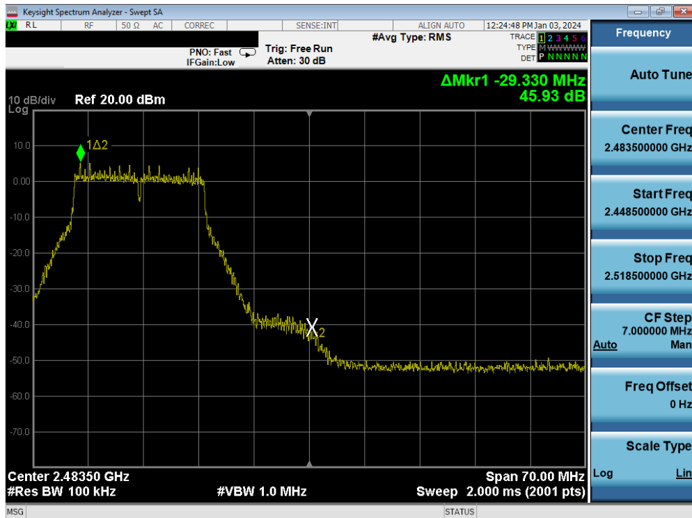
Plot 7-108. Band Edge Plot MIMO ANT2 (802.11g – Ch. 11)
