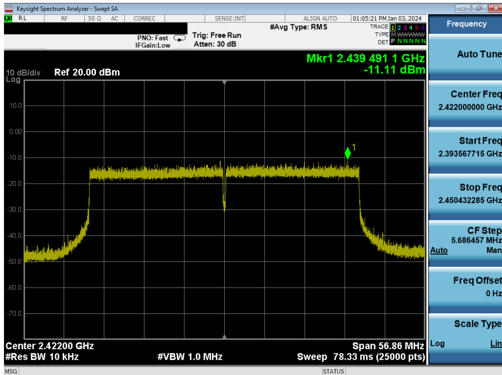
Plot 7-65. Power Spectral Density Plot MIMO ANT1 (802.11be (2.4GHz) – Ch. 3)
