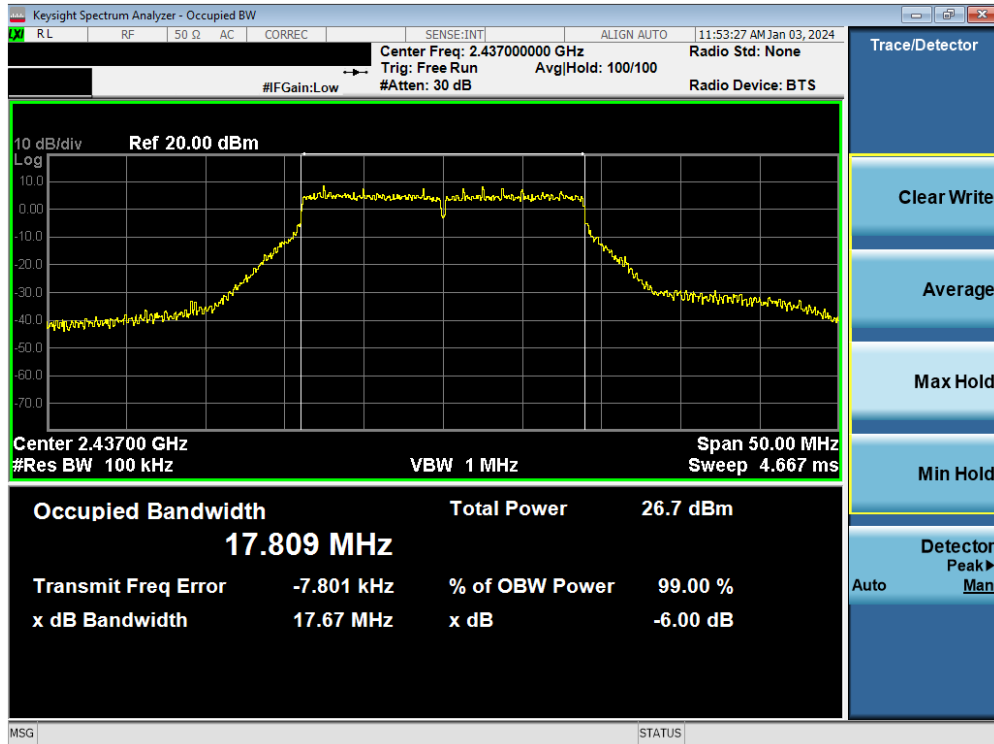
Plot 7-21. 6dB Bandwidth Plot MIMO ANT2 (802.11n (2.4GHz) – Ch. 6)
