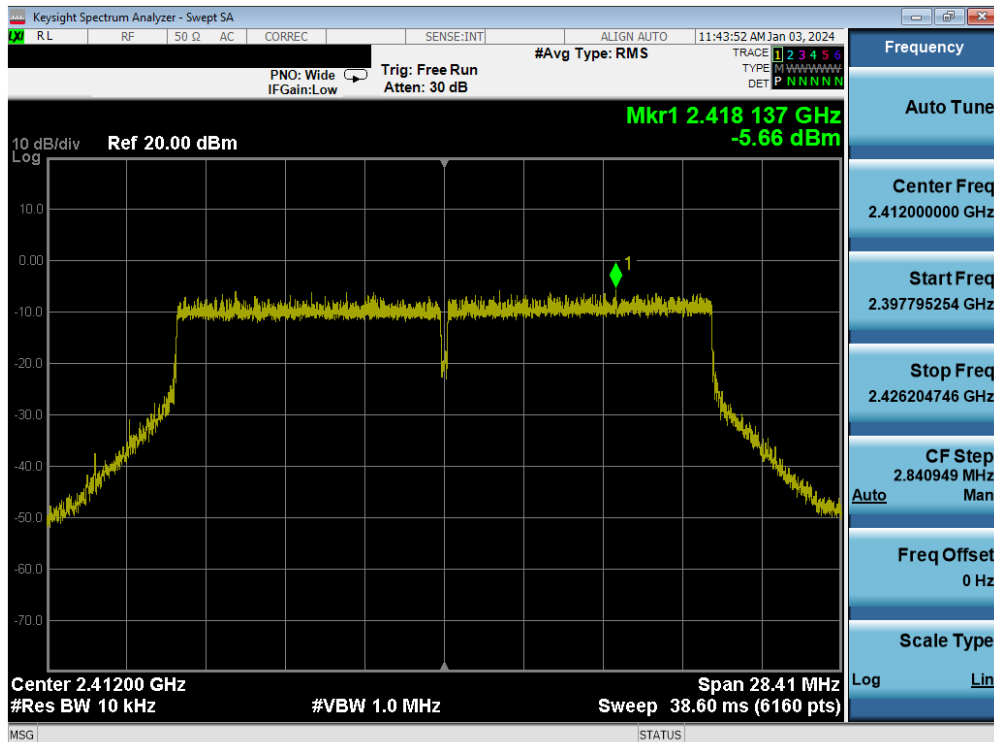
Plot 7-59. Power Spectral Density Plot MIMO ANT2 (802.11be (2.4GHz) – Ch. 1)
