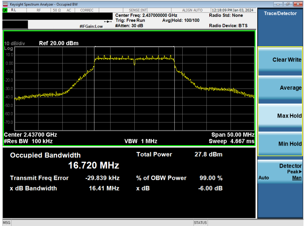
Plot 7-6. 6dB Bandwidth Plot MIMO ANT1 (802.11g – Ch. 6)
