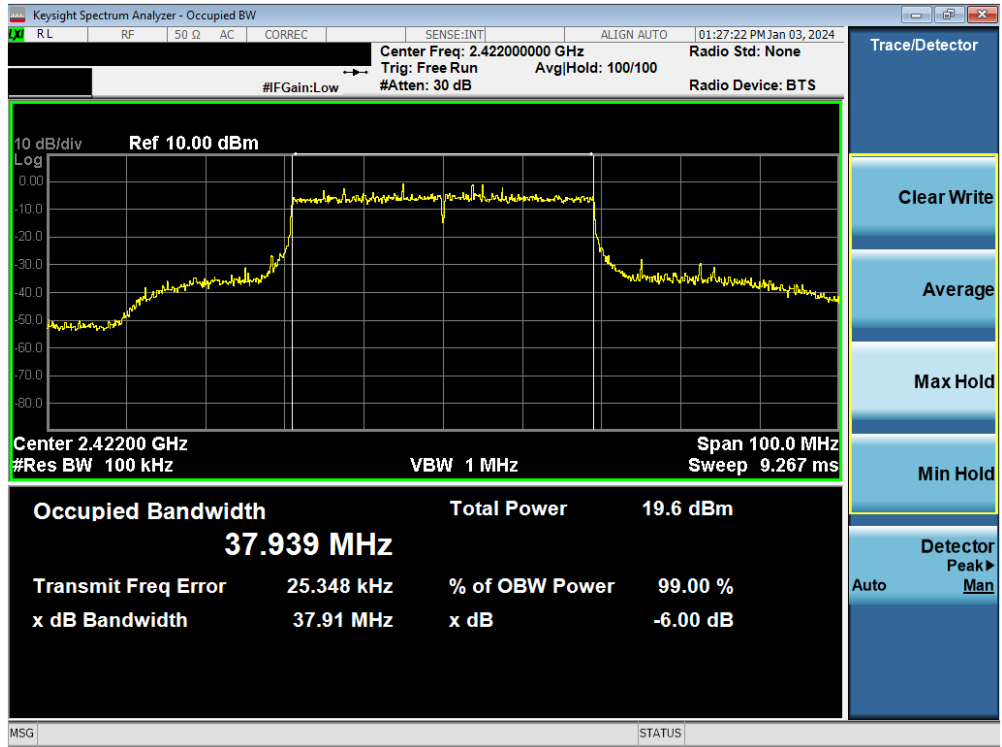
Plot 7-35. 6dB Bandwidth Plot MIMO ANT2 (802.11be (2.4GHz) – Ch. 3)
