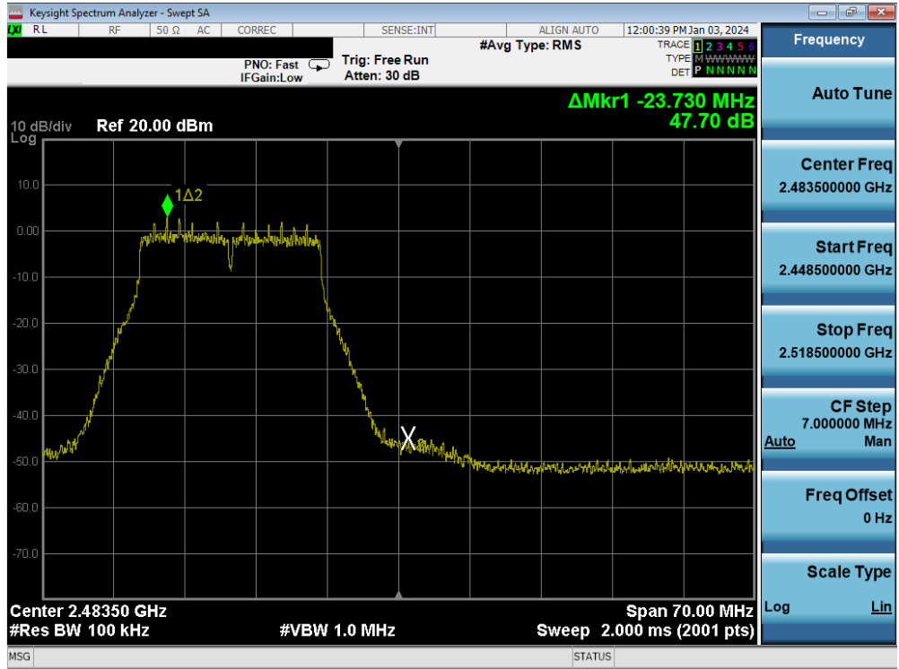
Plot 7-90. Band Edge Plot MIMO ANT1 (802.11n (2.4GHz) – Ch. 12)
