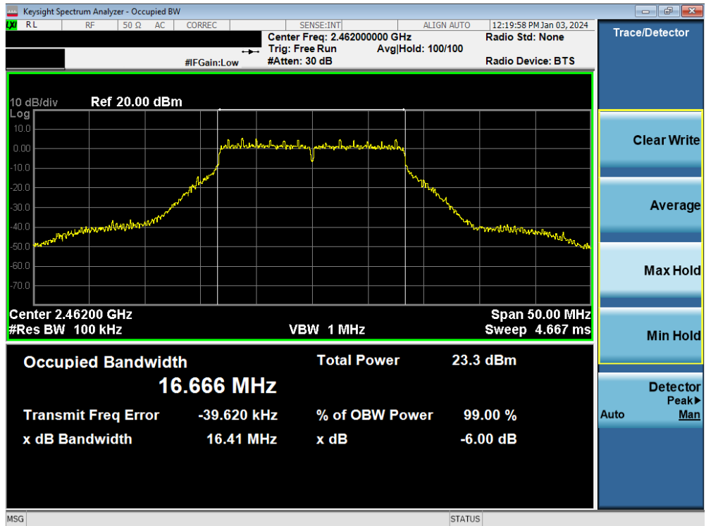
Plot 7-7. 6dB Bandwidth Plot MIMO ANT1 (802.11g – Ch. 11)
