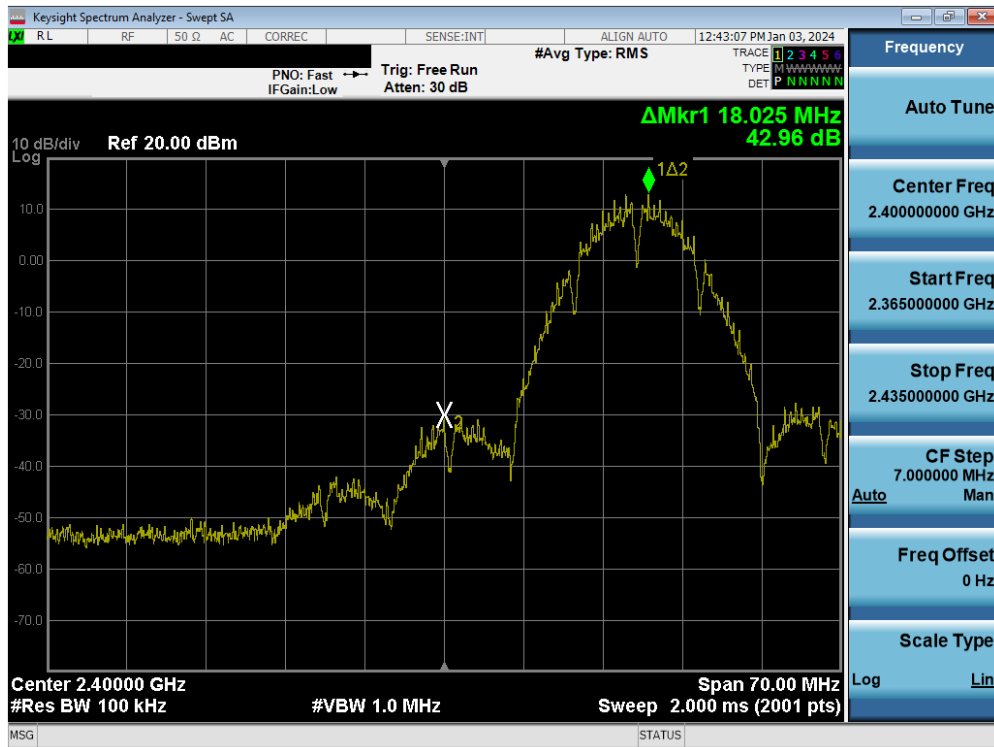
Plot 7-75. Band Edge Plot MIMO ANT1 (802.11b – Ch. 2)
