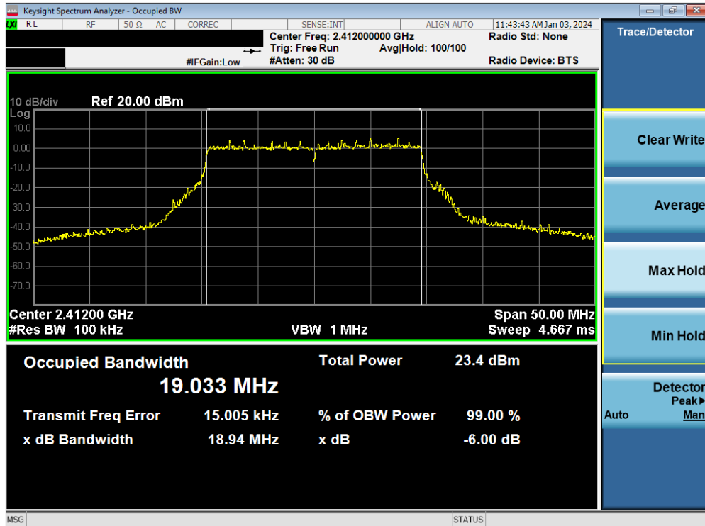
Plot 7-23. 6dB Bandwidth Plot MIMO ANT2 (802.11be (2.4GHz) – Ch. 1)
