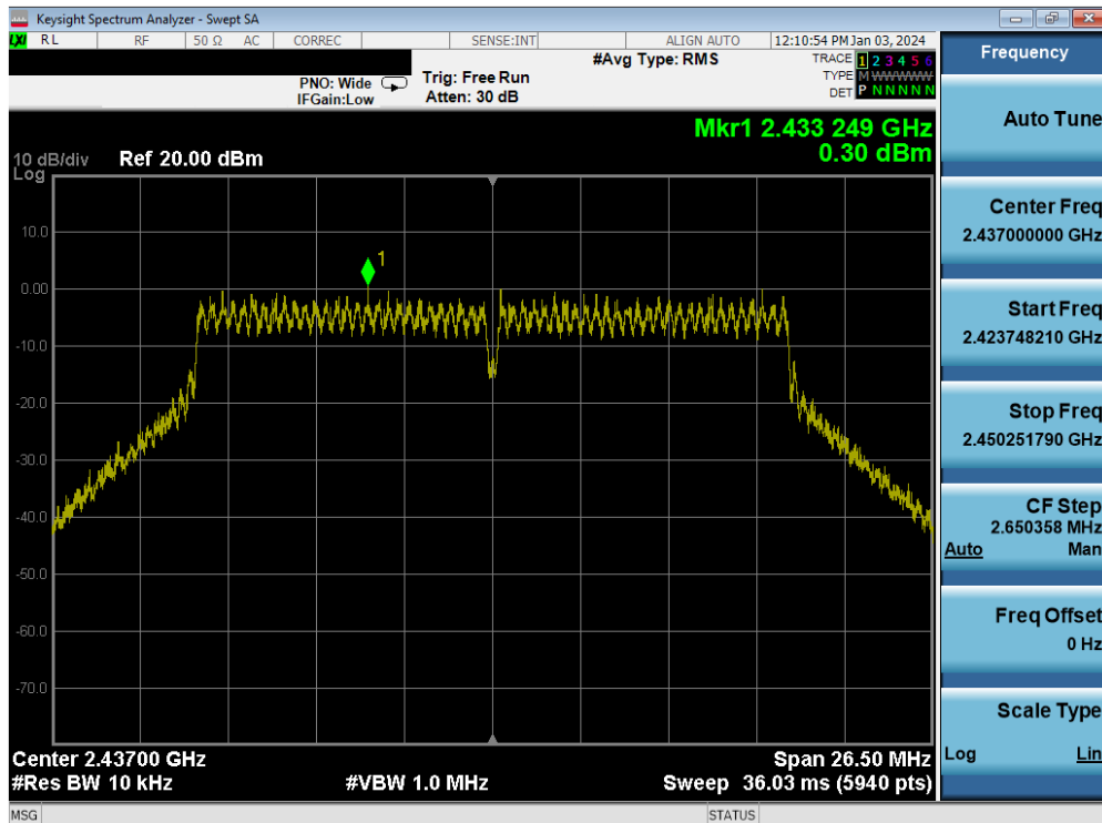
Plot 7-45. Power Spectral Density Plot MIMO ANT1 (802.11n (2.4GHz) – Ch. 6)
