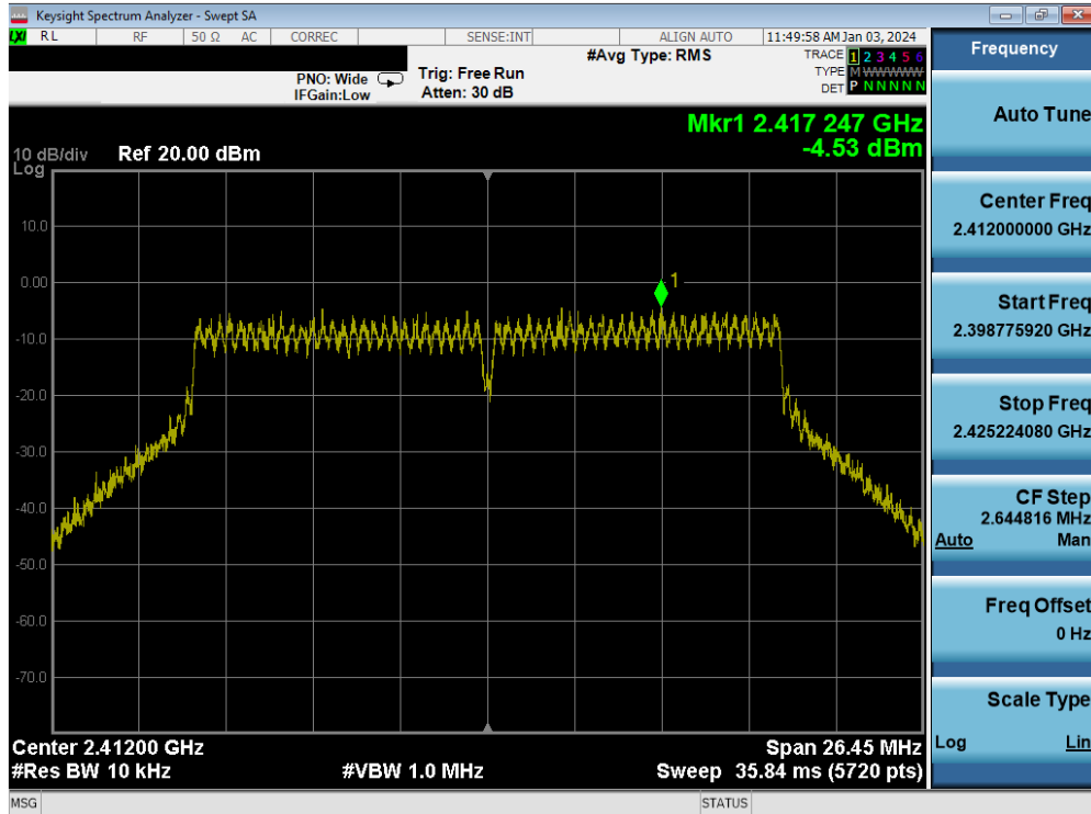
Plot 7-56. Power Spectral Density Plot MIMO ANT2 (802.11n (2.4GHz) – Ch. 1)
