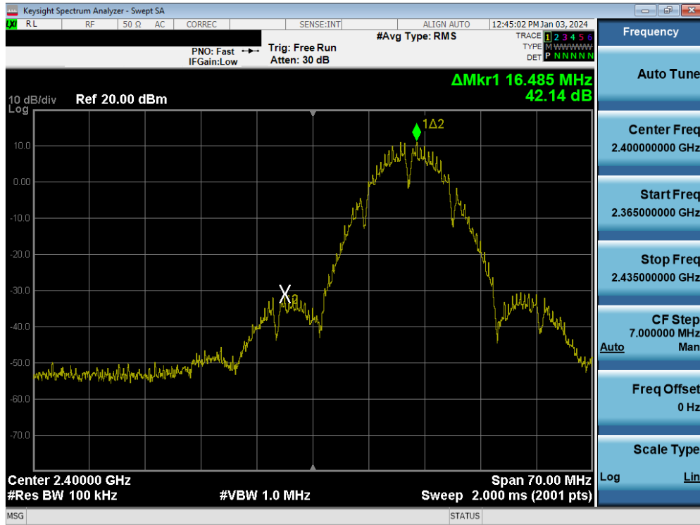
Plot 7-74. Band Edge Plot MIMO ANT1 (802.11b – Ch. 1)
