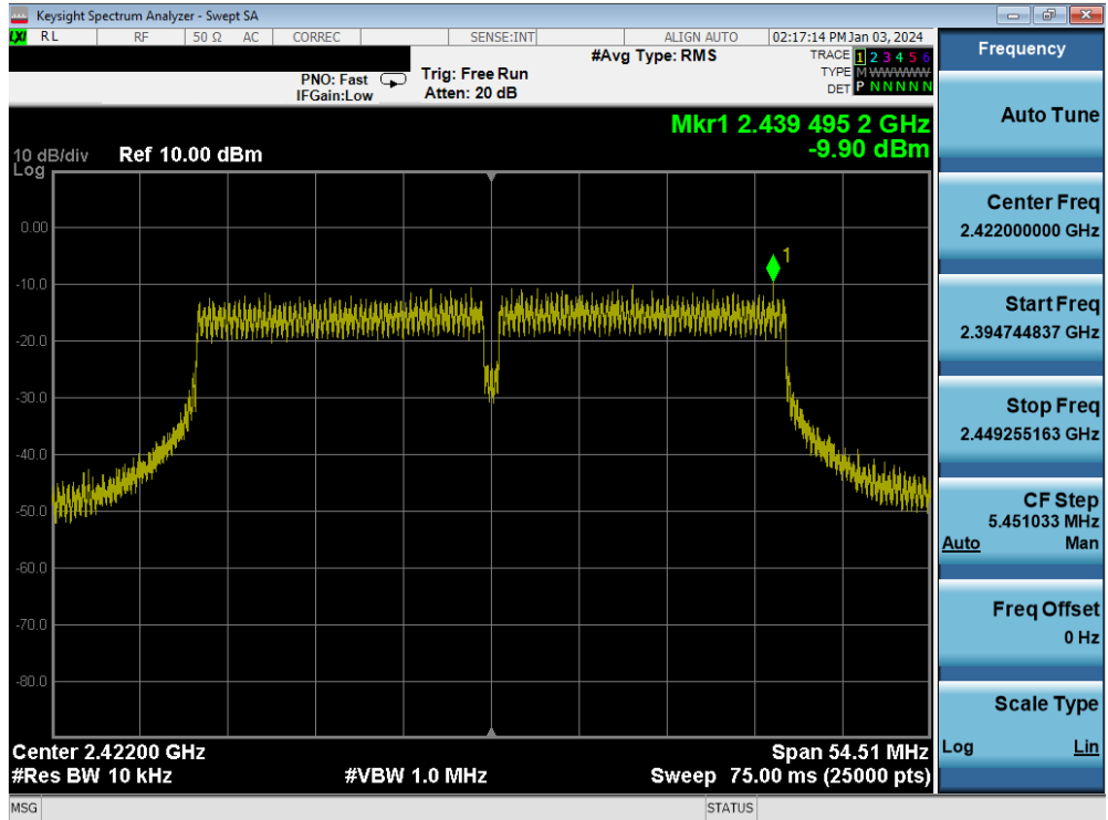
Plot 7-62. Power Spectral Density Plot MIMO ANT1 (802.11n (2.4GHz) – Ch. 3)
