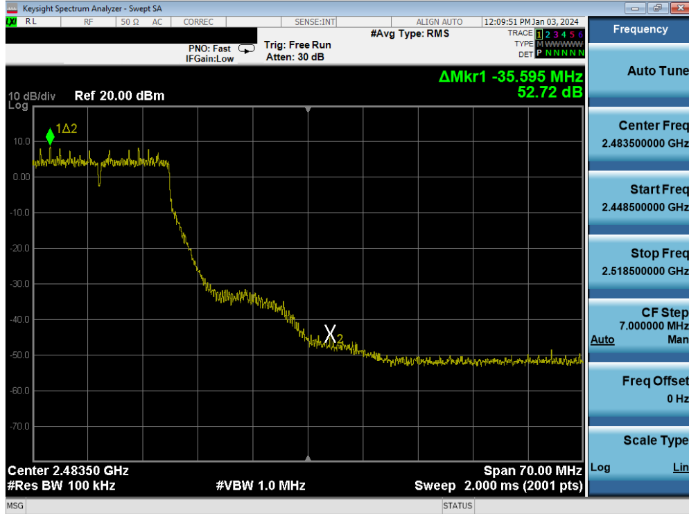
Plot 7-88. Band Edge Plot MIMO ANT1 (802.11n (2.4GHz) – Ch. 10)
