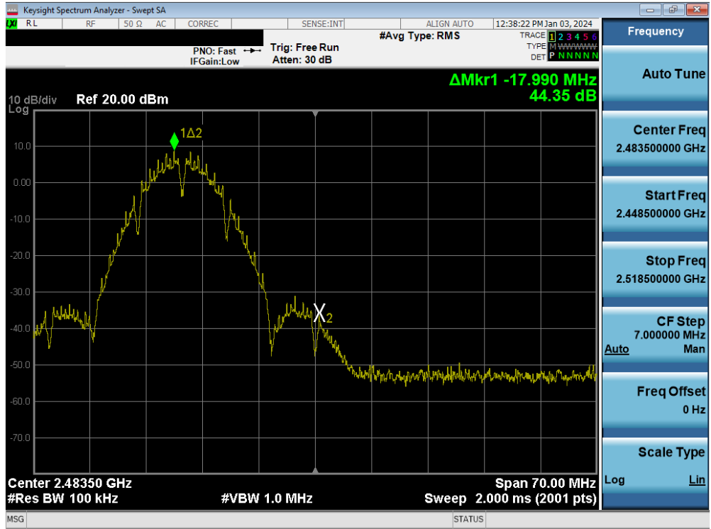
Plot 7-103. Band Edge Plot MIMO ANT2 (802.11b – Ch. 12)
