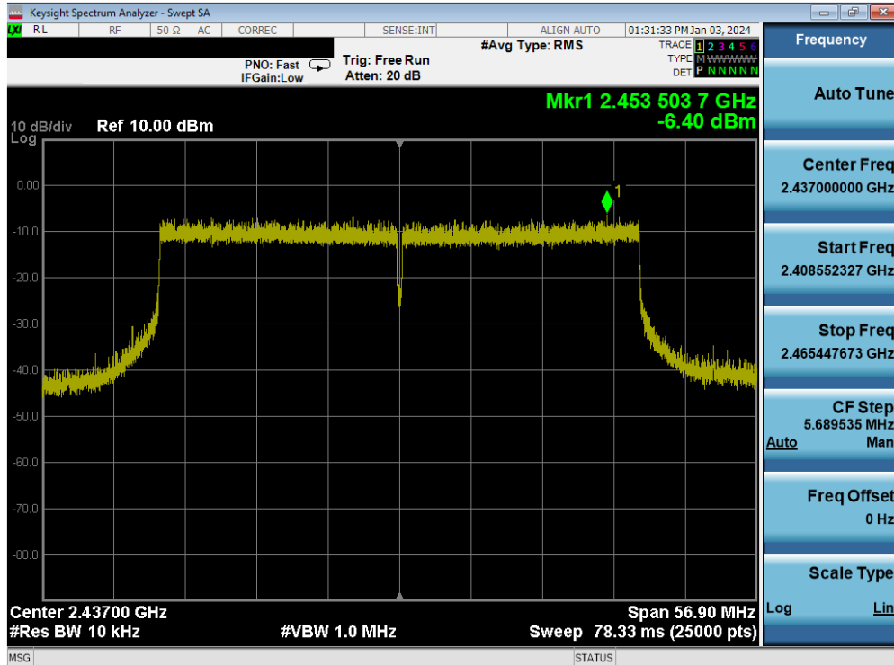
Plot 7-72. Power Spectral Density Plot MIMO ANT2 (802.11be (2.4GHz) – Ch. 6)
