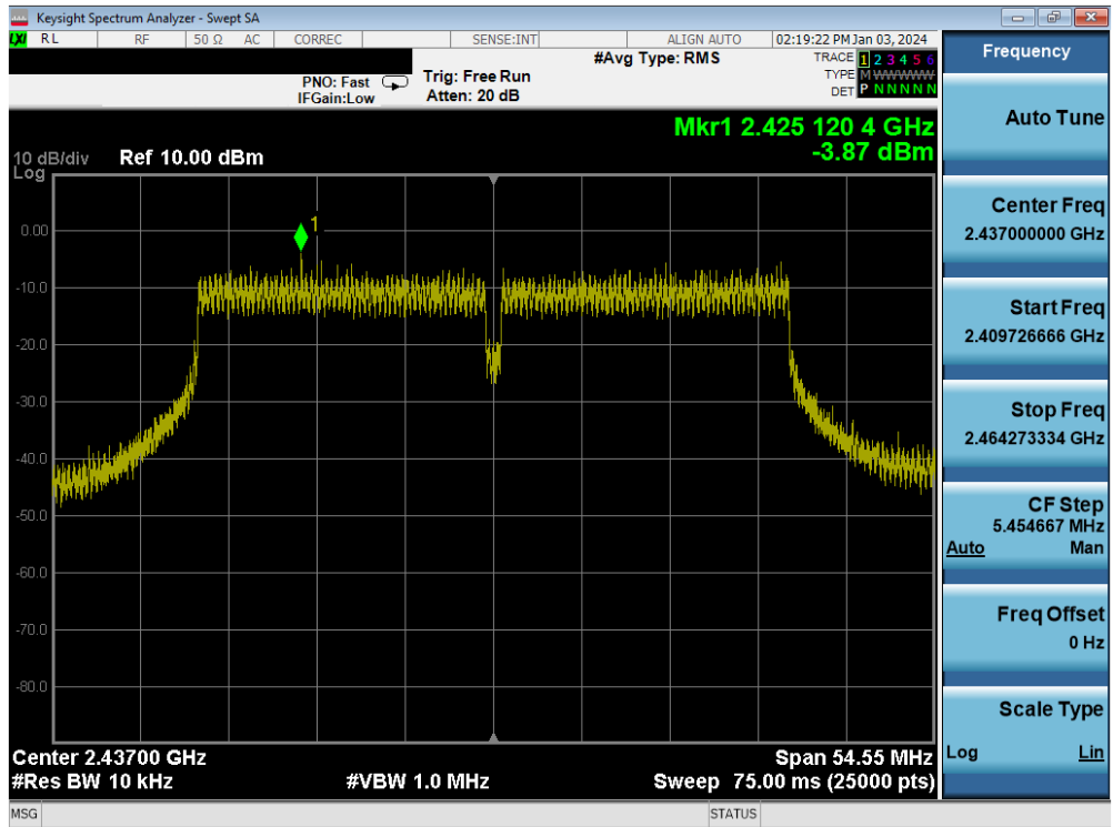
Plot 7-63. Power Spectral Density Plot MIMO ANT1 (802.11n (2.4GHz) – Ch. 6)
