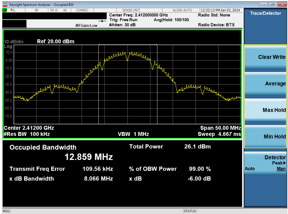
Plot 7-14. 6dB Bandwidth Plot MIMO ANT2 (802.11b – Ch. 1)
