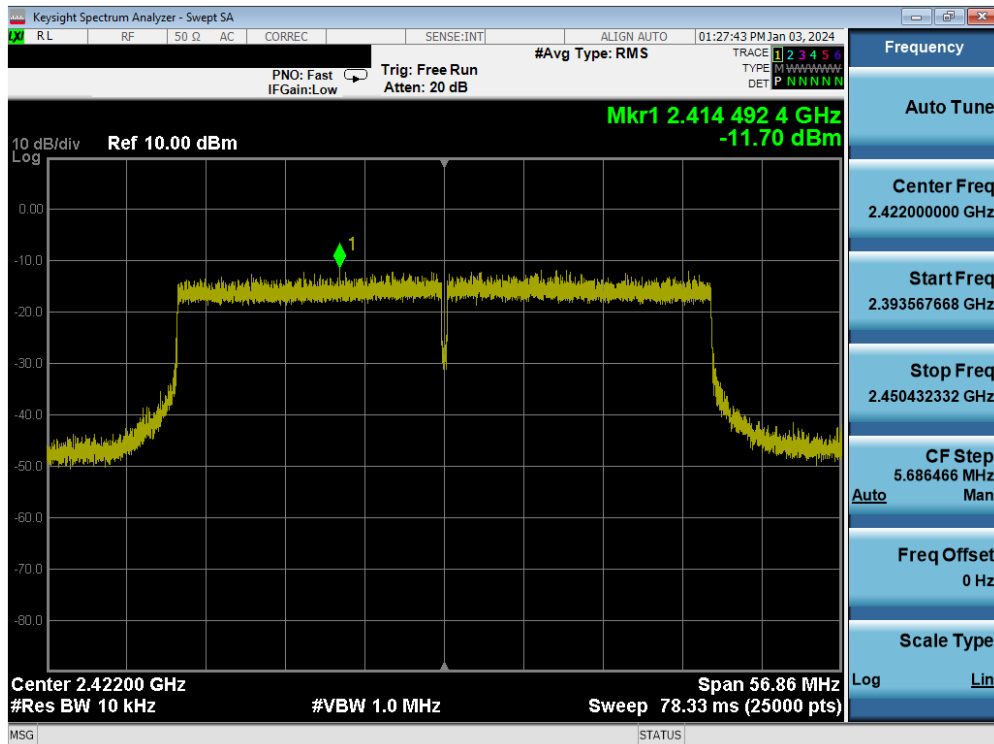
Plot 7-71. Power Spectral Density Plot MIMO ANT2 (802.11be (2.4GHz) – Ch. 3)
