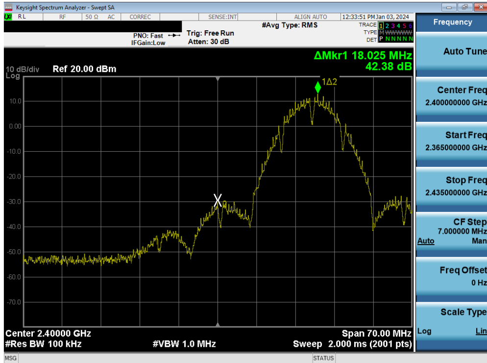
Plot 7-100. Band Edge Plot MIMO ANT2 (802.11b – Ch. 2)
