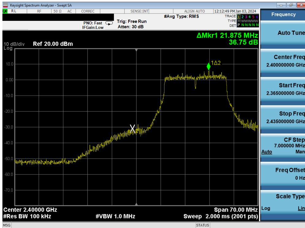
Plot 7-87. Band Edge Plot MIMO ANT1 (802.11n (2.4GHz) – Ch. 2)
