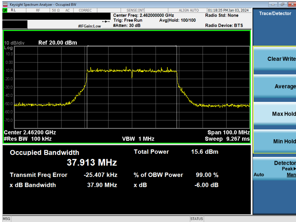
Plot 7-31. 6dB Bandwidth Plot MIMO ANT1 (802.11be (2.4GHz) – Ch. 11)
