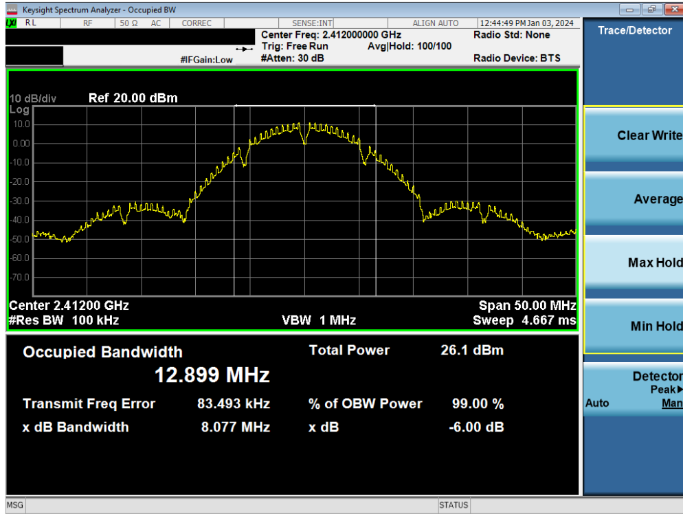
Plot 7-2. 6dB Bandwidth Plot MIMO ANT1 (802.11b – Ch. 1)
