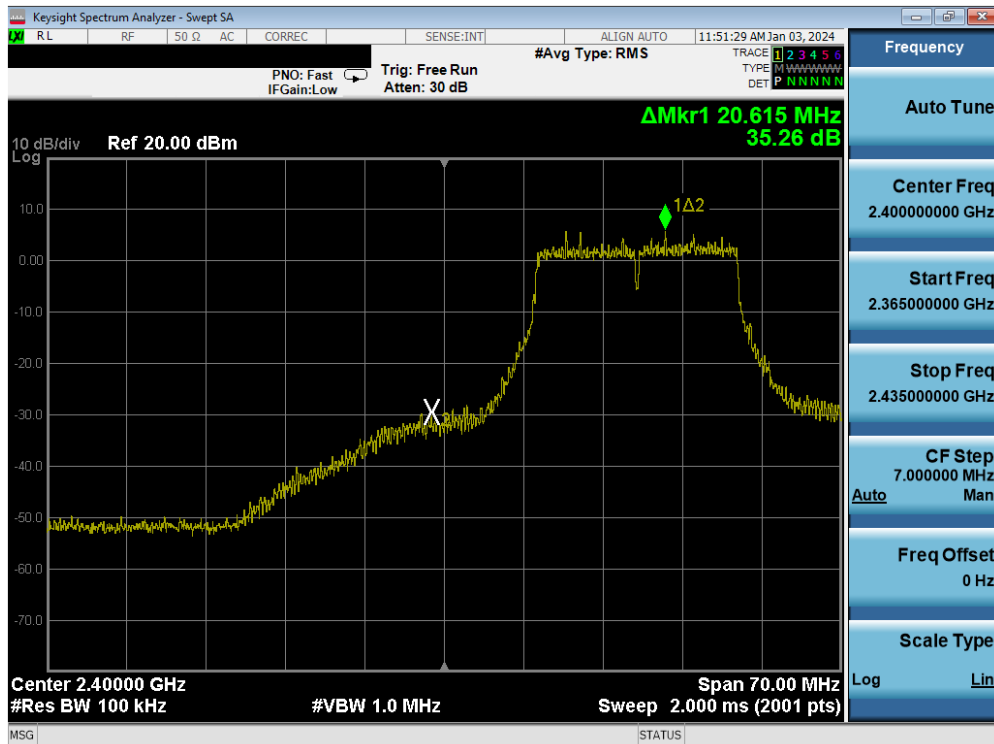
Plot 7-112. Band Edge Plot MIMO ANT2 (802.11n (2.4GHz) – Ch. 2)
