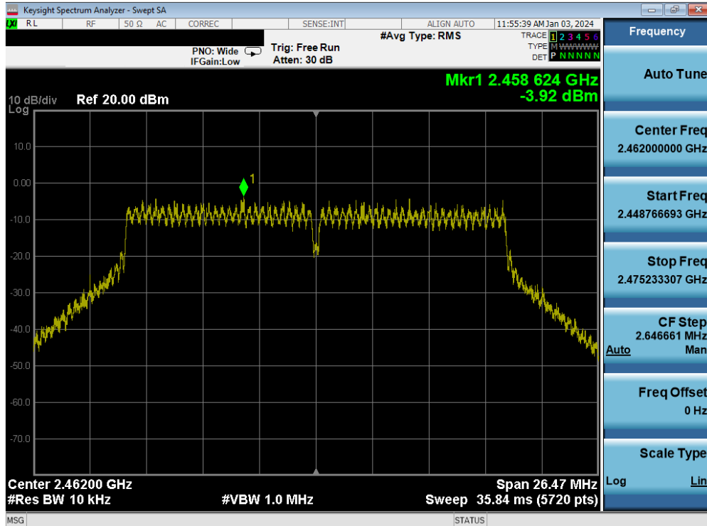
Plot 7-58. Power Spectral Density Plot MIMO ANT2 (802.11n (2.4GHz) – Ch. 11)
