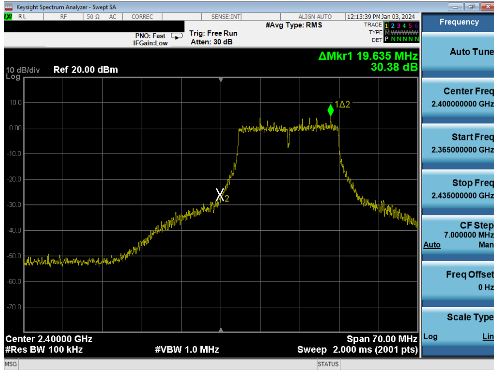
Plot 7-86. Band Edge Plot MIMO ANT1 (802.11n (2.4GHz) – Ch. 1)
