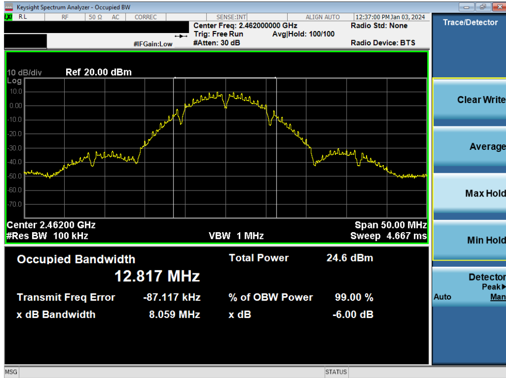
Plot 7-16. 6dB Bandwidth Plot MIMO ANT2 (802.11b – Ch. 11)
