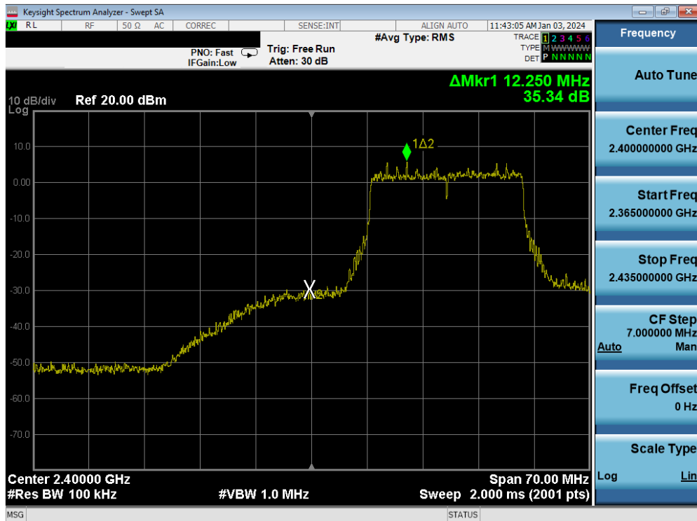
Plot 7-118. Band Edge Plot MIMO ANT2 (802.11be (2.4GHz) – Ch. 2)
