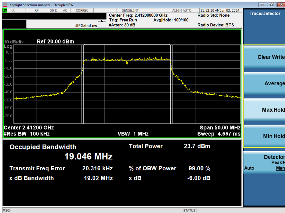
Plot 7-11. 6dB Bandwidth Plot MIMO ANT1 (802.11be (2.4GHz) – Ch. 1)
