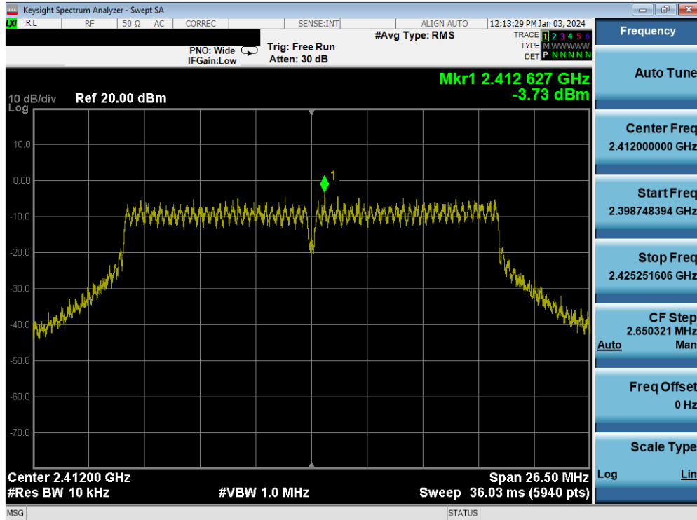
Plot 7-44. Power Spectral Density Plot MIMO ANT1 (802.11n (2.4GHz) – Ch. 1)
