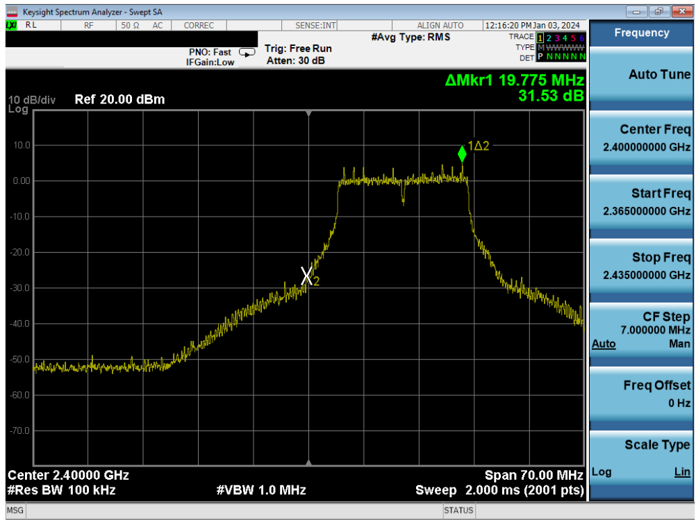
Plot 7-81. Band Edge Plot MIMO ANT1 (802.11g– Ch. 2)
