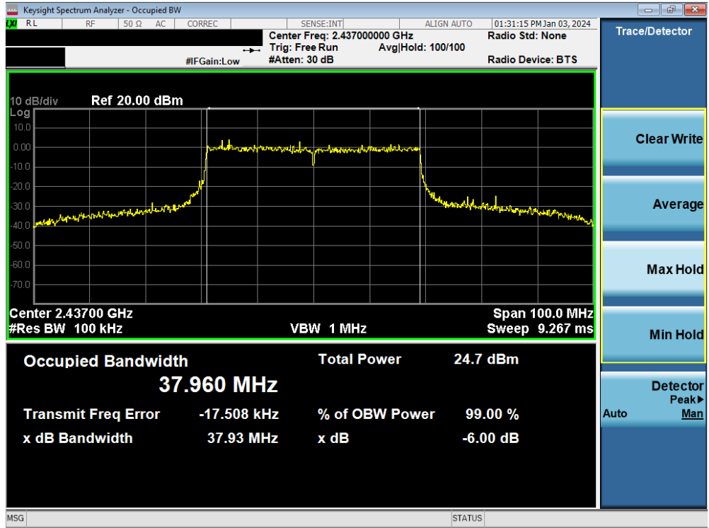
Plot 7-36. 6dB Bandwidth Plot MIMO ANT2 (802.11be (2.4GHz) – Ch. 6)
