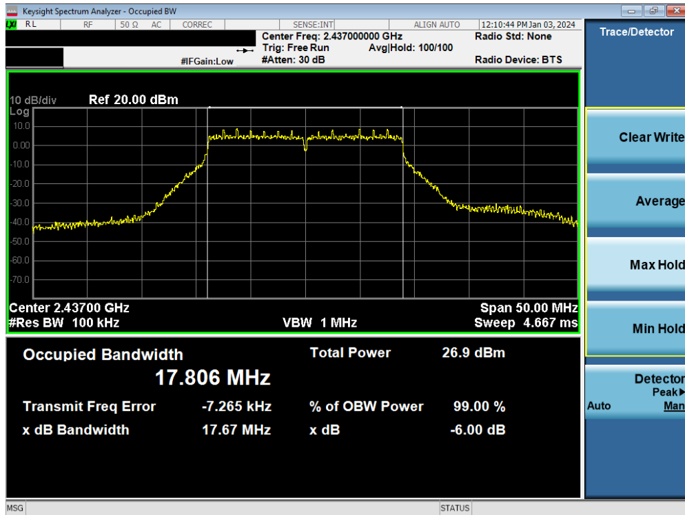
Plot 7-9. 6dB Bandwidth Plot MIMO ANT1 (802.11n (2.4GHz) – Ch. 6)
