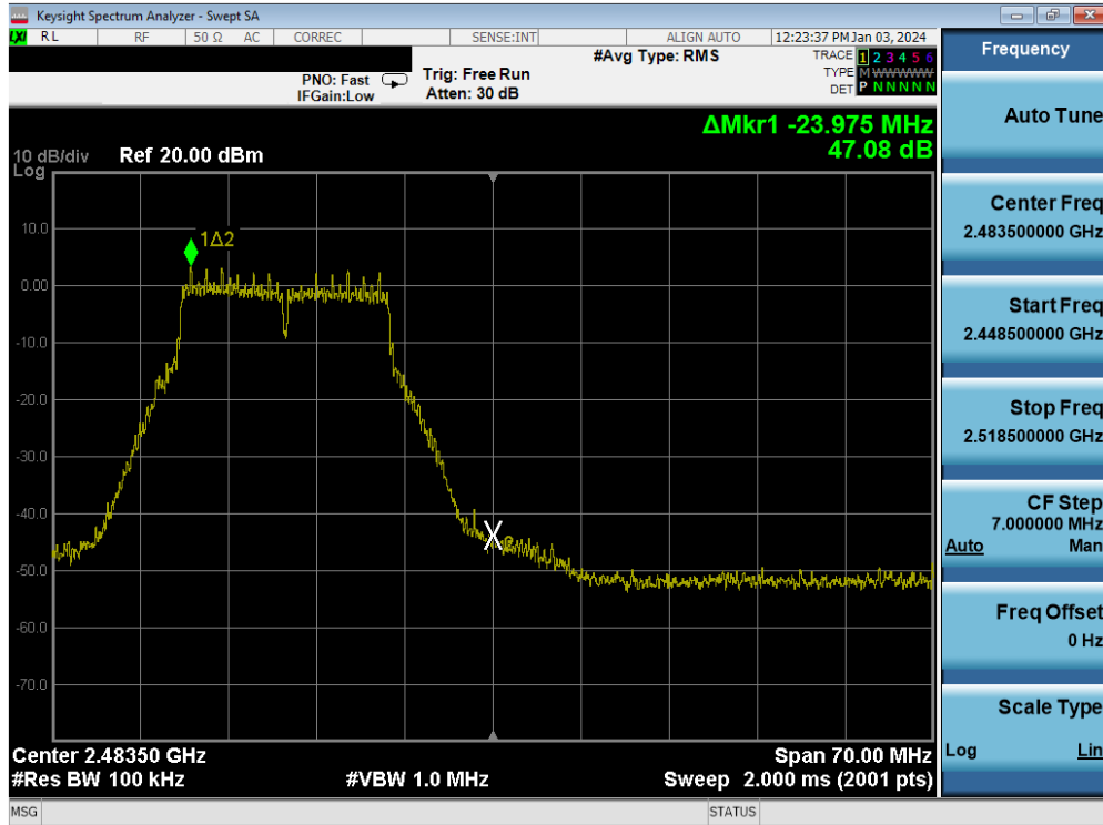
Plot 7-109. Band Edge Plot MIMO ANT2 (802.11g – Ch. 12)
