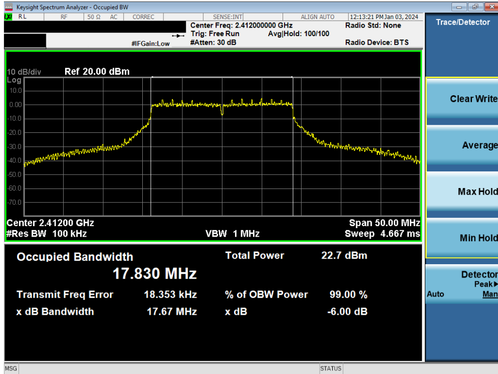
Plot 7-8. 6dB Bandwidth Plot MIMO ANT1 (802.11n (2.4GHz) – Ch. 1)
