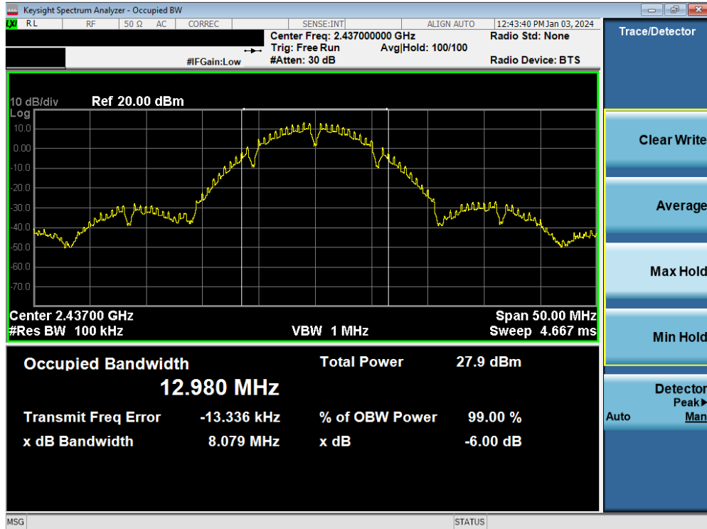
Plot 7-3. 6dB Bandwidth Plot MIMO ANT1 (802.11b – Ch. 6)
