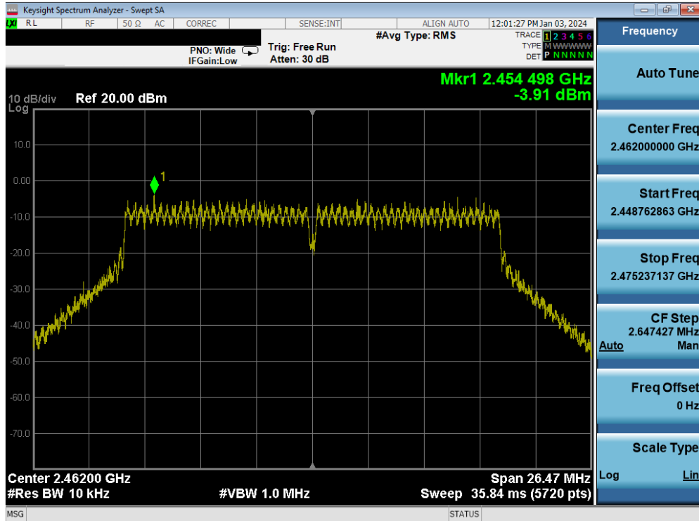
Plot 7-46. Power Spectral Density Plot MIMO ANT1 (802.11n (2.4GHz) – Ch. 11)
