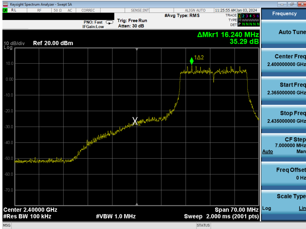
Plot 7-94. Band Edge Plot MIMO ANT1 (802.11be (2.4GHz) – Ch. 3)
