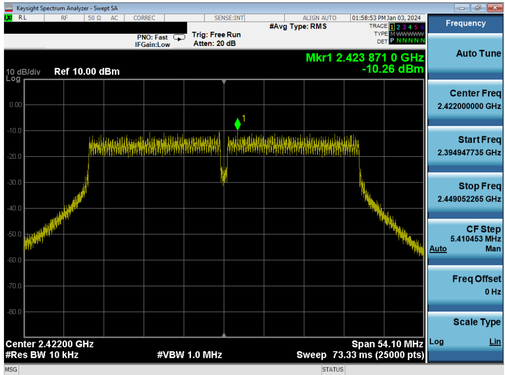
Plot 7-68. Power Spectral Density Plot MIMO ANT2 (802.11n (2.4GHz) – Ch. 3)
