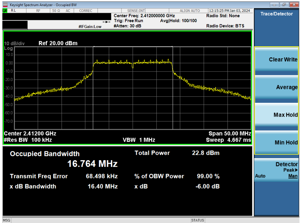
Plot 7-5. 6dB Bandwidth Plot MIMO ANT1 (802.11g – Ch. 1)
