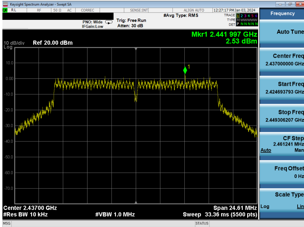
Plot 7-54. Power Spectral Density Plot MIMO ANT2 (802.11g – Ch. 6)
