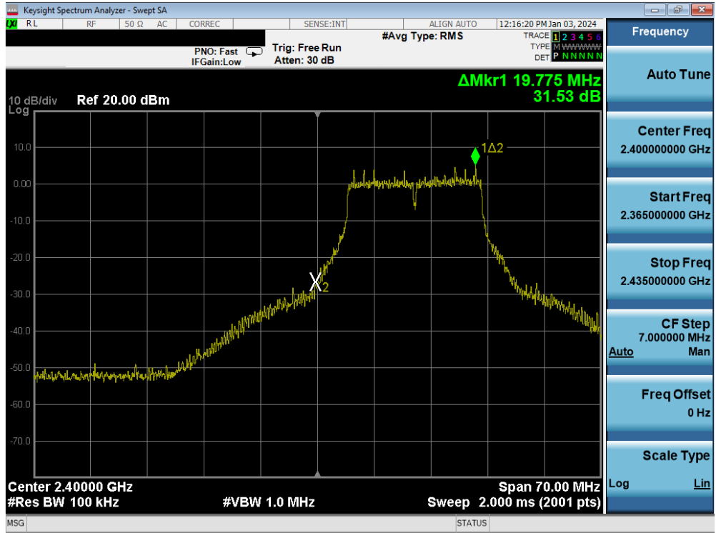
Plot 7-80. Band Edge Plot MIMO ANT1 (802.11g– Ch. 1)
