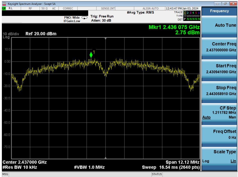
Plot 7-39. Power Spectral Density Plot MIMO ANT1 (802.11b – Ch. 6)
