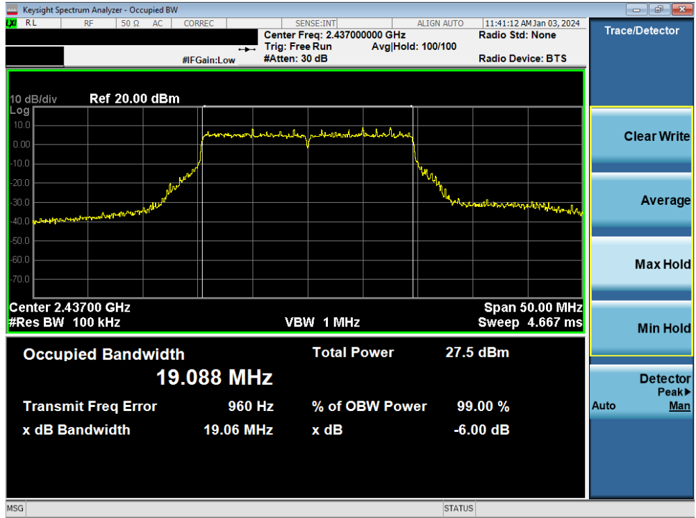
Plot 7-24. 6dB Bandwidth Plot MIMO ANT2 (802.11be (2.4GHz) – Ch. 6)
