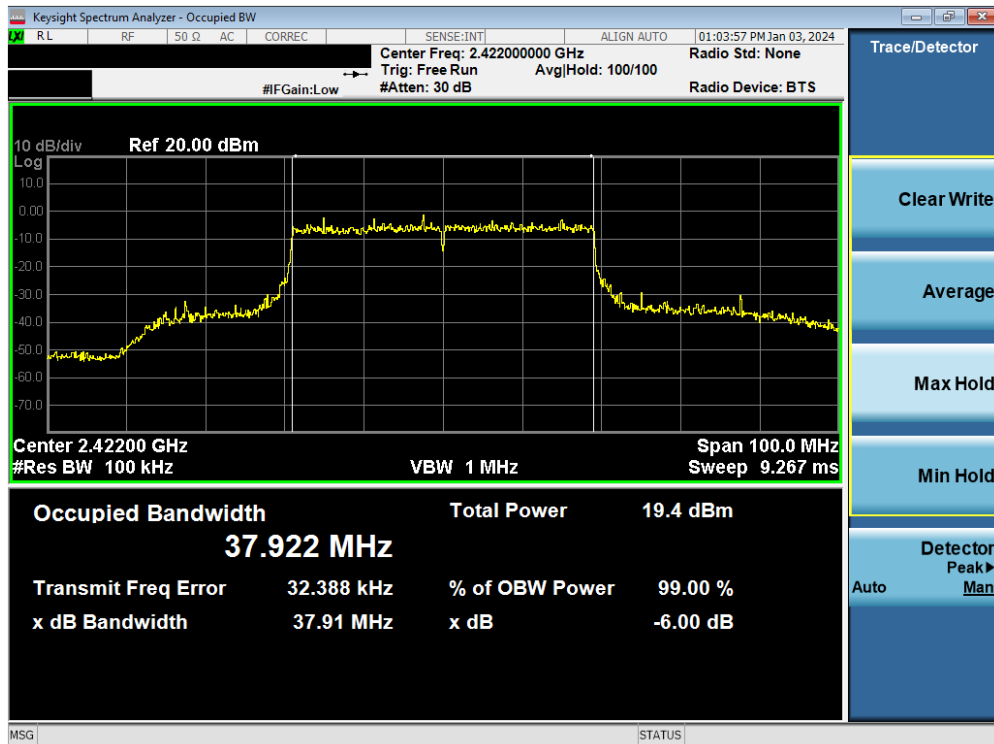
Plot 7-29. 6dB Bandwidth Plot MIMO ANT1 (802.11be (2.4GHz) – Ch. 3)
