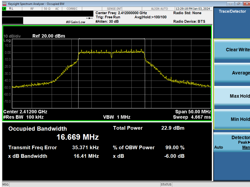
Plot 7-17. 6dB Bandwidth Plot MIMO ANT2 (802.11g – Ch. 1)
