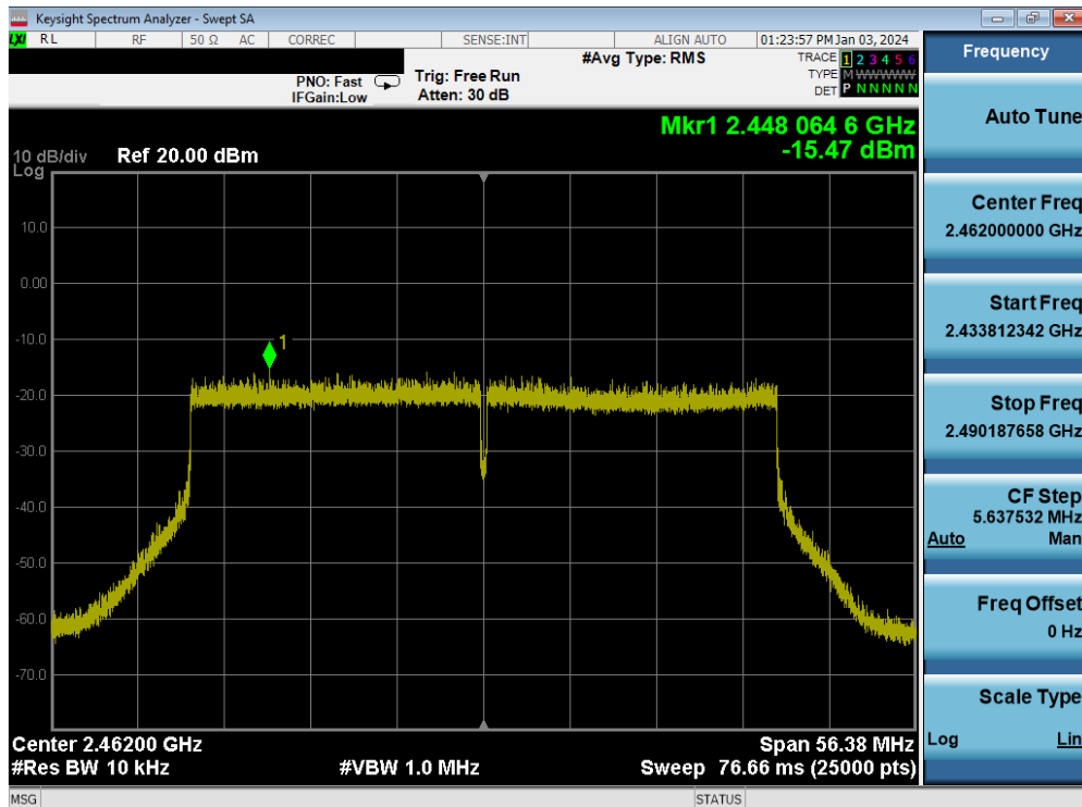
Plot 7-73. Power Spectral Density Plot MIMO ANT2 (802.11be (2.4GHz) – Ch. 11)
