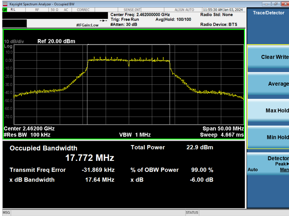
Plot 7-22. 6dB Bandwidth Plot MIMO ANT2 (802.11n (2.4GHz) – Ch. 11)
