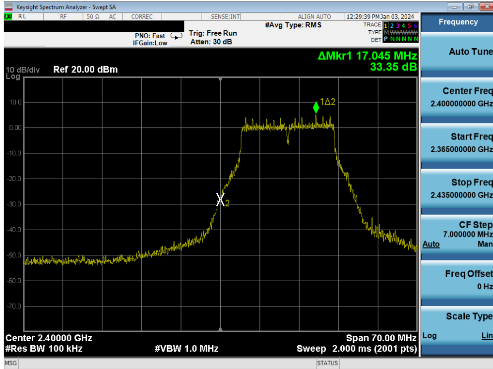
Plot 7-105. Band Edge Plot MIMO ANT2 (802.11g- Ch. 1)
