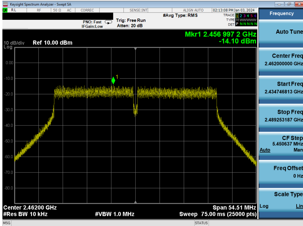
Plot 7-64. Power Spectral Density Plot MIMO ANT1 (802.11n (2.4GHz) – Ch. 11)
