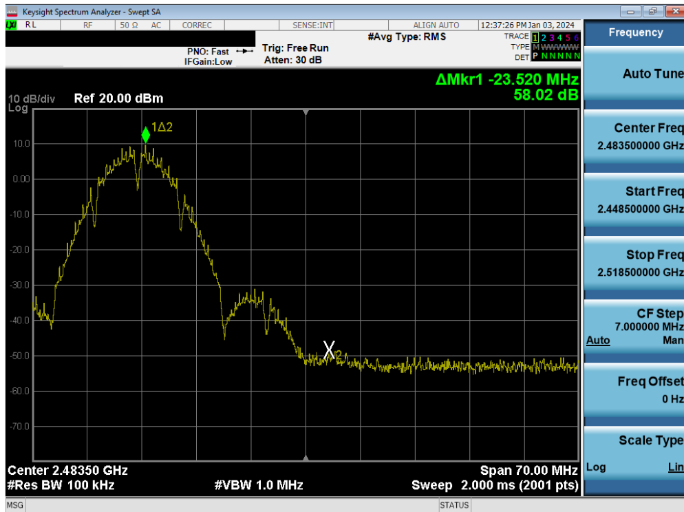
Plot 7-102. Band Edge Plot MIMO ANT2 (802.11b – Ch. 11)
