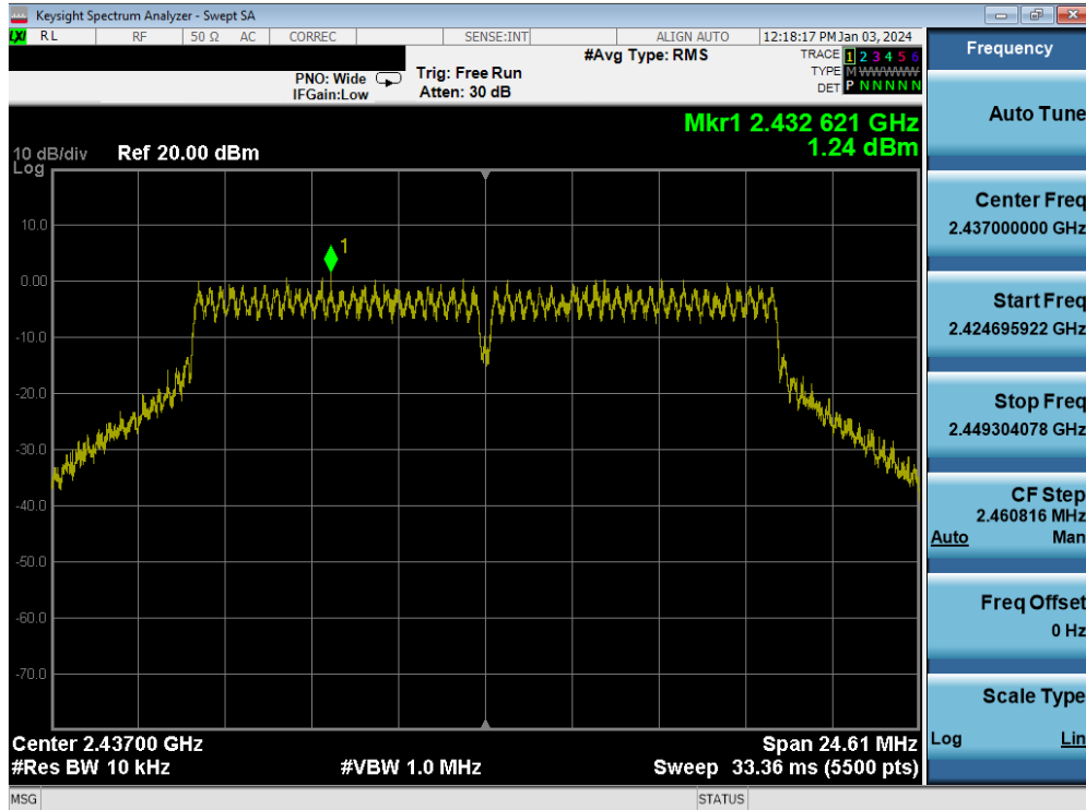
Plot 7-42. Power Spectral Density Plot MIMO ANT1 (802.11g – Ch. 6)
