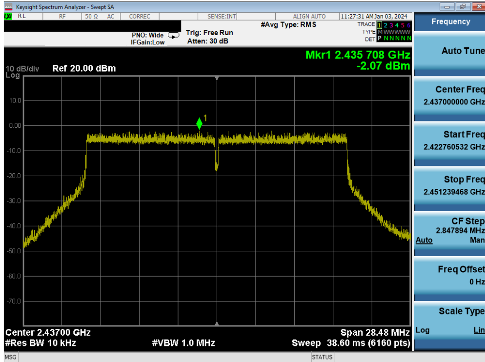
Plot 7-48. Power Spectral Density Plot MIMO ANT1 (802.11be (2.4GHz) – Ch. 6)
