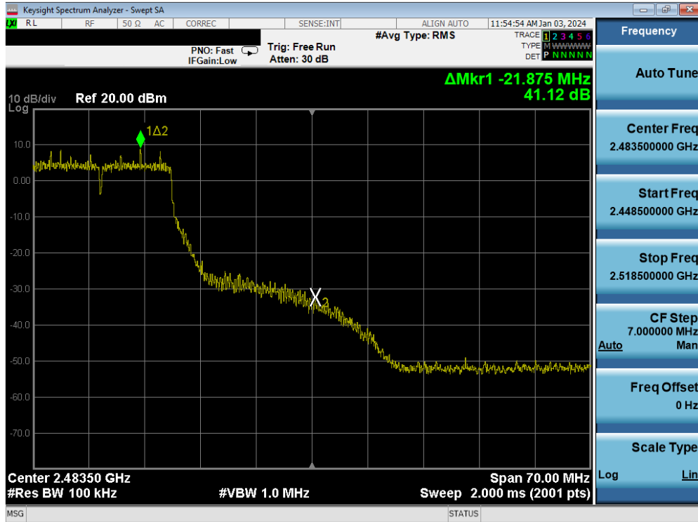
Plot 7-113. Band Edge Plot MIMO ANT2 (802.11n (2.4GHz) – Ch. 10)
