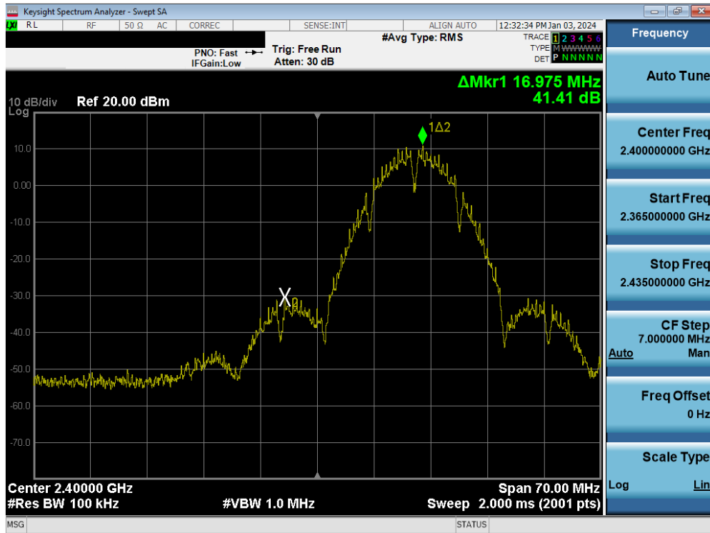
Plot 7-99. Band Edge Plot MIMO ANT2 (802.11b – Ch. 1)
