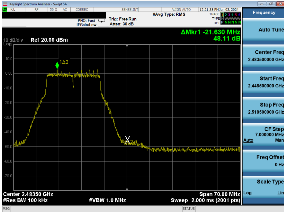
Plot 7-84. Band Edge Plot MIMO ANT1 (802.11g – Ch. 12)
