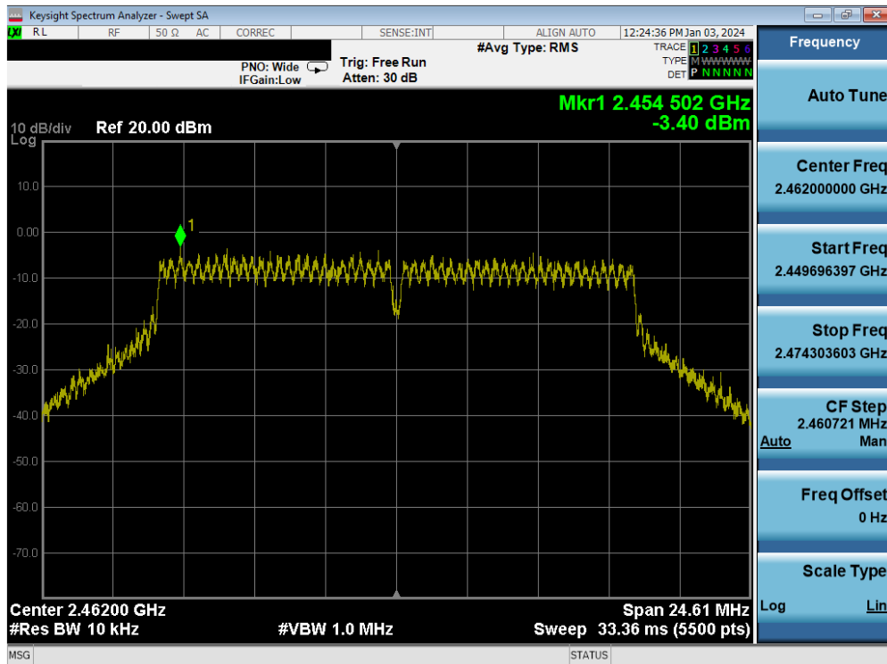
Plot 7-55. Power Spectral Density Plot MIMO ANT2 (802.11g – Ch. 11)
