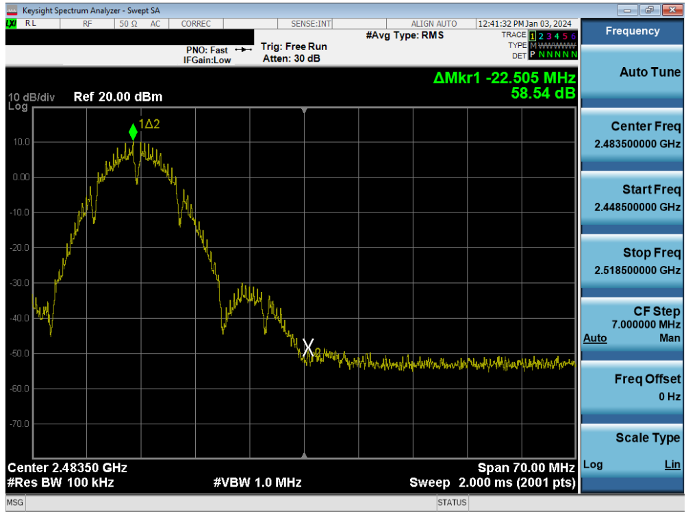
Plot 7-77. Band Edge Plot MIMO ANT1 (802.11b – Ch. 11)
