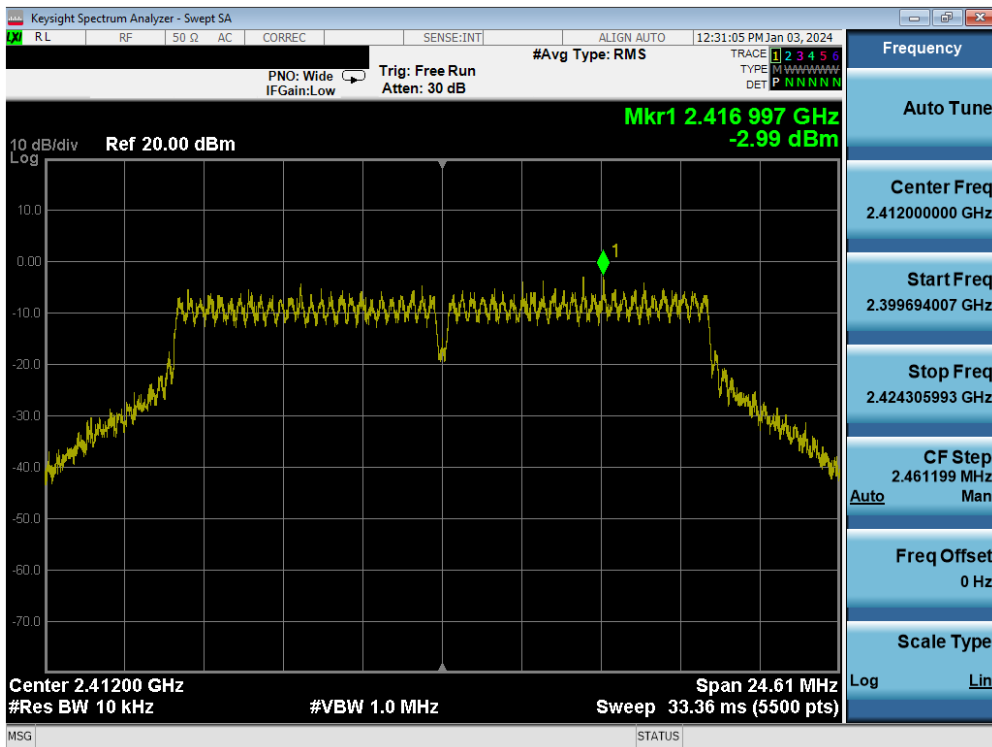
Plot 7-53. Power Spectral Density Plot MIMO ANT2 (802.11g – Ch. 1)
