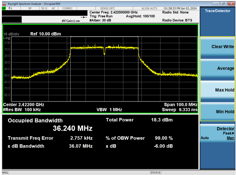
Plot 7-32. 6dB Bandwidth Plot MIMO ANT2 (802.11n (2.4GHz) – Ch. 3)
