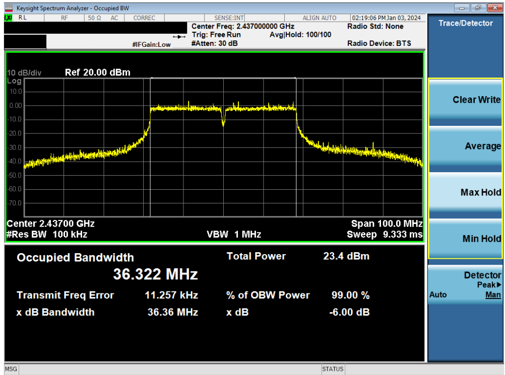
Plot 7-27. 6dB Bandwidth Plot MIMO ANT1 (802.11n (2.4GHz) – Ch. 6)
