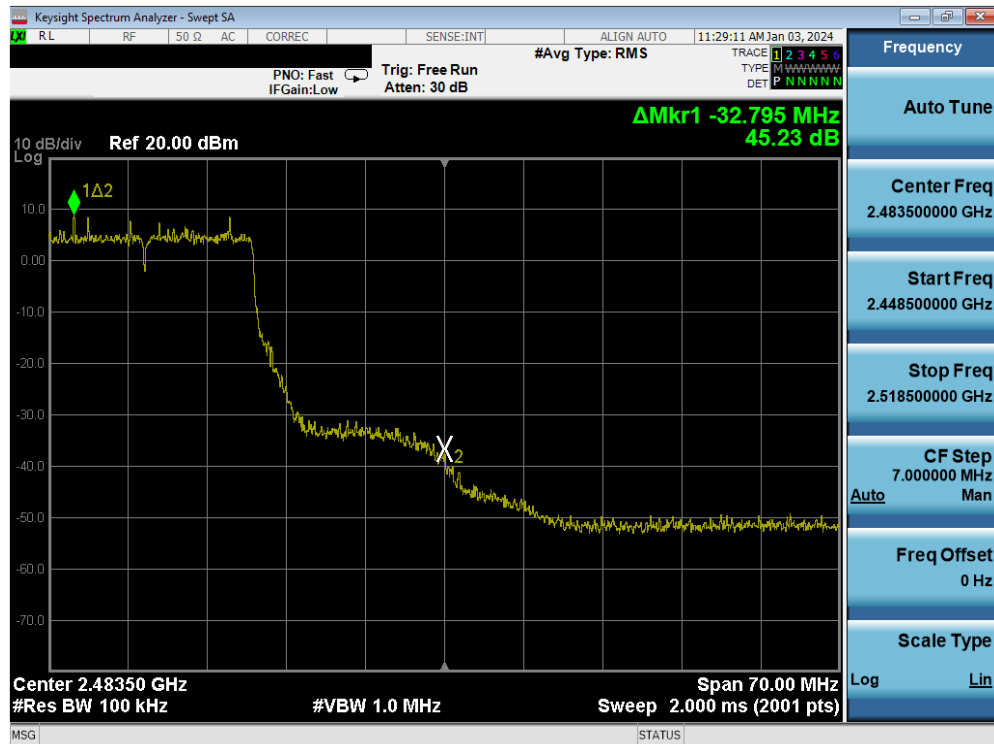
Plot 7-95. Band Edge Plot MIMO ANT1 (802.11be (2.4GHz) – Ch. 10)
