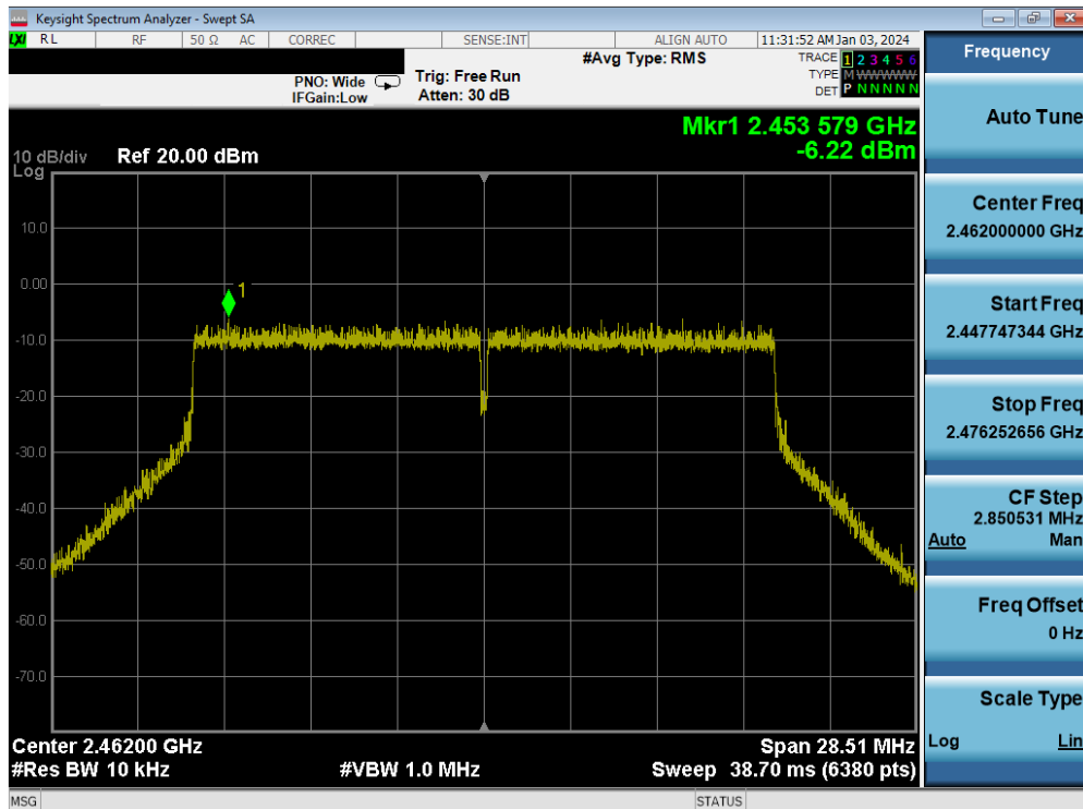
Plot 7-49. Power Spectral Density Plot MIMO ANT1 (802.11be (2.4GHz) – Ch. 11)
