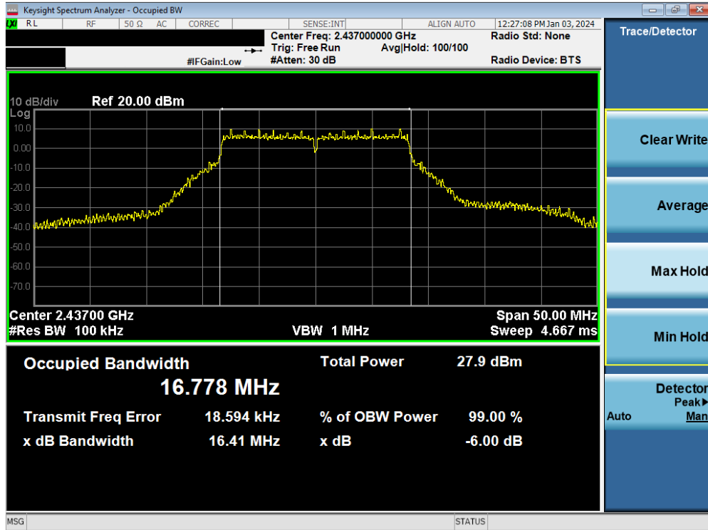
Plot 7-18. 6dB Bandwidth Plot MIMO ANT2 (802.11g – Ch. 6)
