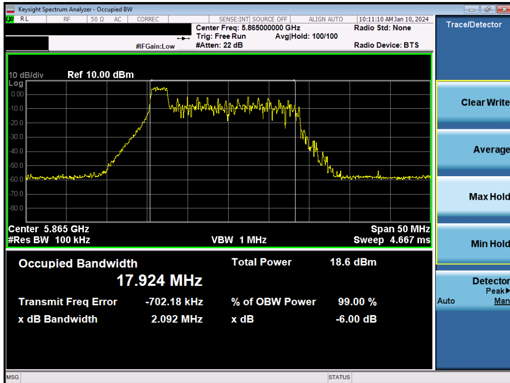
Plot 7-64. 6dB Bandwidth Plot MIMO ANT2 (20MHz BW 802.11be – 26 Tones (UNII Band 4) – Ch. 173)
