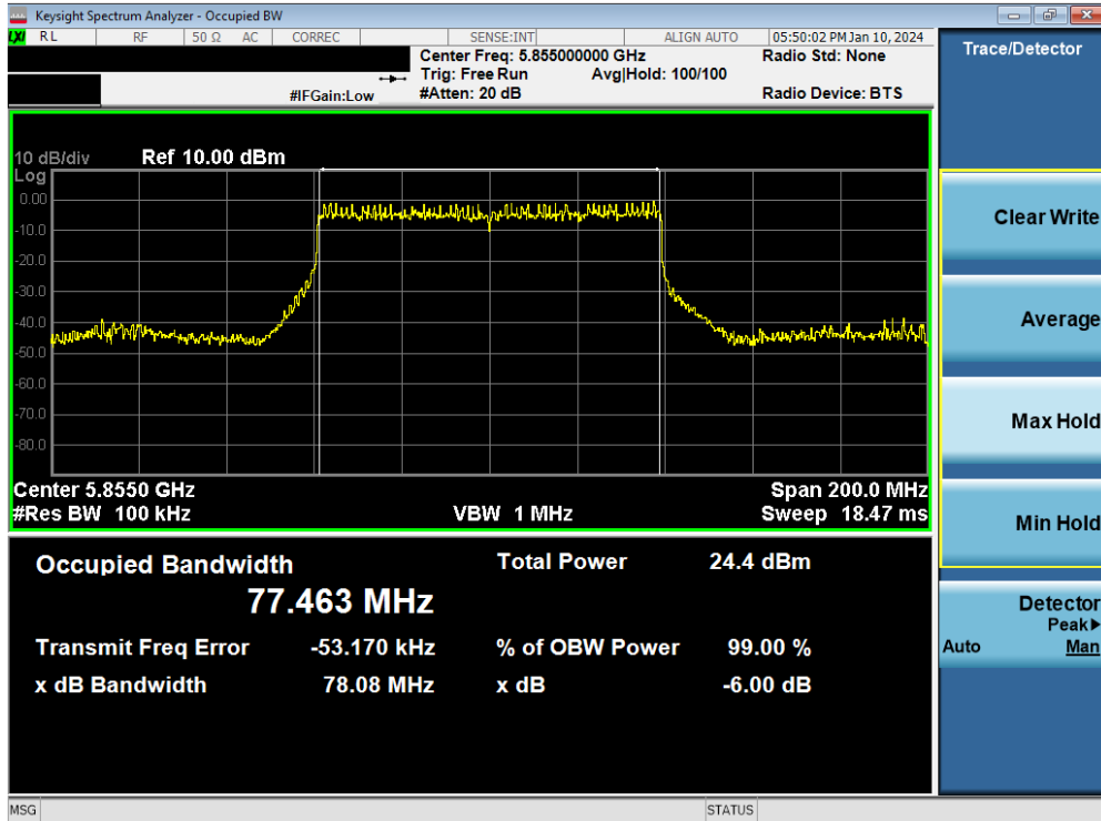
Plot 7-59. 6dB Bandwidth Plot MIMO ANT1 (80MHz BW 802.11be – 996 Tones (UNII Band 3/4) – Ch. 171)
