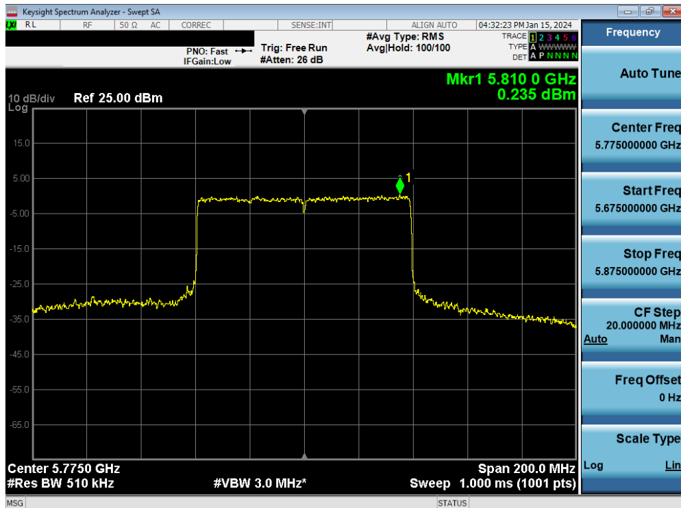
Plot 7-106. Power Spectral Density Plot MIMO ANT1 (80MHz BW 802.11be – 996 Tones (UNII Band 3) – Ch. 155)
