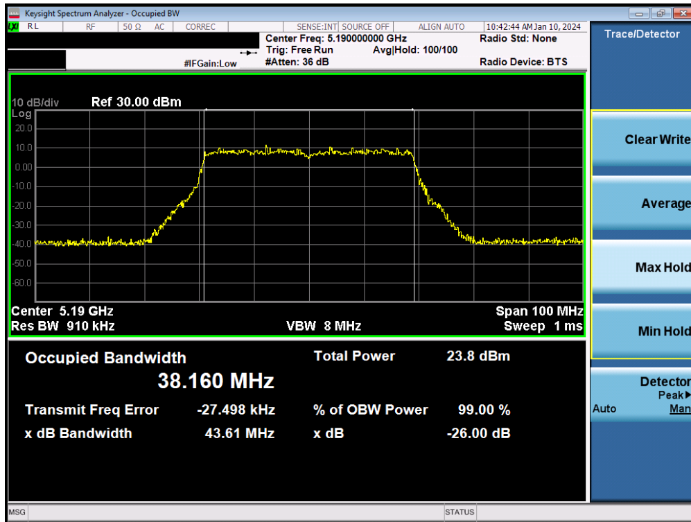
Plot 7-37. 26dB Bandwidth Plot MIMO ANT2 (40MHz BW 802.11be – 484 Tones (UNII Band 1) – Ch. 38)
