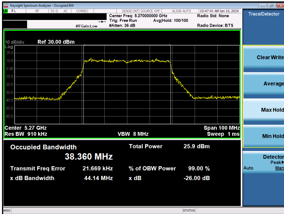
Plot 7-41. 26dB Bandwidth Plot MIMO ANT2 (40MHz BW 802.11be – 484 Tones (UNII Band 2A) – Ch. 54)
