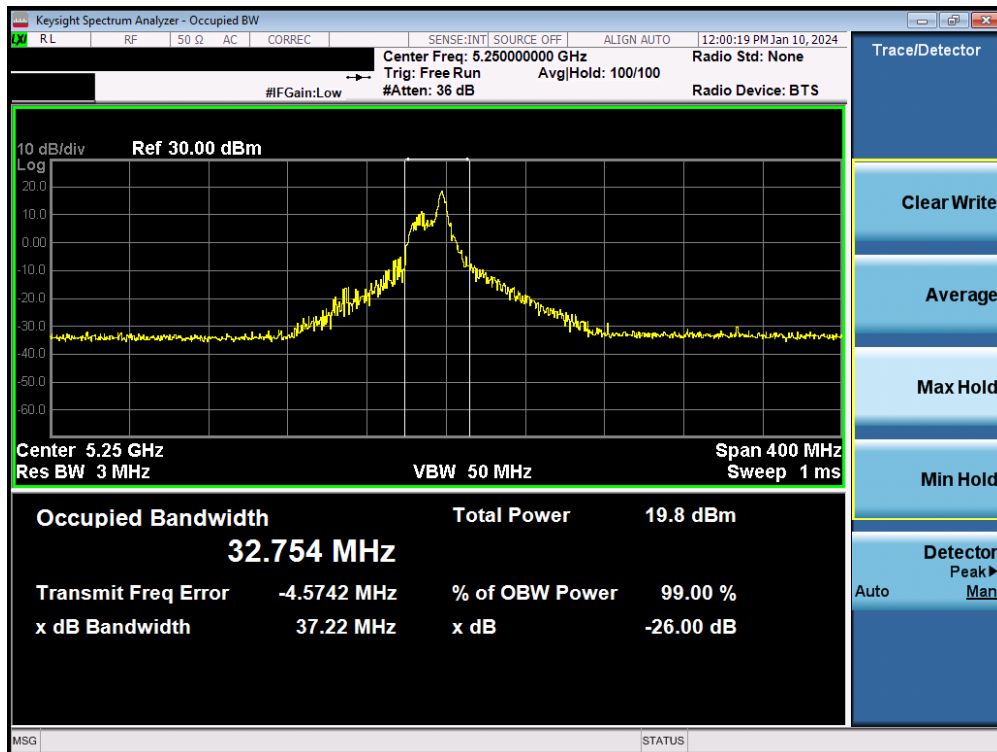
Plot 7-28. 26dB Bandwidth Plot MIMO ANT2 (160MHz(U) BW 802.11be – 26 Tones (UNII Band 1/2A) – Ch. 50)
