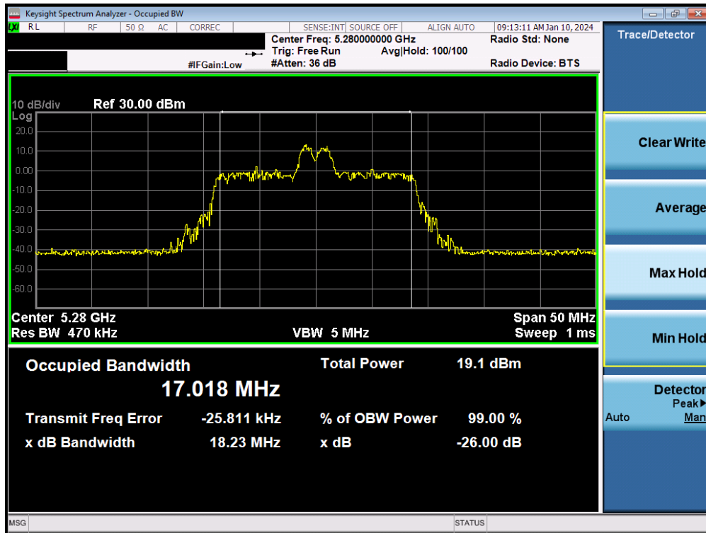
Plot 7-29. 26dB Bandwidth Plot MIMO ANT2 (20MHz BW 802.11be – 26 Tones (UNII Band 2A) – Ch. 56)
