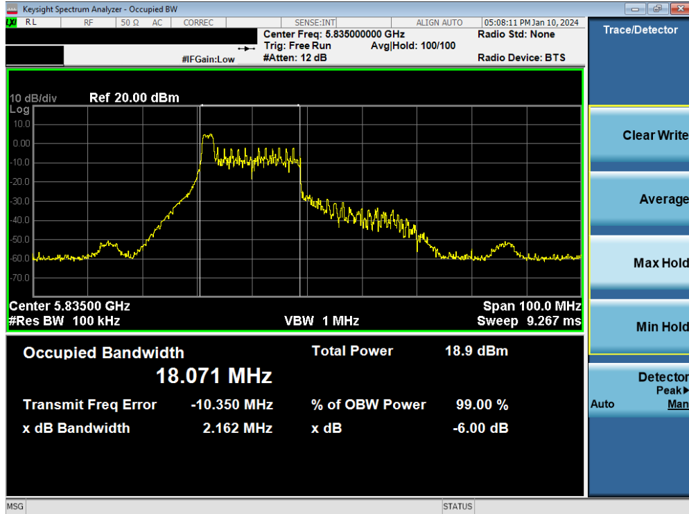
Plot 7-51. 6dB Bandwidth Plot MIMO ANT1 (40MHz BW 802.11be – 26 Tones (UNII Band 3/4) – Ch. 167)
