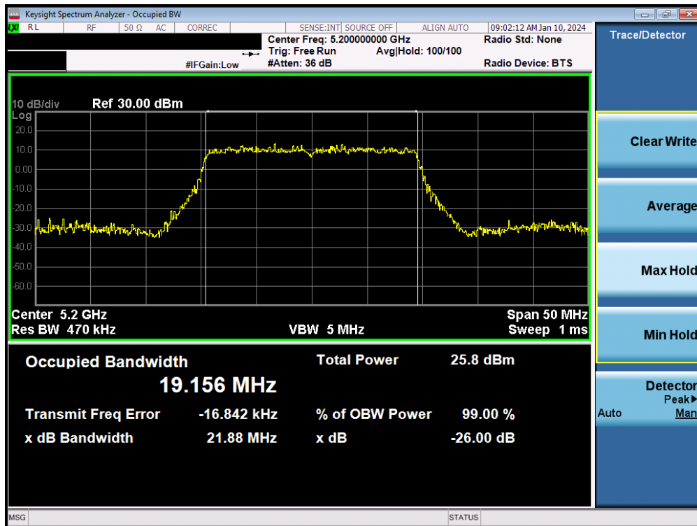
Plot 7-36. 26dB Bandwidth Plot MIMO ANT2 (20MHz BW 802.11be – 242 Tones (UNII Band 1) – Ch. 40)
