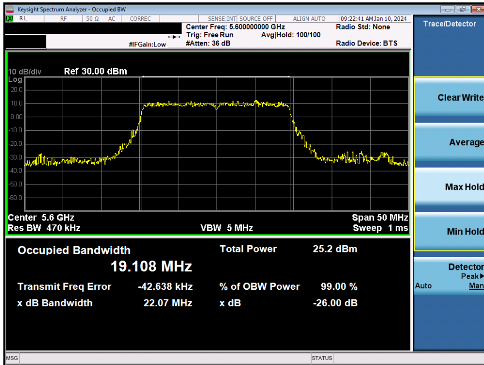
Plot 7-43. 26dB Bandwidth Plot MIMO ANT2 (20MHz BW 802.11be – 242 Tones (UNII Band 2C) – Ch. 120)
