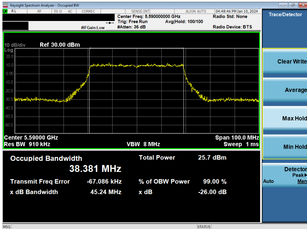
Plot 7-22. 26dB Bandwidth Plot MIMO ANT1 (40MHz BW 802.11be – 484 Tones (UNII Band 2C) – Ch. 118)
