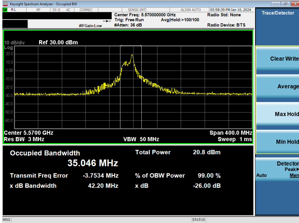
Plot 7-13. 26dB Bandwidth Plot MIMO ANT1 (160MHz BW 802.11be – 26 Tones (UNII Band 2C) – Ch. 114)
