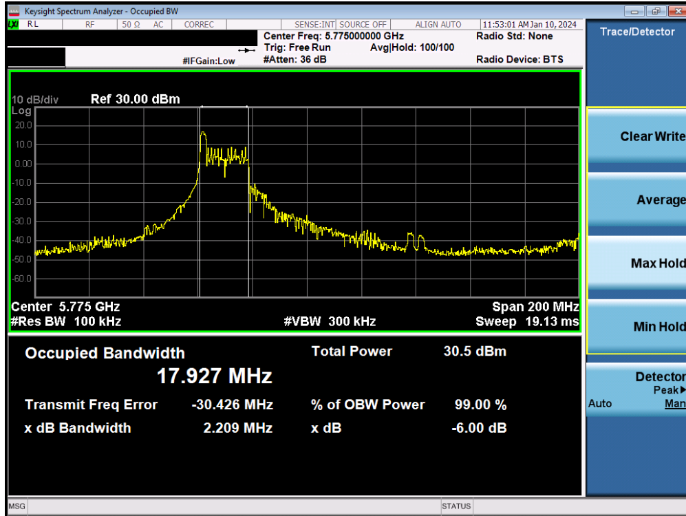
Plot 7-63. 6dB Bandwidth Plot MIMO ANT2 (80MHz BW 802.11be – 26 Tones (UNII Band 3) – Ch. 155)
