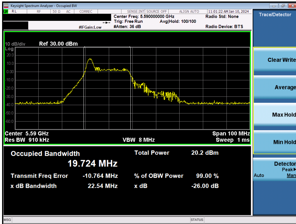
Plot 7-33. 26dB Bandwidth Plot MIMO ANT2 (40MHz BW 802.11be – 26 Tones (UNII Band 2C) – Ch. 118)
