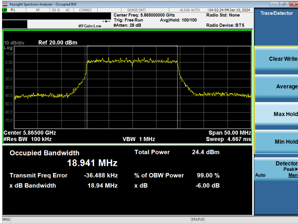
Plot 7-57. 6dB Bandwidth Plot MIMO ANT1 (20MHz BW 802.11be – 242 Tones (UNII Band 4) – Ch. 173)
