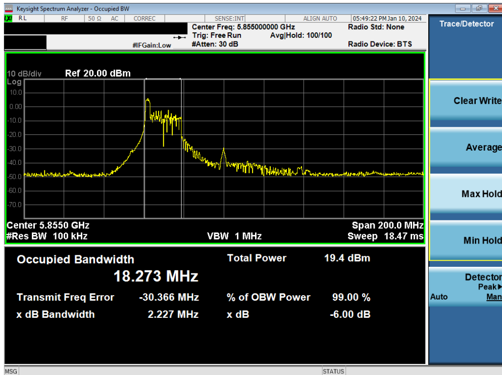
Plot 7-52. 6dB Bandwidth Plot MIMO ANT1 (80MHz BW 802.11be – 26 Tones (UNII Band 3/4) – Ch. 171)
