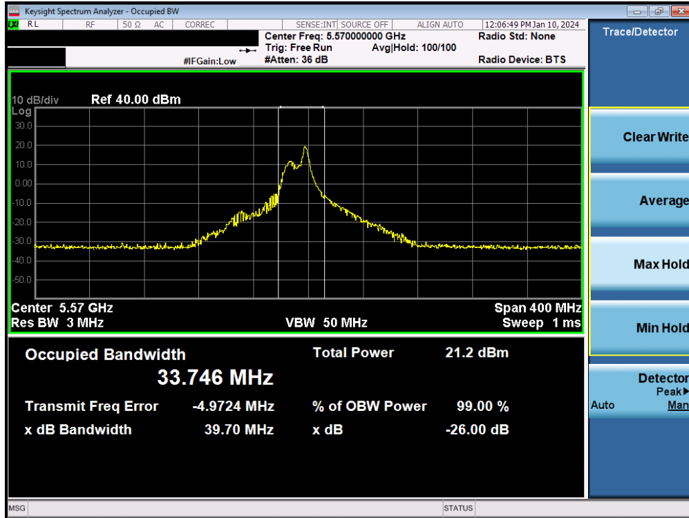
Plot 7-35. 26dB Bandwidth Plot MIMO ANT2 (160MHz BW 802.11be – 26 Tones (UNII Band 2C) – Ch. 114)
