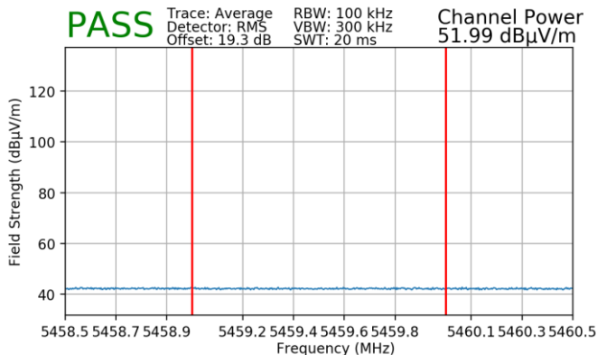
Plot 7-1. Radiated Lower Band Edge Plot MIMO (Average – UNII Band 2C) (Spot-check)
