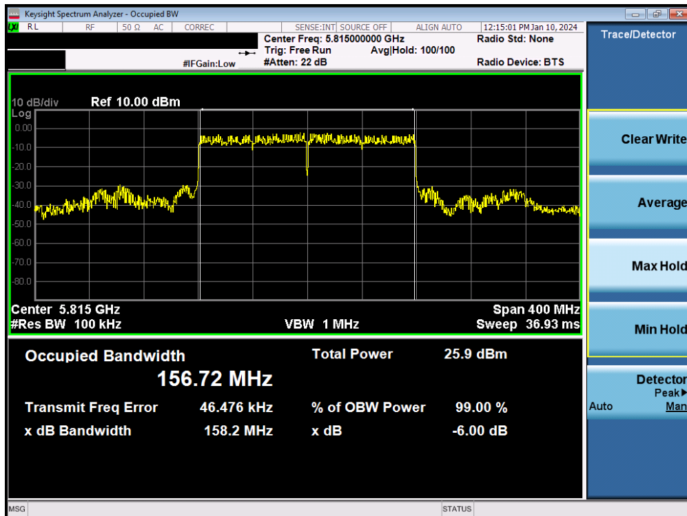
Plot 7-74. 6dB Bandwidth Plot MIMO ANT2 (160MHz BW 802.11be – 996*2 Tones (UNII Band 3/4) – Ch. 163)
