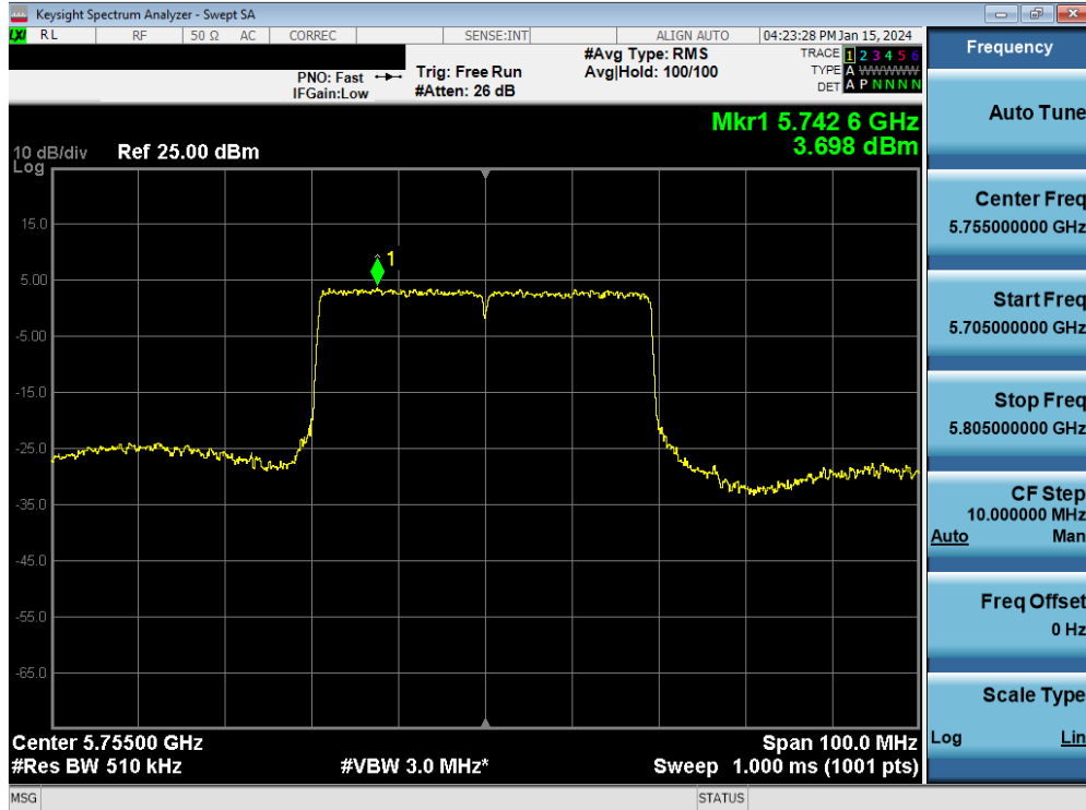
Plot 7-105. Power Spectral Density Plot MIMO ANT1 (40MHz BW 802.11be – 484 Tones (UNII Band 3) – Ch. 151)
