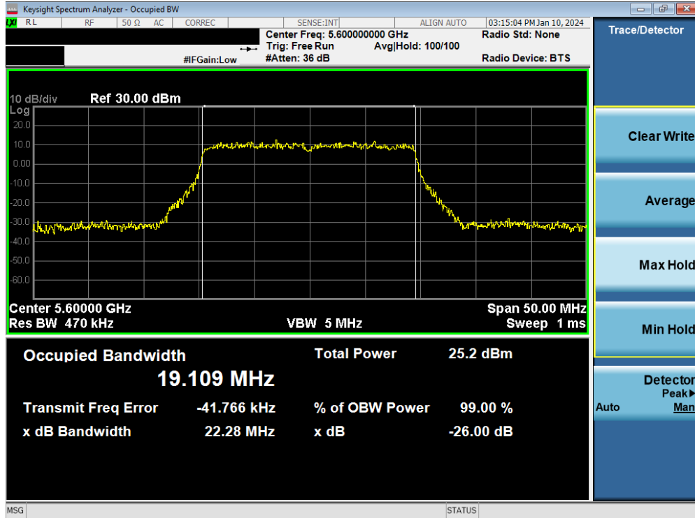
Plot 7-21. 26dB Bandwidth Plot MIMO ANT1 (20MHz BW 802.11be – 242 Tones (UNII Band 2C) – Ch. 120)
