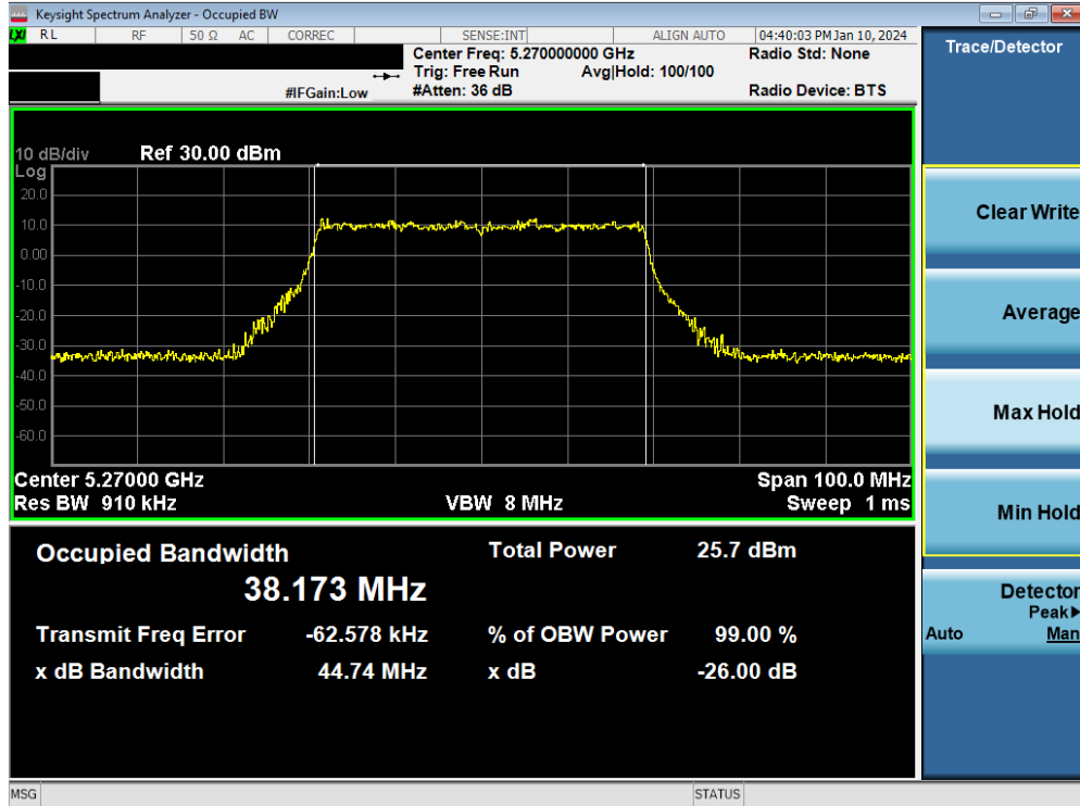
Plot 7-19. 26dB Bandwidth Plot MIMO ANT1 (40MHz BW 802.11be – 484 Tones (UNII Band 2A) – Ch. 54)
