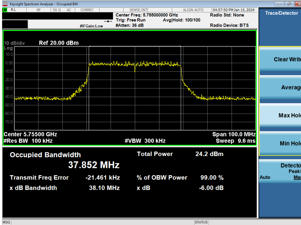
Plot 7-55. 6dB Bandwidth Plot MIMO ANT1 (40MHz BW 802.11be – 484 Tones (UNII Band 3) – Ch. 151)
