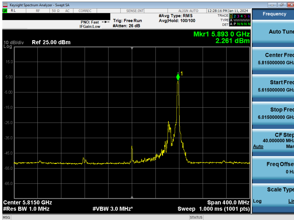
Plot 7-92. Power Spectral Density Plot MIMO ANT1 (160MHz(U) BW 802.11be – 26 Tones (UNII Band 3/4) – Ch. 163)
