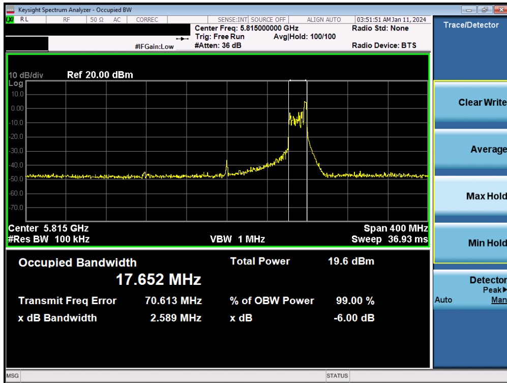
Plot 7-67. 6dB Bandwidth Plot MIMO ANT2 (160MHz(U) BW 802.11be – 26 Tones (UNII Band 3/4) – Ch. 163)
