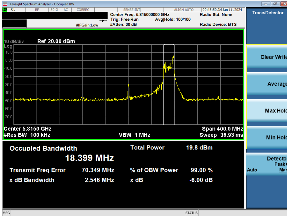
Plot 7-53. 6dB Bandwidth Plot MIMO ANT1 (160MHz(U) BW 802.11be – 26 Tones (UNII Band 3/4) – Ch. 163)
