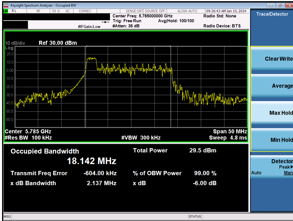
Plot 7-61. 6dB Bandwidth Plot MIMO ANT2 (20MHz BW 802.11be – 26 Tones (UNII Band 3) – Ch. 157)
