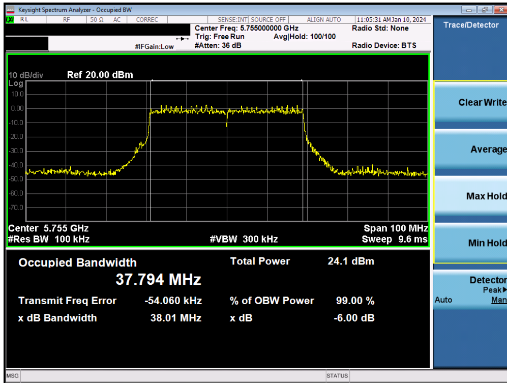
Plot 7-69. 6dB Bandwidth Plot MIMO ANT2 (40MHz BW 802.11be – 484 Tones (UNII Band 3) – Ch. 151)
