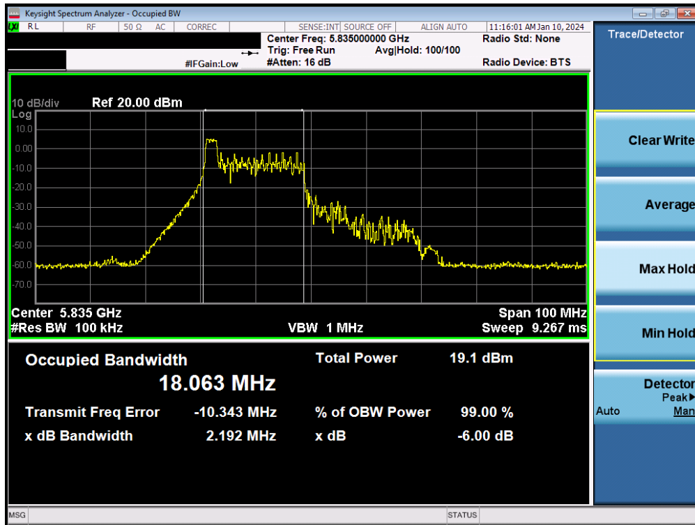
Plot 7-65. 6dB Bandwidth Plot MIMO ANT2 (40MHz BW 802.11be – 26 Tones (UNII Band 3/4) – Ch. 167)
