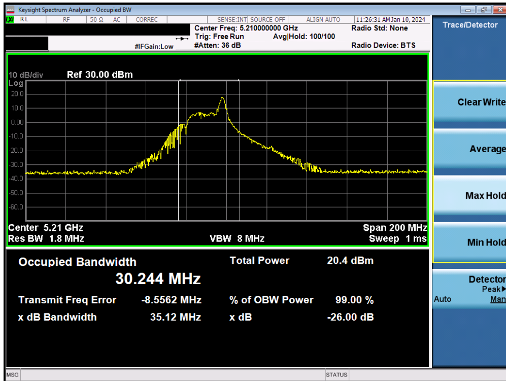
Plot 7-27. 26dB Bandwidth Plot MIMO ANT2 (80MHz BW 802.11be – 26 Tones (UNII Band 1) – Ch. 42)
