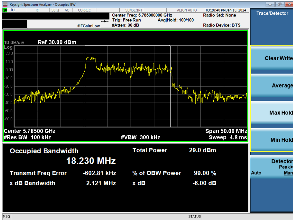
Plot 7-47. 6dB Bandwidth Plot MIMO ANT1 (20MHz BW 802.11be – 26 Tones (UNII Band 3) – Ch. 157)
