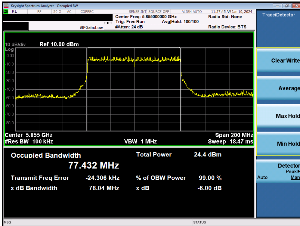
Plot 7-73. 6dB Bandwidth Plot MIMO ANT2 (80MHz BW 802.11be – 996 Tones (UNII Band 3/4) – Ch. 171)
