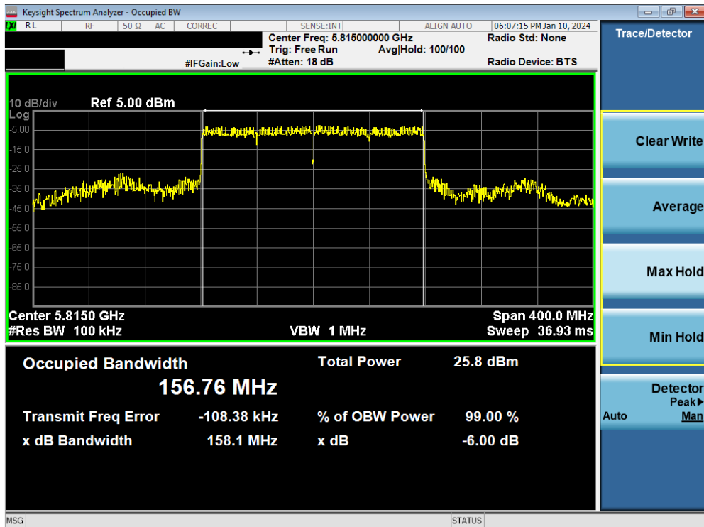
Plot 7-60. 6dB Bandwidth Plot MIMO ANT1 (160MHz BW 802.11be – 996*2 Tones (UNII Band 3/4) – Ch. 163)
