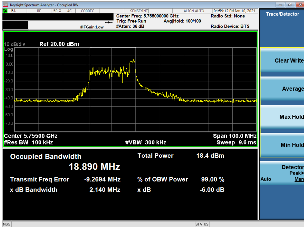
Plot 7-48. 6dB Bandwidth Plot MIMO ANT1 (40MHz BW 802.11be – 26 Tones (UNII Band 3) – Ch. 151)
