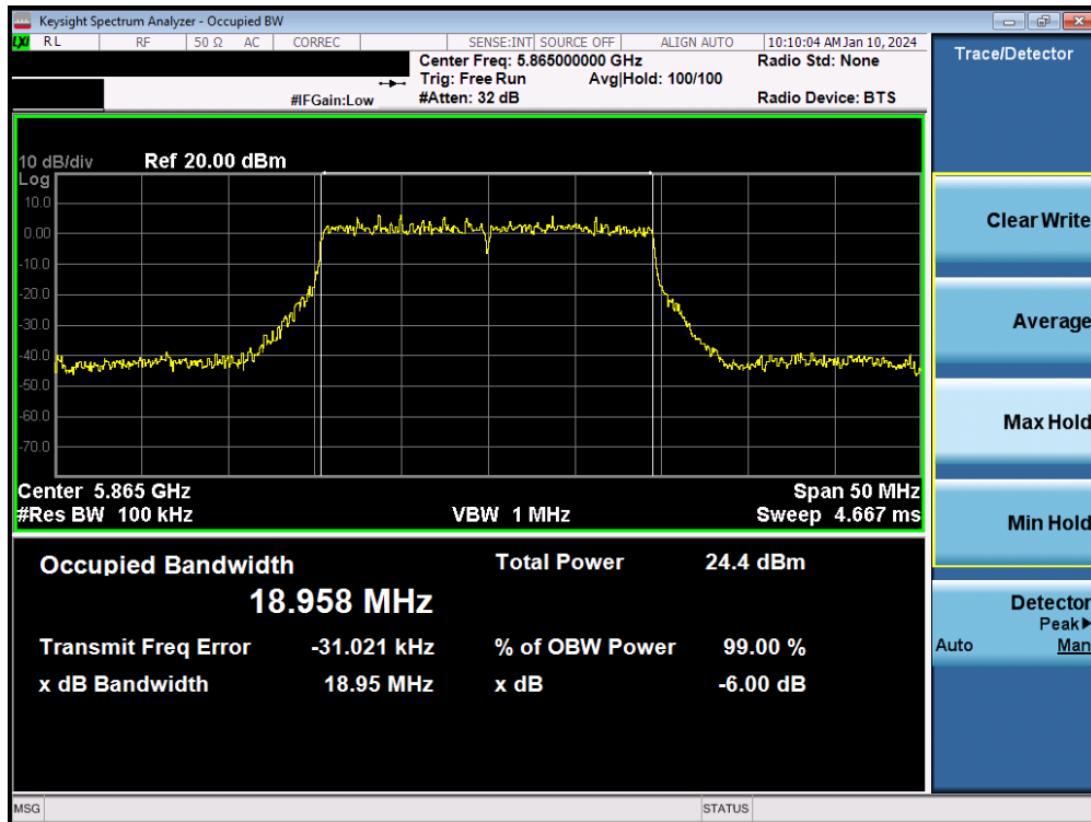
Plot 7-71. 6dB Bandwidth Plot MIMO ANT2 (20MHz BW 802.11be – 242 Tones (UNII Band 4) – Ch. 173)
