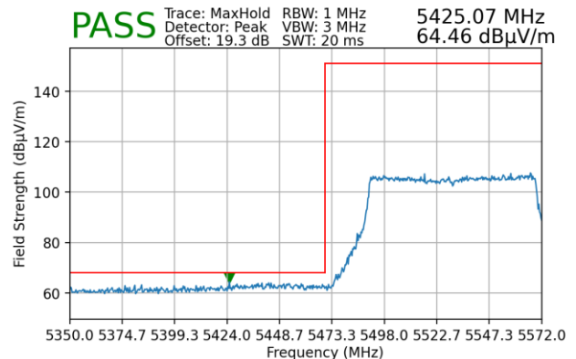
Plot 7-2. Radiated Lower Band Edge Plot MIMO (Peak – UNII Band 2C) (Spot-check)
