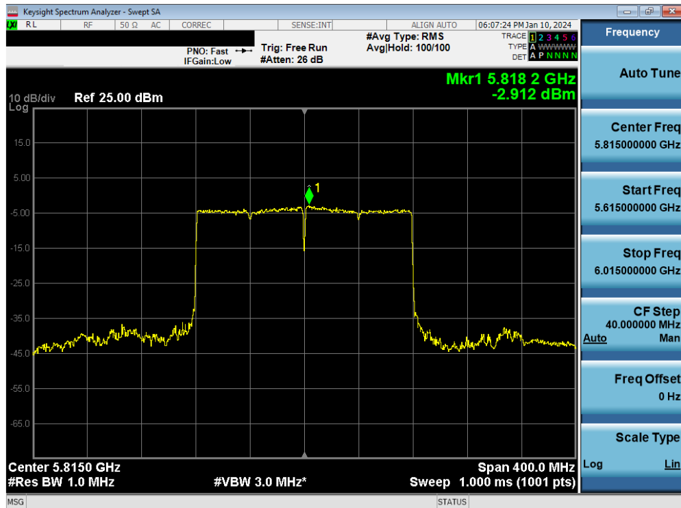
Plot 7-110. Power Spectral Density Plot MIMO ANT1 (160MHz BW 802.11be – 2x996 Tones (UNII Band 3/4) – Ch. 163)
