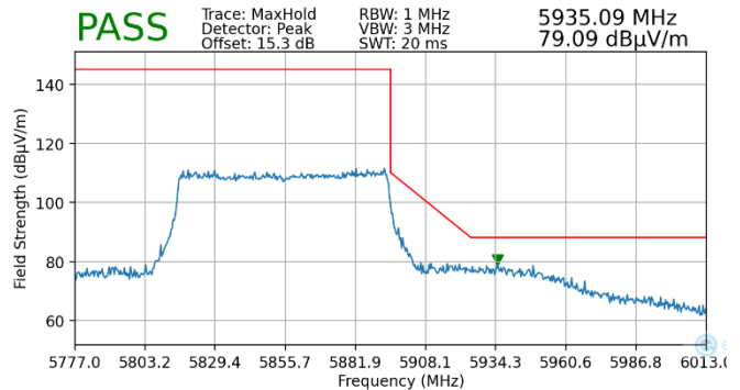
Plot 7-218. Radiated Upper Band Edge Plot MIMO (Peak – UNII Band 4)
