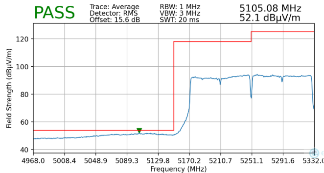
Plot 7-219. Radiated Lower Band Edge Plot MIMO (Average – UNII Band 1)
