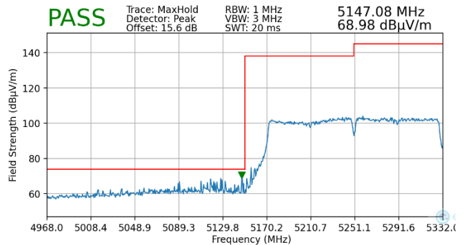
Plot 7-220. Radiated Lower Band Edge Plot MIMO (Peak – UNII Band 1)
