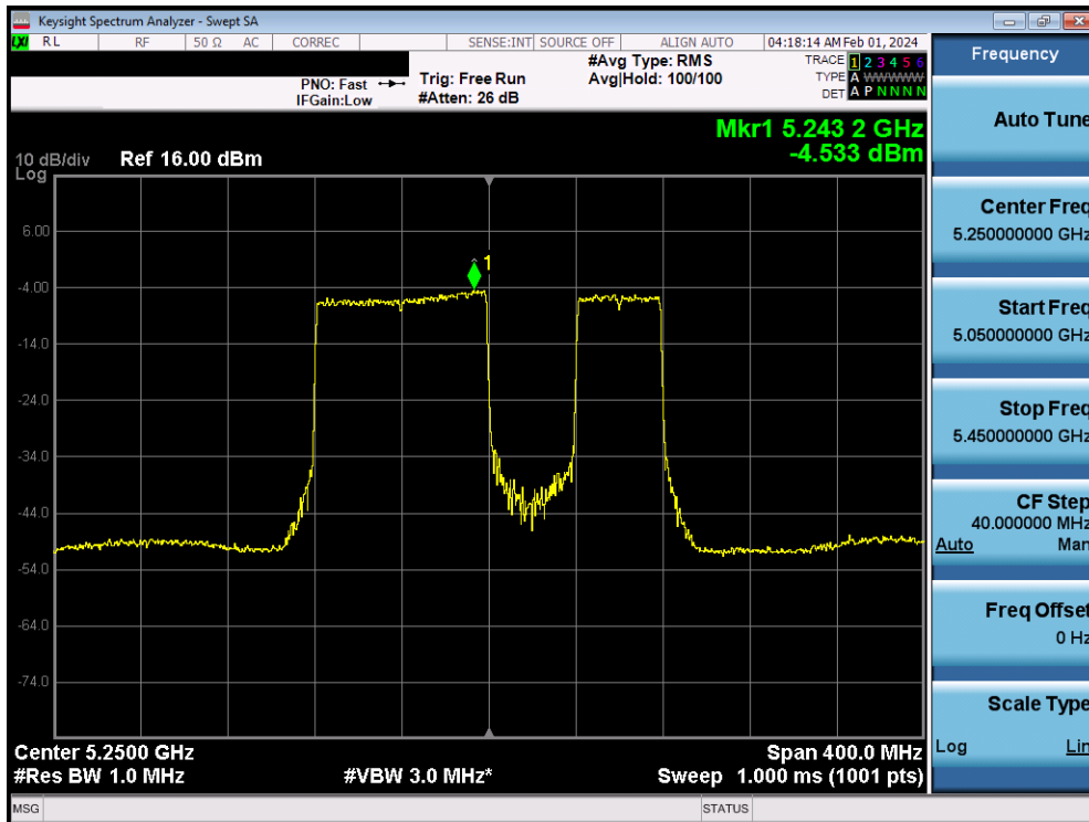
Plot 7-175. Power Spectral Density Plot MIMO ANT2 (160MHz BW 802.11be (UNII Band 1/2A) – Ch. 50)
