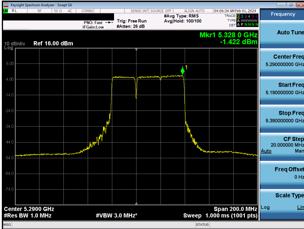
Plot 7-176. Power Spectral Density Plot MIMO ANT2 (80MHz BW 802.11be (UNII Band 2A) – Ch. 58)
