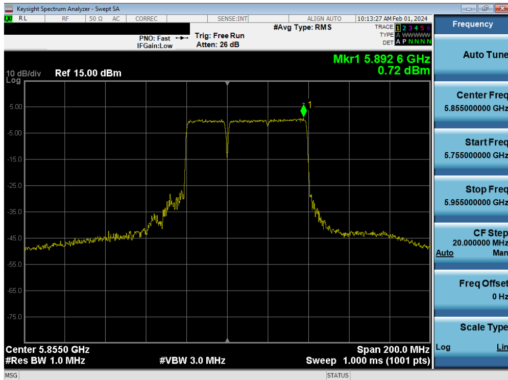
Plot 7-172. Power Spectral Density Plot MIMO ANT1 (80MHz BW 802.11be (UNII Band 3/4) – Ch. 171)
