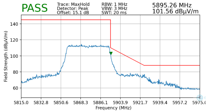
Plot 7-208. Radiated Upper Band Edge Plot MIMO (Peak – UNII Band 4)
