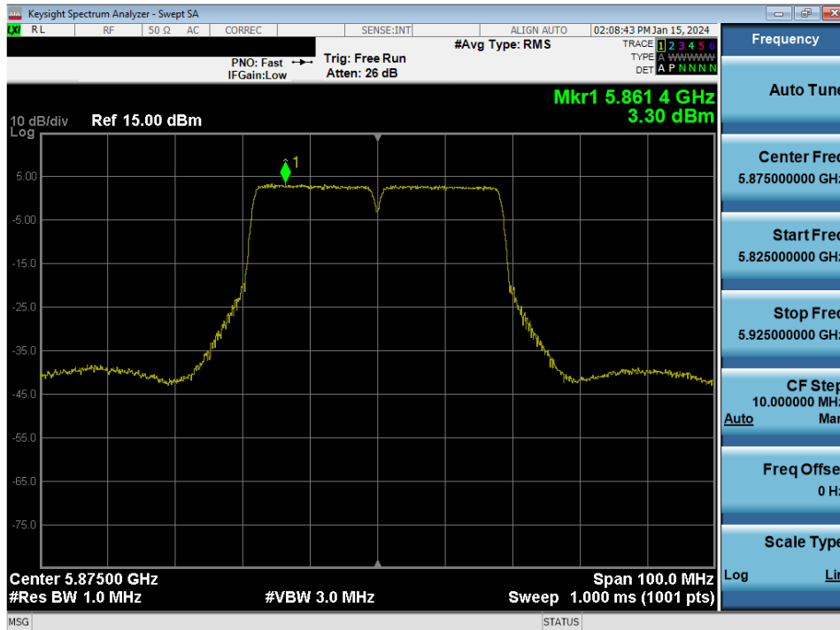
Plot 7-120. Power Spectral Density Plot MIMO ANT1 (40MHz BW 802.11n (UNII Band 4) – Ch. 175)
