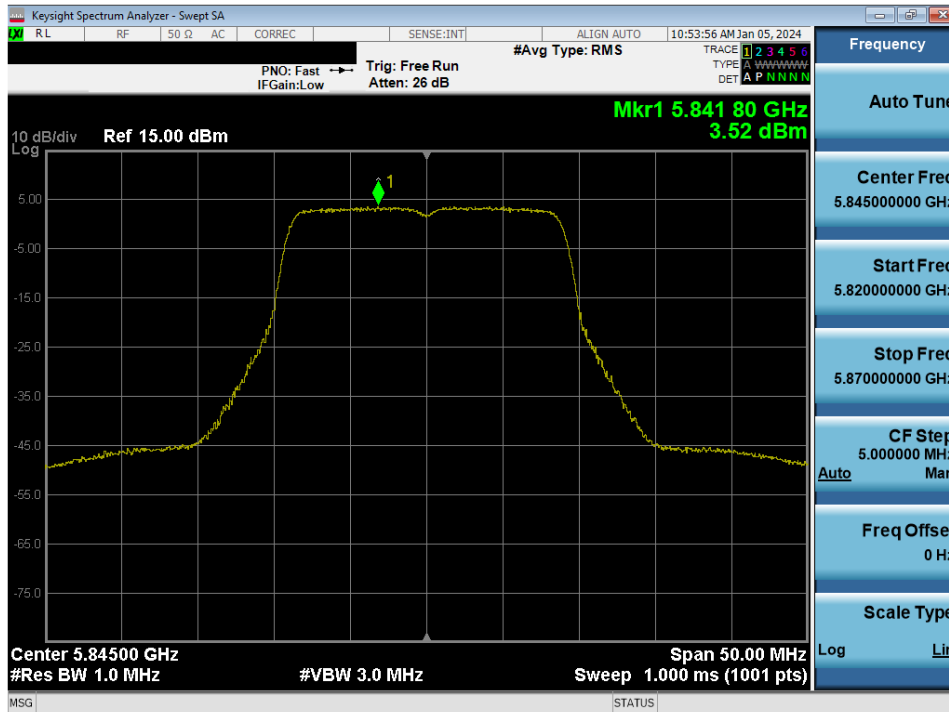
Plot 7-118. Power Spectral Density Plot MIMO ANT1 (20MHz BW 802.11n (UNII Band 3/4) – Ch. 169)
