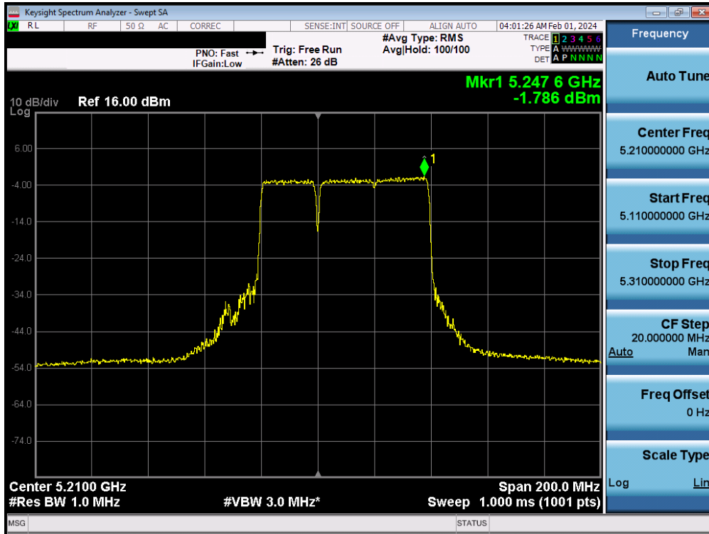
Plot 7-174. Power Spectral Density Plot MIMO ANT2 (80MHz BW 802.11be (UNII Band 1) – Ch. 42)
