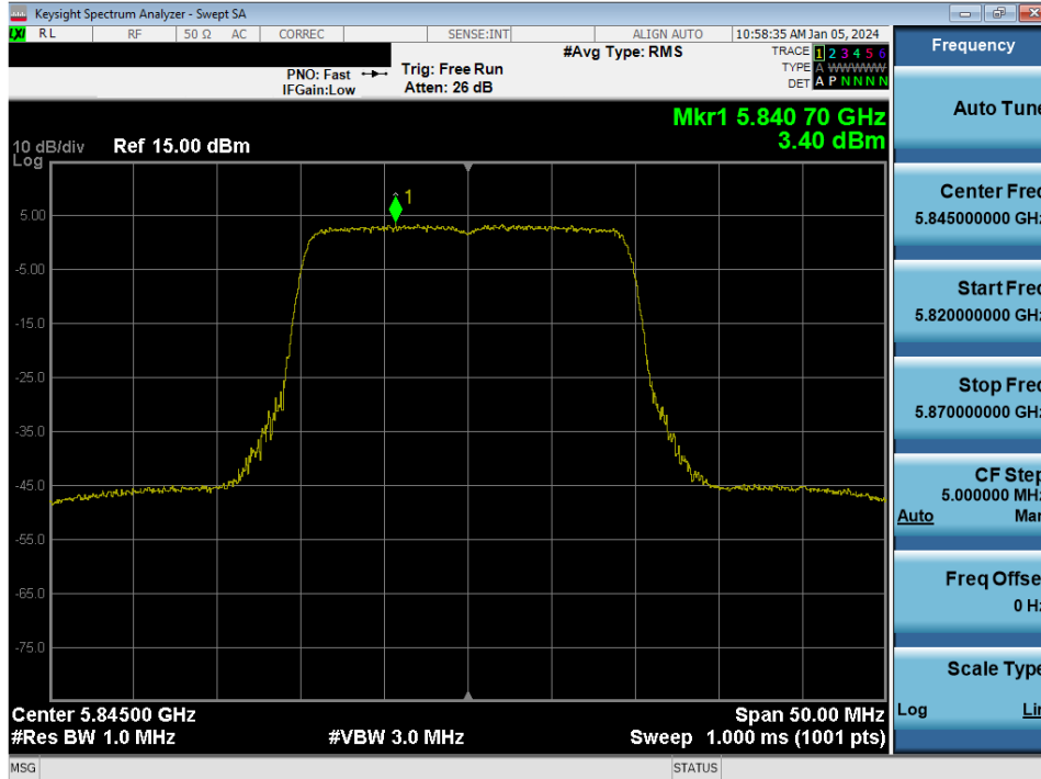
Plot 7-119. Power Spectral Density Plot MIMO ANT1 (20MHz BW 802.11ax/be (UNII Band 3/4) – Ch. 169)
