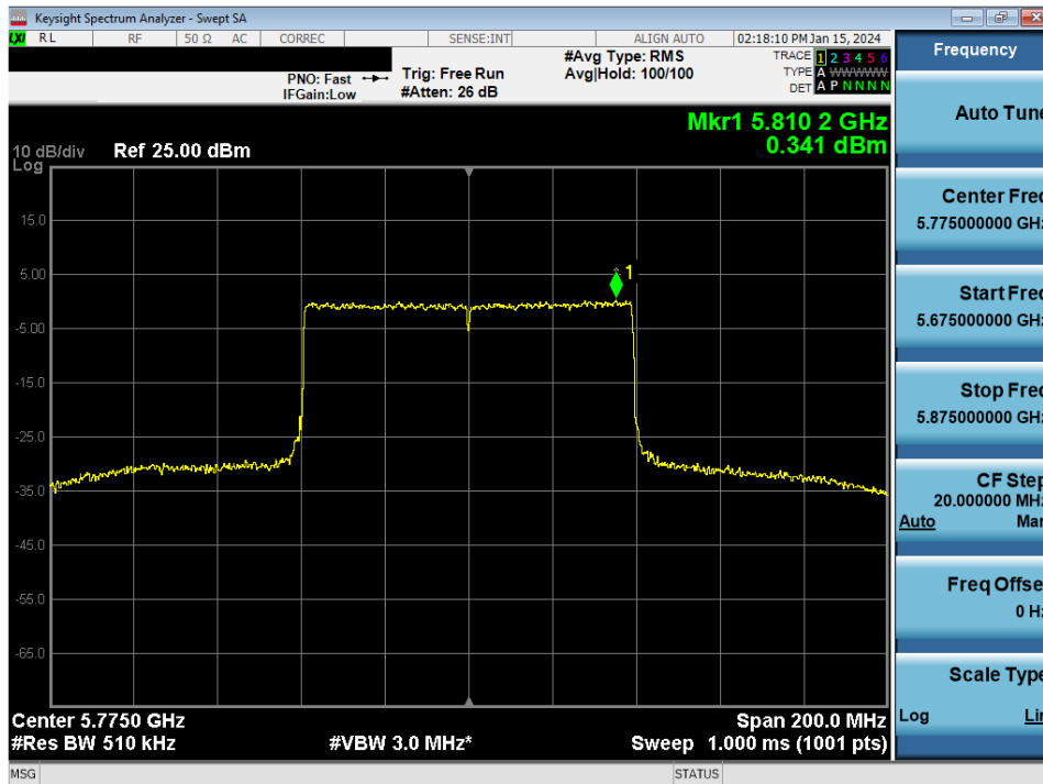
Plot 7-116. Power Spectral Density Plot MIMO ANT1 (80MHz BW 802.11ax/be (UNII Band 3) – Ch. 155)
