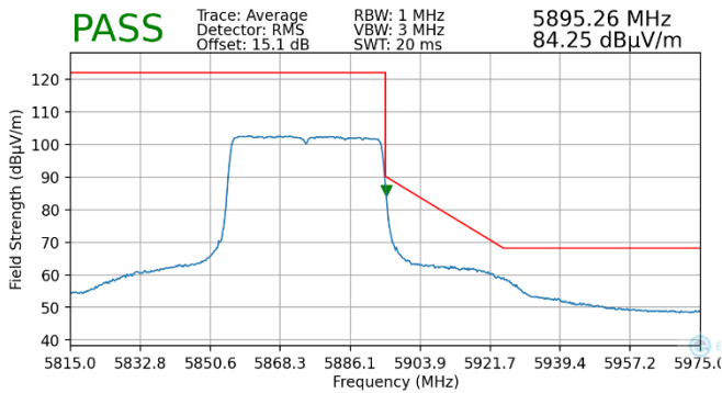
Plot 7-207. Radiated Upper Band Edge Plot MIMO (Average – UNII Band 4)
