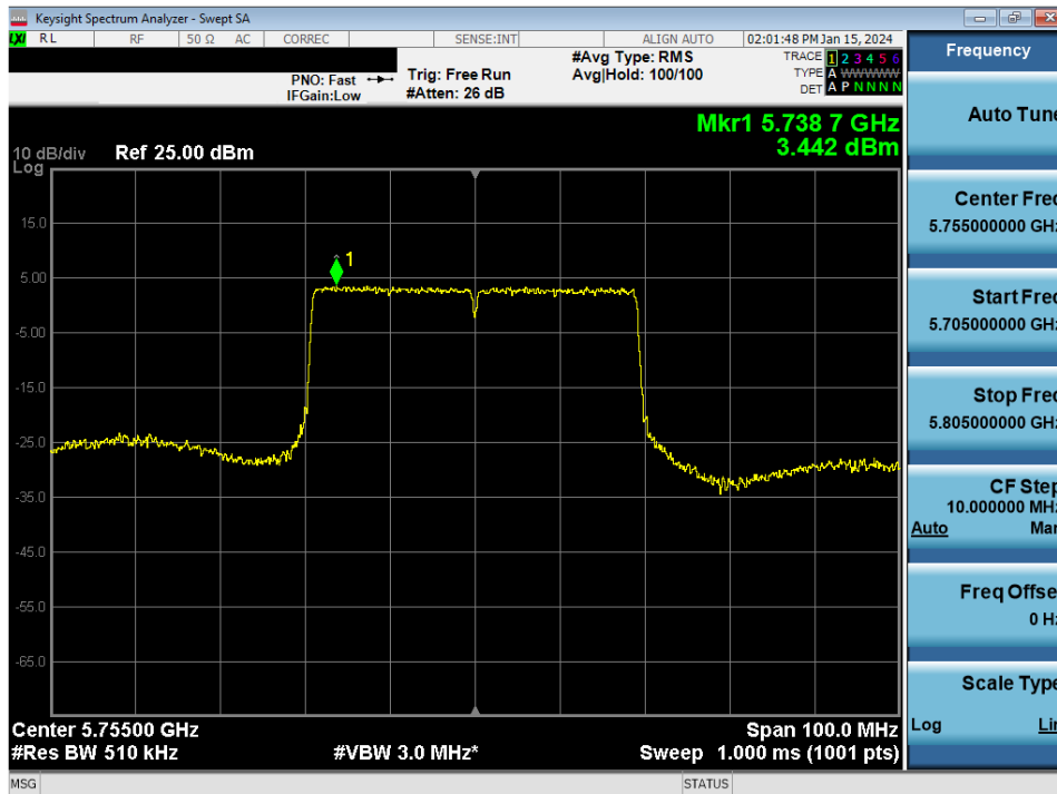
Plot 7-114. Power Spectral Density Plot MIMO ANT1 (40MHz BW 802.11ax/be (UNII Band 3) – Ch. 151)
