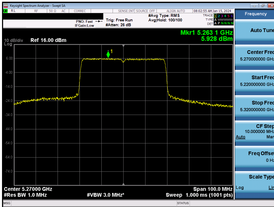
Plot 7-139. Power Spectral Density Plot MIMO ANT2 (40MHz BW 802.11ax/be (UNII Band 2A) – Ch. 54)
