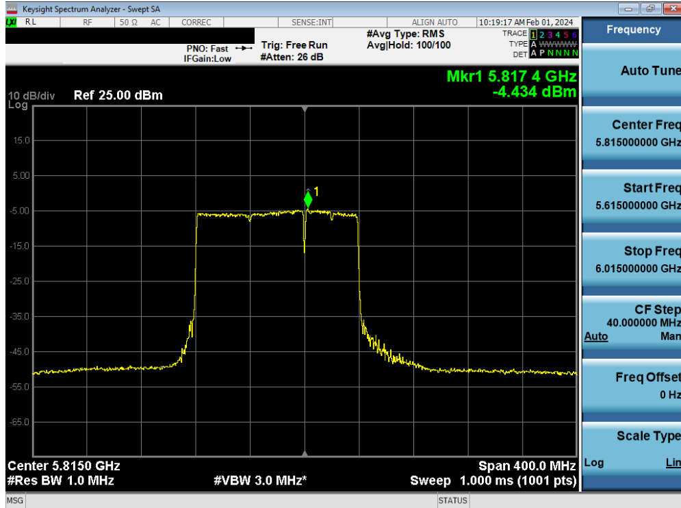
Plot 7-173. Power Spectral Density Plot MIMO ANT1 (160MHz BW 802.11be (UNII Band 3/4) – Ch. 163)
