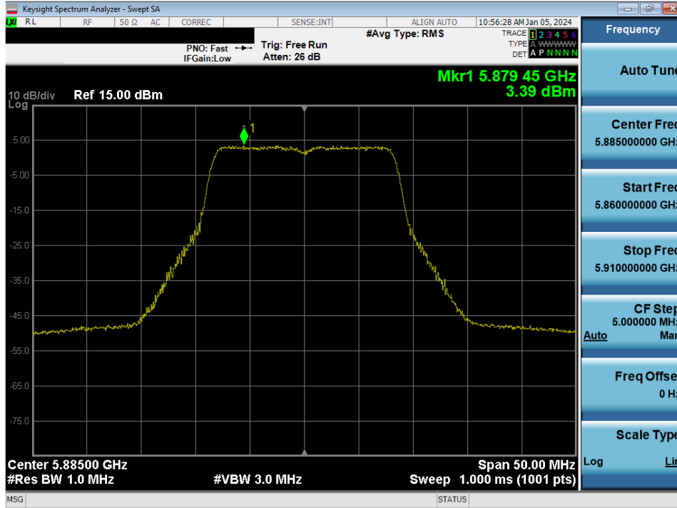
Plot 7-117. Power Spectral Density Plot MIMO ANT1 (20MHz BW 802.11a (UNII Band 4) – Ch. 177)
