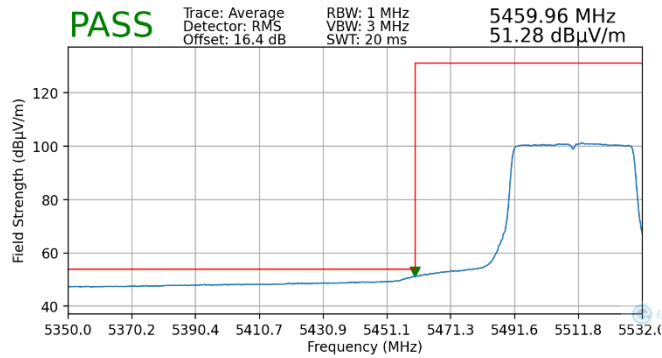
Plot 7-203. Radiated Lower Band Edge Plot MIMO (Average – UNII Band 2C)
