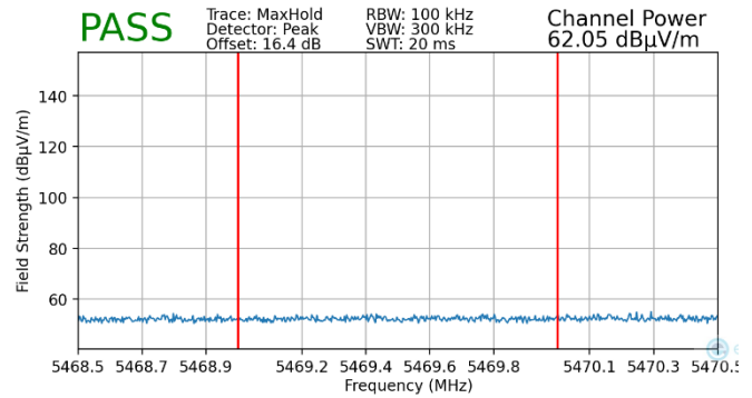
Plot 7-204. Radiated Lower Band Edge Plot MIMO (Peak – UNII Band 2C)
