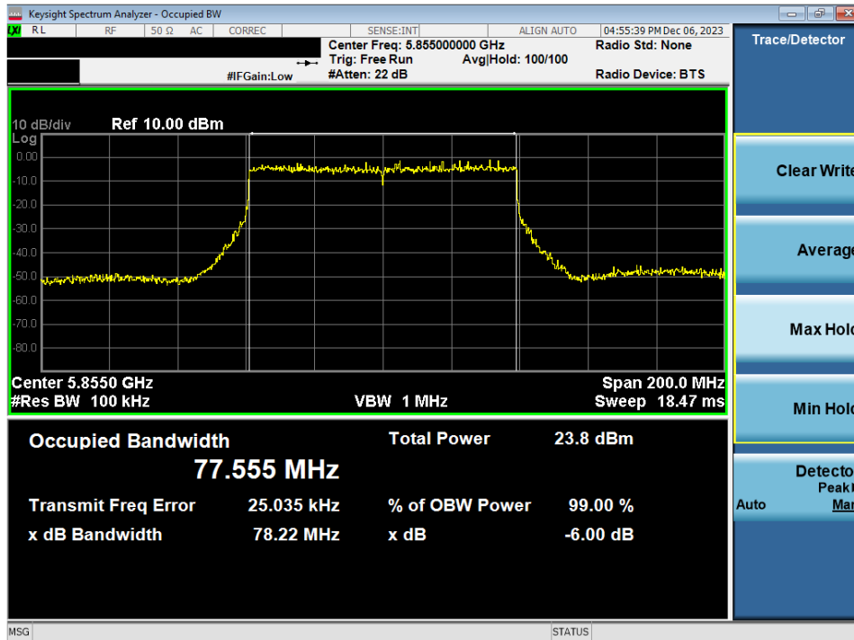
Plot 7-82. 6dB Bandwidth Plot MIMO ANT2 (80MHz BW 802.11ax/be (UNII Band 3/4) – Ch. 171)
