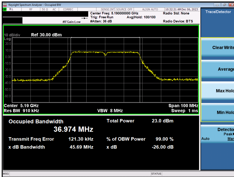
Plot 7-6. 26dB Bandwidth Plot MIMO ANT1 (40MHz BW 802.11n (UNII Band 1) – Ch. 38)
