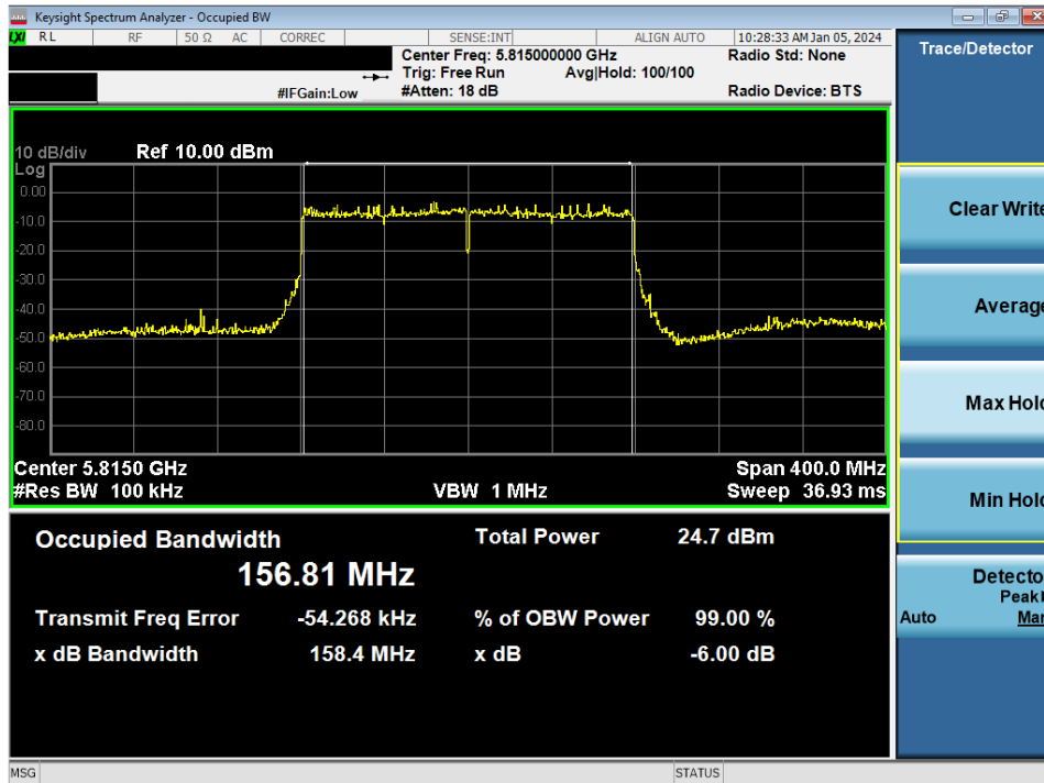
Plot 7-68. 6dB Bandwidth Plot MIMO ANT1 (160MHz BW 802.11ax/be (UNII Band 3/4) – Ch. 163)
