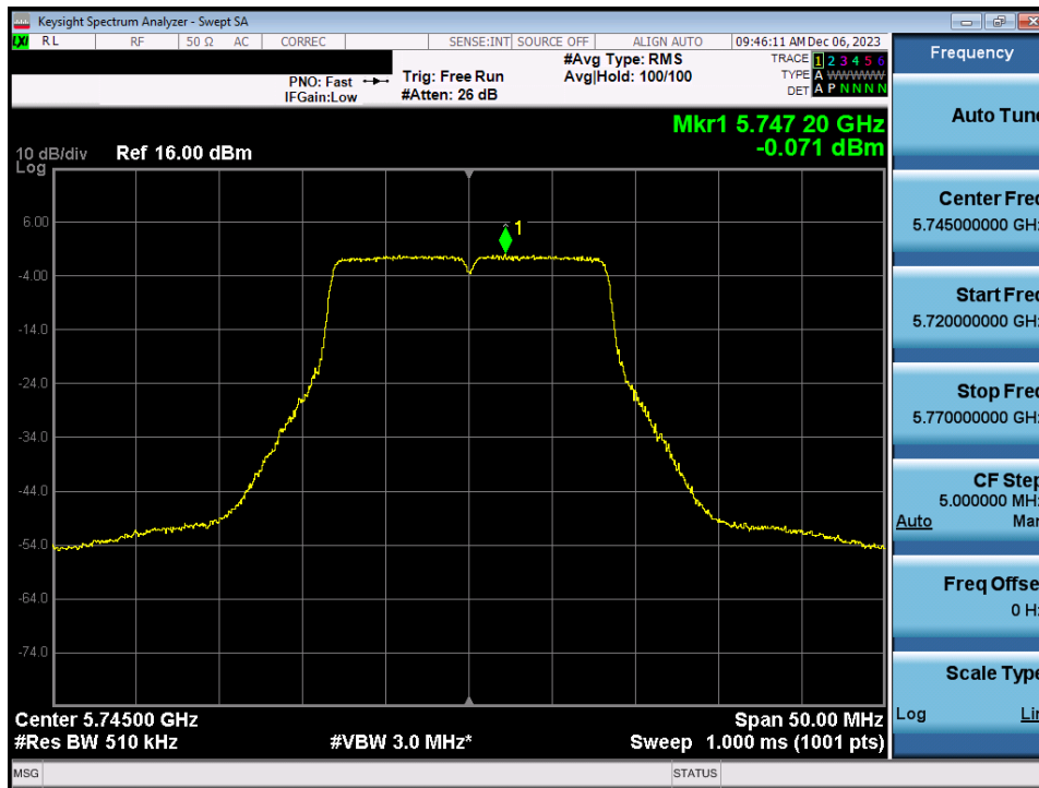
Plot 7-110. Power Spectral Density Plot MIMO ANT1 (802.11a (UNII Band 3) – Ch. 149)
