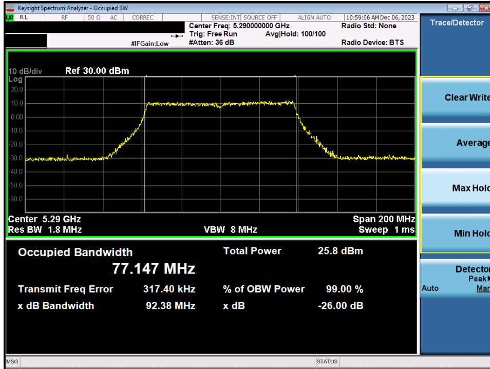
Plot 7-17. 26dB Bandwidth Plot MIMO ANT1 (80MHz BW 802.11ac (UNII Band 2A) – Ch. 58)
