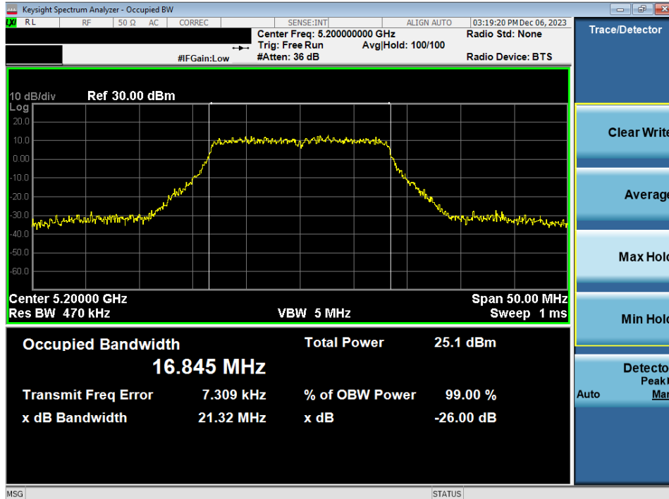
Plot 7-28. 26dB Bandwidth Plot MIMO ANT2 (802.11a (UNII Band 1) – Ch. 40)
