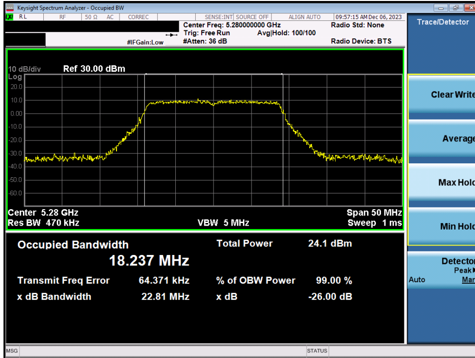
Plot 7-13. 26dB Bandwidth Plot MIMO ANT1 (20MHz BW 802.11n (UNII Band 2A) – Ch. 56)
