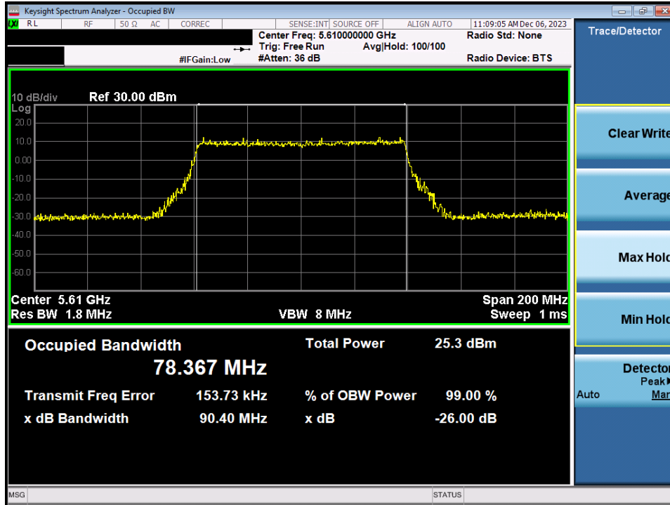
Plot 7-25. 26dB Bandwidth Plot MIMO ANT1 (80MHz BW 802.11ax/be (UNII Band 2C) – Ch. 122)
