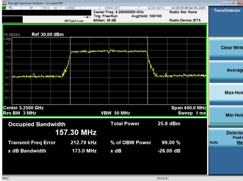
Plot 7-11. 26dB Bandwidth Plot MIMO ANT1 (160MHz BW 802.11ax/be (UNII Band 1/2A) – Ch. 50)
