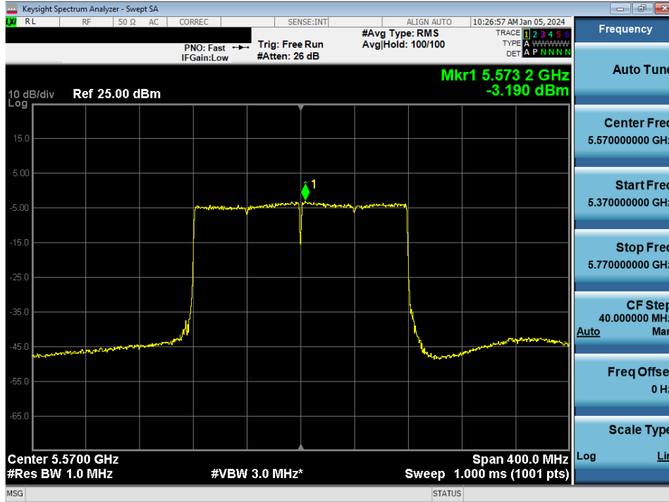
Plot 7-109. Power Spectral Density Plot MIMO ANT1 (160MHz BW 802.11ax/be (UNII Band 2C) – Ch. 114)
