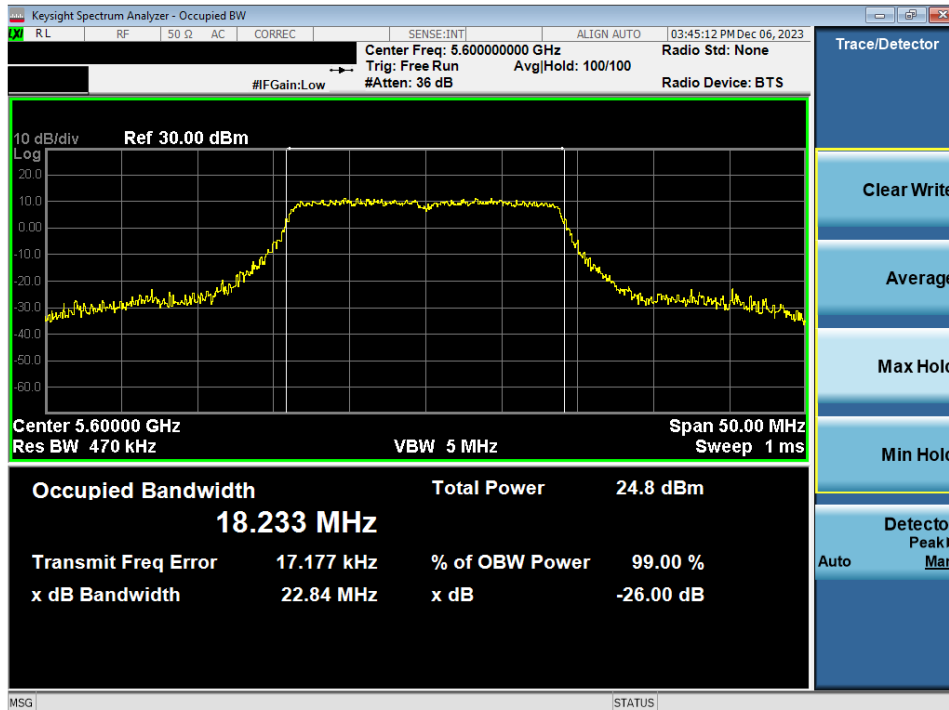
Plot 7-45. 26dB Bandwidth Plot MIMO ANT2 (20MHz BW 802.11n (UNII Band 2C) – Ch. 120)
