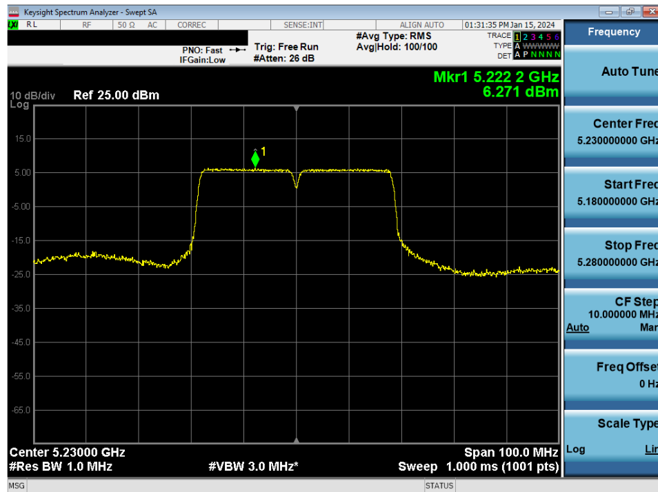
Plot 7-88. Power Spectral Density Plot MIMO ANT1 (40MHz BW 802.11n (UNII Band 1) – Ch. 46)
