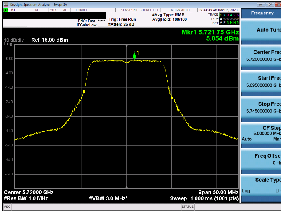
Plot 7-101. Power Spectral Density Plot MIMO ANT1 (802.11a (UNII Band 2C) – Ch. 144)
