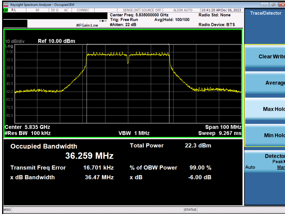
Plot 7-63. 6dB Bandwidth Plot MIMO ANT1 (40MHz BW 802.11n (UNII Band 3/4) – Ch. 167)
