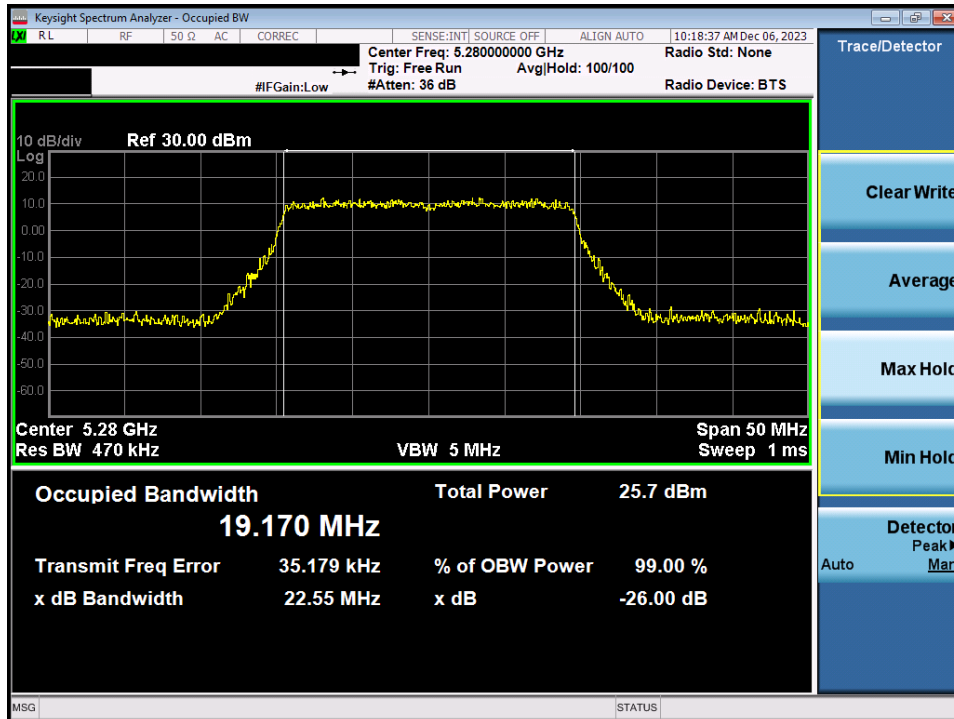
Plot 7-14. 26dB Bandwidth Plot MIMO ANT1 (20MHz BW 802.11ax/be (UNII Band 2A) – Ch. 56)
