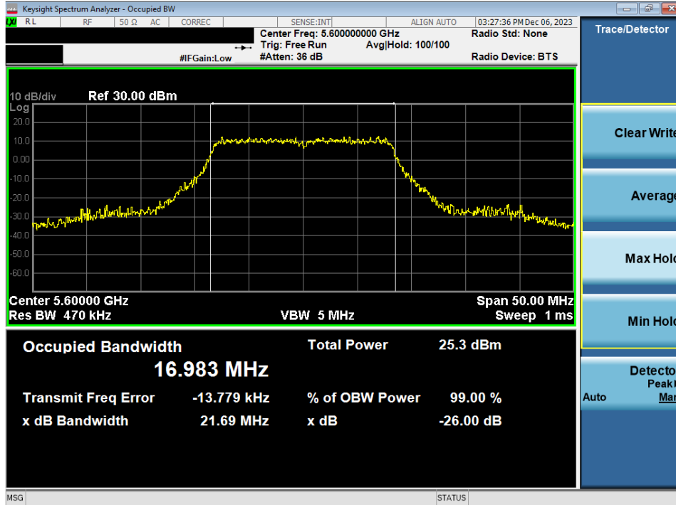
Plot 7-44. 26dB Bandwidth Plot MIMO ANT2 (802.11a (UNII Band 2C) – Ch. 120)
