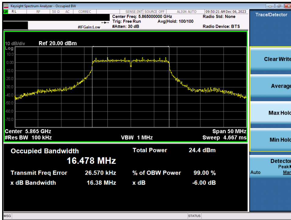
Plot 7-60. 6dB Bandwidth Plot MIMO ANT1 (20MHz BW 802.11a (UNII Band 4) – Ch. 173)
