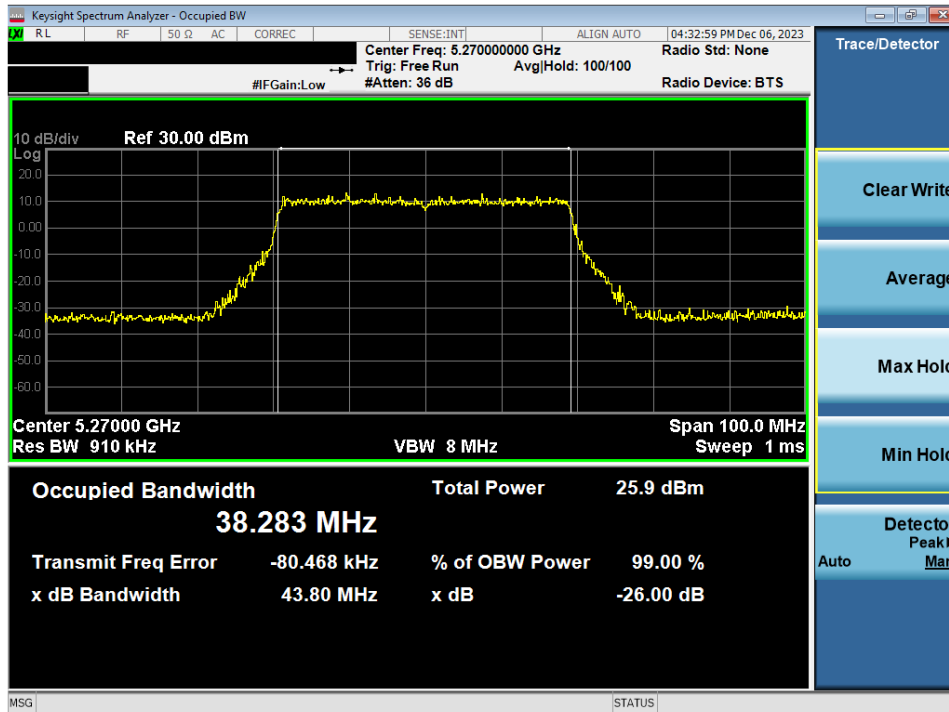
Plot 7-41. 26dB Bandwidth Plot MIMO ANT2 (40MHz BW 802.11ax/be (UNII Band 2A) – Ch. 54)
