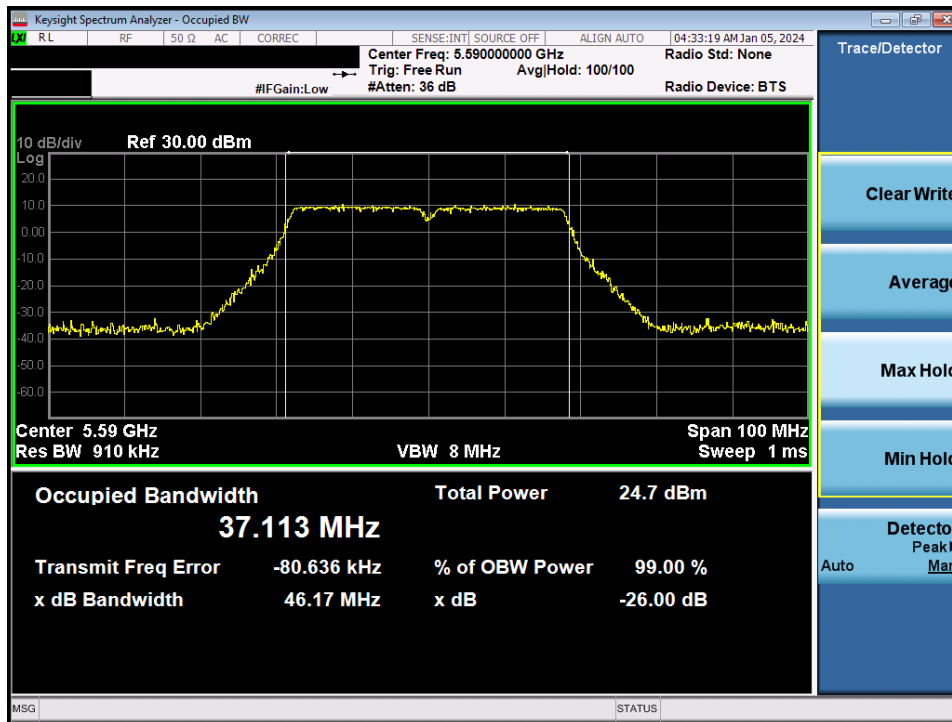
Plot 7-47. 26dB Bandwidth Plot MIMO ANT2 (40MHz BW 802.11n (UNII Band 2C) – Ch. 118)
