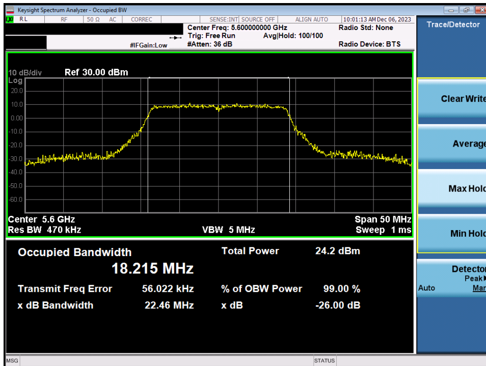
Plot 7-20. 26dB Bandwidth Plot MIMO ANT1 (20MHz BW 802.11n (UNII Band 2C) – Ch. 120)
