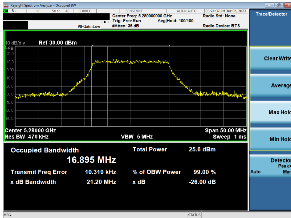
Plot 7-37. 26dB Bandwidth Plot MIMO ANT2 (802.11a (UNII Band 2A) – Ch. 56)
