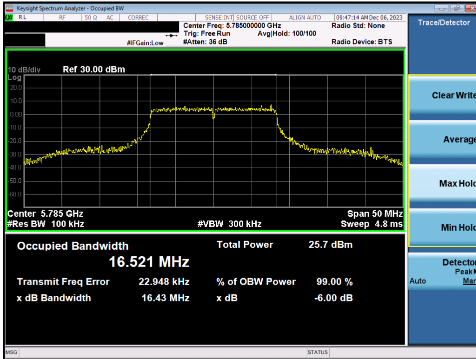
Plot 7-53. 6dB Bandwidth Plot MIMO ANT1 (802.11a (UNII Band 3) – Ch. 157)
