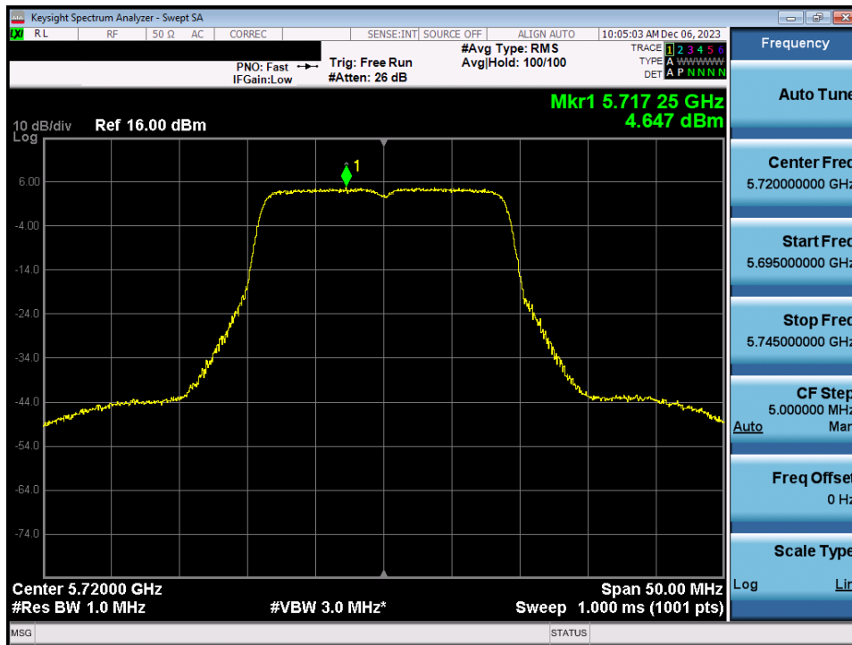
Plot 7-102. Power Spectral Density Plot MIMO ANT1 (20MHz BW 802.11n (UNII Band 2C) – Ch. 144)
