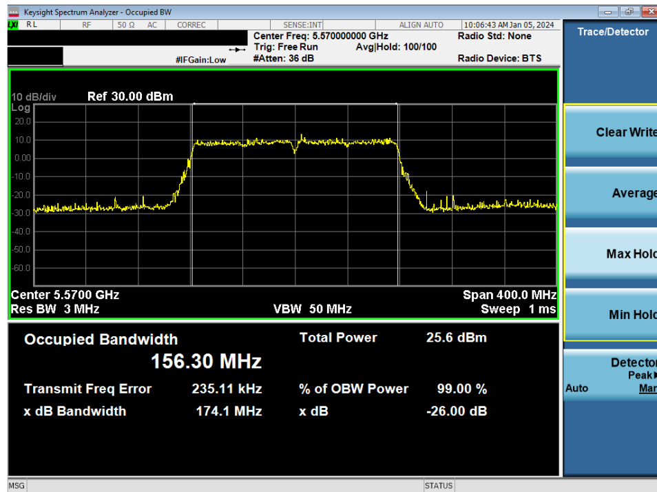
Plot 7-26. 26dB Bandwidth Plot MIMO ANT1 (160MHz BW 802.11ac (UNII Band 2C) – Ch. 114)
