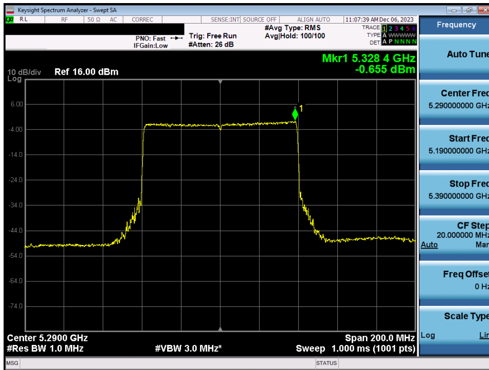
Plot 7-100. Power Spectral Density Plot MIMO ANT1 (80MHz BW 802.11ax/be (UNII Band 2A) – Ch. 58)
