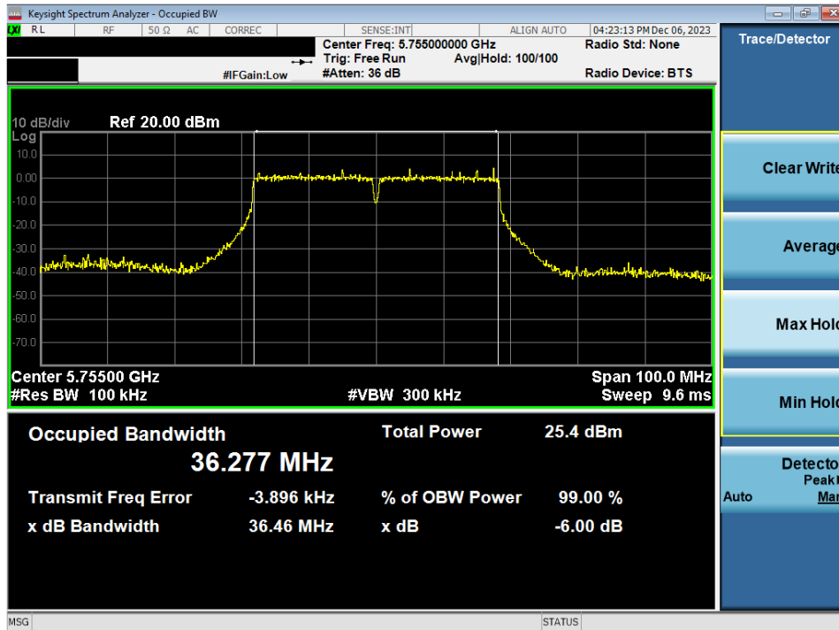
Plot 7-72. 6dB Bandwidth Plot MIMO ANT2 (40MHz BW 802.11n (UNII Band 3) – Ch. 151)
