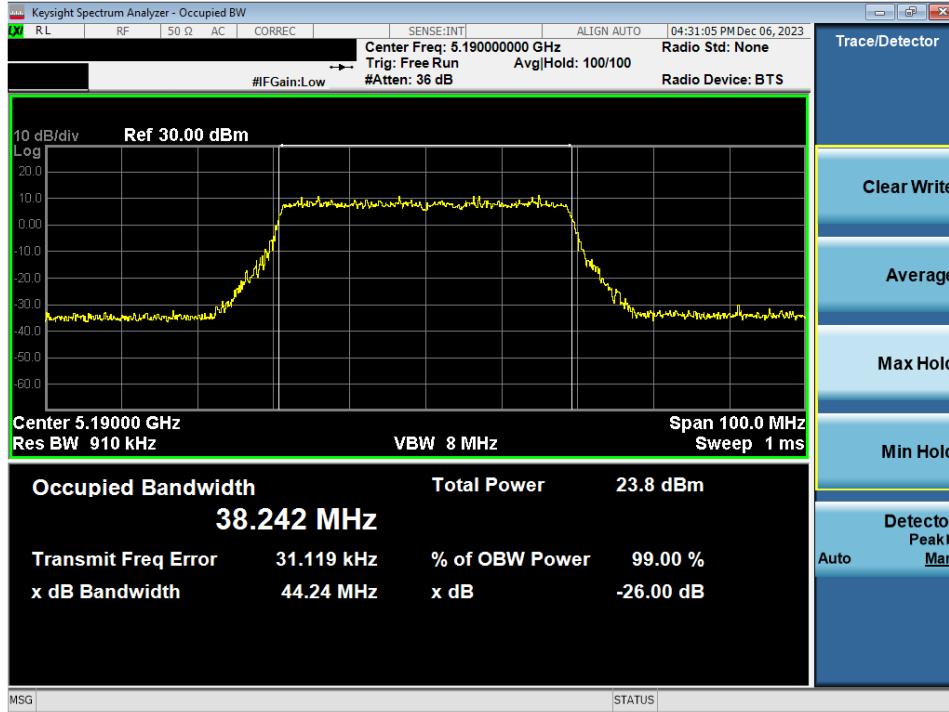
Plot 7-32. 26dB Bandwidth Plot MIMO ANT2 (40MHz BW 802.11ax/be (UNII Band 1) – Ch. 38)
