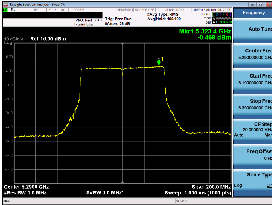
Plot 7-99. Power Spectral Density Plot MIMO ANT1 (80MHz BW 802.11ac (UNII Band 2A) – Ch. 58)
