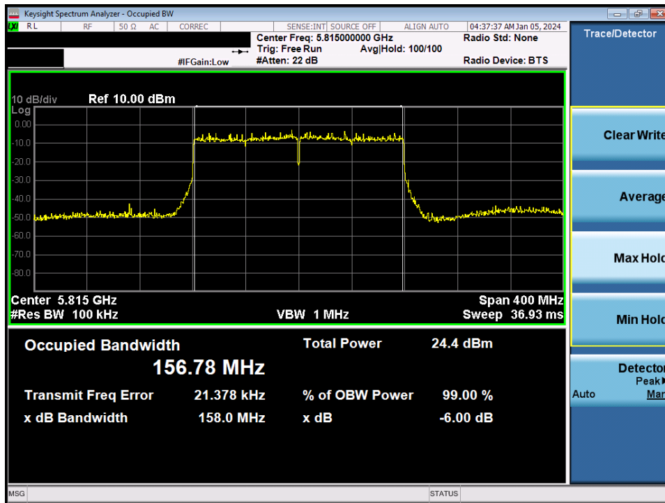
Plot 7-84. 6dB Bandwidth Plot MIMO ANT2 (160MHz BW 802.11ax/be (UNII Band 3/4) – Ch. 163)
