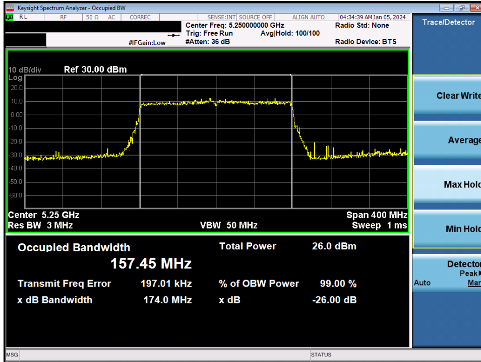
Plot 7-36. 26dB Bandwidth Plot MIMO ANT2 (160MHz BW 802.11ax/be (UNII Band 1/2A) – Ch. 50)
