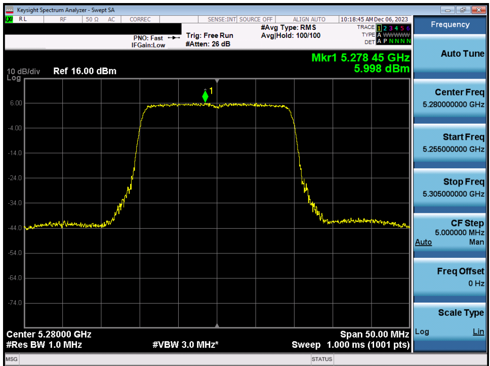
Plot 7-96. Power Spectral Density Plot MIMO ANT1 (20MHz BW 802.11ax/be (UNII Band 2A) – Ch. 56)
