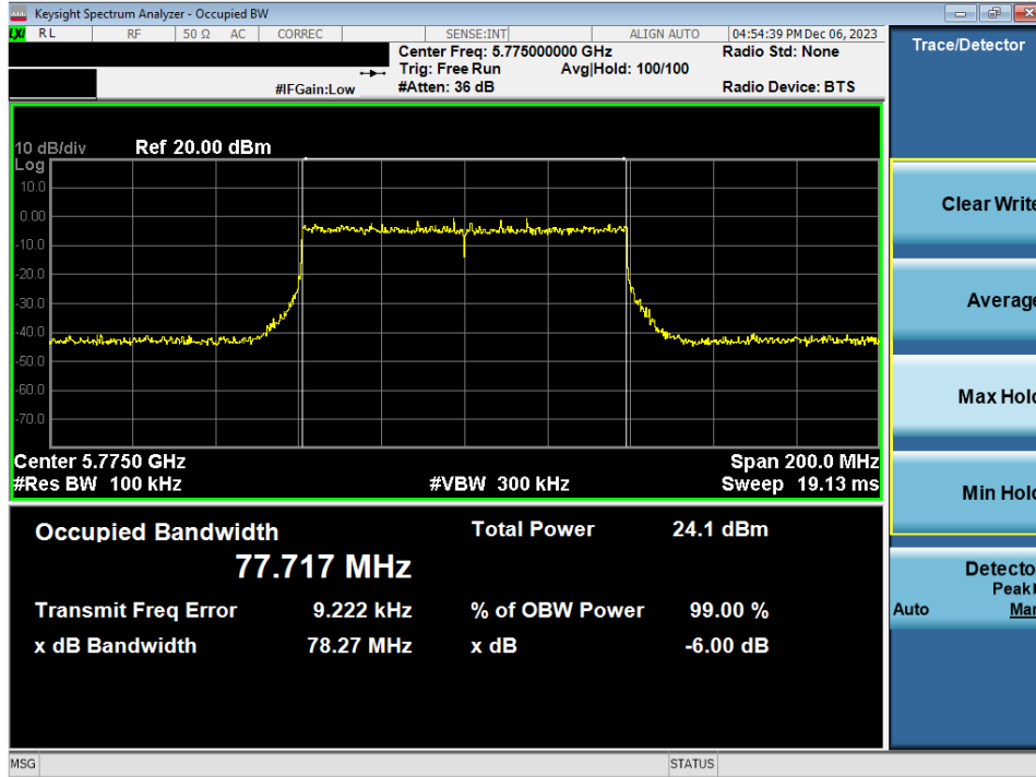
Plot 7-75. 6dB Bandwidth Plot MIMO ANT2 (80MHz BW 802.11ax/be (UNII Band 3) – Ch. 155)
