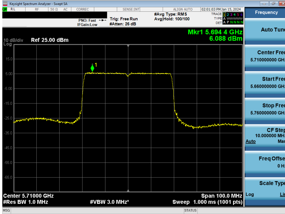
Plot 7-105. Power Spectral Density Plot MIMO ANT1 (40MHz BW 802.11ax/be (UNII Band 2C) – Ch. 142)
