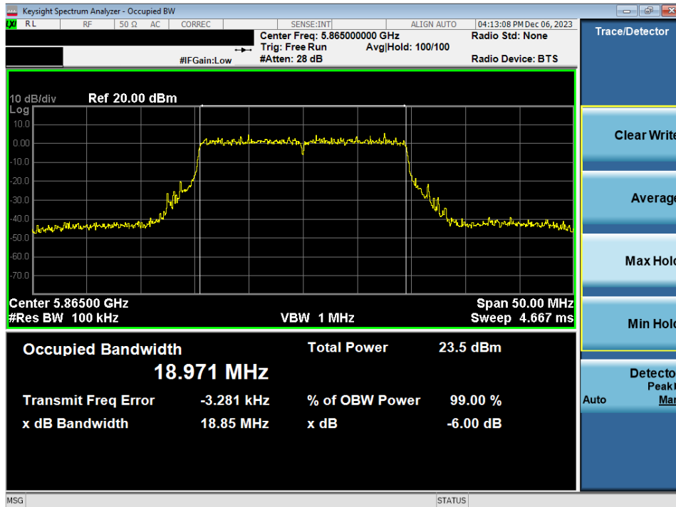
Plot 7-78. 6dB Bandwidth Plot MIMO ANT2 (20MHz BW 802.11ax/be (UNII Band 4) – Ch. 173)
