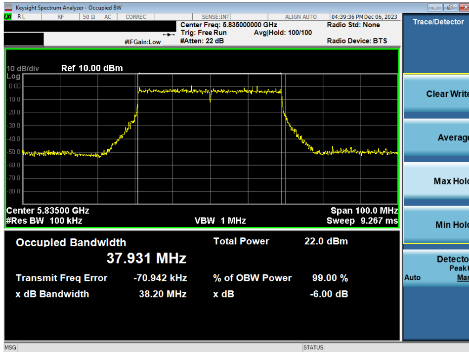
Plot 7-80. 6dB Bandwidth Plot MIMO ANT2 (40MHz BW 802.11ax/be (UNII Band 3/4) – Ch. 167)
