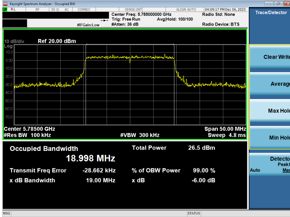
Plot 7-71. 6dB Bandwidth Plot MIMO ANT2 (20MHz BW 802.11ax/be (UNII Band 3) – Ch. 157)
