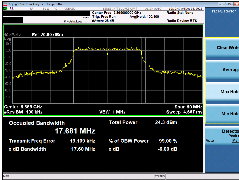
Plot 7-61. 6dB Bandwidth Plot MIMO ANT1 (20MHz BW 802.11n (UNII Band 4) – Ch. 173)
