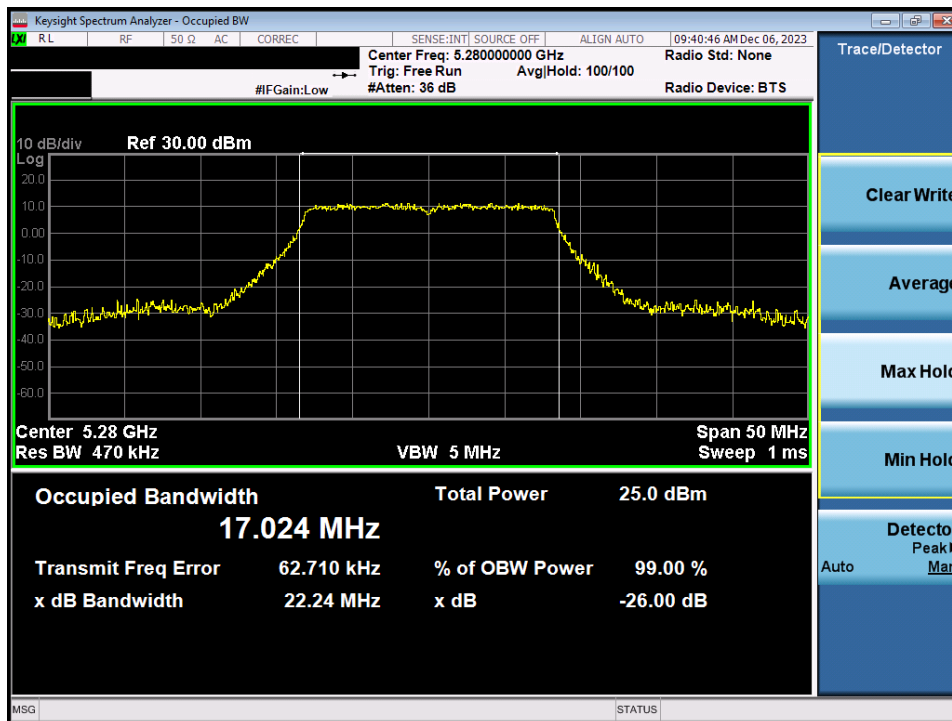
Plot 7-12. 26dB Bandwidth Plot MIMO ANT1 (802.11a (UNII Band 2A) – Ch. 56)
