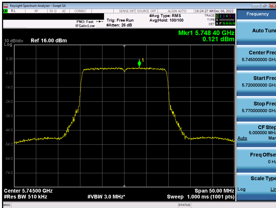
Plot 7-112. Power Spectral Density Plot MIMO ANT1 (20MHz BW 802.11ax/be (UNII Band 3) – Ch. 149)
