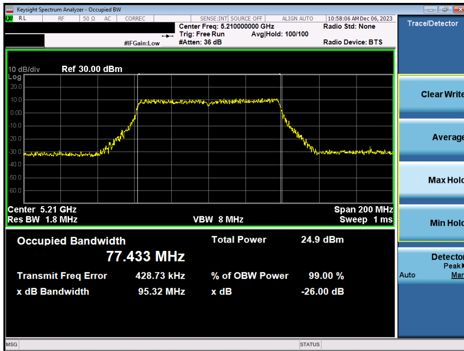
Plot 7-8. 26dB Bandwidth Plot MIMO ANT1 (80MHz BW 802.11ac (UNII Band 1) – Ch. 42)
