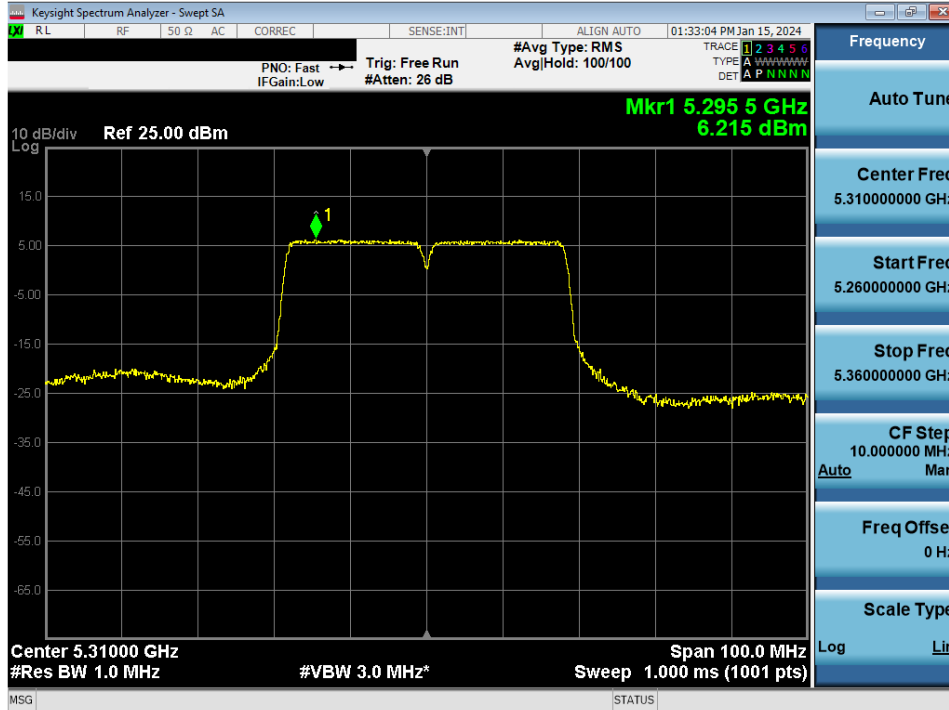
Plot 7-97. Power Spectral Density Plot MIMO ANT1 (40MHz BW 802.11n (UNII Band 2A) – Ch. 62)
