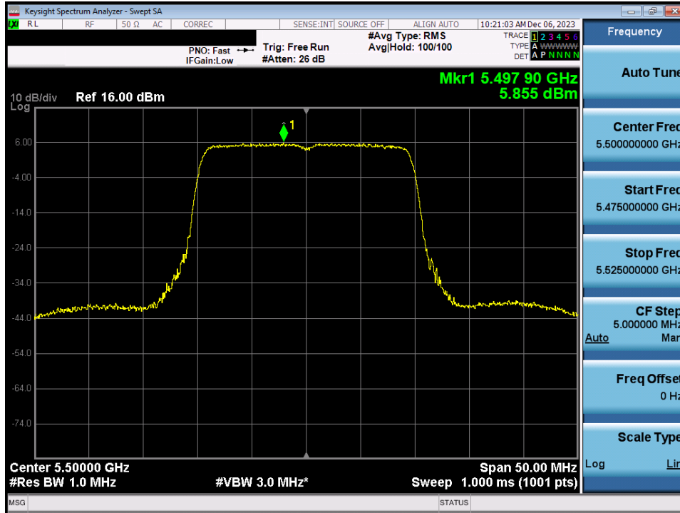
Plot 7-103. Power Spectral Density Plot MIMO ANT1 (20MHz BW 802.11ax/be (UNII Band 2C) – Ch. 100)
