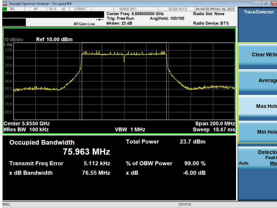
Plot 7-81. 6dB Bandwidth Plot MIMO ANT2 (80MHz BW 802.11ac (UNII Band 3/4) – Ch. 171)
