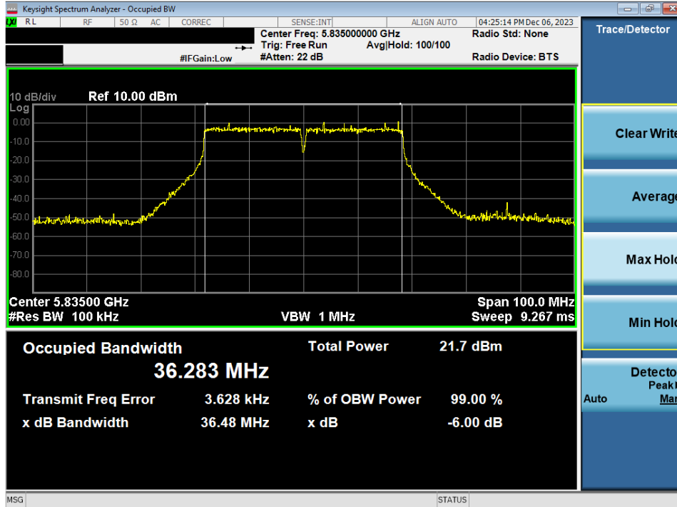
Plot 7-79. 6dB Bandwidth Plot MIMO ANT2 (40MHz BW 802.11n (UNII Band 3/4) – Ch. 167)
