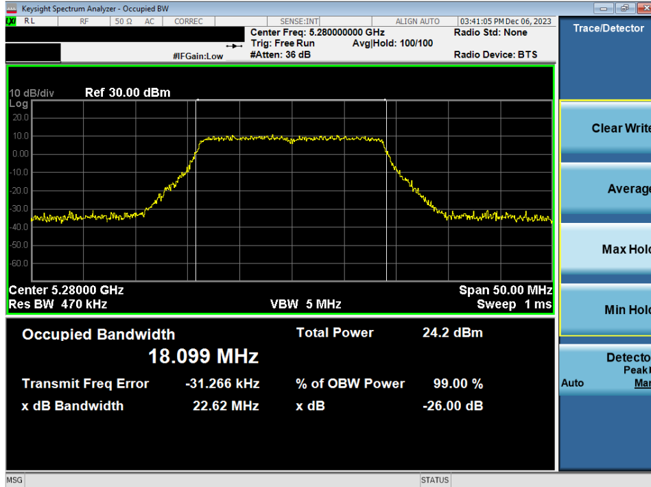
Plot 7-38. 26dB Bandwidth Plot MIMO ANT2 (20MHz BW 802.11n (UNII Band 2A) – Ch. 56)
