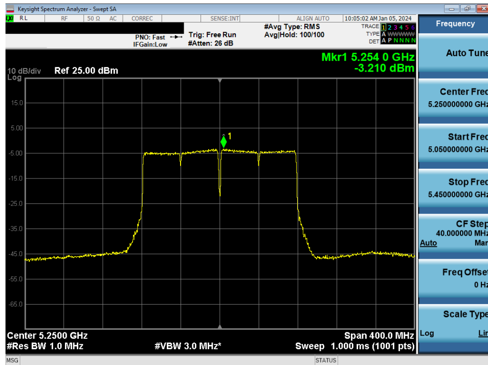
Plot 7-92. Power Spectral Density Plot MIMO ANT1 (160MHz BW 802.11ac (UNII Band 1/2A) – Ch. 50)
