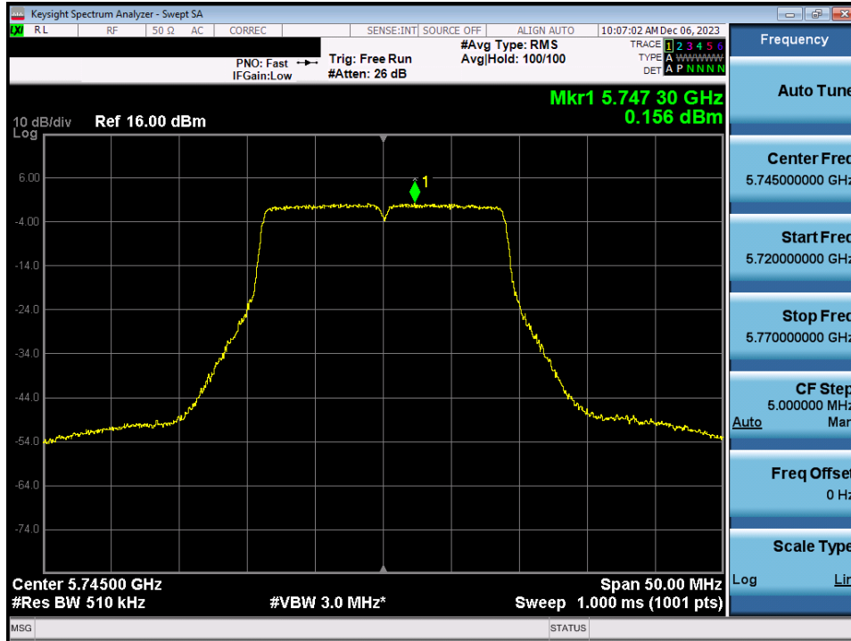
Plot 7-111. Power Spectral Density Plot MIMO ANT1 (20MHz BW 802.11n (UNII Band 3) – Ch. 149)
