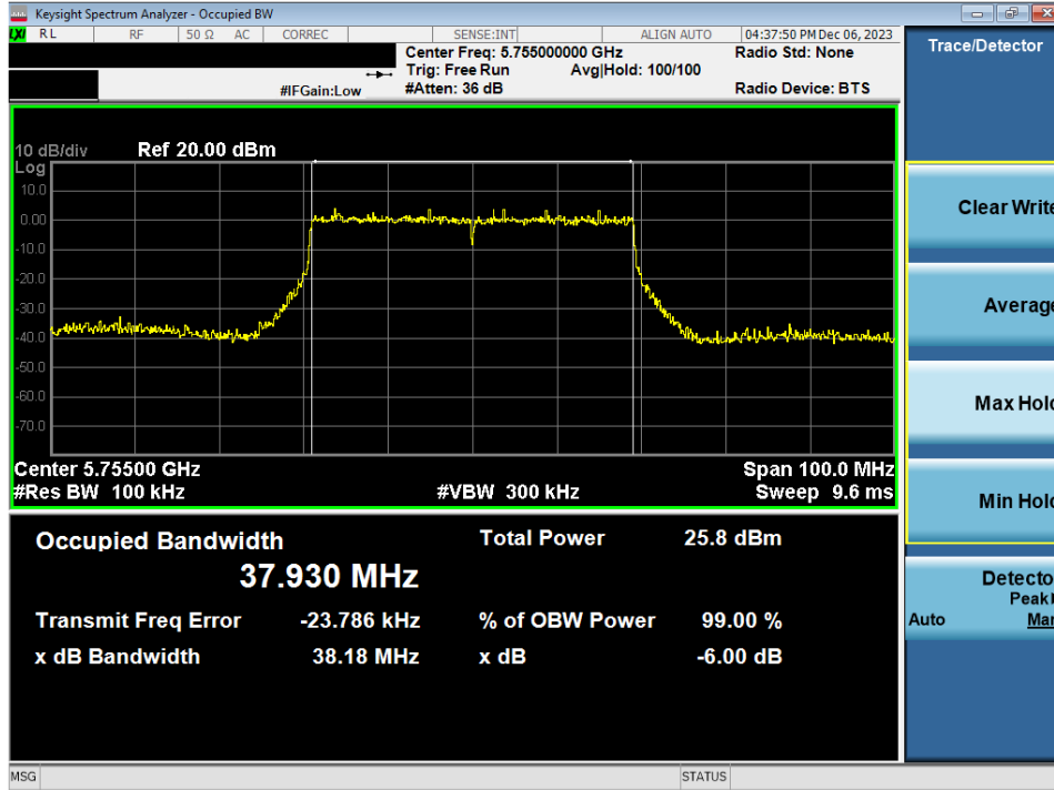
Plot 7-73. 6dB Bandwidth Plot MIMO ANT2 (40MHz BW 802.11ax/be (UNII Band 3) – Ch. 151)
