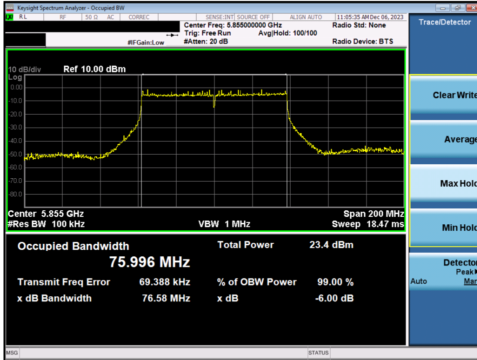
Plot 7-65. 6dB Bandwidth Plot MIMO ANT1 (80MHz BW 802.11ac (UNII Band 3/4) – Ch. 171)
