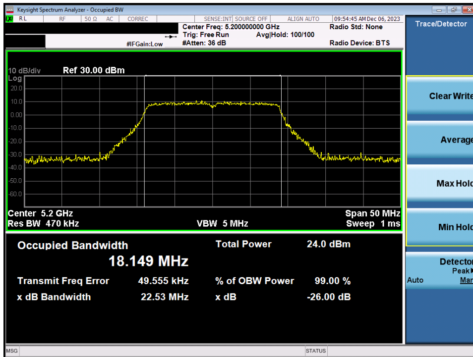
Plot 7-4. 26dB Bandwidth Plot MIMO ANT1 (20MHz BW 802.11n (UNII Band 1) – Ch. 40)
