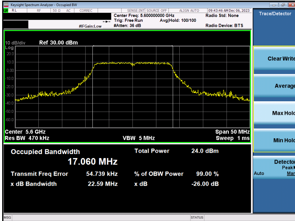
Plot 7-19. 26dB Bandwidth Plot MIMO ANT1 (802.11a (UNII Band 2C) – Ch. 120)
