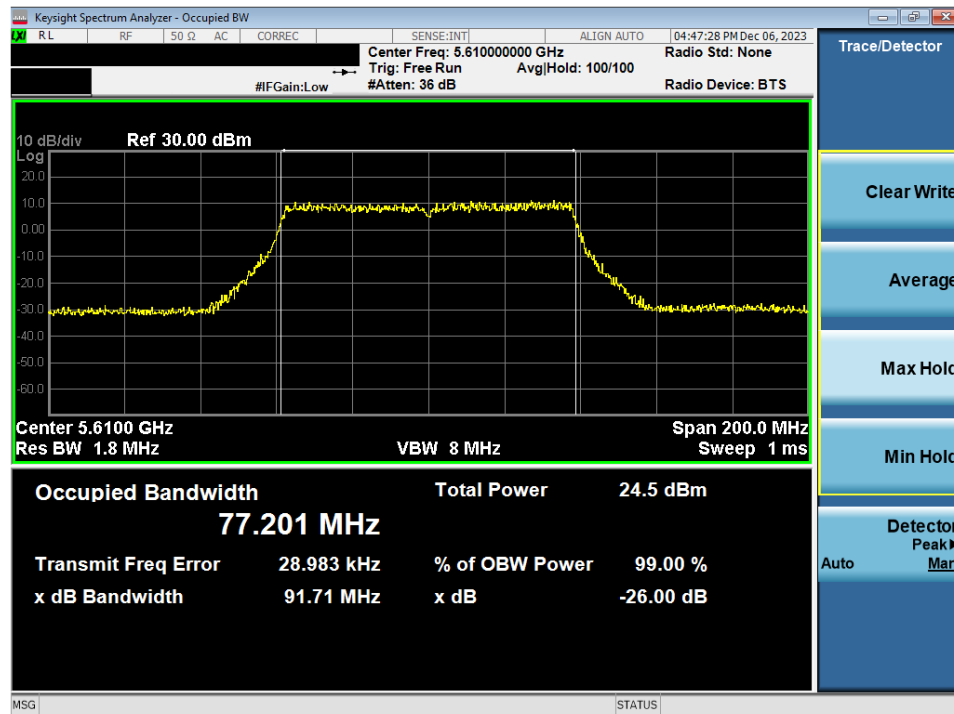
Plot 7-49. 26dB Bandwidth Plot MIMO ANT2 (80MHz BW 802.11ac (UNII Band 2C) – Ch. 122)
