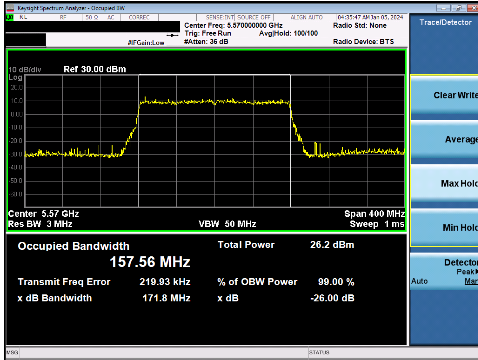
Plot 7-52. 26dB Bandwidth Plot MIMO ANT2 (160MHz BW 802.11ax/be (UNII Band 2C) – Ch. 114)
