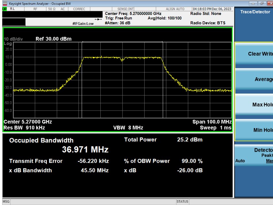
Plot 7-40. 26dB Bandwidth Plot MIMO ANT2 (40MHz BW 802.11n (UNII Band 2A) – Ch. 54)
