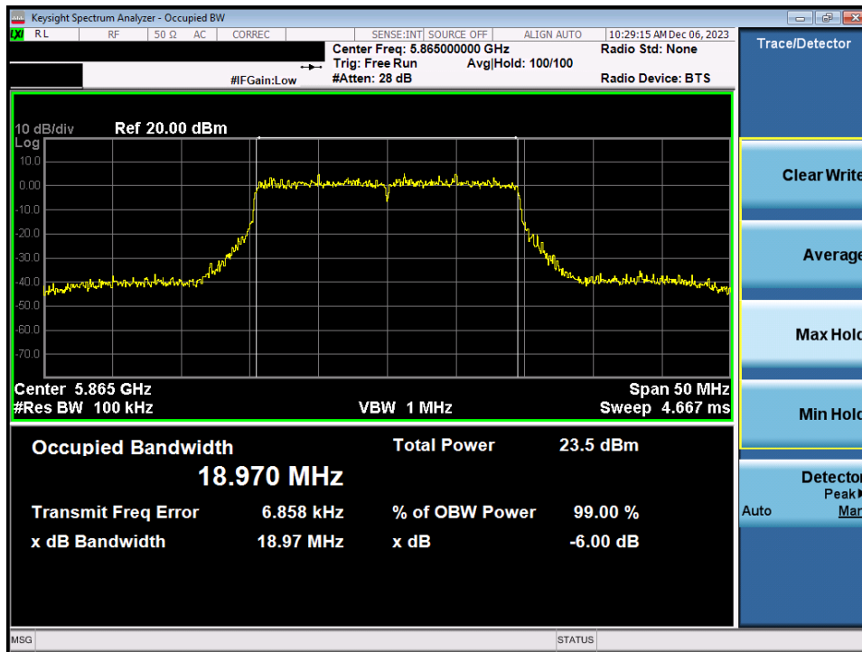
Plot 7-62. 6dB Bandwidth Plot MIMO ANT1 (20MHz BW 802.11ax/be (UNII Band 4) – Ch. 173)
