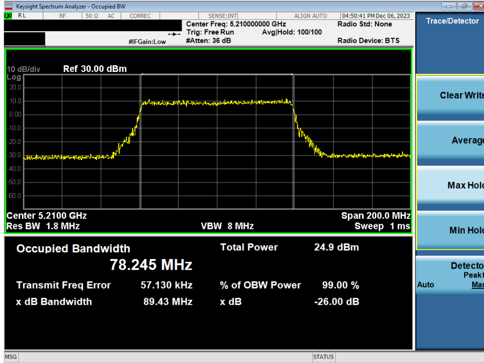
Plot 7-34. 26dB Bandwidth Plot MIMO ANT2 (80MHz BW 802.11ax/be (UNII Band 1) – Ch. 42)
