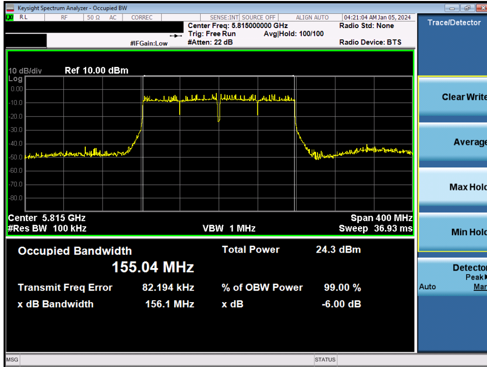
Plot 7-83. 6dB Bandwidth Plot MIMO ANT2 (160MHz BW 802.11ac (UNII Band 3/4) – Ch. 163)
