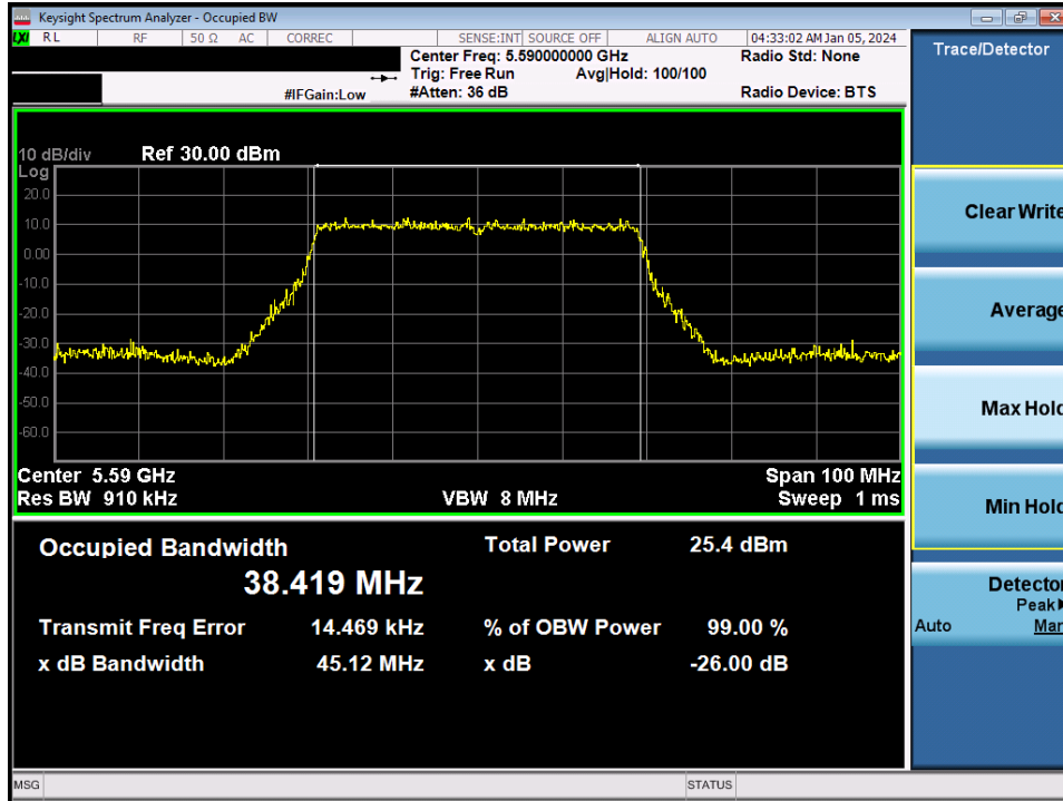
Plot 7-48. 26dB Bandwidth Plot MIMO ANT2 (40MHz BW 802.11ax/be (UNII Band 2C) – Ch. 118)
