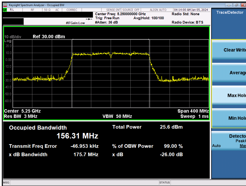
Plot 7-35. 26dB Bandwidth Plot MIMO ANT2 (160MHz BW 802.11ac (UNII Band 1/2A) – Ch. 50)
