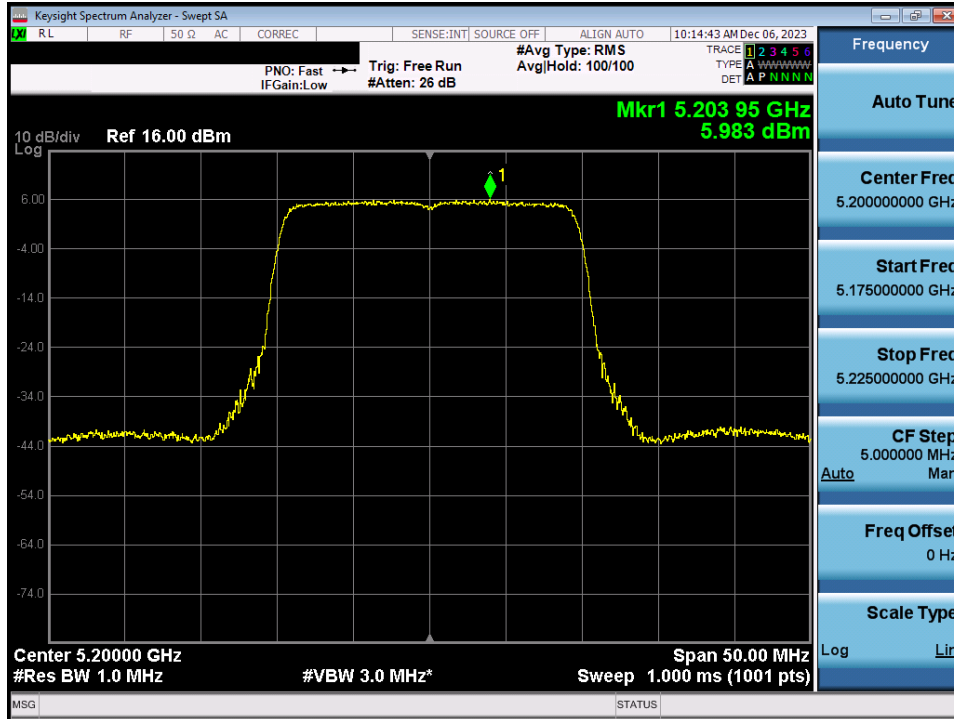
Plot 7-87. Power Spectral Density Plot MIMO ANT1 (20MHz BW 802. 11ax/be (UNII Band 1) – Ch. 40)
