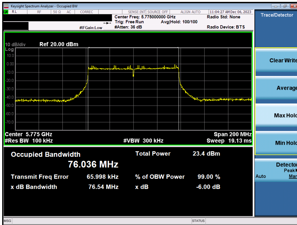
Plot 7-58. 6dB Bandwidth Plot MIMO ANT1 (80MHz BW 802.11ac (UNII Band 3) – Ch. 155)
