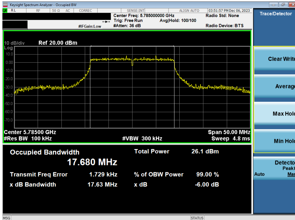
Plot 7-70. 6dB Bandwidth Plot MIMO ANT2 (20MHz BW 802.11n (UNII Band 3) – Ch. 157)
