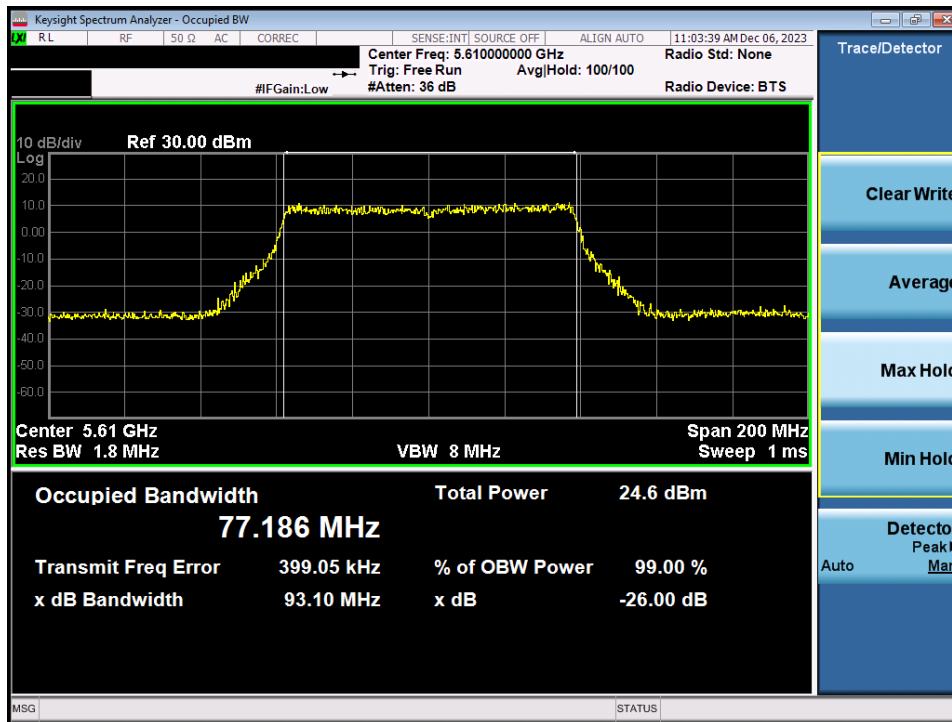
Plot 7-24. 26dB Bandwidth Plot MIMO ANT1 (80MHz BW 802.11ac (UNII Band 2C) – Ch. 122)
