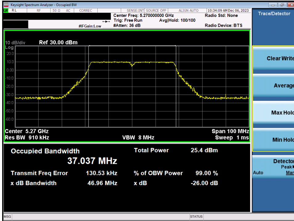
Plot 7-15. 26dB Bandwidth Plot MIMO ANT1 (40MHz BW 802.11n (UNII Band 2A) – Ch. 54)
