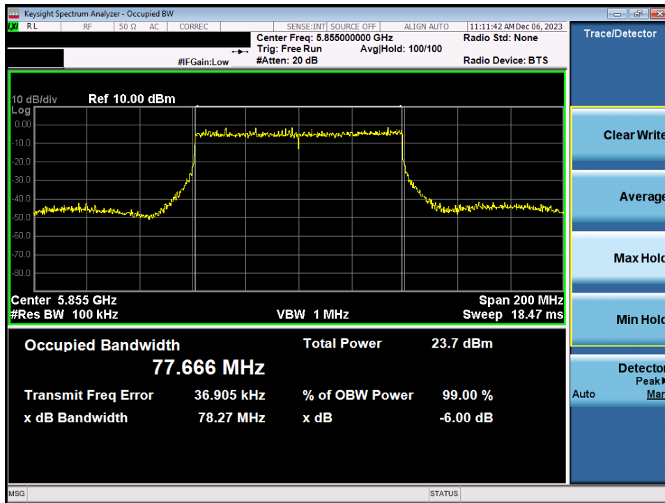
Plot 7-66. 6dB Bandwidth Plot MIMO ANT1 (80MHz BW 802.11ax/be (UNII Band 3/4) – Ch. 171)
