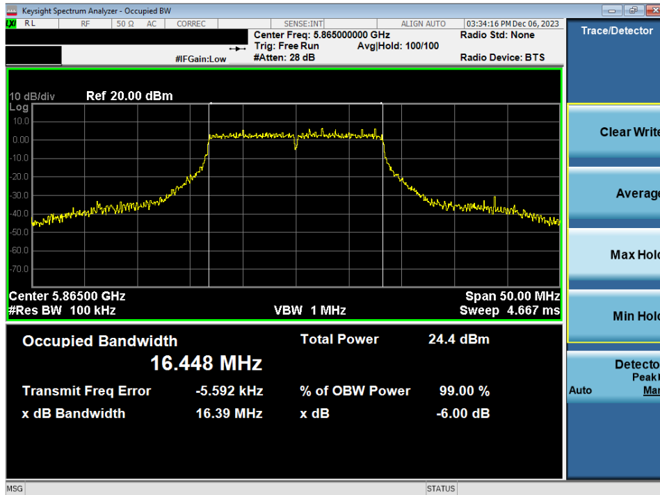
Plot 7-76. 6dB Bandwidth Plot MIMO ANT2 (20MHz BW 802.11a (UNII Band 4) – Ch. 173)
