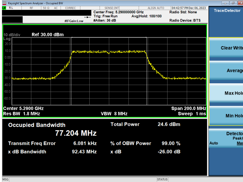
Plot 7-42. 26dB Bandwidth Plot MIMO ANT2 (80MHz BW 802.11ac (UNII Band 2A) – Ch. 58)
