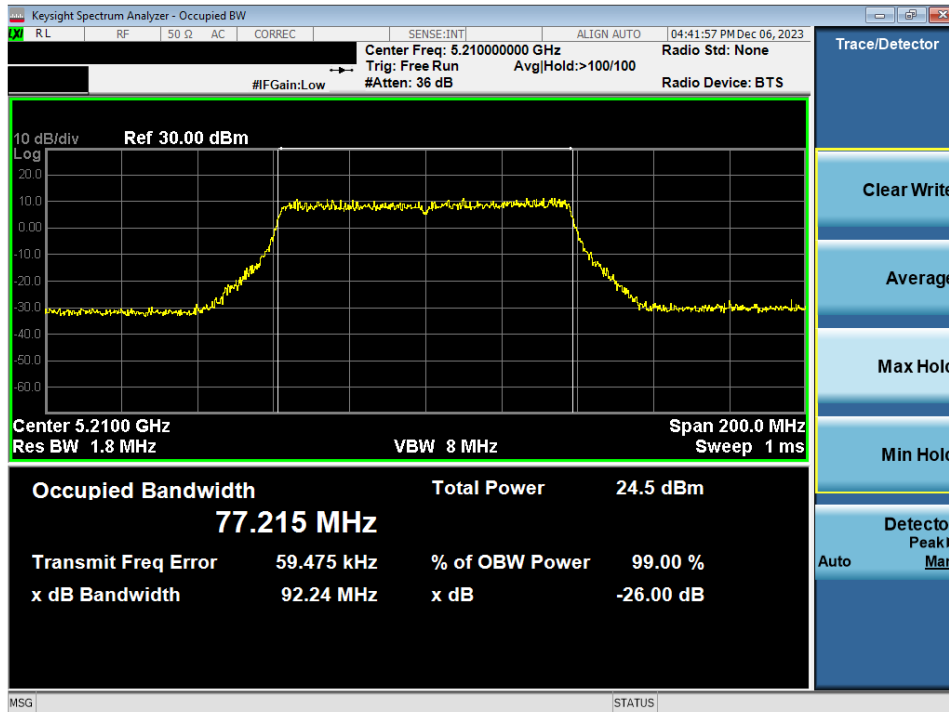
Plot 7-33. 26dB Bandwidth Plot MIMO ANT2 (80MHz BW 802.11ac (UNII Band 1) – Ch. 42)
