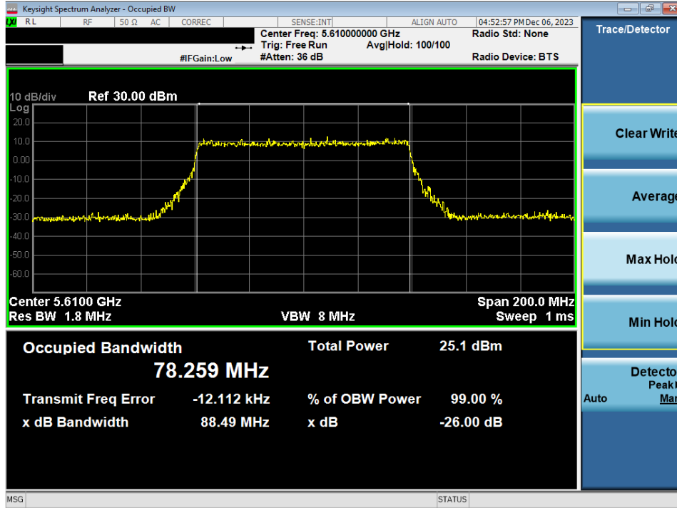
Plot 7-50. 26dB Bandwidth Plot MIMO ANT2 (80MHz BW 802.11ax/be (UNII Band 2C) – Ch. 122)
