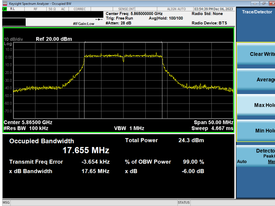
Plot 7-77. 6dB Bandwidth Plot MIMO ANT2 (20MHz BW 802.11n (UNII Band 4) – Ch. 173)
