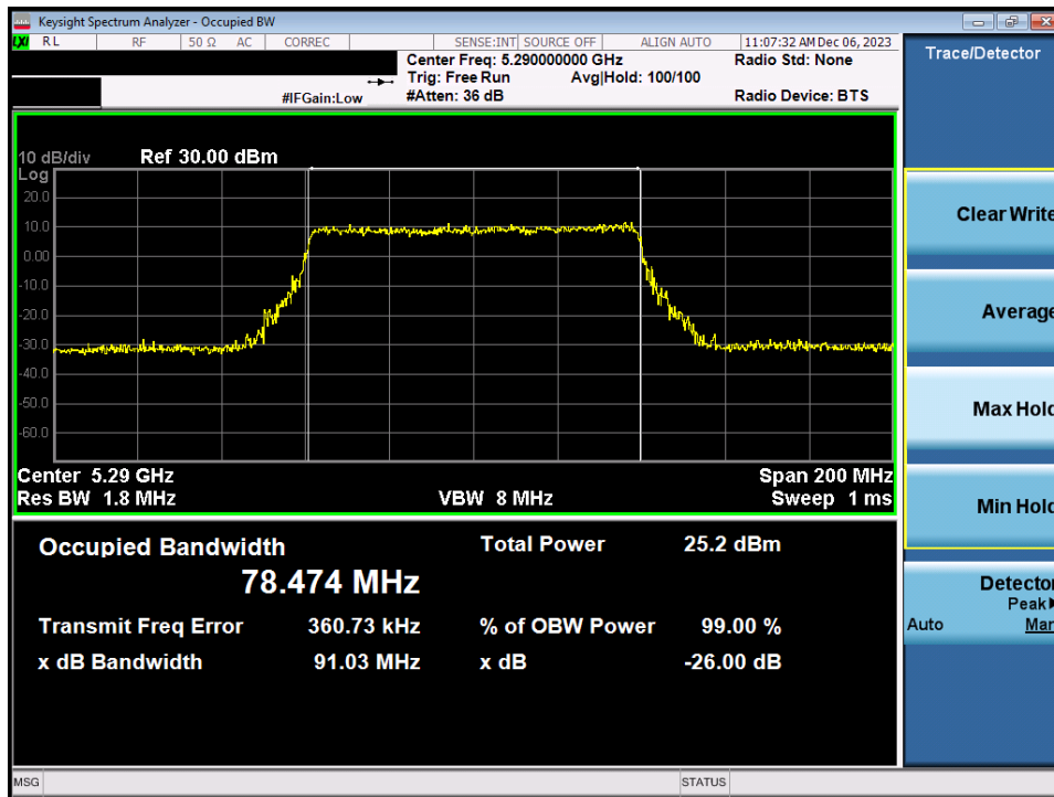
Plot 7-18. 26dB Bandwidth Plot MIMO ANT1 (80MHz BW 802.11ax/be (UNII Band 2A) – Ch. 58)
