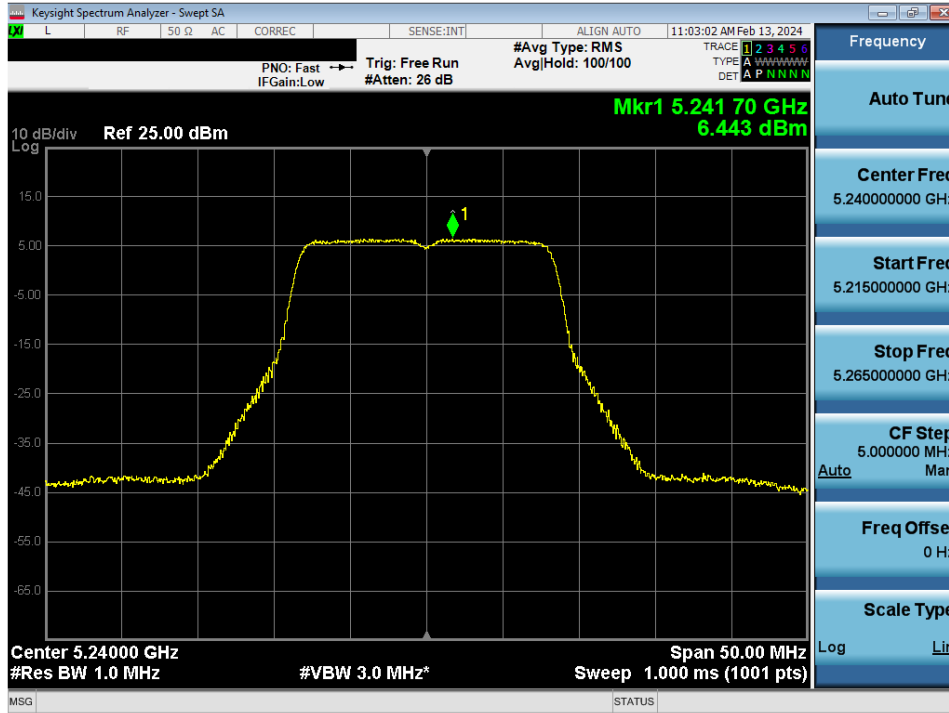
Plot 7-85. Power Spectral Density Plot MIMO ANT1 (802.11a (UNII Band 1) – Ch. 48)
