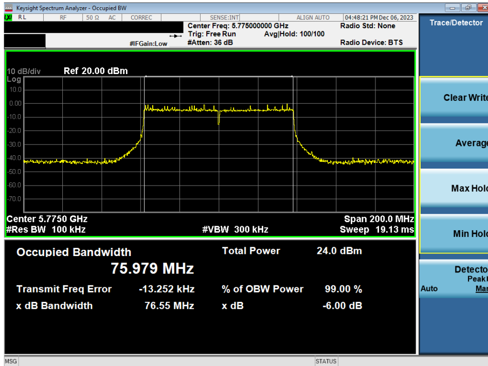
Plot 7-74. 6dB Bandwidth Plot MIMO ANT2 (80MHz BW 802.11ac (UNII Band 3) – Ch. 155)
