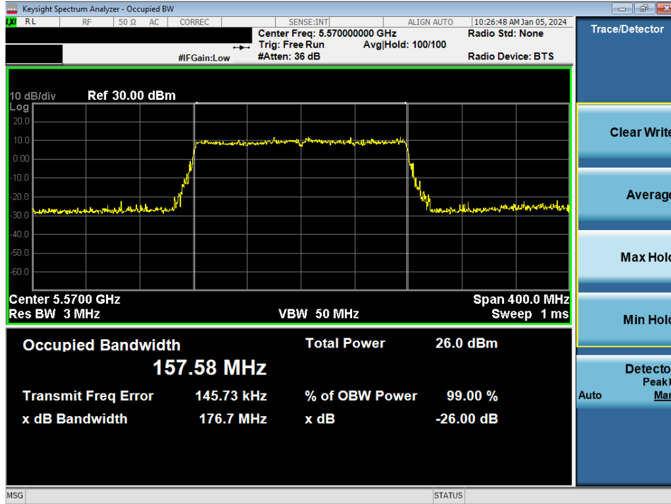
Plot 7-27. 26dB Bandwidth Plot MIMO ANT1 (160MHz BW 802.11ax/be (UNII Band 2C) – Ch. 114)
