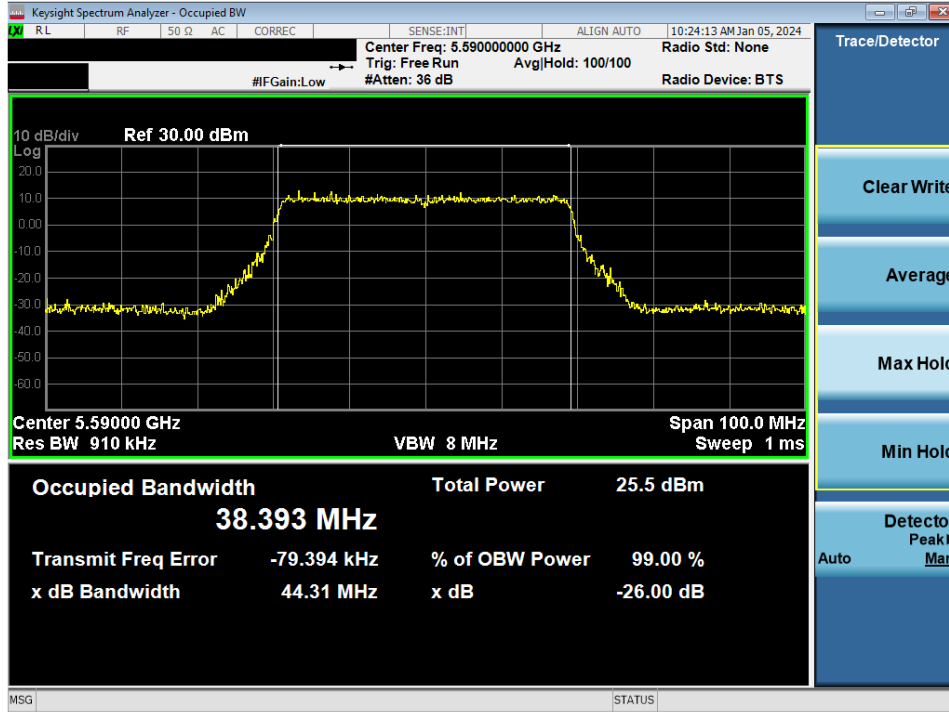
Plot 7-23. 26dB Bandwidth Plot MIMO ANT1 (40MHz BW 802.11ax/be (UNII Band 2C) – Ch. 118)
