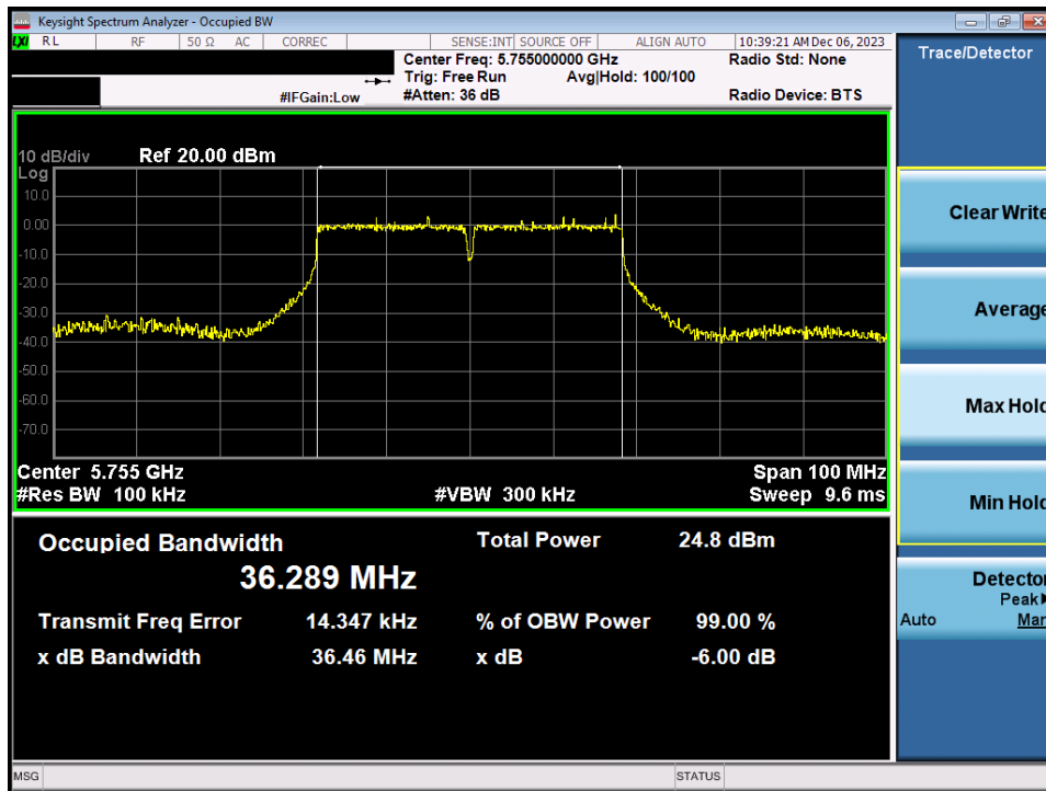
Plot 7-56. 6dB Bandwidth Plot MIMO ANT1 (40MHz BW 802.11n (UNII Band 3) – Ch. 151)
