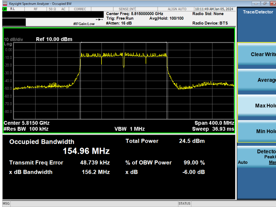
Plot 7-67. 6dB Bandwidth Plot MIMO ANT1 (160MHz BW 802.11ac (UNII Band 3/4) – Ch. 163)
