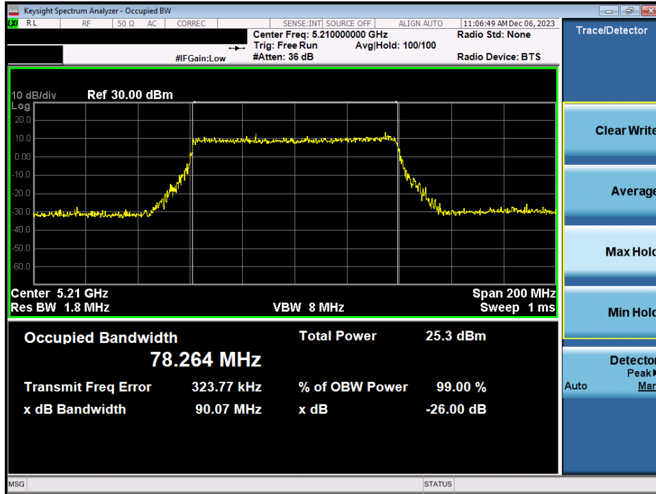
Plot 7-9. 26dB Bandwidth Plot MIMO ANT1 (80MHz BW 802.11ax/be (UNII Band 1) – Ch. 42)
