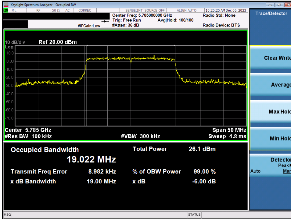
Plot 7-55. 6dB Bandwidth Plot MIMO ANT1 (20MHz BW 802.11ax/be (UNII Band 3) – Ch. 157)
