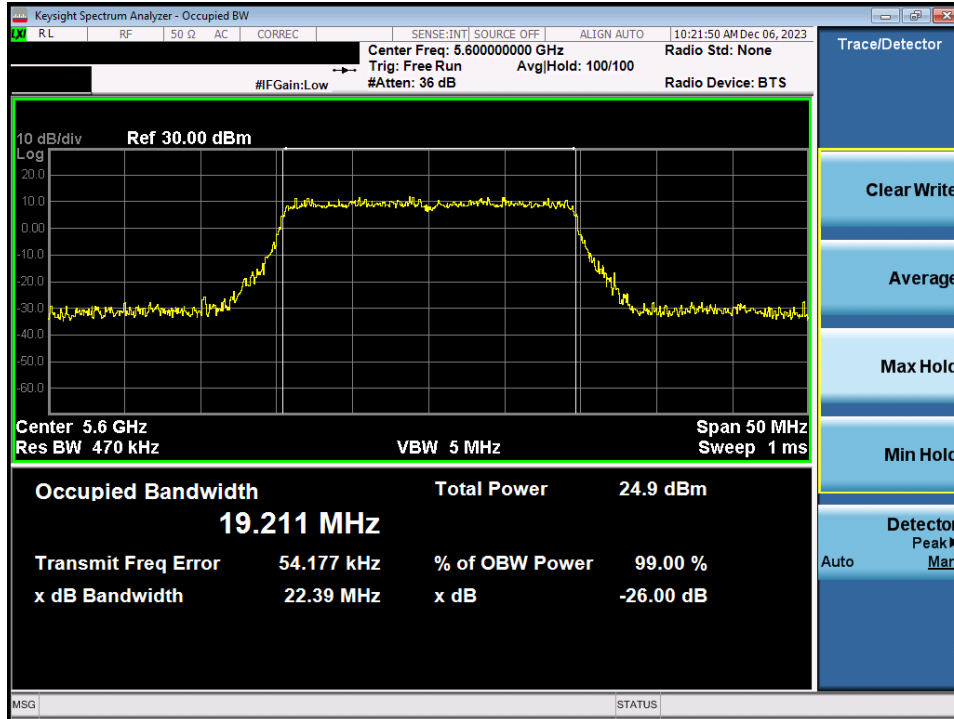
Plot 7-21. 26dB Bandwidth Plot MIMO ANT1 (20MHz BW 802.11ax/be (UNII Band 2C) – Ch. 120)
