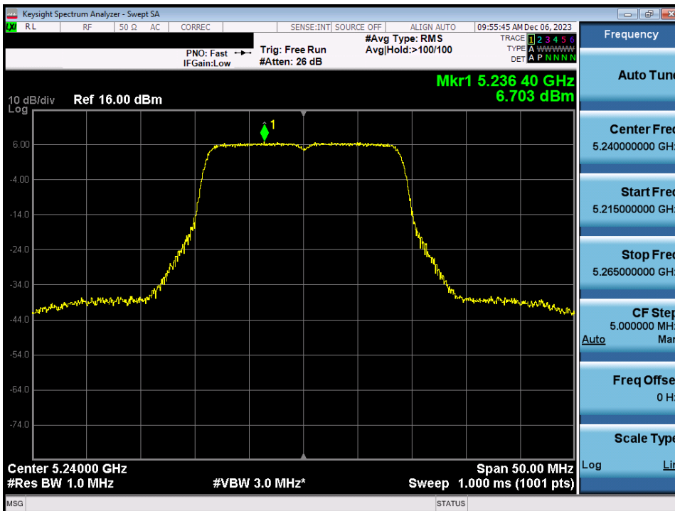
Plot 7-86. Power Spectral Density Plot MIMO ANT1 (20MHz BW 802.11n (UNII Band 1) – Ch. 48)
