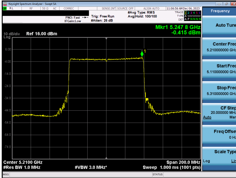
Plot 7-91. Power Spectral Density Plot MIMO ANT1 (80MHz BW 802. 11ax/be (UNII Band 1) – Ch. 42)
