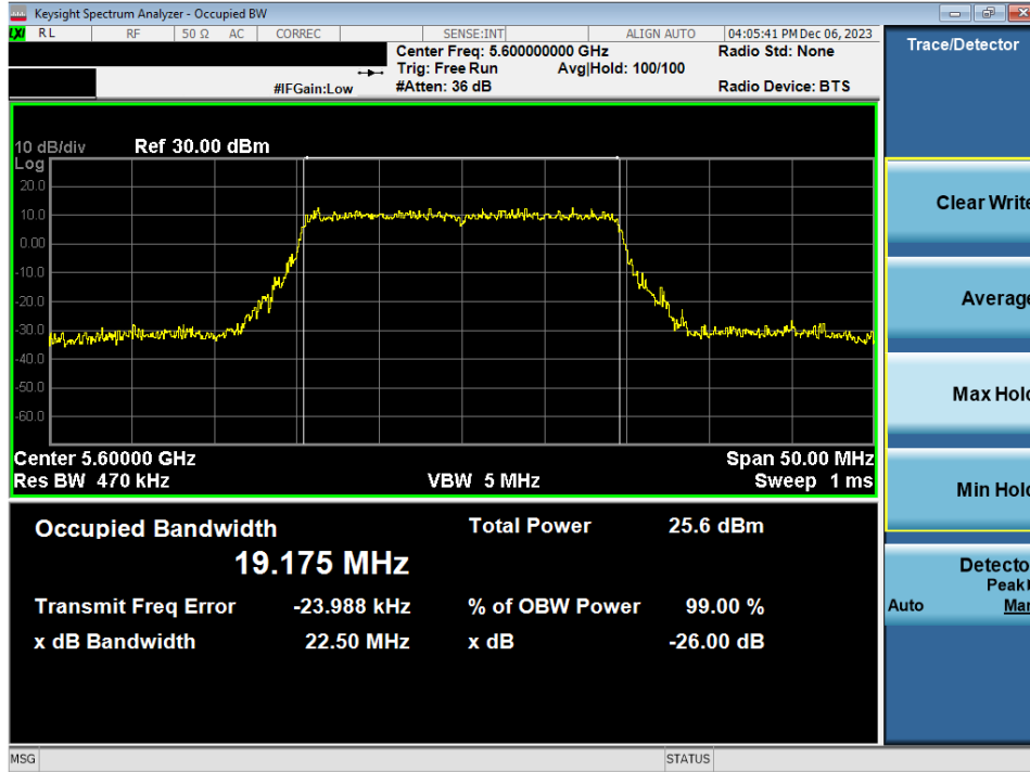
Plot 7-46. 26dB Bandwidth Plot MIMO ANT2 (20MHz BW 802.11ax/be (UNII Band 2C) – Ch. 120)
