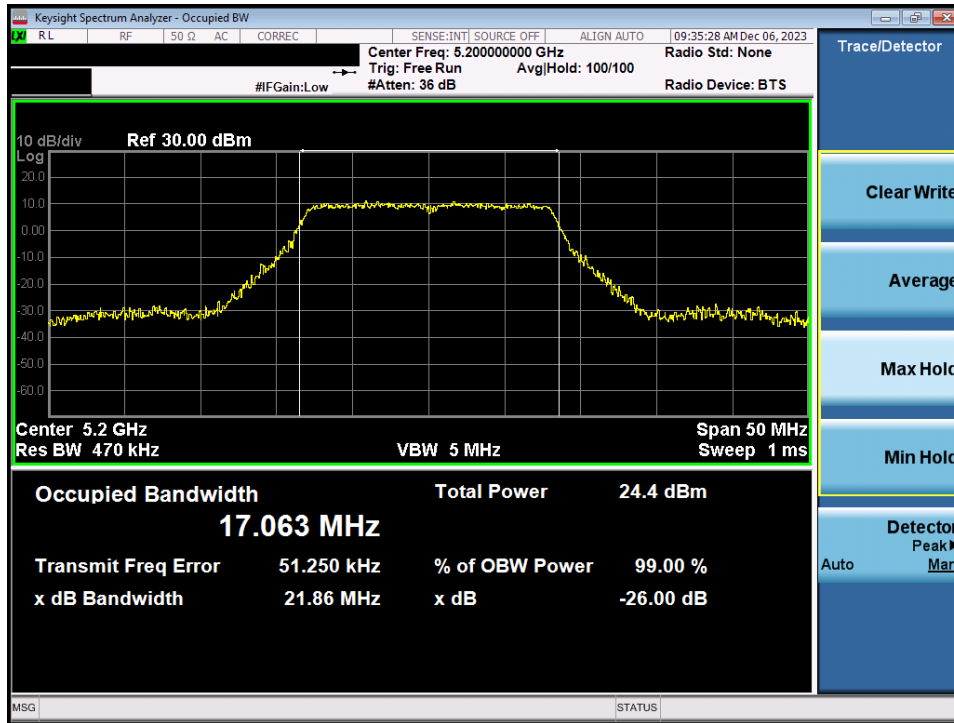
Plot 7-3. 26dB Bandwidth Plot MIMO ANT1 (802.11a (UNII Band 1) – Ch. 40)
