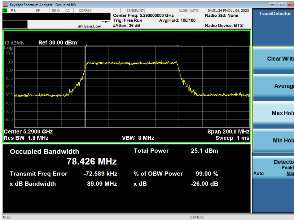
Plot 7-43. 26dB Bandwidth Plot MIMO ANT2 (80MHz BW 802.11ax/be (UNII Band 2A) – Ch. 58)
