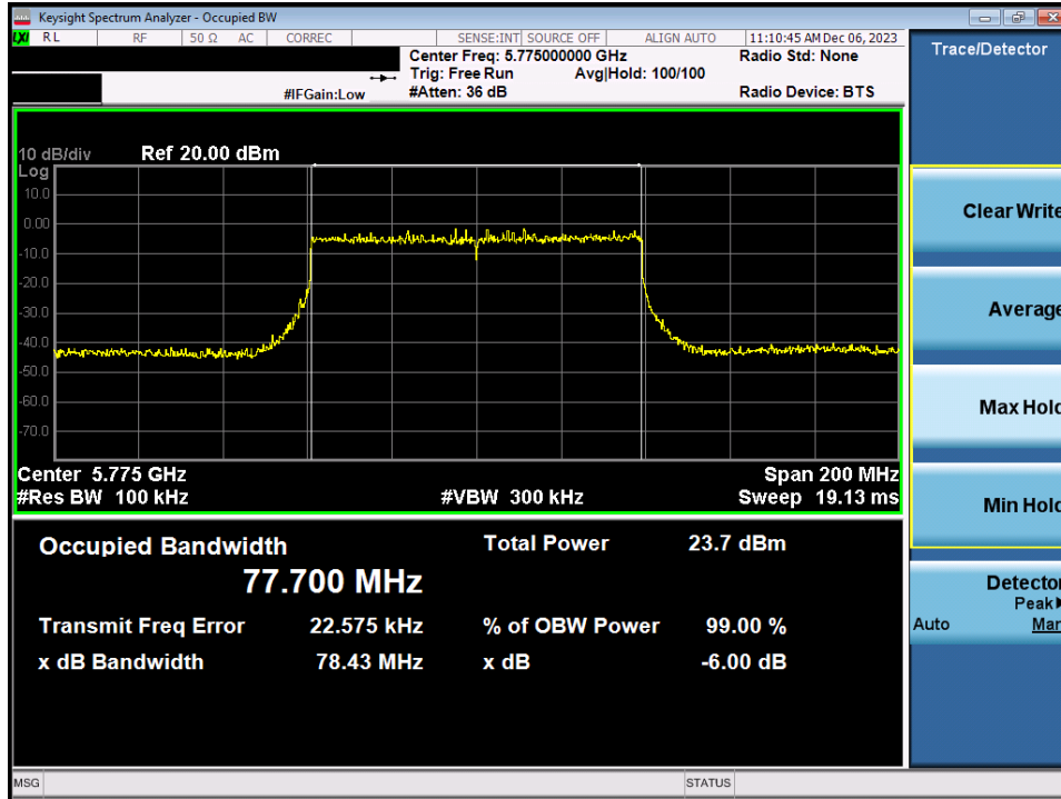
Plot 7-59. 6dB Bandwidth Plot MIMO ANT1 (80MHz BW 802.11ax/be (UNII Band 3) – Ch. 155)
