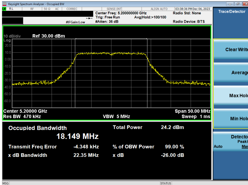
Plot 7-29. 26dB Bandwidth Plot MIMO ANT2 (20MHz BW 802.11n (UNII Band 1) – Ch. 40)
