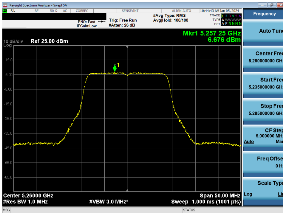
Plot 7-94. Power Spectral Density Plot MIMO ANT1 (802.11a (UNII Band 2A) – Ch. 52)
