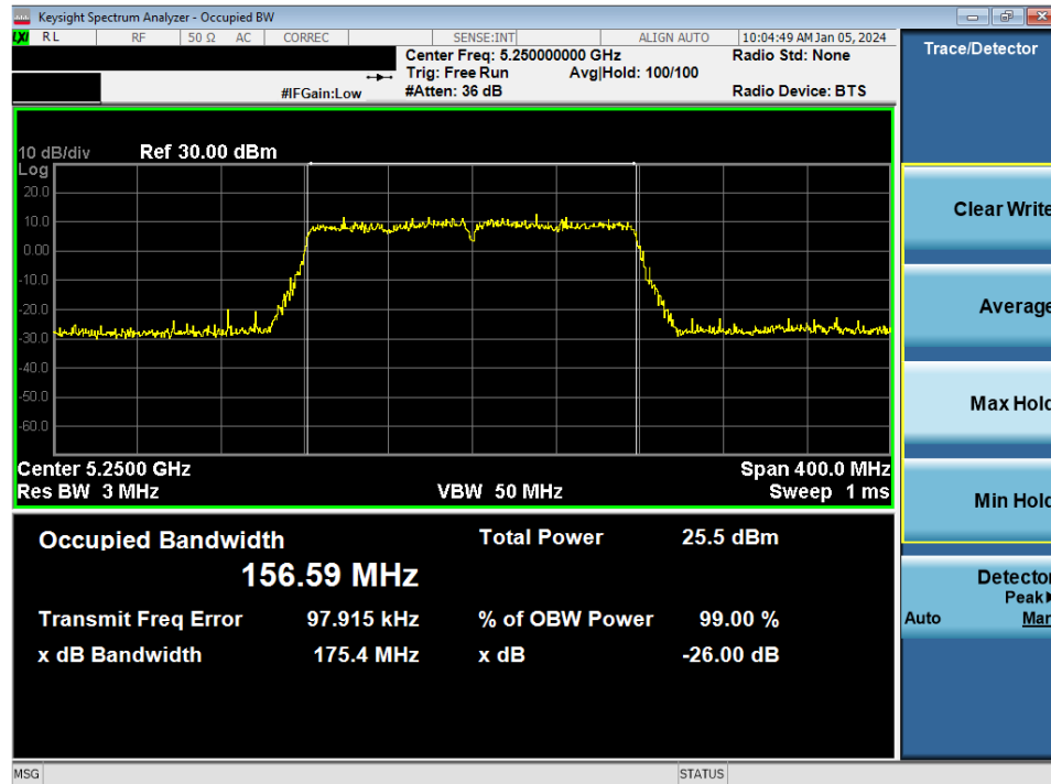
Plot 7-10. 26dB Bandwidth Plot MIMO ANT1 (160MHz BW 802.11ac (UNII Band 1/2A) – Ch. 50)
