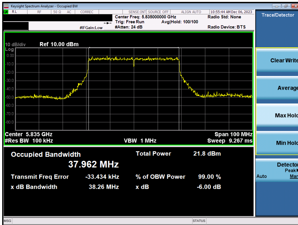
Plot 7-64. 6dB Bandwidth Plot MIMO ANT1 (40MHz BW 802.11ax/be (UNII Band 3/4) – Ch. 167)
