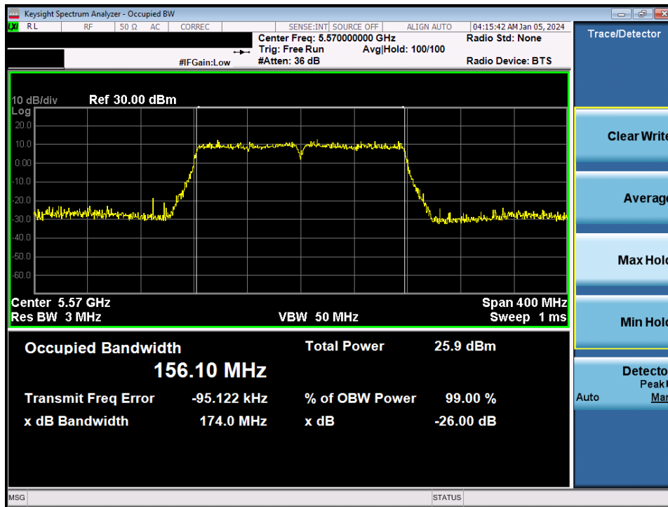
Plot 7-51. 26dB Bandwidth Plot MIMO ANT2 (160MHz BW 802.11ac (UNII Band 2C) – Ch. 114)
