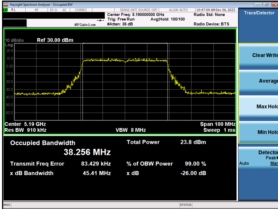
Plot 7-7. 26dB Bandwidth Plot MIMO ANT1 (40MHz BW 802.11ax/be (UNII Band 1) – Ch. 38)
