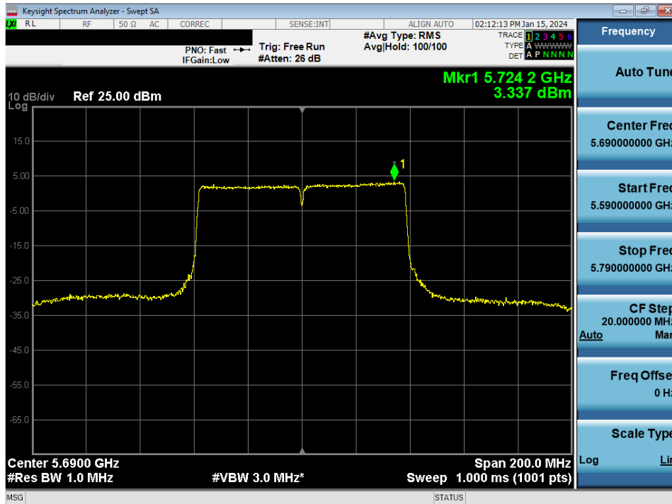
Plot 7-106. Power Spectral Density Plot MIMO ANT1 (80MHz BW 802.11ac (UNII Band 2C) – Ch. 138)
