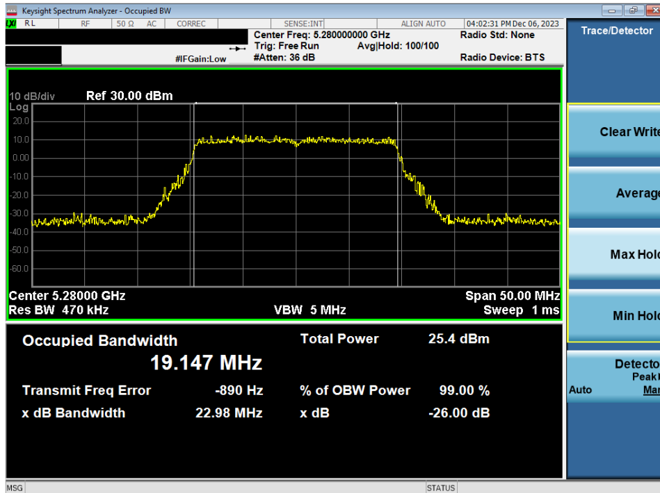
Plot 7-39. 26dB Bandwidth Plot MIMO ANT2 (20MHz BW 802.11ax/be (UNII Band 2A) – Ch. 56)
