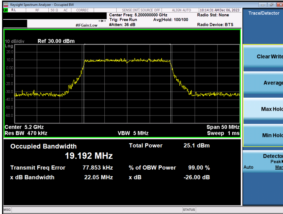
Plot 7-5. 26dB Bandwidth Plot MIMO ANT1 (20MHz BW 802. 11ax/be (UNII Band 1) – Ch. 40)
