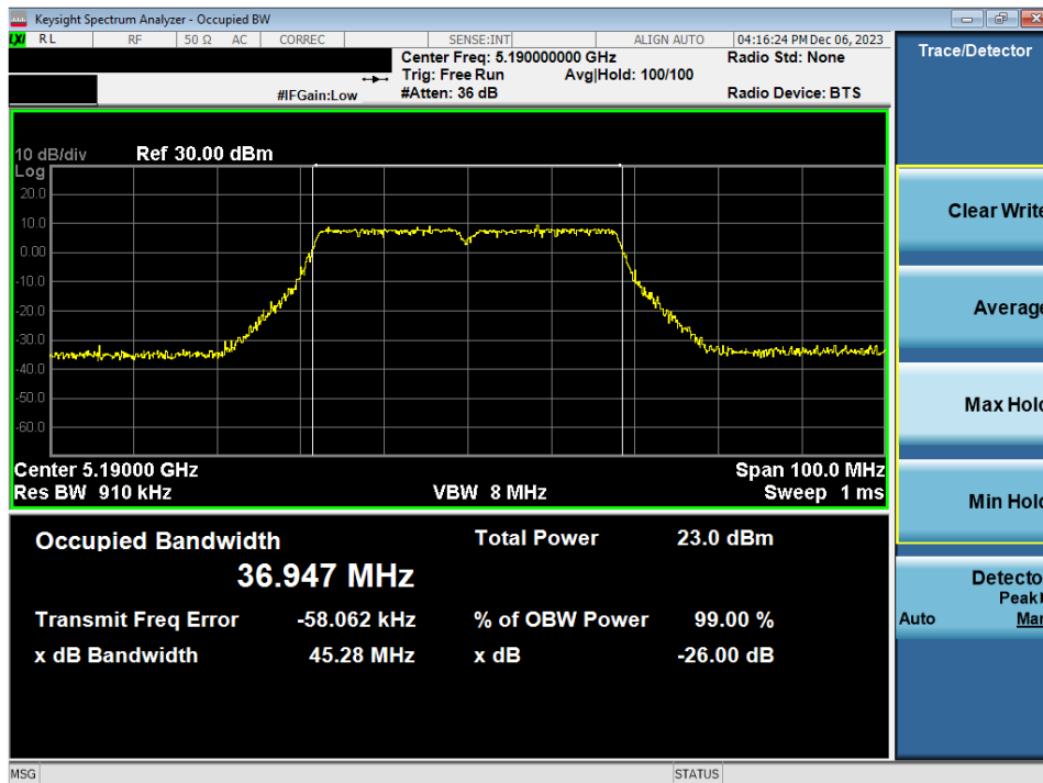
Plot 7-31. 26dB Bandwidth Plot MIMO ANT2 (40MHz BW 802.11n (UNII Band 1) – Ch. 38)
