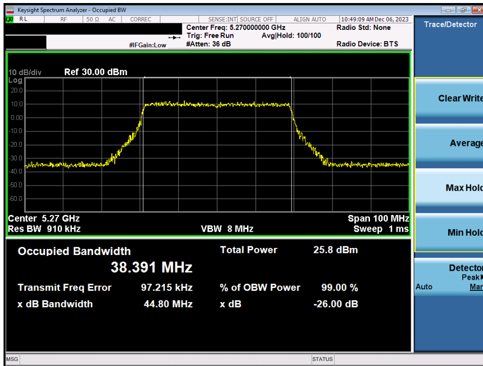
Plot 7-16. 26dB Bandwidth Plot MIMO ANT1 (40MHz BW 802.11ax/be (UNII Band 2A) – Ch. 54)
