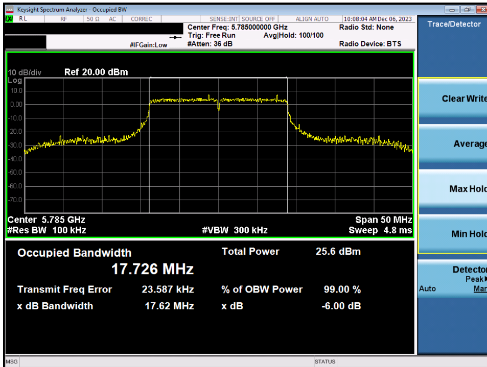
Plot 7-54. 6dB Bandwidth Plot MIMO ANT1 (20MHz BW 802.11n (UNII Band 3) – Ch. 157)
