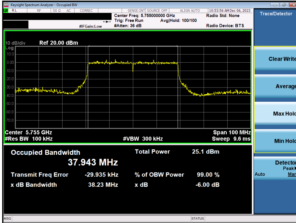
Plot 7-57. 6dB Bandwidth Plot MIMO ANT1 (40MHz BW 802.11ax/be (UNII Band 3) – Ch. 151)
