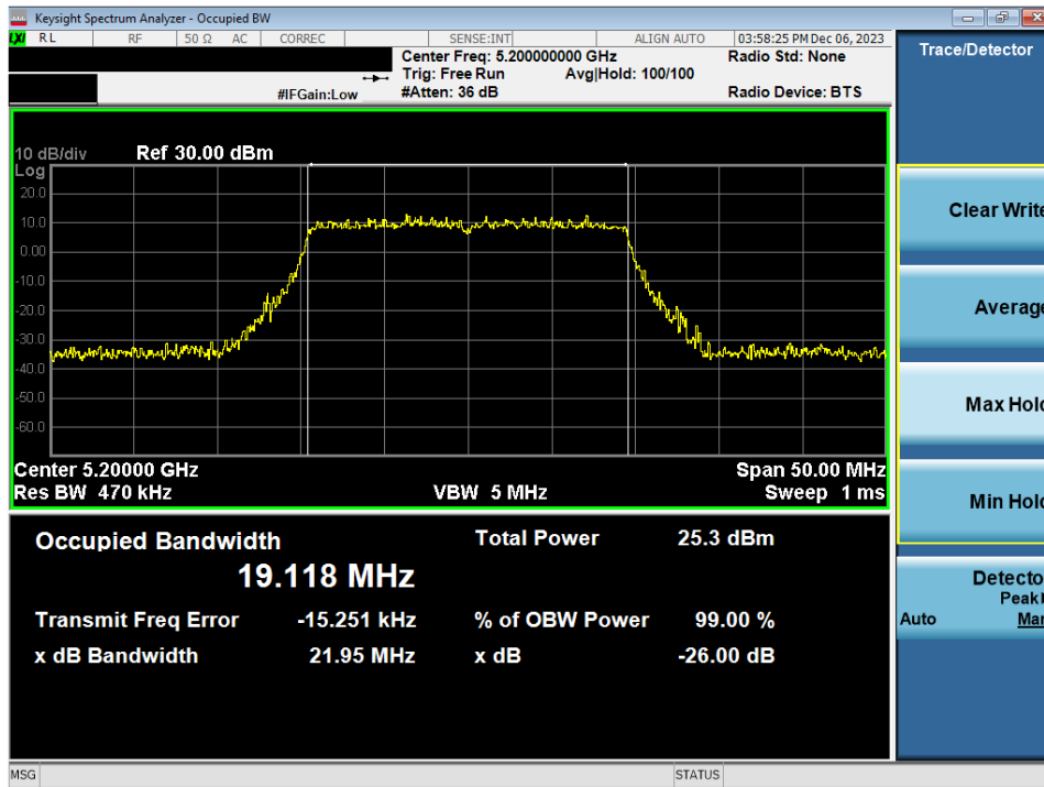
Plot 7-30. 26dB Bandwidth Plot MIMO ANT2 (20MHz BW 802. 11ax/be (UNII Band 1) – Ch. 40)
