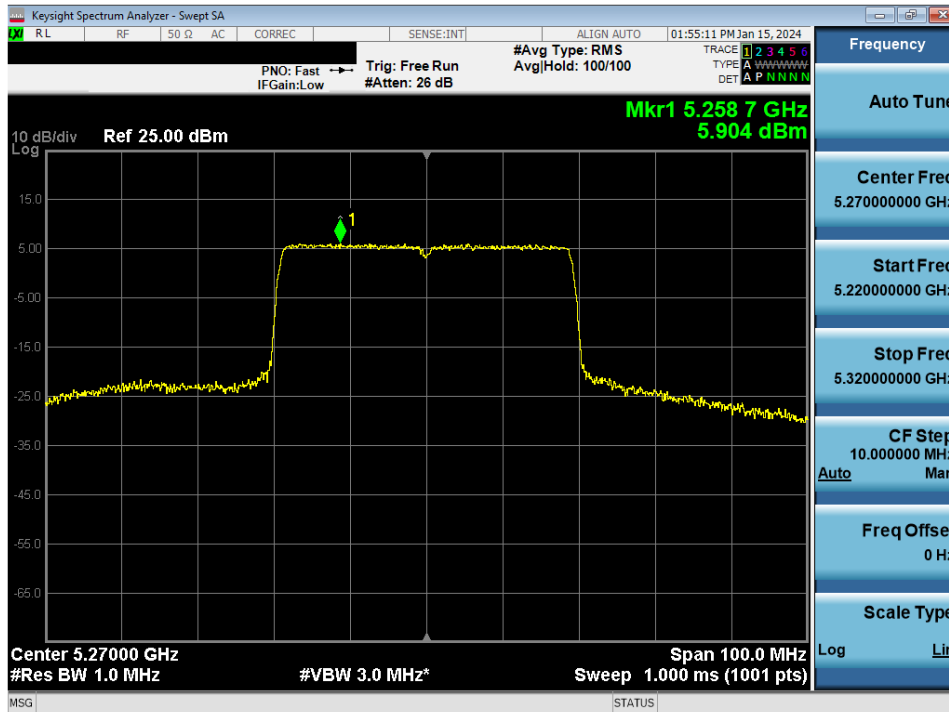
Plot 7-98. Power Spectral Density Plot MIMO ANT1 (40MHz BW 802.11ax/be (UNII Band 2A) – Ch. 54)
