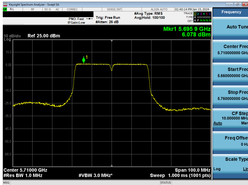
Plot 7-104. Power Spectral Density Plot MIMO ANT1 (40MHz BW 802.11n (UNII Band 2C) – Ch. 142)
