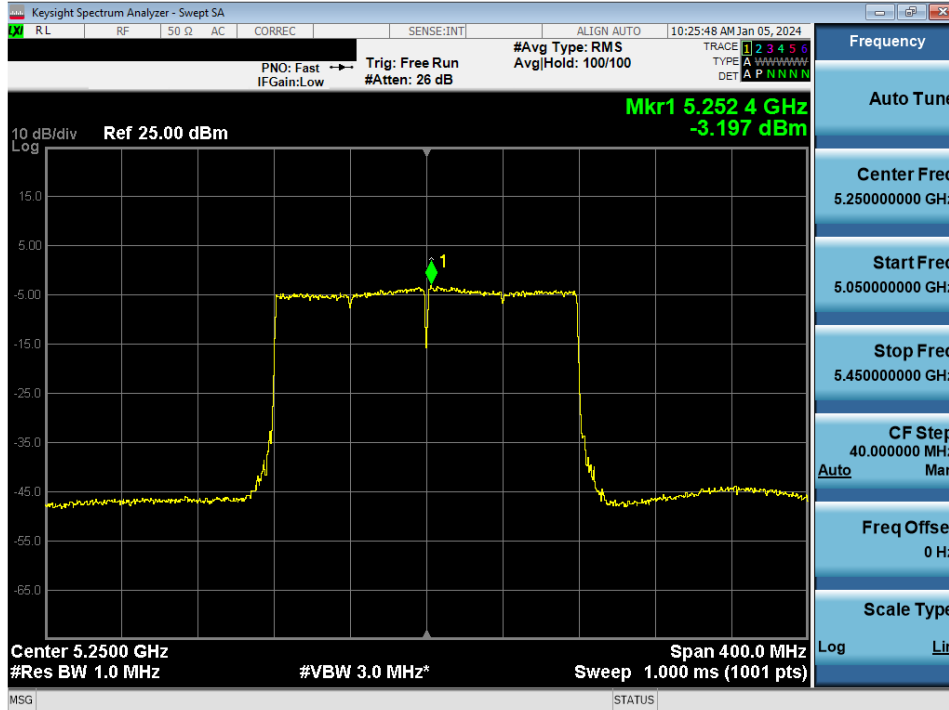
Plot 7-93. Power Spectral Density Plot MIMO ANT1 (160MHz BW 802. 11ax/be (UNII Band 1/2A) – Ch. 50)
