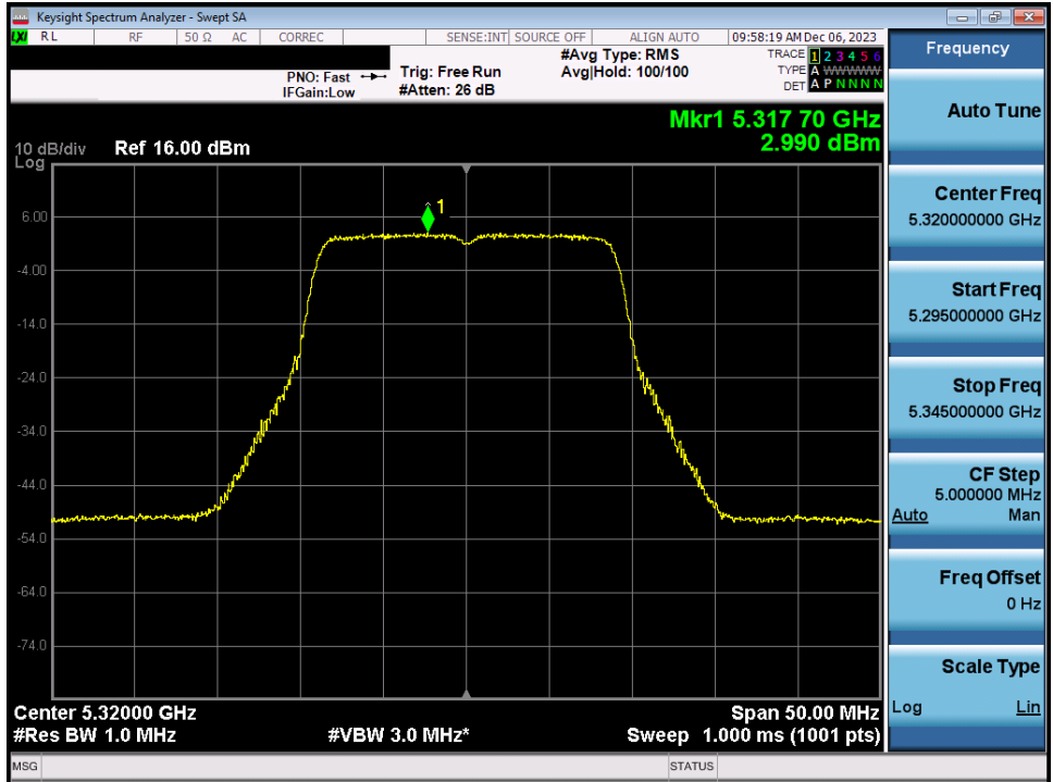
Plot 7-95. Power Spectral Density Plot MIMO ANT1 (20MHz BW 802.11n (UNII Band 2A) – Ch. 64)
