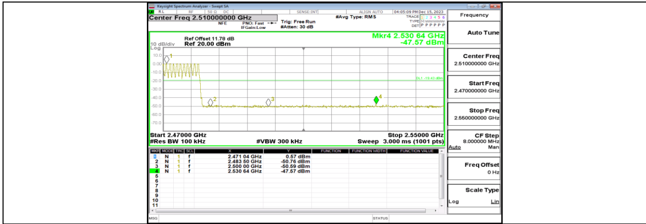
DH5_Ant1_High_Hop_2480
