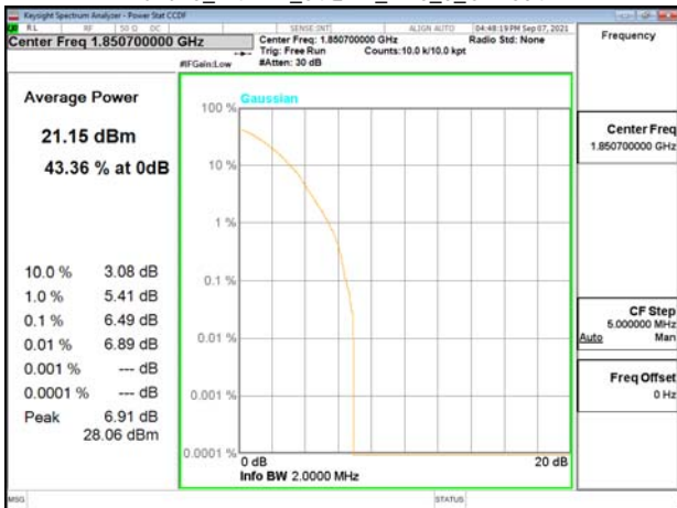
Band25_1.4MHz_64QAM_RB6_0_CH26047
