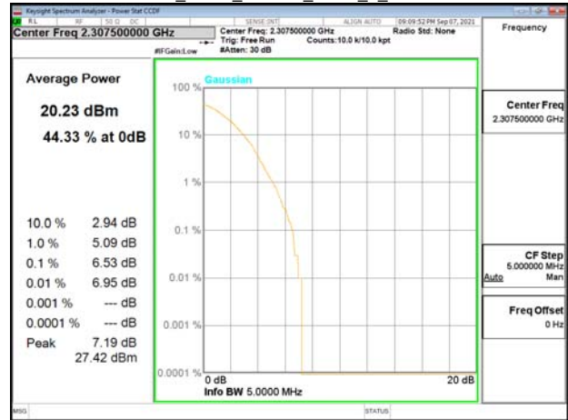
Band30_5MHz_64QAM_RB25_0_CH27710
