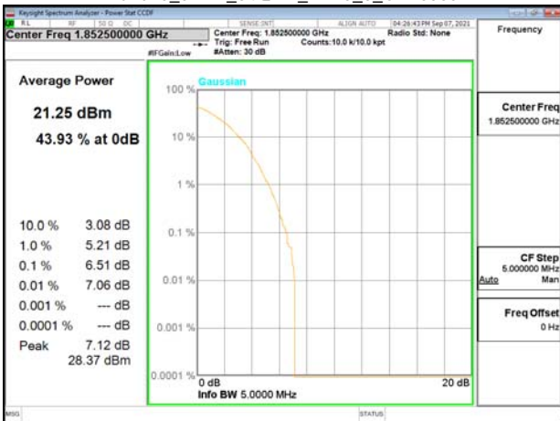
Band25_5MHz_64QAM_RB25_0_CH26065
