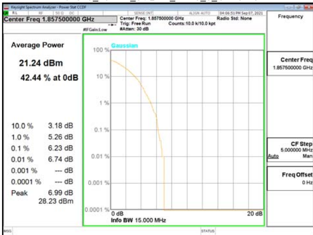
Band25_15MHz_64QAM_RB75_0_CH26115
