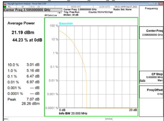
Band38_20MHz_64QAM_RB100_0_CH38000
