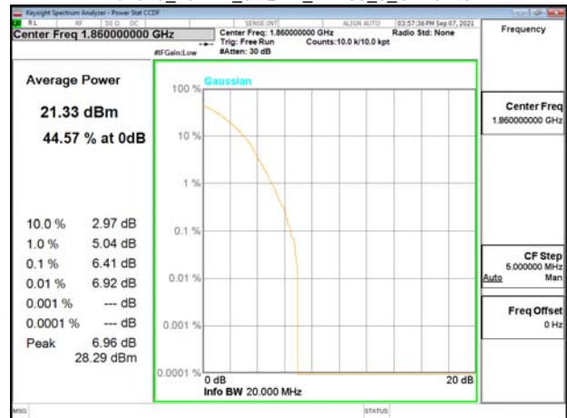
Band25_20MHz_64QAM_RB100_0_CH26140
