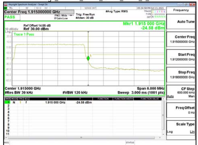
Band Edge_Band25_3MHz_QPSK_RB15_0_CH26675
