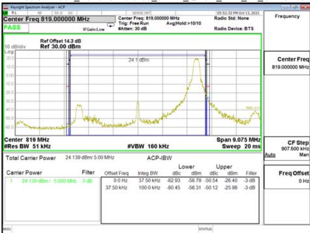
Emission Mask_Band26-Part90s_5MHz_QPSK_RB1_24_CH26740
