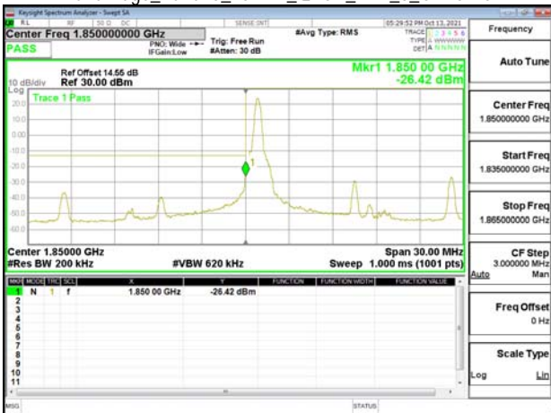
Band Edge_Band25_15MHz_QPSK_RB1_0_CH26115
