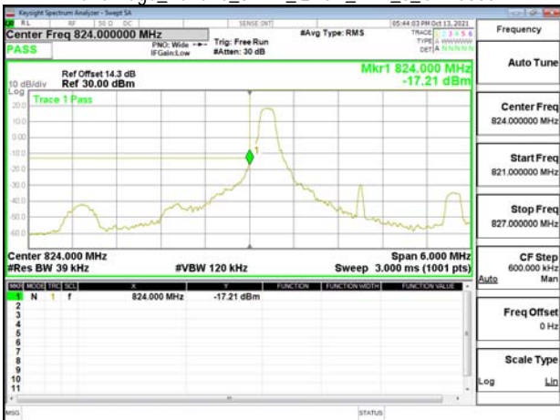
Band Edge_Band26_3MHz_QPSK_RB1_0_CH26805
