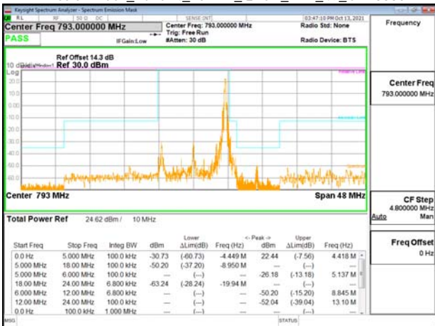
Emission Mask_Band14_10MHz_OPSK_RB1_49_CH23330
