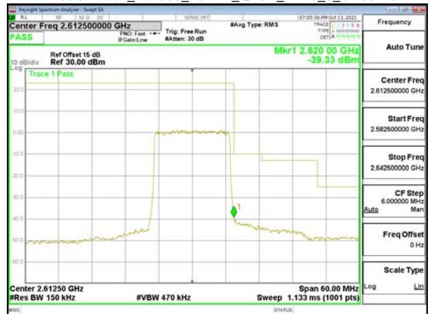
Emission Mask_Band38_15MHz_QPSK_RB75_0_CH38175
