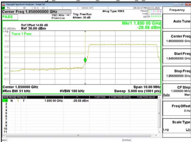
Band Edge_Band25_5MHz_OPSK_RB25_0_CH26065
