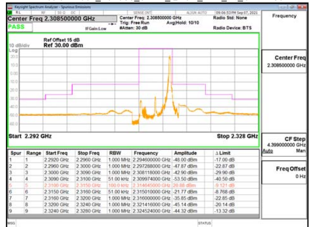
Emission Mask_Band30_5MHz_OPSK_RB1_24_CH27735
