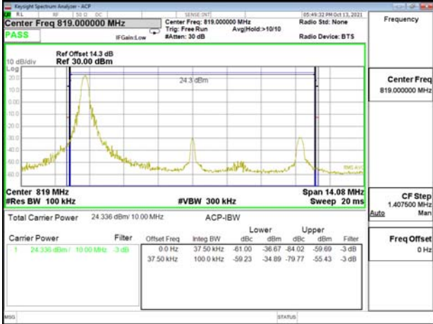
Emission Mask_Band26-Part90s_10MHz_QPSK_RB1_49_CH26740
