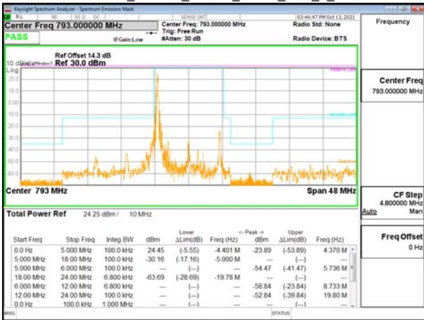
Emission Mask_Band14_10MHz_OPSK_RB1_49_CH23330
