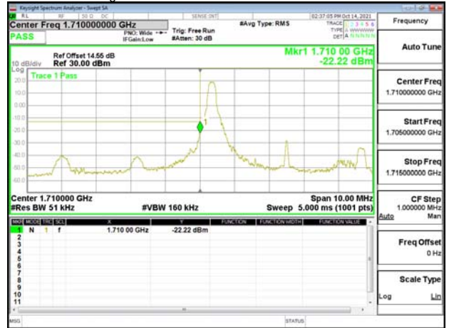
Band Edge_Band66_5MHz_QPSK_RB1_24_CH132647
