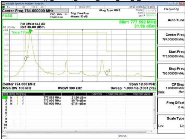
Band Edge_Band13_10MHz_OPSK_RB1_49_CH23230
