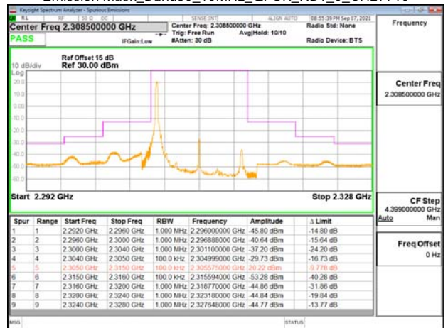
Emission Mask_Band30_10MHz_OPSK_RB1_49_CH27710
