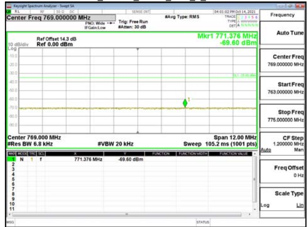
Band13_10MHz_OPSK_RB1_49_CH23230
