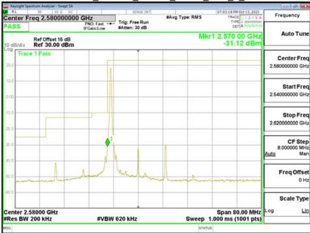
Emission Mask_Band38_20MHz_QPSK_RB1_99_CH38150
