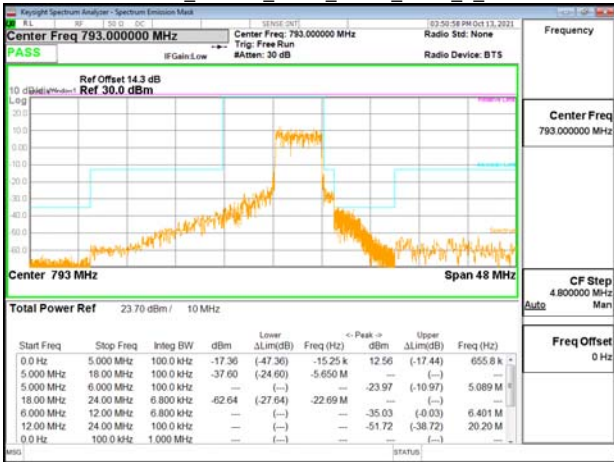
Emission Mask_Band14_10MHz_OPSK_RB1_0_CH23330
