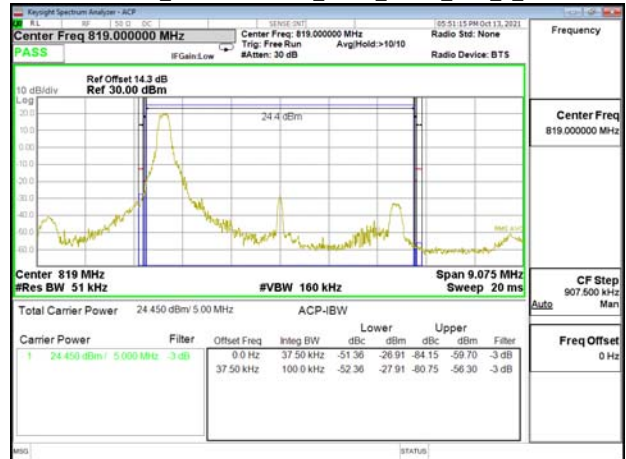
Emission Mask_Band26-Part90s_5MHz_OPSK_RB1_0_CH26740
