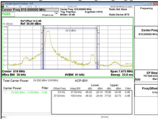
Emission Mask_Band26-Part90s_3MHz_QPSK_RB1_0_CH26740
