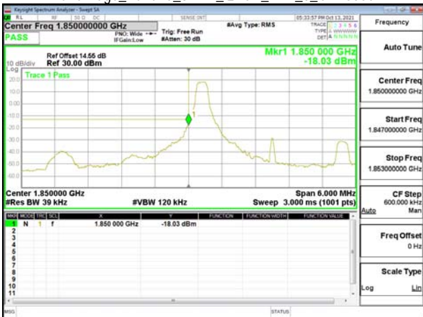
Band Edge_Band25_3MHz_QPSK_RB1_0_CH26055
