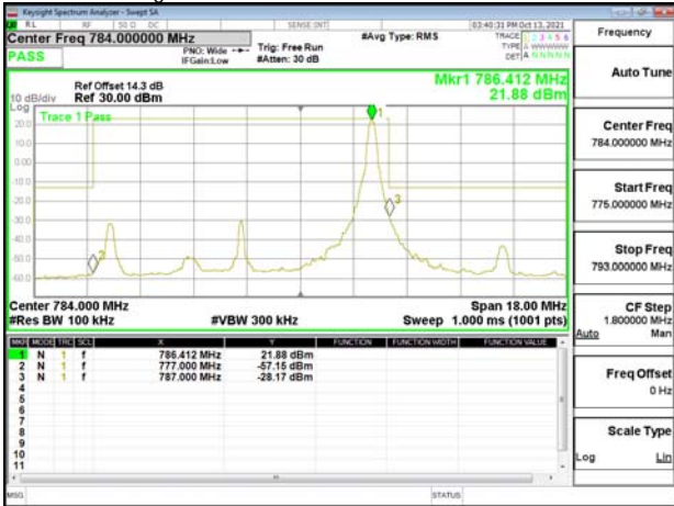
Band Edge_Band13_10MHz_OPSK_RB50_0_CH23230
