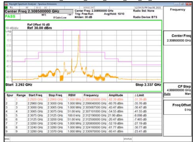
Emission Mask_Band30_5MHz_OPSK_RB1_24_CH27735
