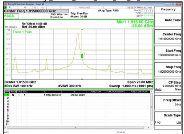
Band Edge_Band25_10MHz_OPSK_RB1_49_CH26640
