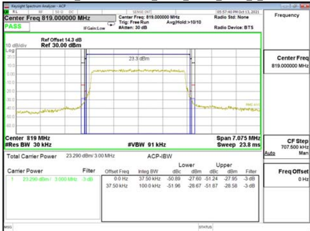
Emission Mask_Band26-Part90s_3MHz_OPSK_RB15_0_CH26740
