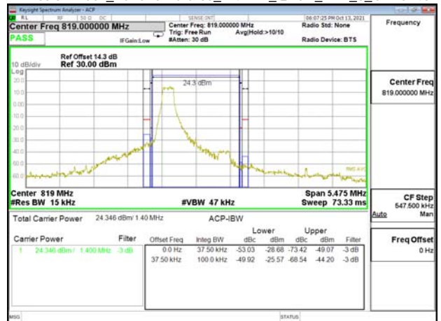
Emission Mask_Band26-Part90s_1.4MHz_QPSK_RB1_0_CH26740
