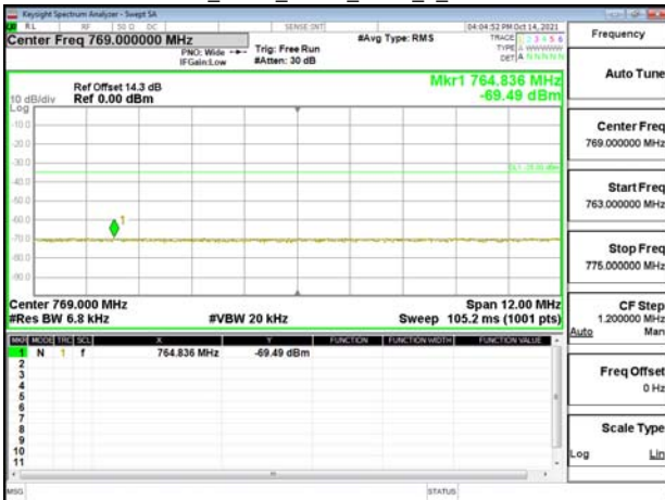
Band13_5MHz_QPSK_RB1_0_CH23205
