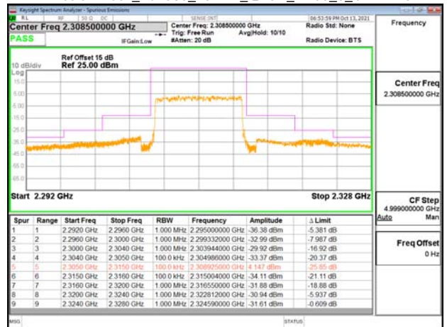
Emission Mask_Band30_10MHz_OPSK_RB50_0_CH27710
