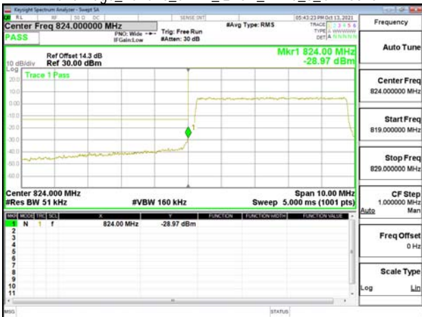
Band Edge_Band26_5MHz_OPSK_RB25_0_CH26815
