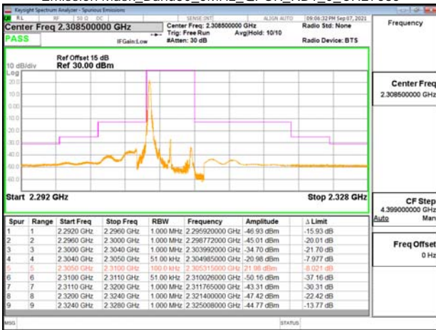
Emission Mask_Band30_5MHz_OPSK_RB1_0_CH27710
