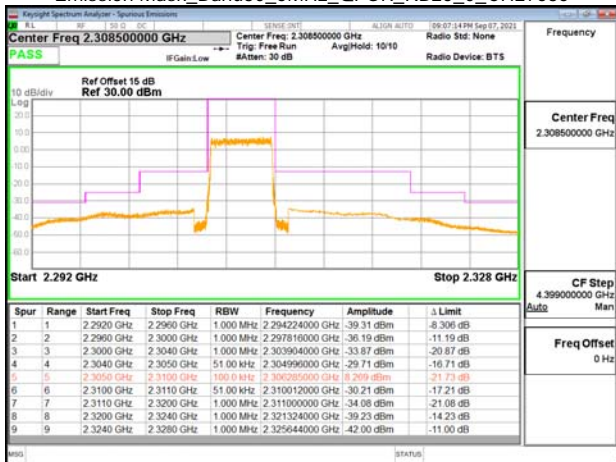
Emission Mask_Band30_5MHz_OPSK_RB25_0_CH27710
