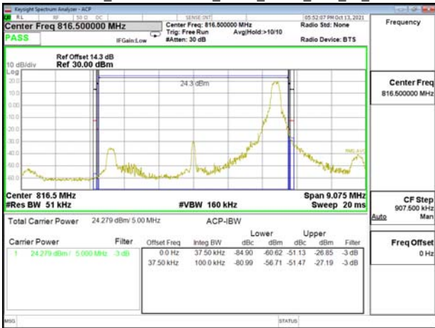
Emission Mask_Band26-Part90s_5MHz_QPSK_RB1_24_CH26740
