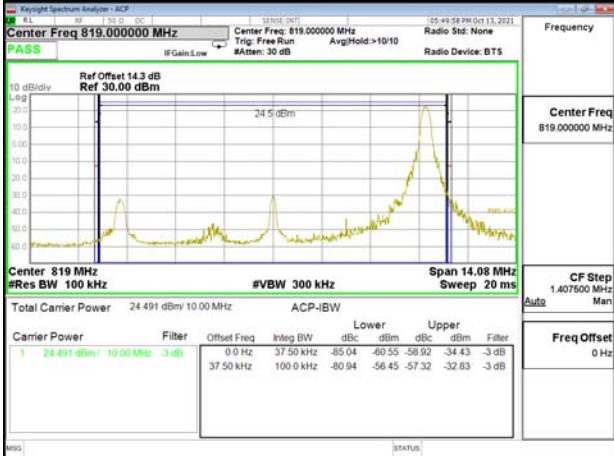
Emission Mask_Band26-Part90s_10MHz_QPSK_RB1_49_CH26740
