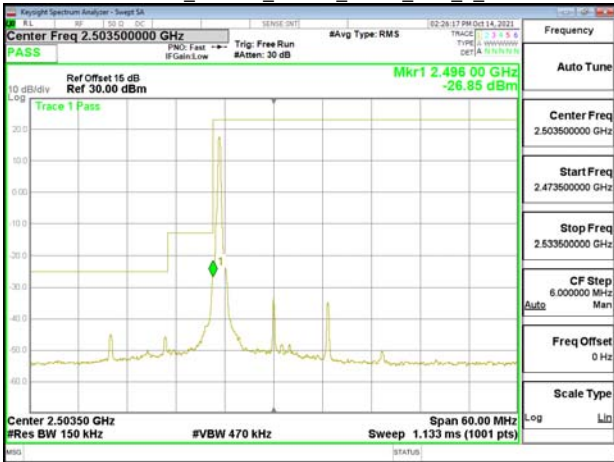
Emission Mask_Band41_15MHz_QPSK_RB1_74_CH41515
