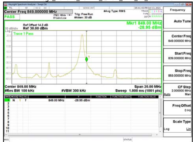
Band Edge_Band26_10MHz_OPSK_RB1_49_CH26990
