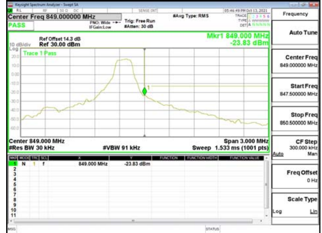
Band Edge_Band26_1.4MHz_QPSK_RB1_5_CH27033
