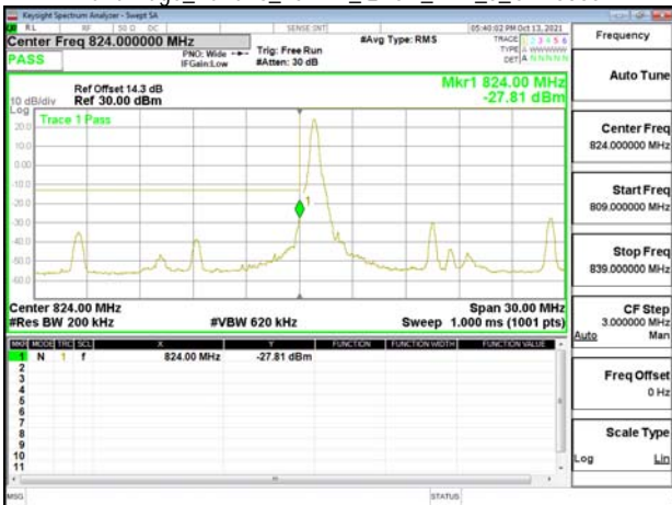
Band Edge_Band26_15MHz_OPSK_RB1_0_CH26865
