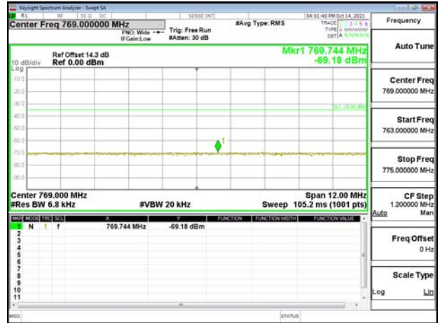
Band13_10MHz_OPSK_RB50_0_CH23230
