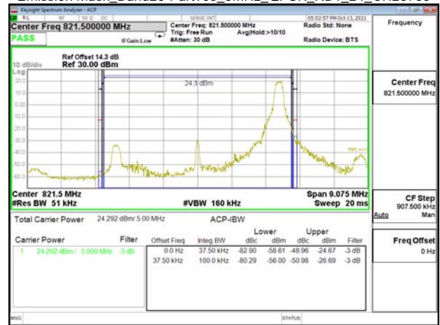
Emission Mask_Band26-Part90s_5MHz_QPSK_RB25_0_CH26715
