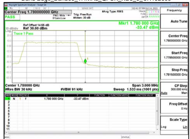
Band Edge_Band66_1.4MHz_OPSK_RB6_0_CH132665
