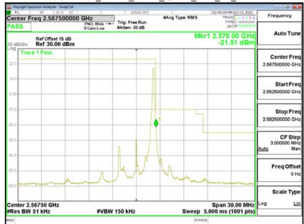
Emission Mask_Band7_5MHz_OPSK_RB1_24_CH21425
