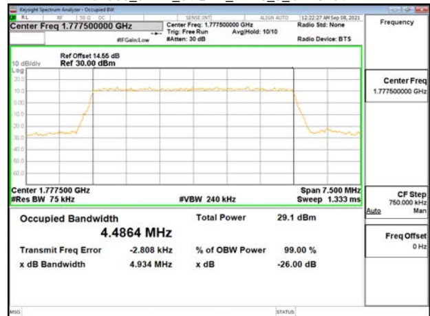
Band66_5MHz_64QAM_RB25_0_CH132647
