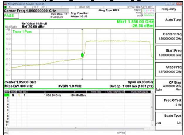
Band Edge_Band2_20MHz_OPSK_RB100_0_CH19100
