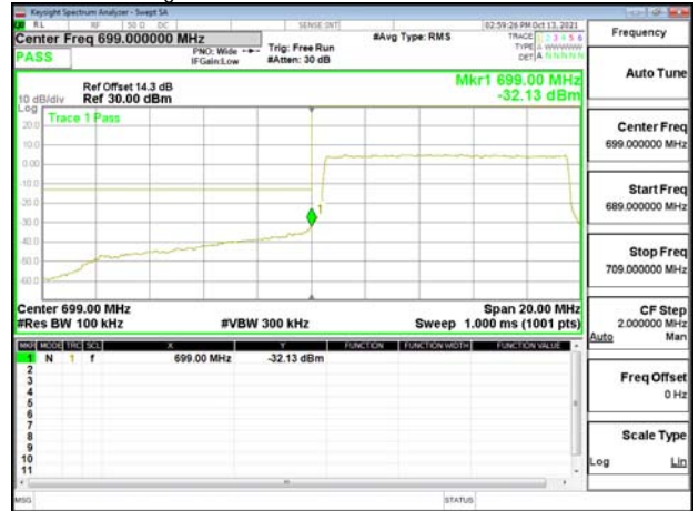
Band Edge_Band12_10MHz_OPSK_RB50_0_CH23130
