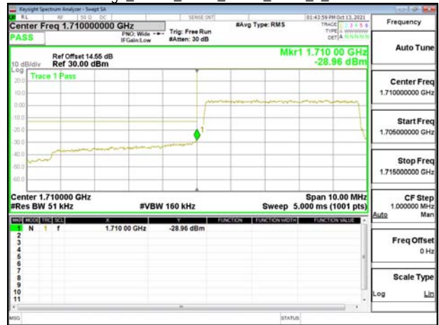
Band Edge_Band4_5MHz_QPSK_RB25_0_CH20375
