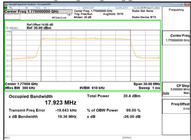
Band66_20MHz_16QAM_RB100_0_CH132572
