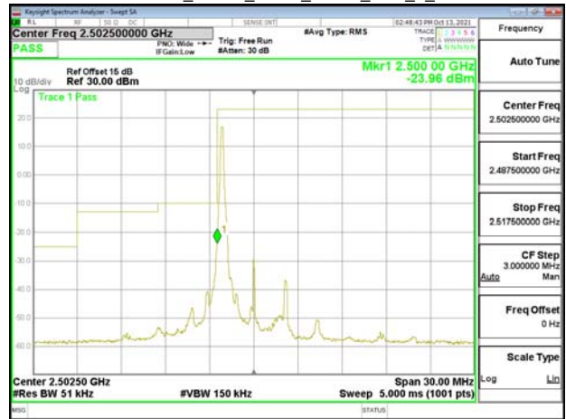
Emission Mask_Band7_5MHz_OPSK_RB1_24_CH21425
