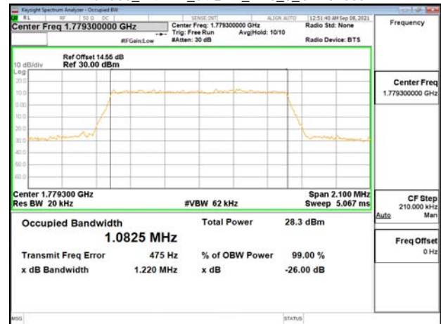
Band66_1.4MHz_64QAM_RB6_0_CH132665
