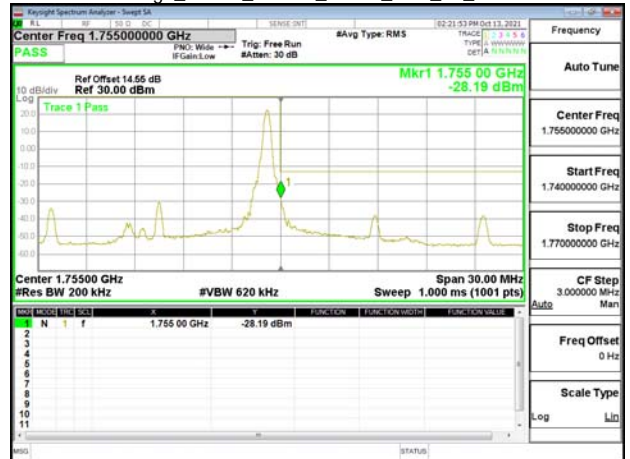
Band Edge_Band4_15MHz_OPSK_RB1_74_CH20325
