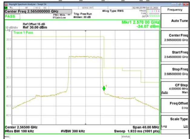
Emission Mask_Band7_10MHz_QPSK_RB50_0_CH21400
