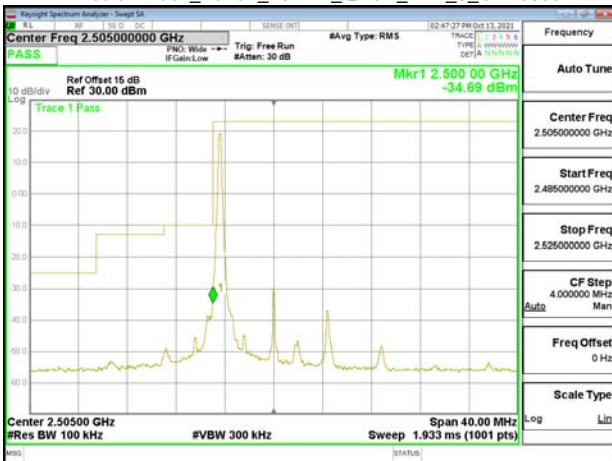
Emission Mask_Band7_10MHz_QPSK_RB1_0_CH20800
