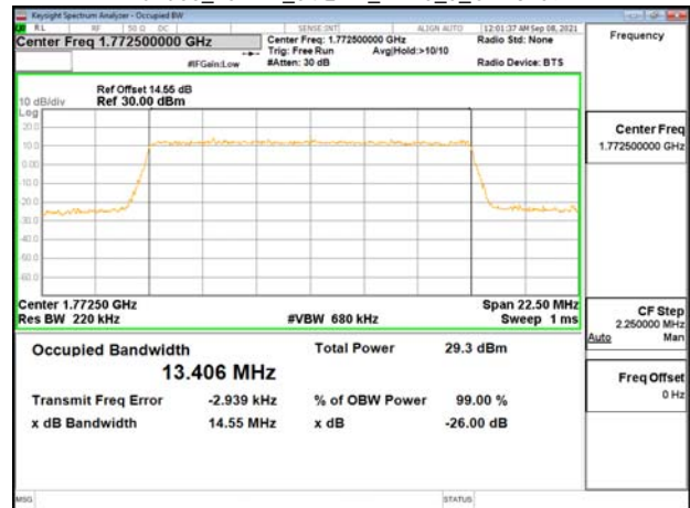
Band66_15MHz_64QAM_RB75_0_CH132597
