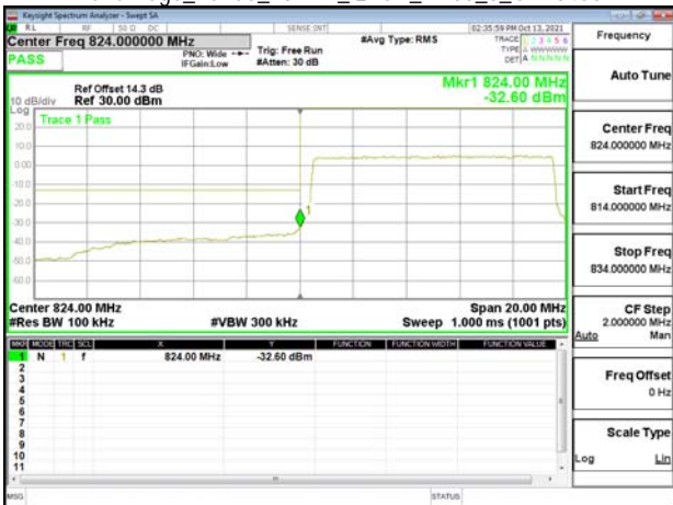
Band Edge_Band5_10MHz_OPSK_RB50_0_CH20450
