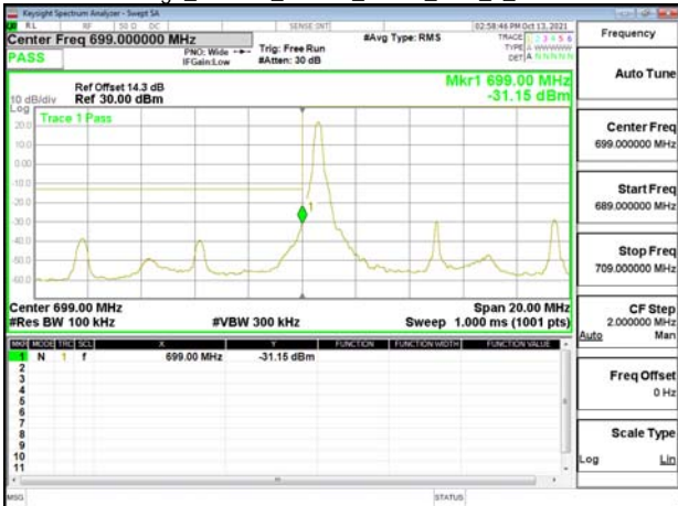
Band Edge_Band12_10MHz_OPSK_RB1_0_CH23060
