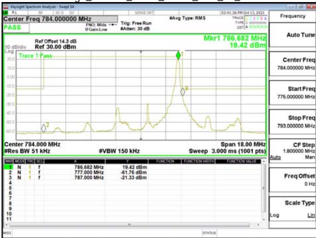
Band Edge_Band13_5MHz_OPSK_RB25_0_CH23205
