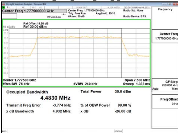
Band66_5MHz_16QAM_RB25_0_CH132647
