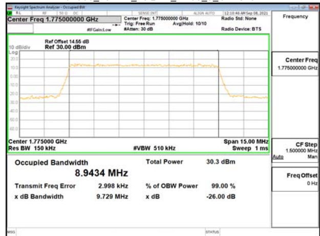
Band66_10MHz_16QAM_RB50_0_CH132622
