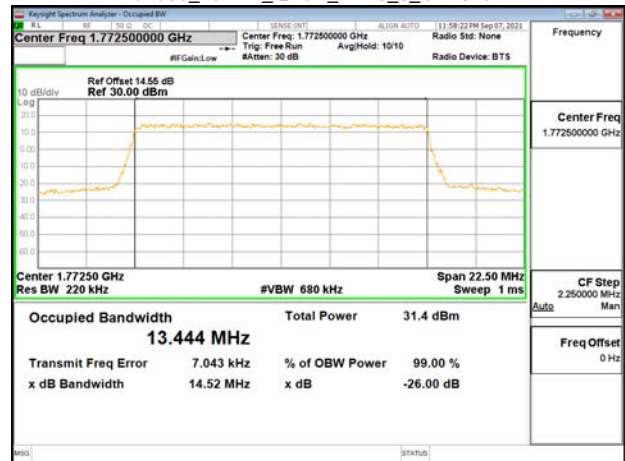
Band66_15MHz_QPSK_RB75_0_CH132597
