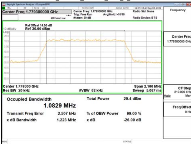
Band66_1.4MHz_16QAM_RB6_0_CH132665
