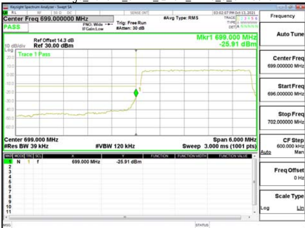
Band Edge_Band12_3MHz_OPSK_RB15_0_CH23025
