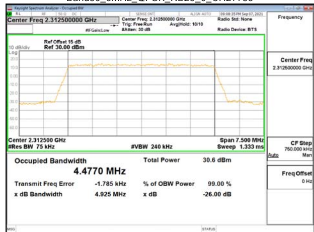
Band30_5MHz_QPSK_RB25_0_CH27735
