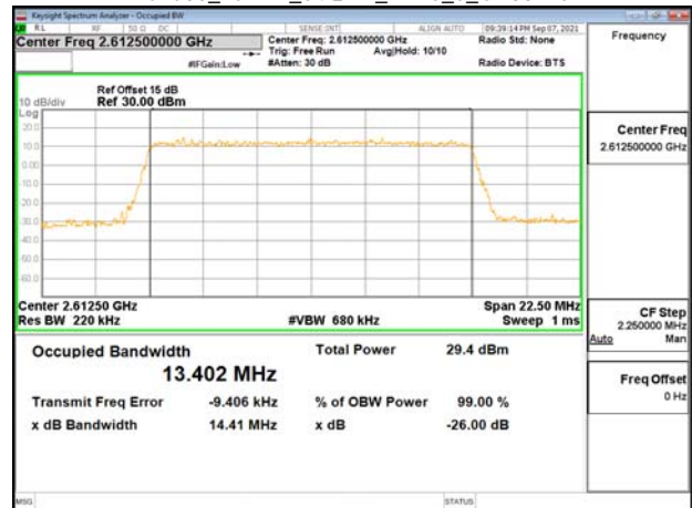
Band38_15MHz_64QAM_RB75_0_CH38175
