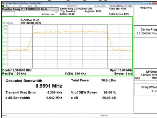
Band30_10MHz_16QAM_RB50_0_CH27710
