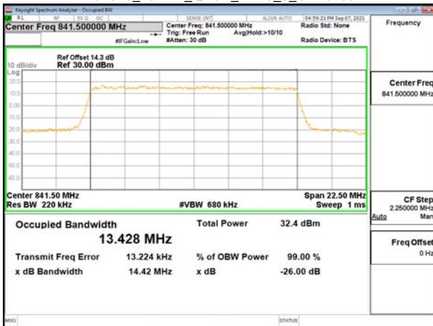
Band26_15MHz_QPSK_RB75_0_CH26965
