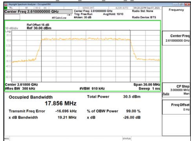
Band38_20MHz_16QAM_RB100_0_CH38150
