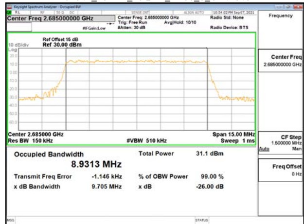
Band41_10MHz_16QAM_RB50_0_CH41540
