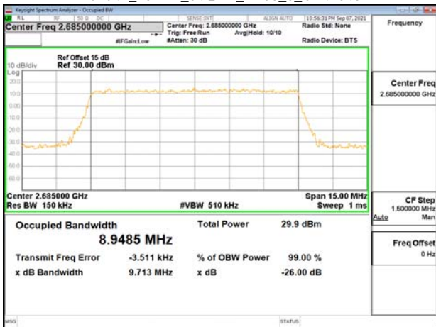
Band41_10MHz_64QAM_RB50_0_CH41540
