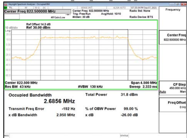
Band26-Part90s_3MHz_QPSK_RB15_0_CH26775
