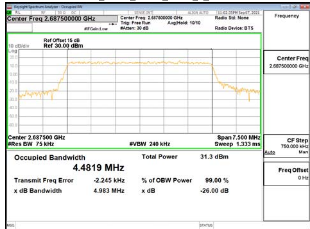
Band41_5MHz_QPSK_RB25_0_CH41565
