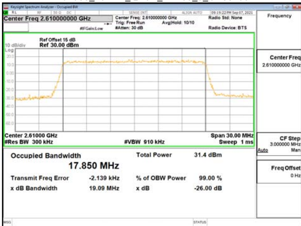
Band38_20MHz_QPSK_RB100_0_CH38150
