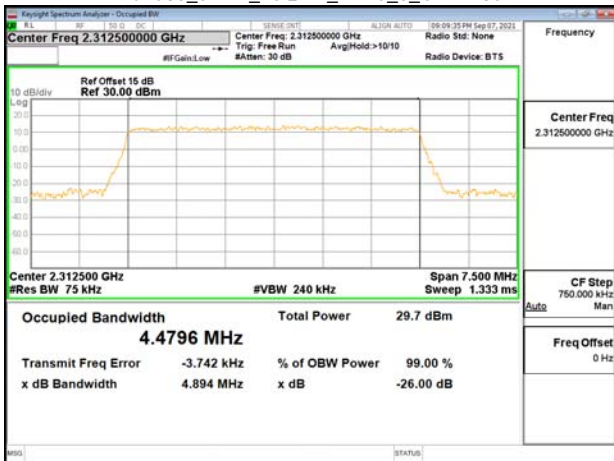
Band30_5MHz_16QAM_RB25_0_CH27735
