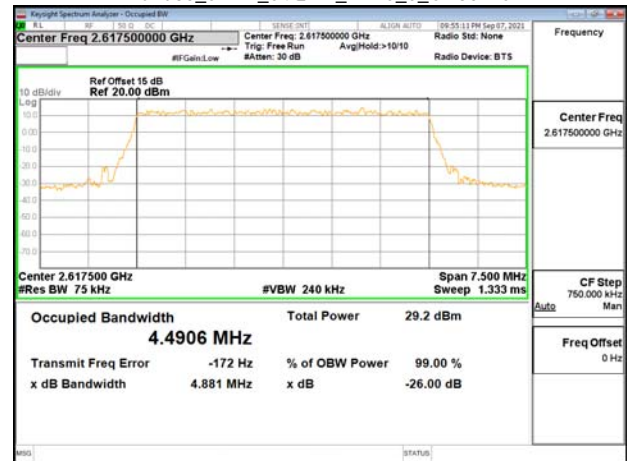
Band38_5MHz_64QAM_RB25_0_CH38225
