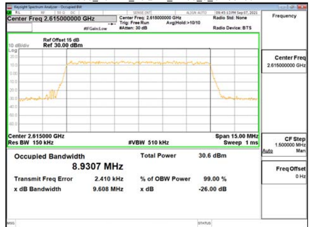
Band38_10MHz_16QAM_RB50_0_CH38200
