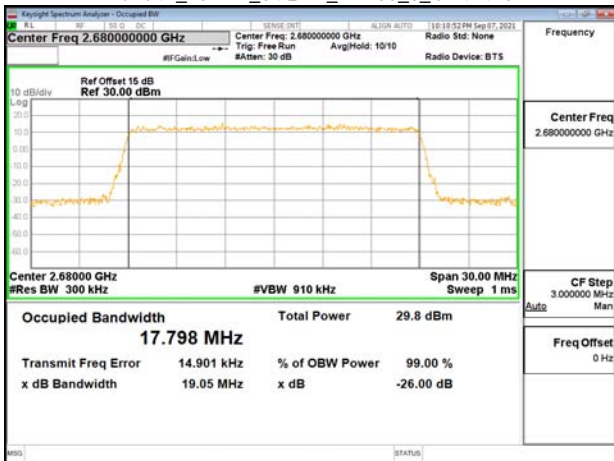
Band41_20MHz_64QAM_RB100_0_CH41490
