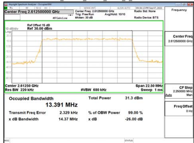
Band38_15MHz_QPSK_RB75_0_CH38175
