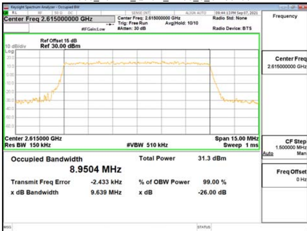
Band38_10MHz_QPSK_RB50_0_CH38200
