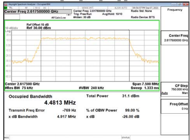
Band38_5MHz_OPSK_RB25_0_CH38225
