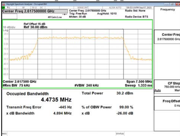
Band38_5MHz_16QAM_RB25_0_CH38225
