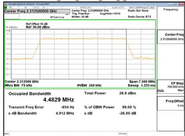
Band30_5MHz_64QAM_RB25_0_CH27735
