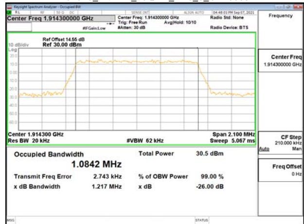
Band25_1.4MHz_16QAM_RB6_0_CH26683
