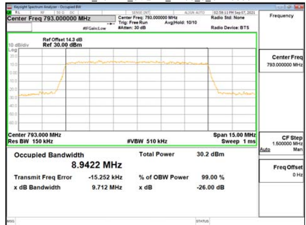
Band14_10MHz_64QAM_RB50_0_CH23330
