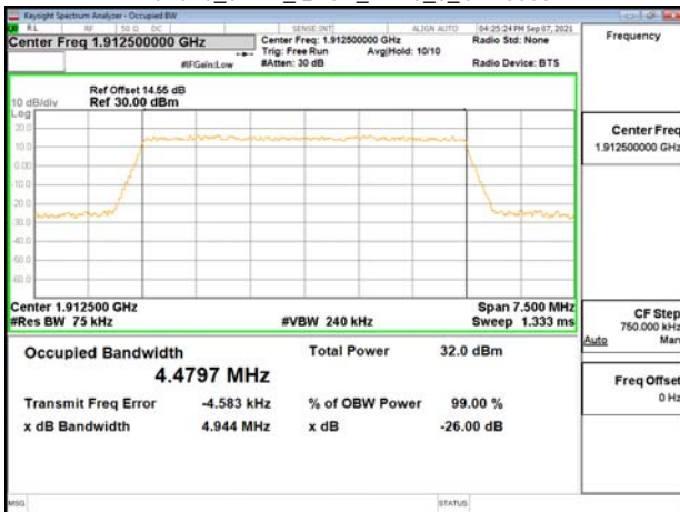
Band25_5MHz_QPSK_RB25_0_CH26665
