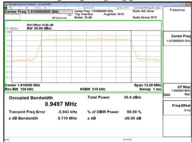
Band25_10MHz_64QAM_RB50_0_CH26640
