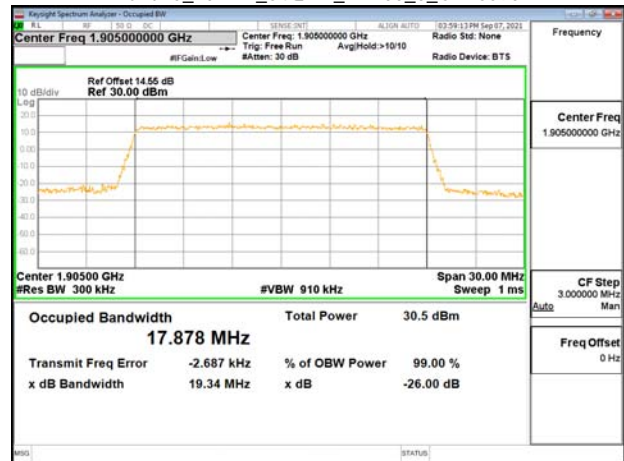
Band25_20MHz_64QAM_RB100_0_CH26590
