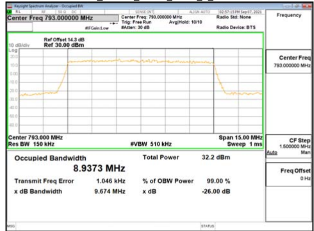
Band14_10MHz_16QAM_RB50_0_CH23330
