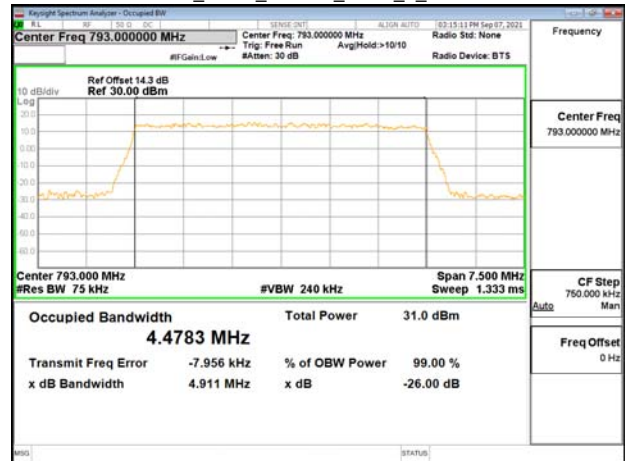
Band14_5MHz_16QAM_RB25_0_CH23355
