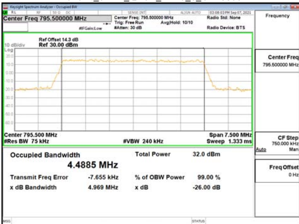
Band14_5MHz_QPSK_RB25_0_CH23355
