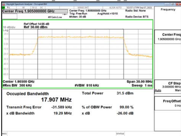
Band25_20MHz_16QAM_RB100_0_CH26590
