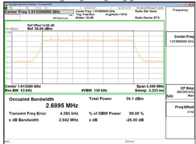
Band25_3MHz_64QAM_RB15_0_CH26675
