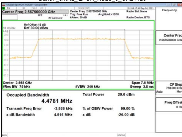
Band7_5MHz_QPSK_RB25_0_CH21425
