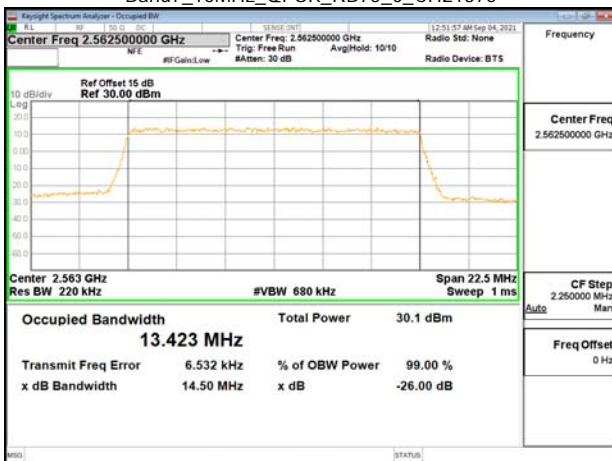
Band7_15MHz_QPSK_RB75_0_CH21375
