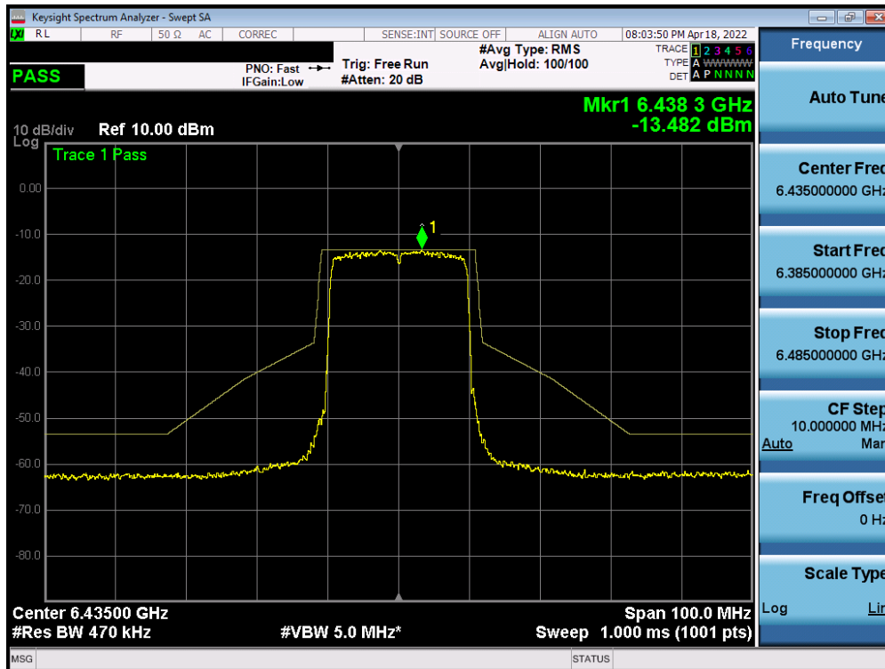
Plot 7-539. In-Band Emission Plot Measurement MIMO ANT1 (20MHz 802.11ax (UNII Band 6) – Ch. 97)
