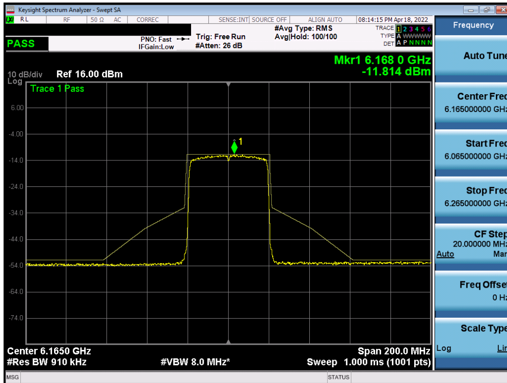
Plot 7-528. In-Band Emission Plot Measurement MIMO ANT1 (40MHz 802.11ax (UNII Band 5) – Ch. 43)
