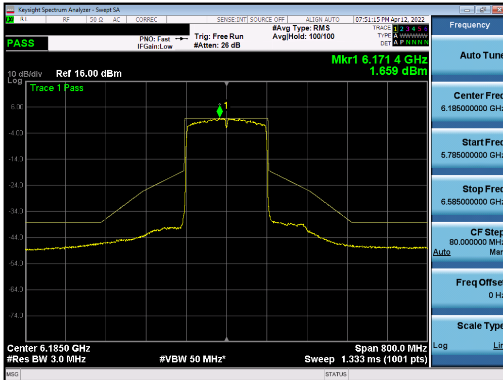
Plot 7-482. In-Band Emission Plot Measurement SISO ANT2 (160MHz 802.11ax (UNII Band 5) – Ch. 47)
