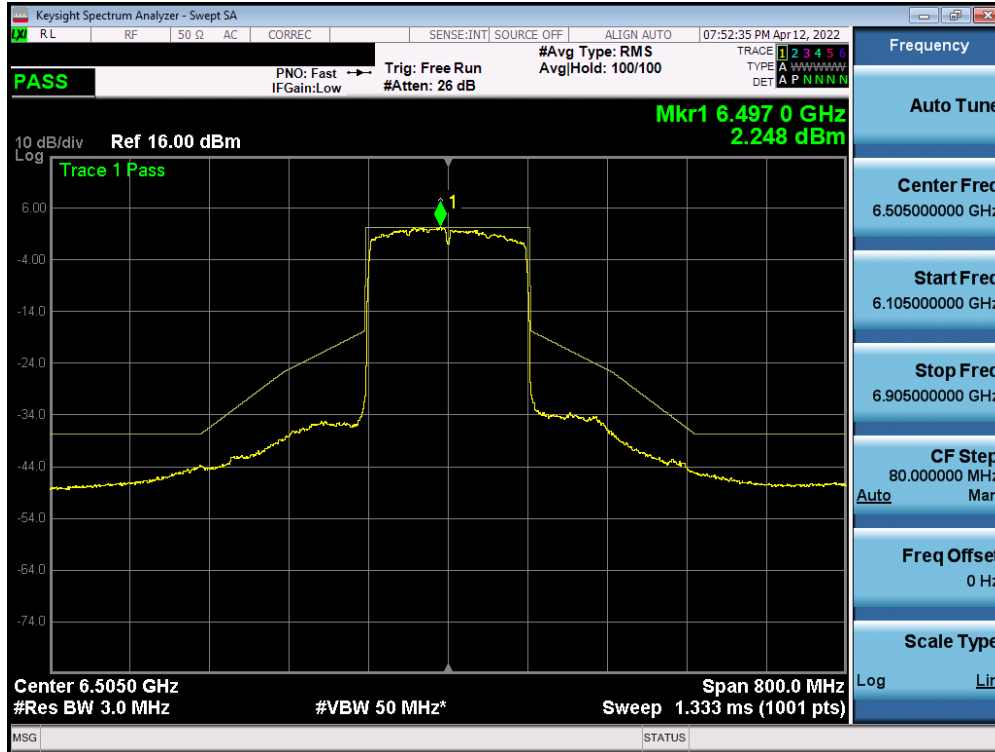
Plot 7-494. In-Band Emission Plot Measurement SISO ANT2 (160MHz 802.11ax (UNII Band 6) – Ch. 111)
