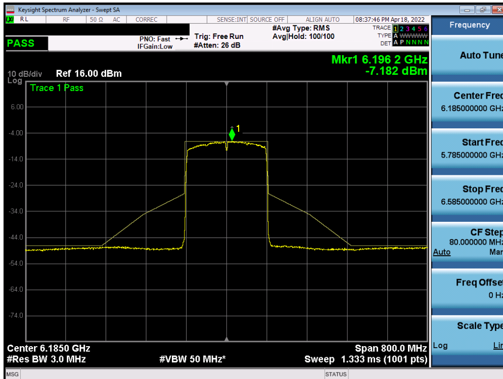
Plot 7-534. In-Band Emission Plot Measurement MIMO ANT1 (160MHz 802.11ax (UNII Band 5) – Ch. 47)
