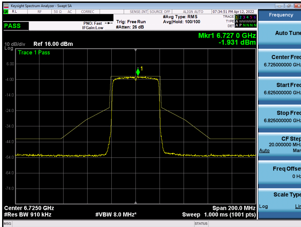
Plot 7-502. In-Band Emission Plot Measurement SISO ANT2 (40MHz 802.11ax (UNII Band 7) – Ch. 155)
