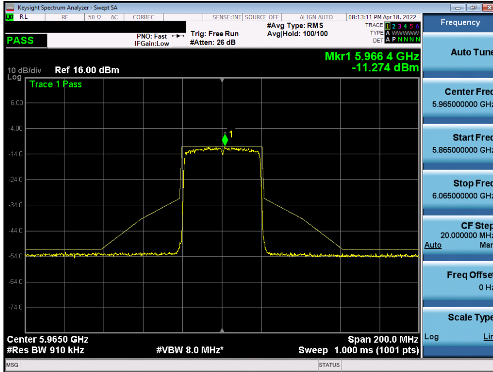
Plot 7-527. In-Band Emission Plot Measurement MIMO ANT1 (40MHz 802.11ax (UNII Band 5) – Ch. 3)
