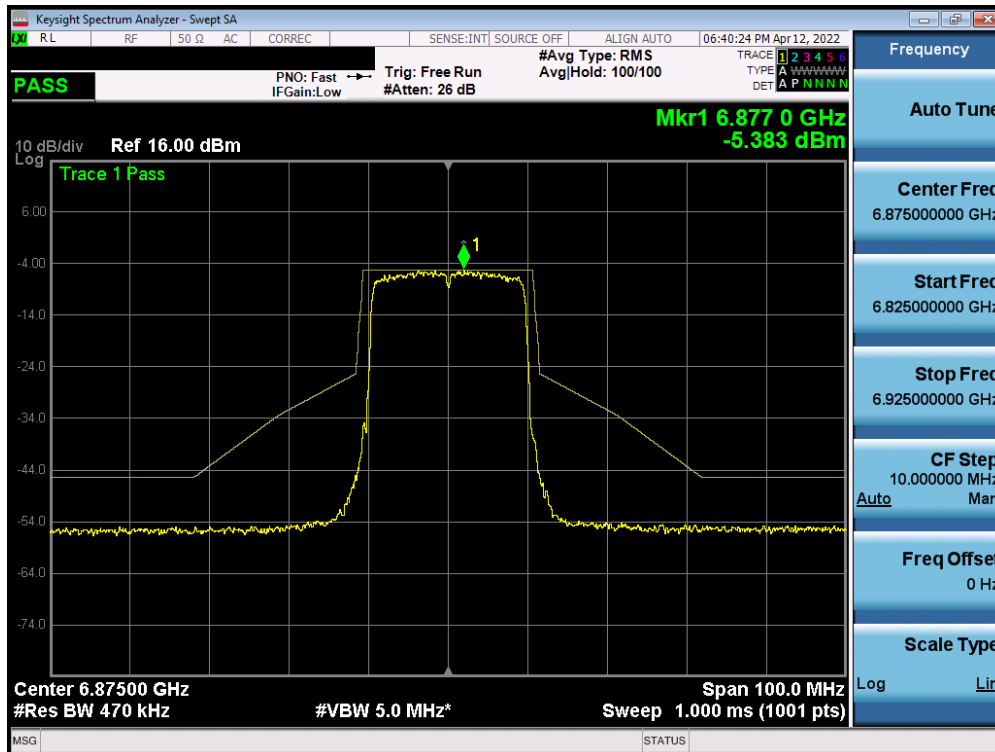
Plot 7-500. In-Band Emission Plot Measurement SISO ANT2 (20MHz 802.11ax (UNII Band 7) – Ch. 185)
