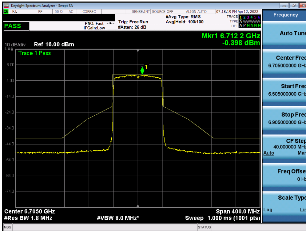
Plot 7-453. In-Band Emission Plot Measurement SISO ANT1 (80MHz 802.11ax (UNII Band 7) – Ch. 151)
