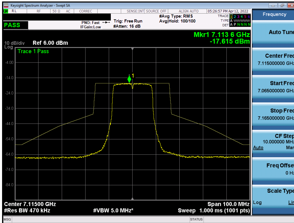
Plot 7-459. In-Band Emission Plot Measurement SISO ANT1 (20MHz 802.11a (UNII Band 8) – Ch. 233)
