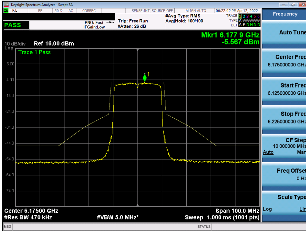
Plot 7-473. In-Band Emission Plot Measurement SISO ANT2 (20MHz 802.11ax (UNII Band 5) – Ch. 45)
