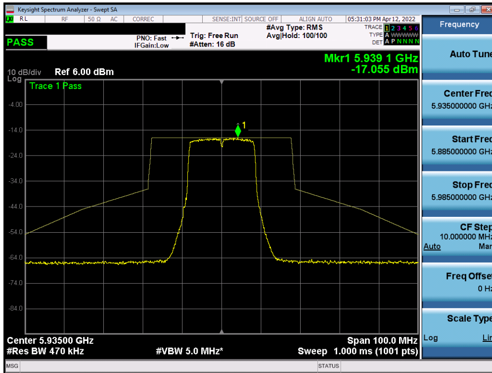
Plot 7-469. In-Band Emission Plot Measurement SISO ANT2 (20MHz 802.11a (UNII Band 5) – Ch. 2)
