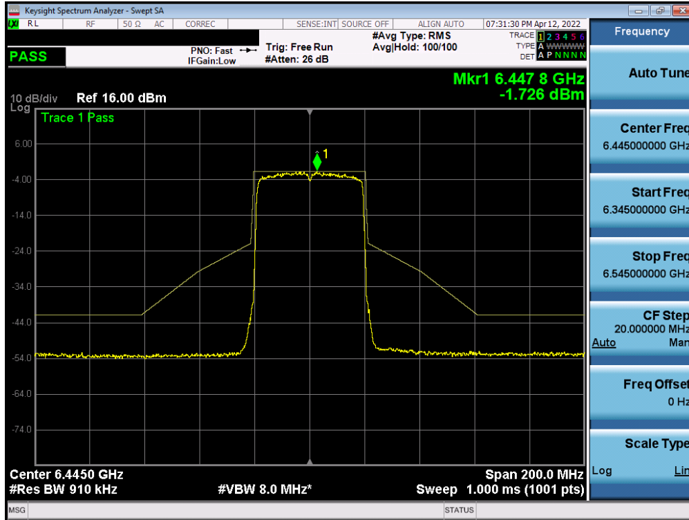
Plot 7-490. In-Band Emission Plot Measurement SISO ANT2 (40MHz 802.11ax (UNII Band 6) – Ch. 99)
