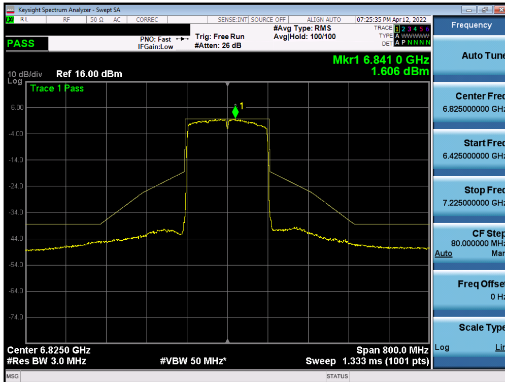
Plot 7-456. In-Band Emission Plot Measurement SISO ANT1 (160MHz 802.11ax (UNII Band 7) – Ch. 175)
