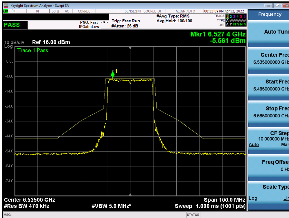
Plot 7-498. In-Band Emission Plot Measurement SISO ANT2 (20MHz 802.11ax (UNII Band 7) – Ch. 117)
