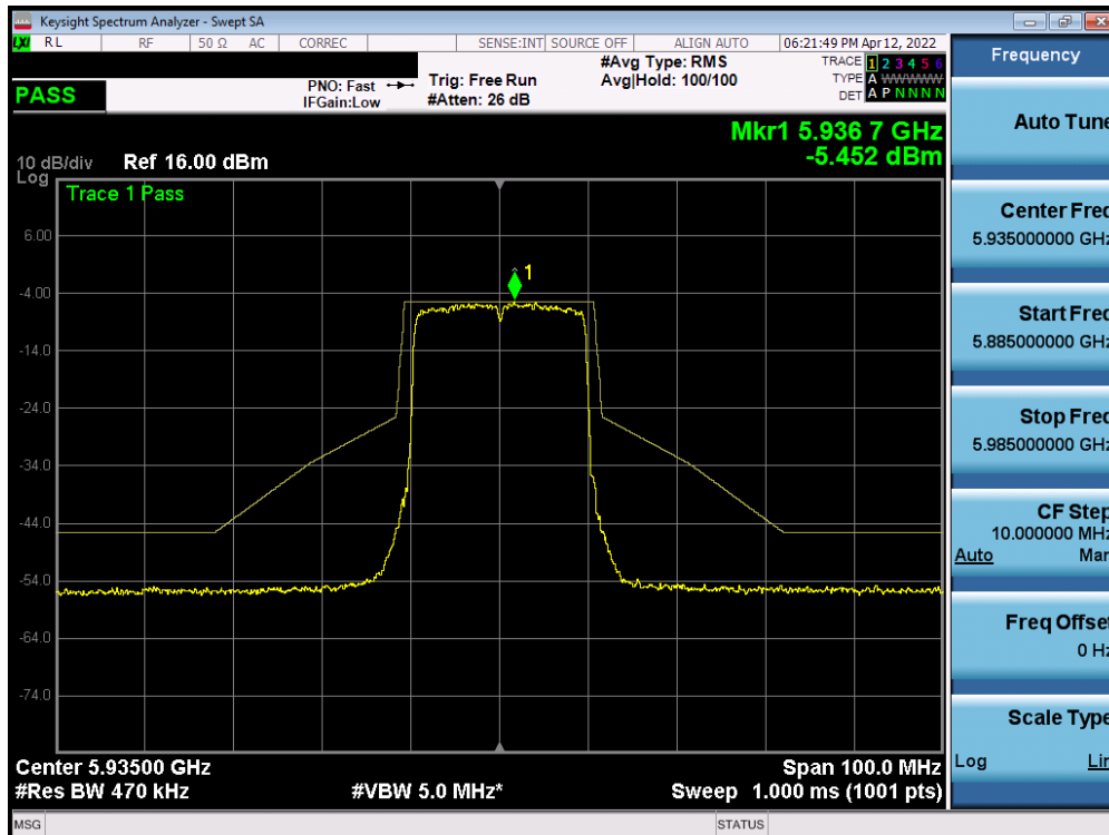
Plot 7-472. In-Band Emission Plot Measurement SISO ANT2 (20MHz 802.11ax (UNII Band 5) – Ch. 2)
