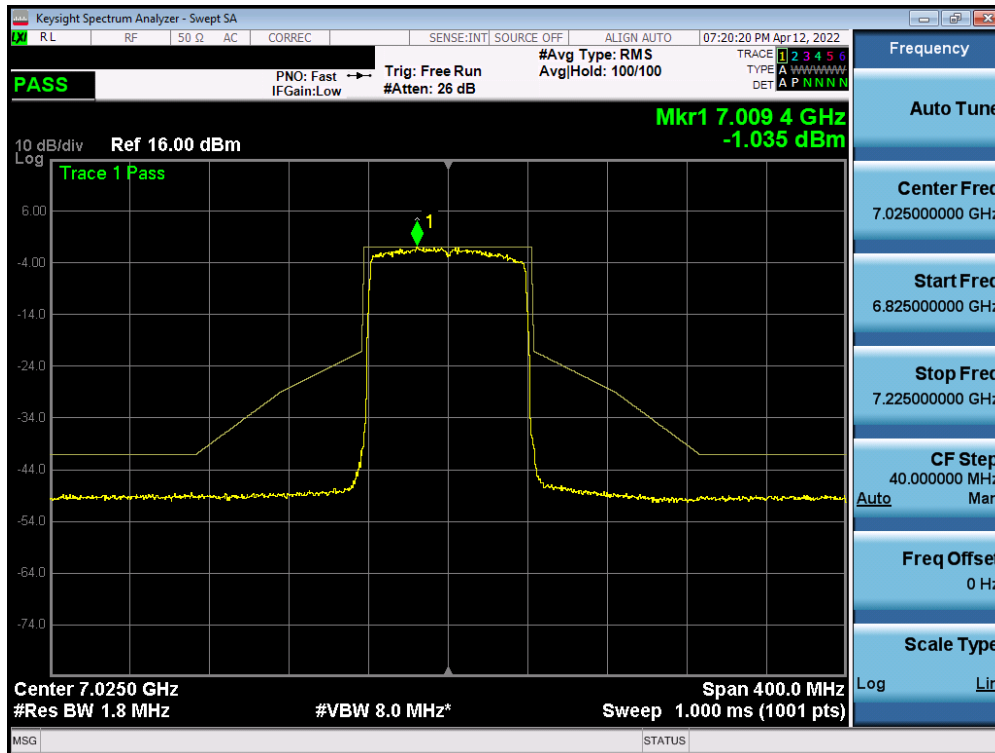
Plot 7-467. In-Band Emission Plot Measurement SISO ANT1 (80MHz 802.11ax (UNII Band 8) – Ch. 215)
