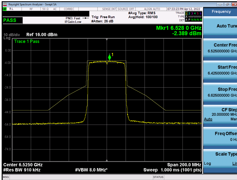
Plot 7-492. In-Band Emission Plot Measurement SISO ANT2 (40MHz 802.11ax (UNII Band 6) – Ch. 115)
