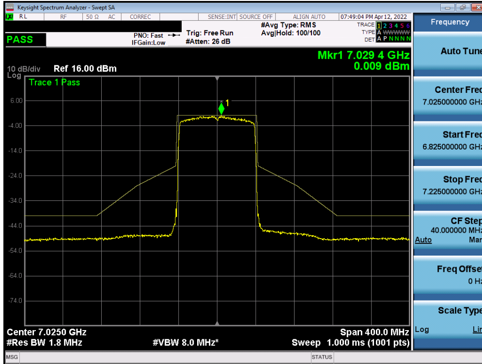
Plot 7-519. In-Band Emission Plot Measurement SISO ANT2 (80MHz 802.11ax (UNII Band 8) – Ch. 215)
