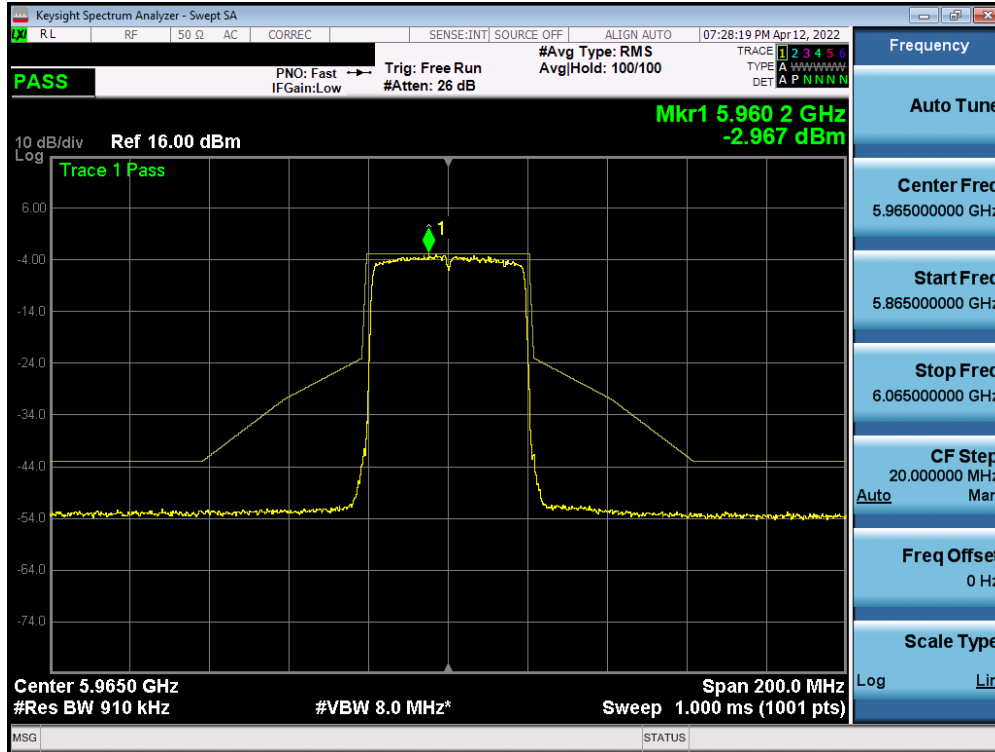
Plot 7-475. In-Band Emission Plot Measurement SISO ANT2 (40MHz 802.11ax (UNII Band 5) – Ch. 3)
