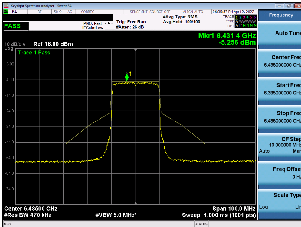
Plot 7-487. In-Band Emission Plot Measurement SISO ANT2 (20MHz 802.11ax (UNII Band 6) – Ch. 97)
