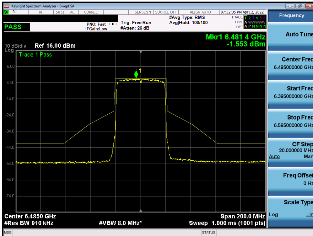
Plot 7-491. In-Band Emission Plot Measurement SISO ANT2 (40MHz 802.11ax (UNII Band 6) – Ch. 107)
