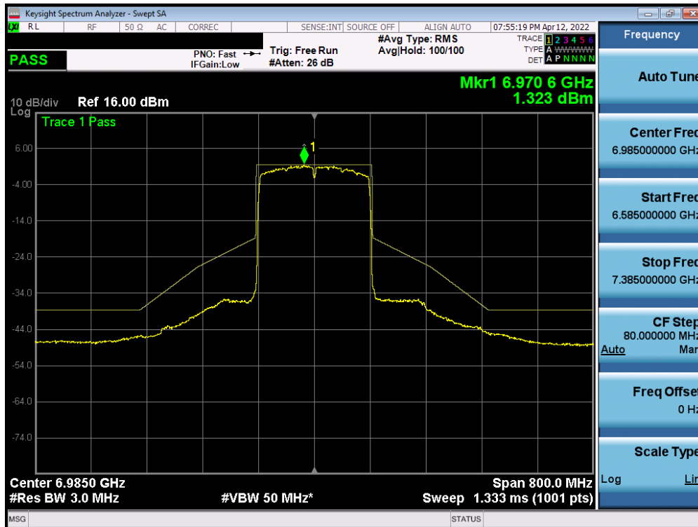
Plot 7-520. In-Band Emission Plot Measurement SISO ANT2 (160MHz 802.11ax (UNII Band 8) – Ch. 207)
