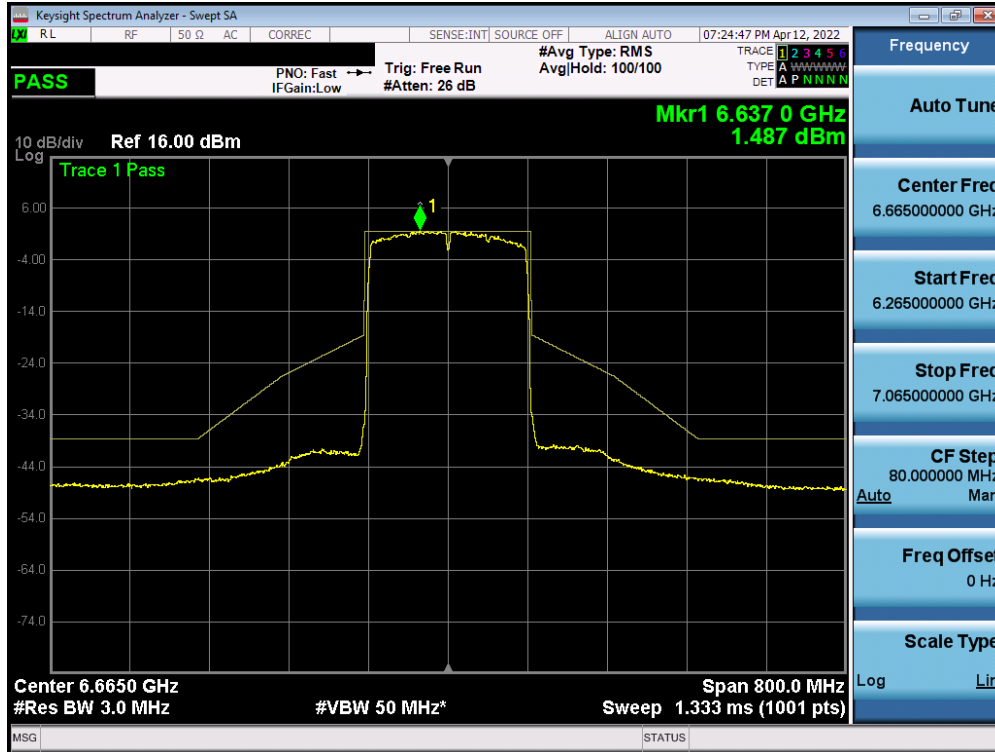
Plot 7-455. In-Band Emission Plot Measurement SISO ANT1 (160MHz 802.11ax (UNII Band 7) – Ch. 143)
