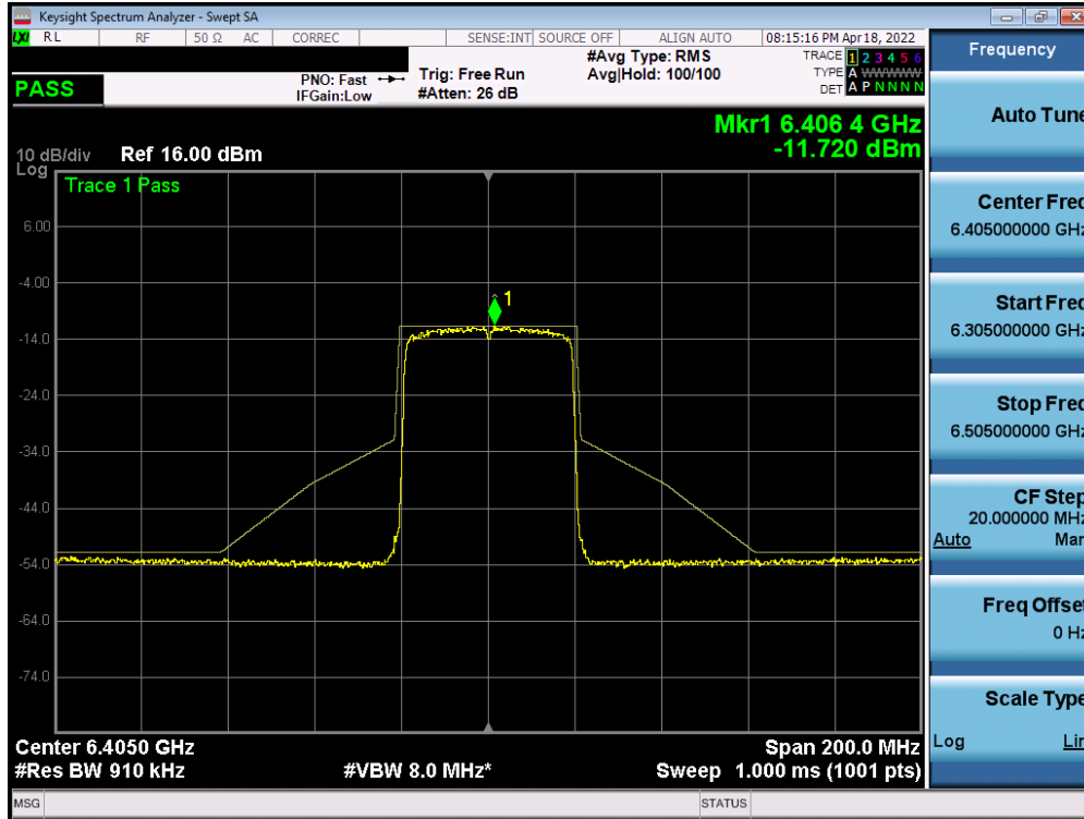
Plot 7-529. In-Band Emission Plot Measurement MIMO ANT1 (40MHz 802.11ax (UNII Band 5) – Ch. 91)
