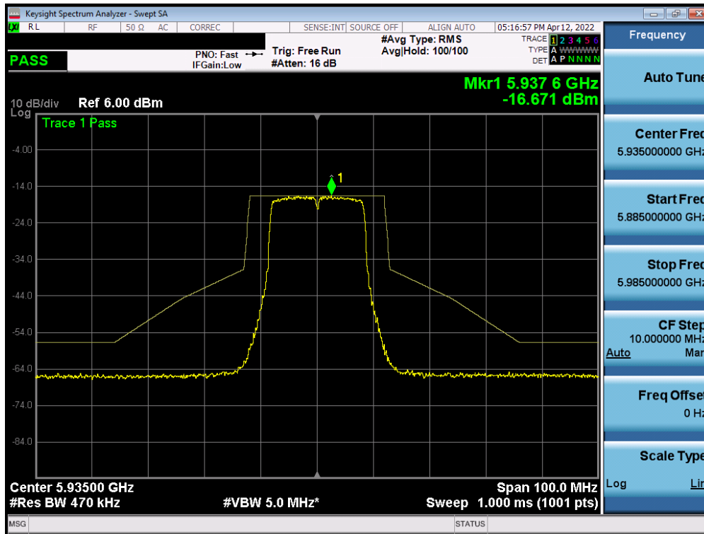
Plot 7-521. In-Band Emission Plot Measurement MIMO ANT1 (20MHz 802.11a (UNII Band 5) – Ch. 2)
