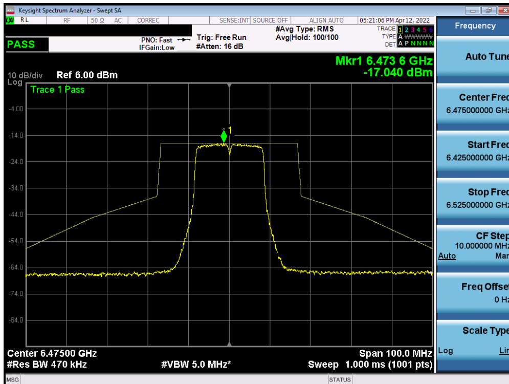
Plot 7-537. In-Band Emission Plot Measurement MIMO ANT1 (20MHz 802.11a (UNII Band 6) – Ch. 105)
