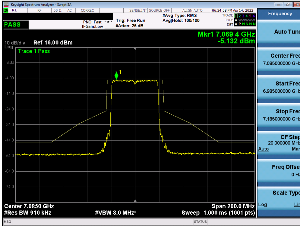
Plot 7-517. In-Band Emission Plot Measurement SISO ANT2 (40MHz 802.11ax (UNII Band 8) – Ch. 227)
