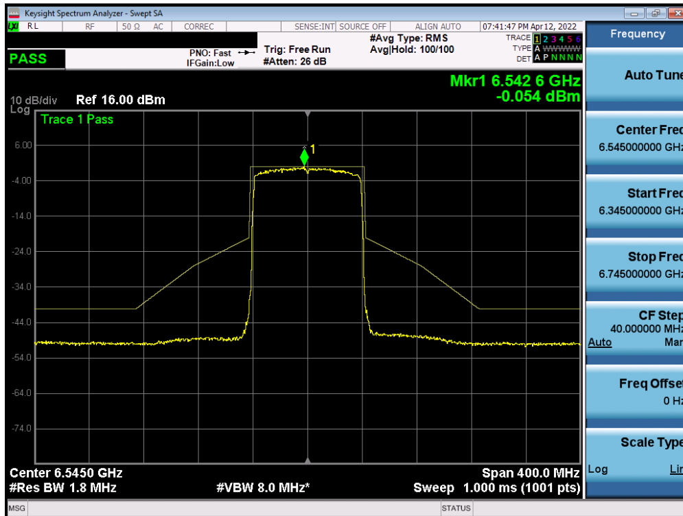
Plot 7-504. In-Band Emission Plot Measurement SISO ANT2 (80MHz 802.11ax (UNII Band 7) – Ch. 119)
