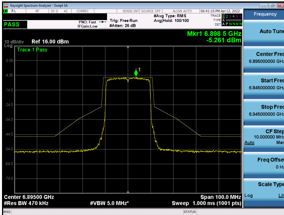
Plot 7-512. In-Band Emission Plot Measurement SISO ANT2 (20MHz 802.11ax (UNII Band 8) – Ch. 189)
