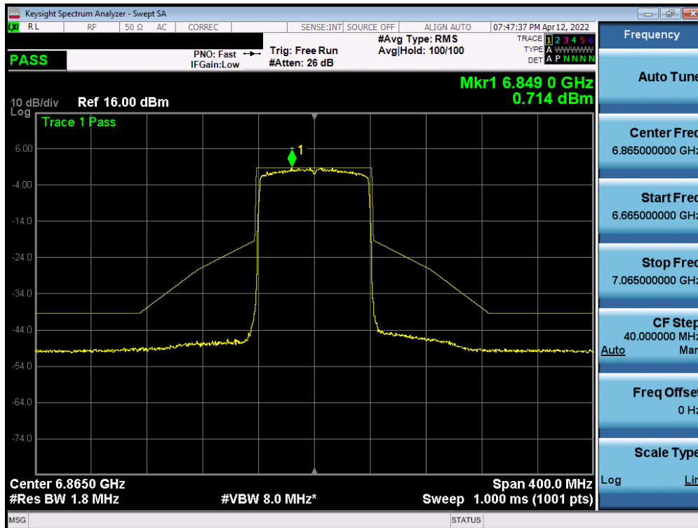
Plot 7-506. In-Band Emission Plot Measurement SISO ANT2 (80MHz 802.11ax (UNII Band 7) – Ch. 183)
