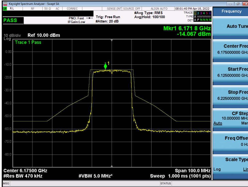
Plot 7-525. In-Band Emission Plot Measurement MIMO ANT1 (20MHz 802.11ax (UNII Band 5) – Ch. 45)
