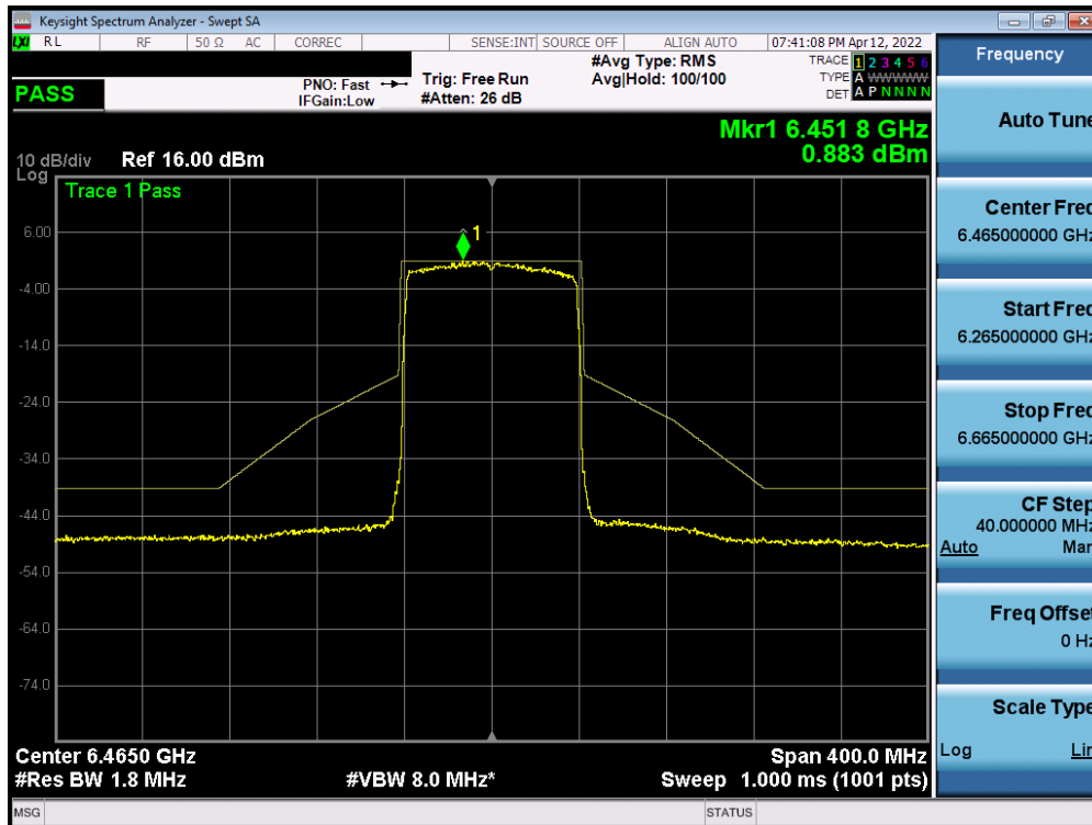
Plot 7-493. In-Band Emission Plot Measurement SISO ANT2 (80MHz 802.11ax (UNII Band 6) – Ch. 103)
