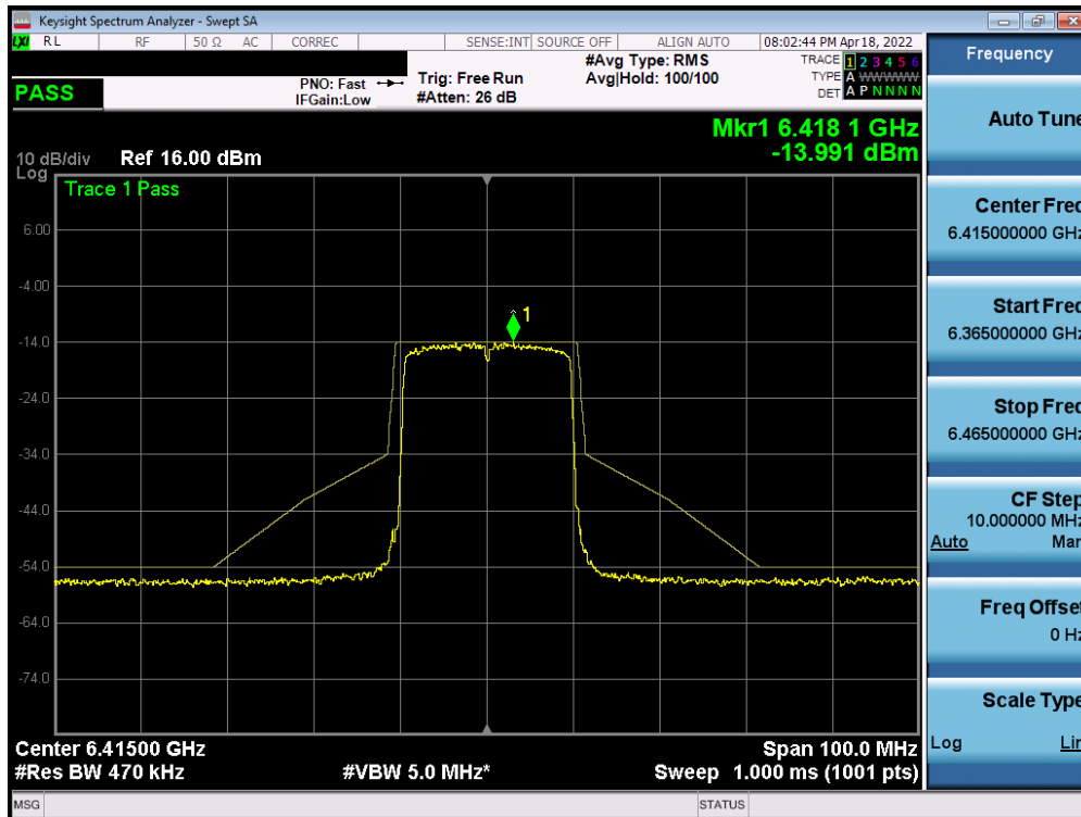
Plot 7-526. In-Band Emission Plot Measurement MIMO ANT1 (20MHz 802.11ax (UNII Band 5) – Ch. 93)
