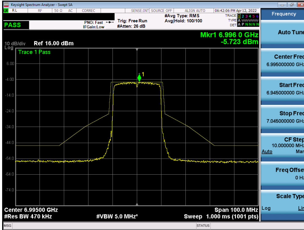
Plot 7-513. In-Band Emission Plot Measurement SISO ANT2 (20MHz 802.11ax (UNII Band 8) – Ch. 209)
