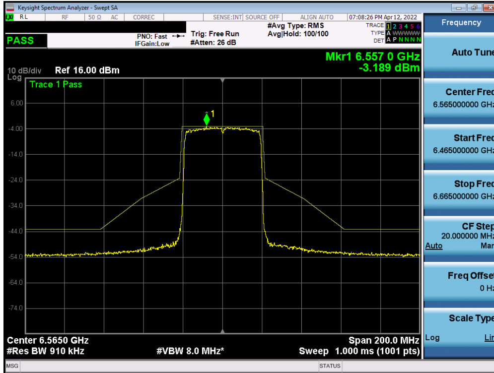
Plot 7-449. In-Band Emission Plot Measurement SISO ANT1 (40MHz 802.11ax (UNII Band 7) – Ch. 123)
