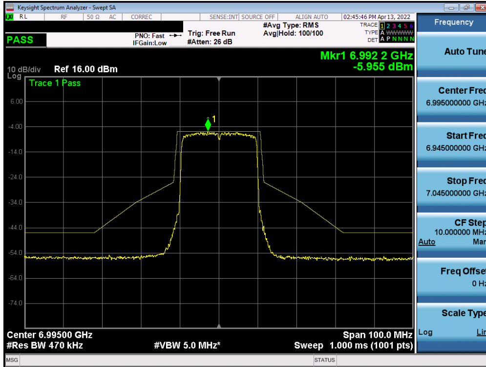
Plot 7-461. In-Band Emission Plot Measurement SISO ANT1 (20MHz 802.11ax (UNII Band 8) – Ch. 209)
