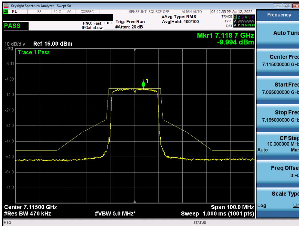
Plot 7-514. In-Band Emission Plot Measurement SISO ANT2 (20MHz 802.11ax (UNII Band 8) – Ch. 233)
