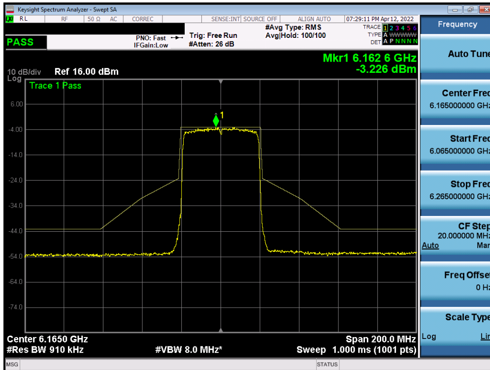
Plot 7-476. In-Band Emission Plot Measurement SISO ANT2 (40MHz 802.11ax (UNII Band 5) – Ch. 43)
