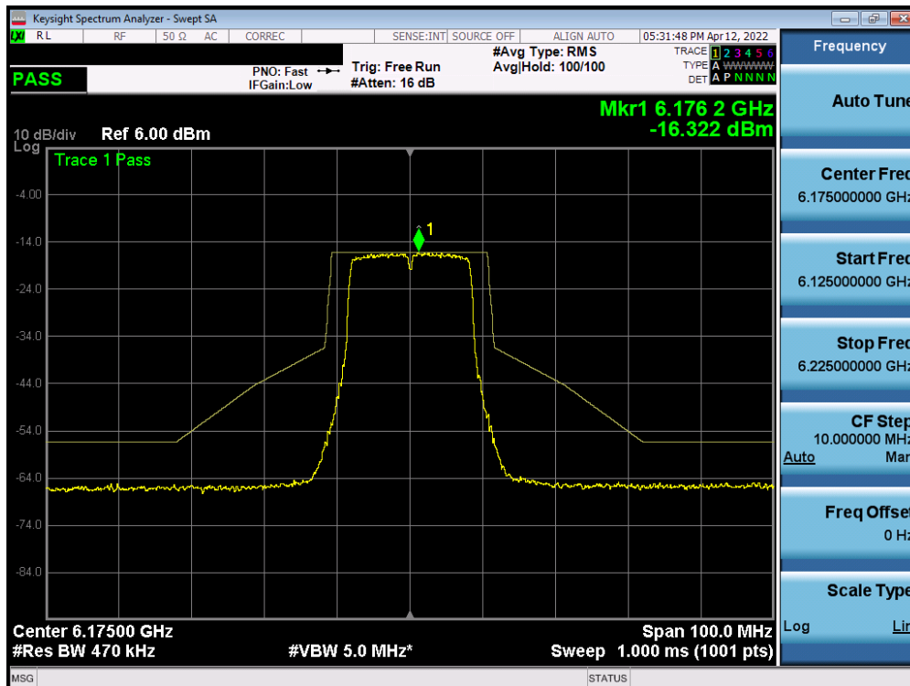
Plot 7-470. In-Band Emission Plot Measurement SISO ANT2 (20MHz 802.11a (UNII Band 5) – Ch. 45)
