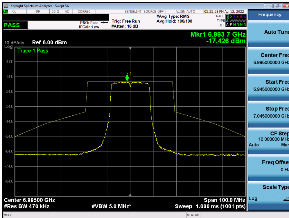
Plot 7-458. In-Band Emission Plot Measurement SISO ANT1 (20MHz 802.11a (UNII Band 8) – Ch. 209)
