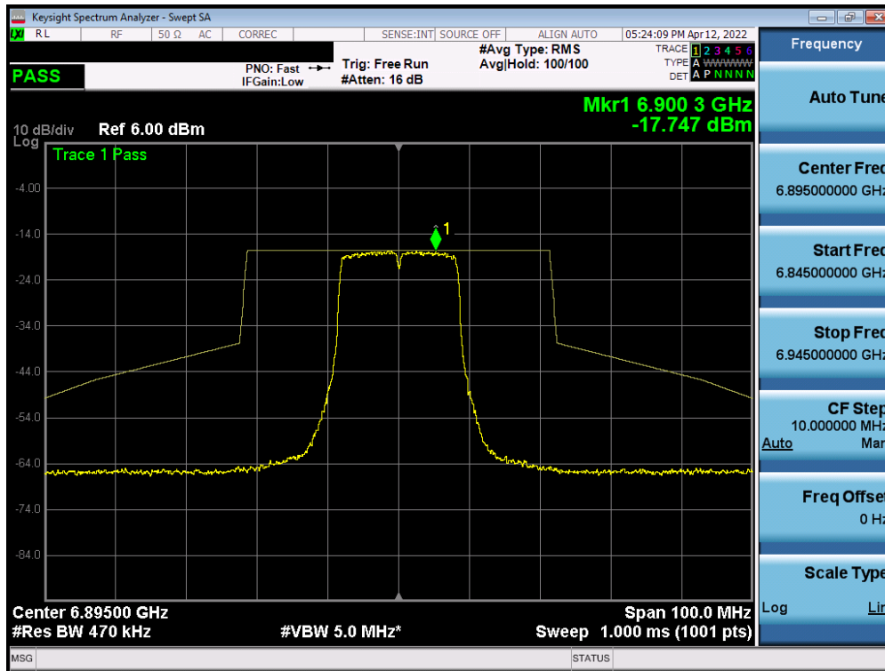
Plot 7-457. In-Band Emission Plot Measurement SISO ANT1 (20MHz 802.11a (UNII Band 8) – Ch. 189)
