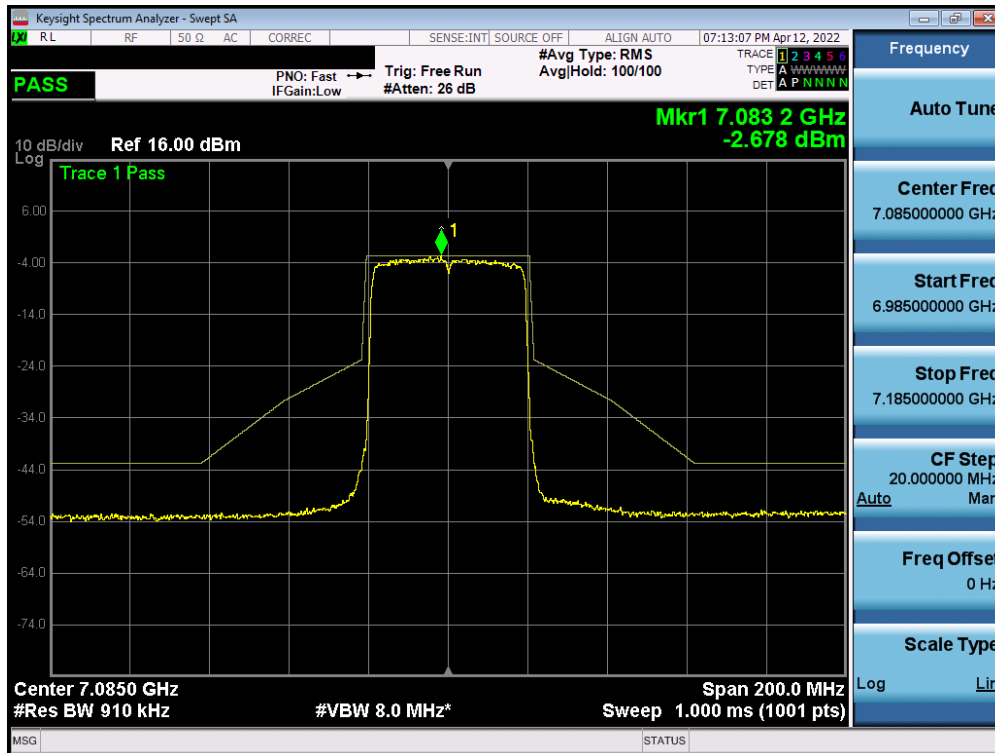
Plot 7-465. In-Band Emission Plot Measurement SISO ANT1 (40MHz 802.11ax (UNII Band 8) – Ch. 227)
