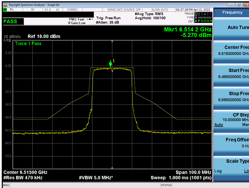
Plot 7-489. In-Band Emission Plot Measurement SISO ANT2 (20MHz 802.11ax (UNII Band 6) – Ch. 113)
