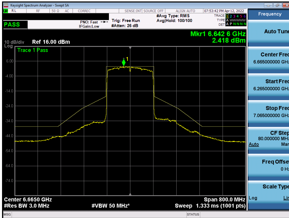
Plot 7-507. In-Band Emission Plot Measurement SISO ANT2 (160MHz 802.11ax (UNII Band 7) – Ch. 143)
