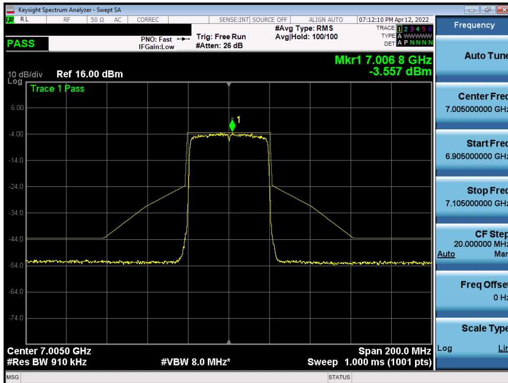
Plot 7-464. In-Band Emission Plot Measurement SISO ANT1 (40MHz 802.11ax (UNII Band 8) – Ch. 211)
