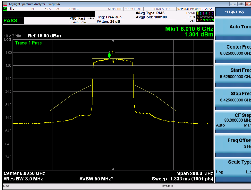
Plot 7-481. In-Band Emission Plot Measurement SISO ANT2 (160MHz 802.11ax (UNII Band 5) – Ch. 15)
