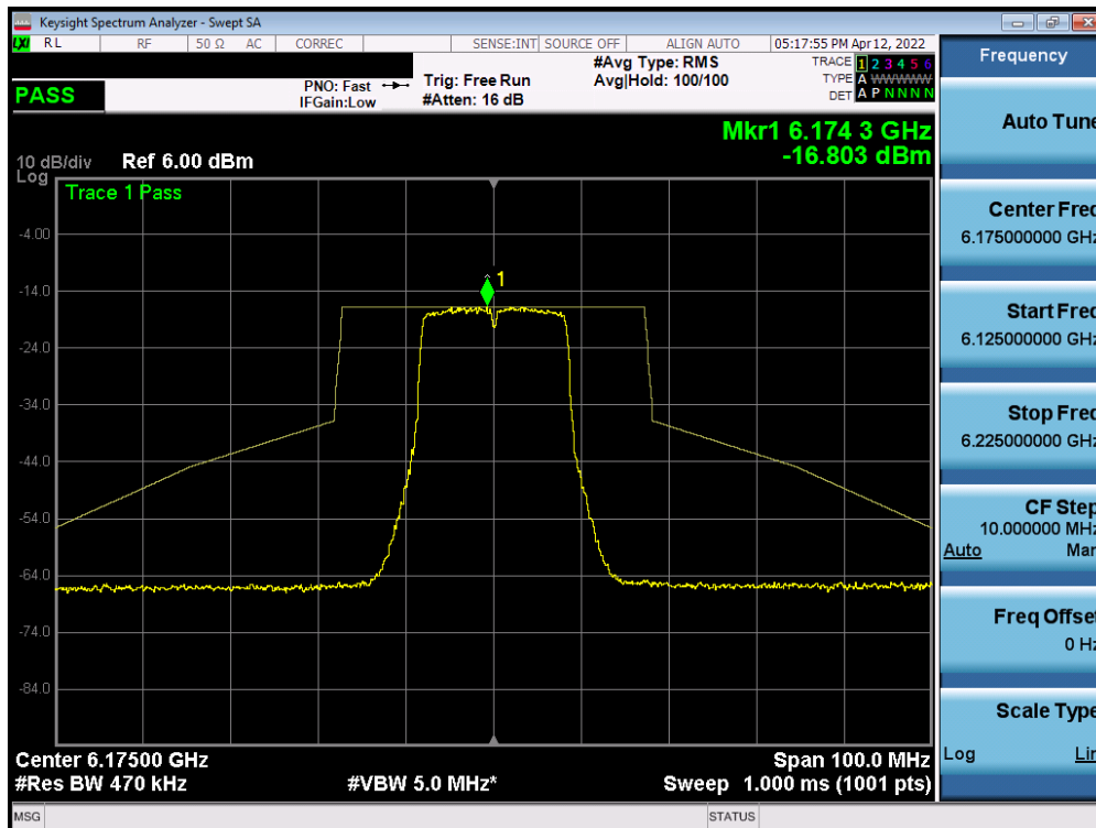
Plot 7-522. In-Band Emission Plot Measurement MIMO ANT1 (20MHz 802.11a (UNII Band 5) – Ch. 45)
