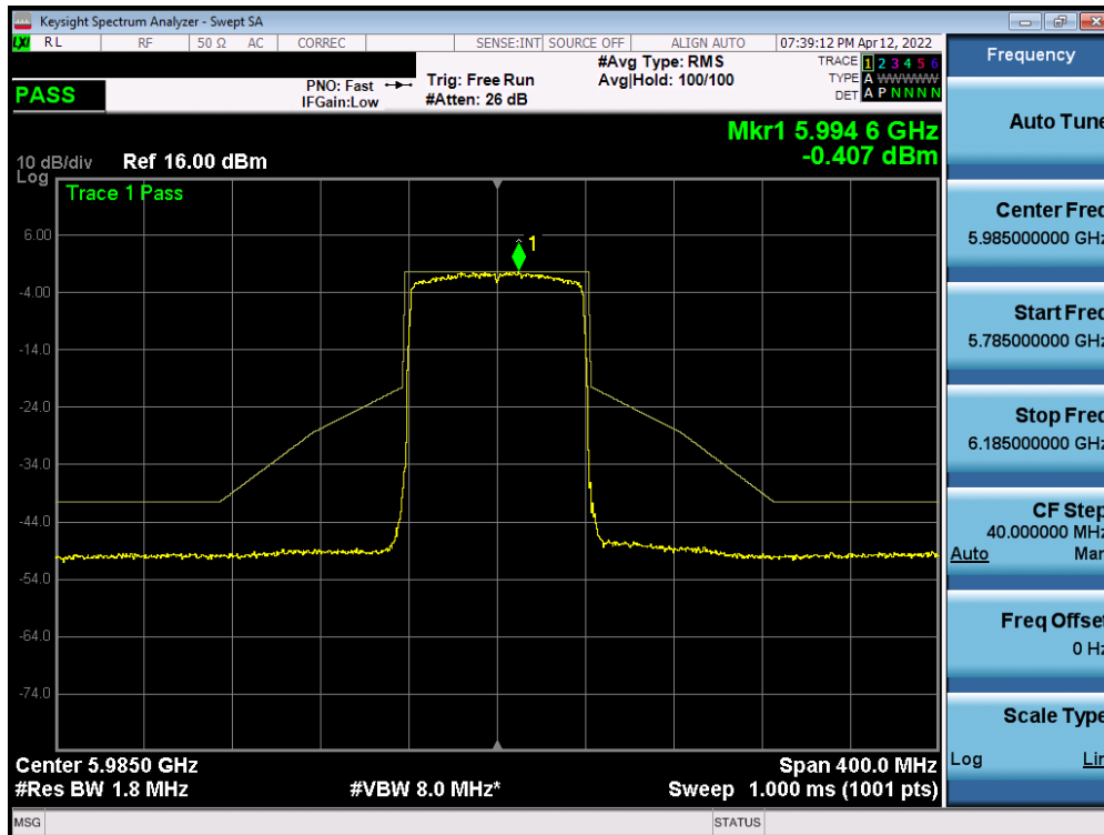
Plot 7-478. In-Band Emission Plot Measurement SISO ANT2 (80MHz 802.11ax (UNII Band 5) – Ch. 7)
