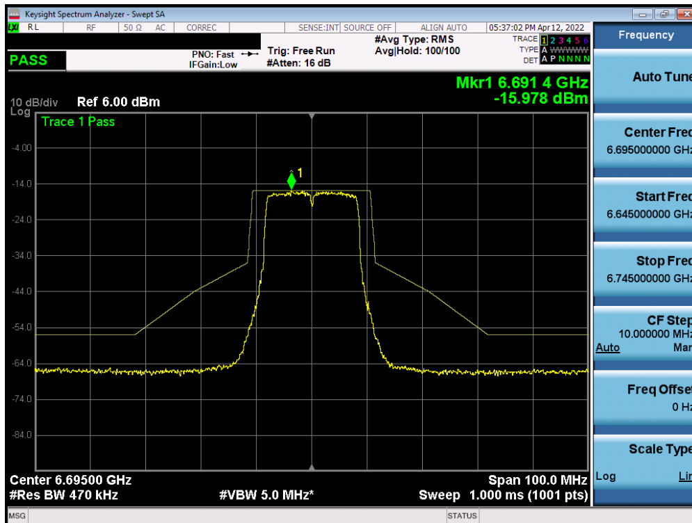
Plot 7-496. In-Band Emission Plot Measurement SISO ANT2 (20MHz 802.11a (UNII Band 7) – Ch. 149)
