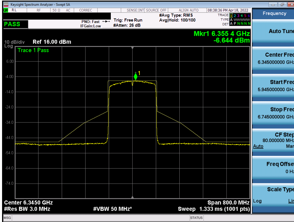
Plot 7-535. In-Band Emission Plot Measurement MIMO ANT1 (160MHz 802.11 ax (UNII Band 5) – Ch. 79)
