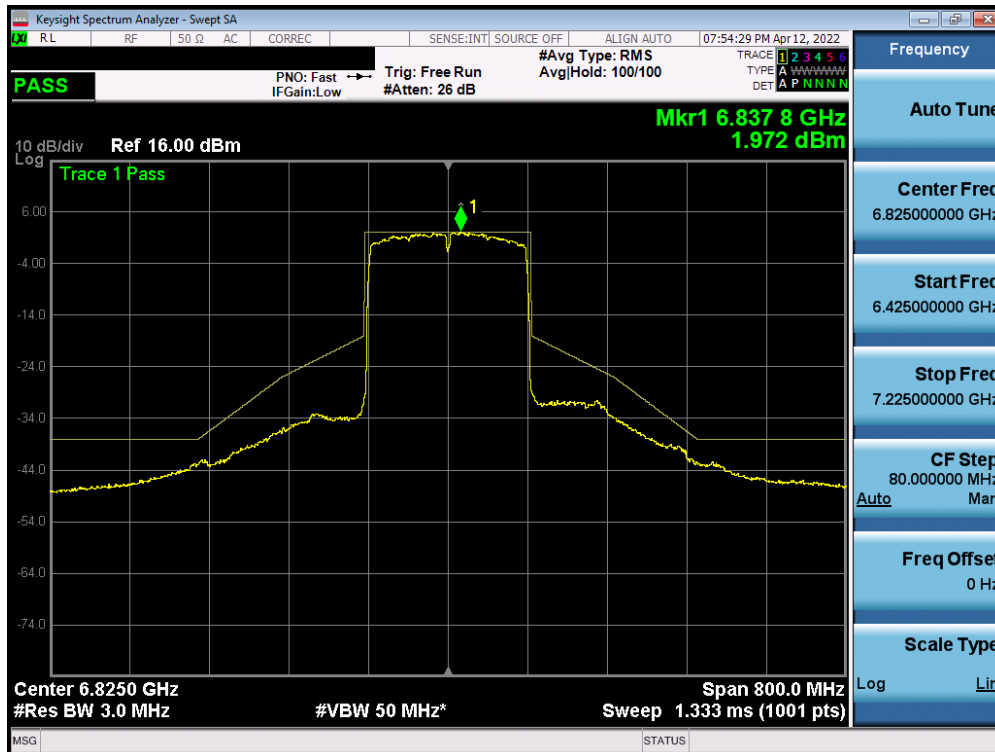
Plot 7-508. In-Band Emission Plot Measurement SISO ANT2 (160MHz 802.11ax (UNII Band 7) – Ch. 175)
