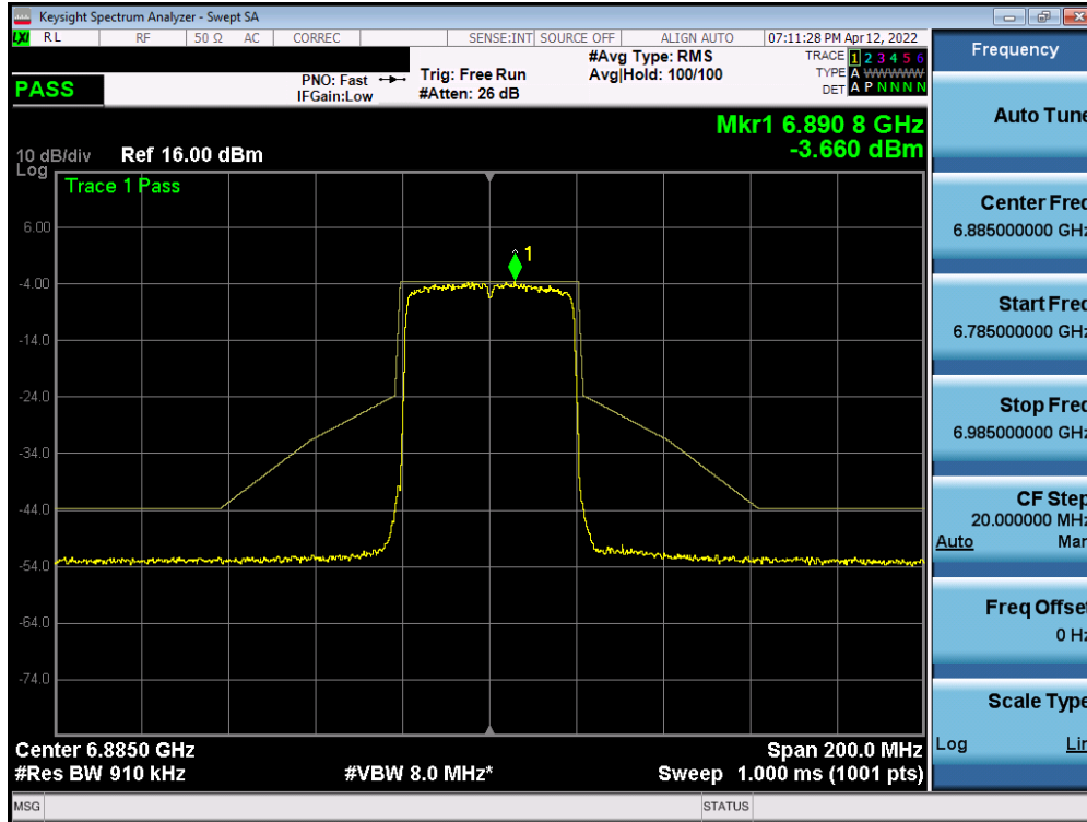
Plot 7-463. In-Band Emission Plot Measurement SISO ANT1 (40MHz 802.11ax (UNII Band 8) – Ch. 187)
