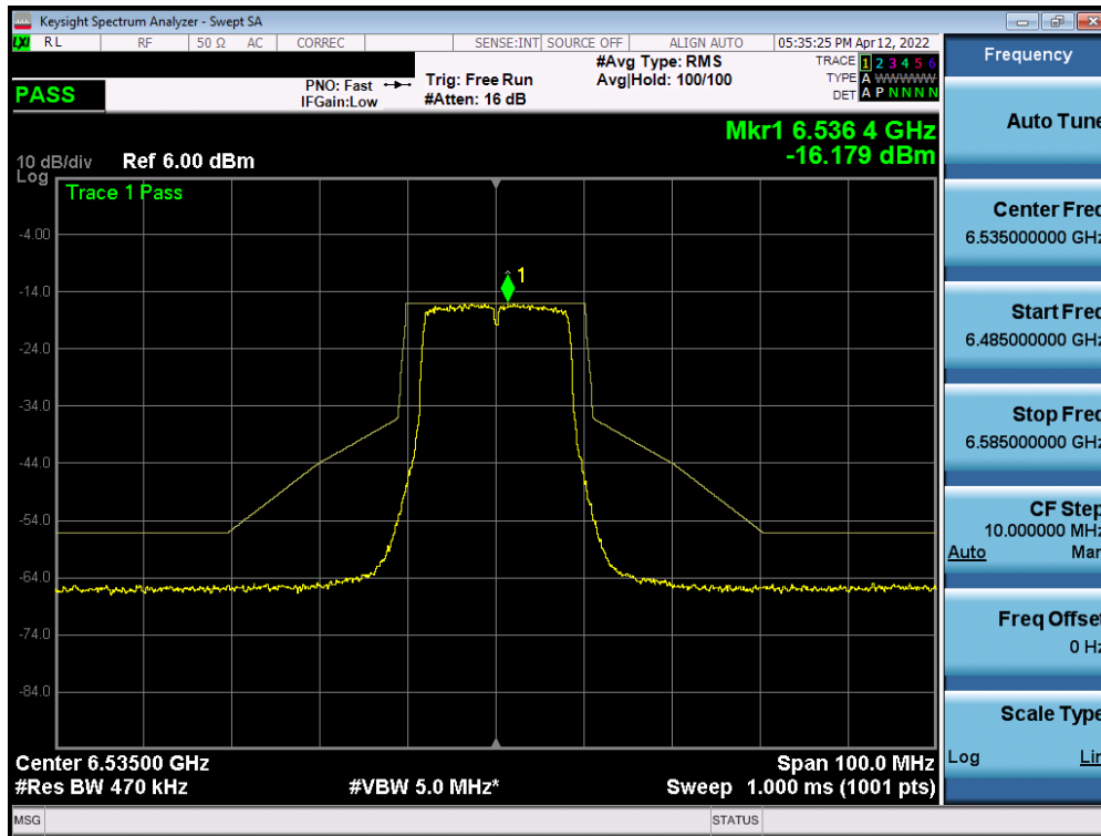
Plot 7-495. In-Band Emission Plot Measurement SISO ANT2 (20MHz 802.11a (UNII Band 7) – Ch. 117)
