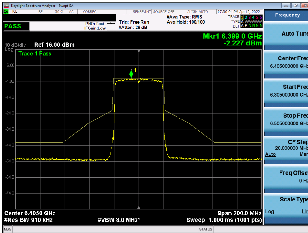
Plot 7-477. In-Band Emission Plot Measurement SISO ANT2 (40MHz 802.11ax (UNII Band 5) – Ch. 91)
