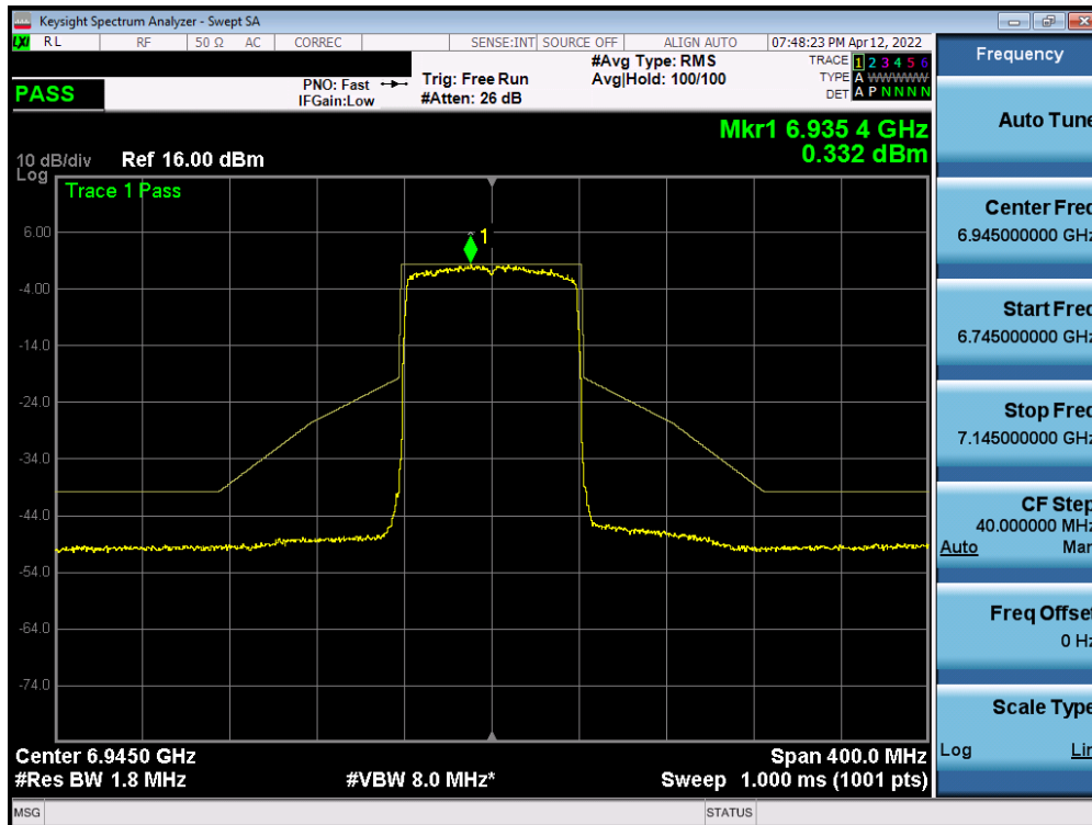
Plot 7-518. In-Band Emission Plot Measurement SISO ANT2 (80MHz 802.11ax (UNII Band 8) – Ch. 199)
