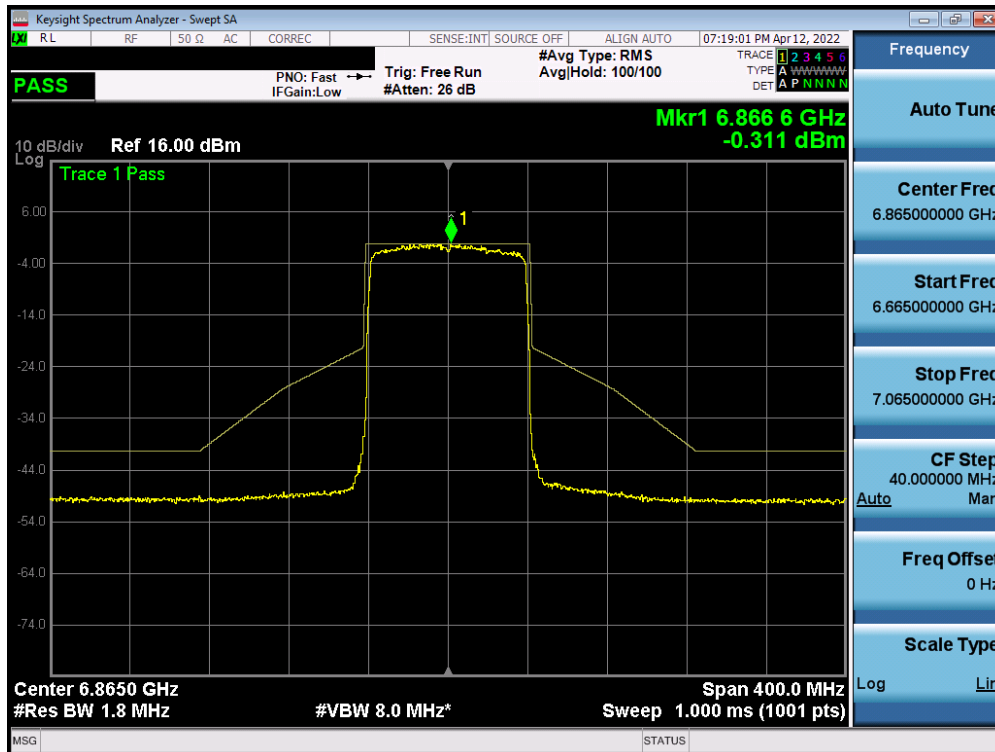
Plot 7-454. In-Band Emission Plot Measurement SISO ANT1 (80MHz 802.11ax (UNII Band 7) – Ch. 183)
