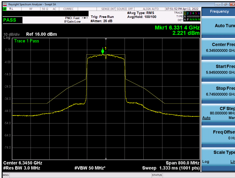
Plot 7-483. In-Band Emission Plot Measurement SISO ANT2 (160MHz 802.11ax (UNII Band 5) – Ch. 79)
