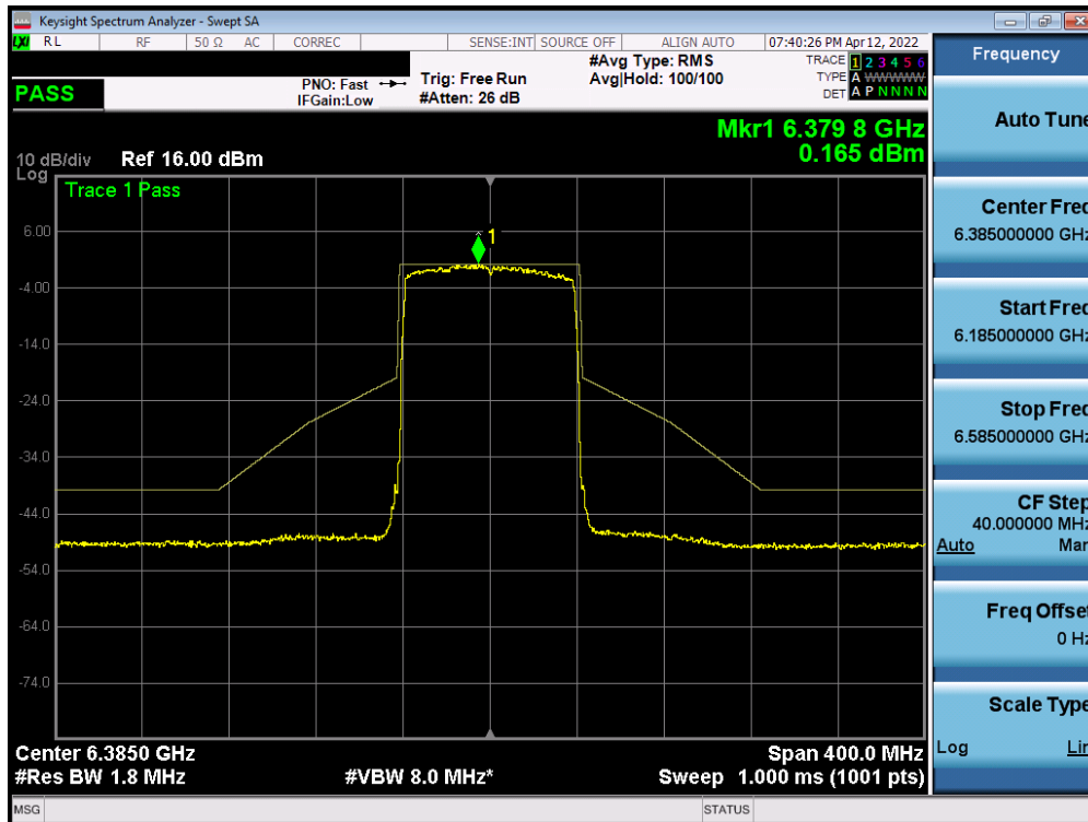
Plot 7-480. In-Band Emission Plot Measurement SISO ANT2 (80MHz 802.11ax (UNII Band 5) – Ch. 87)
