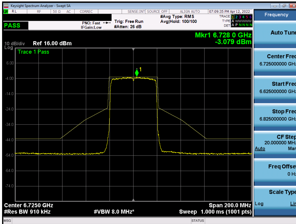
Plot 7-450. In-Band Emission Plot Measurement SISO ANT1 (40MHz 802.11ax (UNII Band 7) – Ch. 155)
