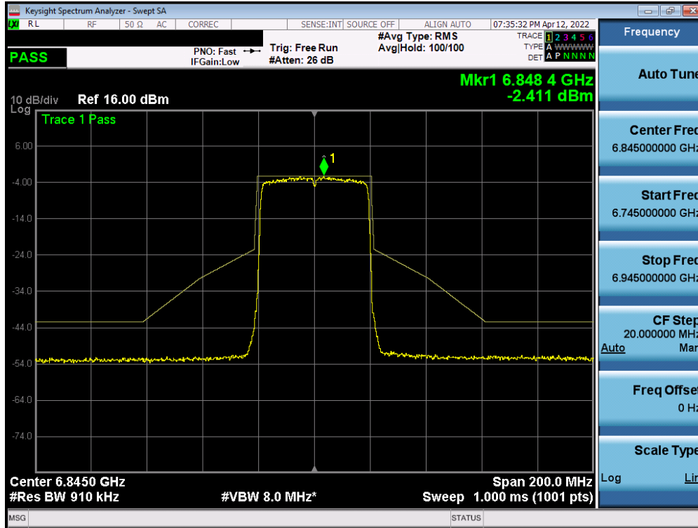
Plot 7-503. In-Band Emission Plot Measurement SISO ANT2 (40MHz 802.11ax (UNII Band 7) – Ch. 179)
