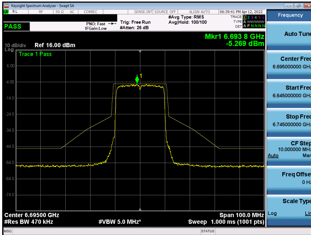
Plot 7-499. In-Band Emission Plot Measurement SISO ANT2 (20MHz 802.11ax (UNII Band 7) – Ch. 149)
