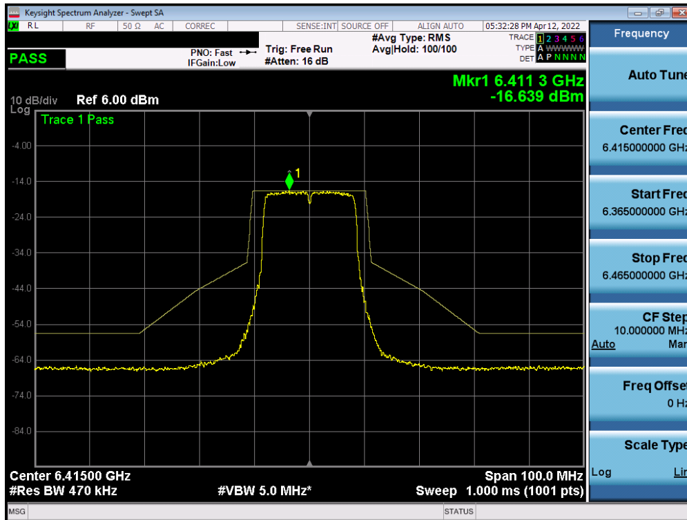
Plot 7-471. In-Band Emission Plot Measurement SISO ANT2 (20MHz 802.11a (UNII Band 5) – Ch. 93)
