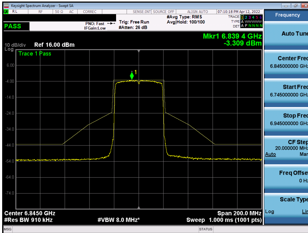
Plot 7-451. In-Band Emission Plot Measurement SISO ANT1 (40MHz 802.11ax (UNII Band 7) – Ch. 179)
