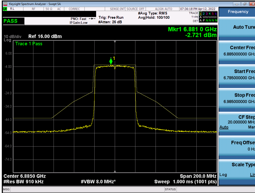
Plot 7-515. In-Band Emission Plot Measurement SISO ANT2 (40MHz 802.11ax (UNII Band 8) – Ch. 187)
