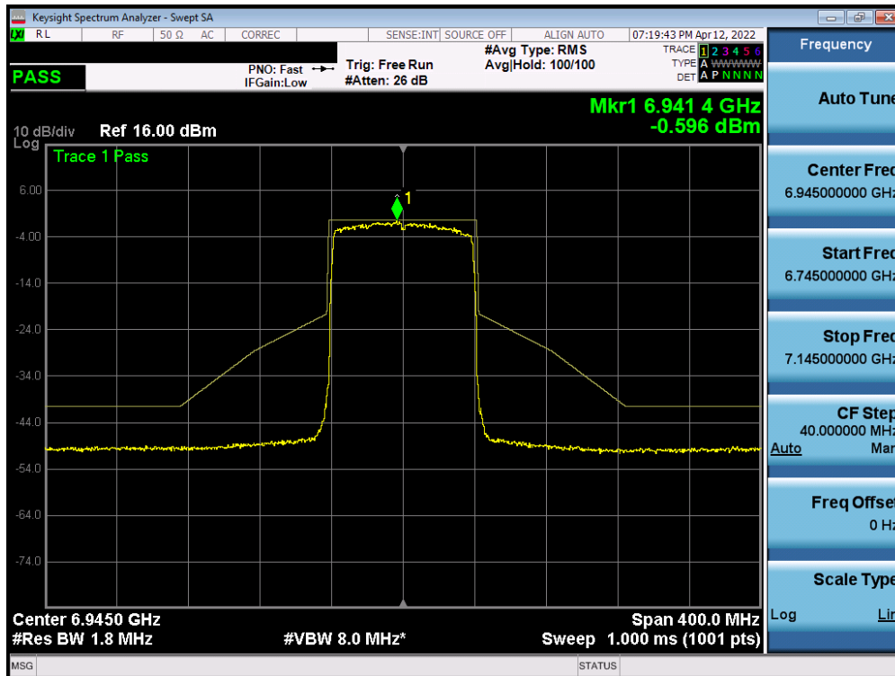
Plot 7-466. In-Band Emission Plot Measurement SISO ANT1 (80MHz 802.11ax (UNII Band 8) – Ch. 199)
