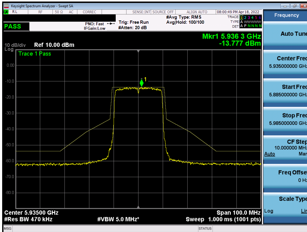
Plot 7-524. In-Band Emission Plot Measurement MIMO ANT1 (20MHz 802.11ax (UNII Band 5) – Ch. 2)
