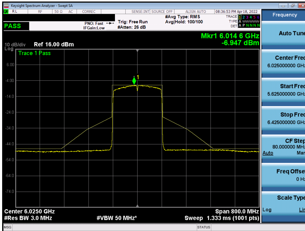
Plot 7-533. In-Band Emission Plot Measurement MIMO ANT1 (160MHz 802.11ax (UNII Band 5) – Ch. 15)
