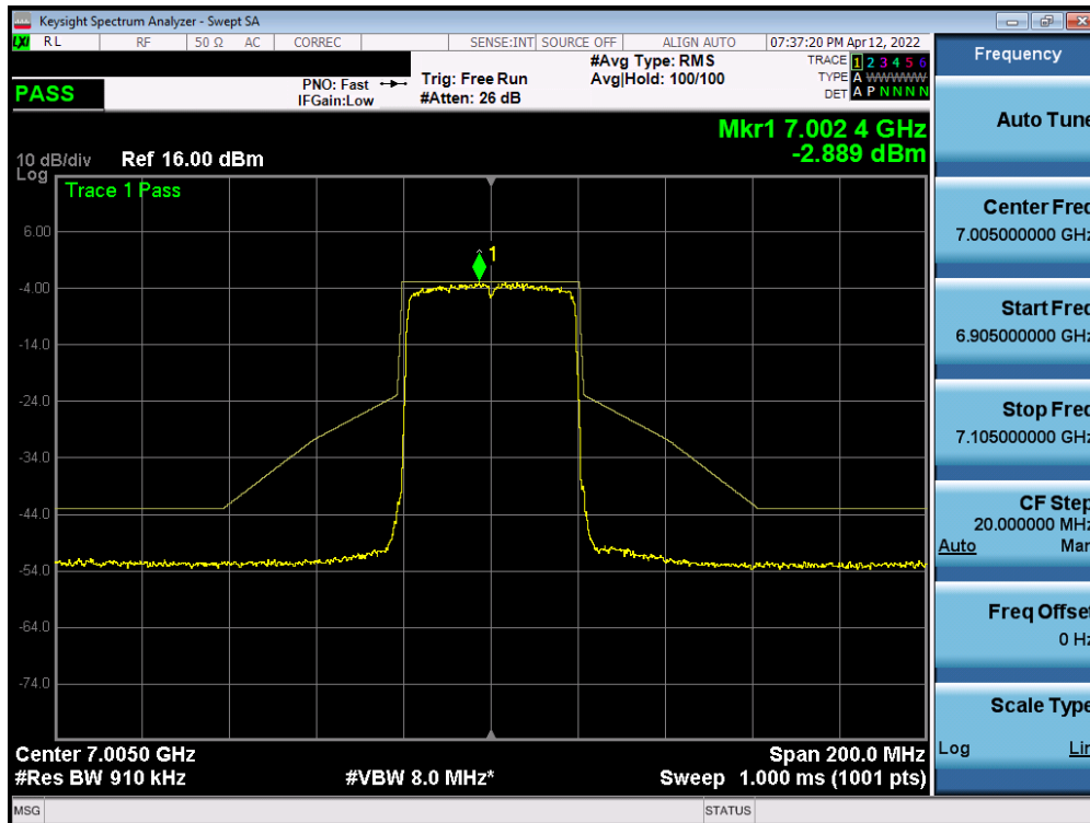
Plot 7-516. In-Band Emission Plot Measurement SISO ANT2 (40MHz 802.11ax (UNII Band 8) – Ch. 211)
