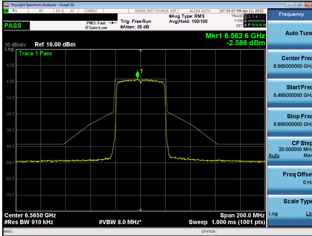
Plot 7-501. In-Band Emission Plot Measurement SISO ANT2 (40MHz 802.11ax (UNII Band 7) – Ch. 123)
