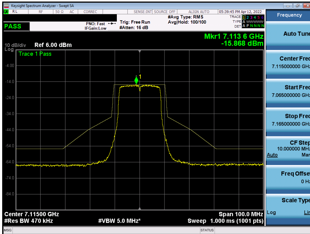
Plot 7-511. In-Band Emission Plot Measurement SISO ANT2 (20MHz 802.11a (UNII Band 8) – Ch. 233)
