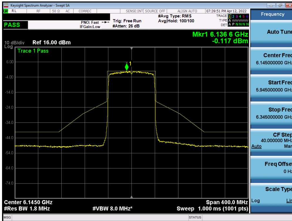
Plot 7-479. In-Band Emission Plot Measurement SISO ANT2 (80MHz 802.11ax (UNII Band 5) – Ch. 39)
