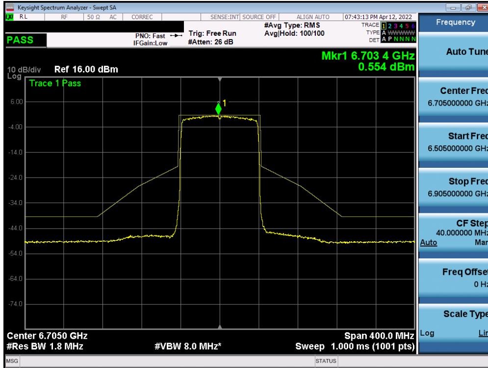
Plot 7-505. In-Band Emission Plot Measurement SISO ANT2 (80MHz 802.11ax (UNII Band 7) – Ch. 151)
