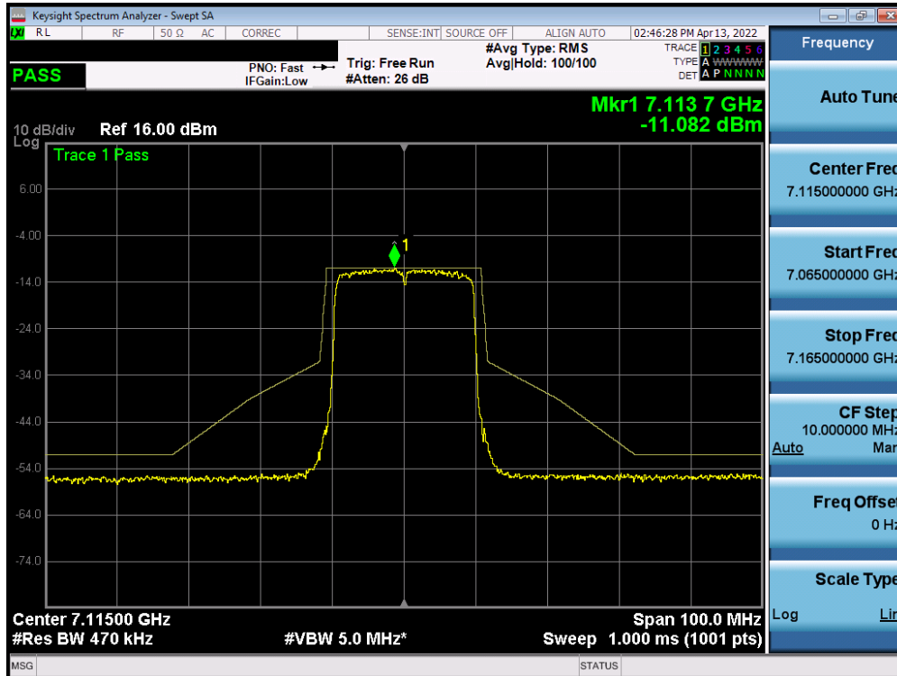
Plot 7-462. In-Band Emission Plot Measurement SISO ANT1 (20MHz 802.11ax (UNII Band 8) – Ch. 233)
