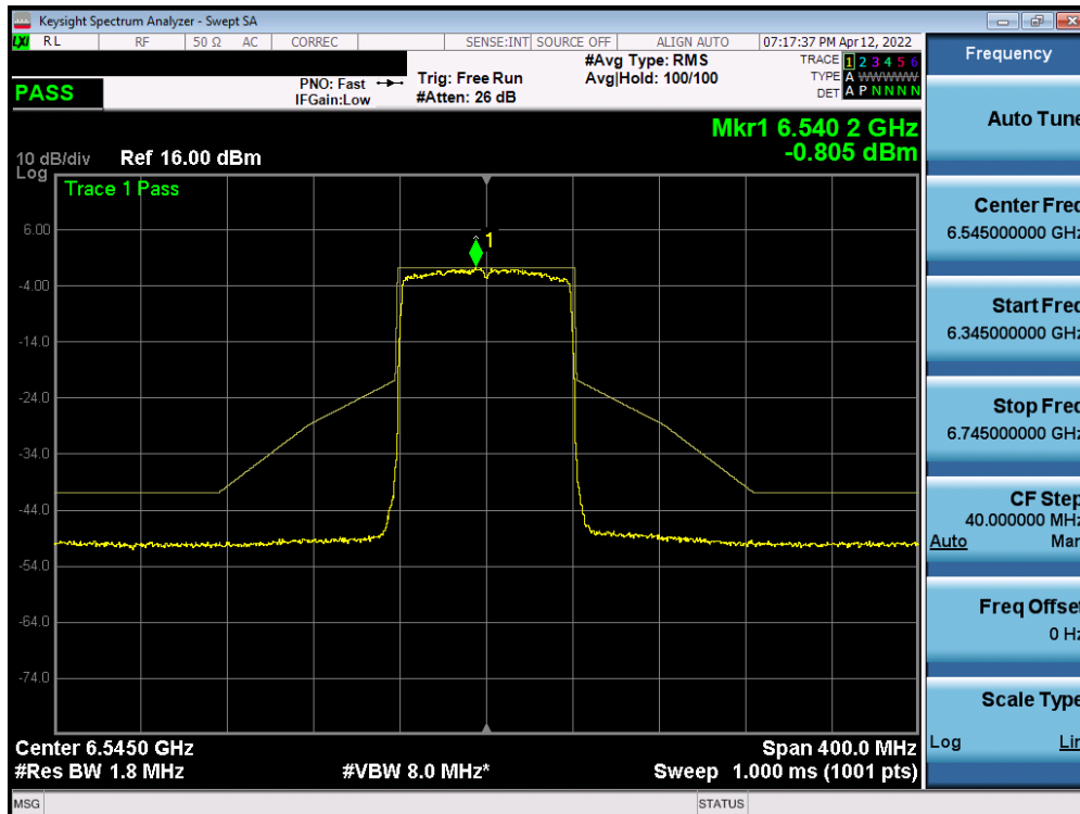
Plot 7-452. In-Band Emission Plot Measurement SISO ANT1 (80MHz 802.11ax (UNII Band 7) – Ch. 119)
