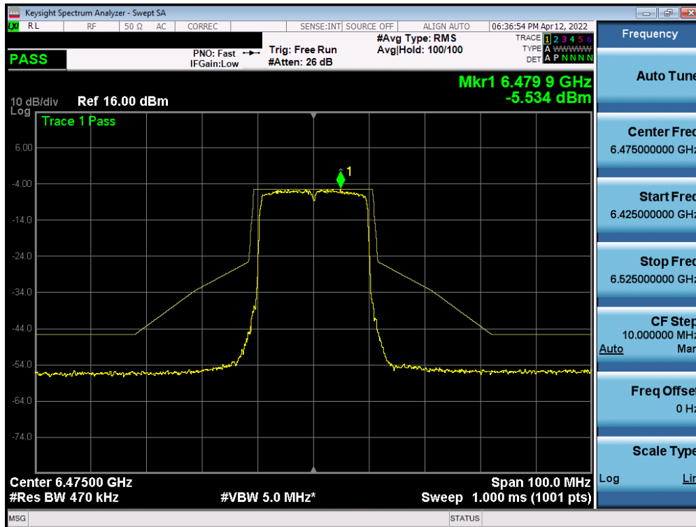
Plot 7-488. In-Band Emission Plot Measurement SISO ANT2 (20MHz 802.11ax (UNII Band 6) – Ch. 105)
