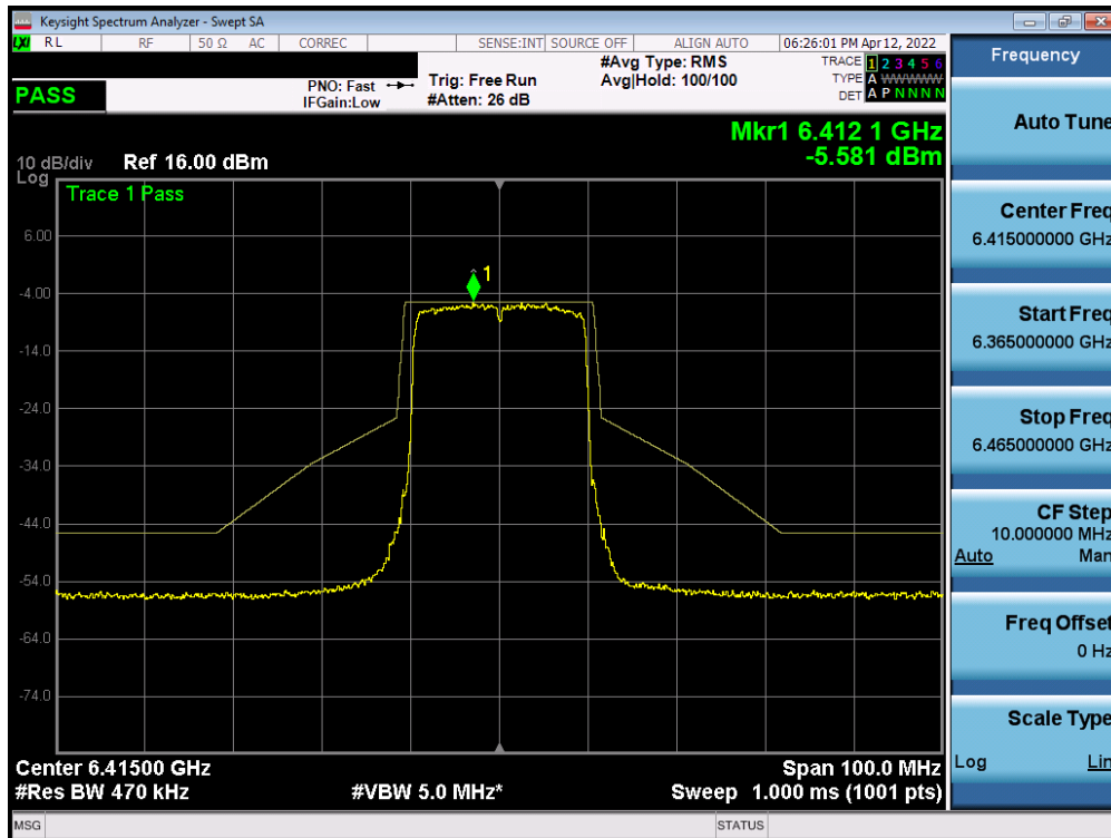
Plot 7-474. In-Band Emission Plot Measurement SISO ANT2 (20MHz 802.11ax (UNII Band 5) – Ch. 93)
