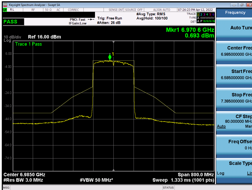
Plot 7-468. In-Band Emission Plot Measurement SISO ANT1 (160MHz 802.11ax (UNII Band 8) – Ch. 207)
