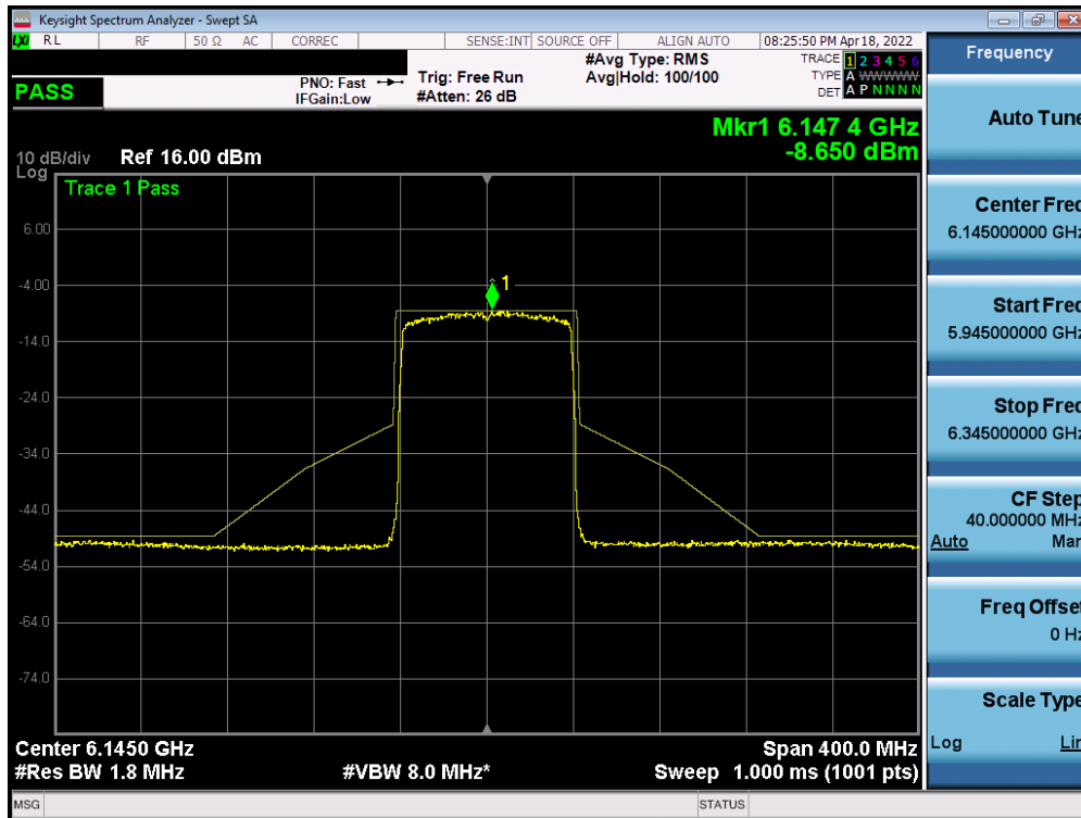
Plot 7-531. In-Band Emission Plot Measurement MIMO ANT1 (80MHz 802.11ax (UNII Band 5) – Ch. 39)
