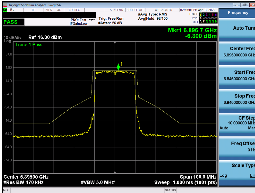
Plot 7-460. In-Band Emission Plot Measurement SISO ANT1 (20MHz 802.11ax (UNII Band 8) – Ch. 189)
