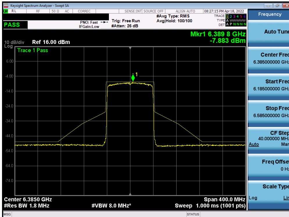
Plot 7-532. In-Band Emission Plot Measurement MIMO ANT1 (80MHz 802.11ax (UNII Band 5) – Ch. 87)
