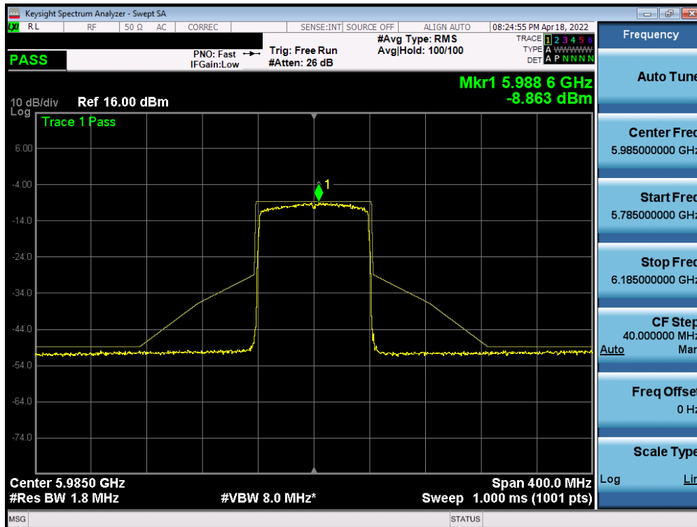
Plot 7-530. In-Band Emission Plot Measurement MIMO ANT1 (80MHz 802.11ax (UNII Band 5) – Ch. 7)
