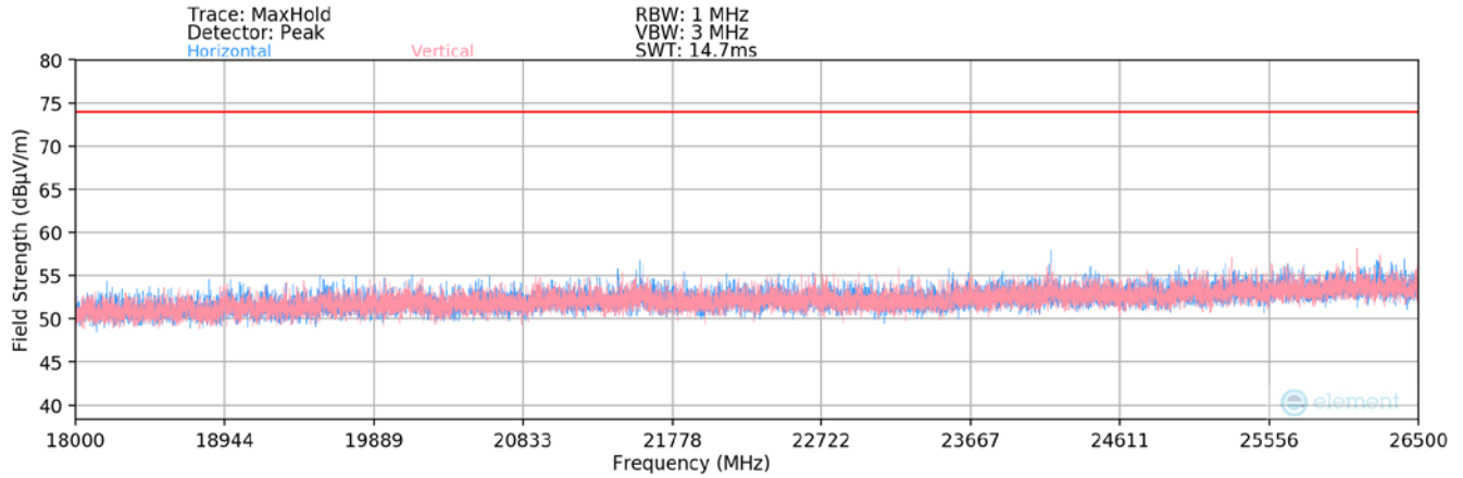
Plot 7-45. Radiated Spurious Plot above 18GHz GFSK
