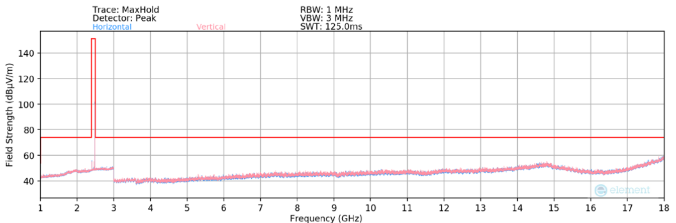
Plot 7-44. Radiated Spurious Plot above 1GHz (BT GFSK – Ch. 78)
