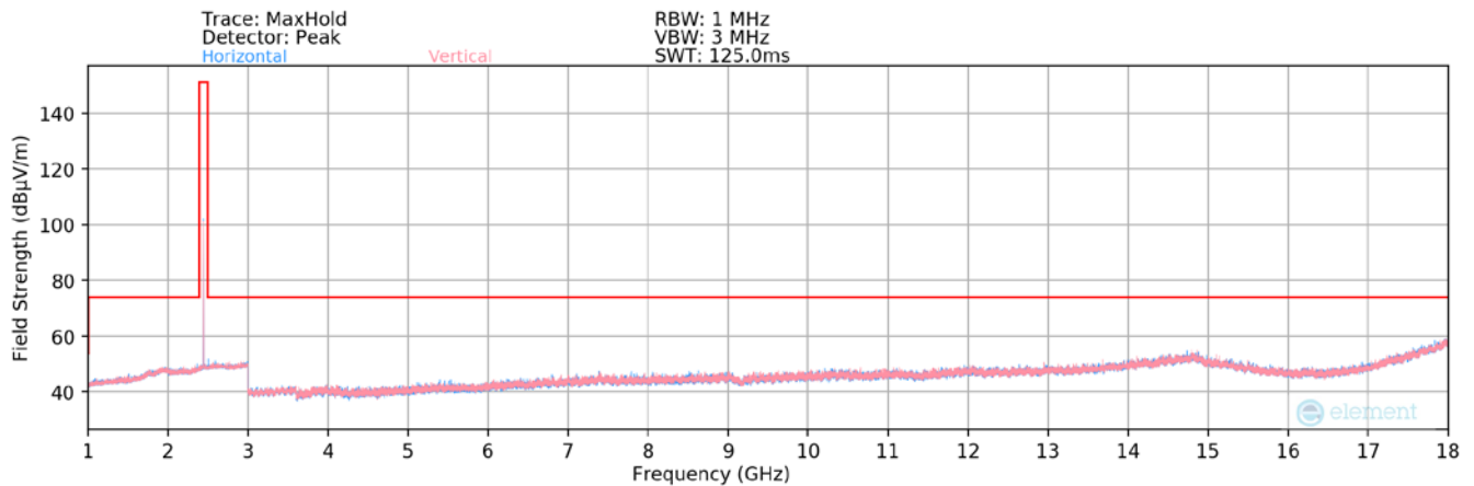
Plot 7-43. Radiated Spurious Plot above 1GHz (BT GFSK – Ch. 39)
