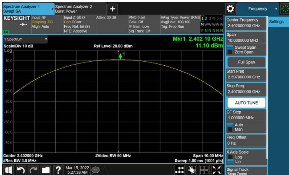
Plot 7-10. Peak Conducted Power (1Mbps – Ch. 0)
