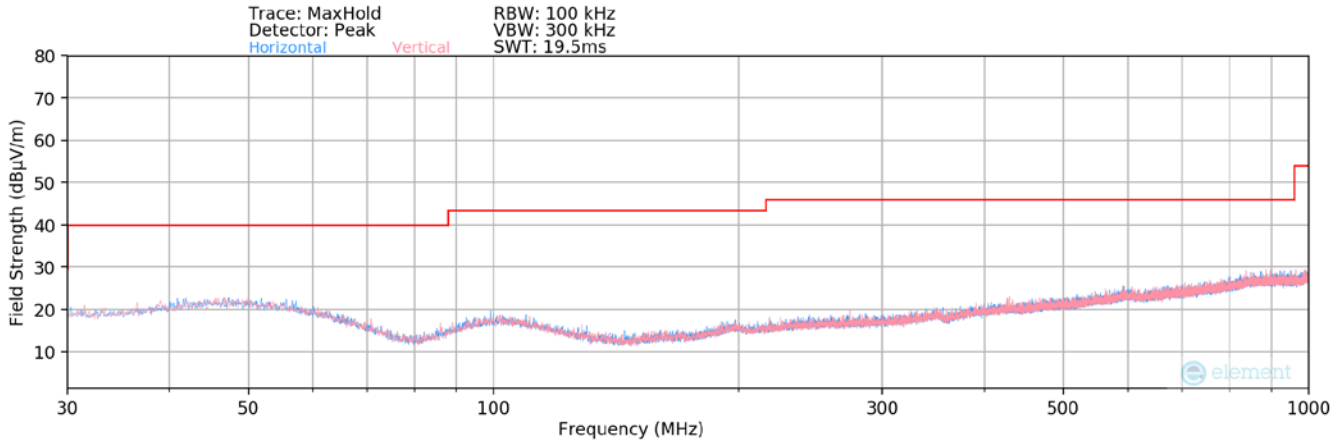
Plot 7-48. Radiated Spurious Plot below 1GHz GFSK
