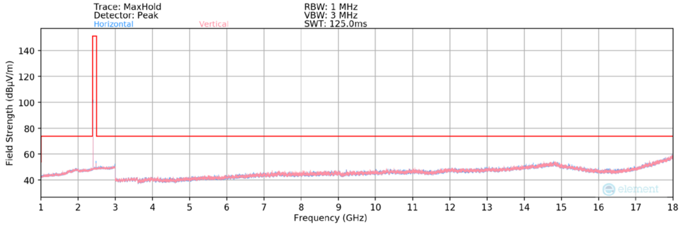
Plot 7-42. Radiated Spurious Plot above 1GHz (BT GFSK – Ch. 0)
