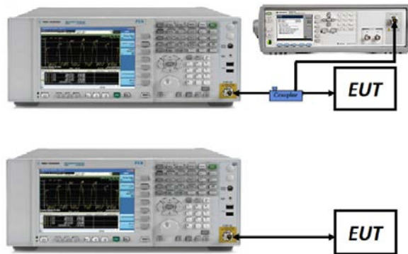
Figure 7-1. Test Instrument & Measurement Setup
