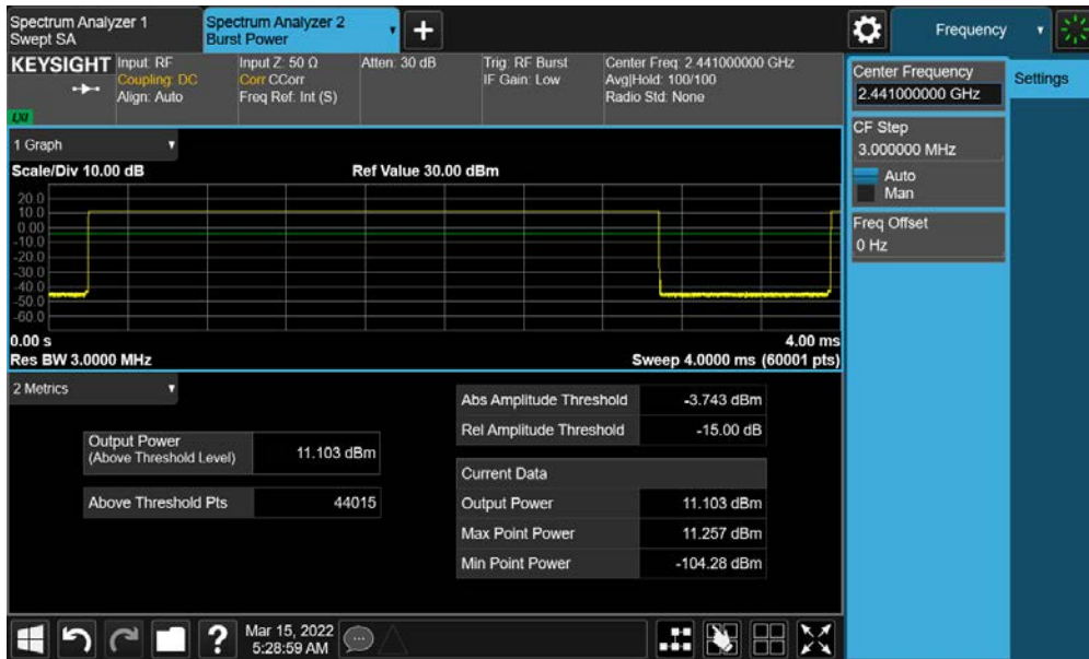
Plot 7-20. Average Conducted Power (1Mbps – Ch. 39)
