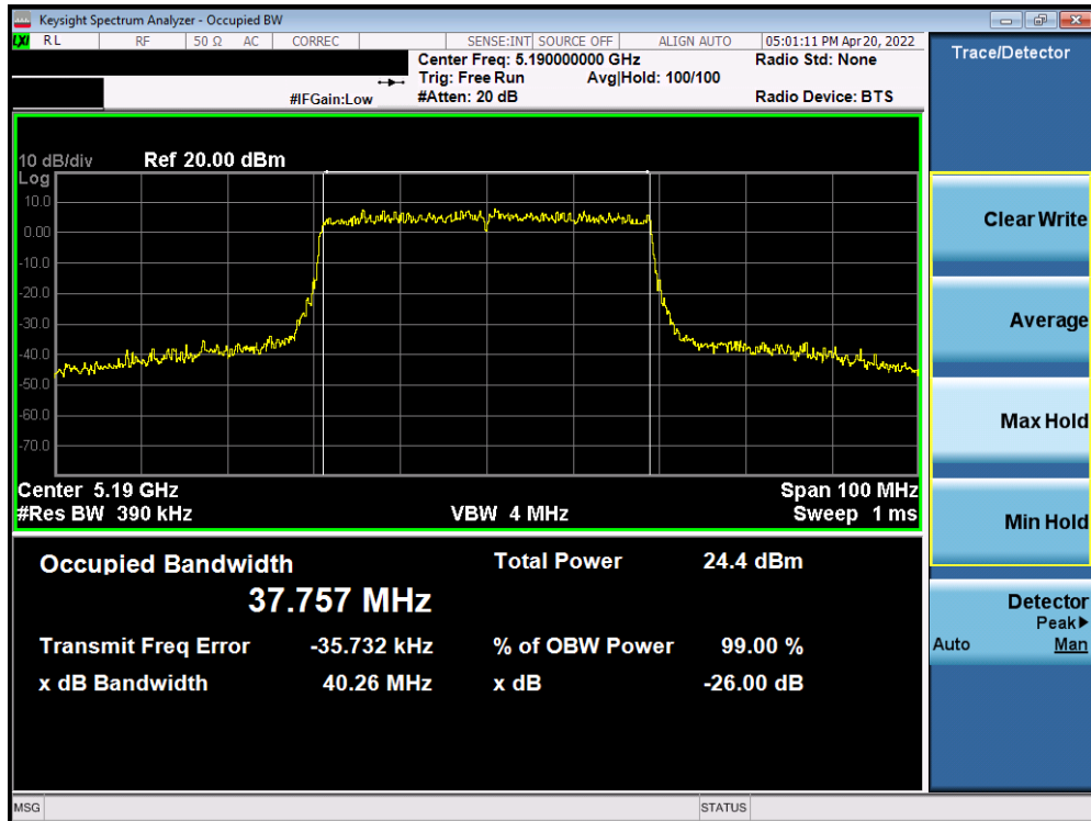
Plot 7-67. 26dB Bandwidth Plot SISO ANT2 (40MHz BW 802.11ax (UNII Band 1) – Ch. 38)
