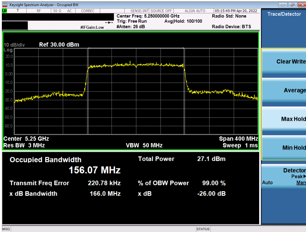
Plot 7-72. 26dB Bandwidth Plot SISO ANT2 (160MHz BW 802.11ax (UNII Band 1/2A) – Ch. 50)
