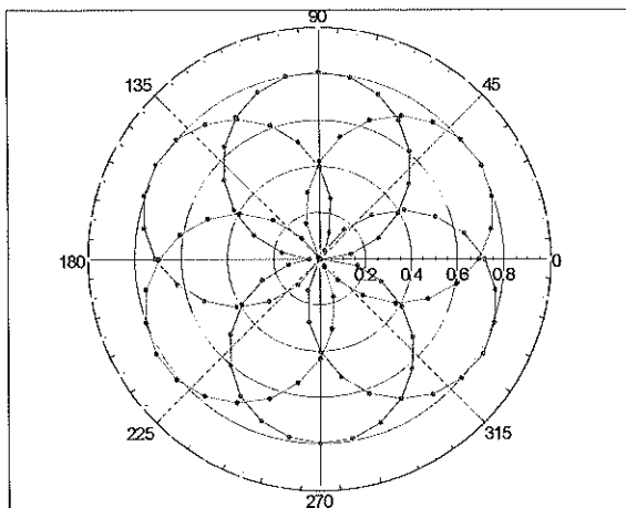
f=600 MHz,TEM
