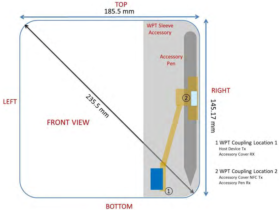
Figure E-3 WPT Sleeve and Pen Accessory Antenna Locations Read/Flat Configuration (Body)
