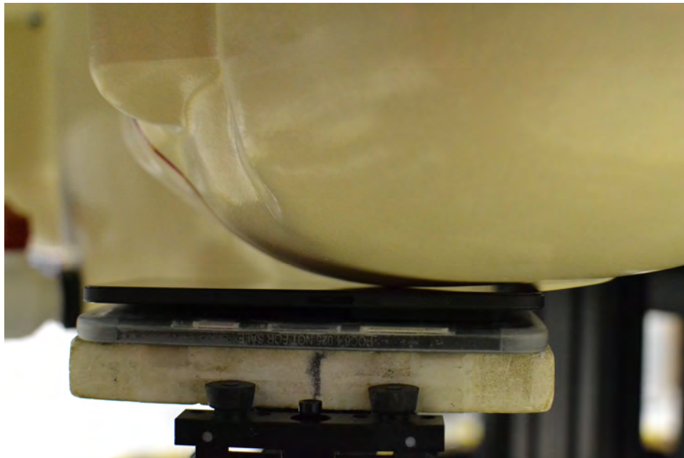
SAR Test Setup Photo 40 – Flip Configuration (Handset) Left Cheek with WPT Sleeve
