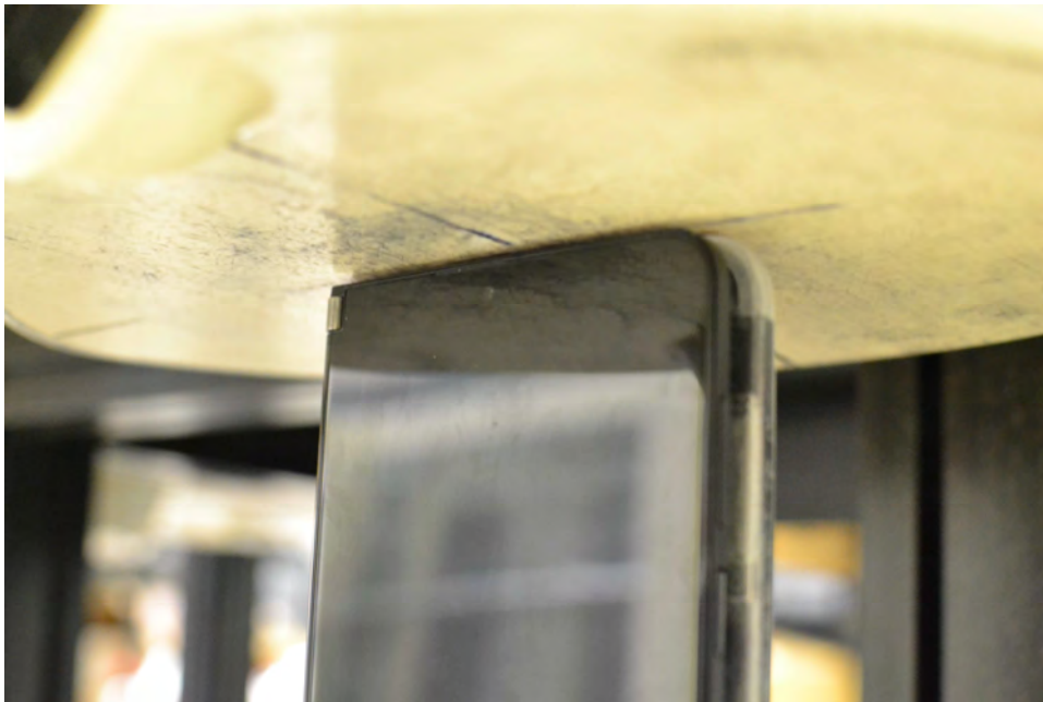
SAR Test Setup Photo 44 – Flip Configuration (Handset) Top Edge at 0 mm with WPT Sleeve
