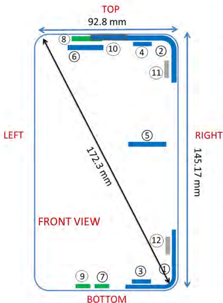
Figure E-1 DUT Antenna Locations Flip/Closed Configuration (Handset)
