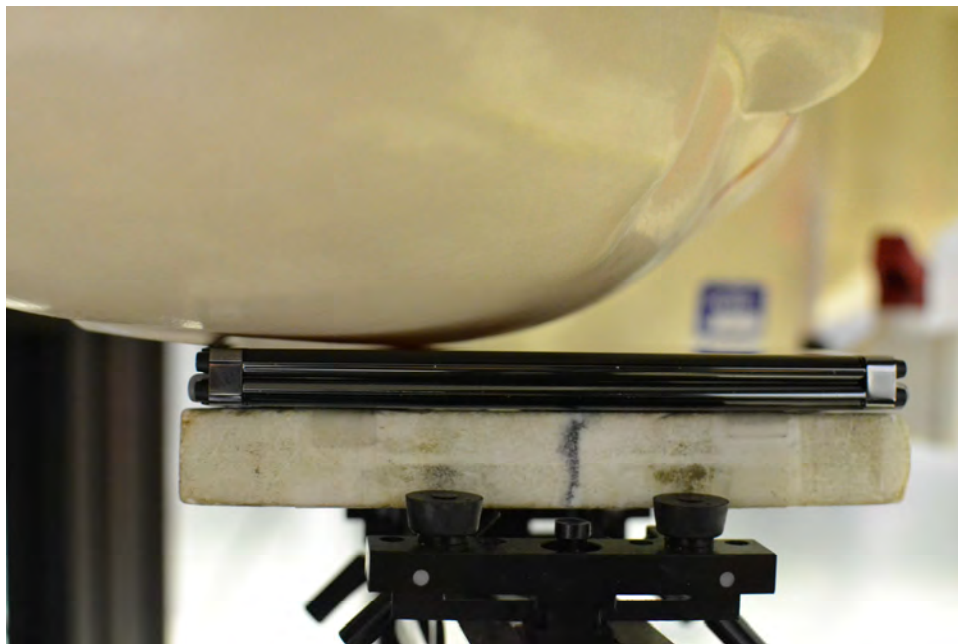
SAR Test Setup Photo 38 – Flip Configuration (Handset) Right Cheek with WPT Sleeve
