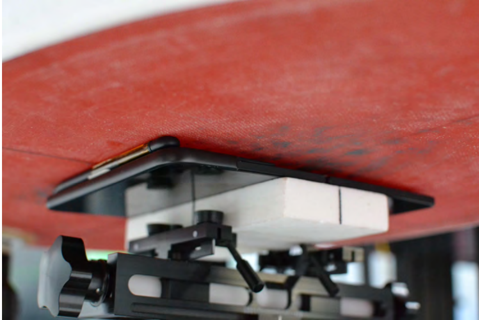
SAR Test Setup Photo 47 – Flat Configuration (Body) – Front Side of Sleeve/Pen at 0mm with WPT Sleeve and Pen
