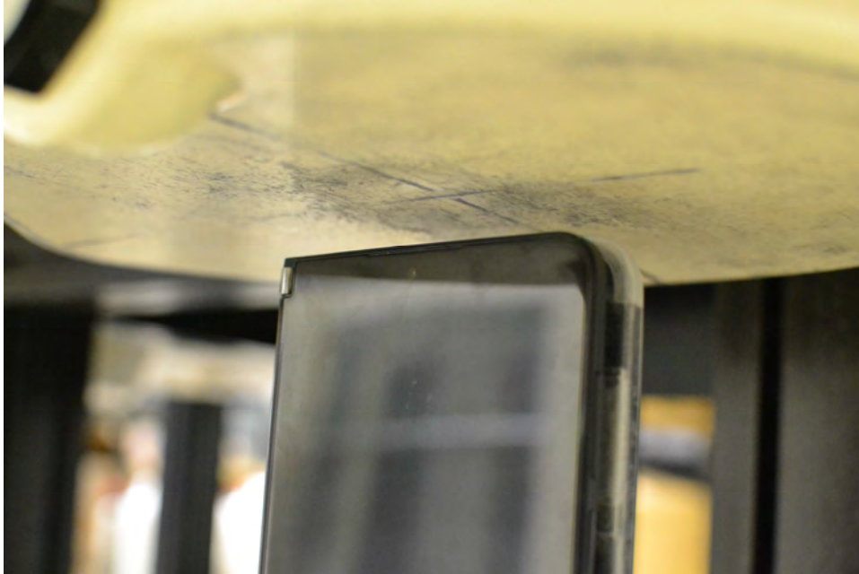
SAR Test Setup Photo 43 – Flip Configuration (Handset) Top Edge at 10 mm with WPT Sleeve
