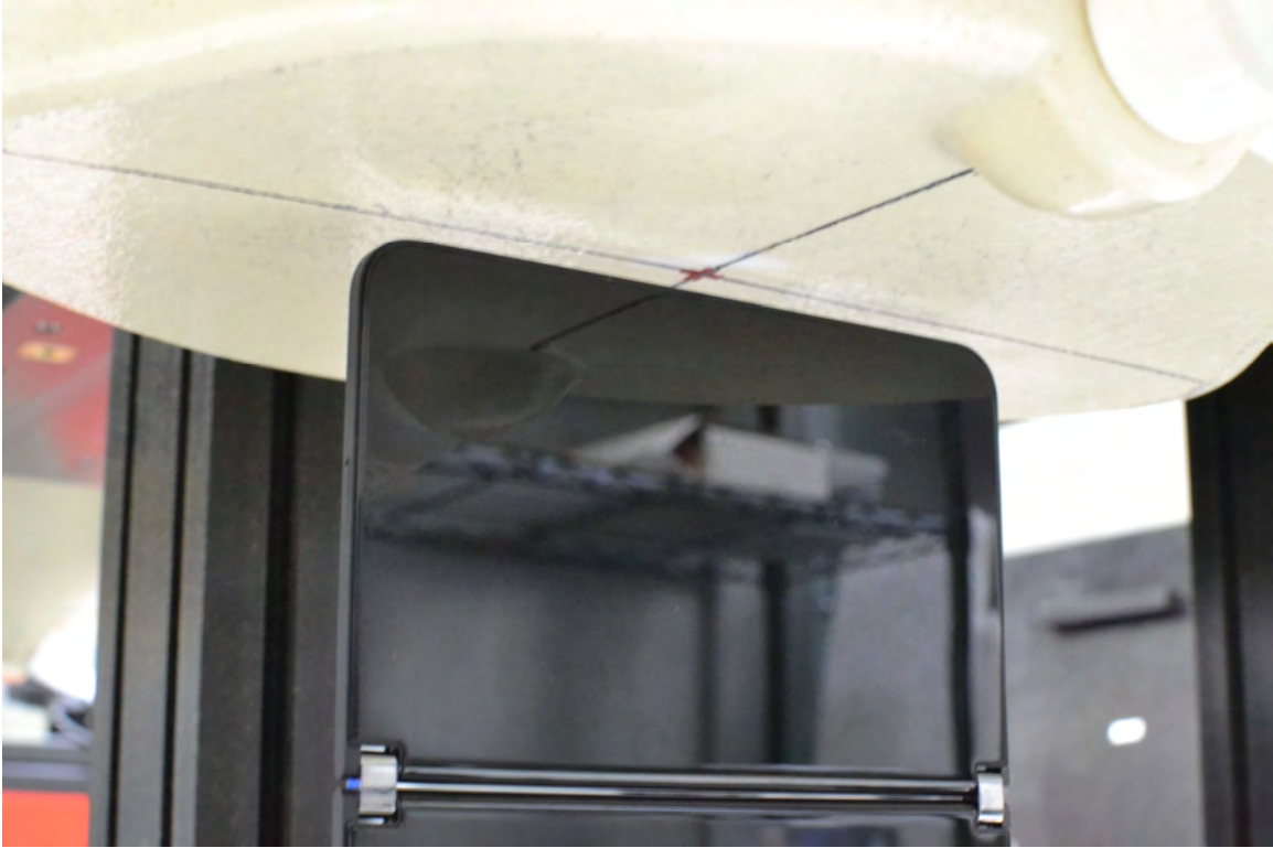
SAR Test Setup Photo 29– Read Configuration (UMPC), UMPC Extremity, Left Edge, 5 mm
