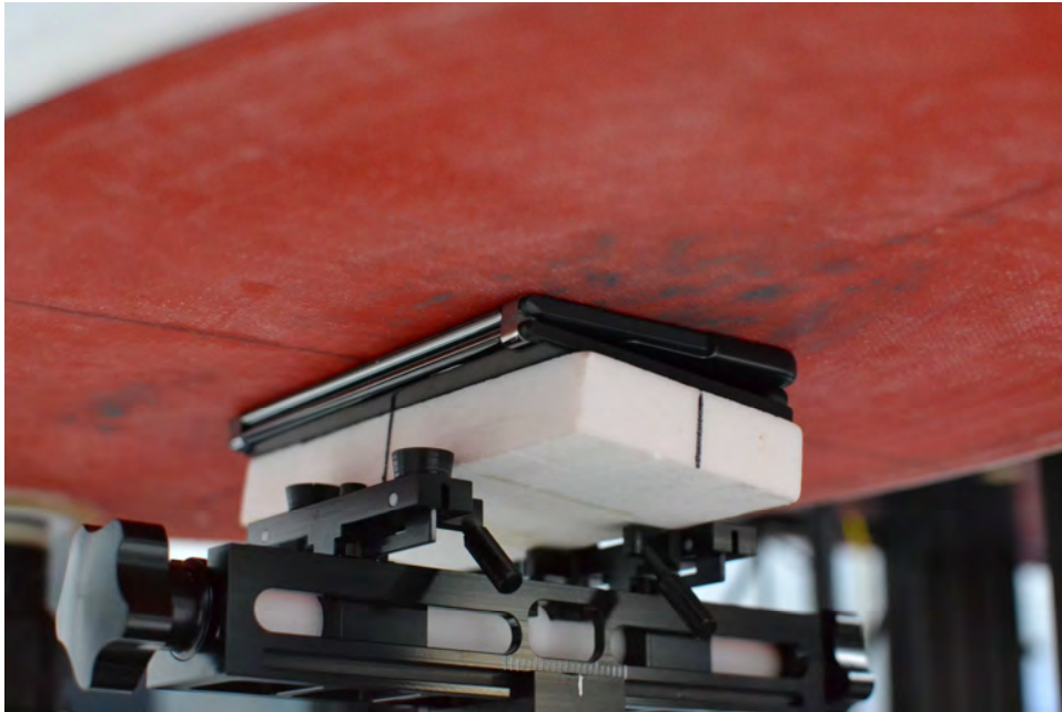
SAR Test Setup Photo 52 – Flip Configuration (Body) – Front Side at 0mm with WPT Sleeve and Pen
