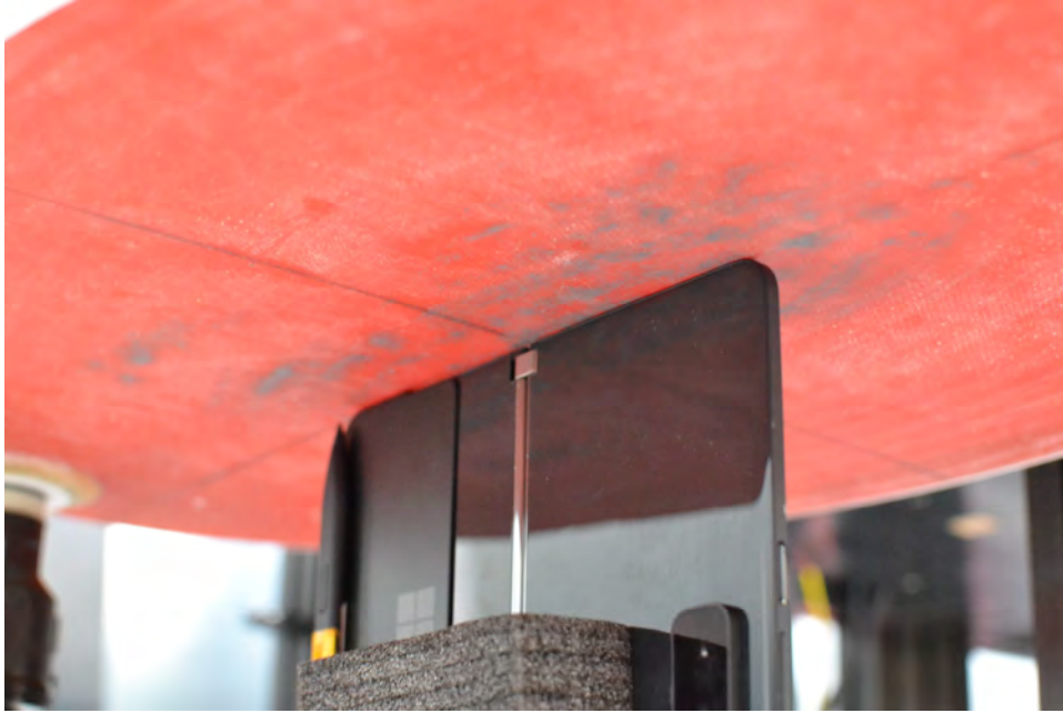
SAR Test Setup Photo 51 – Flat Configuration (Body) – Bottom Edge at 0mm with WPT Sleeve and Pen
