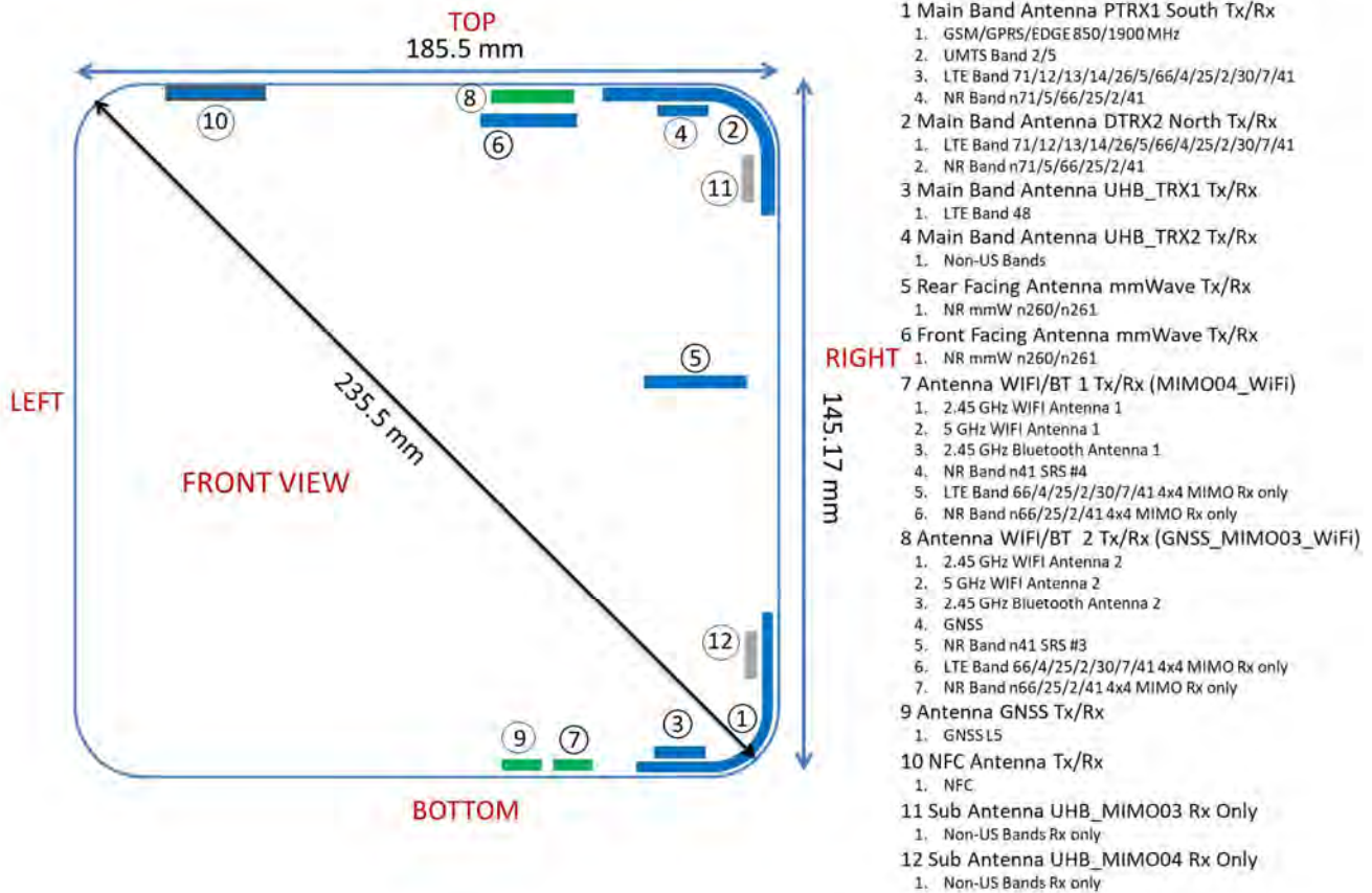
Figure E-2 DUT Antenna Locations Read/Flat Configuration (UMPC and Body)
