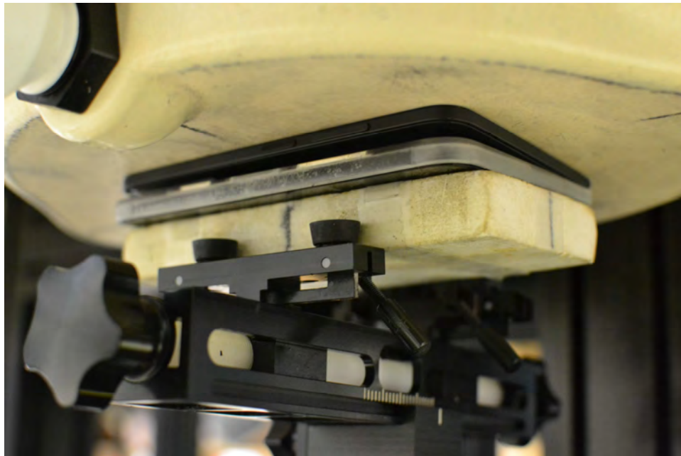
SAR Test Setup Photo 42 – Flip Configuration (Handset) Front Side at 0 mm with WPT Sleeve
