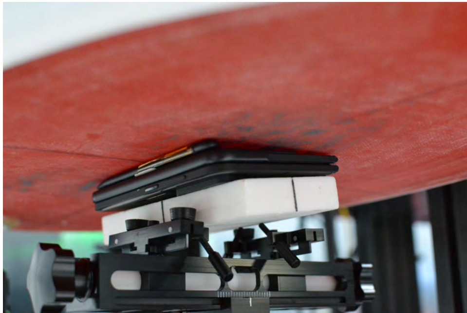
SAR Test Setup Photo 46 – Closed Configuration (Body) – Front Side at 0mm with WPT Sleeve and Pen
