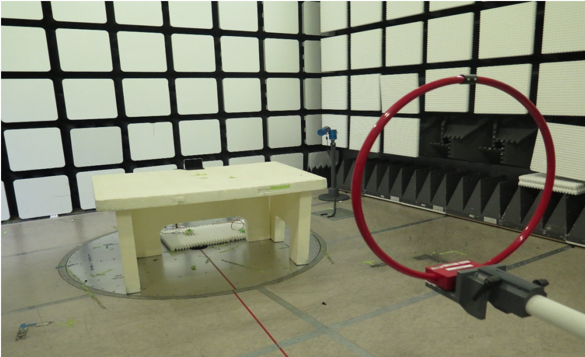
Figure 1 Radiated Spurious Emissions Test Setup (9k-30MHz) – Flat Posture – Y - Parallel
