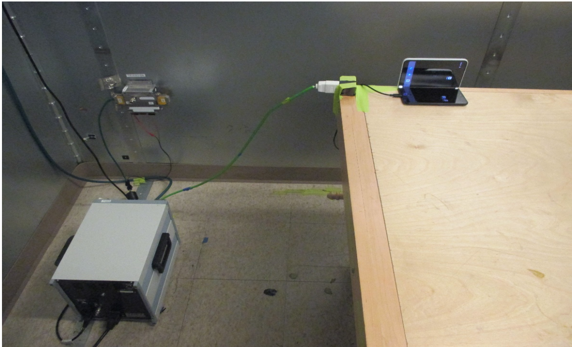
Figure 9 AC Line Conducted Emissions Test Setup
