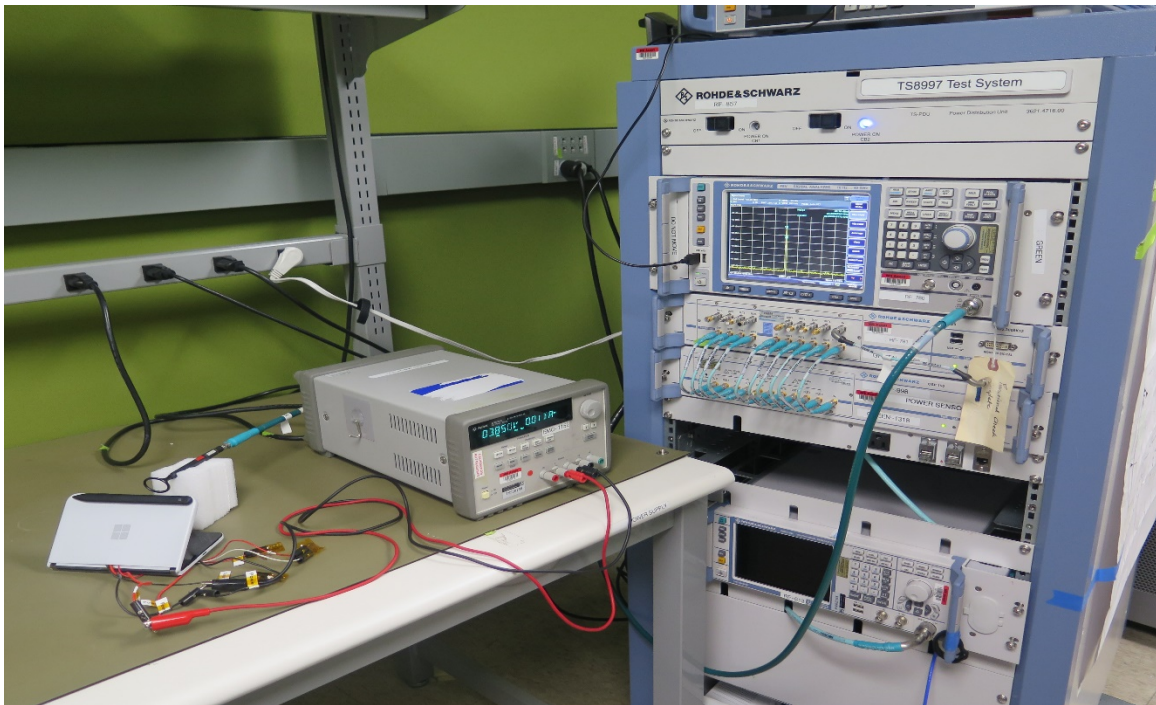
Figure 7 Conducted Test Setup for variable voltage
