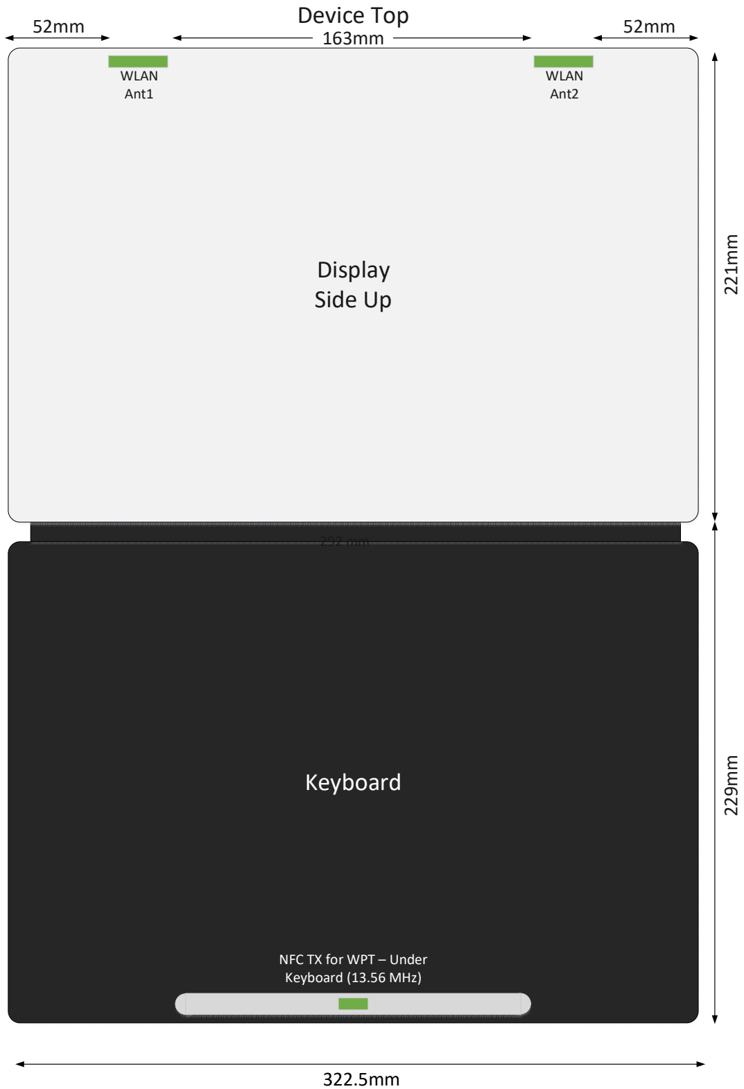
Fig. 1 – Antenna Position Diagram
