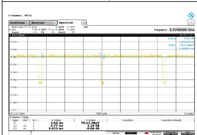
802.11ax HE160 OFDMA, OFDMA MODE: SU
