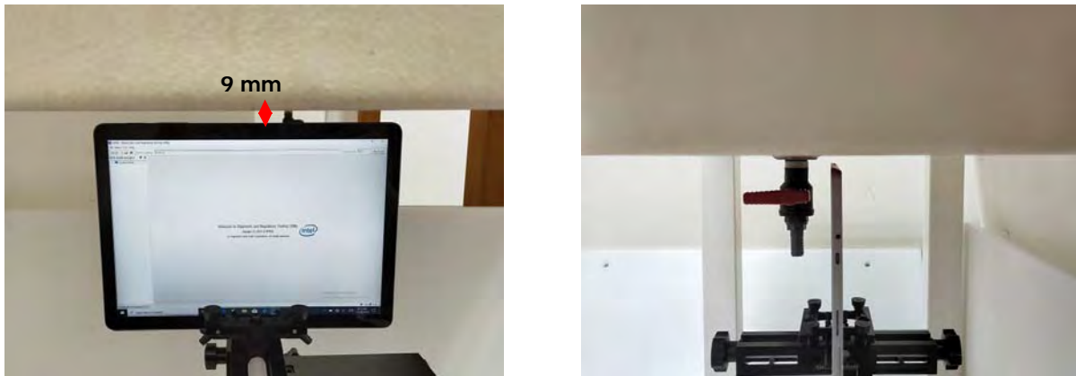
Fig.10 EUT Top side to flat phantom
