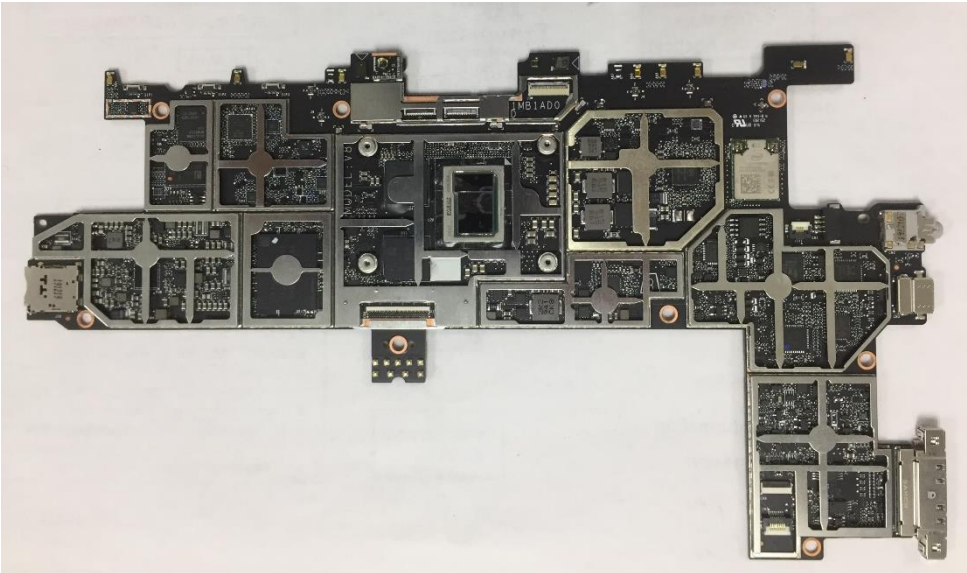
Figure 2 Main logic board-without shield cans-Top View
