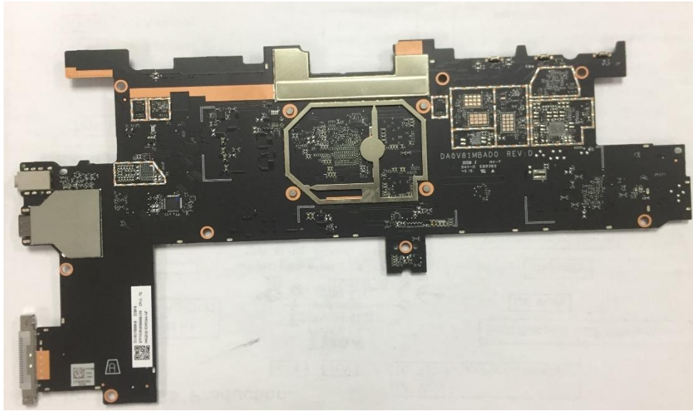
Figure 3 Main logic board-without shield cans-Back View
