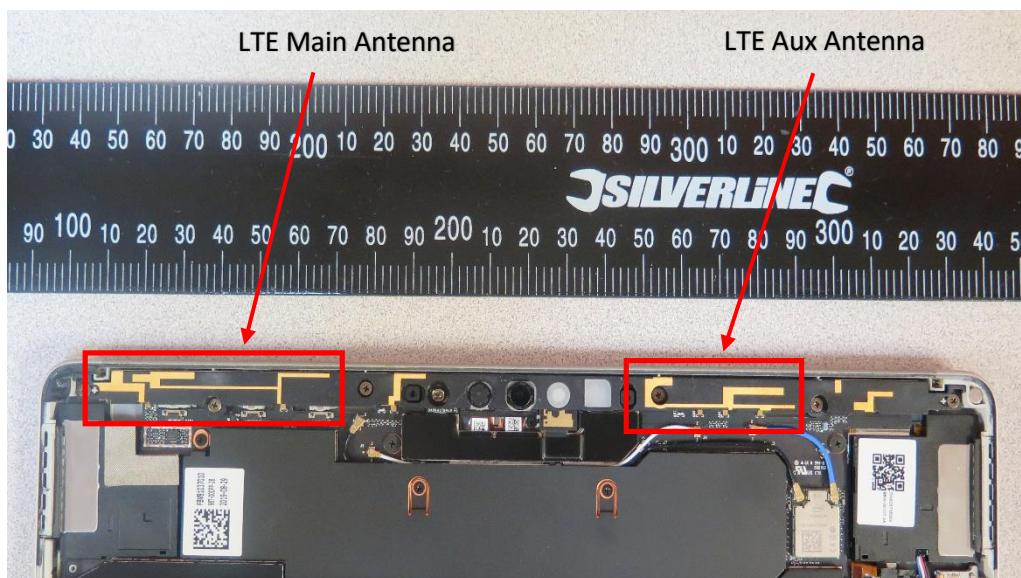
Figure 8 LTE Antenna- Close-up-Top View
