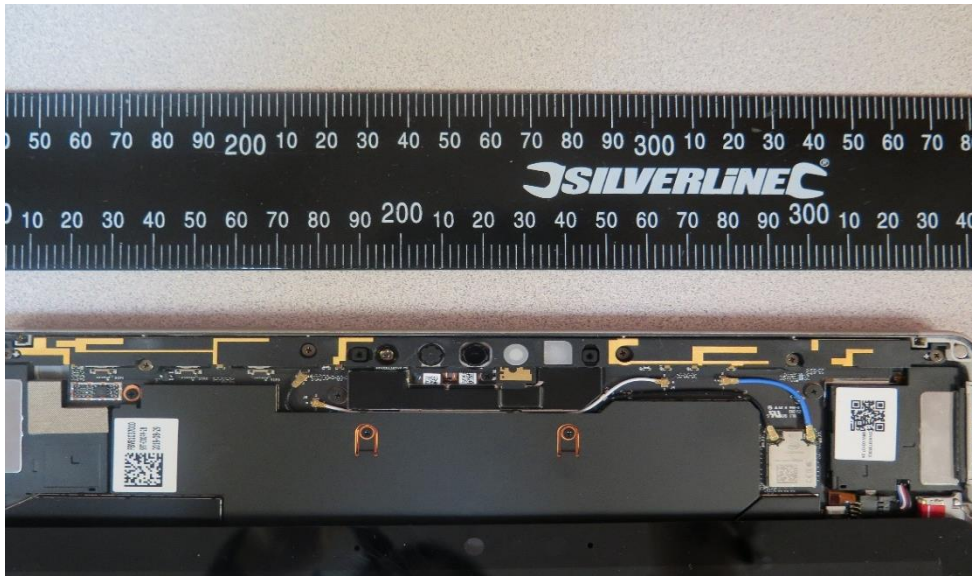
Figure 4 Close up Wi-Fi RF section
