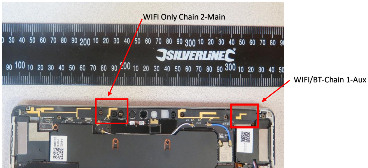
Figure 6 Wi-Fi Antenna- Close-up-Top View
