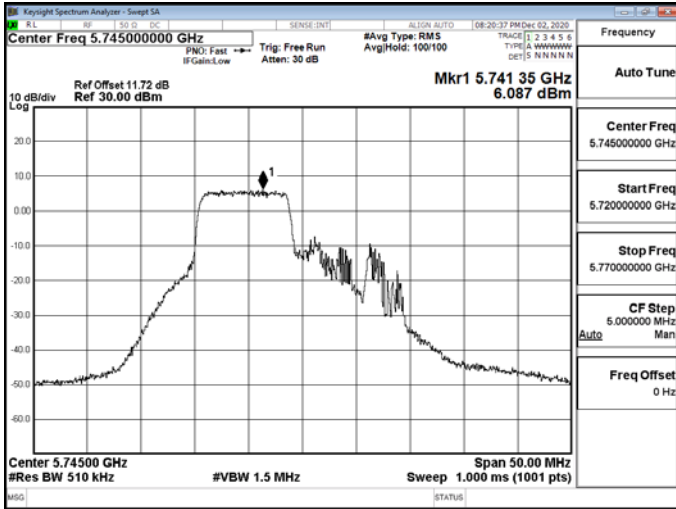
802.11ax_20MHz_RU_26_0_5745MHz-5745
