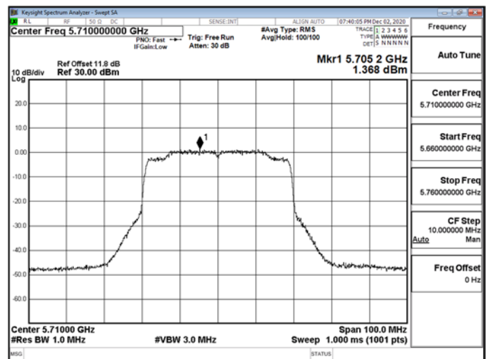
802.11ax_40MHz_5710MHz_UNII 3
