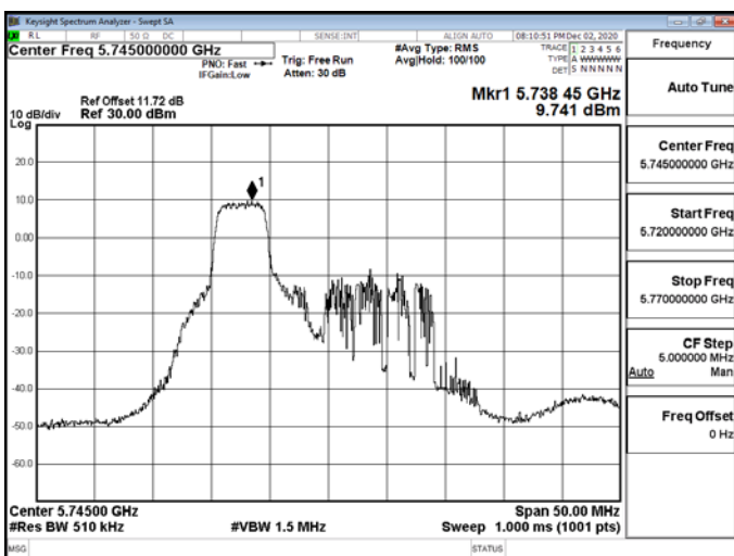
802.11ax_20MHz_RU_52_37_5745MHz-5745
