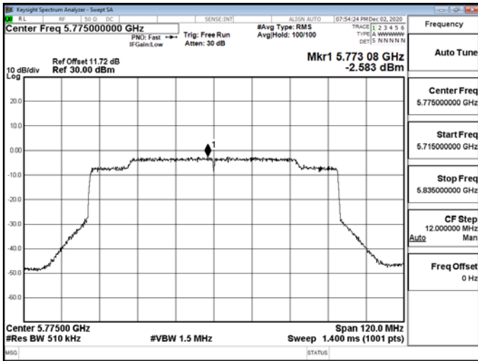
802.11ax_80MHz_RU_484_66_5775MHz-5775
