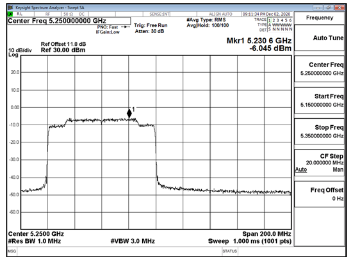
802.11ax_160MHz_RU_996_S67_5250MHz-5250
