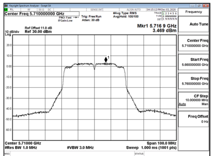
802.11n_40MHz_CH1_5710MHz_UNII 2C
