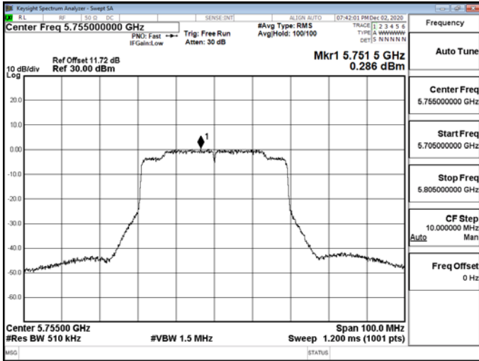
802.11ax_40MHz_RU_242_61_5755MHz-5755
