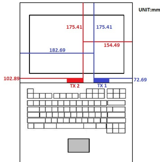
Fig.6 Antenna position of EUT
