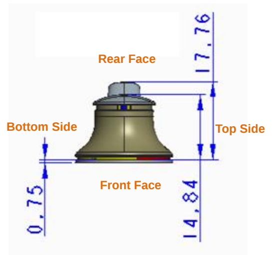
<EUT Left Side View>
