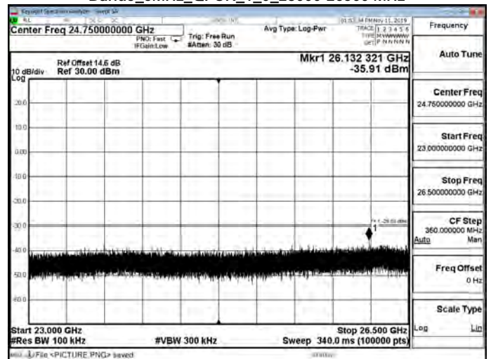
Band5_5MHz_QPSK_1_0_23000-26500 MHz
