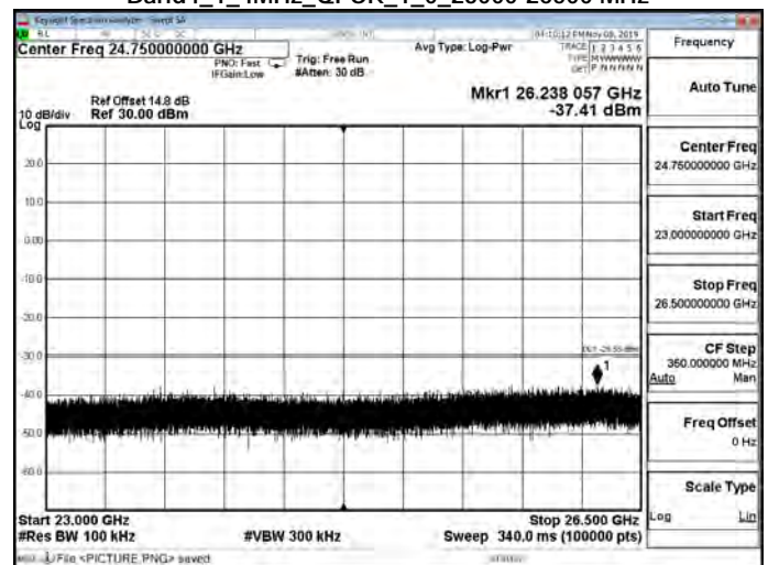
Band4_1_4MHz_QPSK_1_0_23000-26500 MHz
