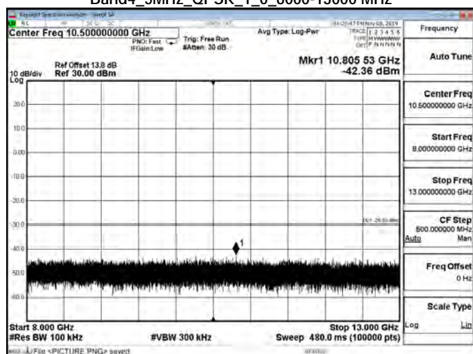
Band4_5MHz_QPSK_1_0_8000-13000 MHz
