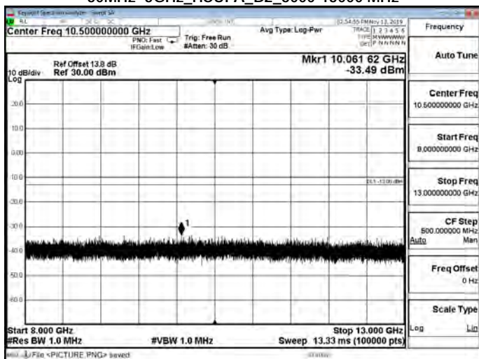
30MHz~3GHz_HSUPA_B2_8000-13000 MHz
