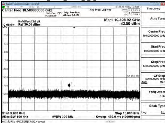
Band5_3MHz_QPSK_1_0_8000-13000 MHz
