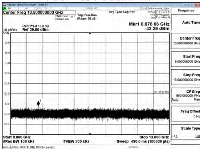
Band2_1_4MHz_QPSK_1_0_8000-13000 MHz
