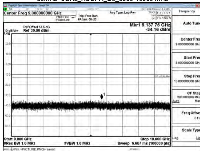
30MHz~3GHz_HSUPA_B5_8000-10000 MHz
