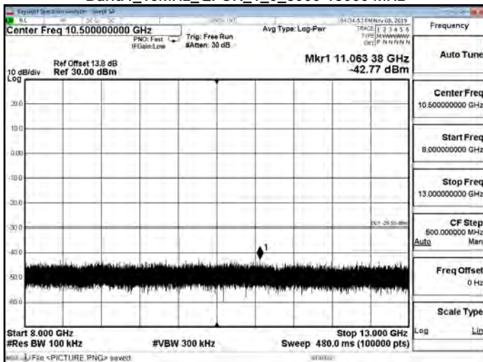
Band4_15MHz_QPSK_1_0_8000-13000 MHz
