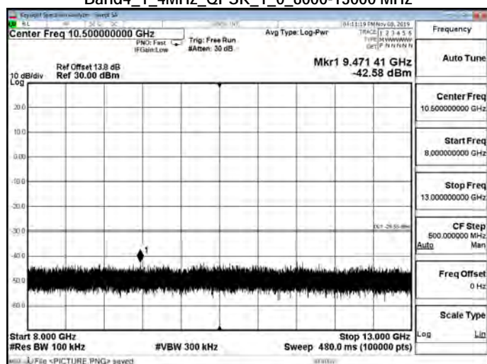
Band4_1_4MHz_QPSK_1_0_8000-13000 MHz
