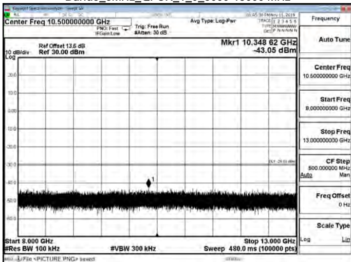
Band5_5MHz_QPSK_1_0_8000-13000 MHz
