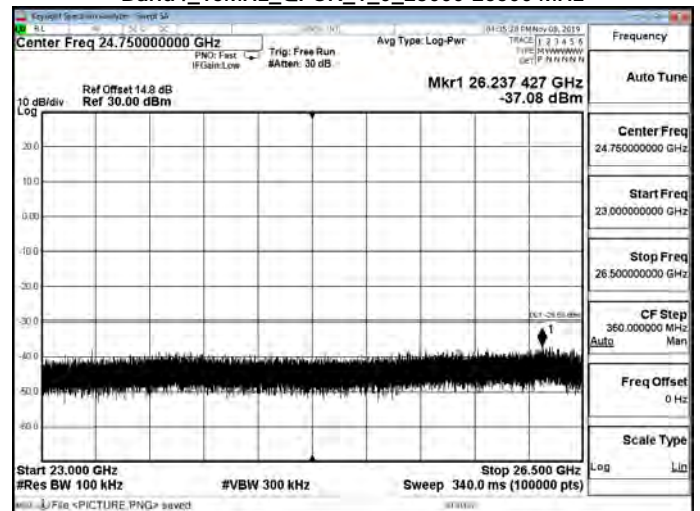
Band4_15MHz_QPSK_1_0_23000-26500 MHz
