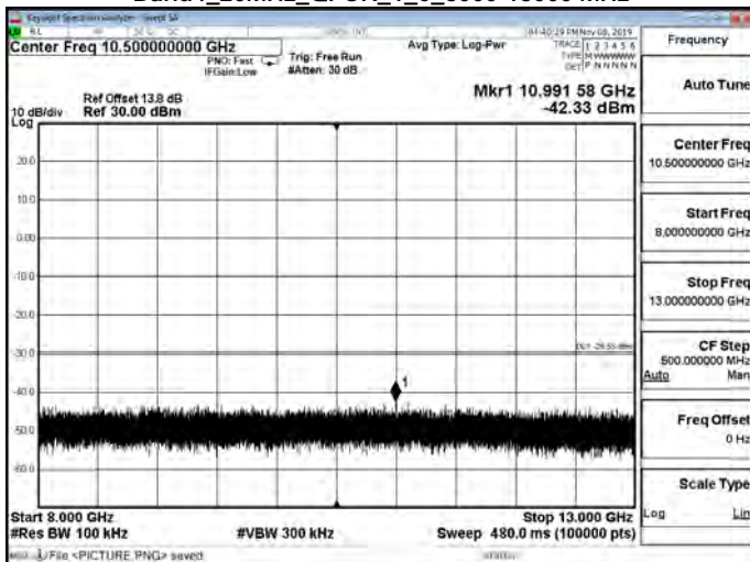
Band4_20MHz_QPSK_1_0_8000-13000 MHz
