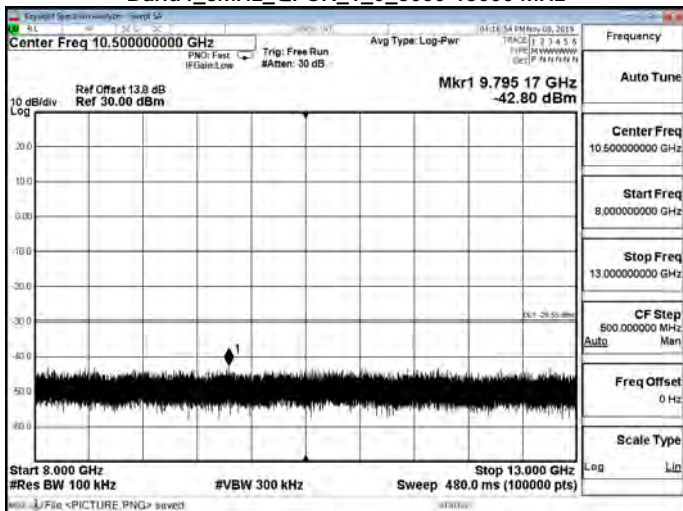
Band4_3MHz_QPSK_1_0_8000-13000 MHz
