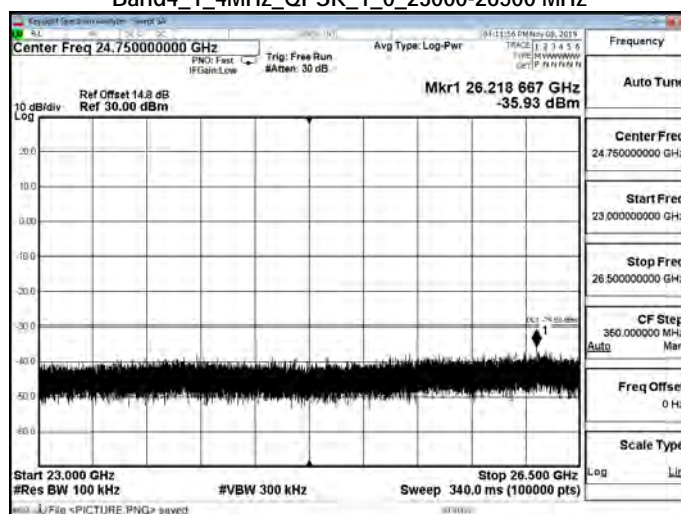
Band4_1_4MHz_QPSK_1_0_23000-26500 MHz
