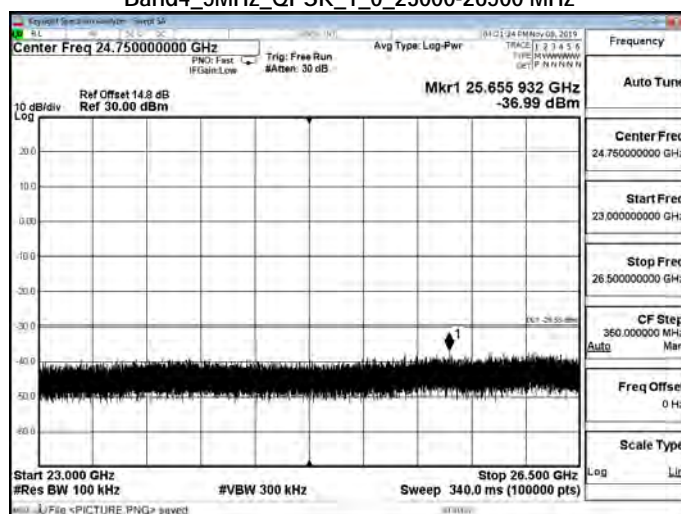
Band4_5MHz_QPSK_1_0_23000-26500 MHz
