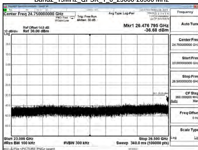
Band2_15MHz_QPSK_1_0_23000-26500 MHz
