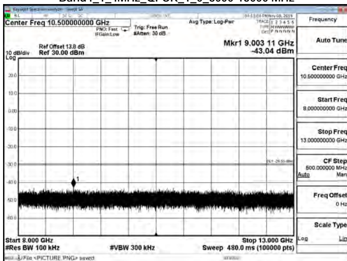
Band4_1_4MHz_QPSK_1_0_8000-13000 MHz
