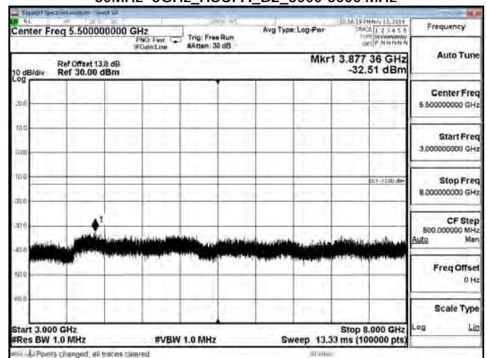
30MHz~3GHz_HSUPA_B2_3000-8000 MHz
