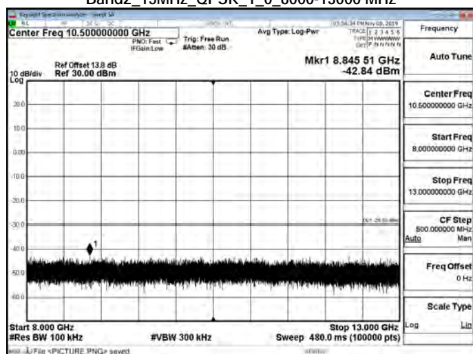
Band2_15MHz_QPSK_1_0_8000-13000 MHz
