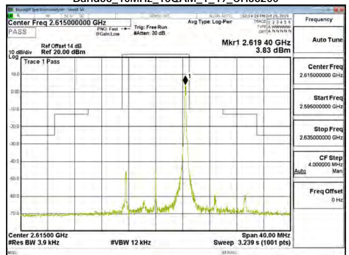
Band38_10MHz_16QAM_1_49_CH38200
