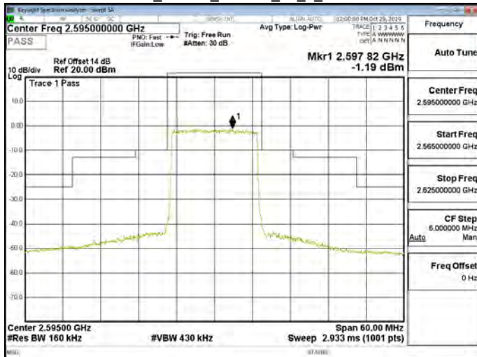
Band38_15MHz_16QAM_75_0_CH38000
