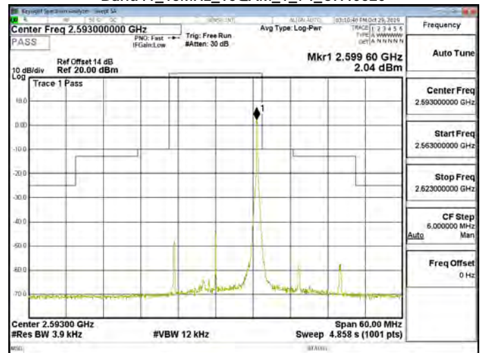
Band41_15MHz_16QAM_1_74_CH40620
