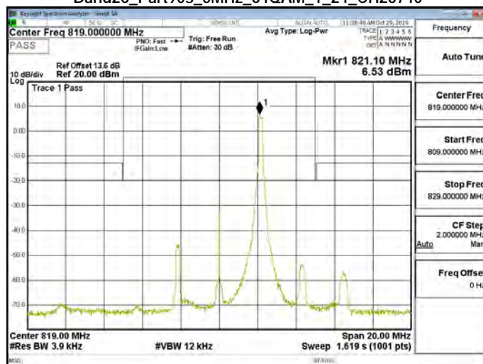
Band26_Part90s_5MHz_64QAM_1_24_CH26740
