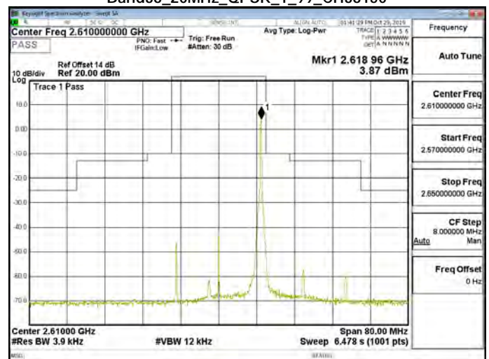
Band38_20MHz_QPSK_1_99_CH38150
