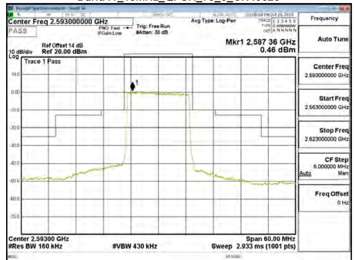
Band41_15MHz_QPSK_75_0_CH40620
