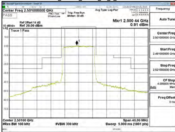
Band41_10MHz_QPSK_50_0_CH39700
