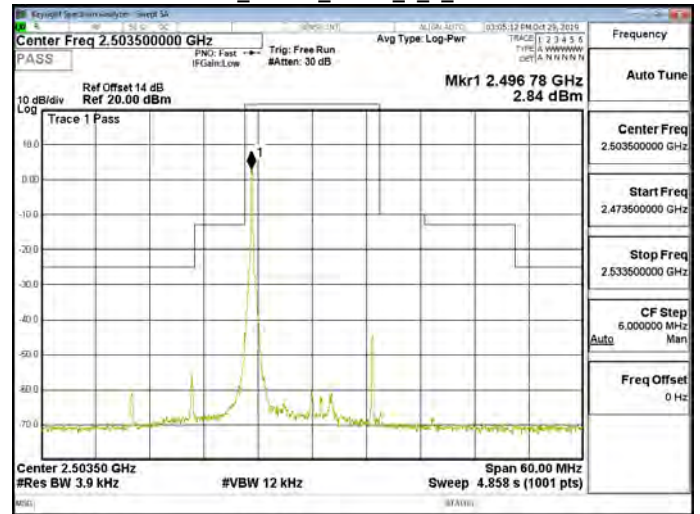
Band41_15MHz_QPSK_1_0_CH39725
