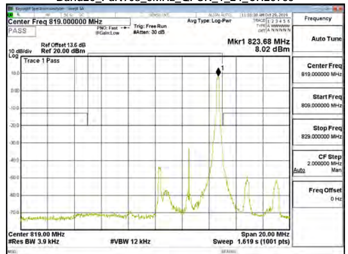
Band26_Part90s_5MHz_QPSK_1_24_CH26765
