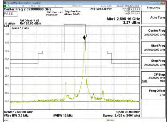
Band41_5MHz_16QAM_1_24_CH40620
