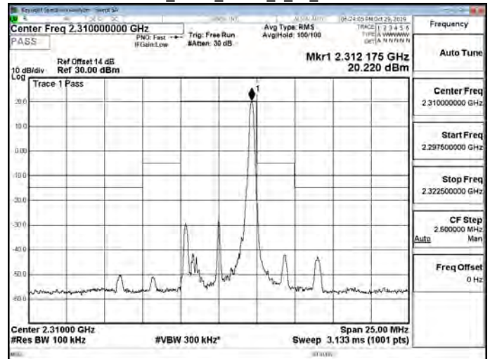
Band30_5MHz_QPSK_1_24_CH27710
