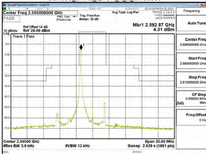
Band38_5MHz_QPSK_1_0_CH38000
