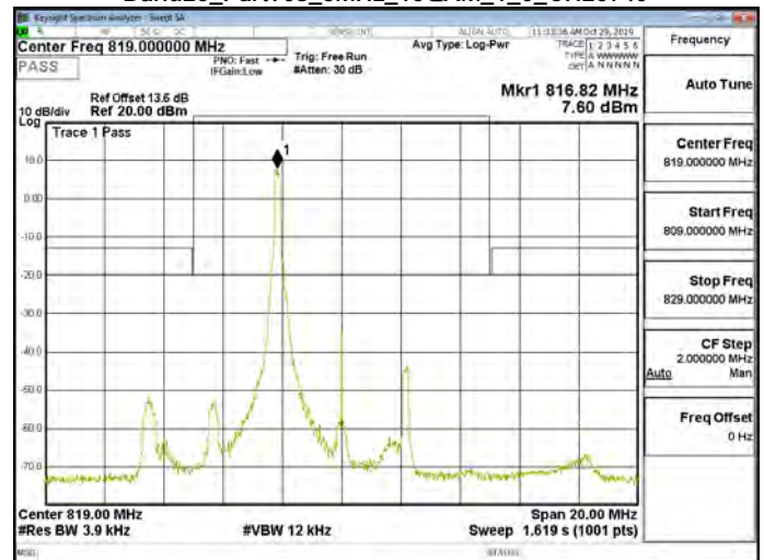
Band26_Part90s_5MHz_16QAM_1_0_CH26740
