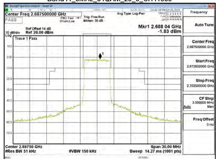
Band41_5MHz_64QAM_25_0_CH41565
