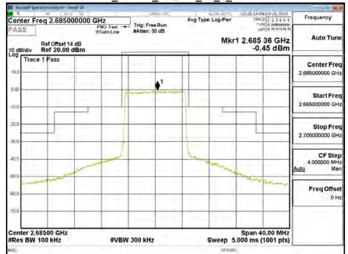
Band41_10MHz_16QAM_50_0_CH41540
