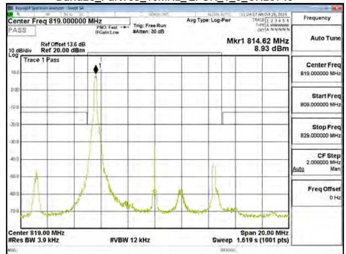
Band26_Part90s_10MHz_QPSK_1_0_CH26740
