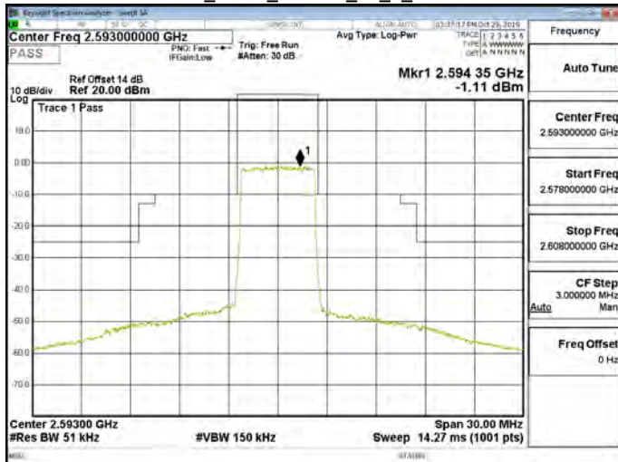
Band41_5MHz_16QAM_25_0_CH40620
