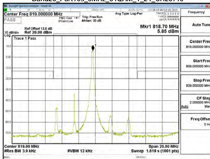
Band26_Part90s_5MHz_64QAM_1_24_CH26715
