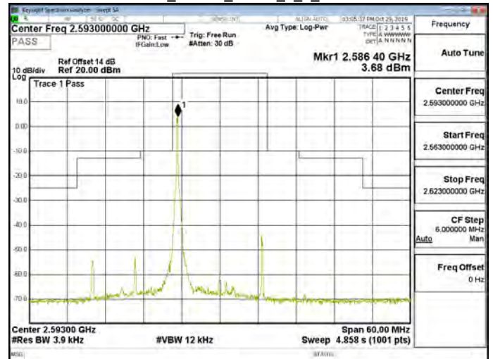
Band41_15MHz_QPSK_1_0_CH40620
