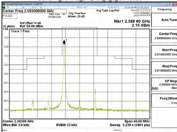
Band41_10MHz_64QAM_1_0_CH40620
