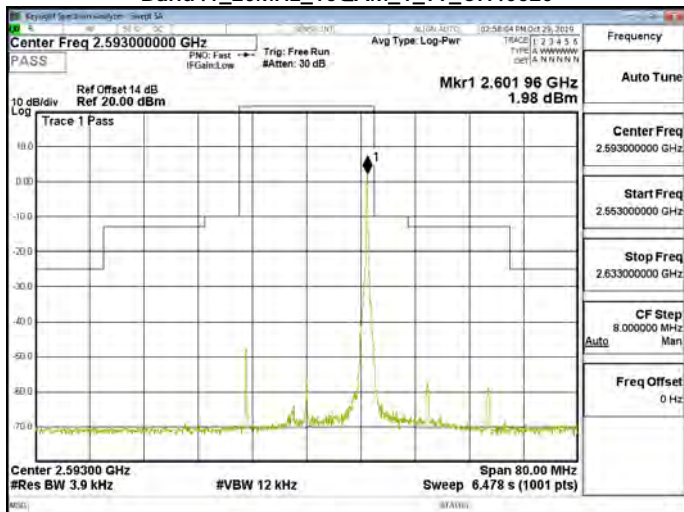
Band41_20MHz_16QAM_1_99_CH40620
