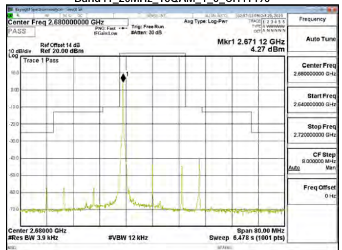
Band41_20MHz_16QAM_1_0_CH41490
