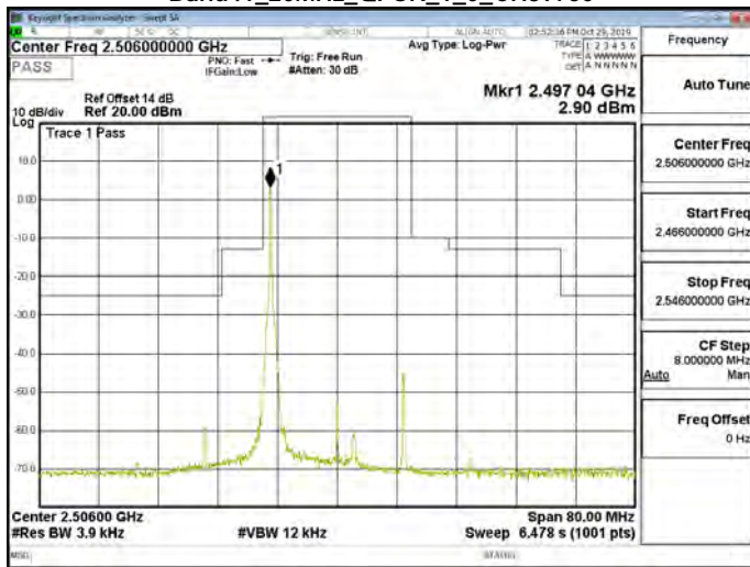
Band41_20MHz_QPSK_1_0_CH39750
