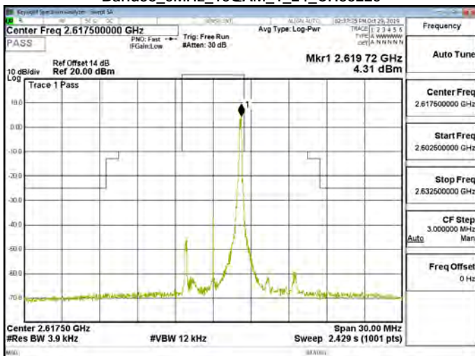
Band38_5MHz_16QAM_1_24_CH38225
