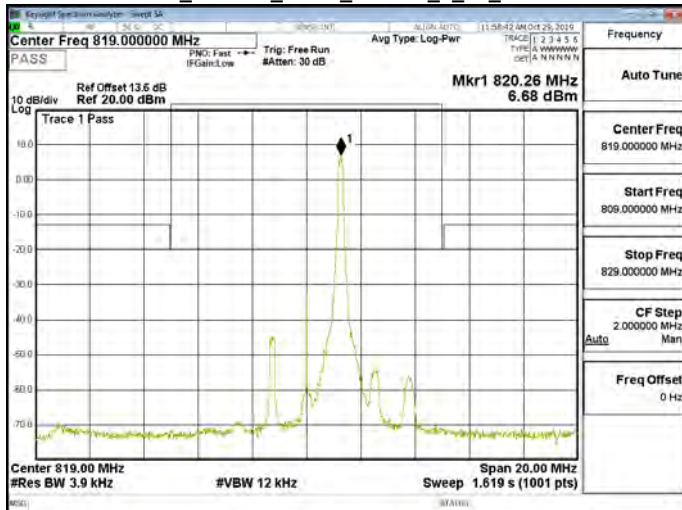
Band26_Part90s_3MHz_64QAM_1_14_CH26740
