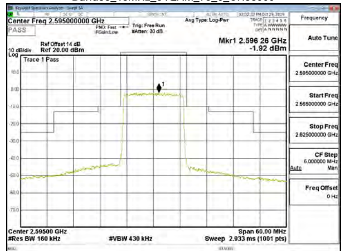
Band38_15MHz_64QAM_75_0_CH38000
