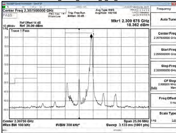
Band30_5MHz_16QAM_1_24_CH27685
