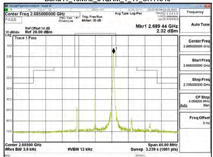
Band41_10MHz_64QAM_1_49_CH41540
