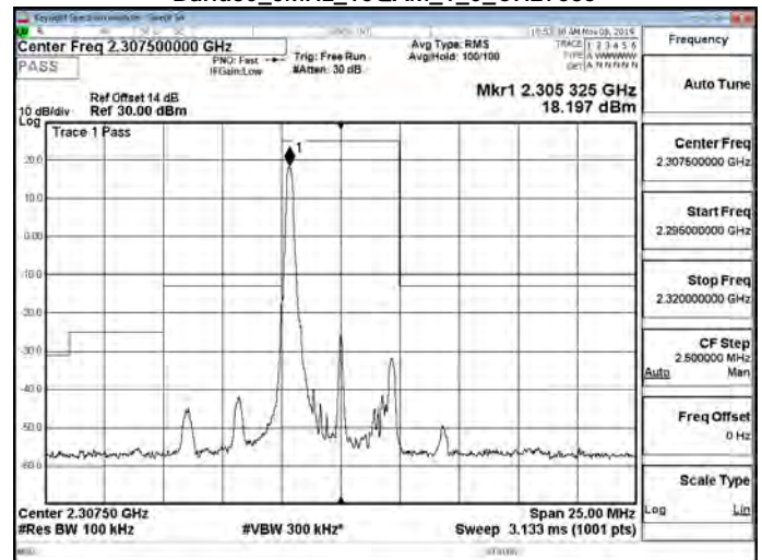
Band30_5MHz_16QAM_1_0_CH27685
