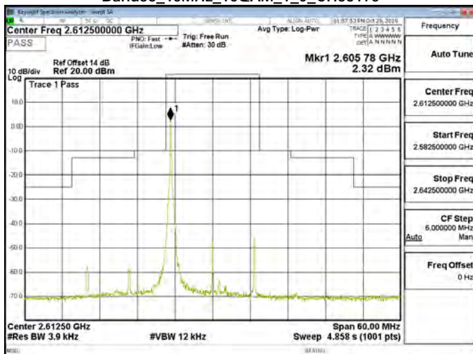
Band38_15MHz_16QAM_1_0_CH38175
