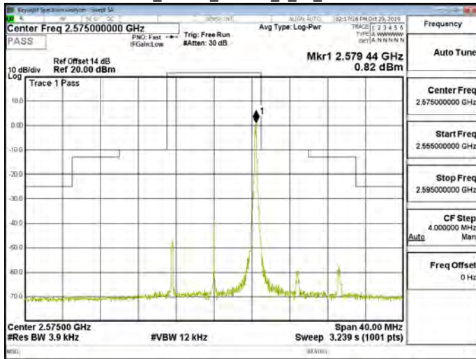
Band38_10MHz_64QAM_1_49_CH37800
