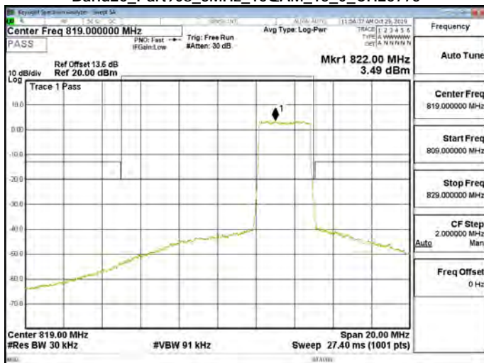
Band26_Part90s_3MHz_16QAM_15_0_CH26775
