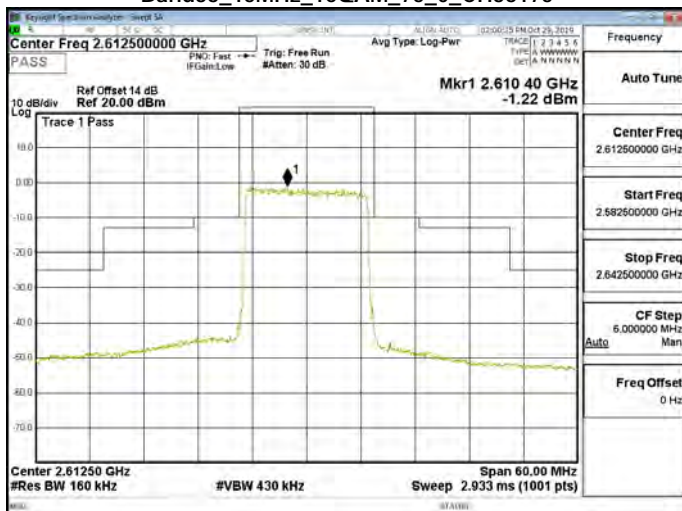
Band38_15MHz_16QAM_75_0_CH38175
