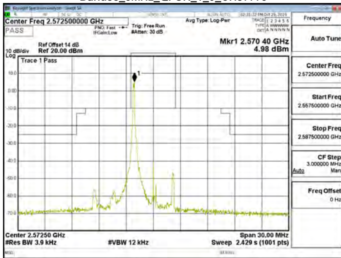
Band38_5MHz_QPSK_1_0_CH37775
