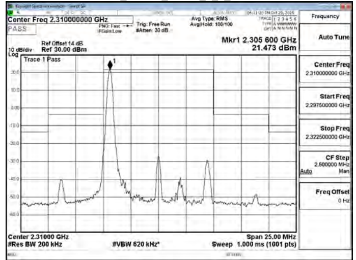
Band30_10MHz_QPSK_1_0_CH27710
