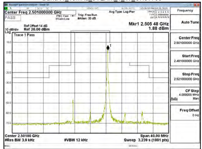
Band41_10MHz_64QAM_1_49_CH39700
