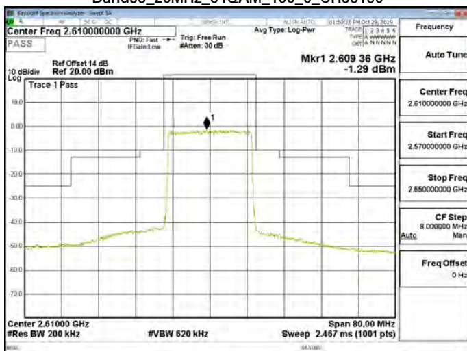
Band38_20MHz_64QAM_100_0_CH38150
