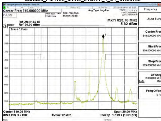
Band26_Part90s_5MHz_64QAM_1_24_CH26765
