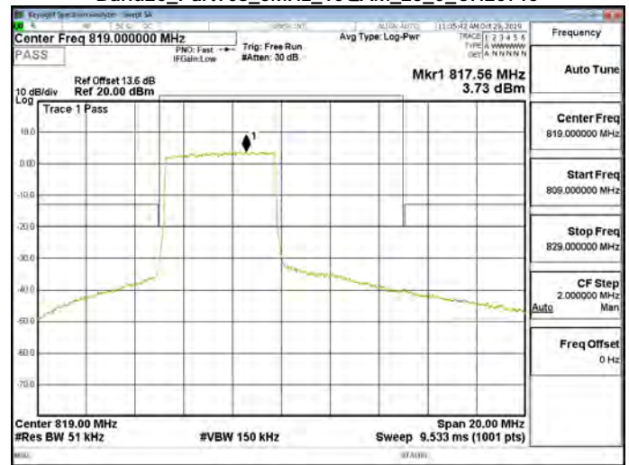
Band26_Part90s_5MHz_16QAM_25_0_CH26715
