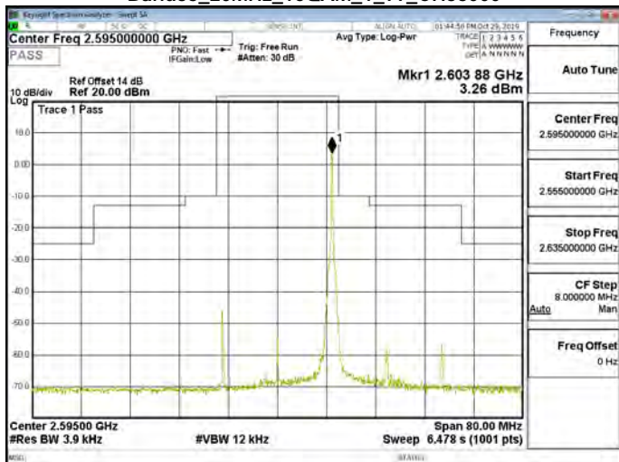
Band38_20MHz_16QAM_1_99_CH38000
