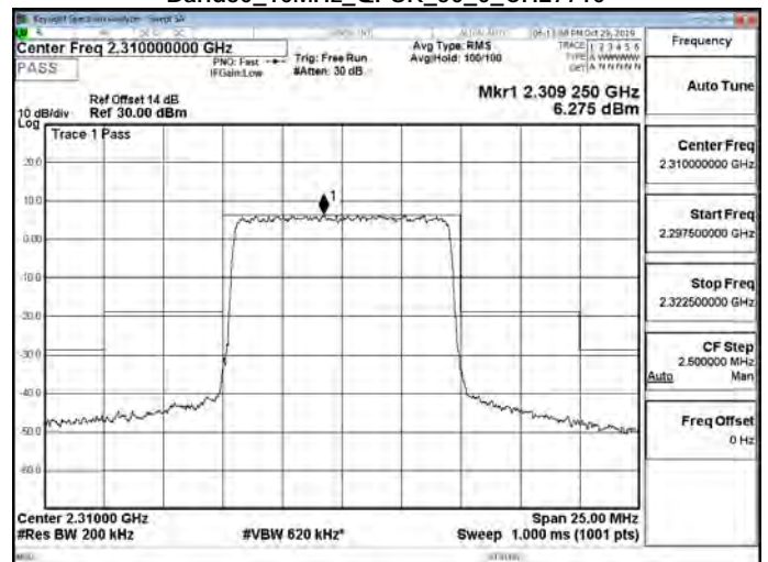
Band30_10MHz_QPSK_50_0_CH27710
