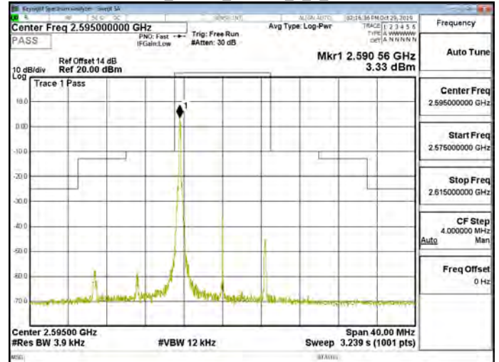
Band38_10MHz_64QAM_1_0_CH38000
