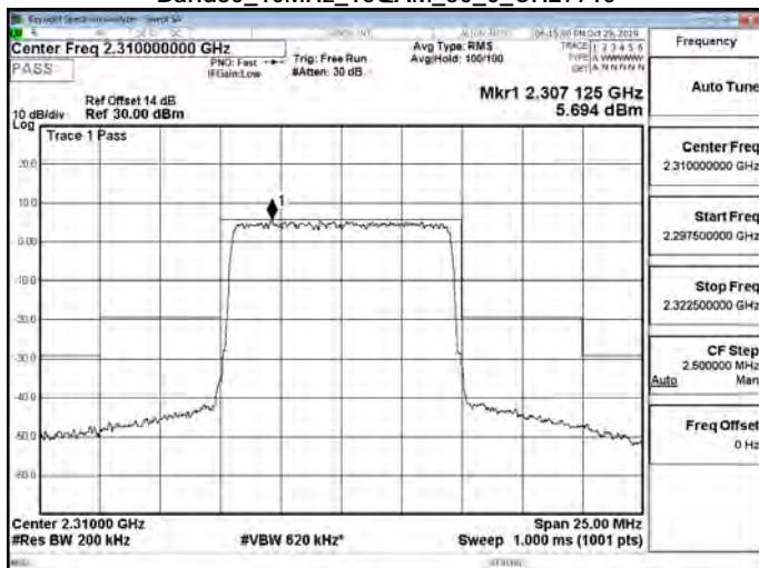
Band30_10MHz_16QAM_50_0_CH27710
