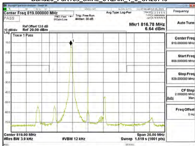
Band26_Part90s_5MHz_64QAM_1_0_CH26740
