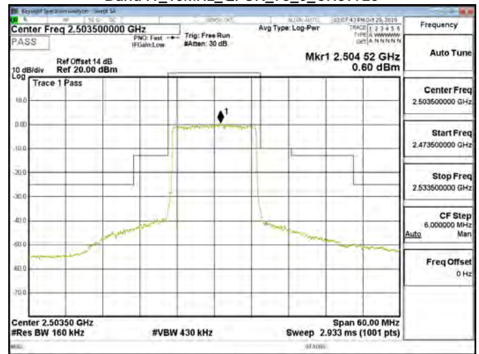
Band41_15MHz_QPSK_75_0_CH39725
