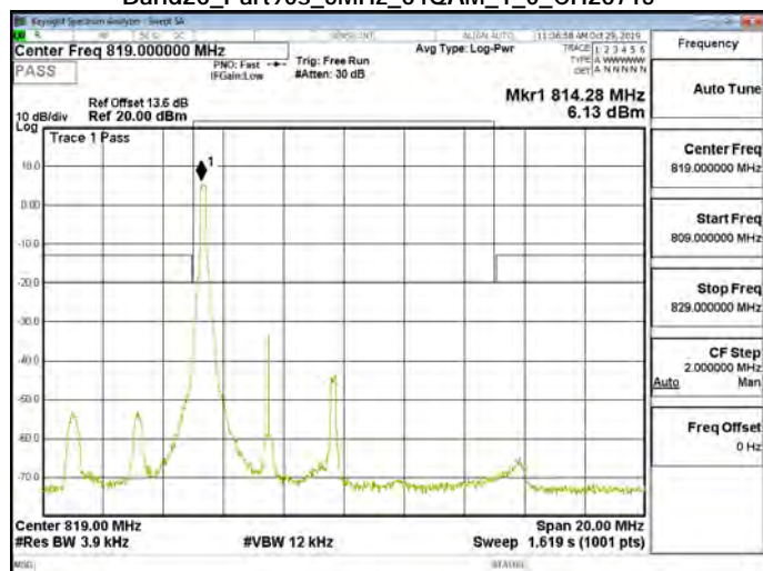
Band26_Part90s_5MHz_64QAM_1_0_CH26715
