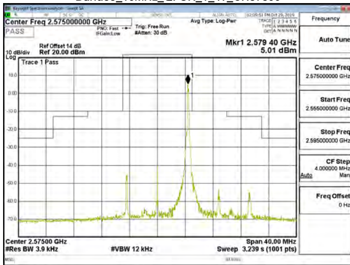
Band38_10MHz_QPSK_1_49_CH37800
