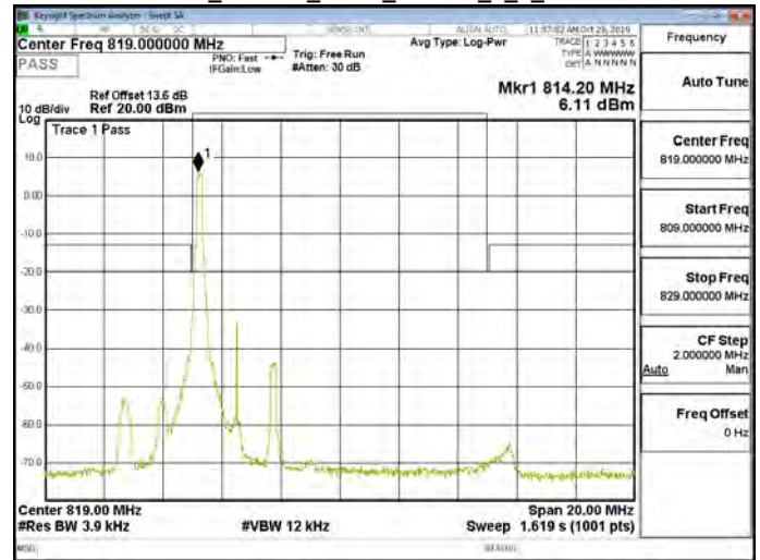
Band26_Part90s_3MHz_64QAM_1_0_CH26705
