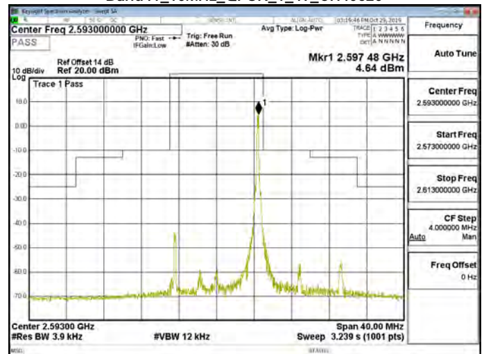
Band41_10MHz_QPSK_1_49_CH40620
