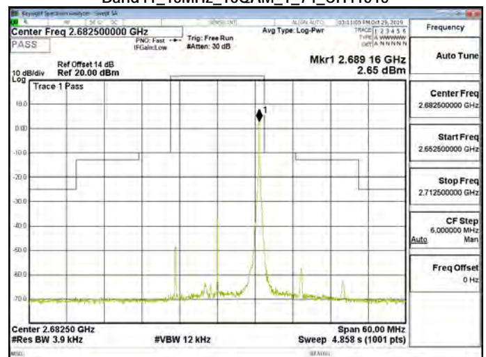
Band41_15MHz_16QAM_1_74_CH41515
