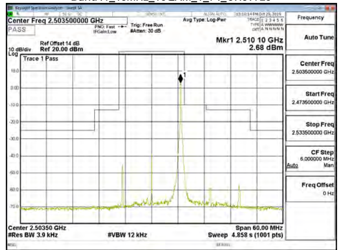
Band41_15MHz_16QAM_1_74_CH39725
