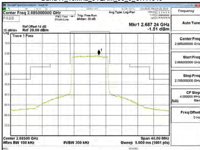
Band41_10MHz_64QAM_50_0_CH41540
