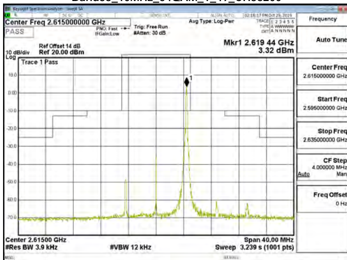
Band38_10MHz_64QAM_1_49_CH38200
