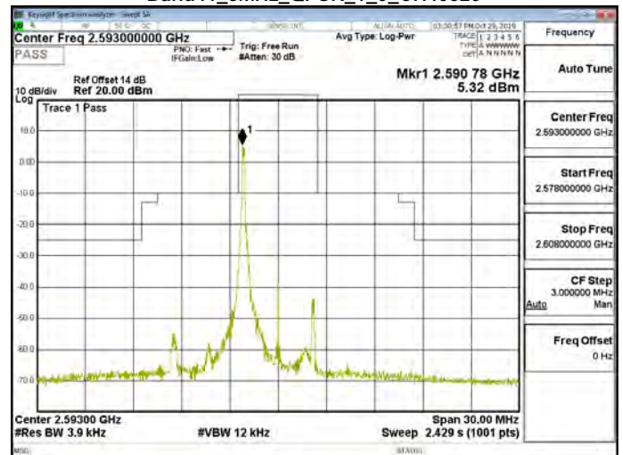
Band41_5MHz_QPSK_1_0_CH40620
