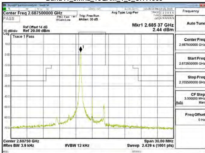
Band41_5MHz_16QAM_1_0_CH41565
