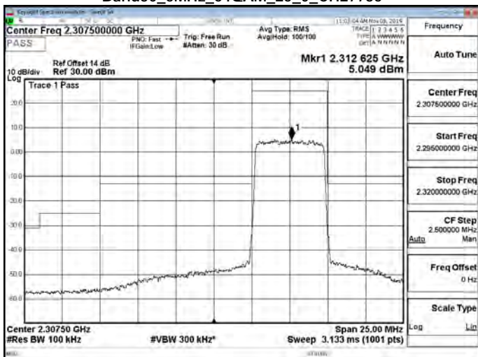
Band30_5MHz_64QAM_25_0_CH27735
