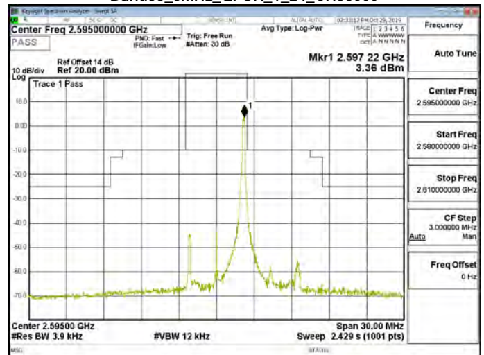
Band38_5MHz_QPSK_1_24_CH38000
