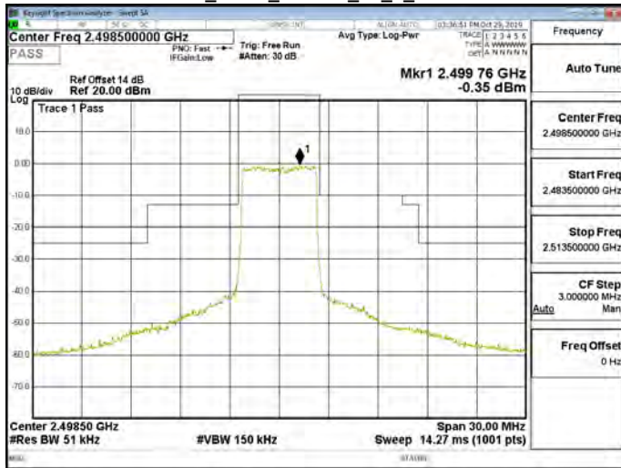
Band41_5MHz_16QAM_25_0_CH39675
