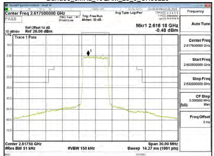
Band38_5MHz_16QAM_25_0_CH38225
