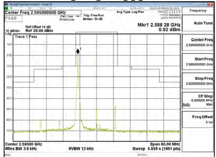
Band38_15MHz_64QAM_1_0_CH38000
