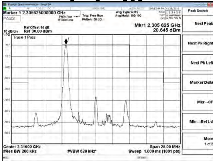
Band30_10MHz_16QAM_1_0_CH27710
