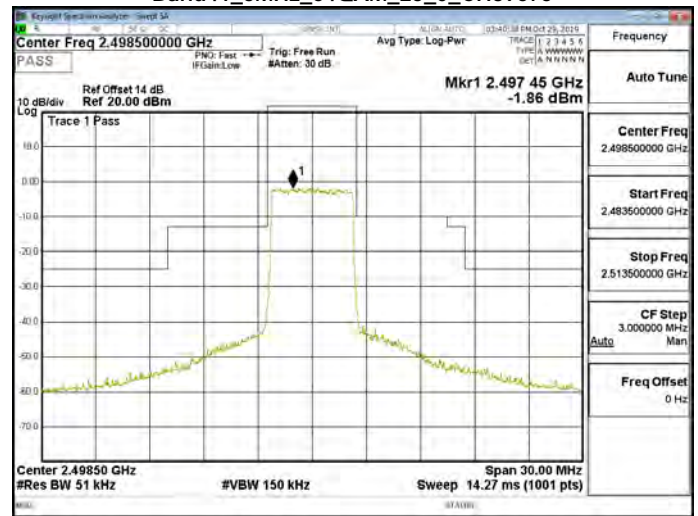
Band41_5MHz_64QAM_25_0_CH39675
