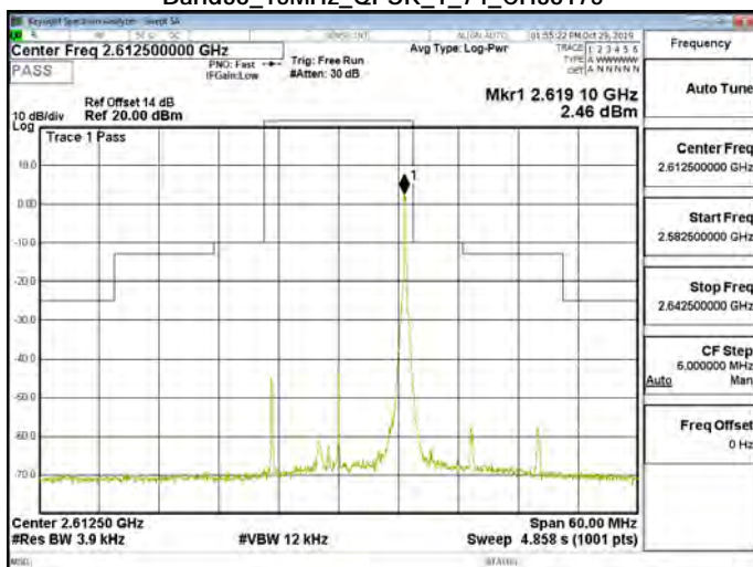
Band38_15MHz_QPSK_1_74_CH38175
