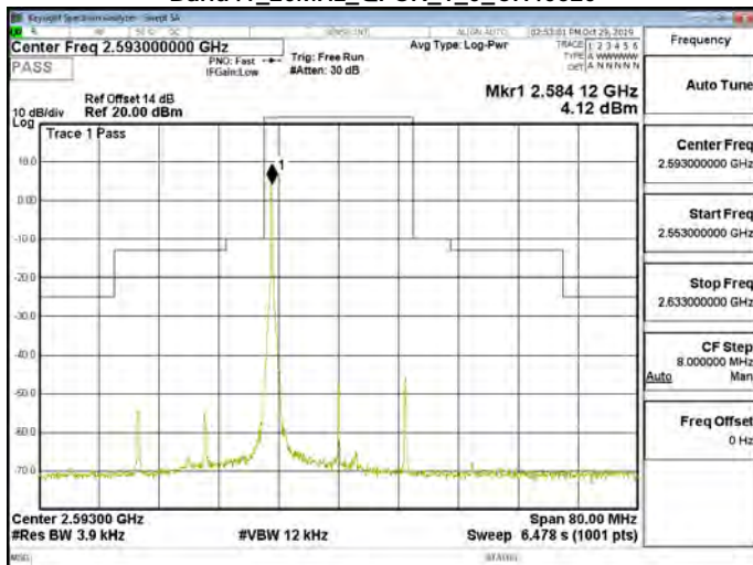
Band41_20MHz_QPSK_1_0_CH40620
