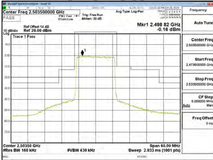
Band41_15MHz_16QAM_75_0_CH39725
