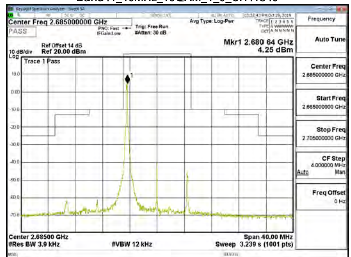
Band41_10MHz_16QAM_1_0_CH41540
