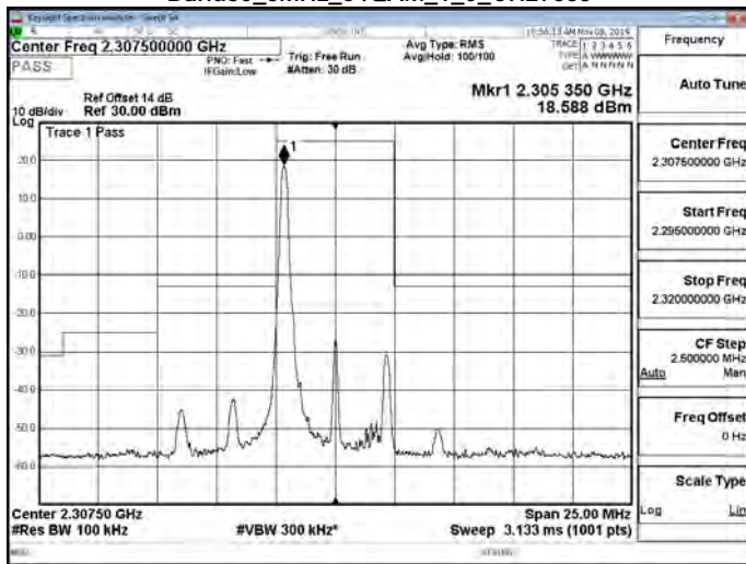
Band30_5MHz_64QAM_1_0_CH27685
