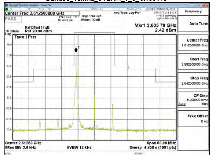
Band38_15MHz_64QAM_1_0_CH38175
