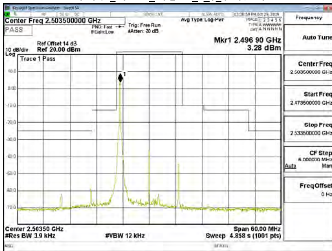
Band41_15MHz_16QAM_1_0_CH39725
