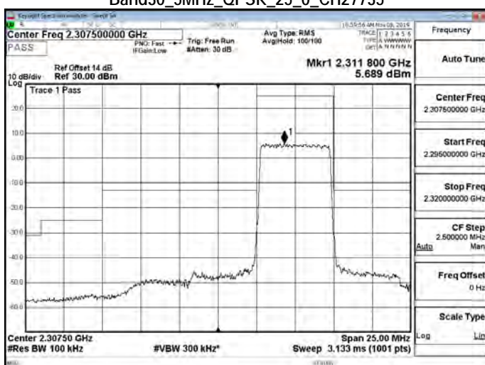
Band30_5MHz_QPSK_25_0_CH27735
