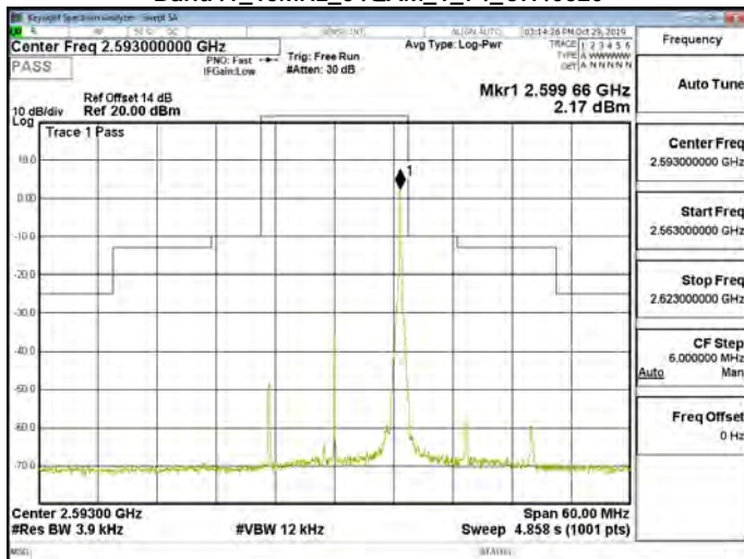
Band41_15MHz_64QAM_1_74_CH40620
