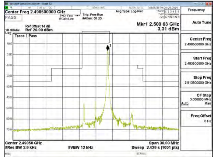
Band41_5MHz_16QAM_1_24_CH39675
