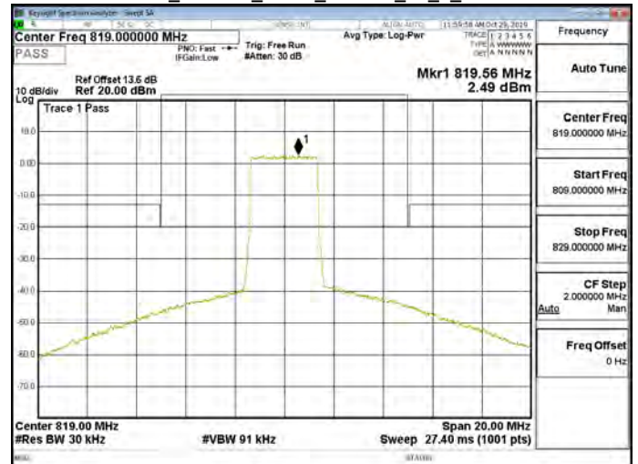
Band26_Part90s_3MHz_64QAM_15_0_CH26740
