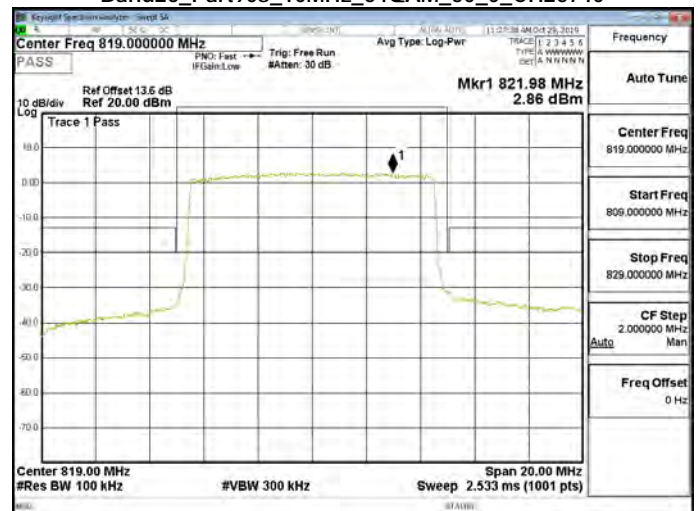
Band26_Part90s_10MHz_64QAM_50_0_CH26740
