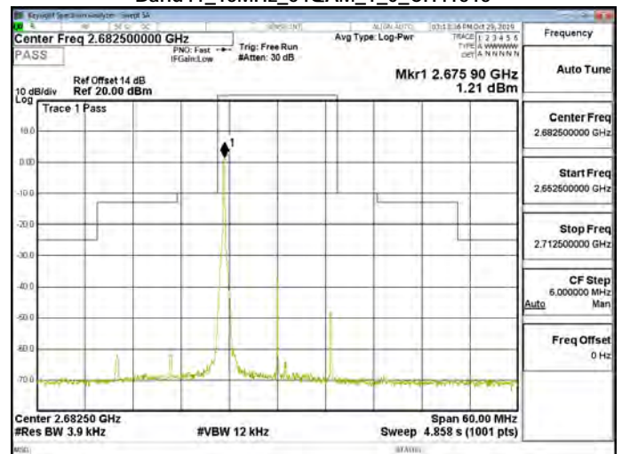
Band41_15MHz_64QAM_1_0_CH41515
