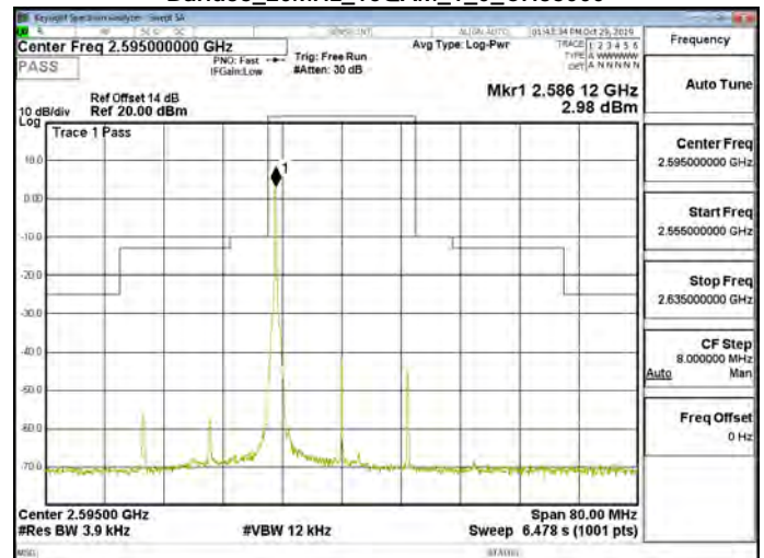
Band38_20MHz_16QAM_1_0_CH38000
