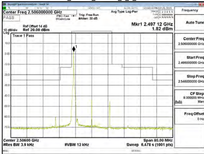
Band41_20MHz_64QAM_1_0_CH39750
