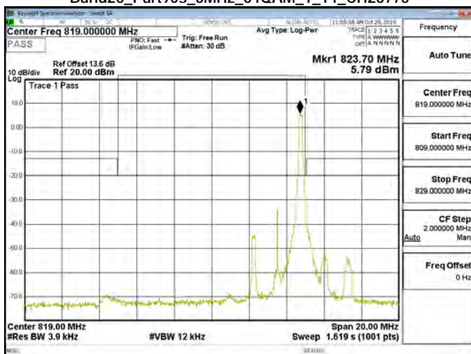
Band26_Part90s_3MHz_64QAM_1_14_CH26775
