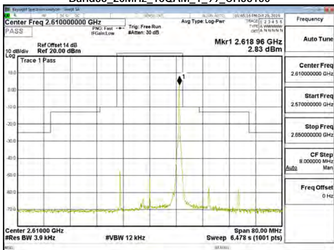
Band38_20MHz_16QAM_1_99_CH38150
