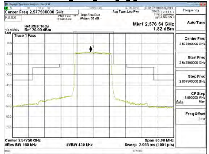
Band38_15MHz_QPSK_75_0_CH37825
