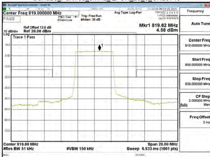
Band26_Part90s_5MHz_QPSK_25_0_CH26740
