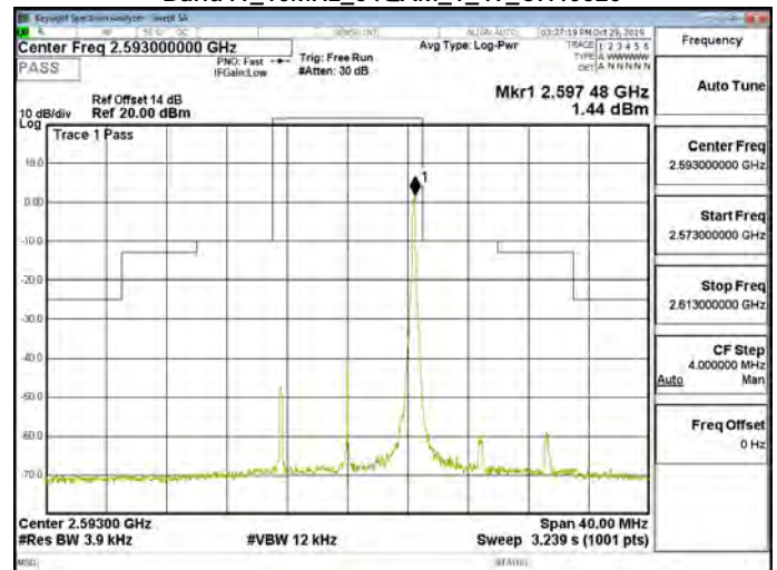
Band41_10MHz_64QAM_1_49_CH40620
