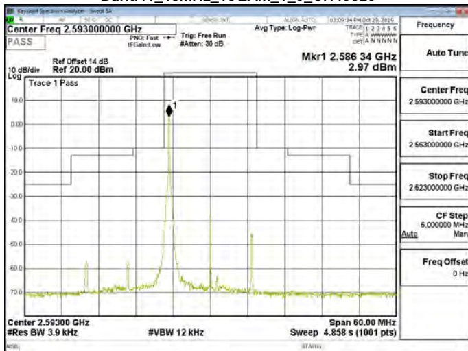
Band41_15MHz_16QAM_1_0_CH40620
