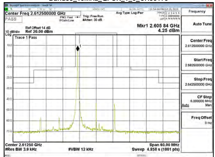
Band38_15MHz_QPSK_1_0_CH38175
