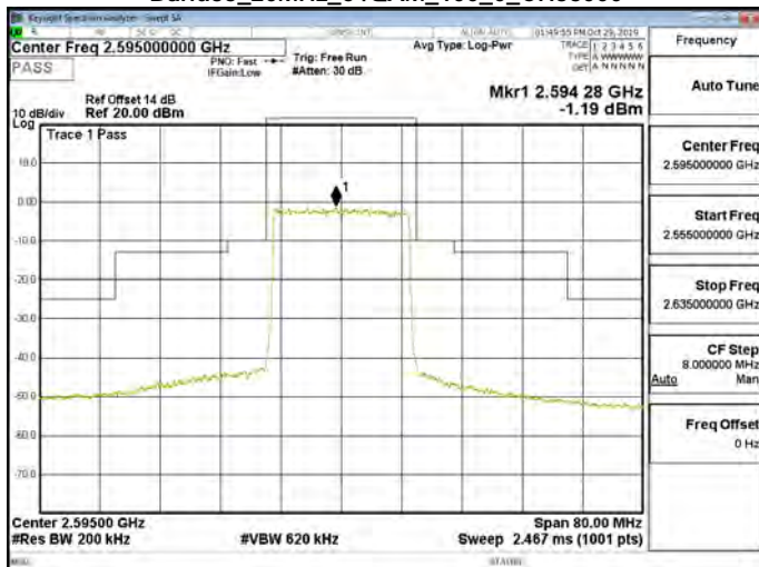
Band38_20MHz_64QAM_100_0_CH38000
