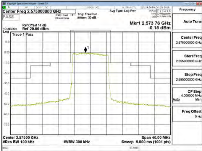
Band38_10MHz_16QAM_50_0_CH37800
