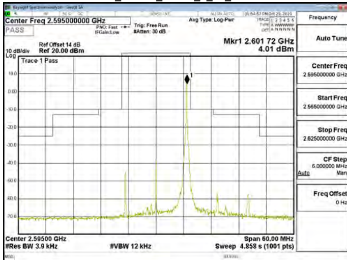
Band38_15MHz_QPSK_1_74_CH38000
