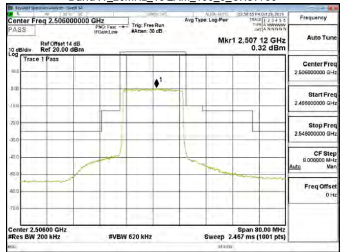
Band41_20MHz_16QAM_100_0_CH39750
