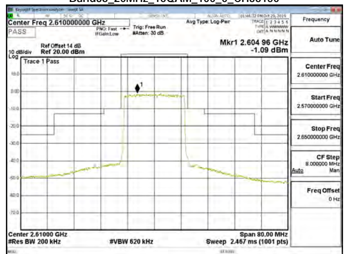
Band38_20MHz_16QAM_100_0_CH38150
