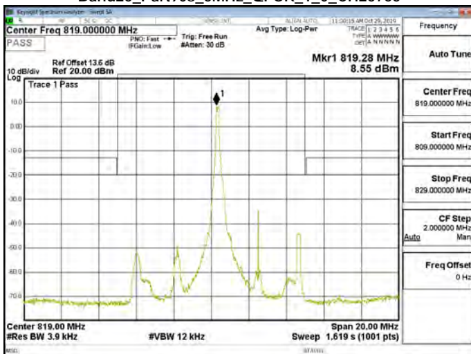
Band26_Part90s_5MHz_QPSK_1_0_CH26765
