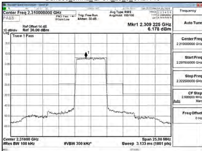
Band30_5MHz_QPSK_25_0_CH27710
