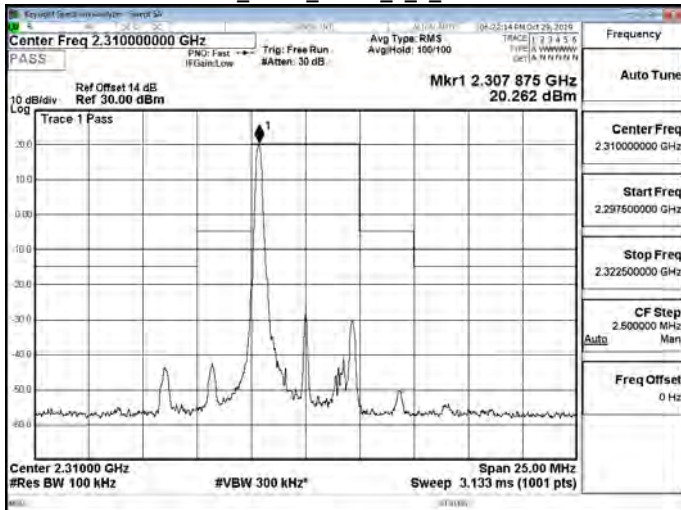
Band30_5MHz_QPSK_1_0_CH27710
