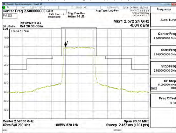
Band38_20MHz_QPSK_100_0_CH37850
