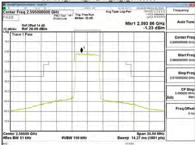
Band38_5MHz_64QAM_25_0_CH38000
