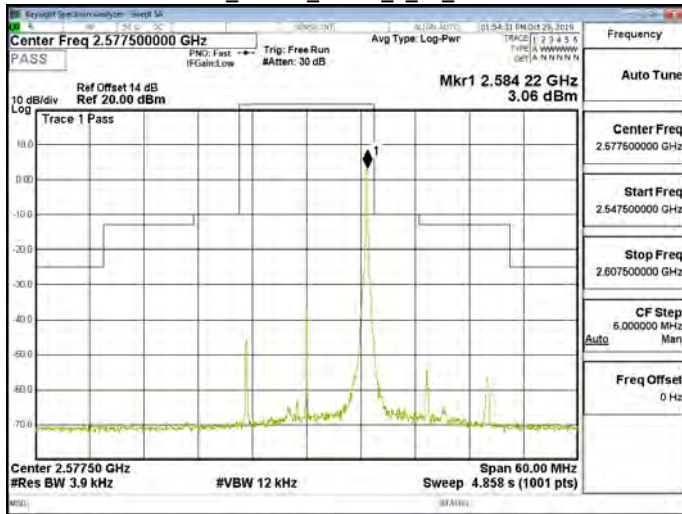
Band38_15MHz_QPSK_1_74_CH37825
