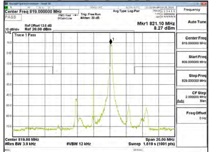
Band26_Part90s_5MHz_QPSK_1_24_CH26740
