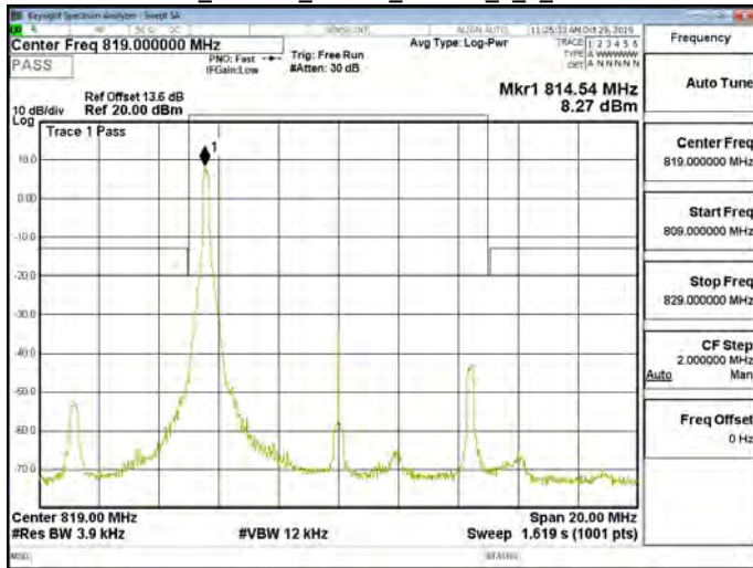
Band26_Part90s_10MHz_16QAM_1_0_CH26740
