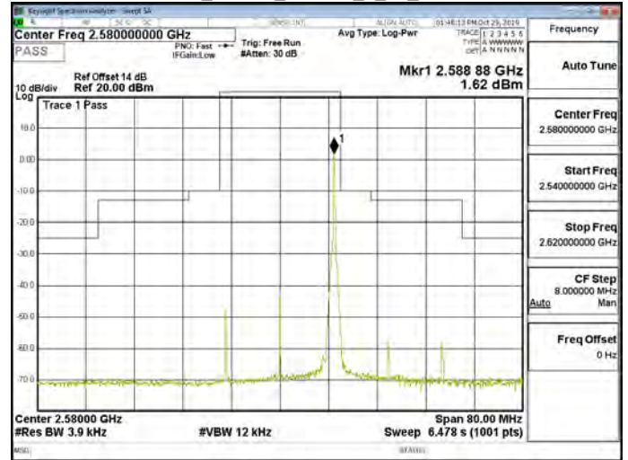
Band38_20MHz_64QAM_1_99_CH37850
