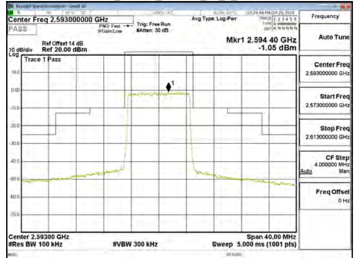
Band41_10MHz_16QAM_50_0_CH40620
