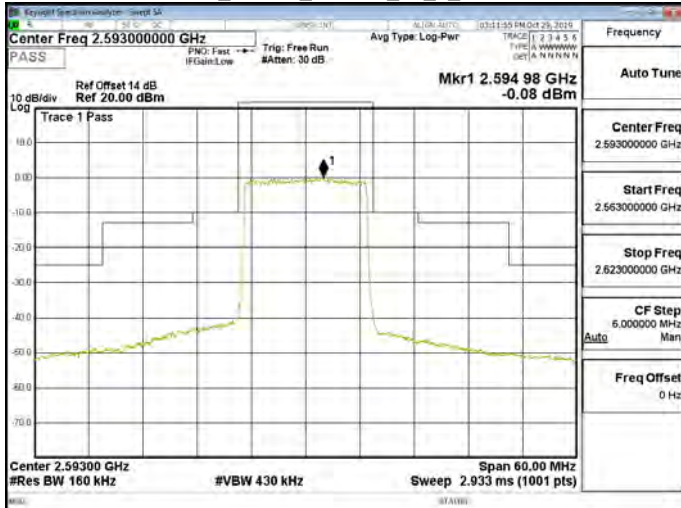
Band41_15MHz_16QAM_75_0_CH40620
