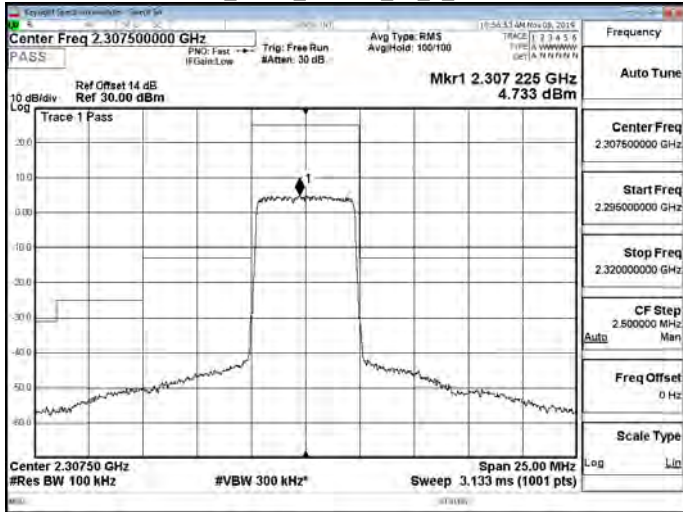
Band30_5MHz_64QAM_25_0_CH27685
