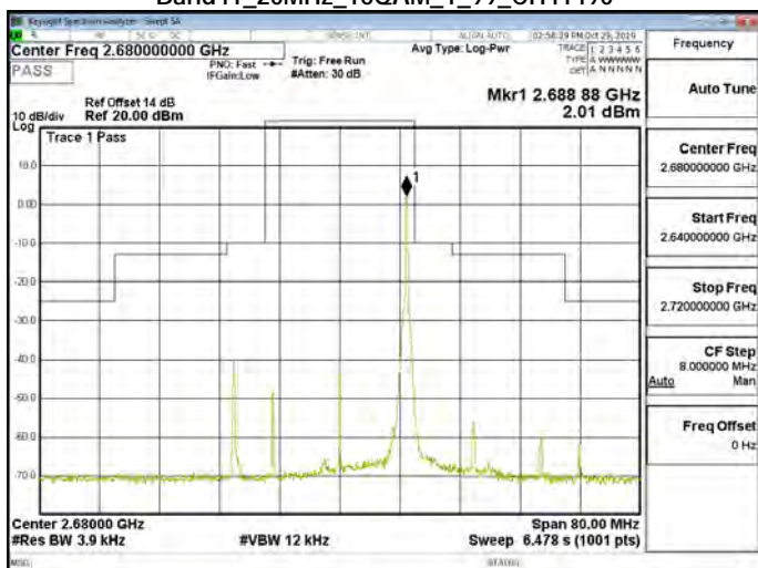
Band41_20MHz_16QAM_1_99_CH41490
