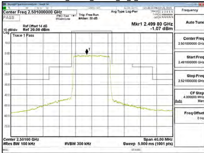
Band41_10MHz_64QAM_50_0_CH39700
