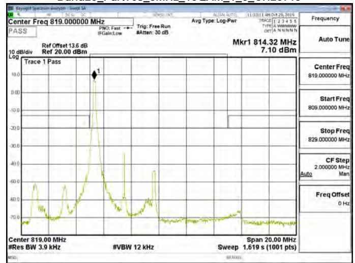
Band26_Part90s_5MHz_16QAM_1_0_CH26715
