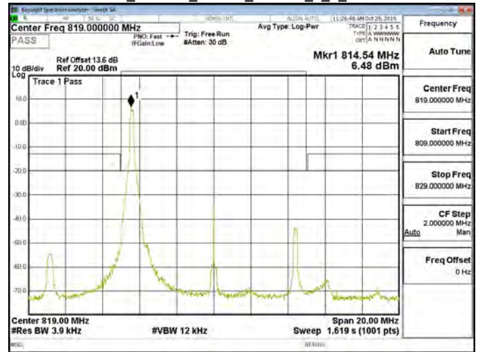
Band26_Part90s_10MHz_64QAM_1_0_CH26740
