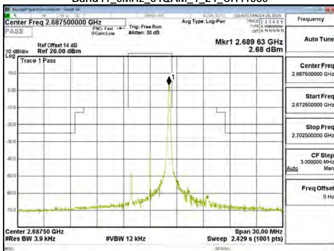
Band41_5MHz_64QAM_1_24_CH41565
