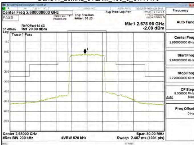
Band41_20MHz_64QAM_100_0_CH41490
