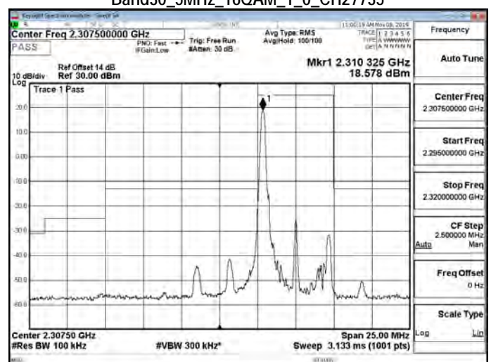
Band30_5MHz_16QAM_1_0_CH27735
