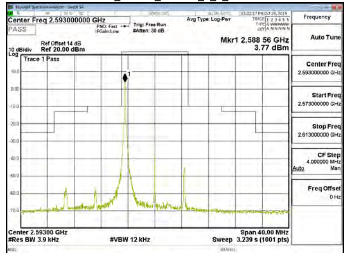
Band41_10MHz_16QAM_1_0_CH40620
