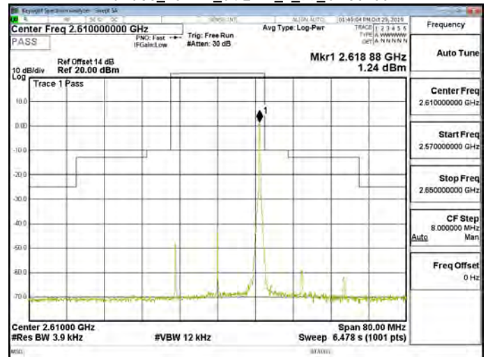
Band38_20MHz_64QAM_1_99_CH38150
