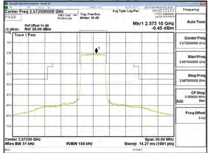
Band38_5MHz_16QAM_25_0_CH37775
