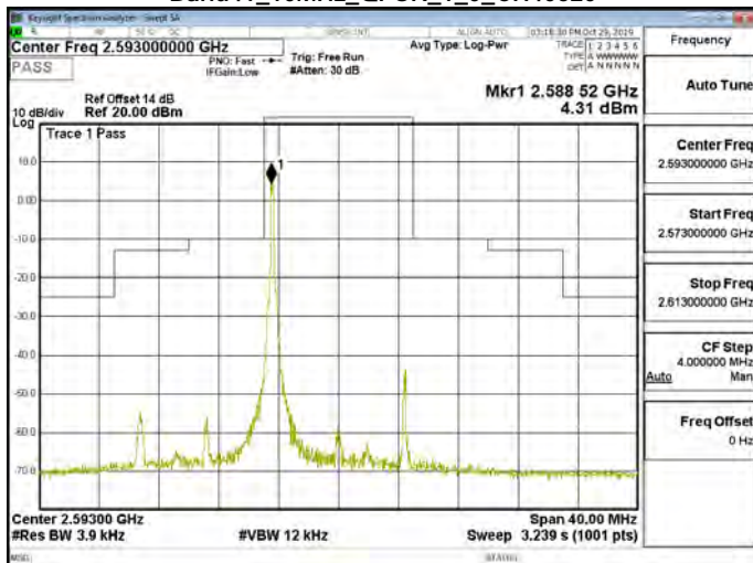
Band41_10MHz_QPSK_1_0_CH40620
