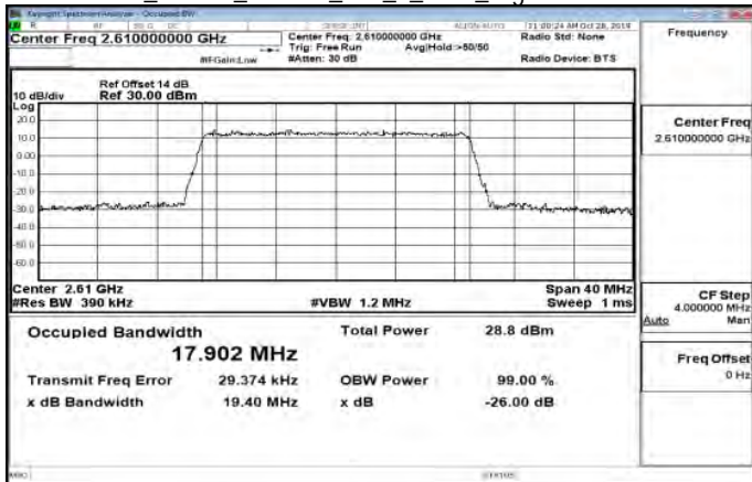
Band38_20MHz_64QAM_100_0_Main_HighCH38150-2610
