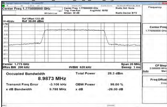
Band66_10MHz_64QAM_50_0_Main_HighCH132622-1775
