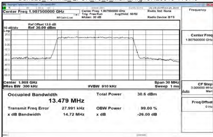
Band25_15MHz_QPSK_75_0_Main_HighCH26615-1907.5
