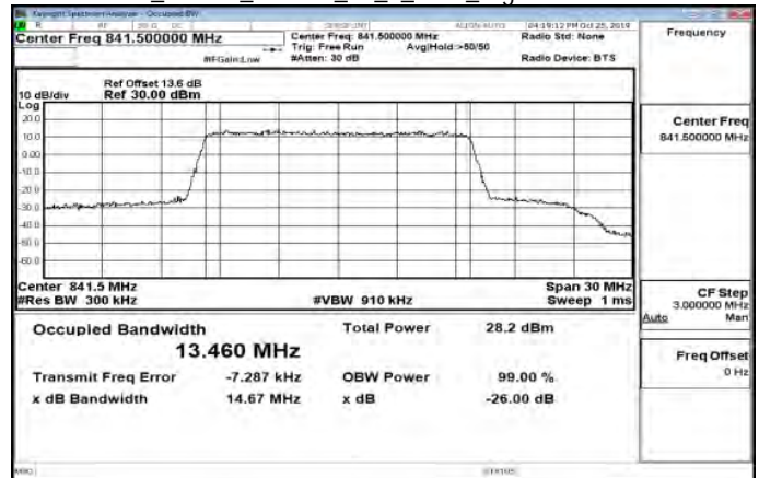
Band26_15MHz_16QAM_75_0_Main_HighCH26965-841.5
