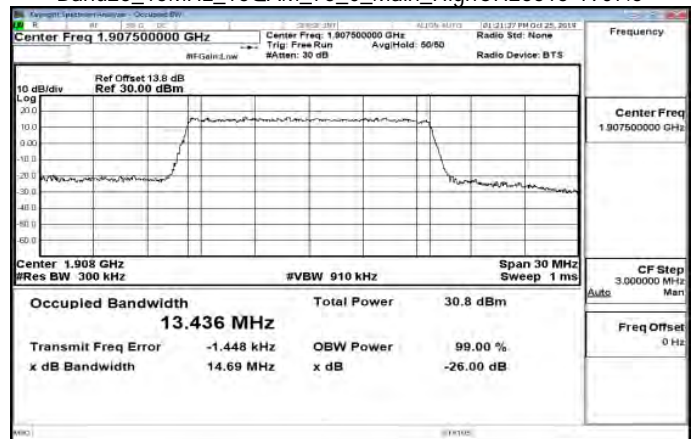
Band25_15MHz_16QAM_75_0_Main_HighCH26615-1907.5
