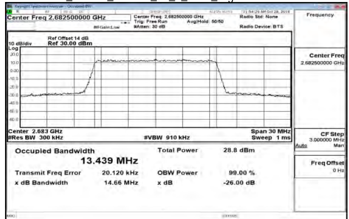
Band41_15MHz_64QAM_75_0_Main_HighCH41515-2682.5
