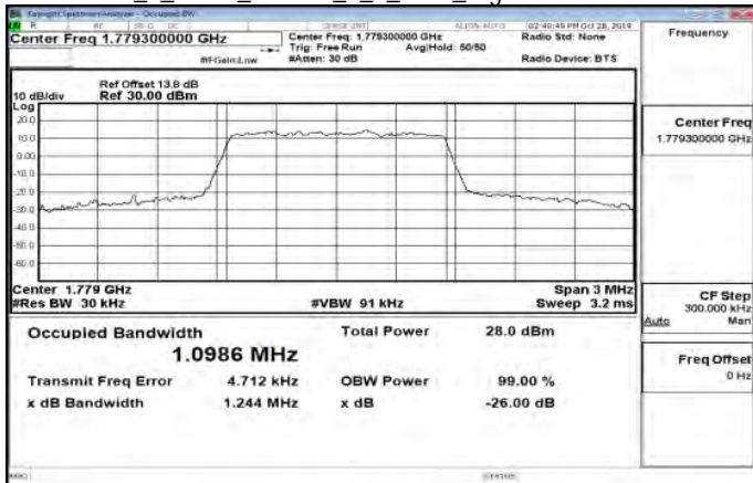
Band66_1_4MHz_16QAM_6_0_Main_HighCH132665-1779.3
