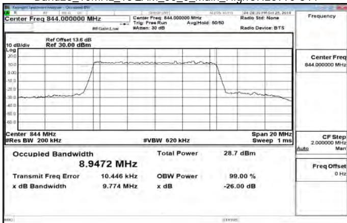
Band26_10MHz_16QAM_50_0_Main_HighCH26990-844
