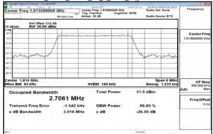
Band25_3MHz_QPSK_15_0_Main_HighCH26675-1913.5
