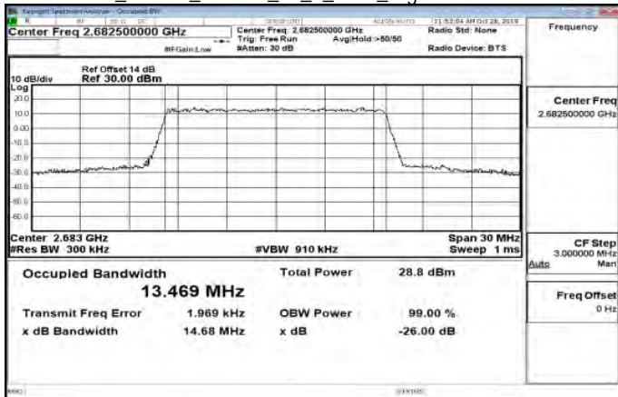
Band41_15MHz_16QAM_75_0_Main_HighCH41515-2682.5
