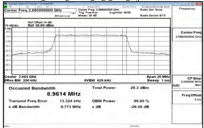
Band41_10MHz_16QAM_50_0_Main_HighCH41540-2685
