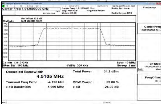
Band25_5MHz_64QAM_25_0_Main_HighCH26665-1912.5
