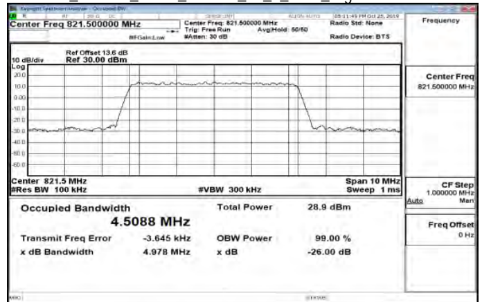
Band26_Part90s_5MHz_64QAM_25_0_Main_HighCH26765-821.5
