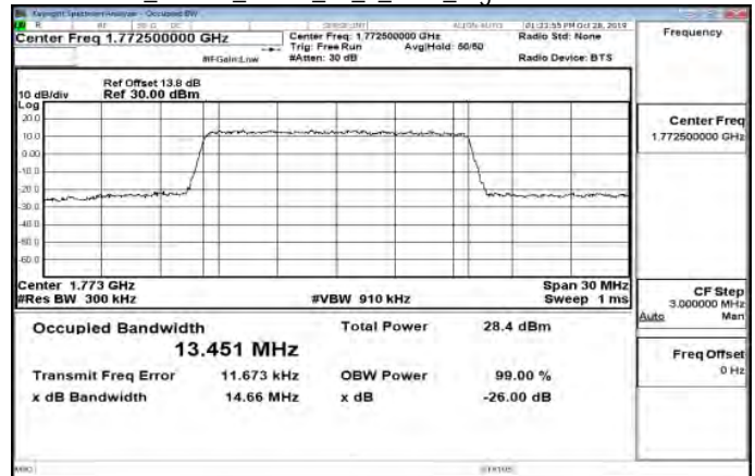
Band66_15MHz_QPSK_75_0_Main_HighCH132597-1772.5
