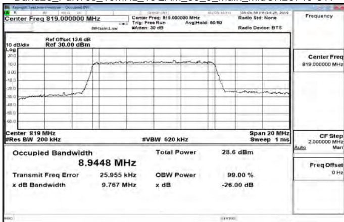
Band26_Part90s_10MHz_64QAM_50_0_Main_MidCH26740-819
