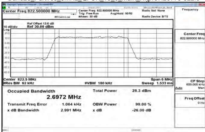
Band26_Part90s_3MHz_QPSK_15_0_Main_HighCH26775-822.5
