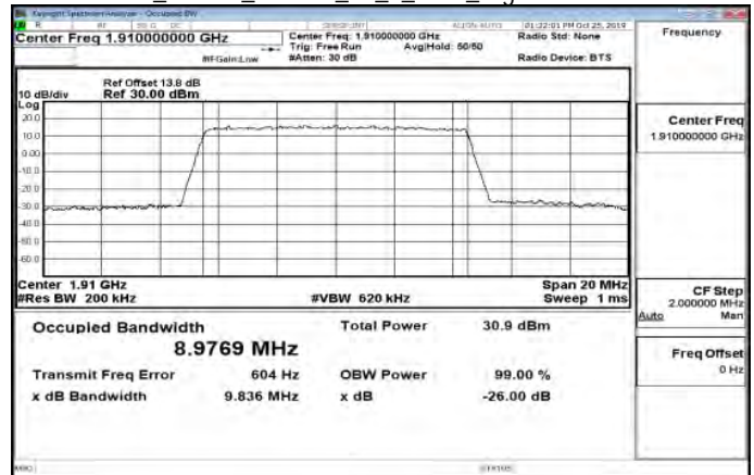
Band25_10MHz_64QAM_50_0_Main_HighCH26640-1910
