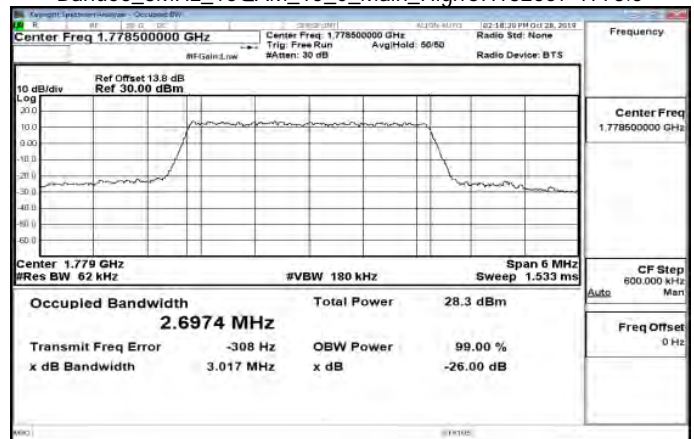
Band66_3MHz_16QAM_15_0_Main_HighCH132657-1778.5
