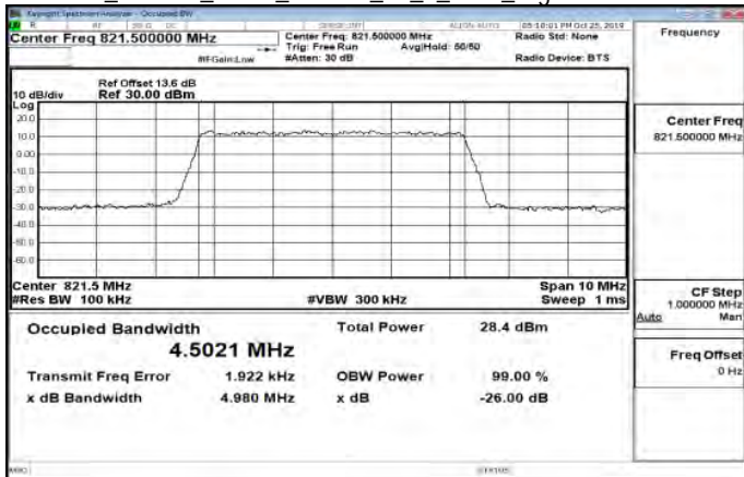
Band26_Part90s_5MHz_16QAM_25_0_Main_HighCH26765-821.5
