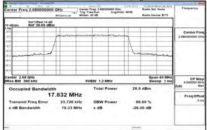
Band41_20MHz_16QAM_100_0_Main_HighCH41490-2680
