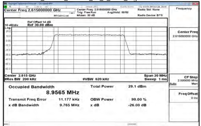
Band38_10MHz_16QAM_50_0_Main_HighCH38200-2615
