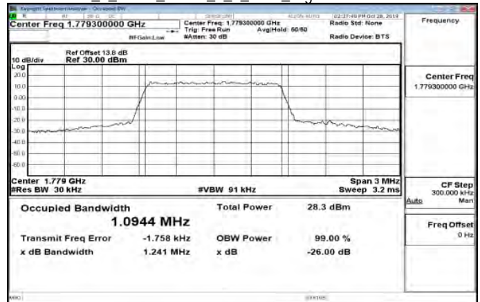
Band66_1_4MHz_QPSK_6_0_Main_HighCH132665-1779.3
