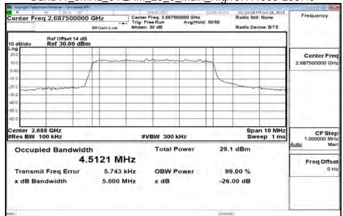
Band41_5MHz_64QAM_25_0_Main_HighCH41565-2687.5
