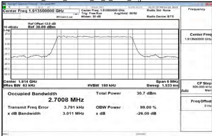
Band25_3MHz_16QAM_15_0_Main_HighCH26675-1913.5
