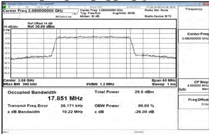
Band41_20MHz_64QAM_100_0_Main_HighCH41490-2680
