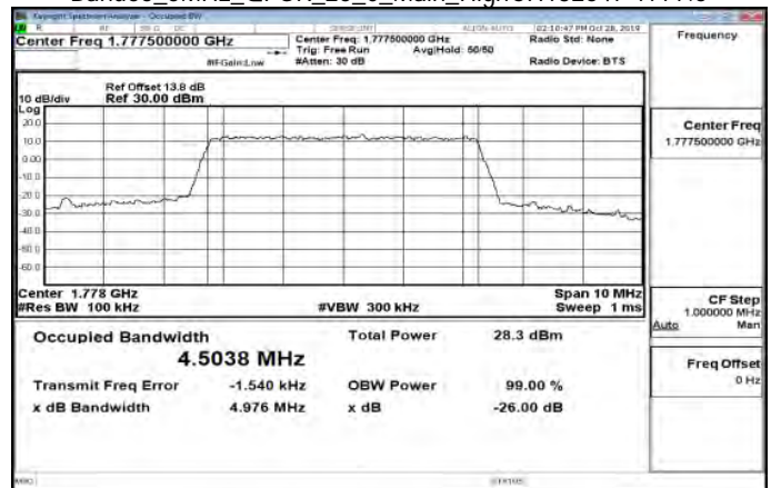
Band66_5MHz_QPSK_25_0_Main_HighCH132647-1777.5
