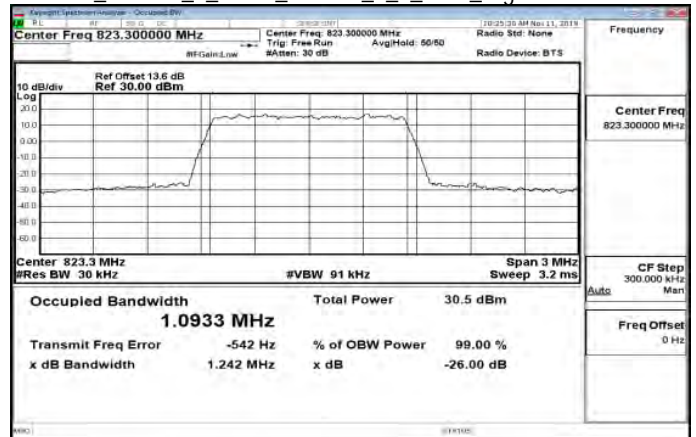
Band26_Part90s_1_4MHz_64QAM_6_0_Main_HighCH26783-823.3
