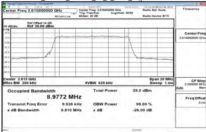
Band38_10MHz_64QAM_50_0_Main_HighCH38200-2615
