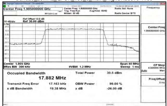
Band25_20MHz_QPSK_100_0_Main_HighCH26590-1905
