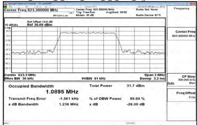
Band26_Part90s_1_4MHz_QPSK_6_0_Main_HighCH26783-823.3
