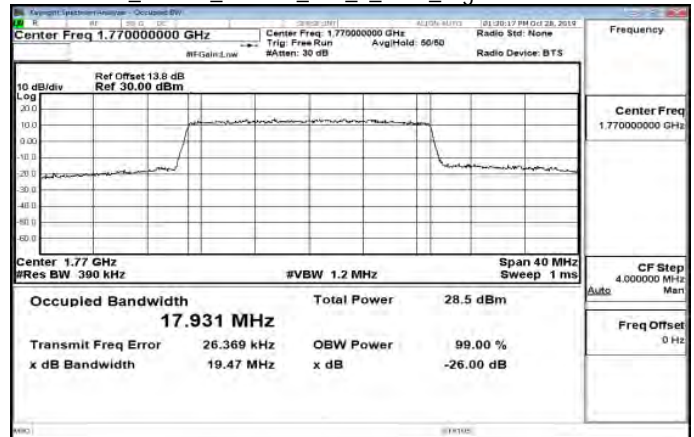
Band66_20MHz_16QAM_100_0_Main_HighCH132572-1770
