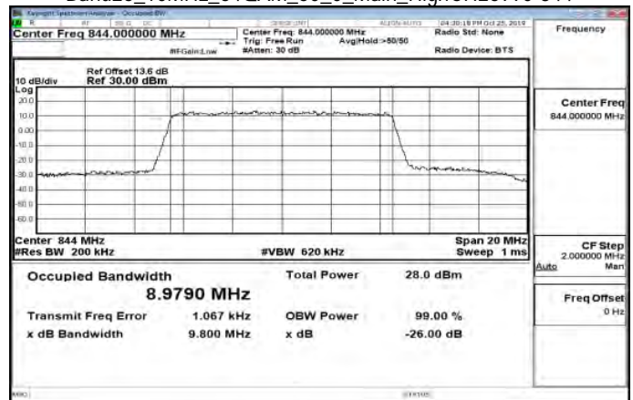
Band26_10MHz_64QAM_50_0_Main_HighCH26990-844
