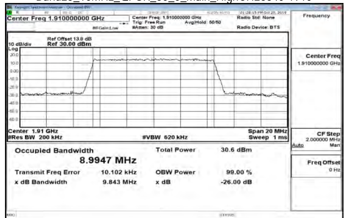
Band25_10MHz_QPSK_50_0_Main_HighCH26640-1910
