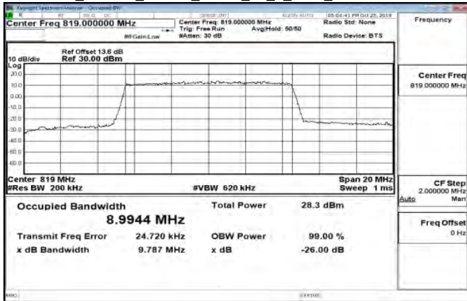
Band26_Part90s_10MHz_16QAM_50_0_Main_MidCH26740-819
