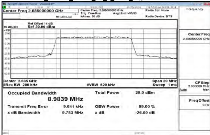
Band41_10MHz_QPSK_50_0_Main_HighCH41540-2685
