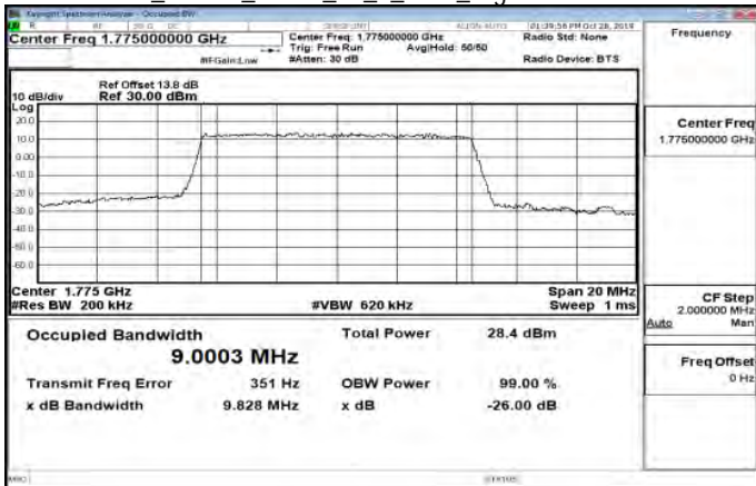
Band66_10MHz_QPSK_50_0_Main_HighCH132622-1775
