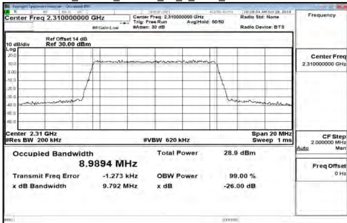
Band30_10MHz_64QAM_50_0_Main_MidCH27710-2310
