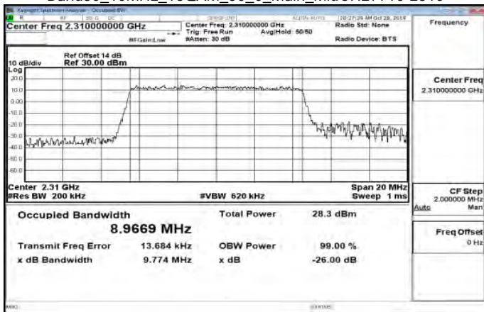
Band30_10MHz_64QAM_50_0_Main_MidCH27710-2310
