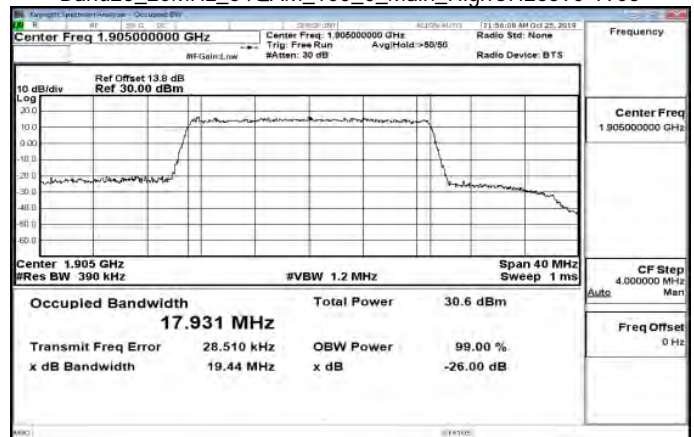
Band25_20MHz_64QAM_100_0_Main_HighCH26590-1905
