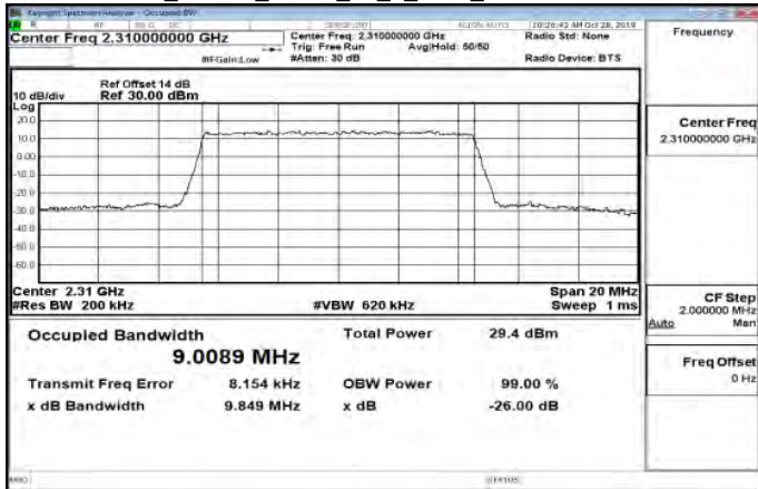
Band30_10MHz_16QAM_50_0_Main_MidCH27710-2310
