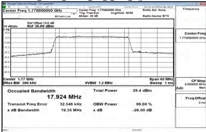
Band66_20MHz_64QAM_100_0_Main_HighCH132572-1770
