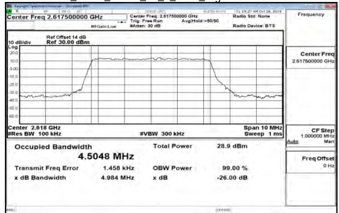
Band38_5MHz_QPSK_25_0_Main_HighCH38225-2617.5
