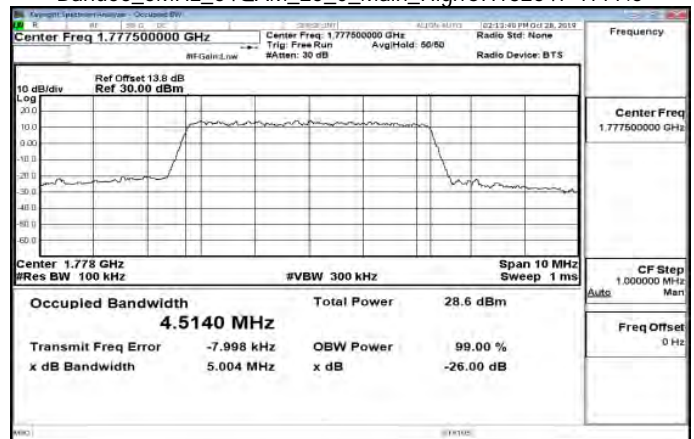
Band66_5MHz_64QAM_25_0_Main_HighCH132647-1777.5
