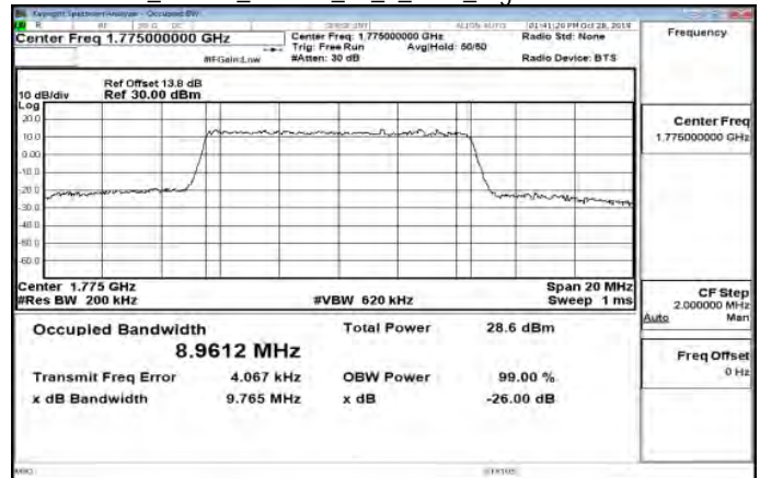
Band66_10MHz_16QAM_50_0_Main_HighCH132622-1775
