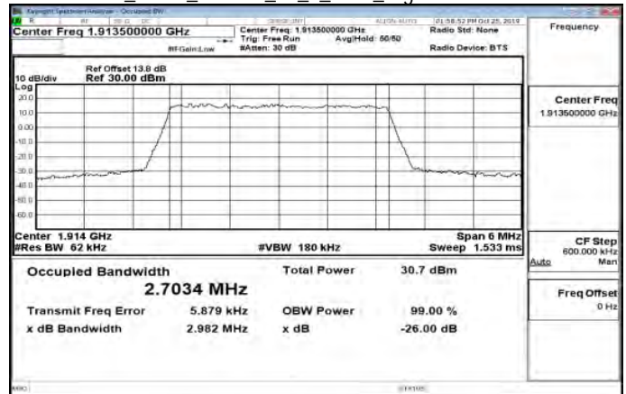
Band25_3MHz_64QAM_15_0_Main_HighCH26675-1913.5
