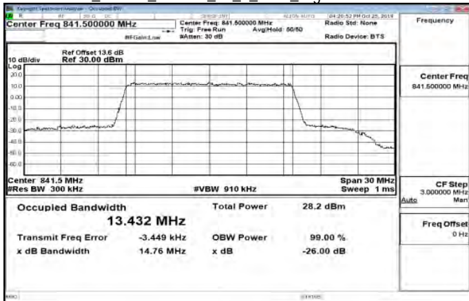
Band26_15MHz_64QAM_75_0_Main_HighCH26965-841.5
