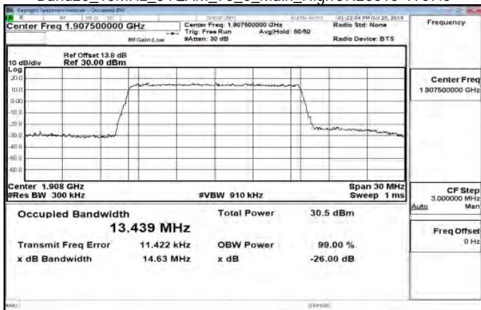
Band25_15MHz_64QAM_75_0_Main_HighCH26615-1907.5
