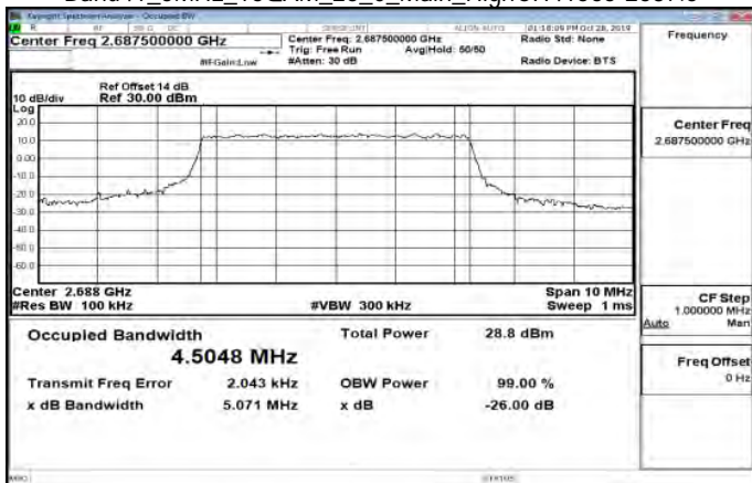
Band41_5MHz_16QAM_25_0_Main_HighCH41565-2687.5
