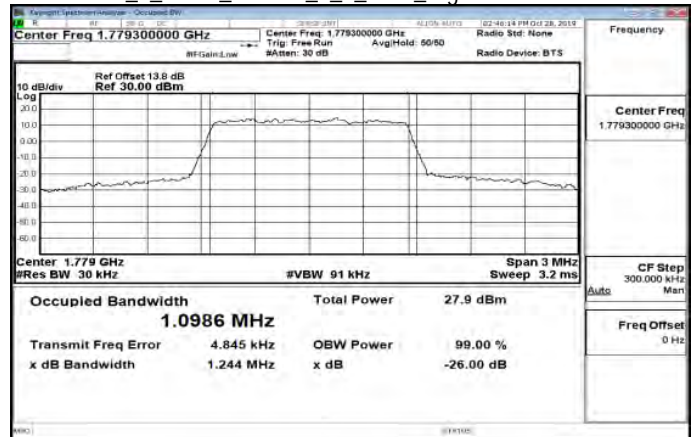
Band66_1_4MHz_64QAM_6_0_Main_HighCH132665-1779.3
