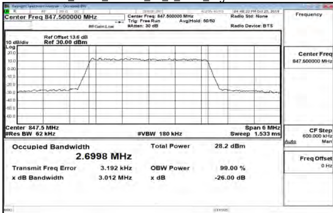
Band26_3MHz_16QAM_15_0_Main_HighCH27025-847.5
