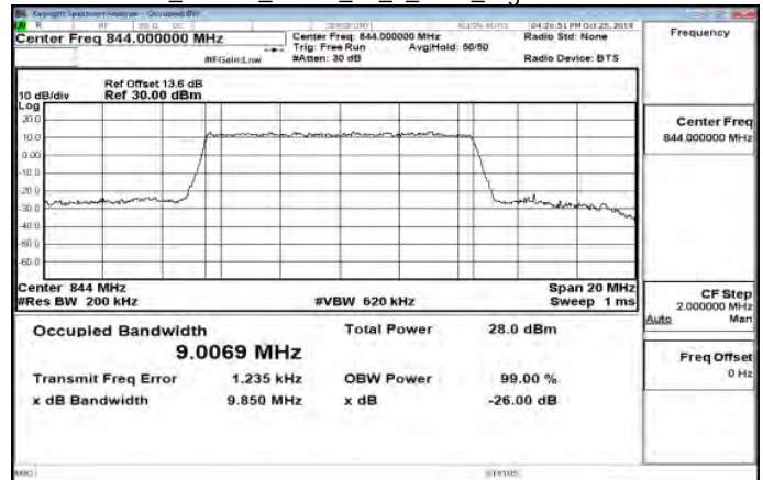
Band26_10MHz_QPSK_50_0_Main_HighCH26990-844
