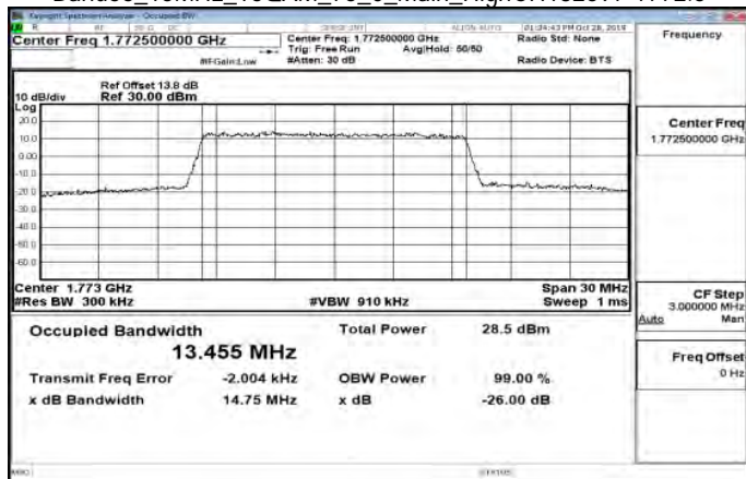
Band66_15MHz_16QAM_75_0_Main_HighCH132597-1772.5
