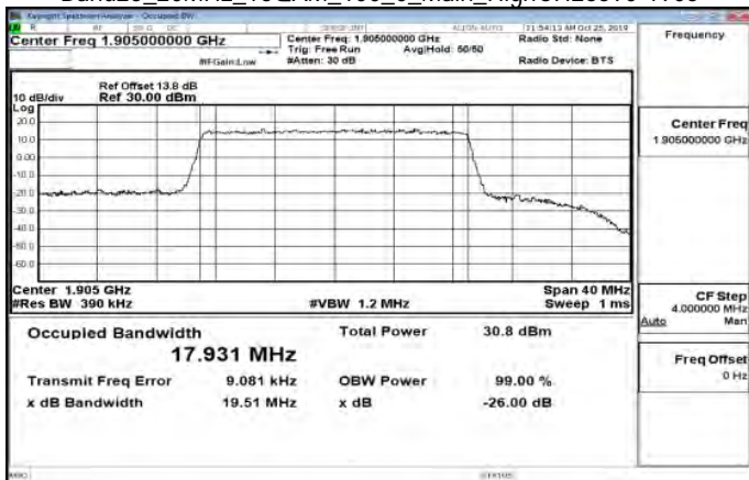
Band25_20MHz_16QAM_100_0_Main_HighCH26590-1905
