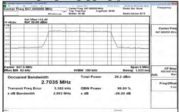
Band26_3MHz_64QAM_15_0_Main_HighCH27025-847.5
