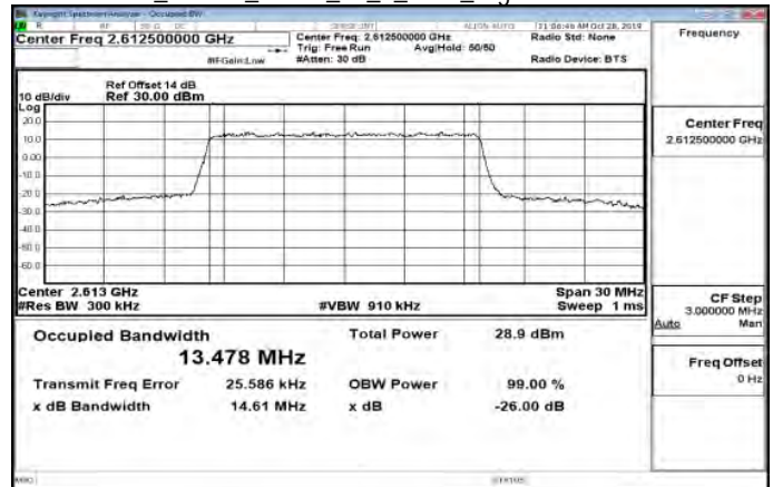
Band38_15MHz_QPSK_75_0_Main_HighCH38175-2612.5
