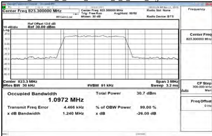
Band26_Part90s_1_4MHz_16QAM_6_0_Main_HighCH26783-823.3
