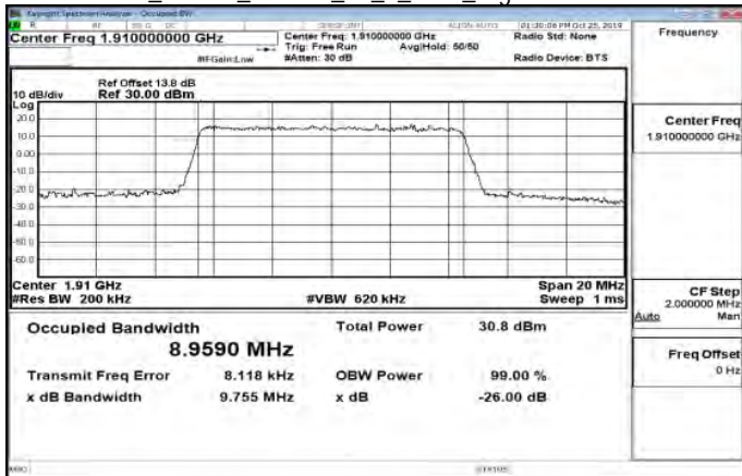
Band25_10MHz_16QAM_50_0_Main_HighCH26640-1910
