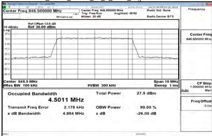
Band26_5MHz_QPSK_25_0_Main_HighCH27015-846.5
