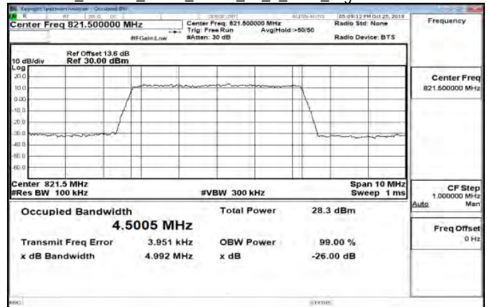
Band26_Part90s_5MHz_QPSK_25_0_Main_HighCH26765-821.5
