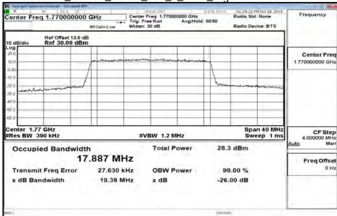
Band66_20MHz_QPSK_100_0_Main_HighCH132572-1770
