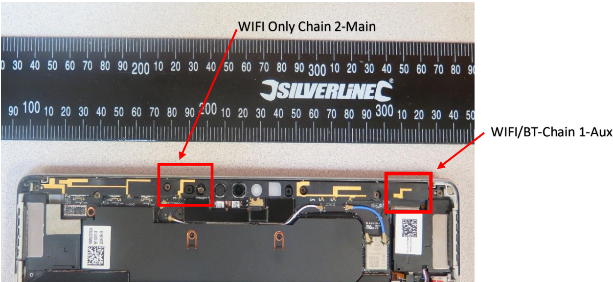
Figure 6 Wi-Fi Antenna- Close-up-Top View
