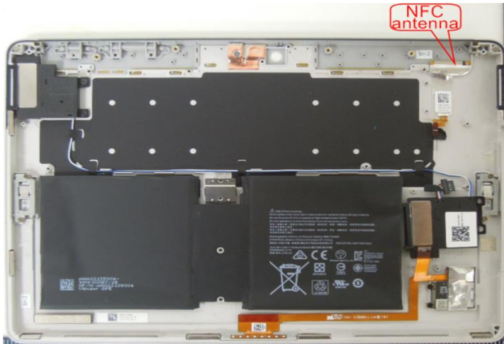
Figure 11 NFC Antenna- Close-up-Top View
