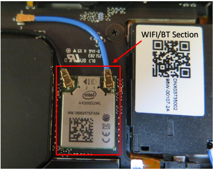
Figure 5 Close up Wi-Fi RF Module -Top View
