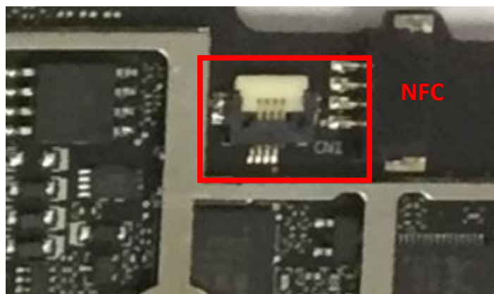
Figure 10 NFC Section- Close-up-Top View
