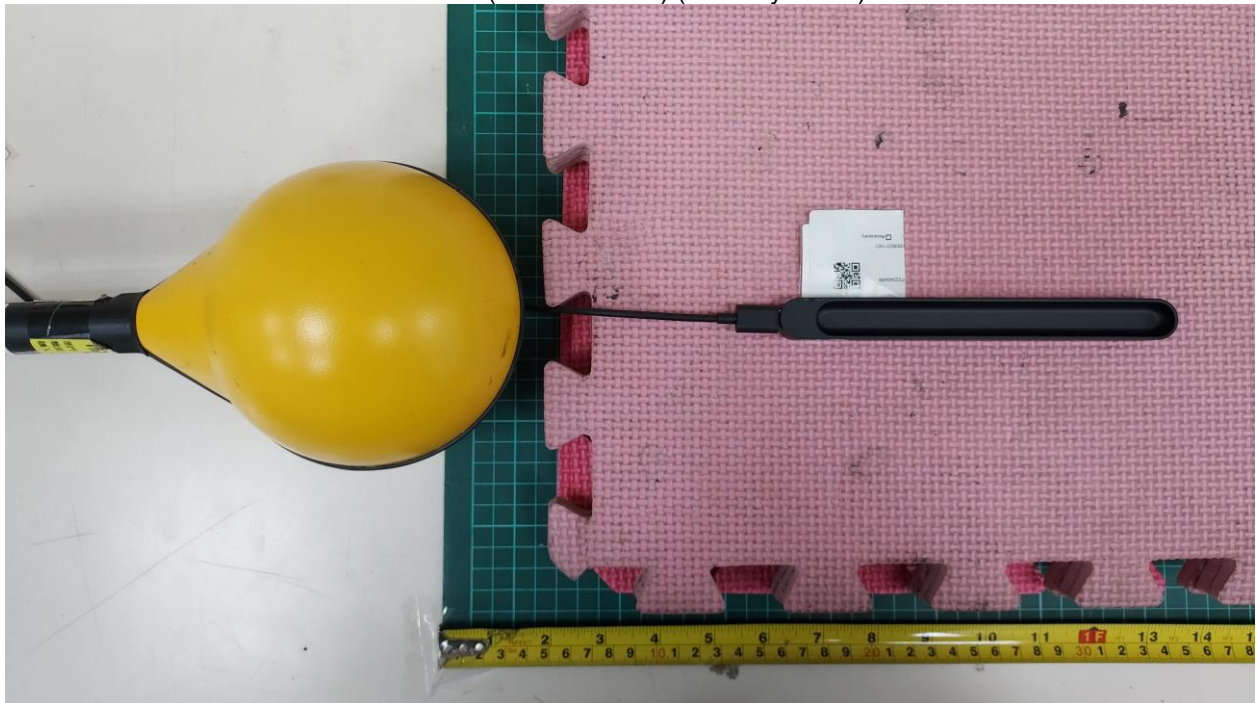
H-Field (Bottom: 15cm) (Standby Mode)
